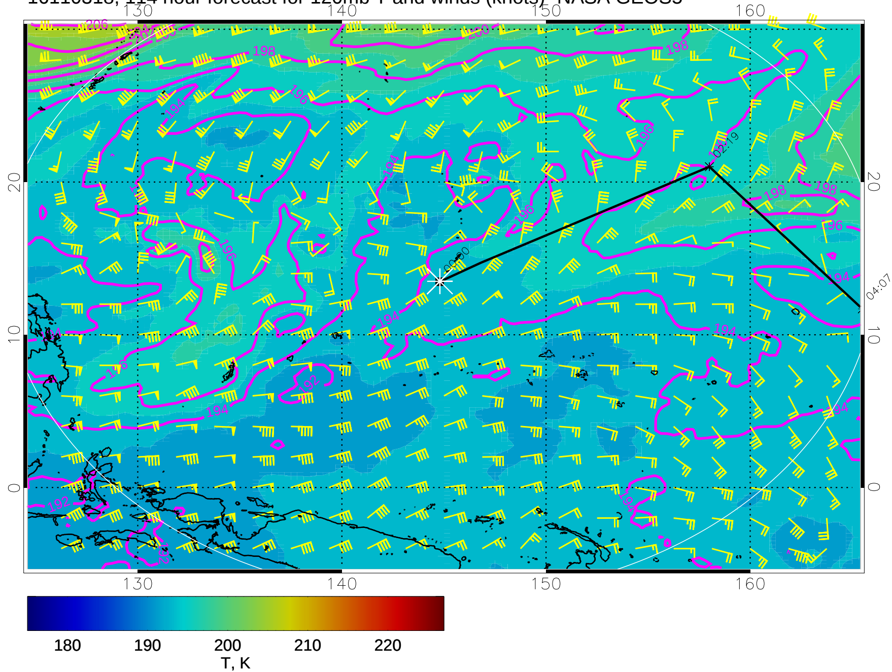
16110318, 114 hour forecast for 120mb T and winds (knots)- NASA GEOS5
