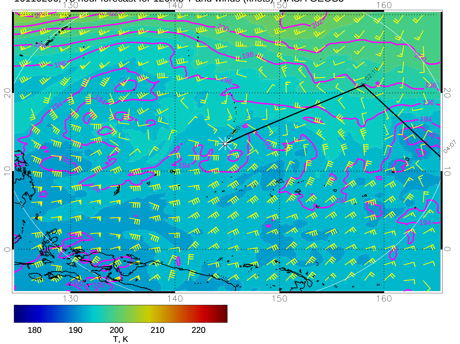
16110206, 78 hour forecast for 120mb T and winds (knots)- NASA GEOS5
