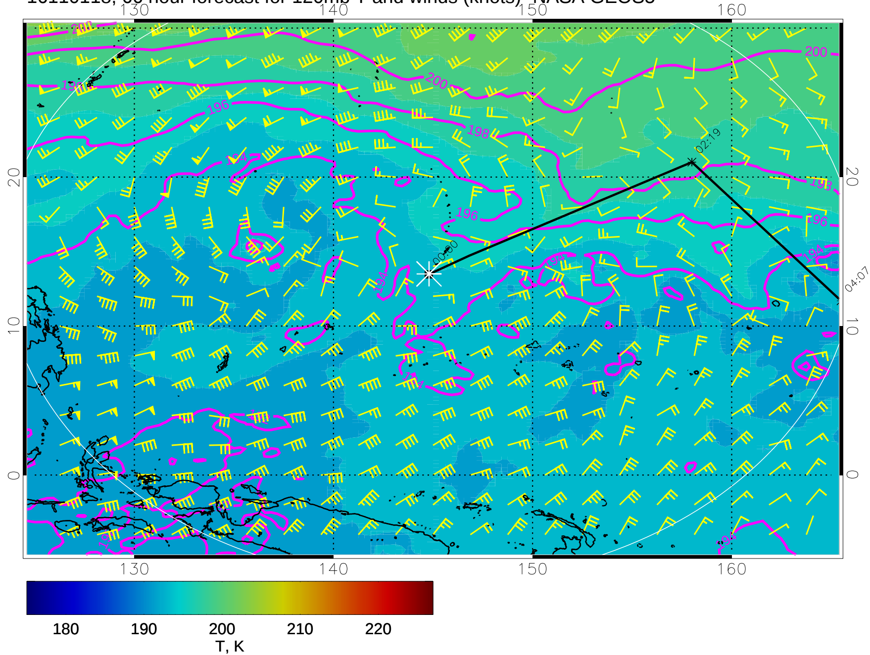
16110118, 66 hour forecast for 120mb T and winds (knots)- NASA GEOS5
