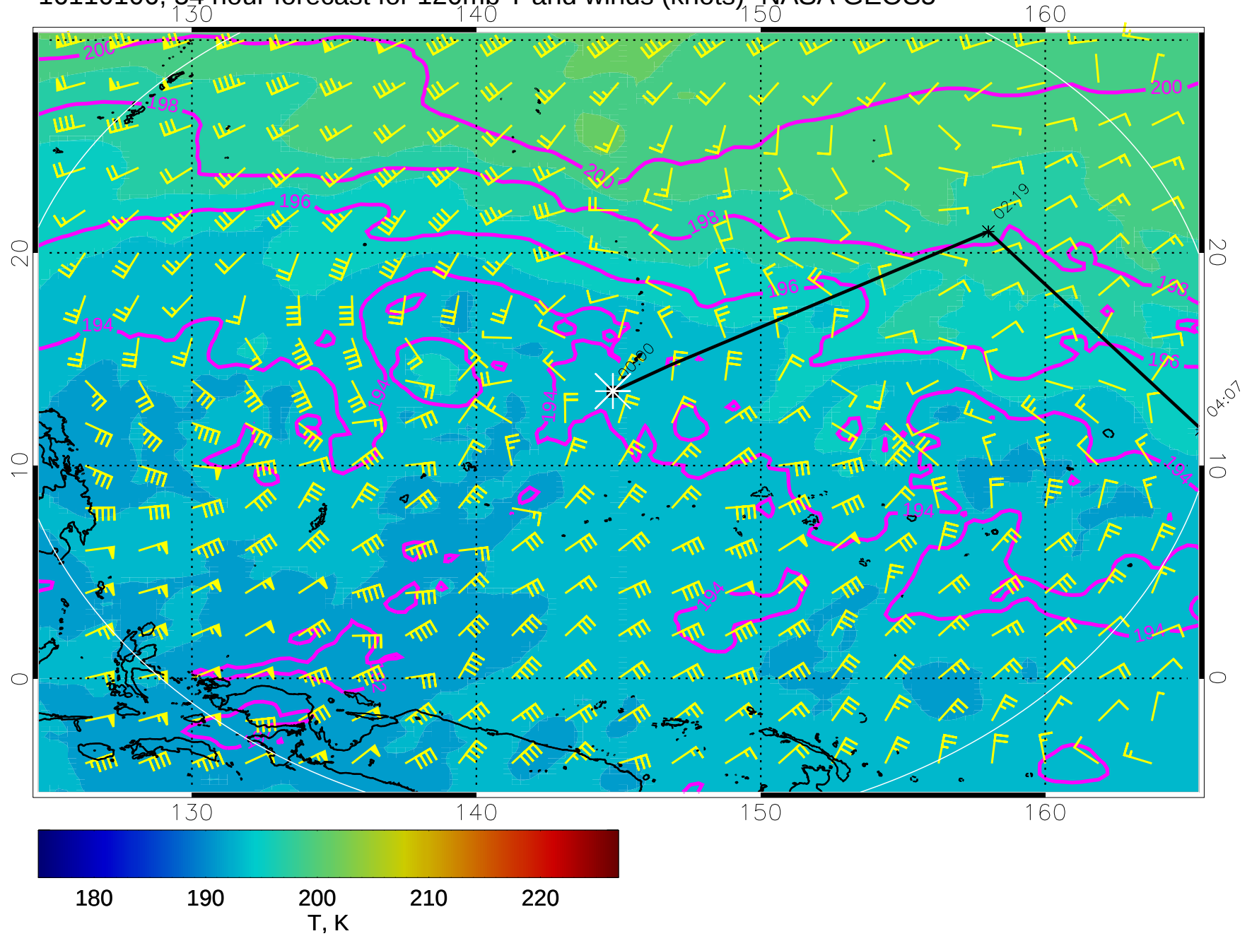
16110106, 54 hour forecast for 120mb T and winds (knots)- NASA GEOS5
