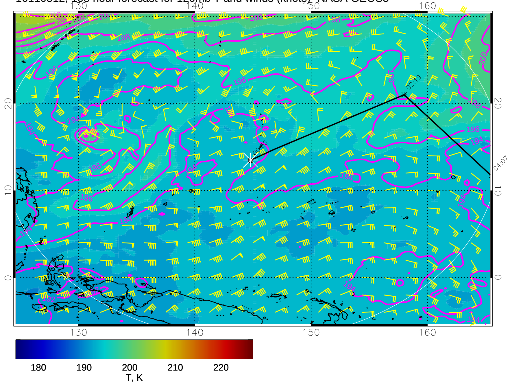
16110312, 108 hour forecast for 120mb T and winds (knots)- NASA GEOS5
