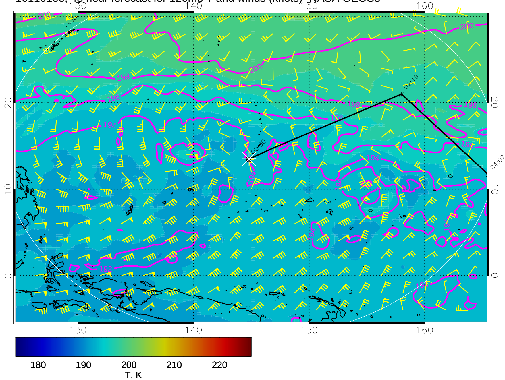
16110100, 48 hour forecast for 120mb T and winds (knots)- NASA GEOS5
