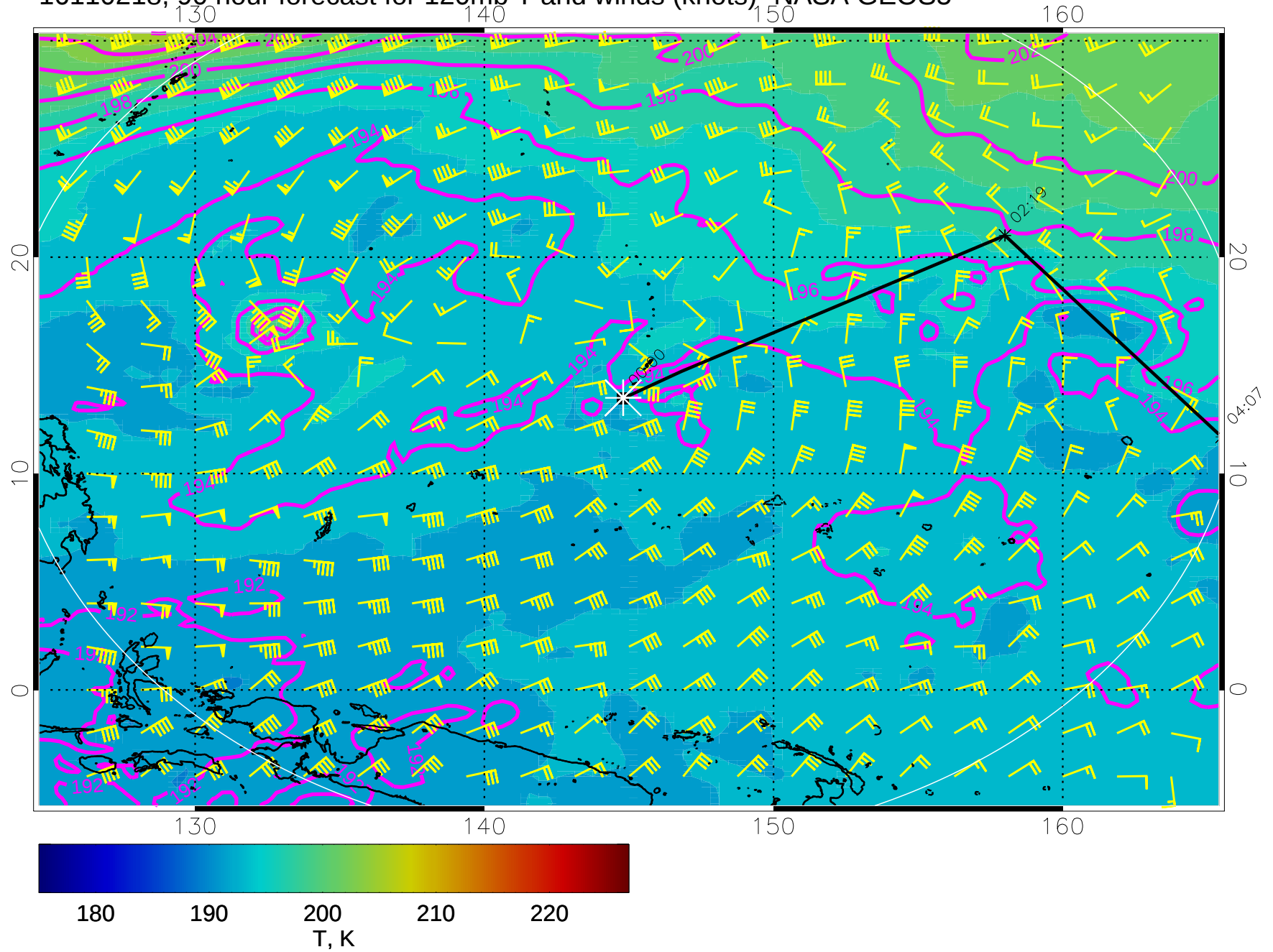
16110218, 90 hour forecast for 120mb T and winds (knots)- NASA GEOS5
