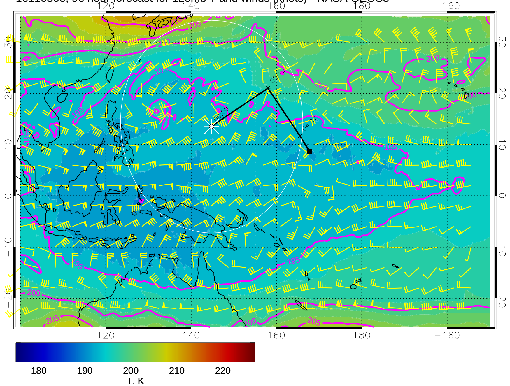
16110300, 96 hour forecast for 120mb T and winds (knots) - NASA GEOS5
