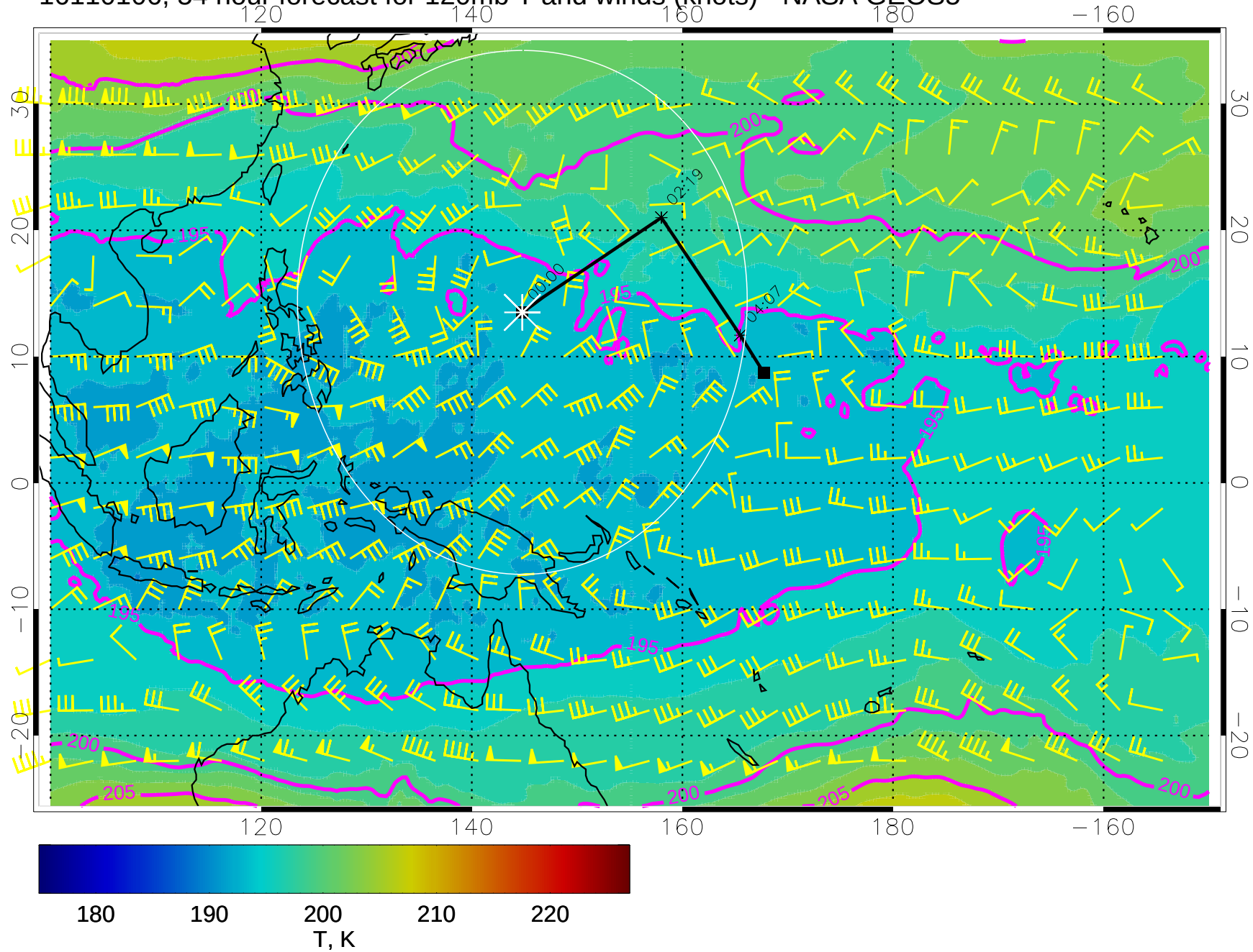
16110106, 54 hour forecast for 120mb T and winds (knots) - NASA GEOS5
