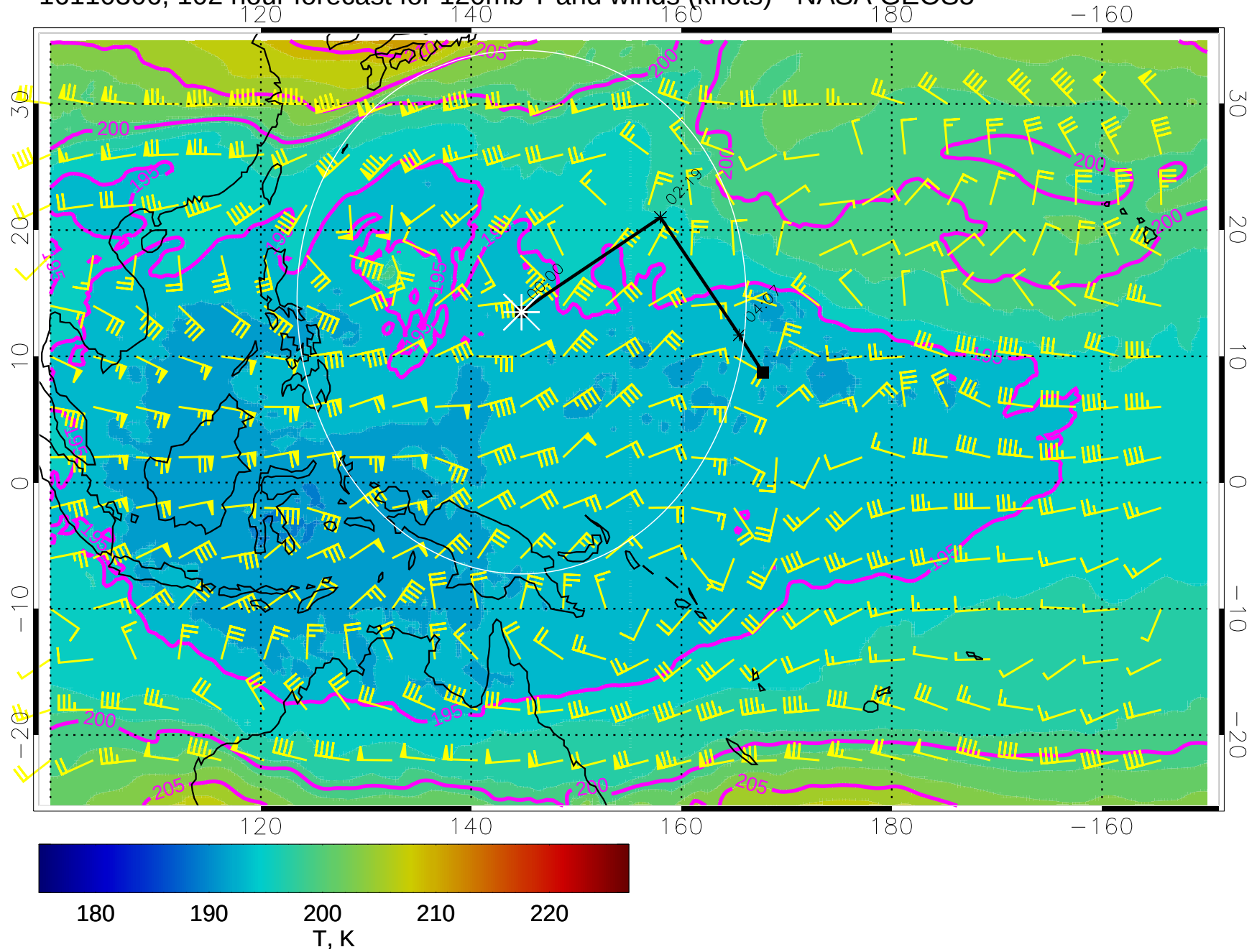
16110306, 102 hour forecast for 120mb T and winds (knots) - NASA GEOS5
