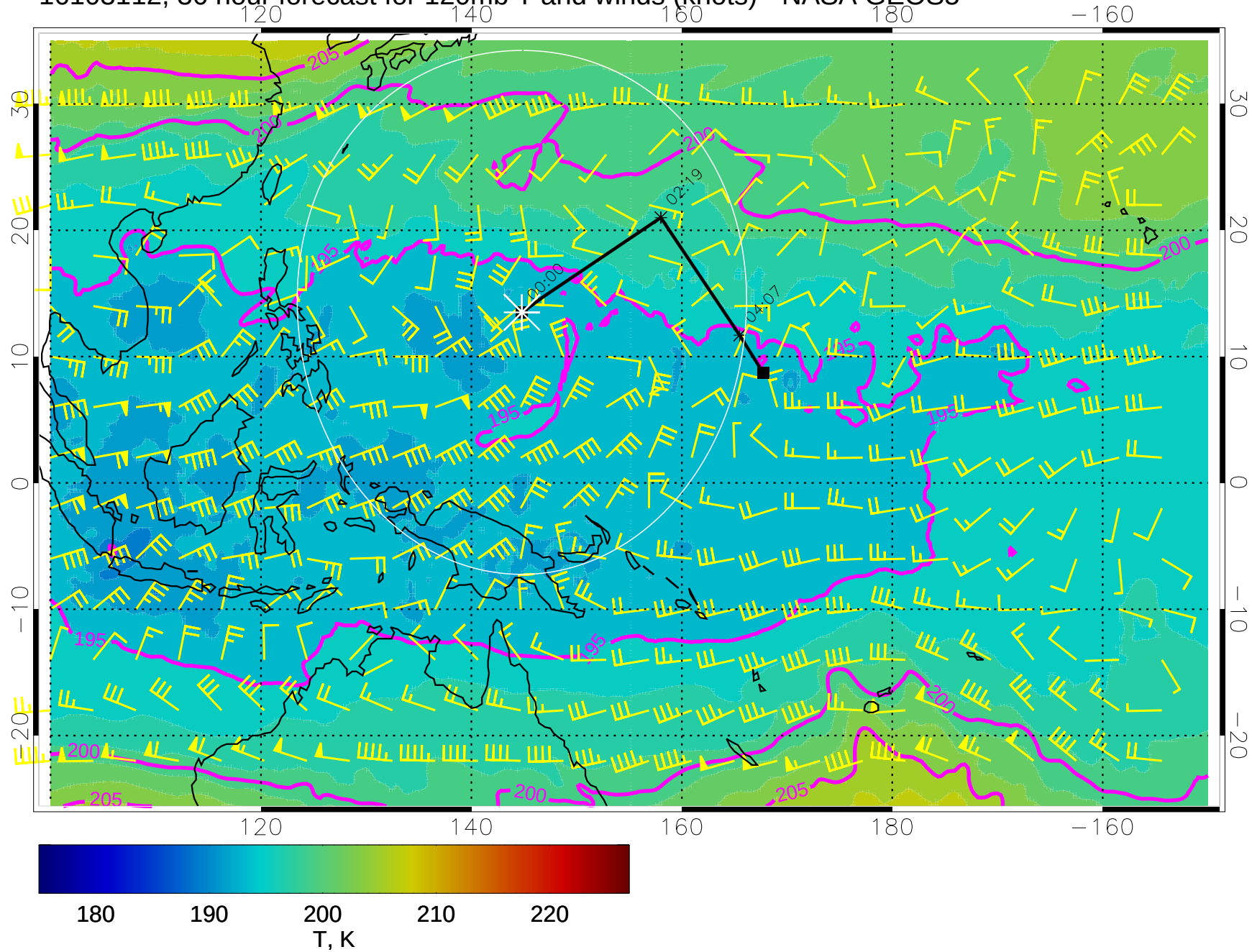
16103112, 36 hour forecast for 120mb T and winds (knots) - NASA GEOS5
