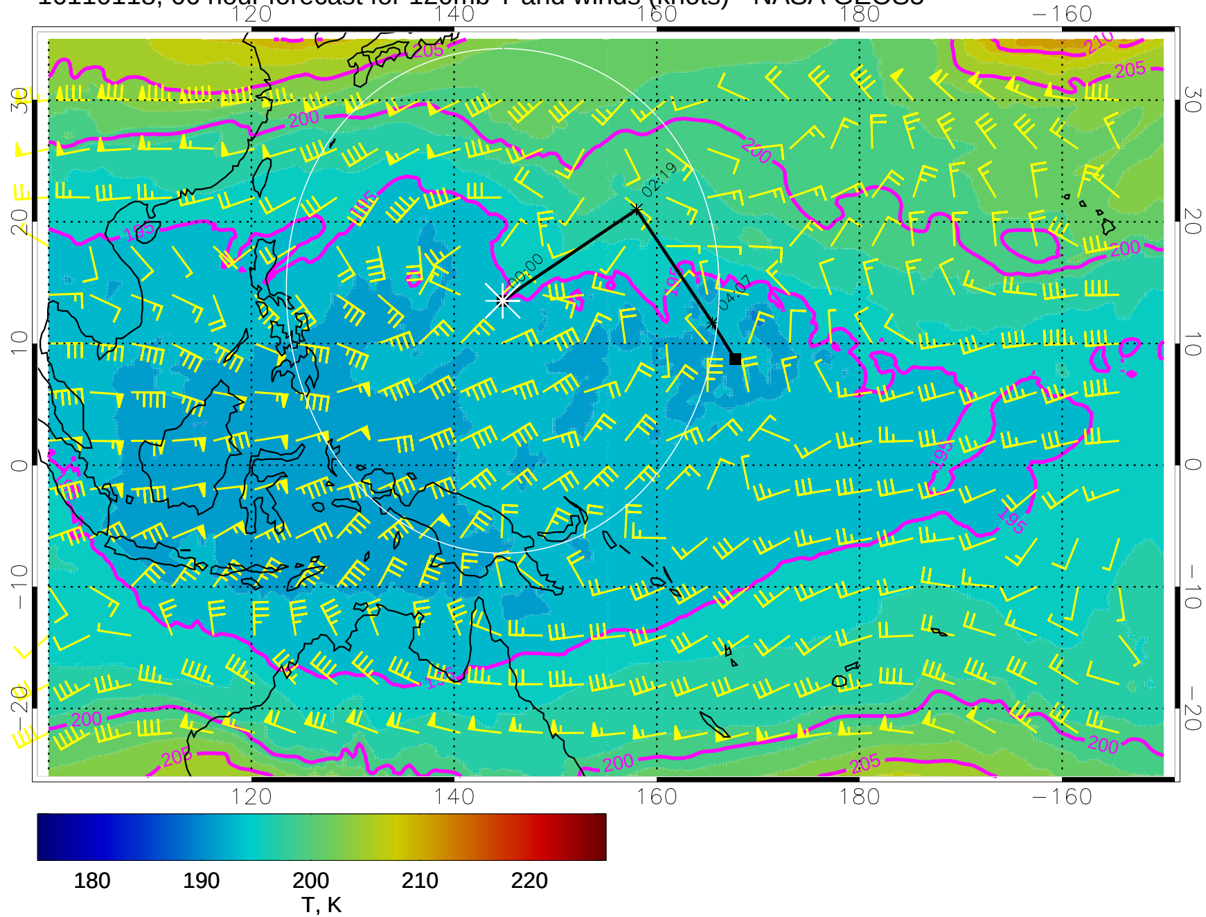
16110118, 66 hour forecast for 120mb T and winds (knots) - NASA GEOS5
