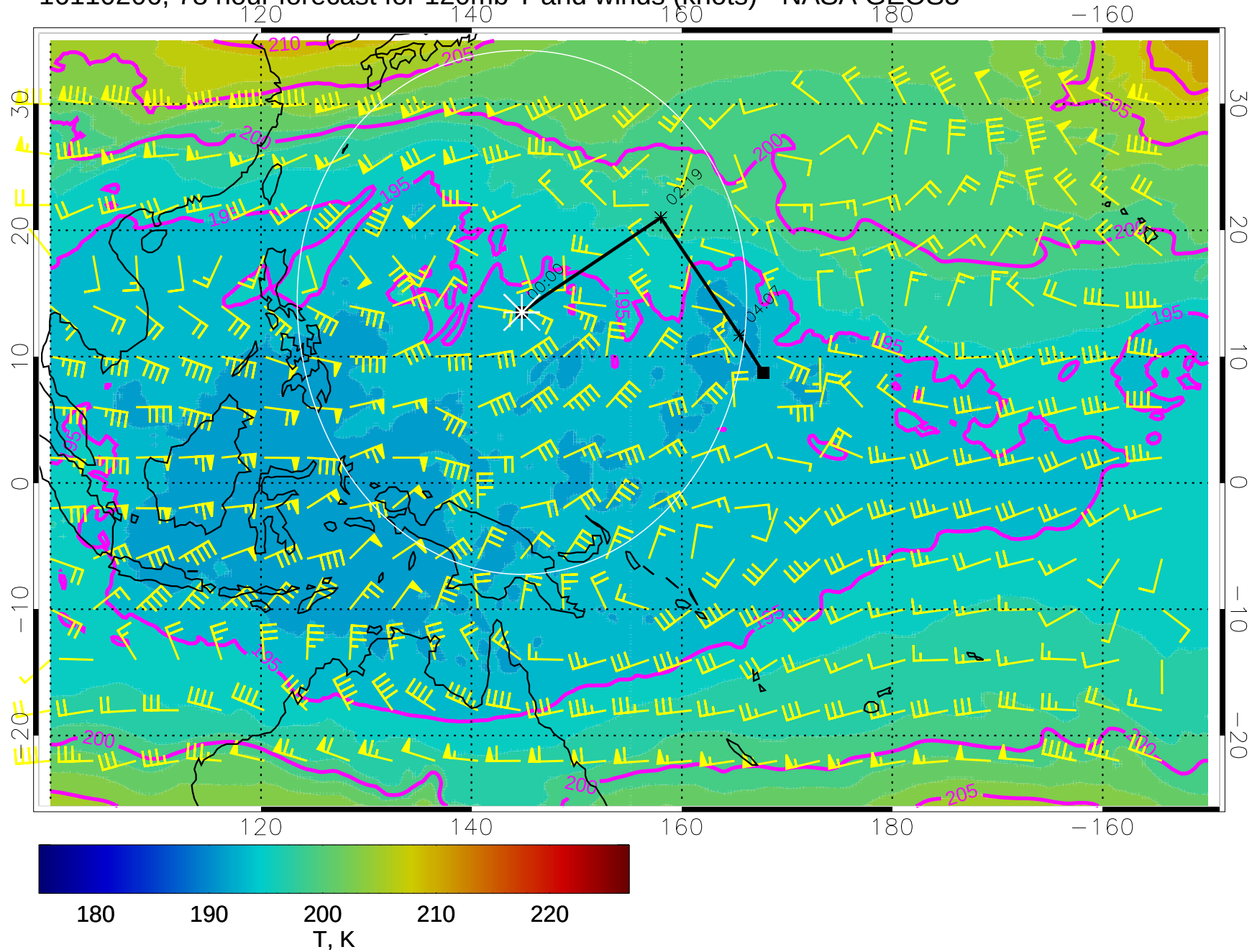
16110206, 78 hour forecast for 120mb T and winds (knots) - NASA GEOS5
