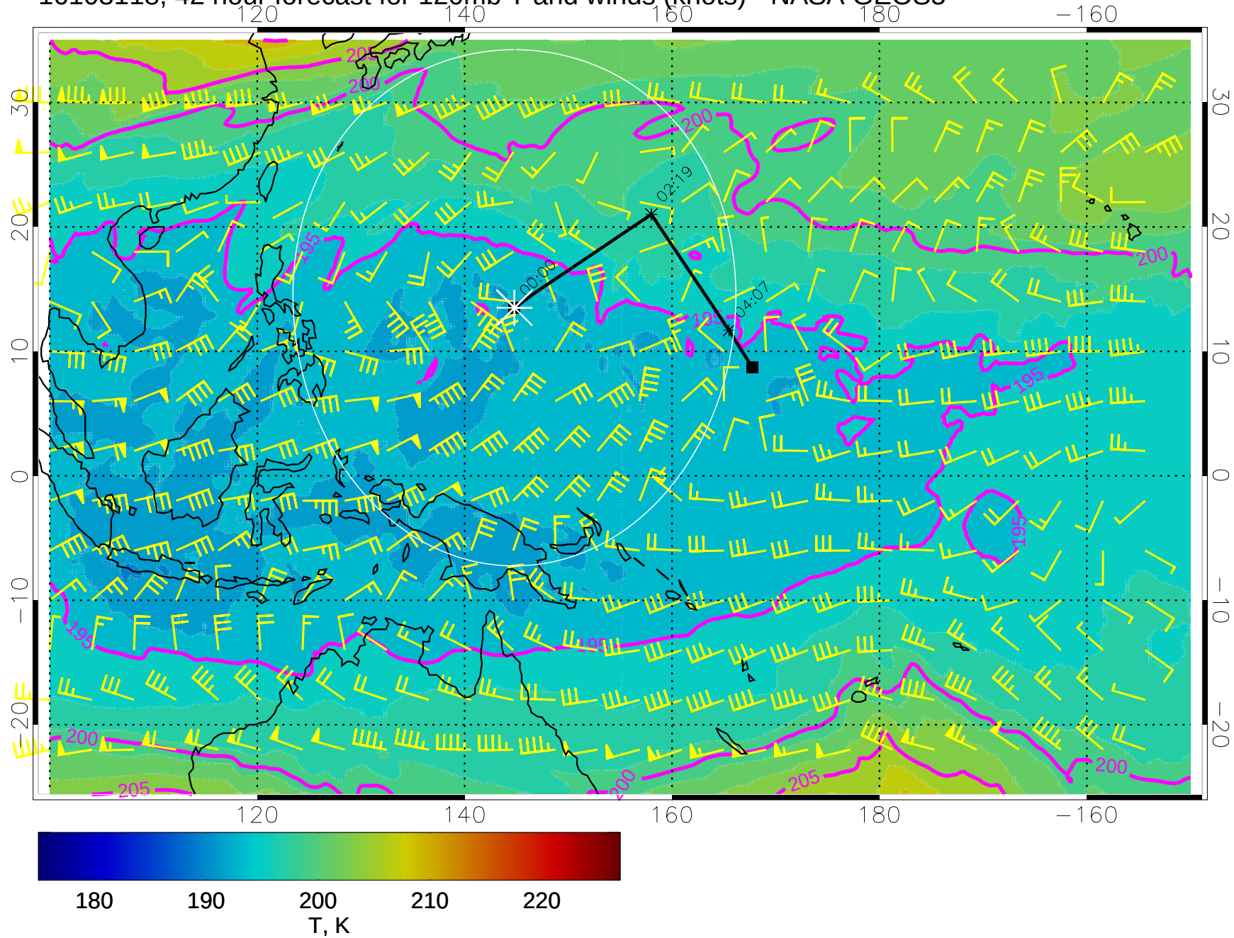
16103118, 42 hour forecast for 120mb T and winds (knots) - NASA GEOS5
