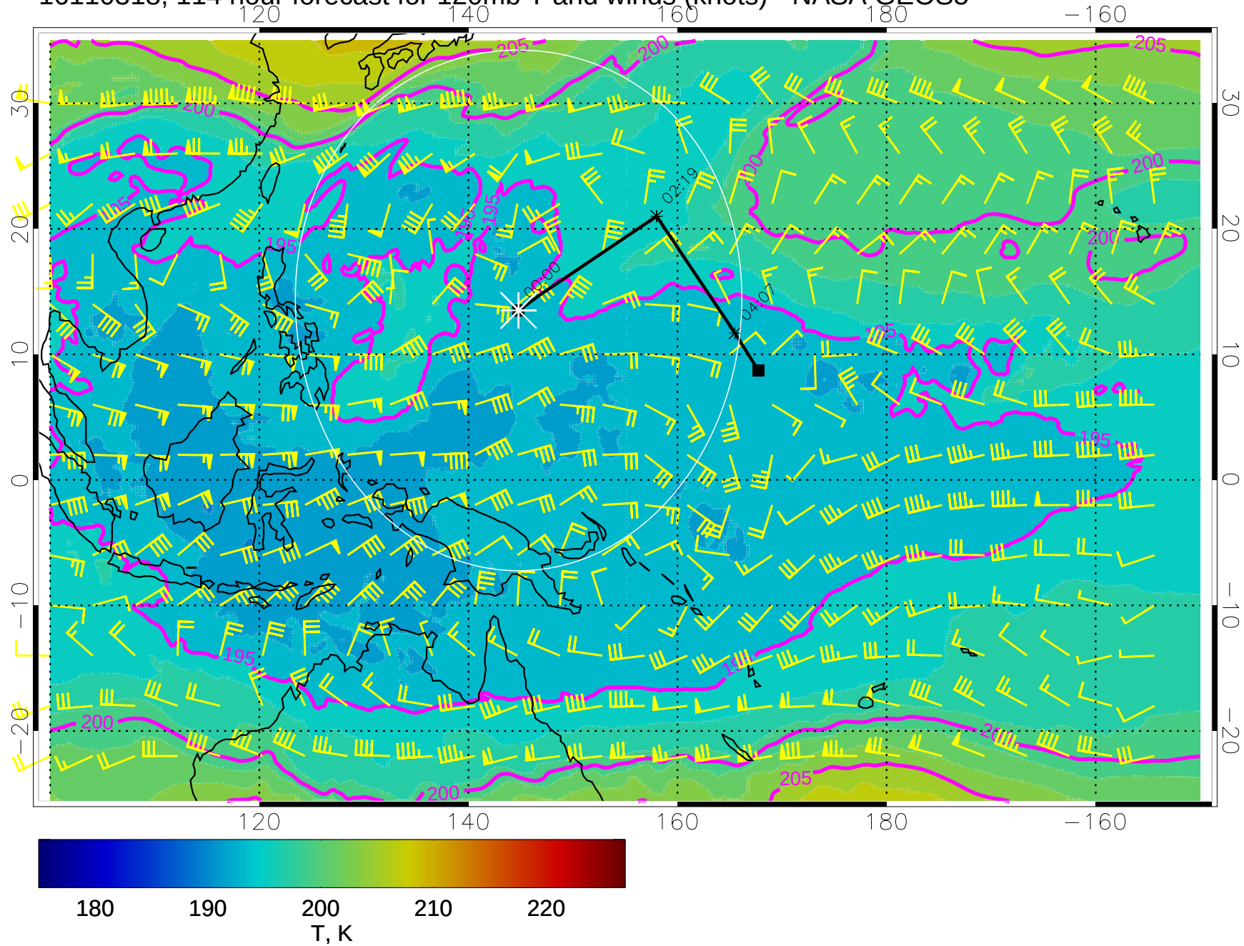
16110318, 114 hour forecast for 120mb T and winds (knots) - NASA GEOS5
