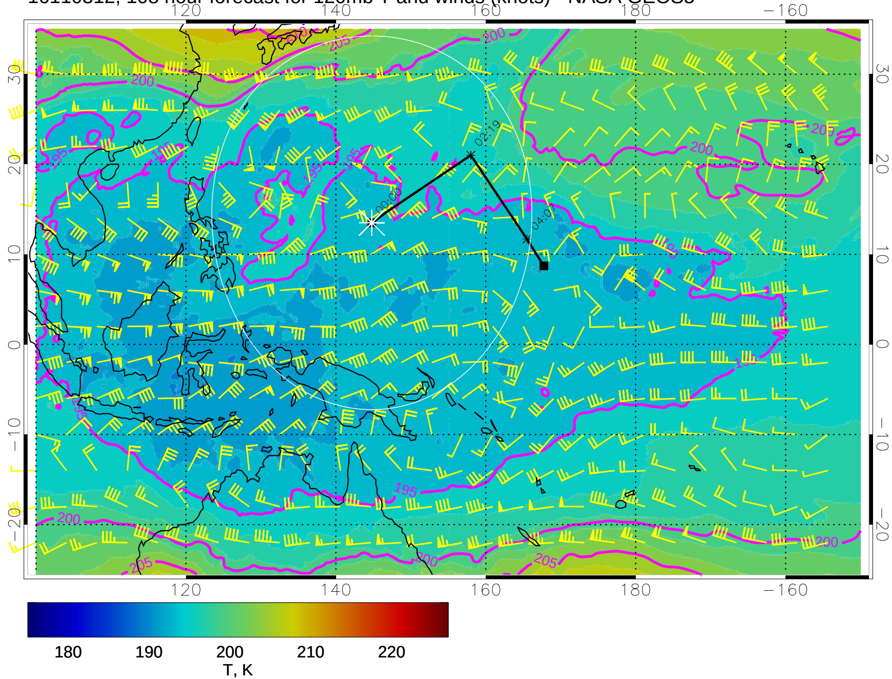
16110312, 108 hour forecast for 120mb T and winds (knots) - NASA GEOS5
