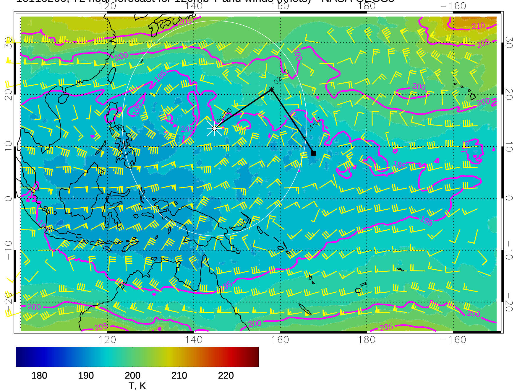
16110200, 72 hour forecast for 120mb T and winds (knots) - NASA GEOS5
