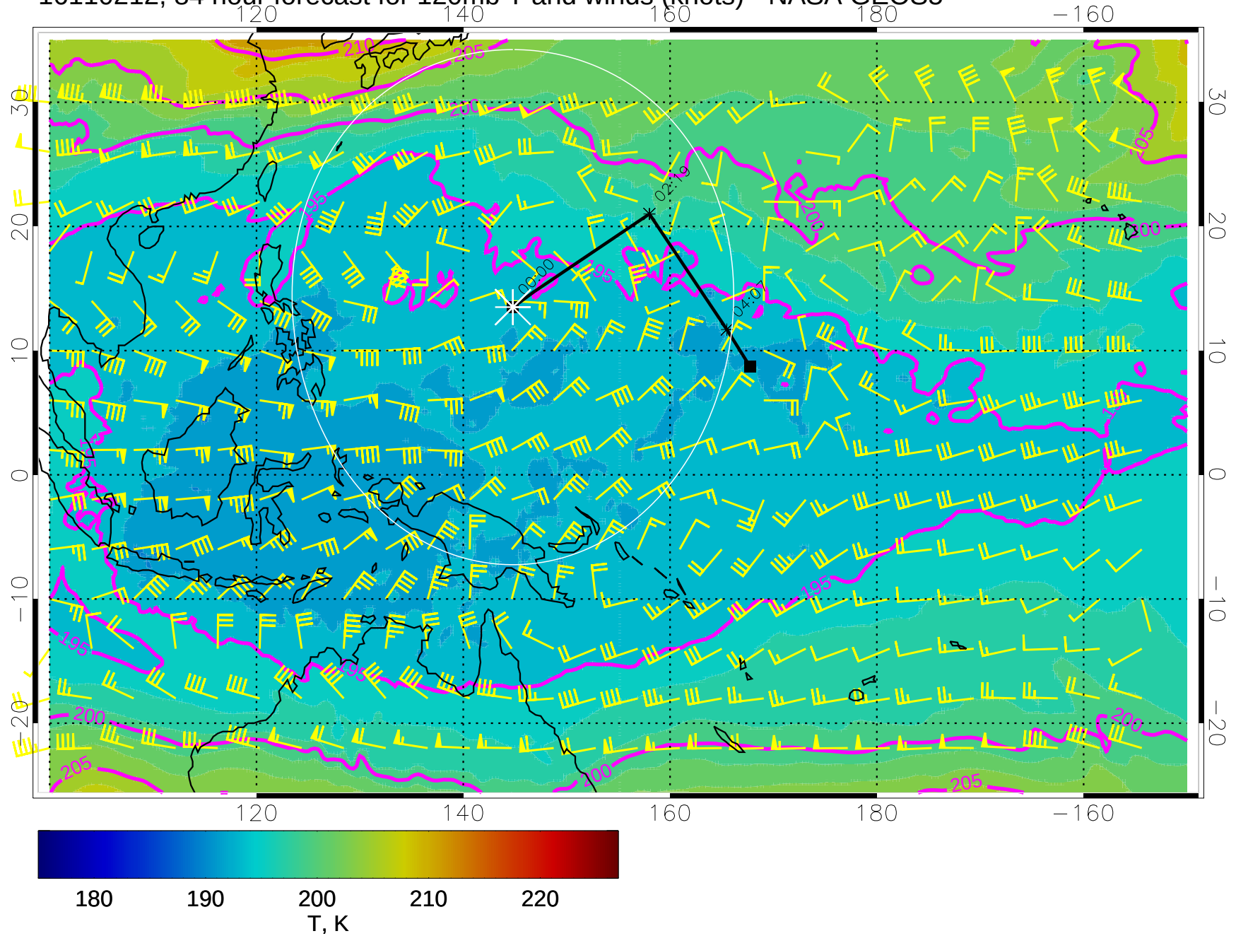
16110212, 84 hour forecast for 120mb T and winds (knots) - NASA GEOS5
