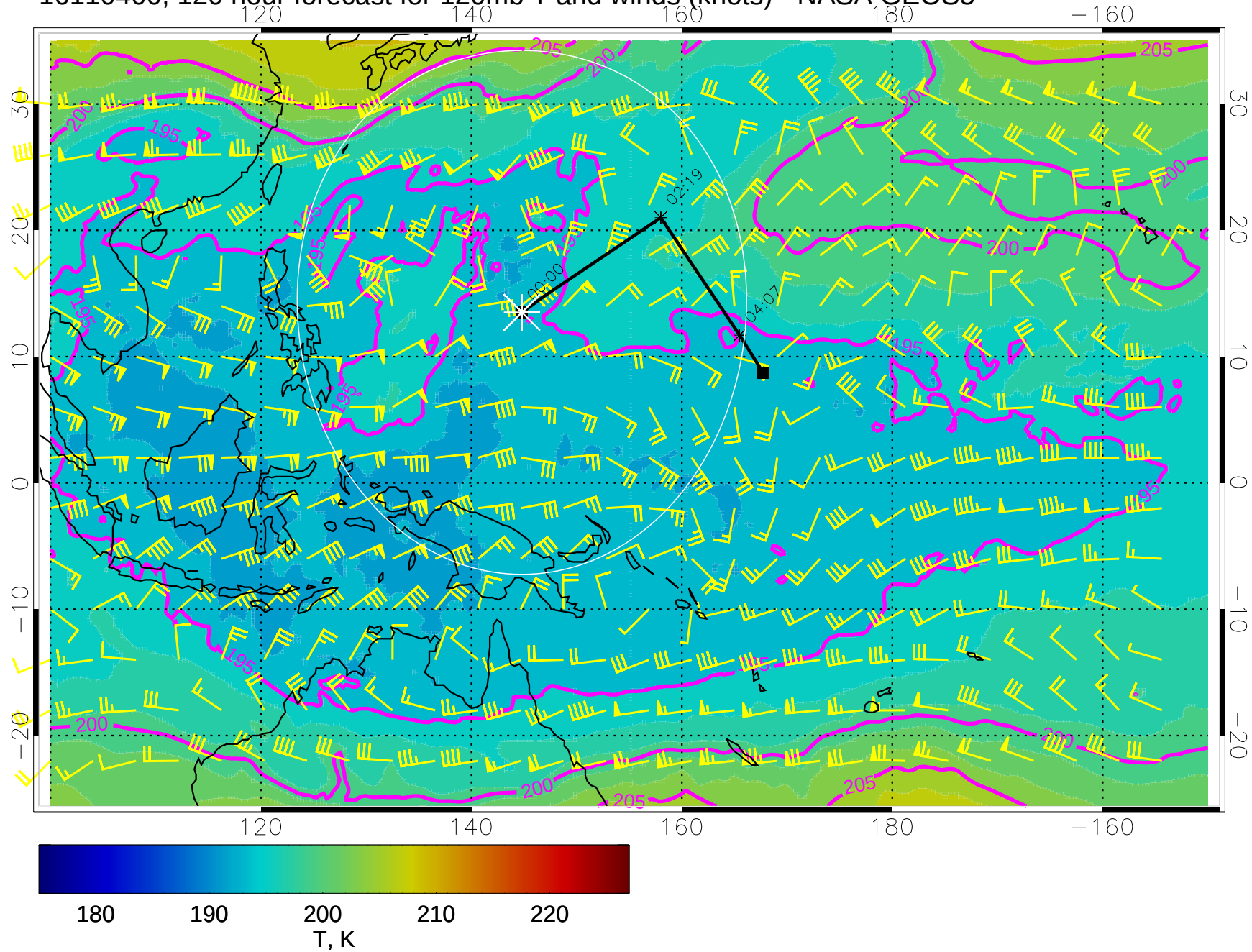
16110400, 120 hour forecast for 120mb T and winds (knots) - NASA GEOS5
