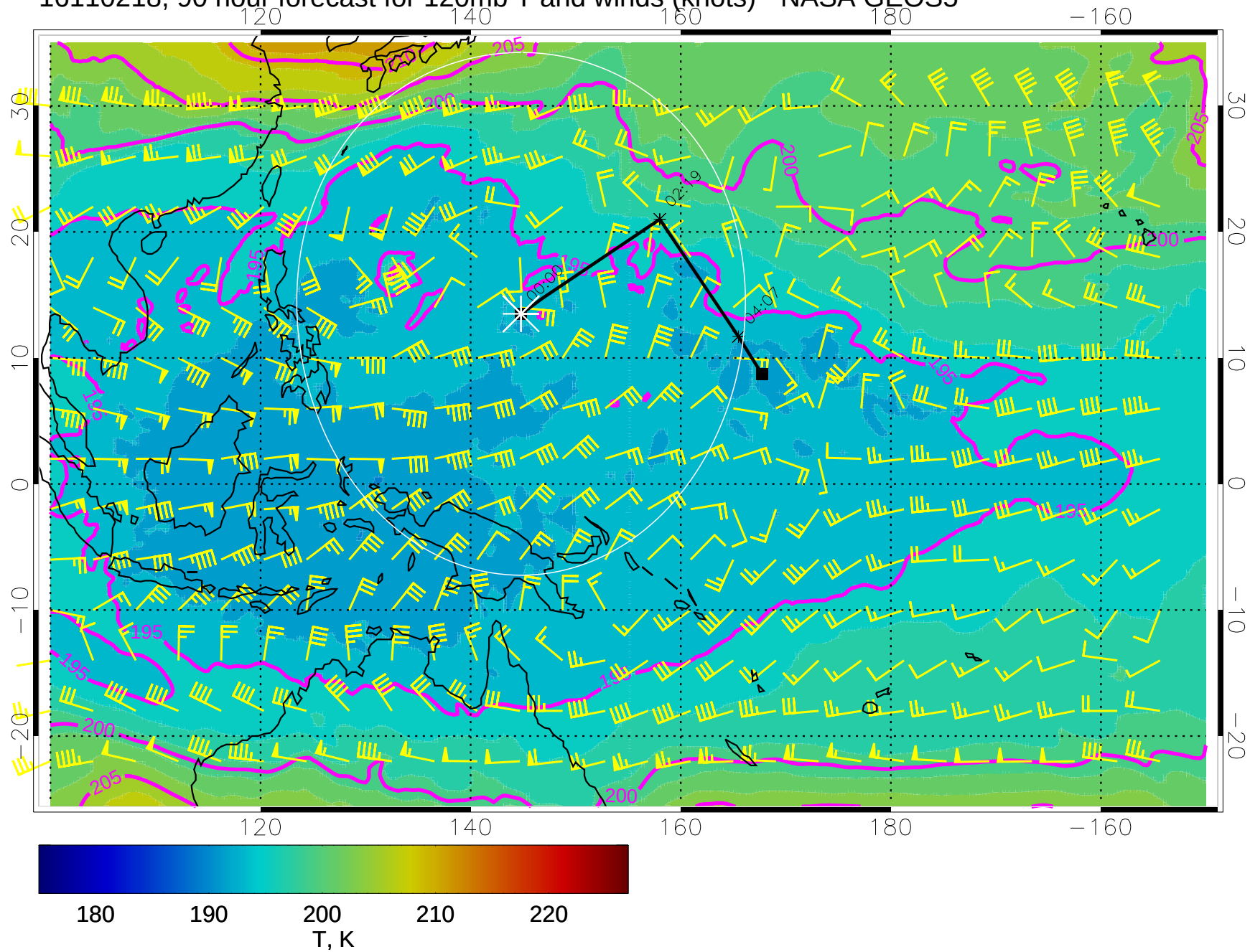
16110218, 90 hour forecast for 120mb T and winds (knots) - NASA GEOS5
