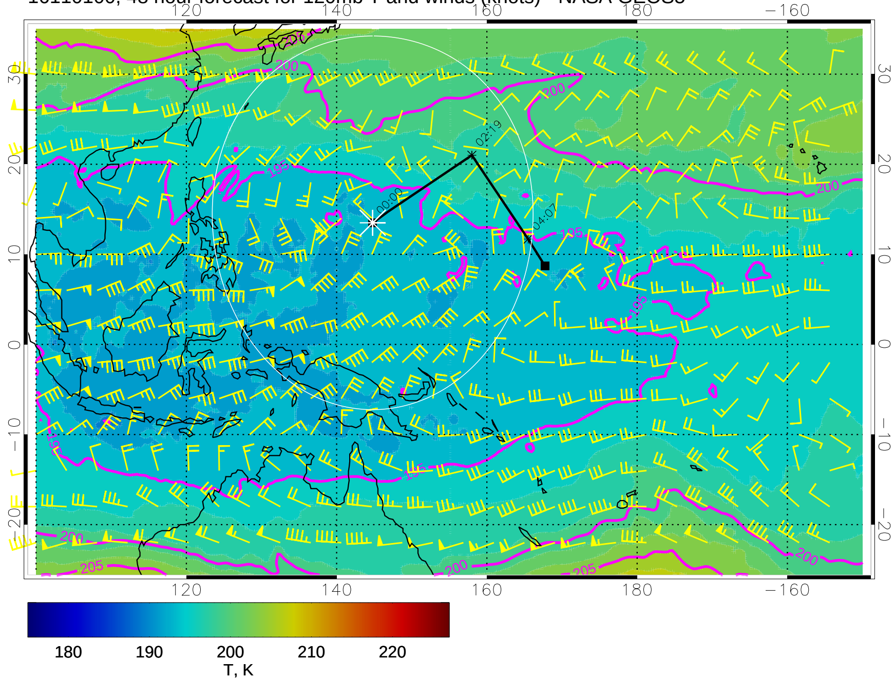
16110100, 48 hour forecast for 120mb T and winds (knots) - NASA GEOS5
