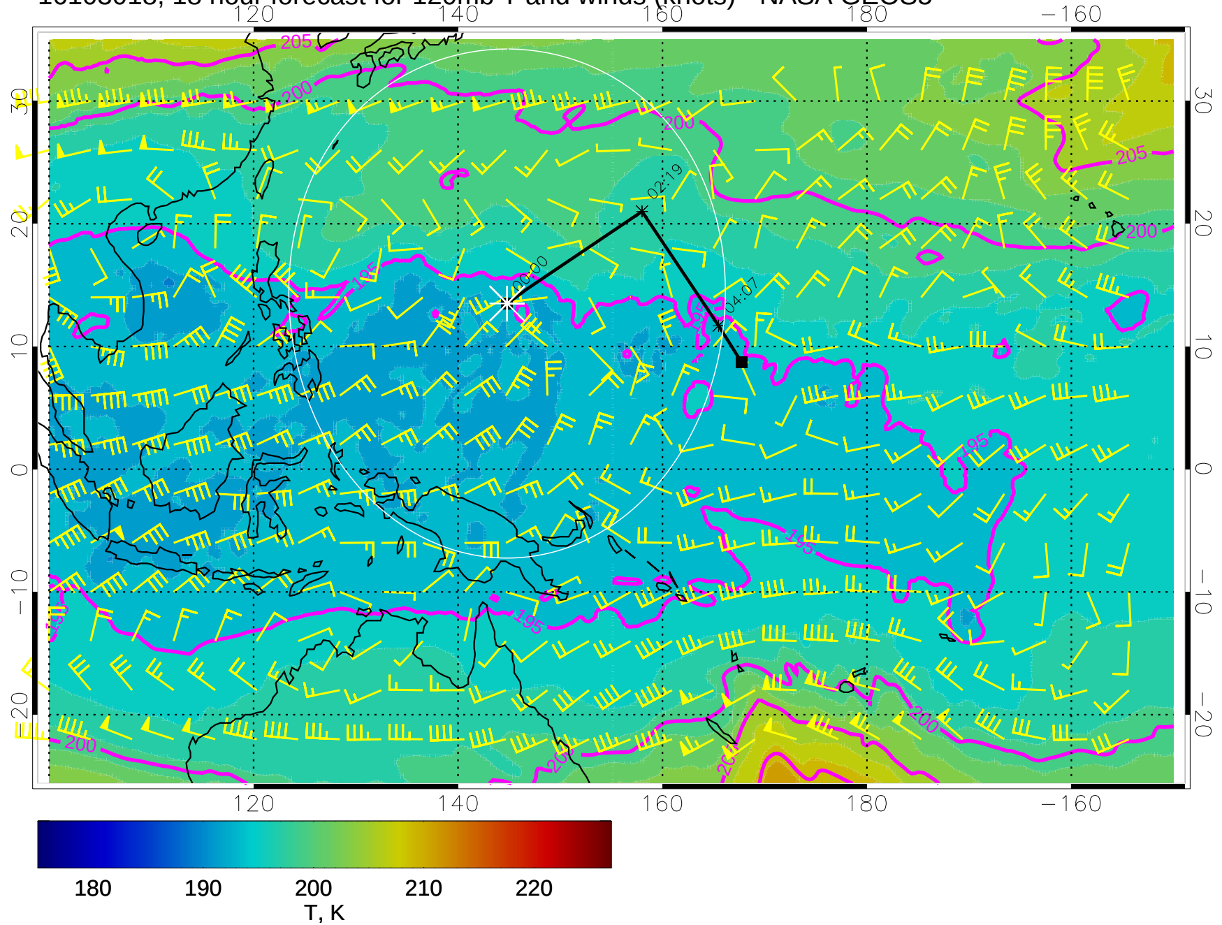
16103018, 18 hour forecast for 120mb T and winds (knots) - NASA GEOS5
