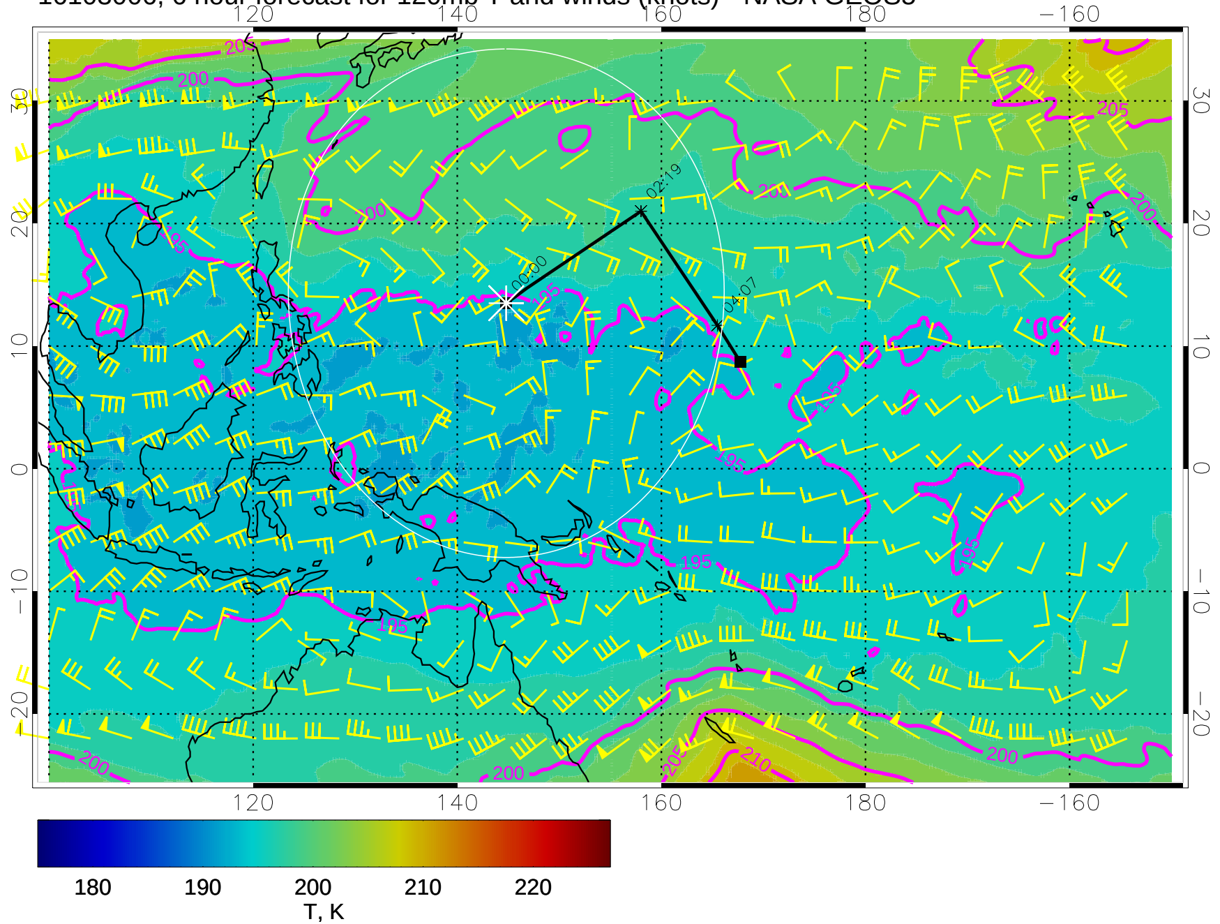
16103006, 6 hour forecast for 120mb T and winds (knots) - NASA GEOS5
