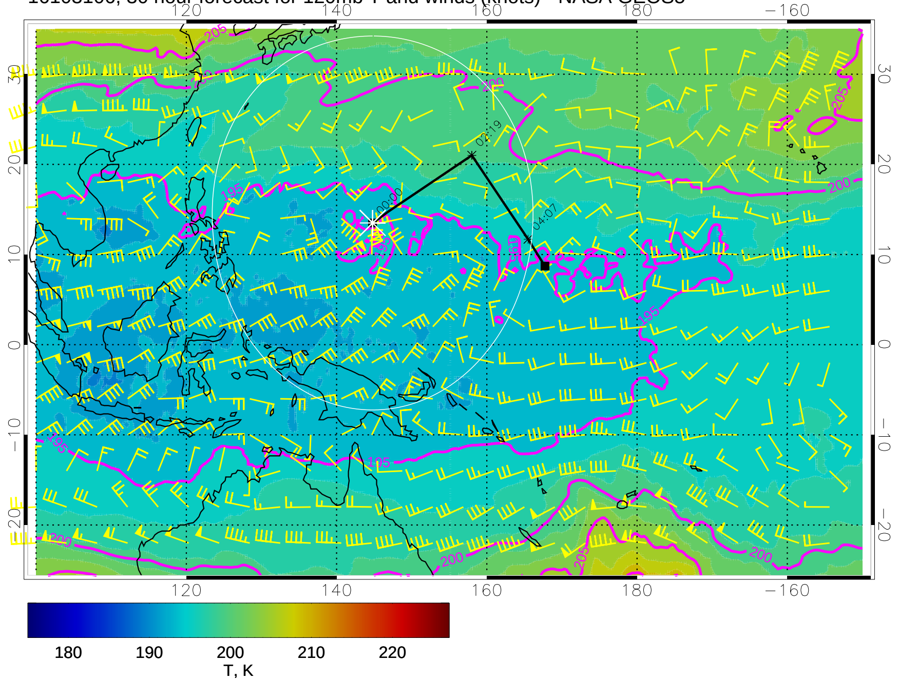
16103106, 30 hour forecast for 120mb T and winds (knots) - NASA GEOS5
