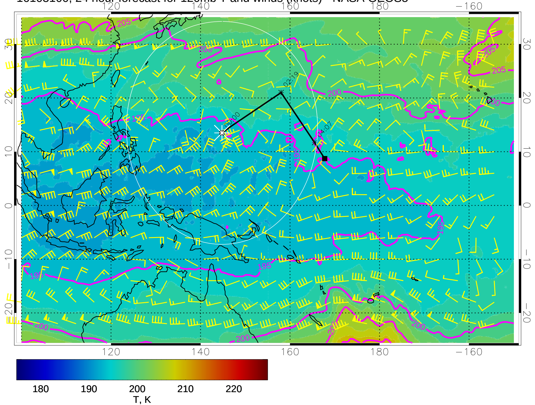
16103100, 24 hour forecast for 120mb T and winds (knots) - NASA GEOS5
