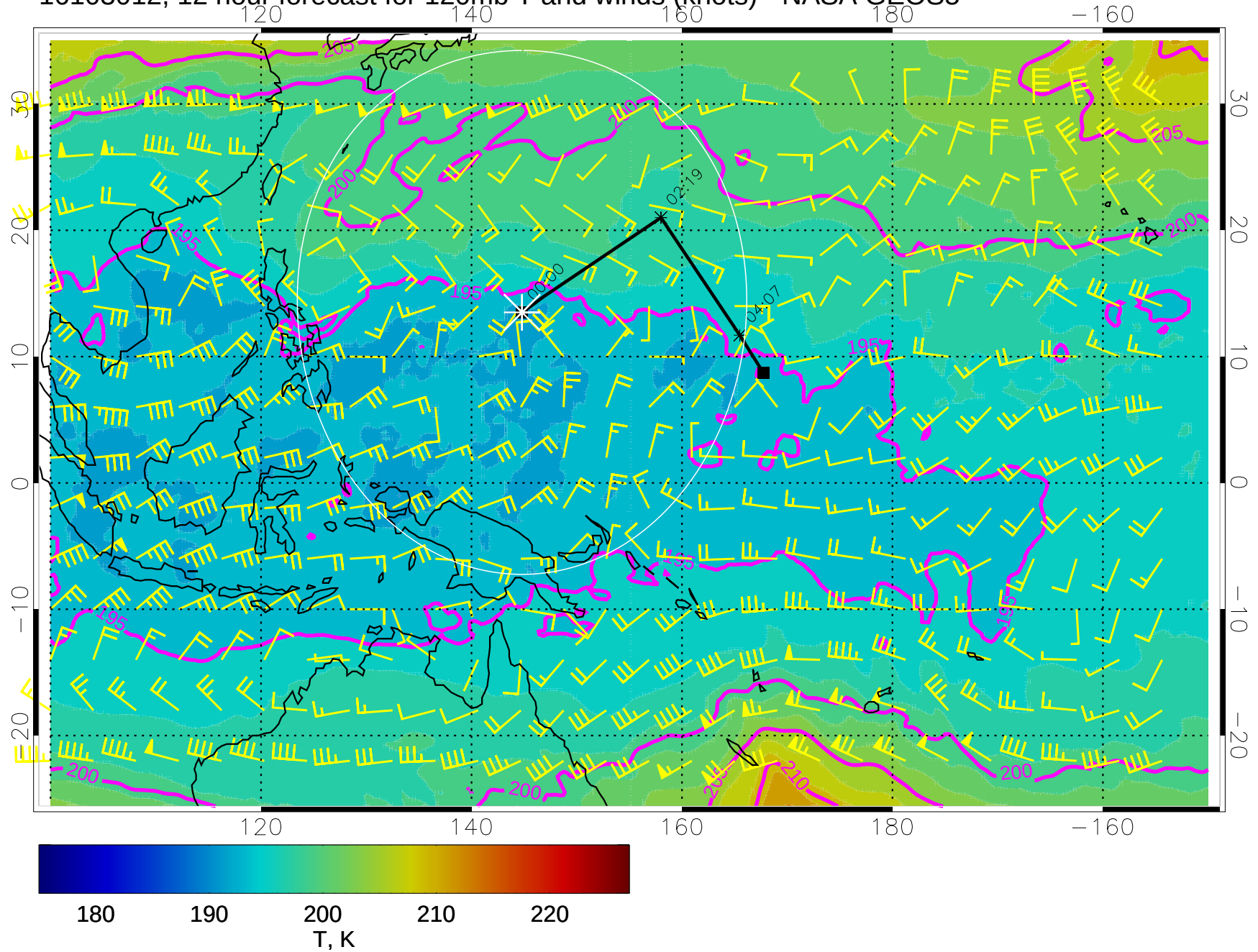
16103012, 12 hour forecast for 120mb T and winds (knots) - NASA GEOS5
