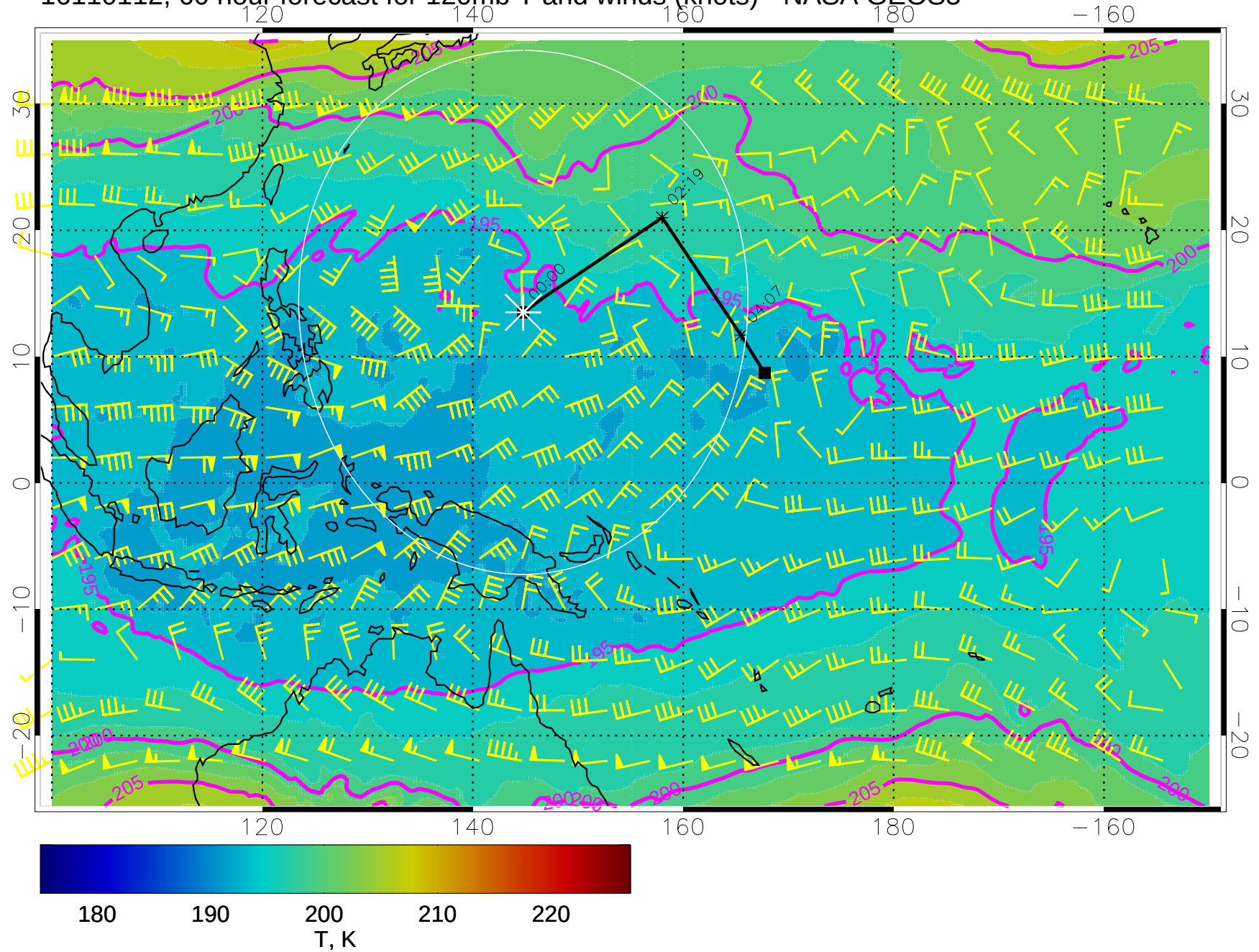
16110112, 60 hour forecast for 120mb T and winds (knots) - NASA GEOS5
