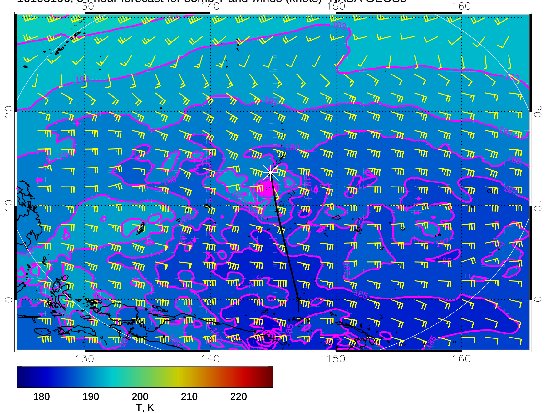
16103106, 54 hour forecast for 85mb T and winds (knots)- NASA GEOS5
