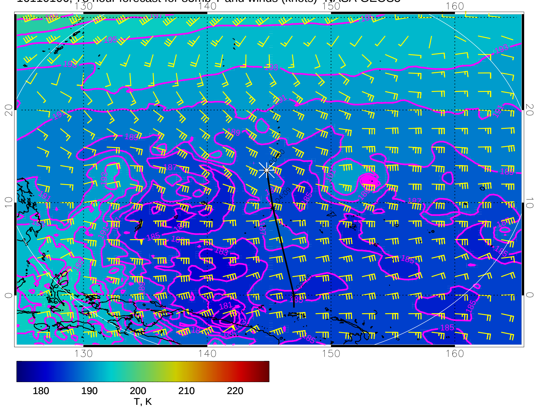
16110106, 78 hour forecast for 85mb T and winds (knots)- NASA GEOS5
