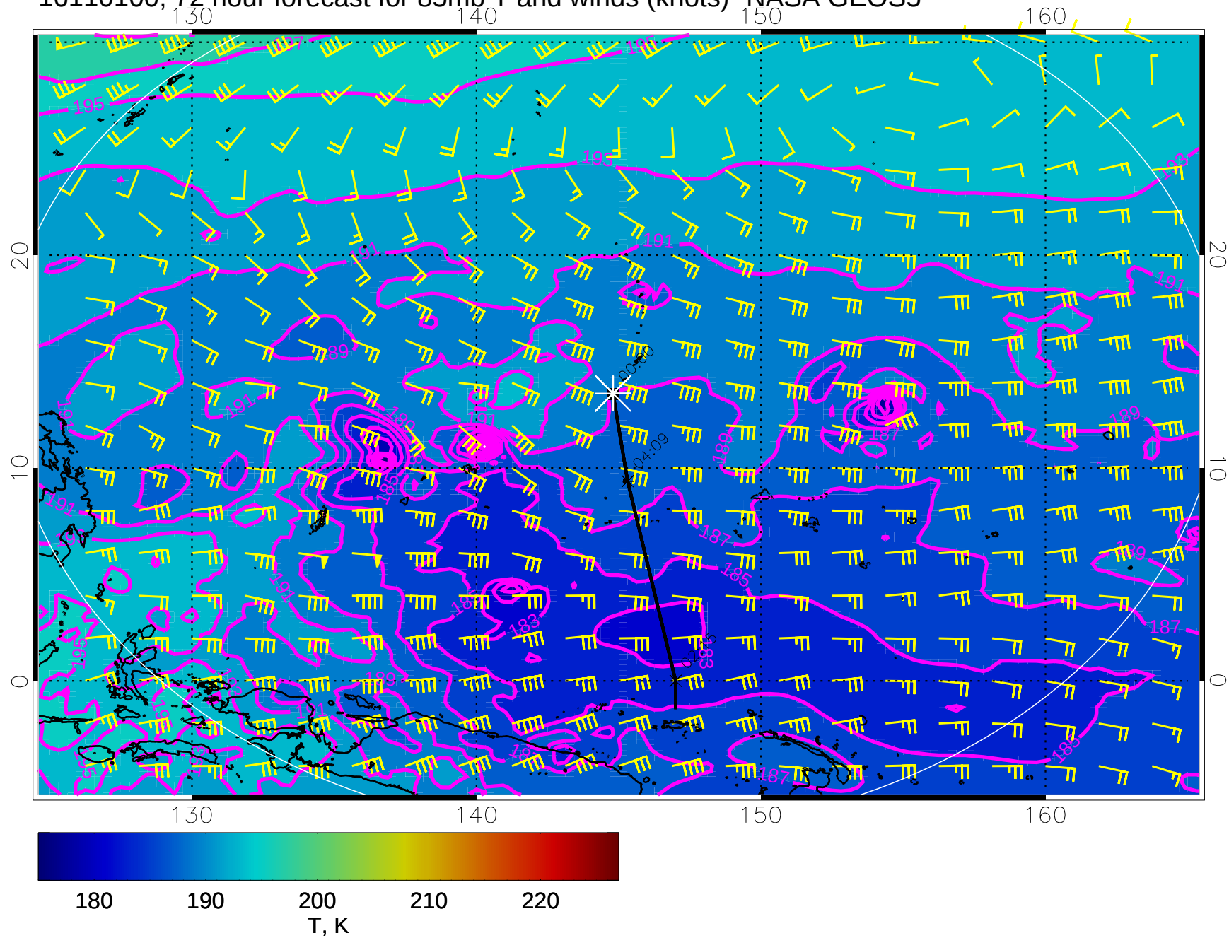
16110100, 72 hour forecast for 85mb T and winds (knots)- NASA GEOS5
