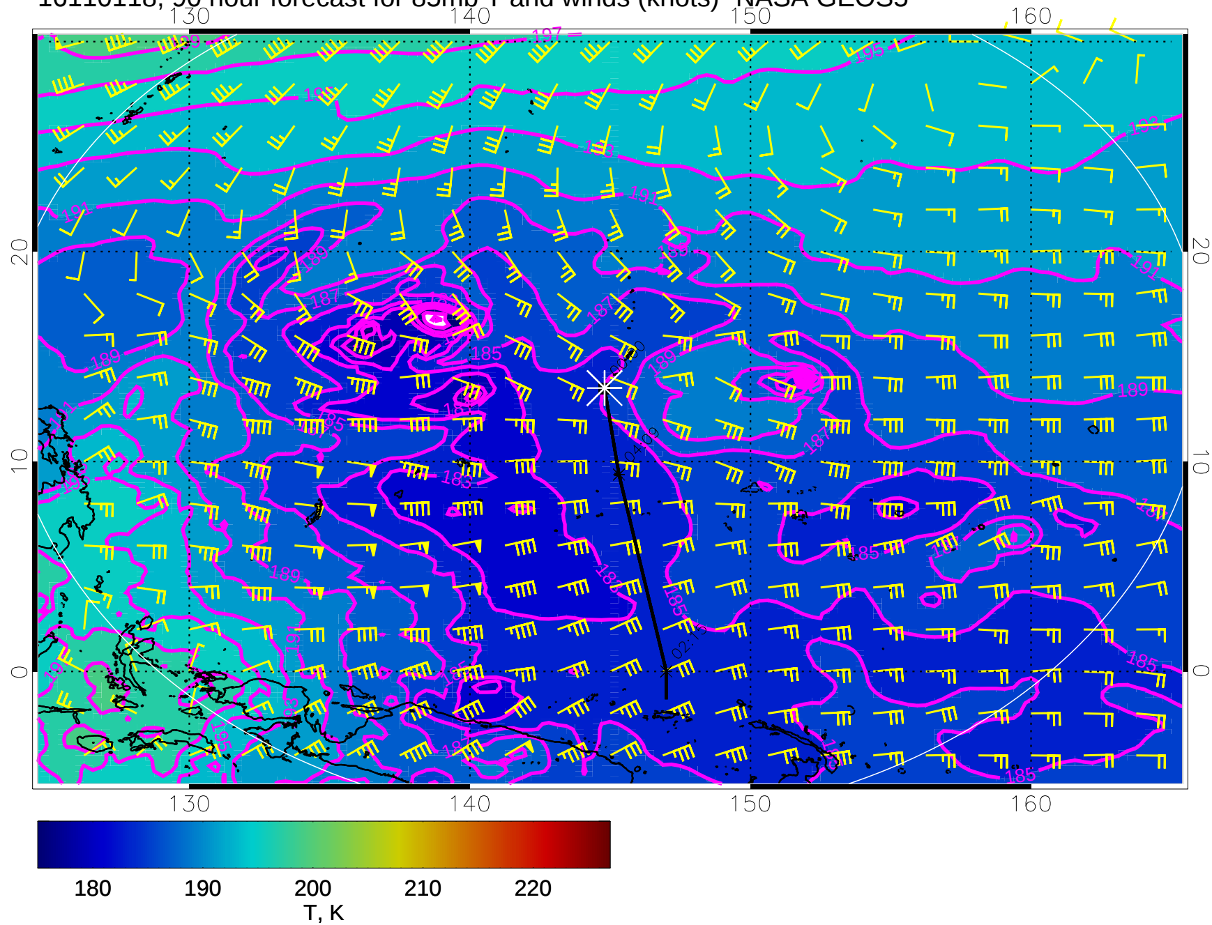
16110118, 90 hour forecast for 85mb T and winds (knots)- NASA GEOS5
