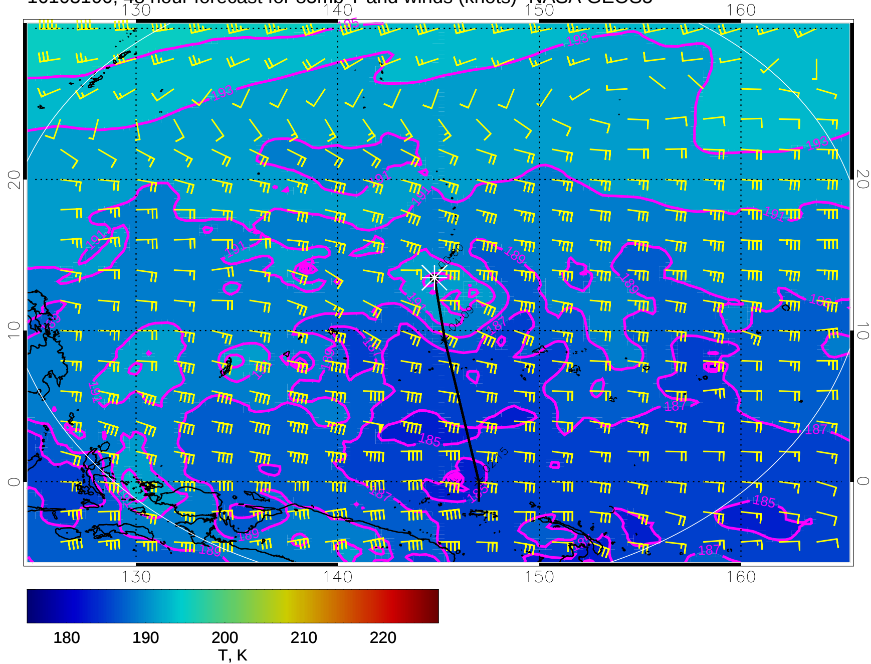
16103100, 48 hour forecast for 85mb T and winds (knots)- NASA GEOS5
