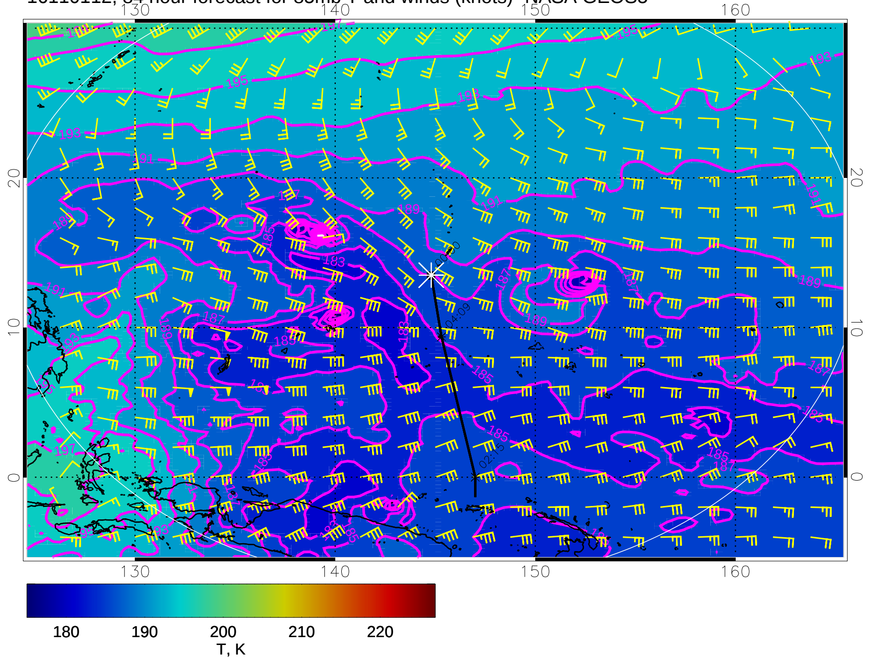
16110112, 84 hour forecast for 85mb T and winds (knots)- NASA GEOS5
