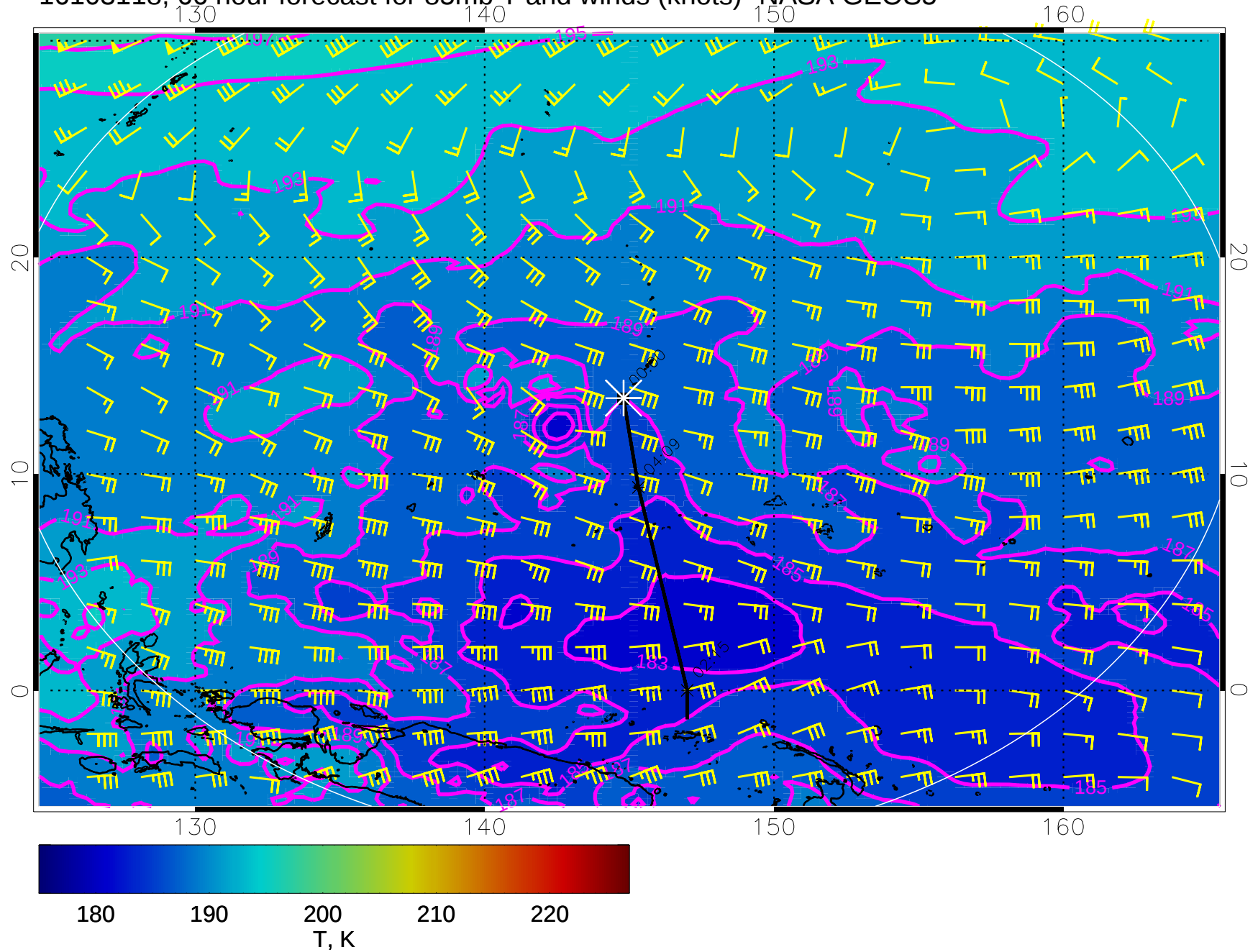
16103118, 66 hour forecast for 85mb T and winds (knots)- NASA GEOS5
