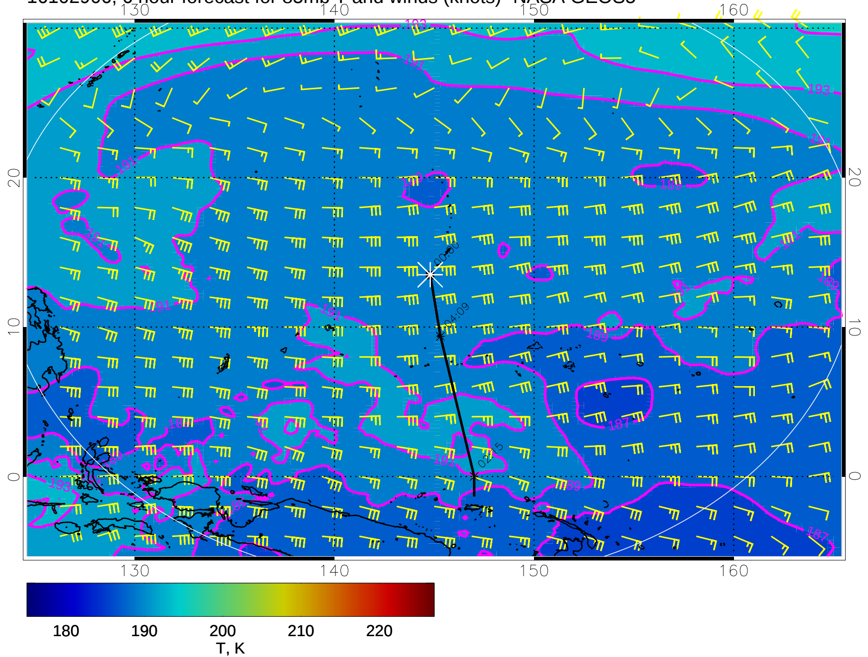
16102906, 6 hour forecast for 85mb T and winds (knots)- NASA GEOS5
