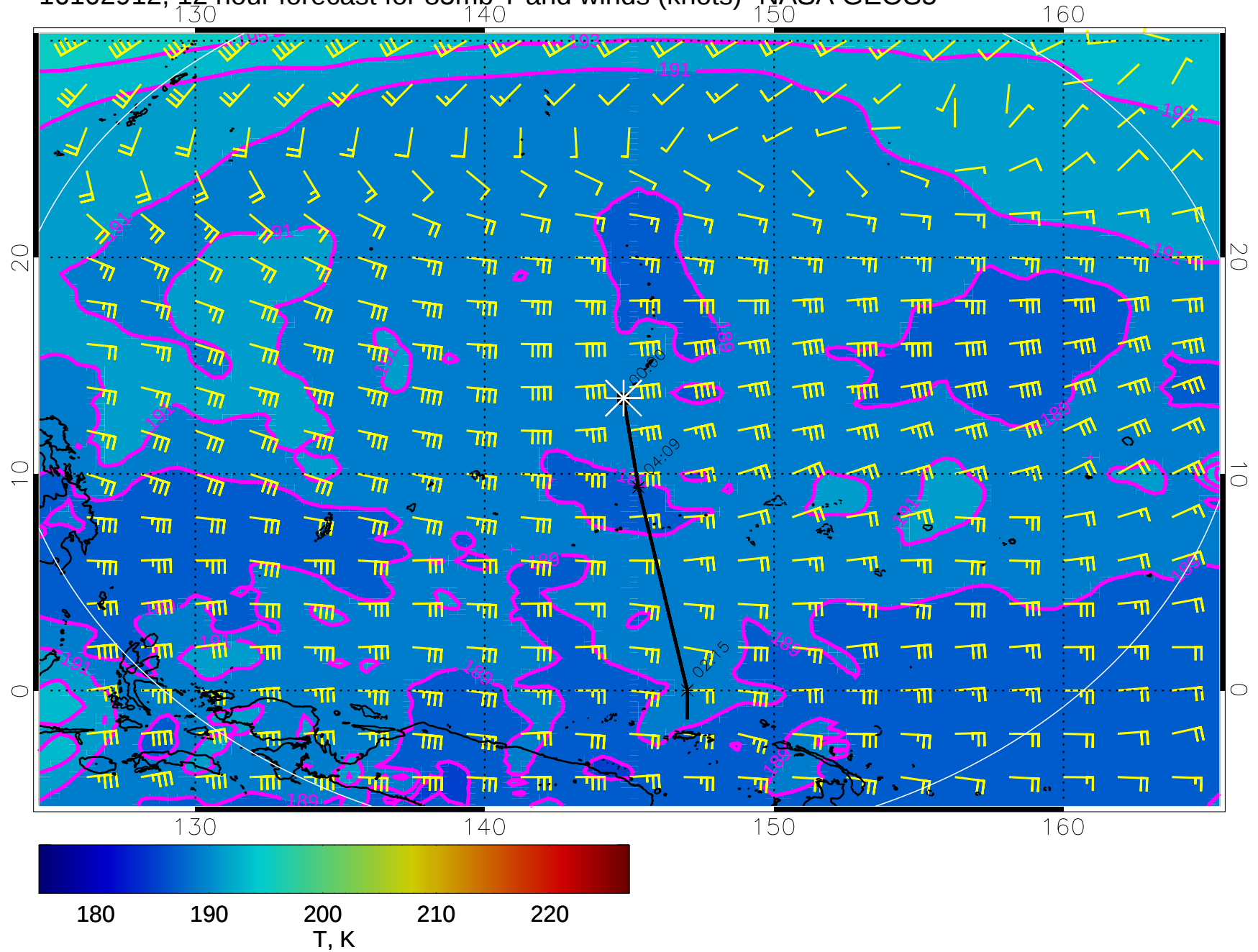
16102912, 12 hour forecast for 85mb T and winds (knots)- NASA GEOS5
