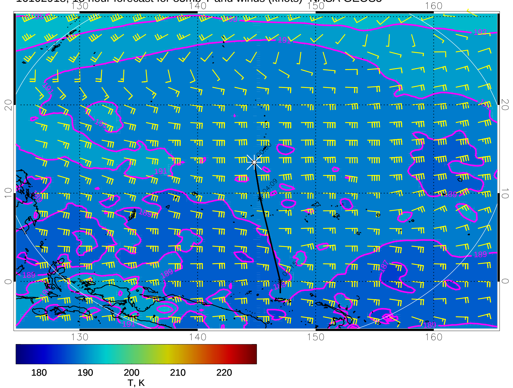
16102918, 18 hour forecast for 85mb T and winds (knots)- NASA GEOS5
