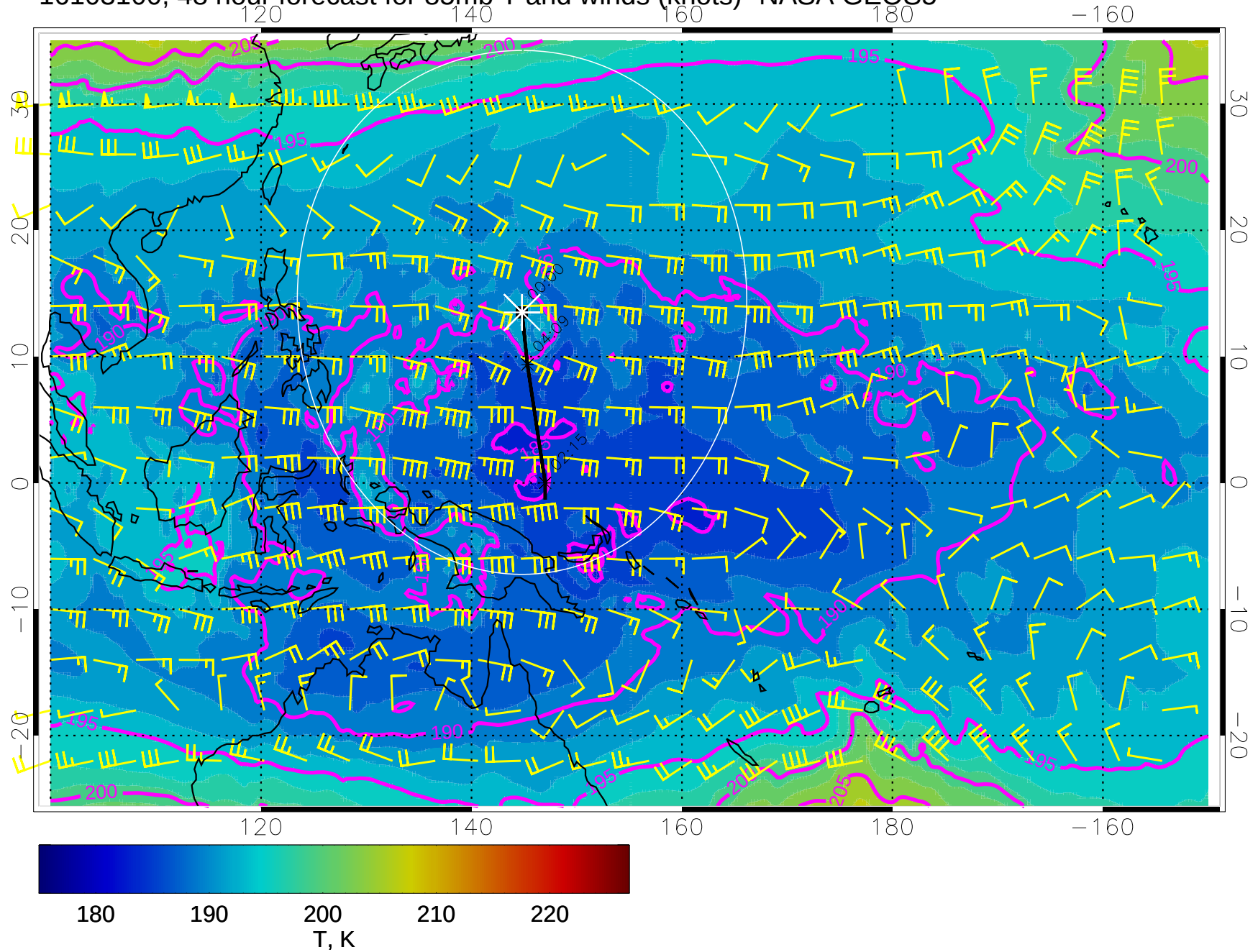
16103100, 48 hour forecast for 85mb T and winds (knots)- NASA GEOS5
