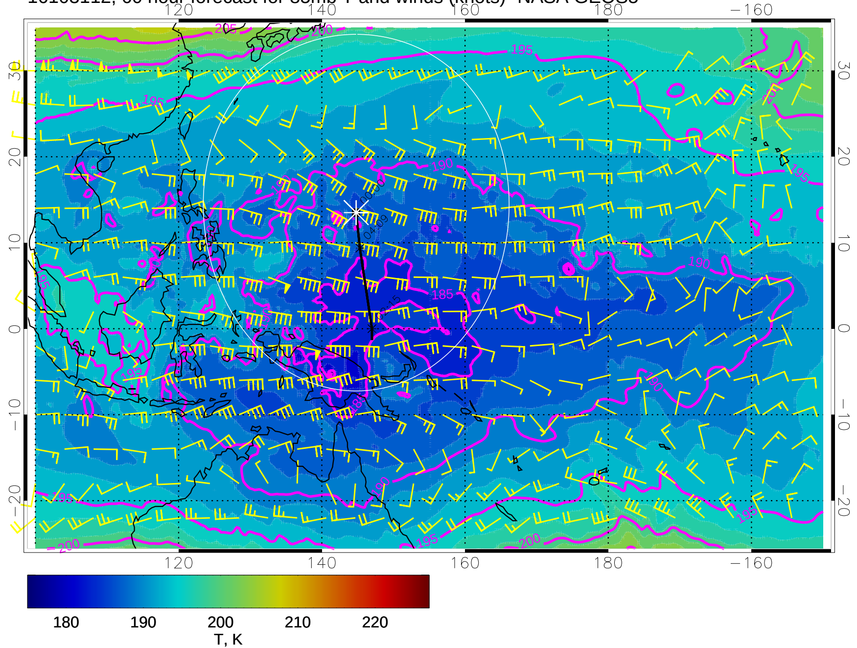
16103112, 60 hour forecast for 85mb T and winds (knots)- NASA GEOS5
