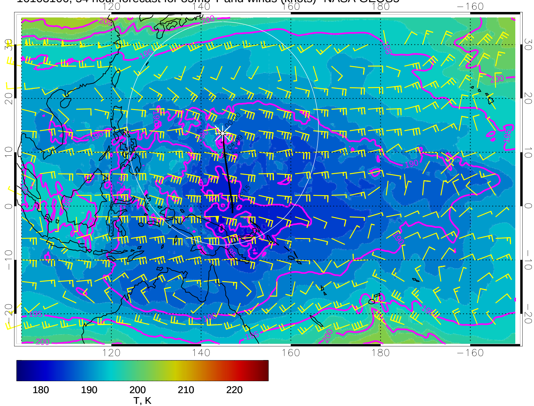
16103106, 54 hour forecast for 85mb T and winds (knots)- NASA GEOS5
