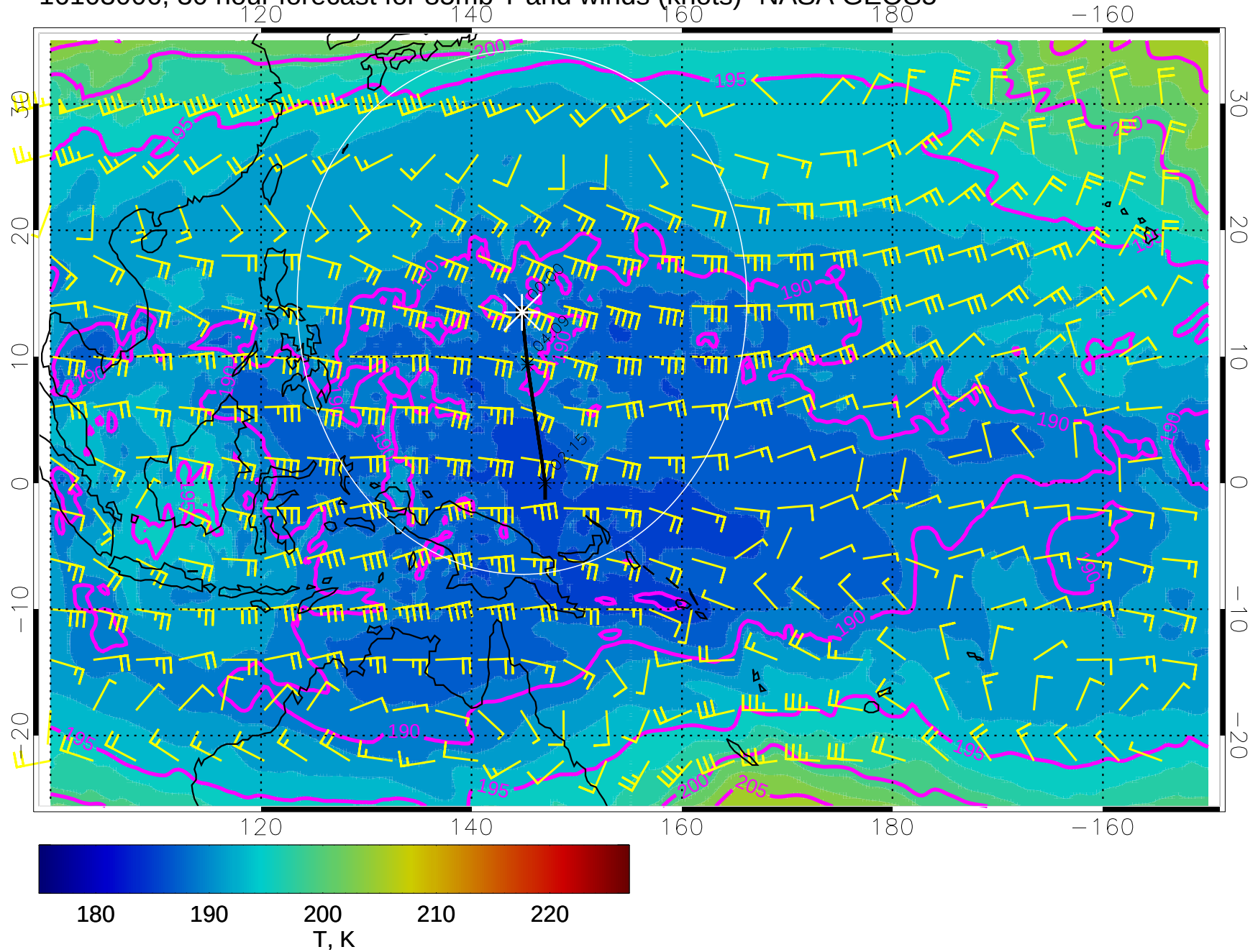
16103006, 30 hour forecast for 85mb T and winds (knots)- NASA GEOS5
