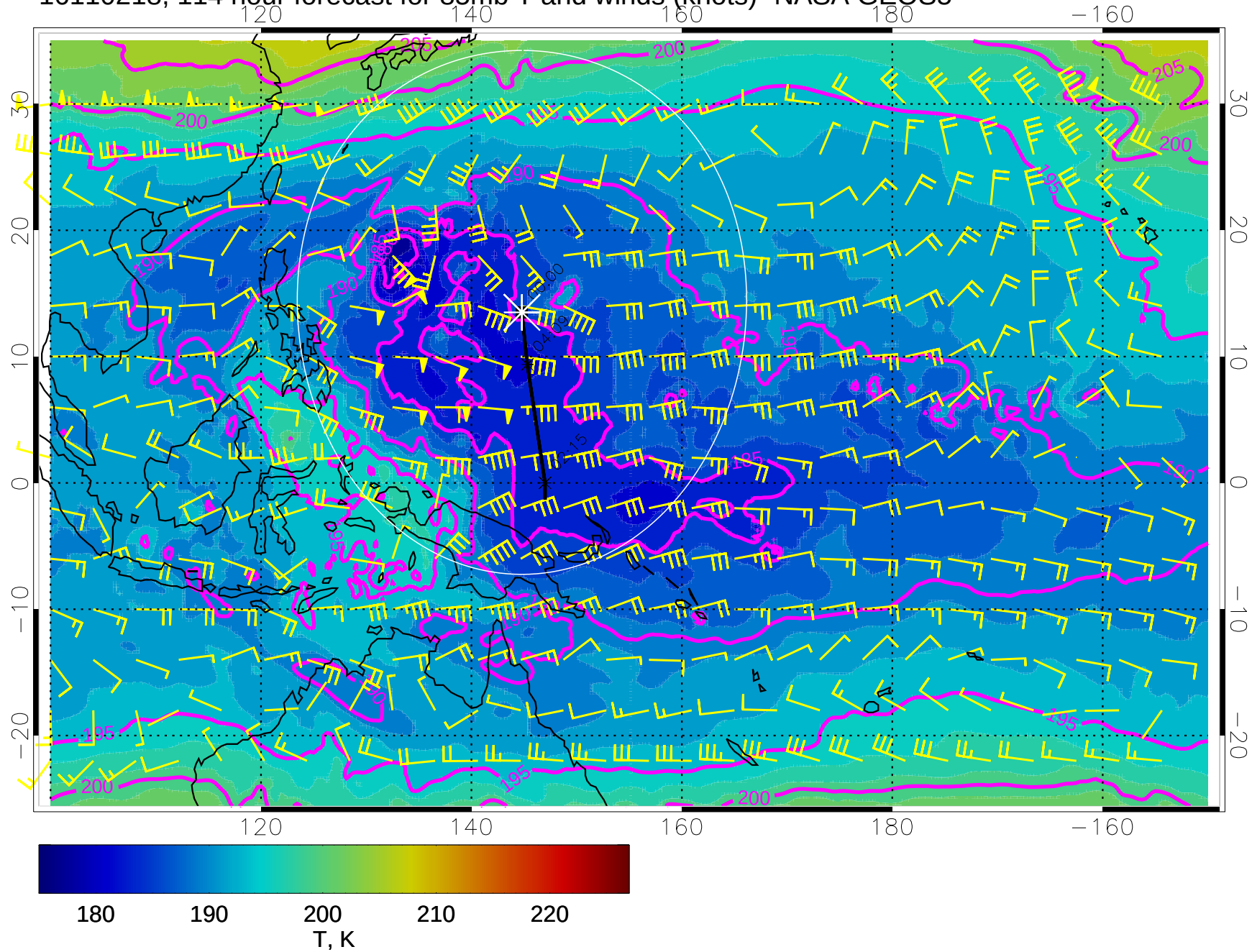
16110218, 114 hour forecast for 85mb T and winds (knots)- NASA GEOS5
