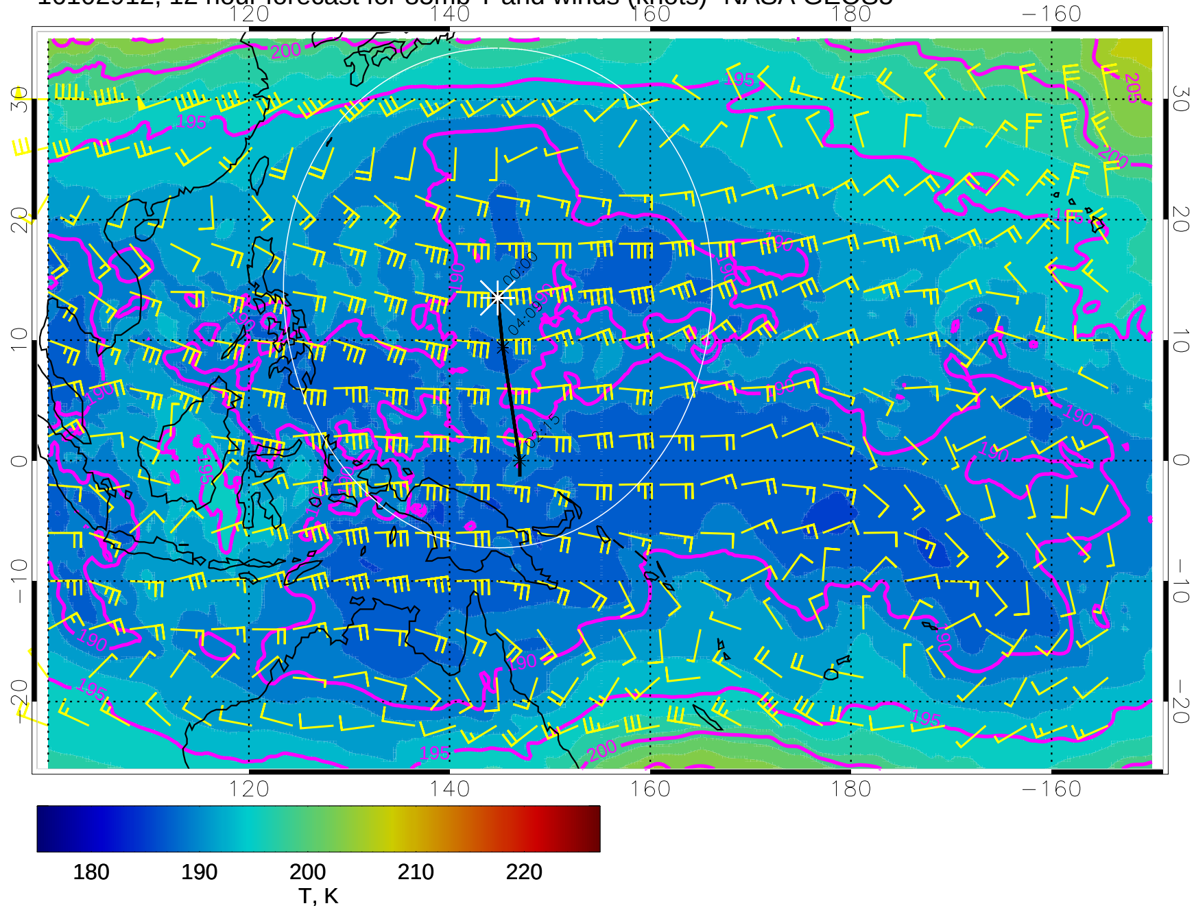
16102912, 12 hour forecast for 85mb T and winds (knots)- NASA GEOS5
