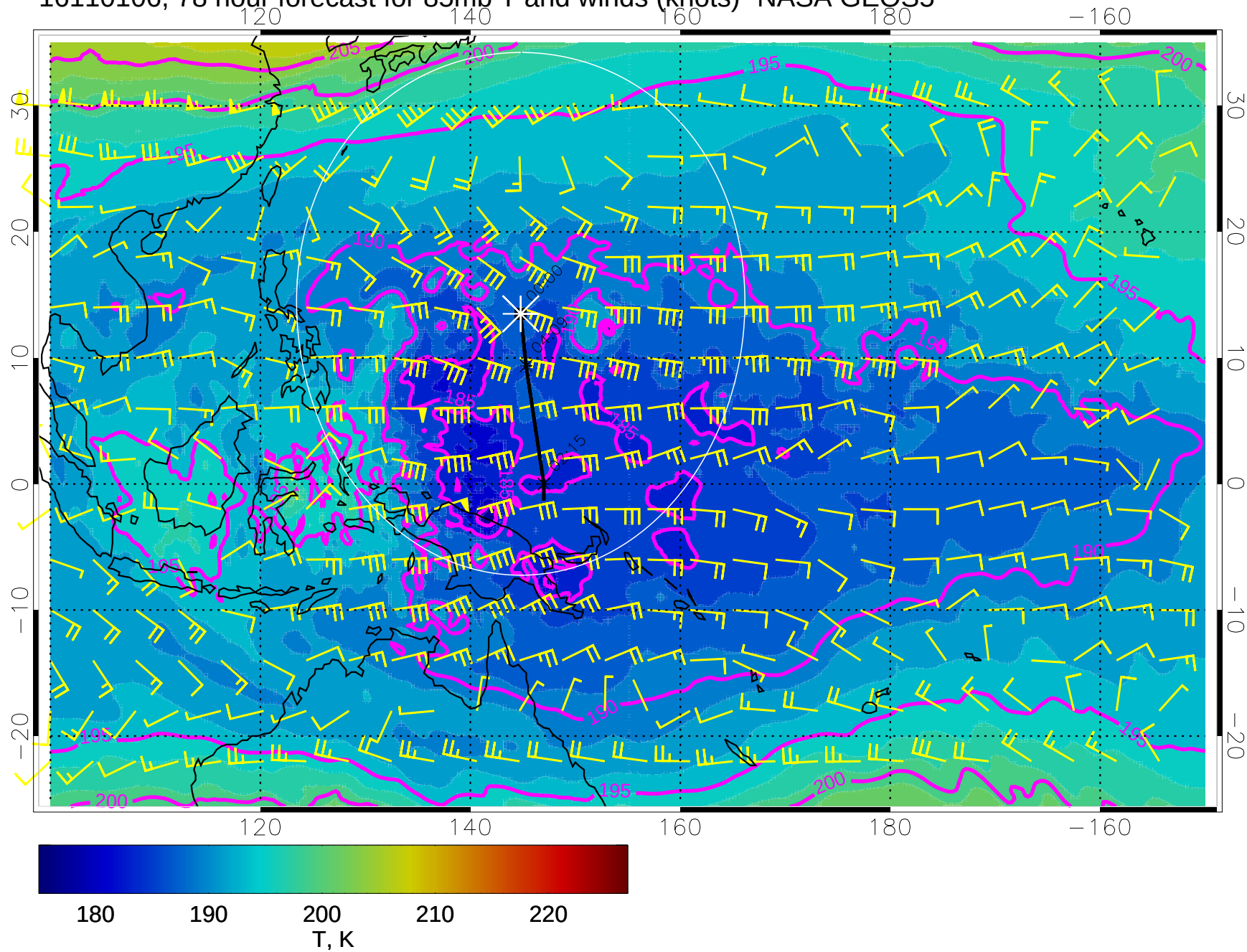
16110106, 78 hour forecast for 85mb T and winds (knots)- NASA GEOS5
