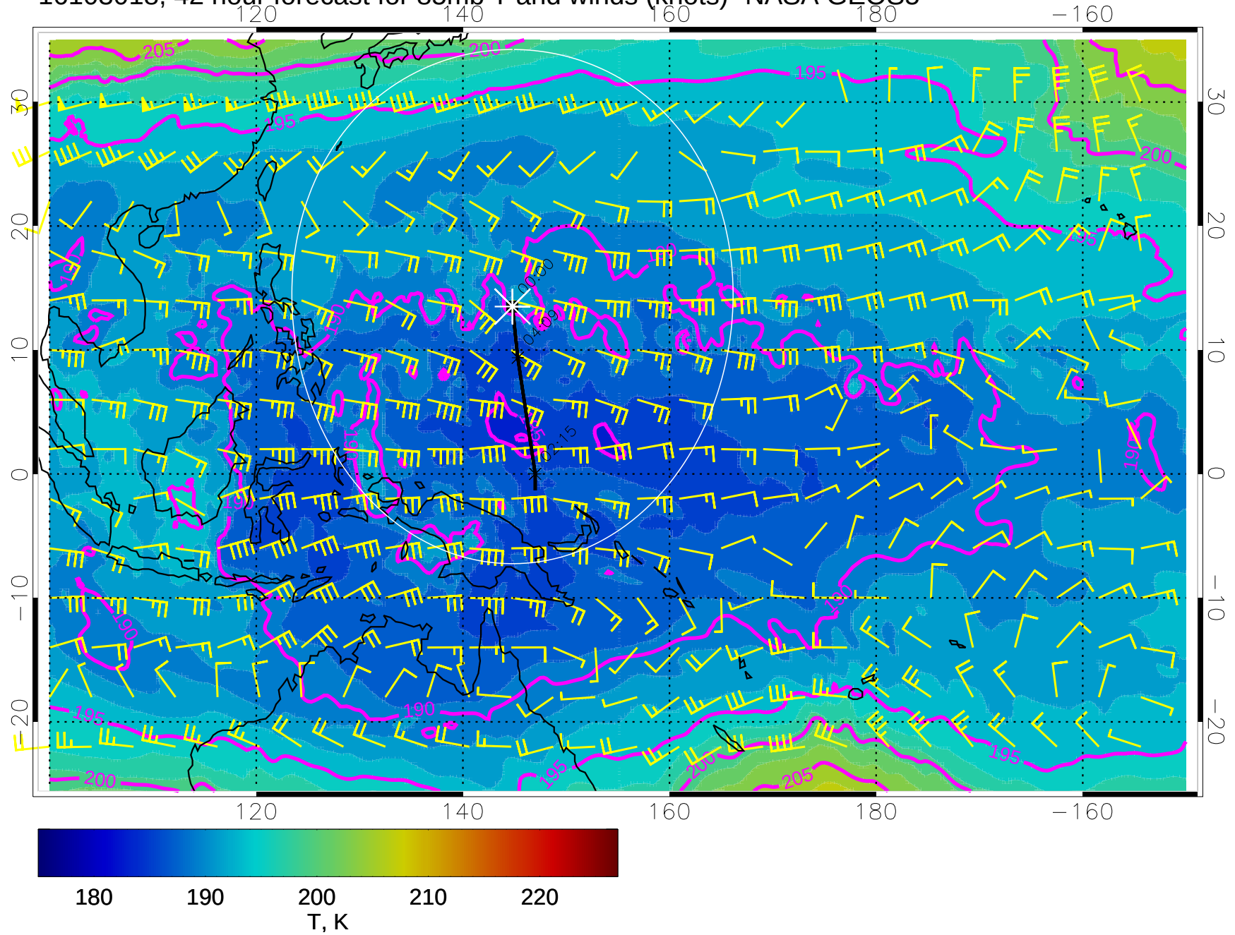
16103018, 42 hour forecast for 85mb T and winds (knots)- NASA GEOS5
