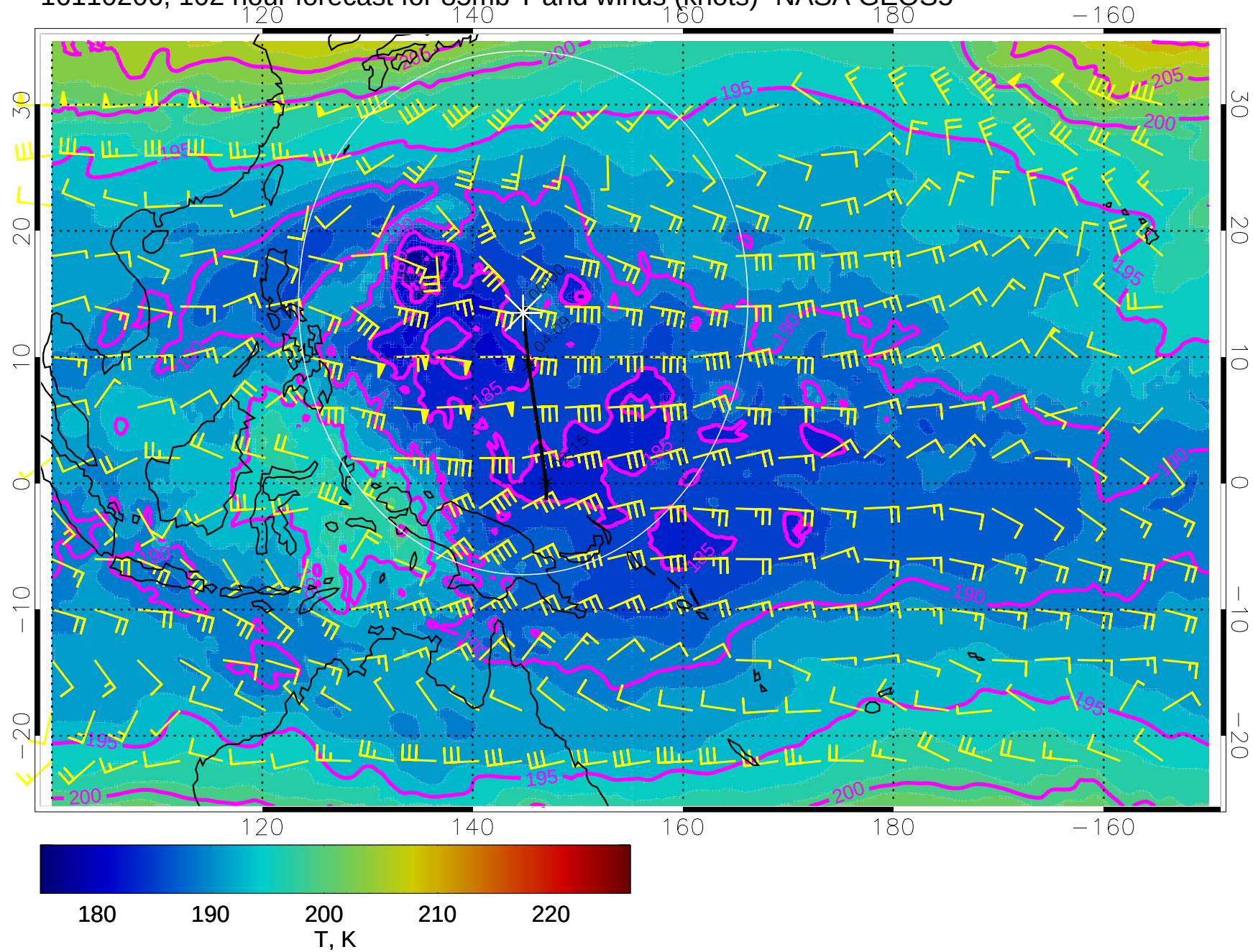
16110206, 102 hour forecast for 85mb T and winds (knots)- NASA GEOS5
