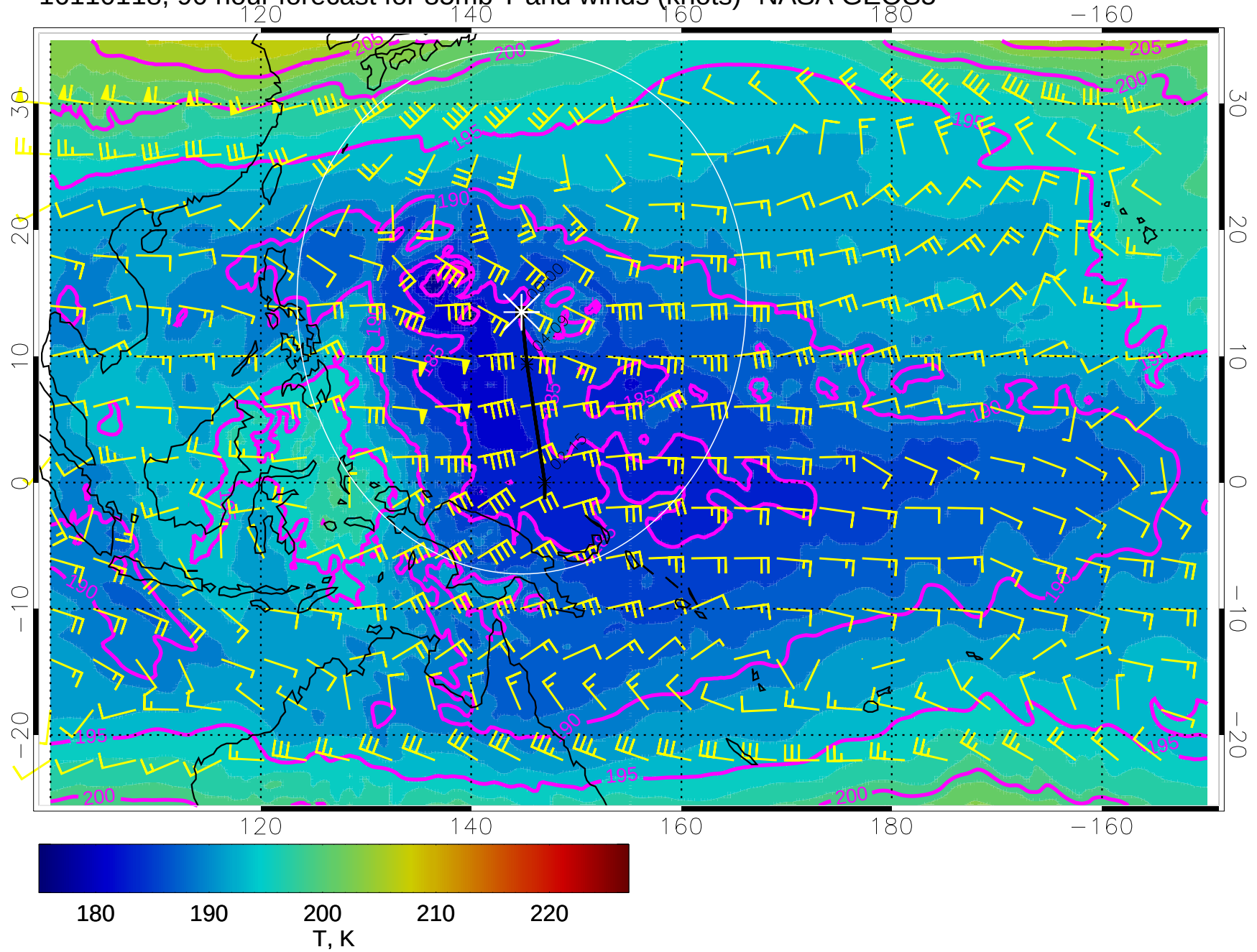
16110118, 90 hour forecast for 85mb T and winds (knots)- NASA GEOS5
