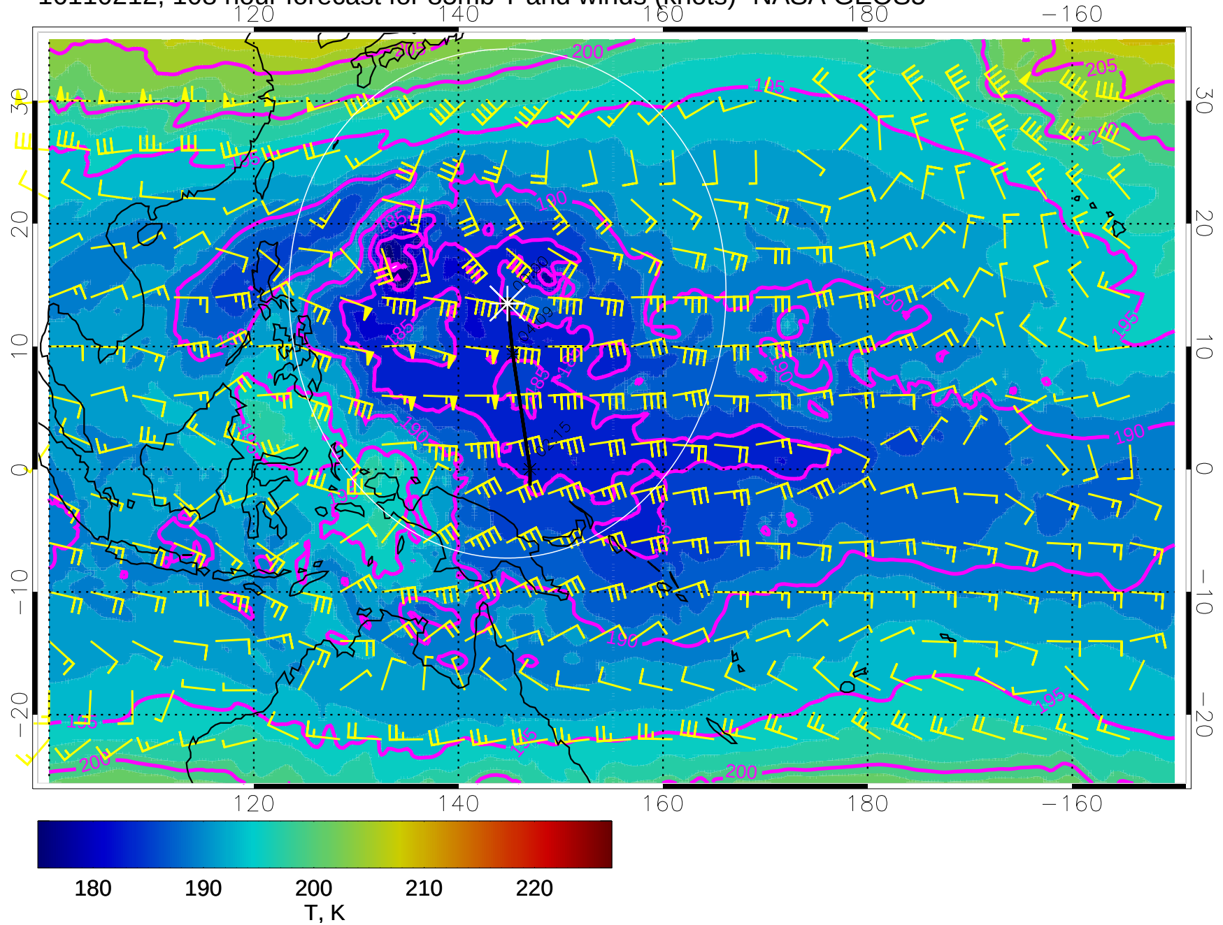
16110212, 108 hour forecast for 85mb T and winds (knots)- NASA GEOS5
