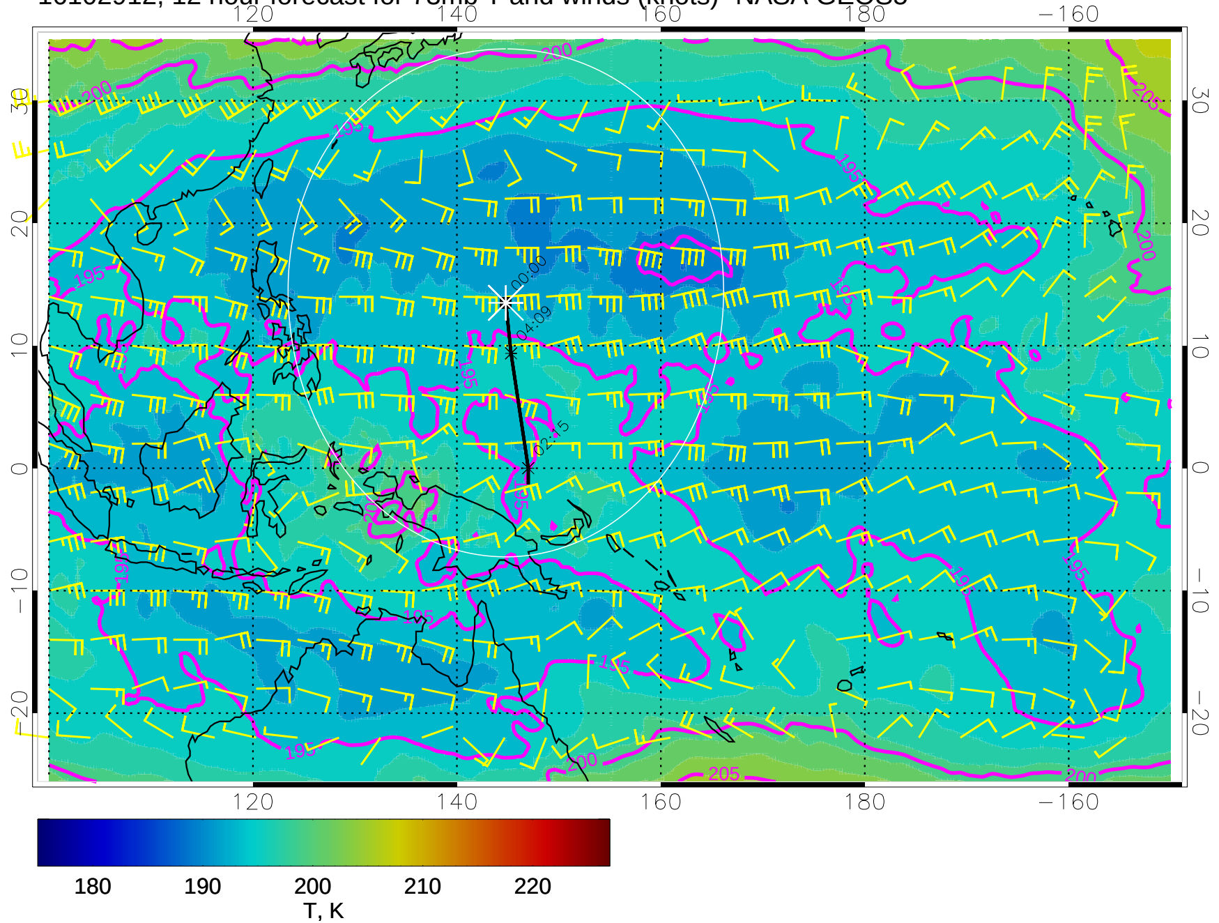
16102912, 12 hour forecast for 73mb T and winds (knots)- NASA GEOS5
