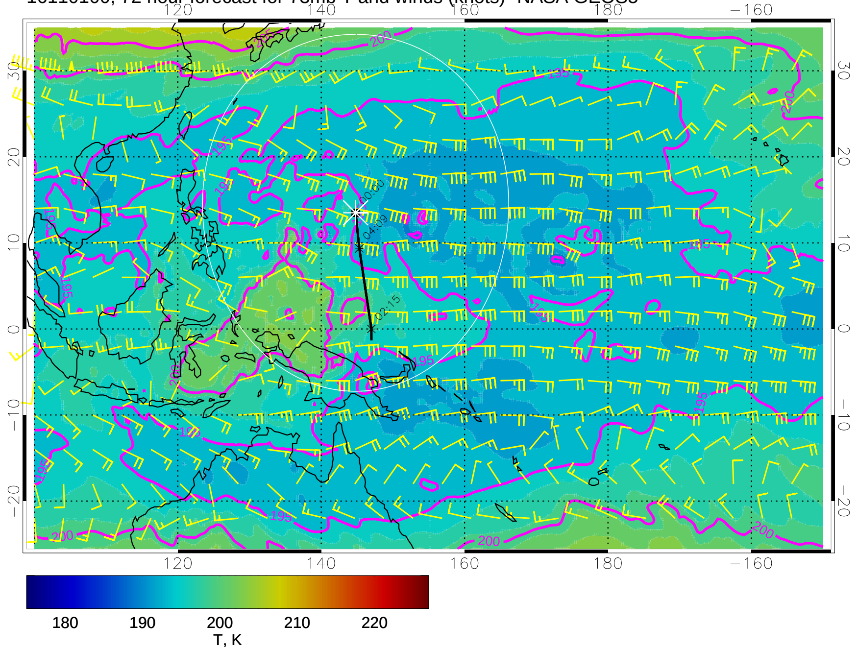
16110100, 72 hour forecast for 73mb T and winds (knots)- NASA GEOS5
