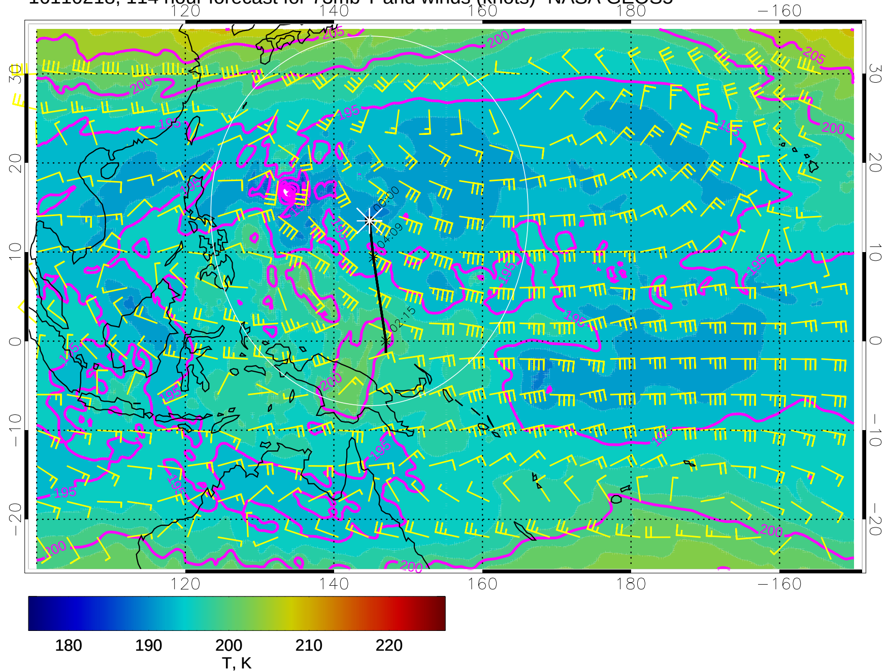
16110218, 114 hour forecast for 73mb T and winds (knots)- NASA GEOS5
