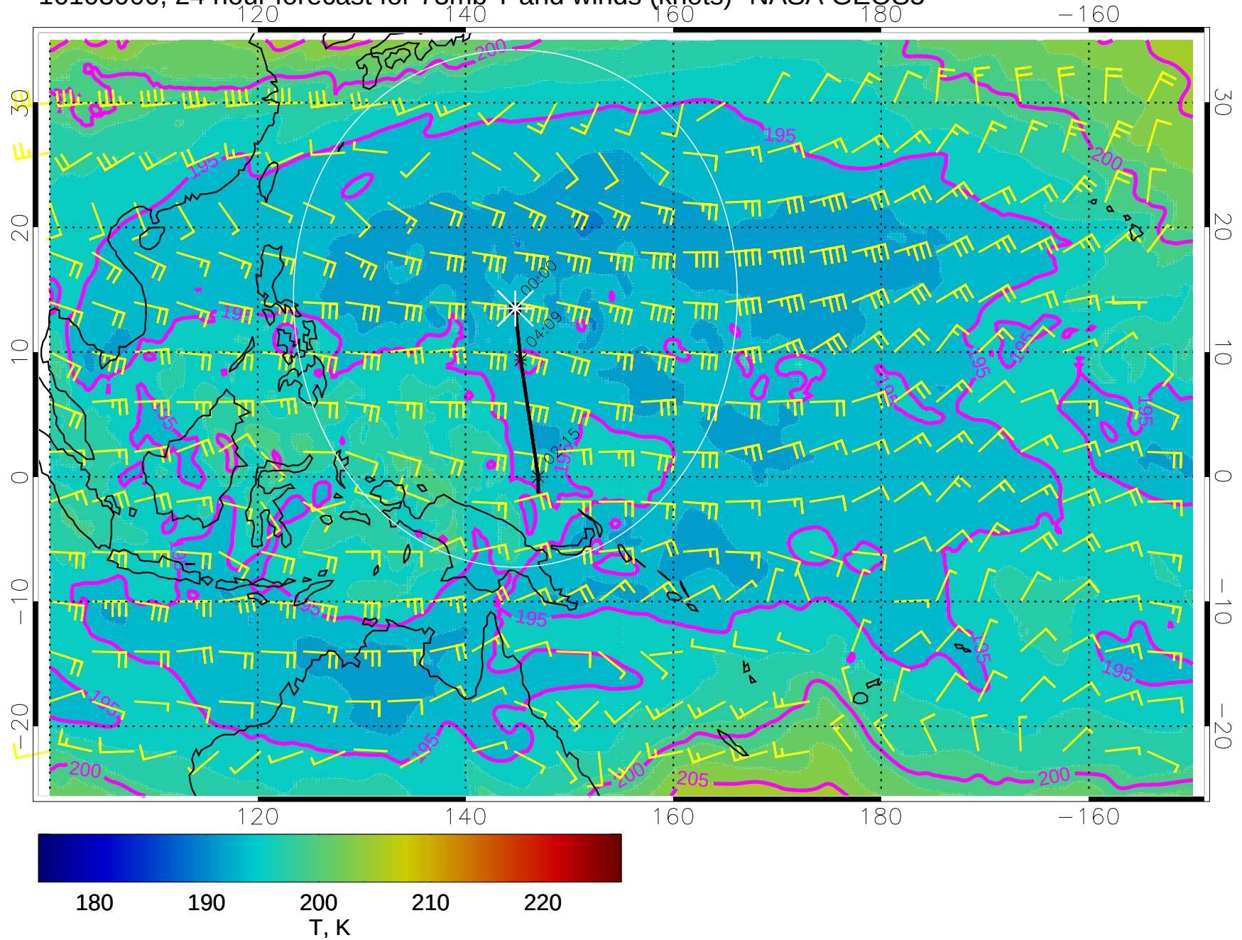
16103000, 24 hour forecast for 73mb T and winds (knots)- NASA GEOS5
