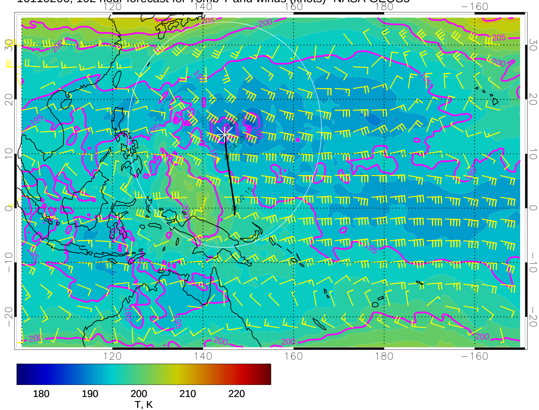
16110206, 102 hour forecast for 73mb T and winds (knots)- NASA GEOS5
