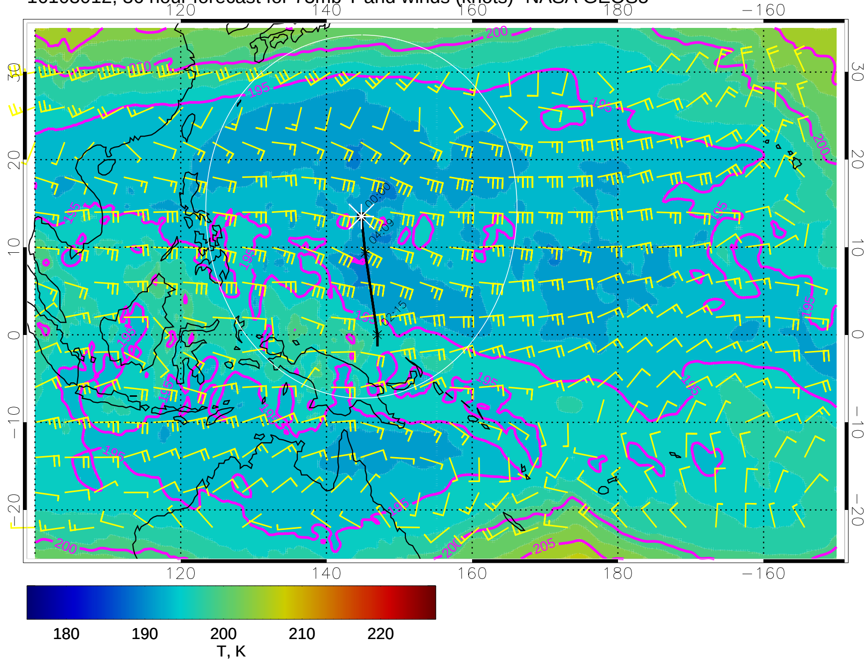
16103012, 36 hour forecast for 73mb T and winds (knots)- NASA GEOS5
