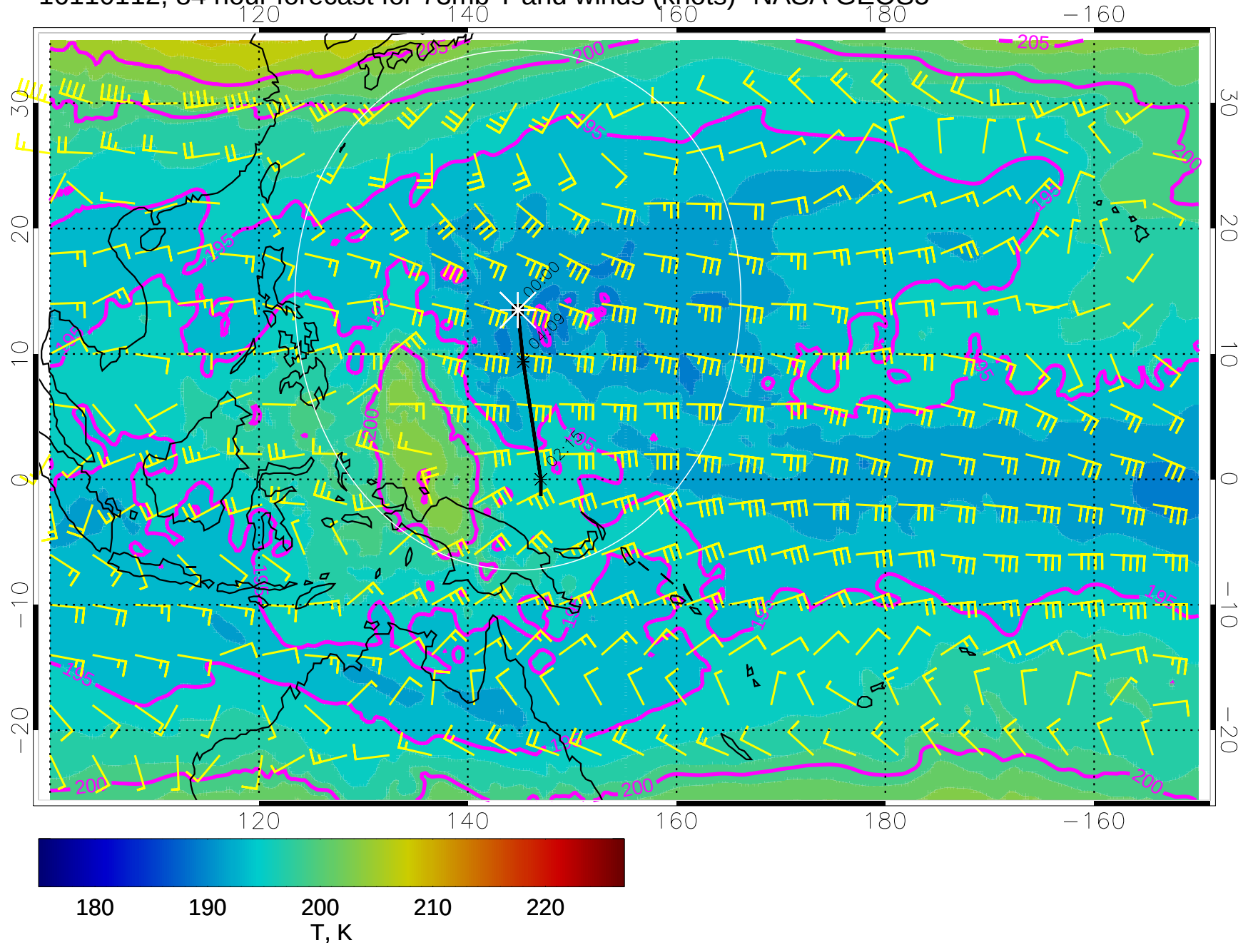
16110112, 84 hour forecast for 73mb T and winds (knots)- NASA GEOS5
