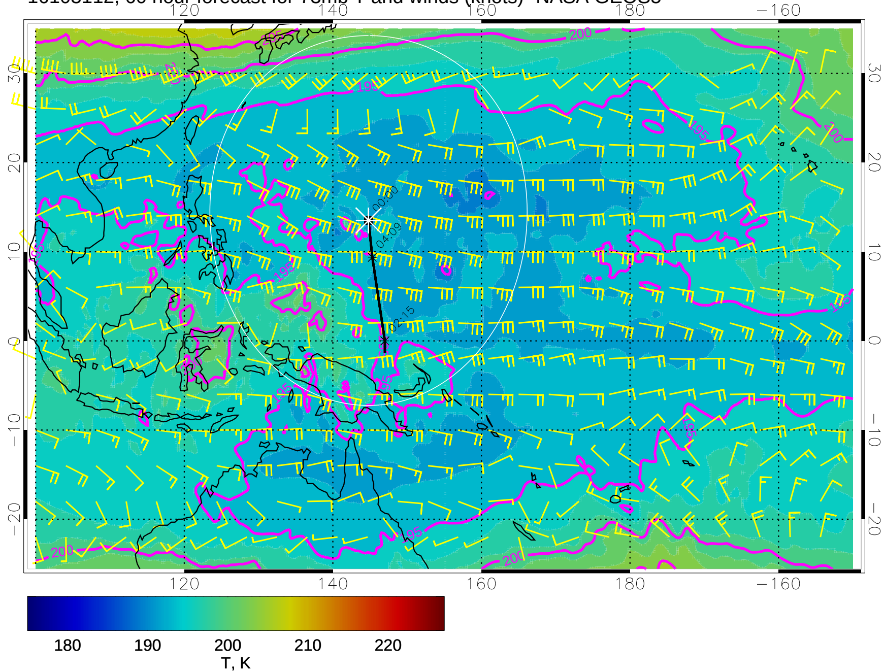
16103112, 60 hour forecast for 73mb T and winds (knots)- NASA GEOS5
