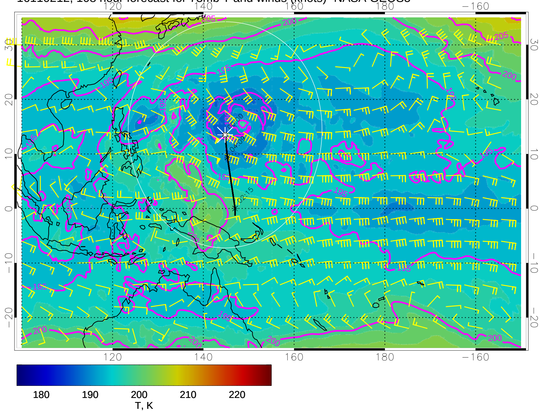
16110212, 108 hour forecast for 73mb T and winds (knots)- NASA GEOS5
