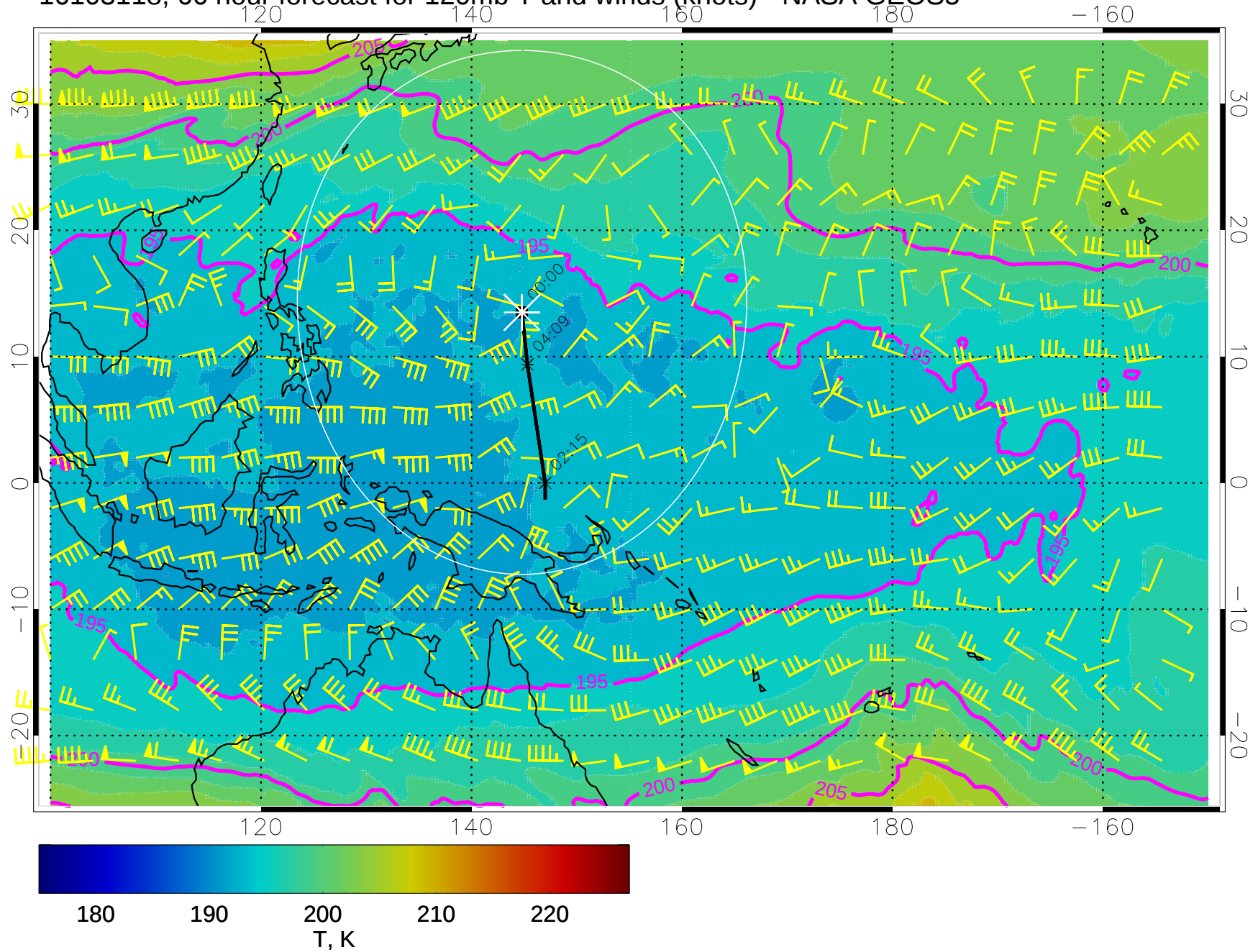
16103118, 66 hour forecast for 120mb T and winds (knots) - NASA GEOS5
