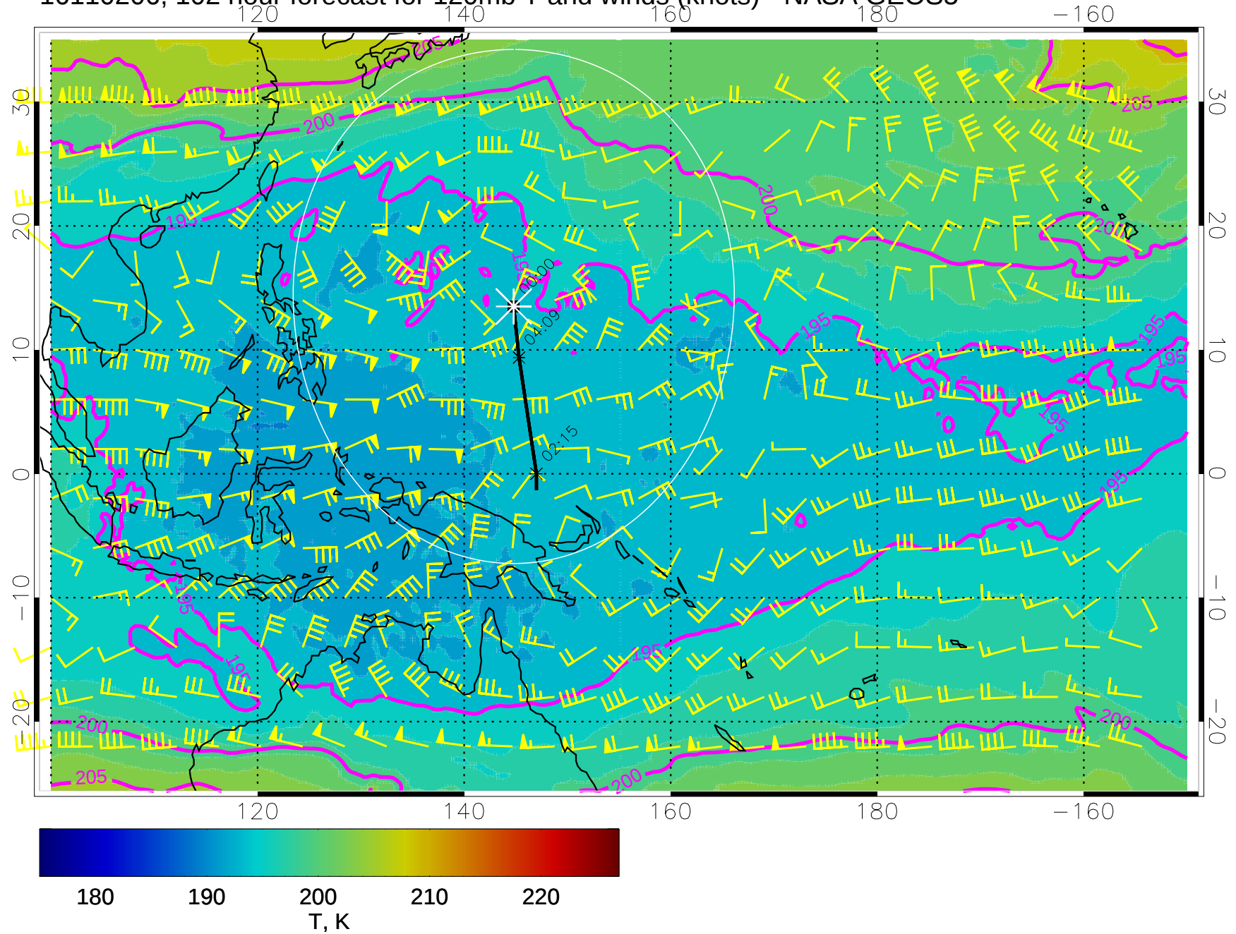
16110206, 102 hour forecast for 120mb T and winds (knots) - NASA GEOS5
