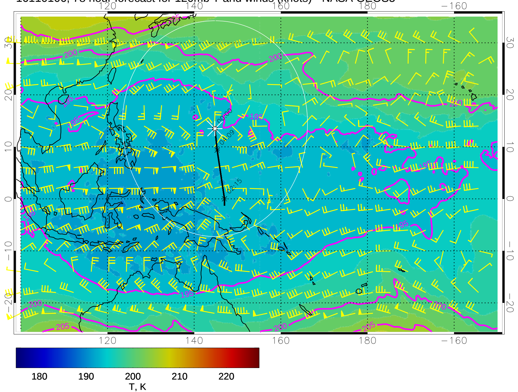
16110106, 78 hour forecast for 120mb T and winds (knots) - NASA GEOS5
