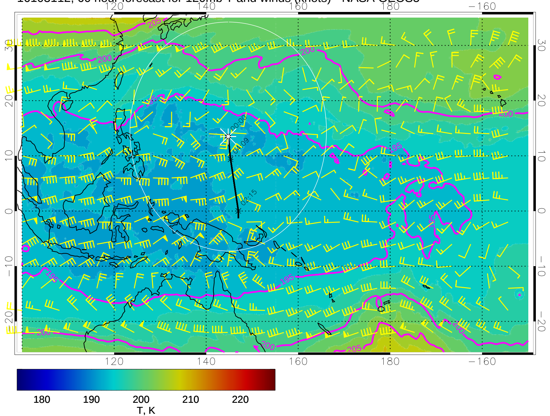
16103112, 60 hour forecast for 120mb T and winds (knots) - NASA GEOS5
