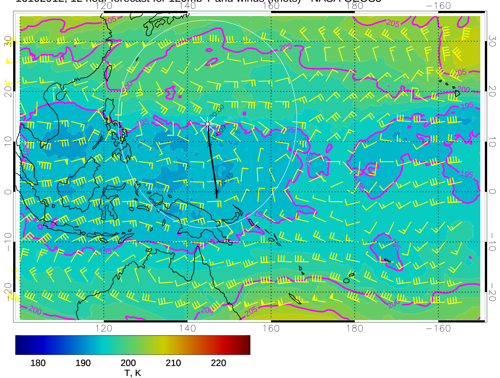
16102912, 12 hour forecast for 120mb T and winds (knots) - NASA GEOS5
