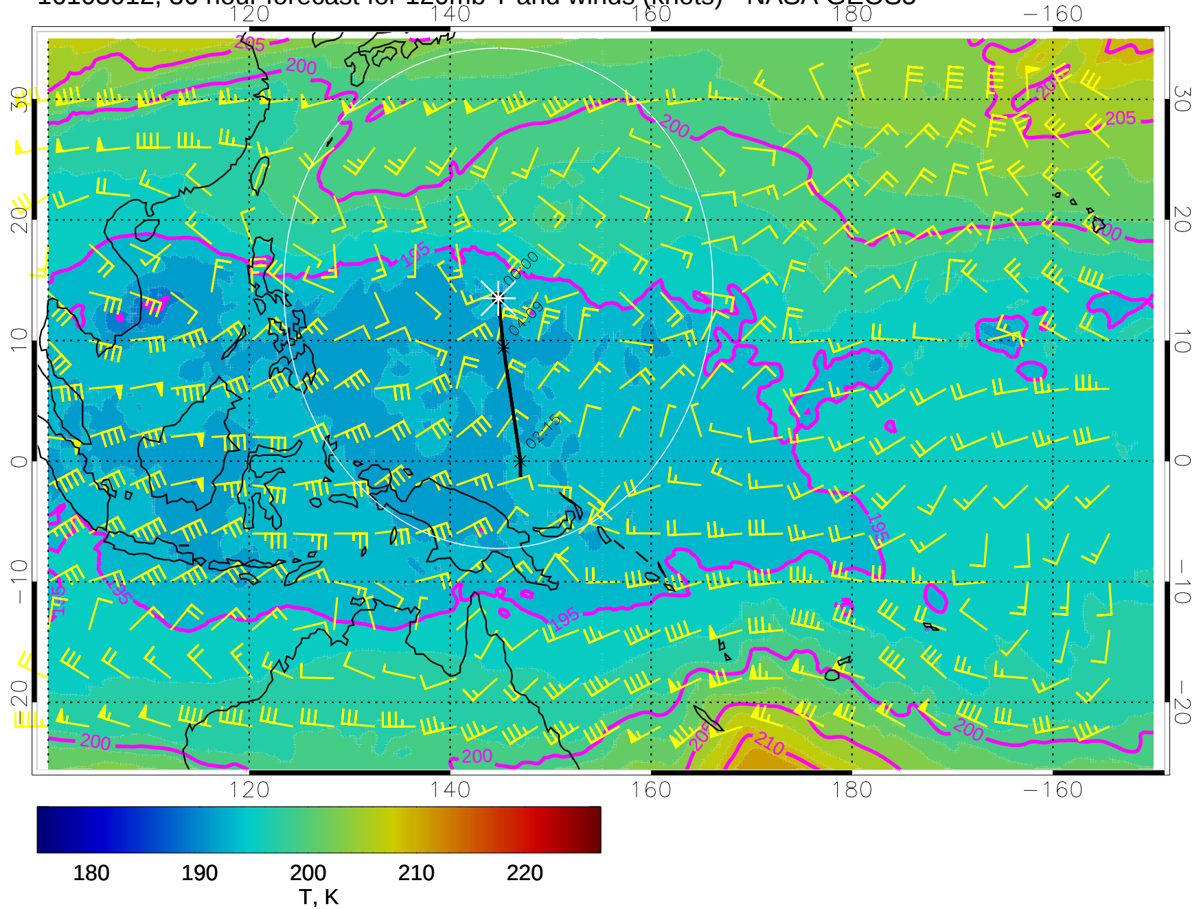
16103012, 36 hour forecast for 120mb T and winds (knots) - NASA GEOS5
