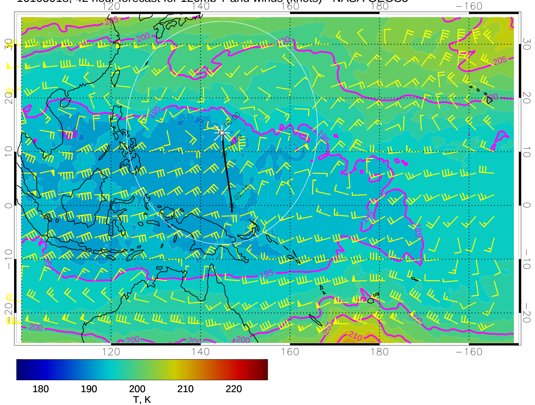
16103018, 42 hour forecast for 120mb T and winds (knots) - NASA GEOS5
