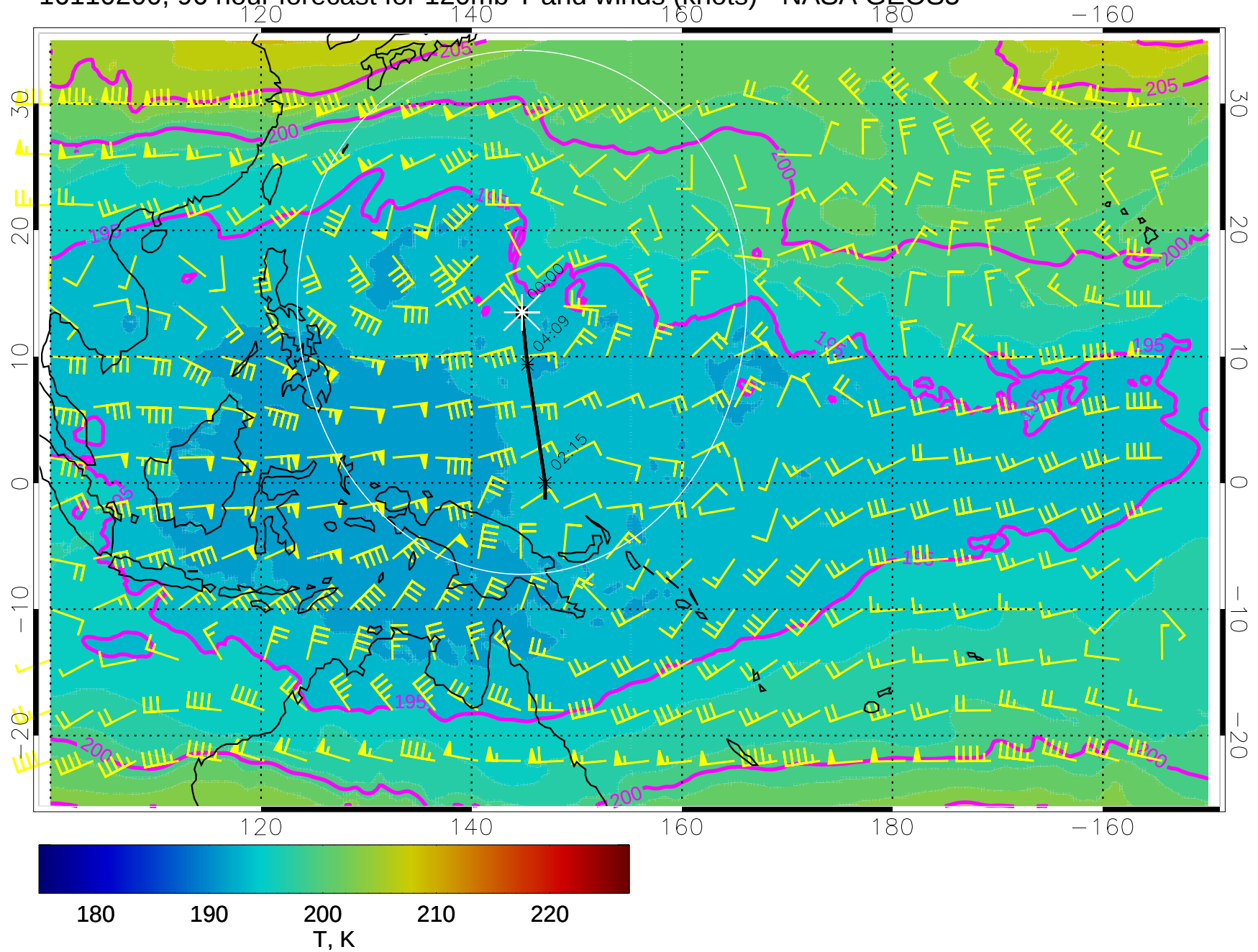
16110200, 96 hour forecast for 120mb T and winds (knots) - NASA GEOS5
