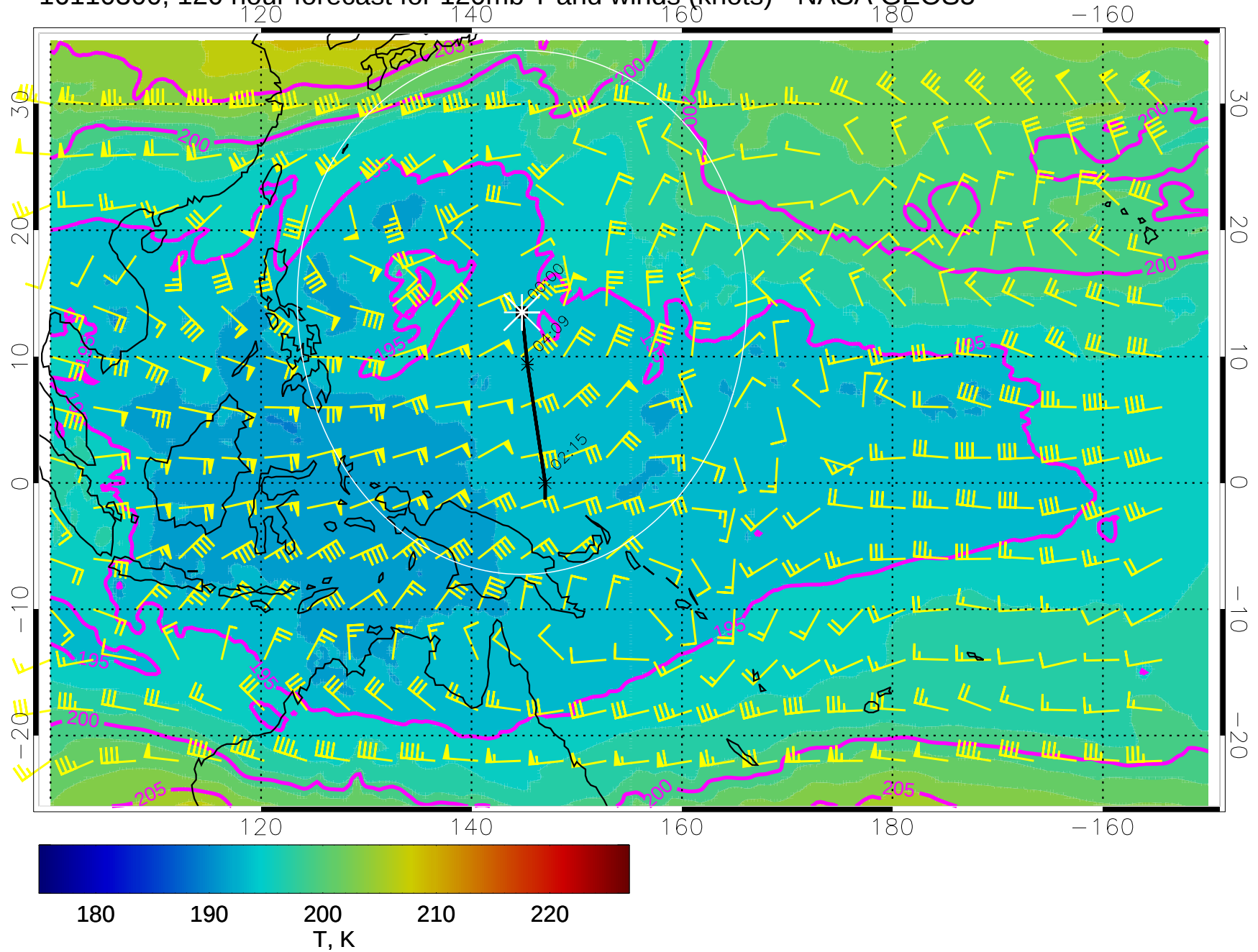
16110300, 120 hour forecast for 120mb T and winds (knots) - NASA GEOS5
