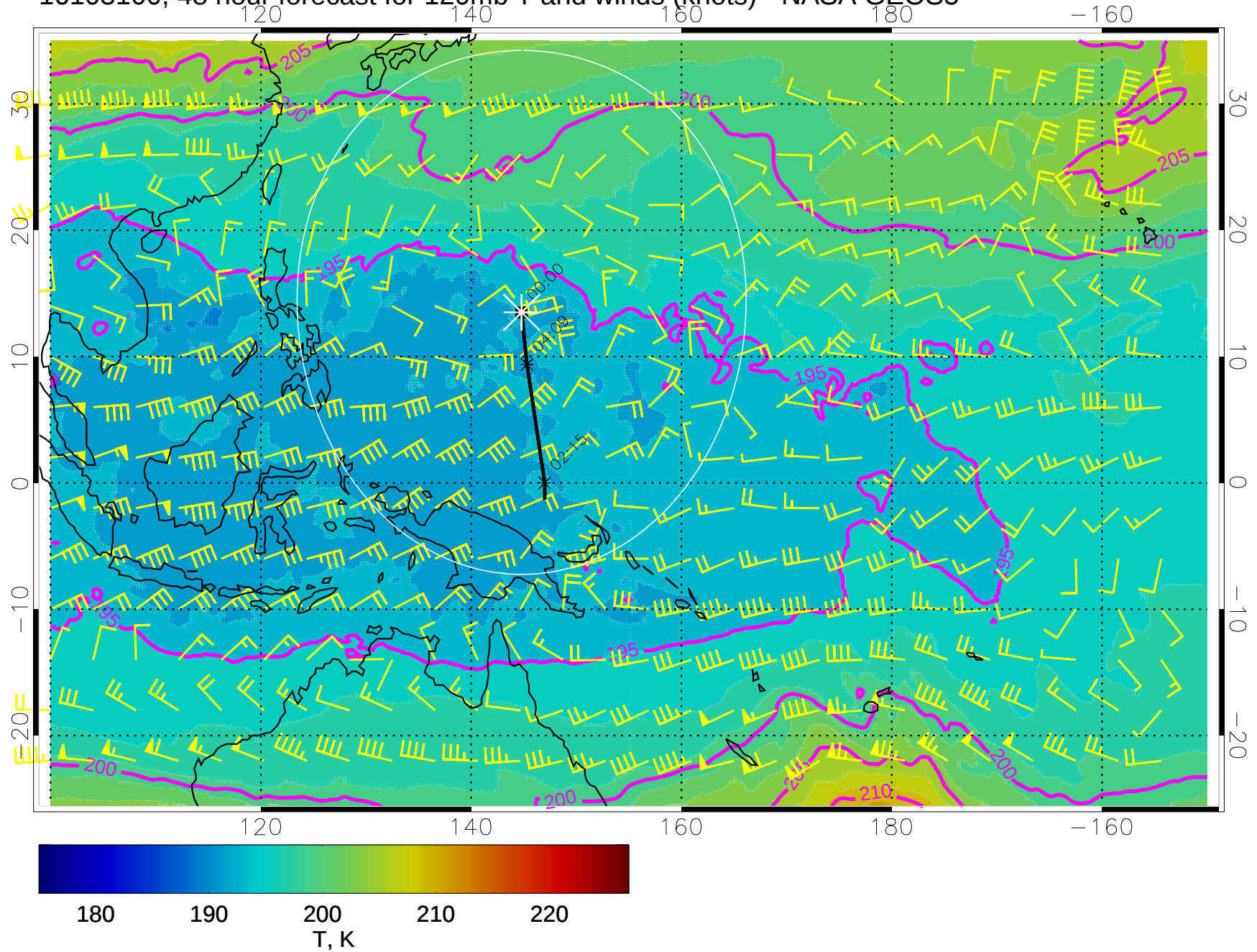
16103100, 48 hour forecast for 120mb T and winds (knots) - NASA GEOS5
