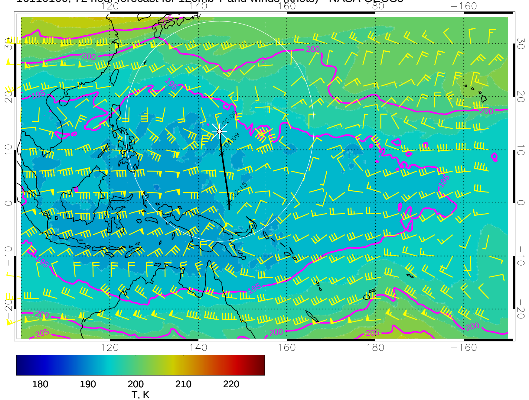
16110100, 72 hour forecast for 120mb T and winds (knots) - NASA GEOS5
