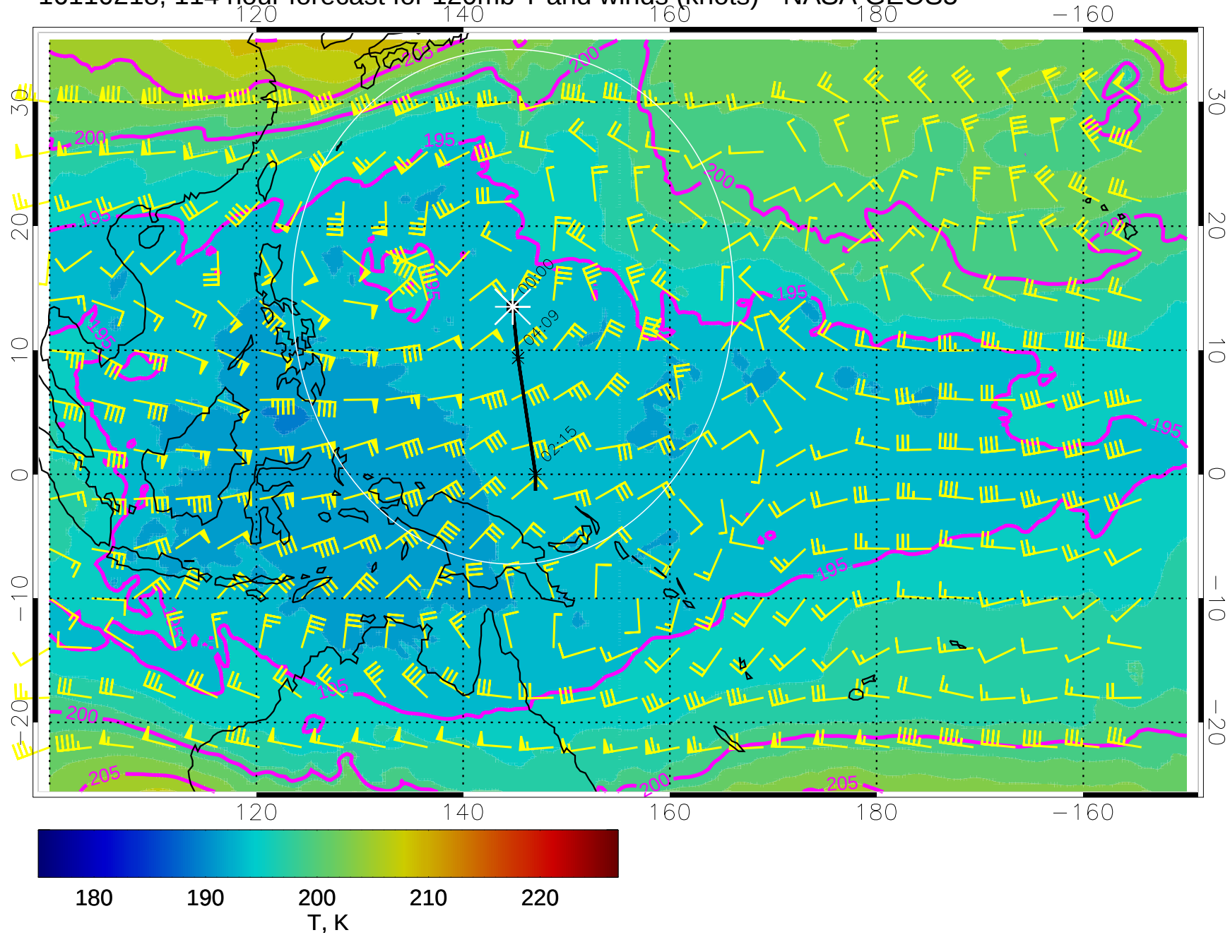
16110218, 114 hour forecast for 120mb T and winds (knots) - NASA GEOS5
