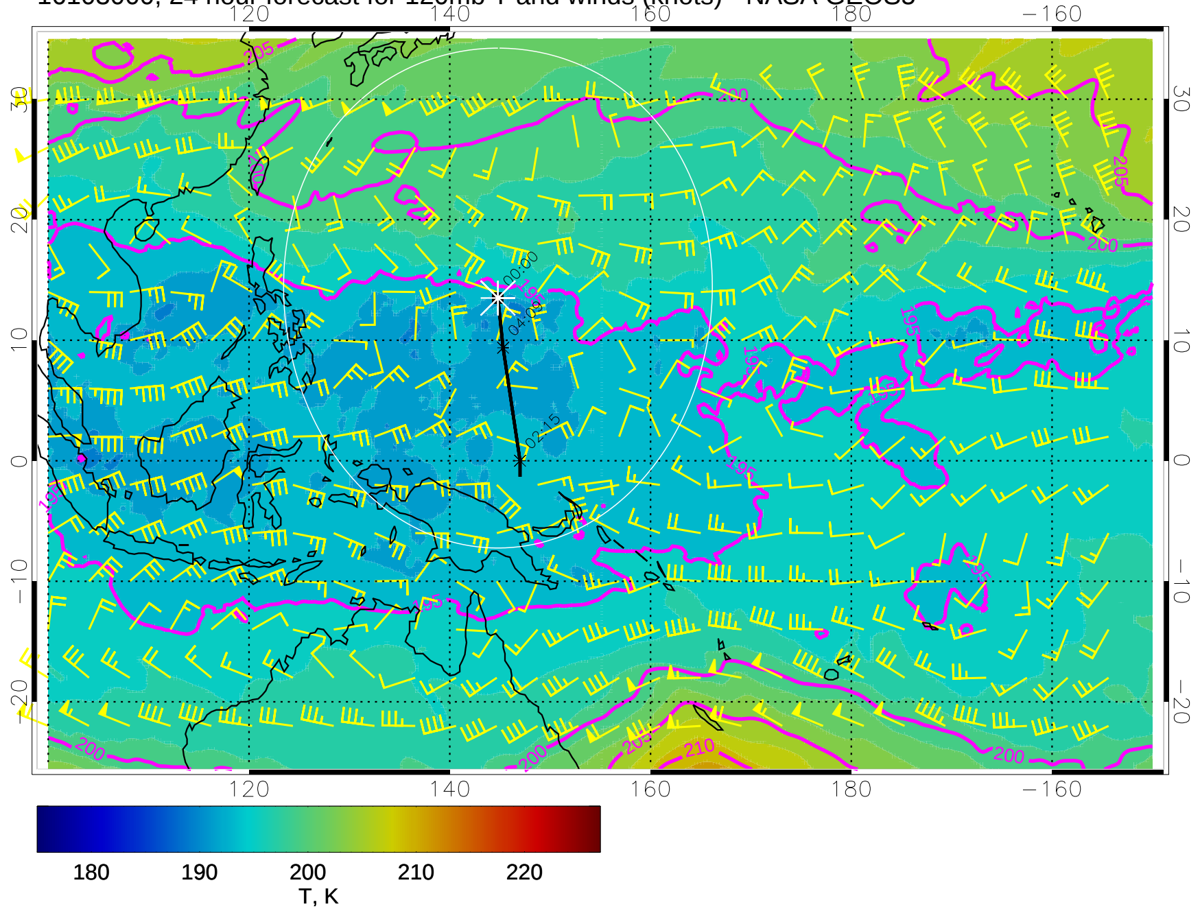
16103000, 24 hour forecast for 120mb T and winds (knots) - NASA GEOS5
