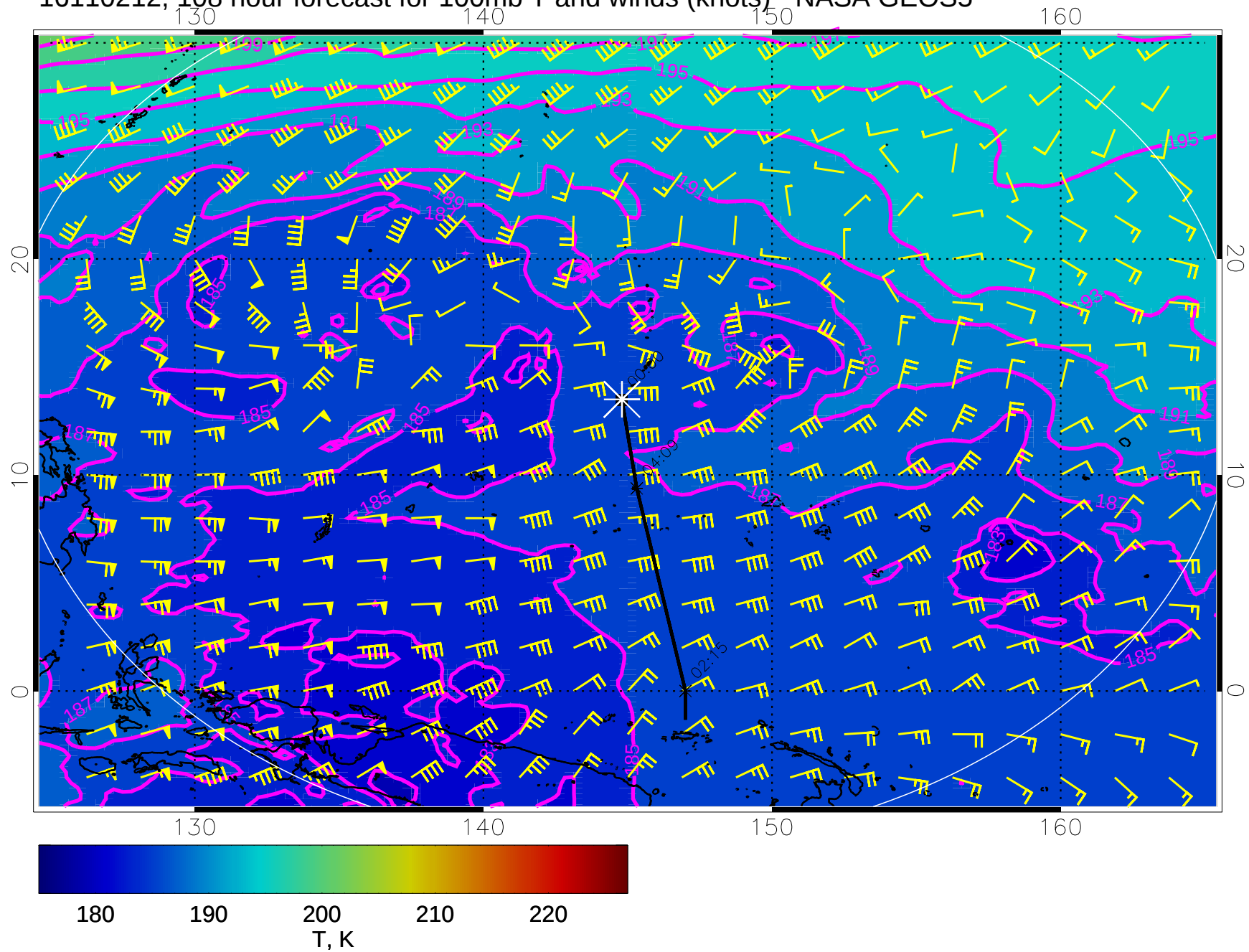
16110212, 108 hour forecast for 100mb T and winds (knots) - NASA GEOS5
