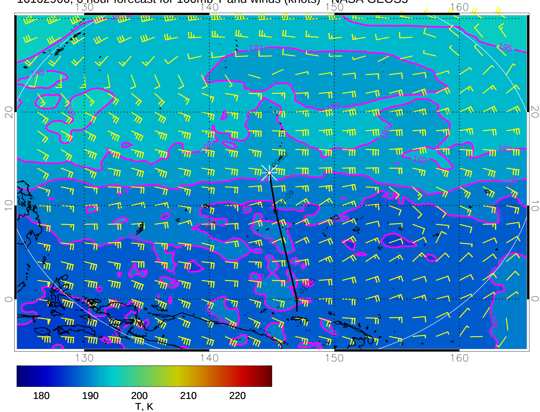
16102906, 6 hour forecast for 100mb T and winds (knots) - NASA GEOS5
