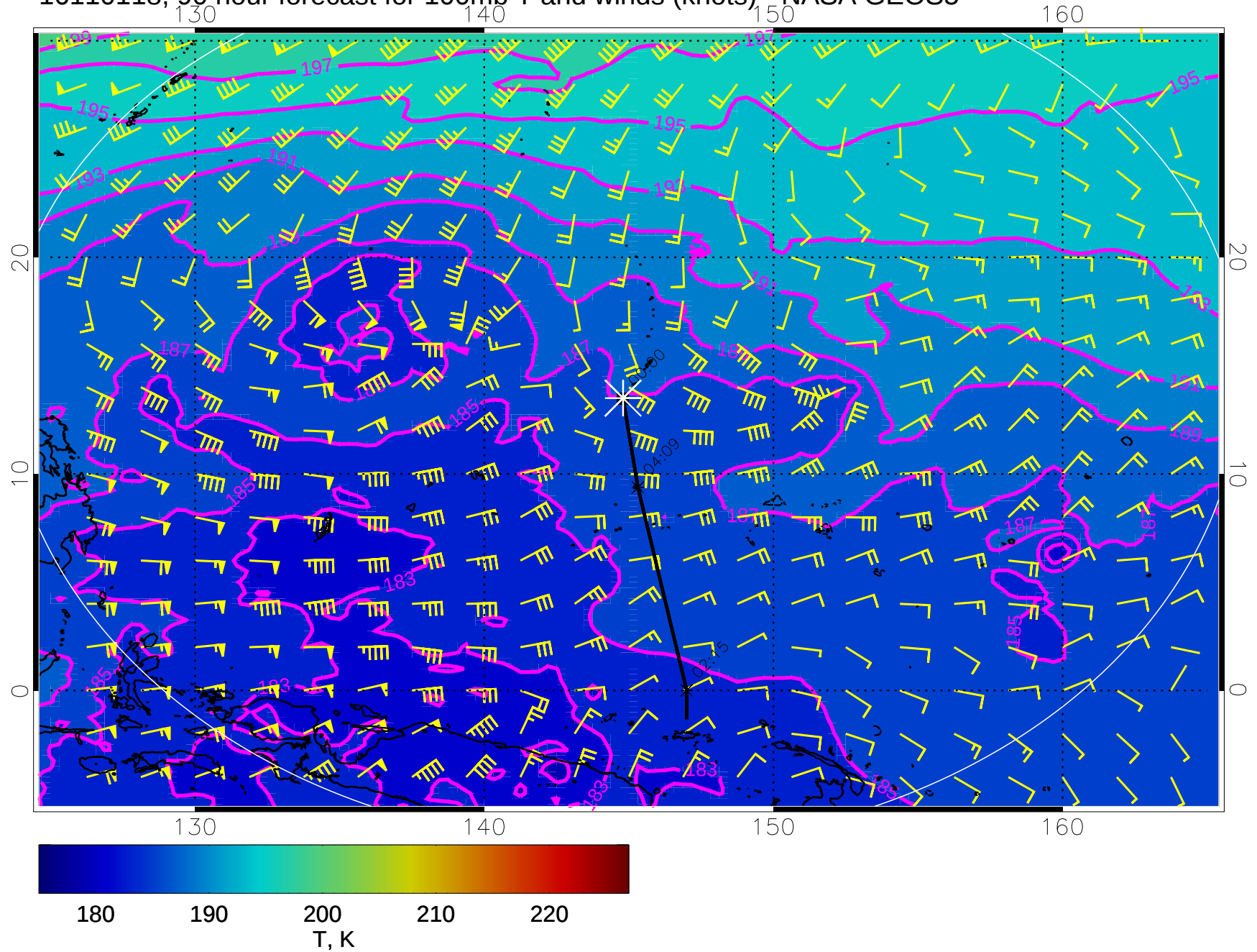
16110118, 90 hour forecast for 100mb T and winds (knots) - NASA GEOS5
