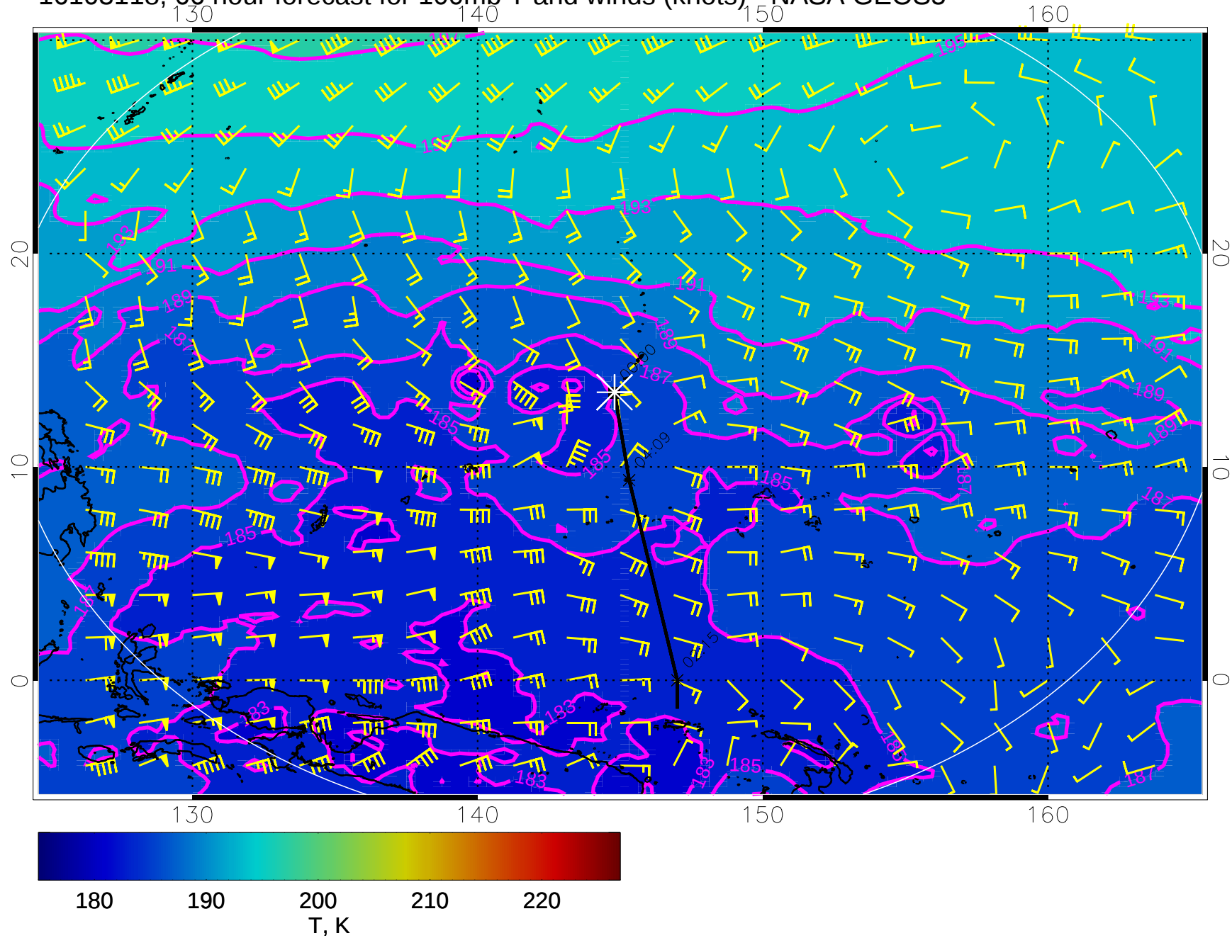
16103118, 66 hour forecast for 100mb T and winds (knots) - NASA GEOS5
