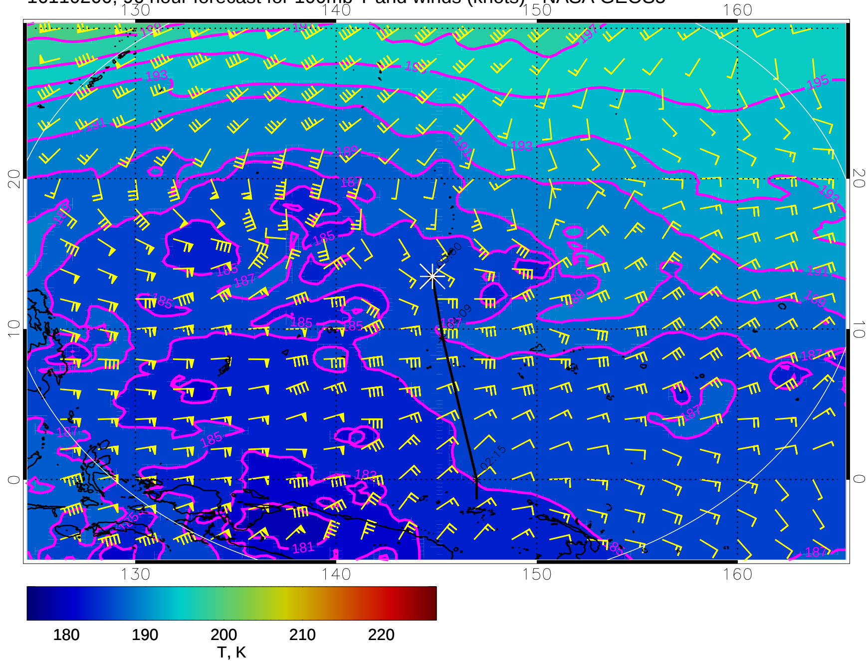
16110200, 96 hour forecast for 100mb T and winds (knots) - NASA GEOS5
