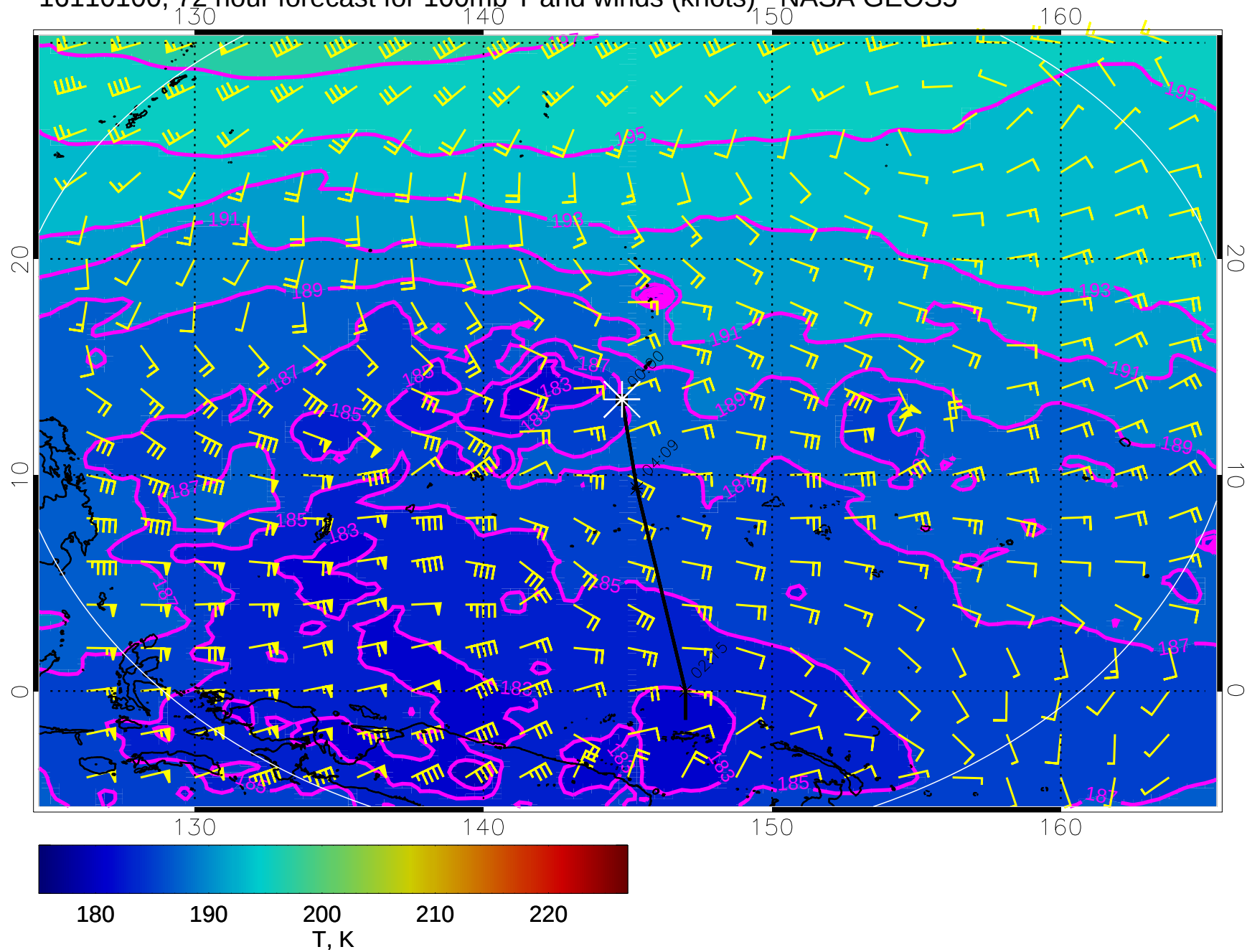
16110100, 72 hour forecast for 100mb T and winds (knots) - NASA GEOS5
