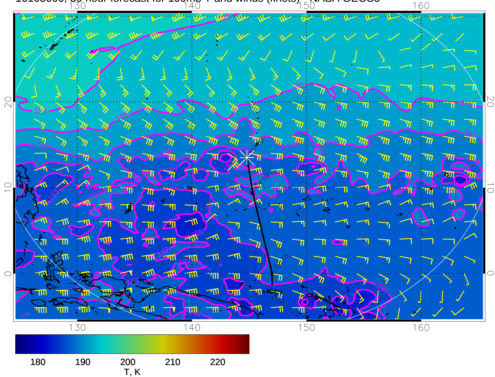
16103006, 30 hour forecast for 100mb T and winds (knots) - NASA GEOS5
