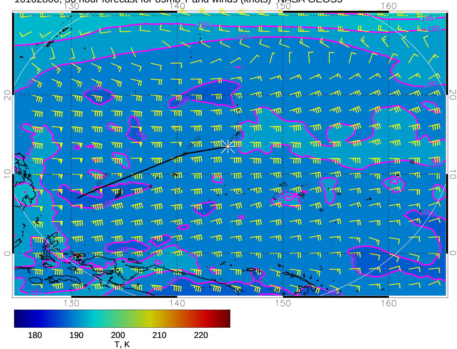
16102800, 36 hour forecast for 85mb T and winds (knots)- NASA GEOS5
