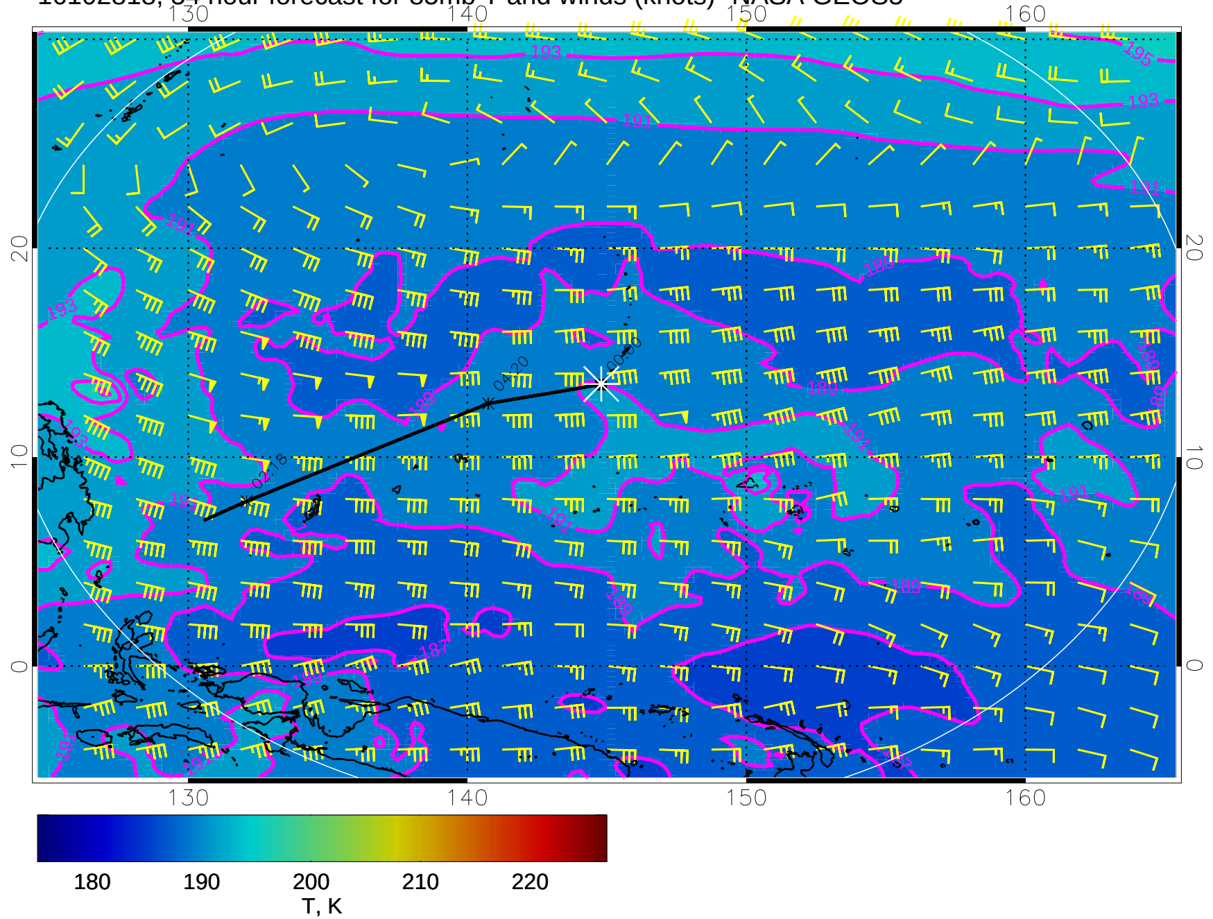
16102818, 54 hour forecast for 85mb T and winds (knots)- NASA GEOS5
