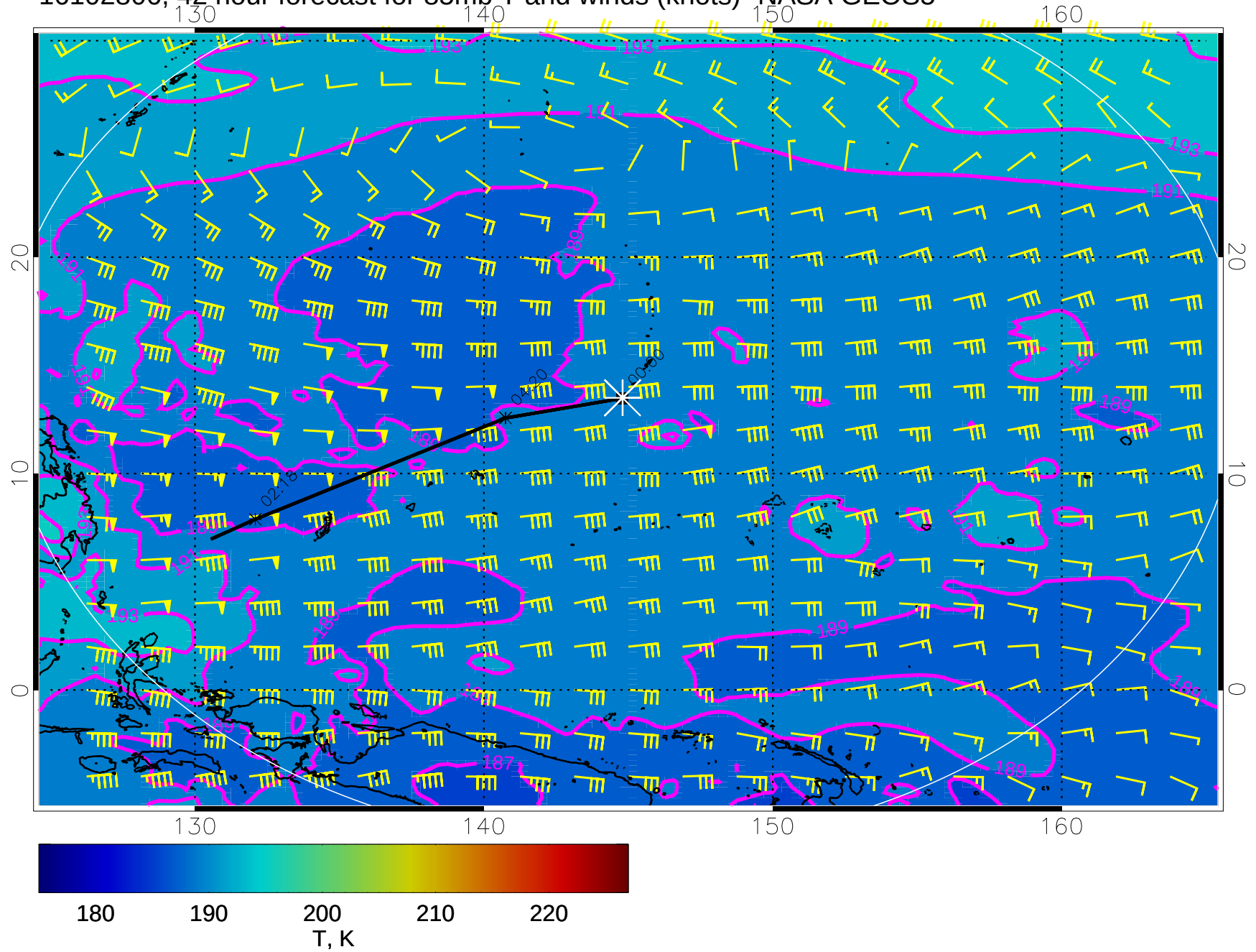
16102806, 42 hour forecast for 85mb T and winds (knots)- NASA GEOS5
