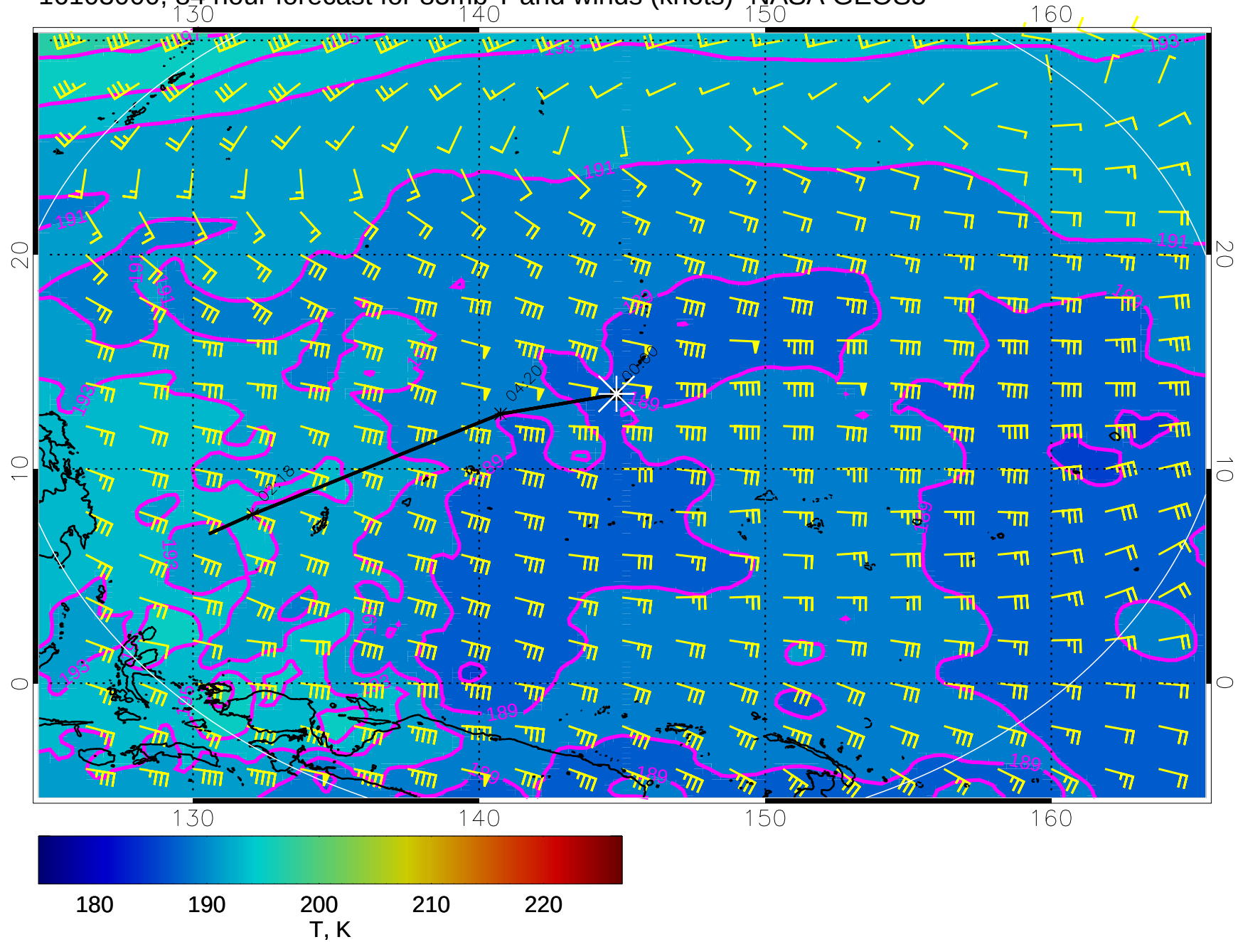
16103000, 84 hour forecast for 85mb T and winds (knots)- NASA GEOS5
