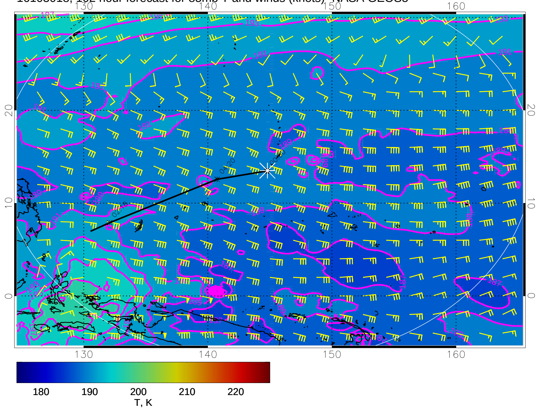
16103018, 102 hour forecast for 85mb T and winds (knots)- NASA GEOS5
