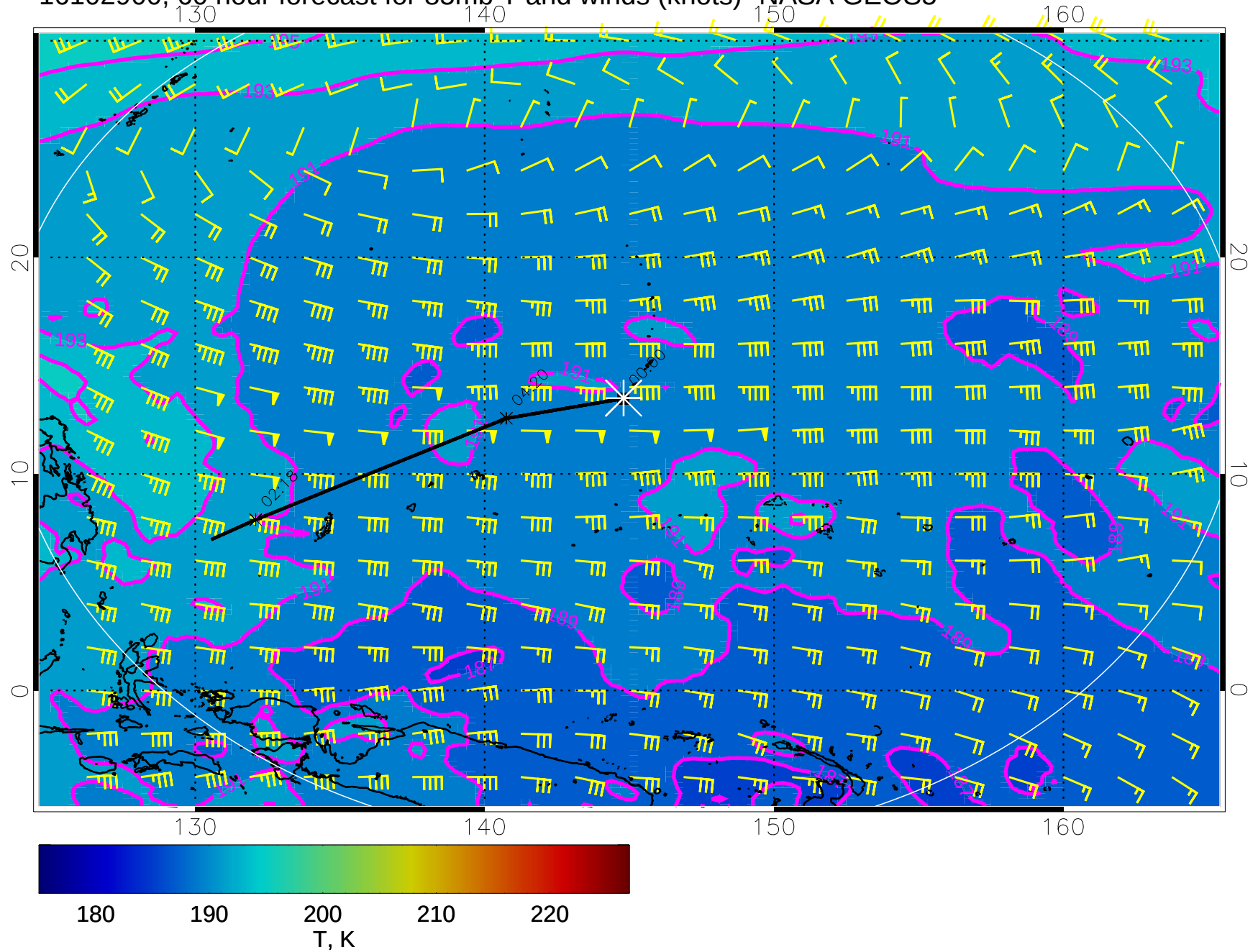
16102900, 60 hour forecast for 85mb T and winds (knots)- NASA GEOS5
