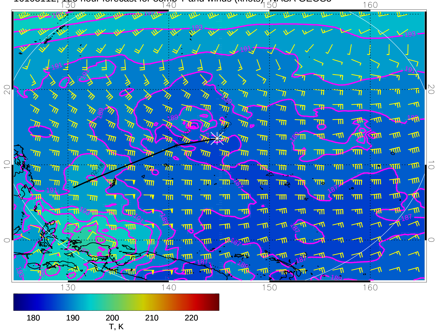
16103112, 120 hour forecast for 85mb T and winds (knots)- NASA GEOS5
