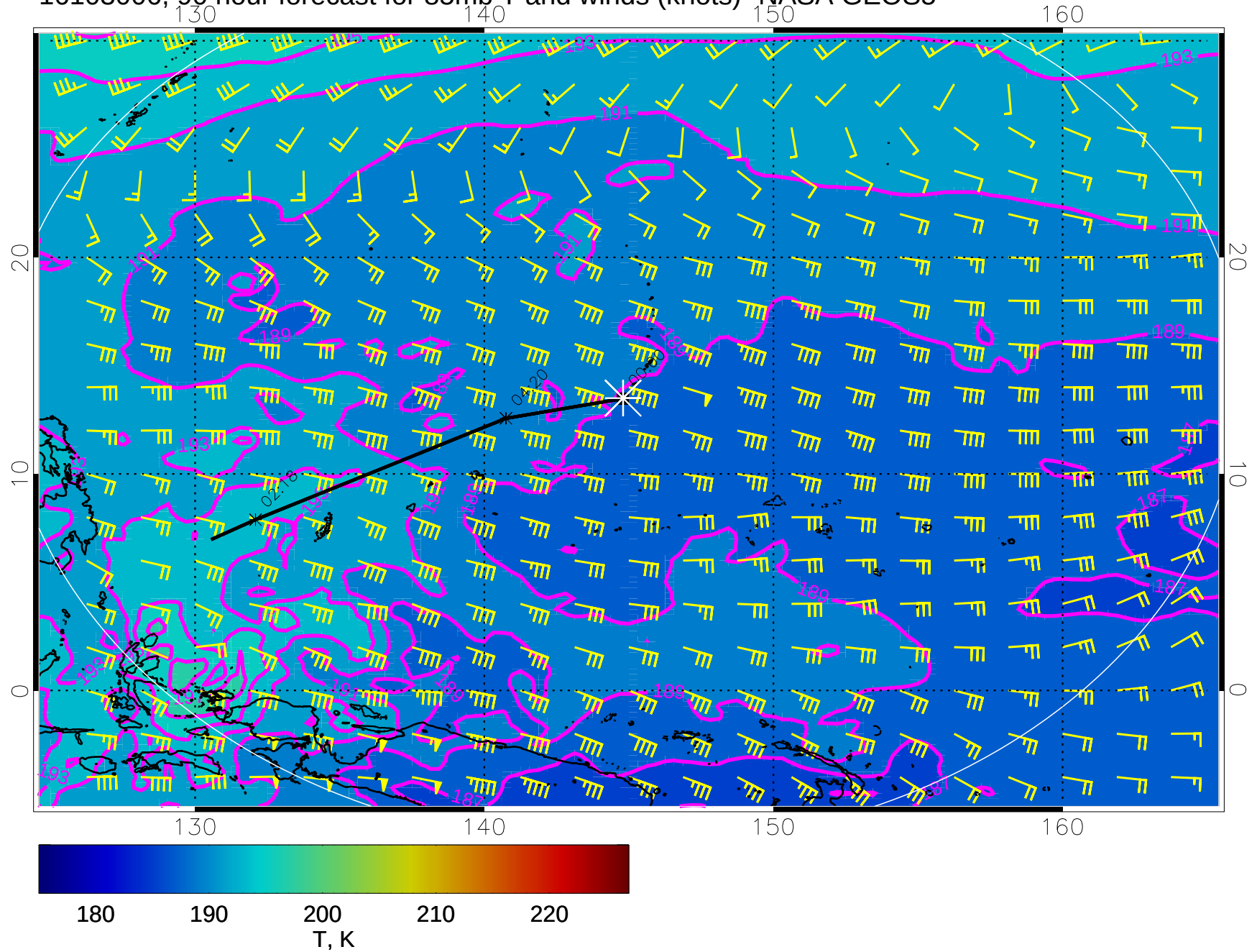
16103006, 90 hour forecast for 85mb T and winds (knots)- NASA GEOS5
