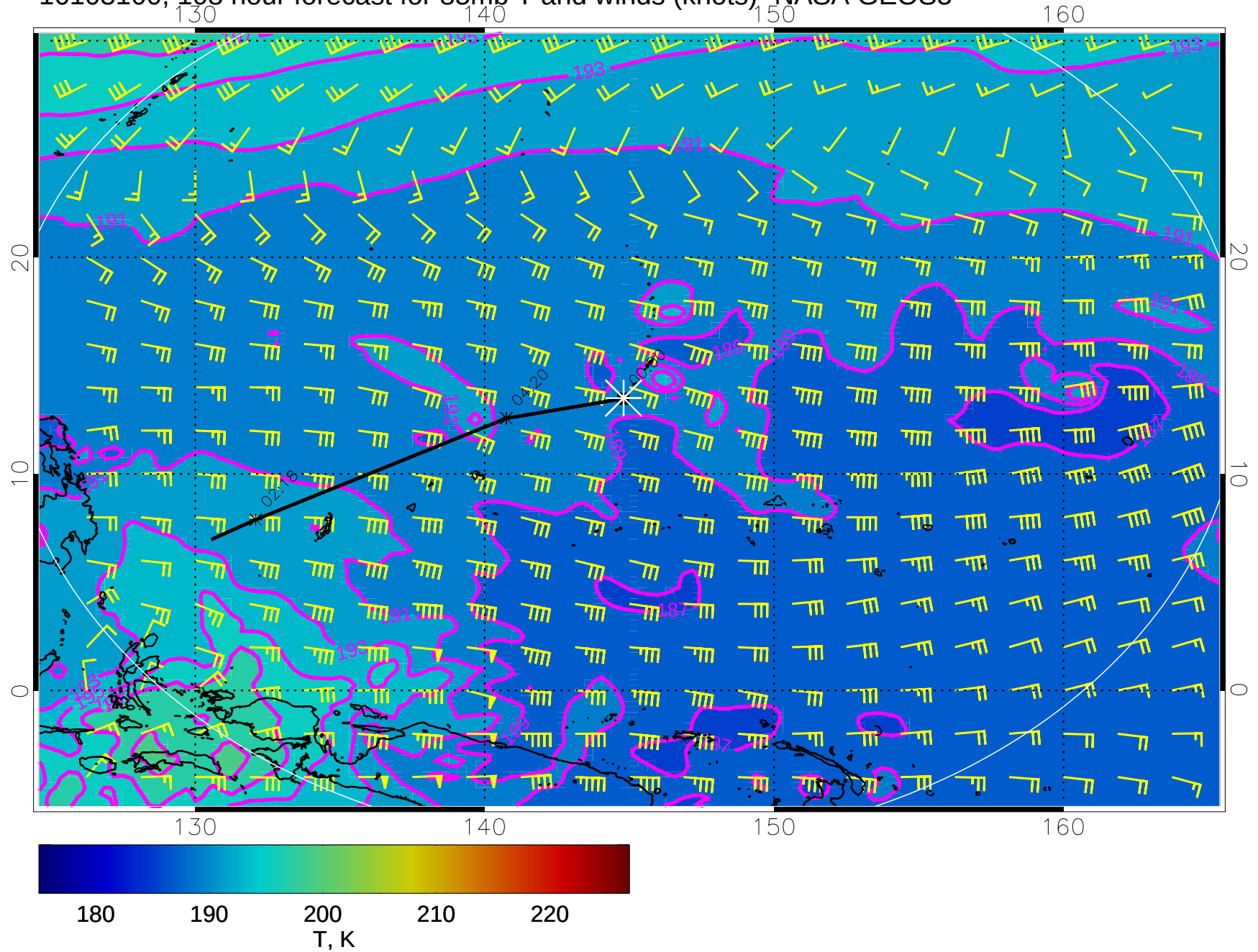
16103100, 108 hour forecast for 85mb T and winds (knots)- NASA GEOS5
