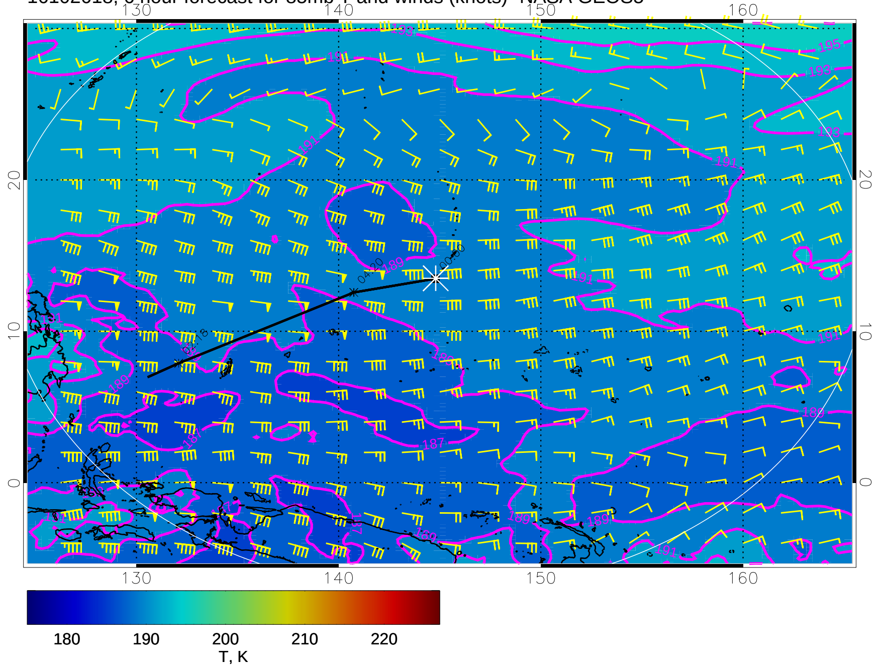
16102618, 6 hour forecast for 85mb T and winds (knots)- NASA GEOS5
