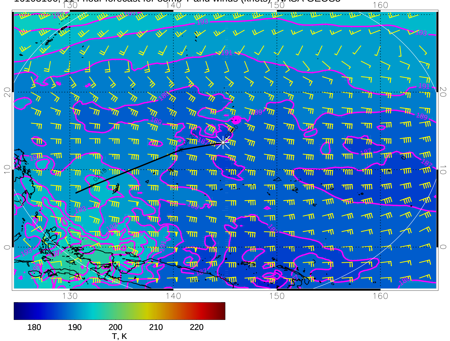
16103106, 114 hour forecast for 85mb T and winds (knots)- NASA GEOS5
