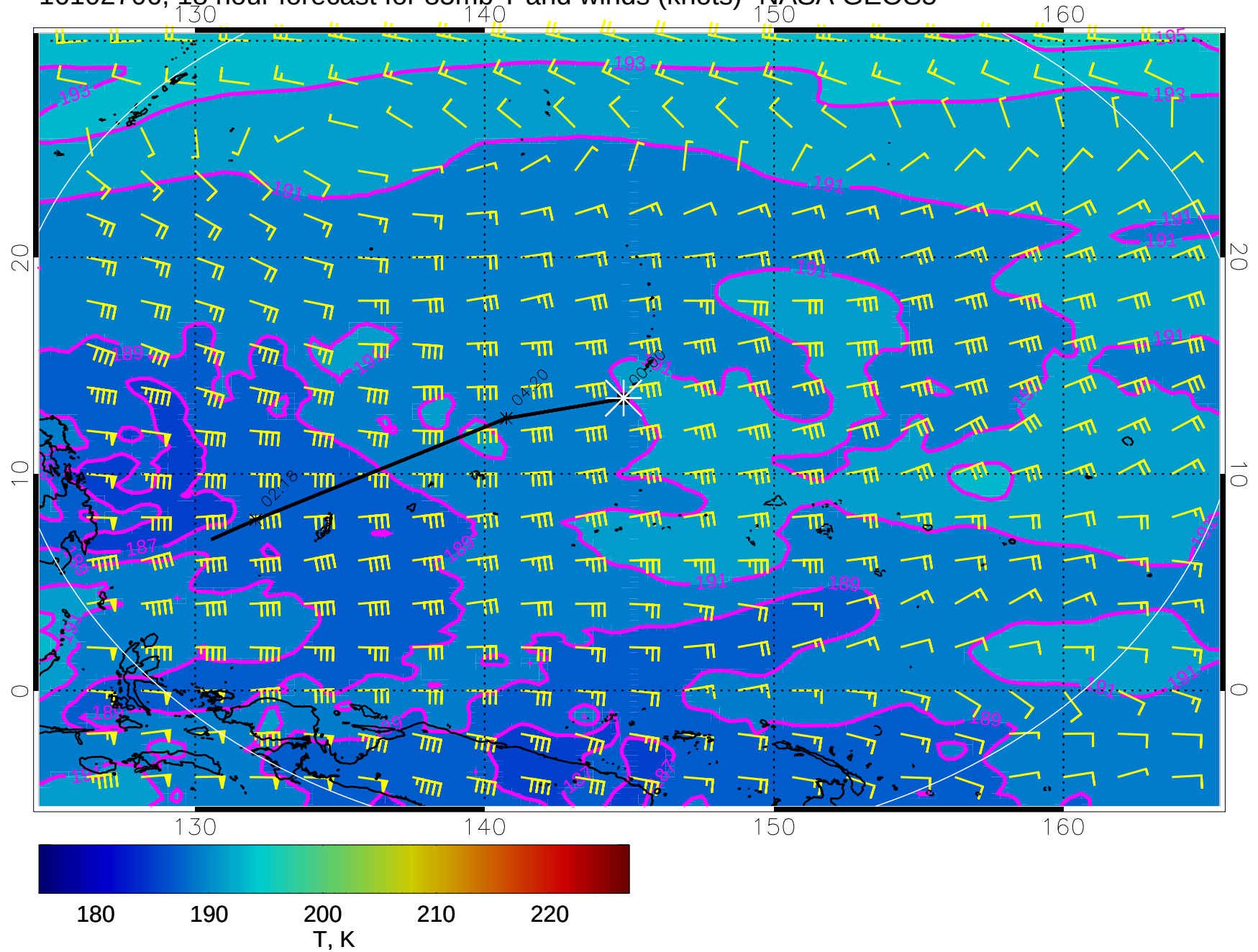
16102706, 18 hour forecast for 85mb T and winds (knots)- NASA GEOS5
