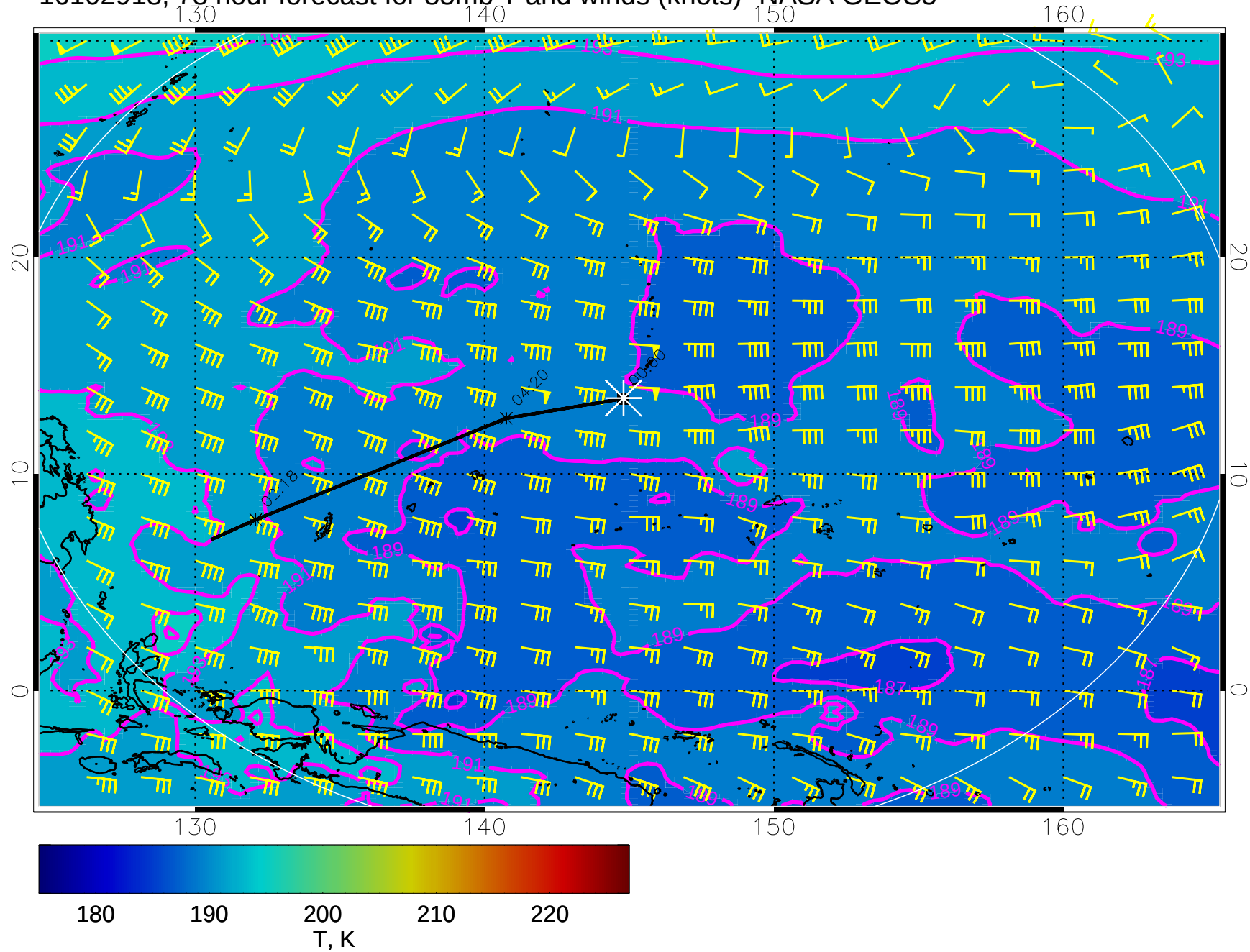
16102918, 78 hour forecast for 85mb T and winds (knots)- NASA GEOS5
