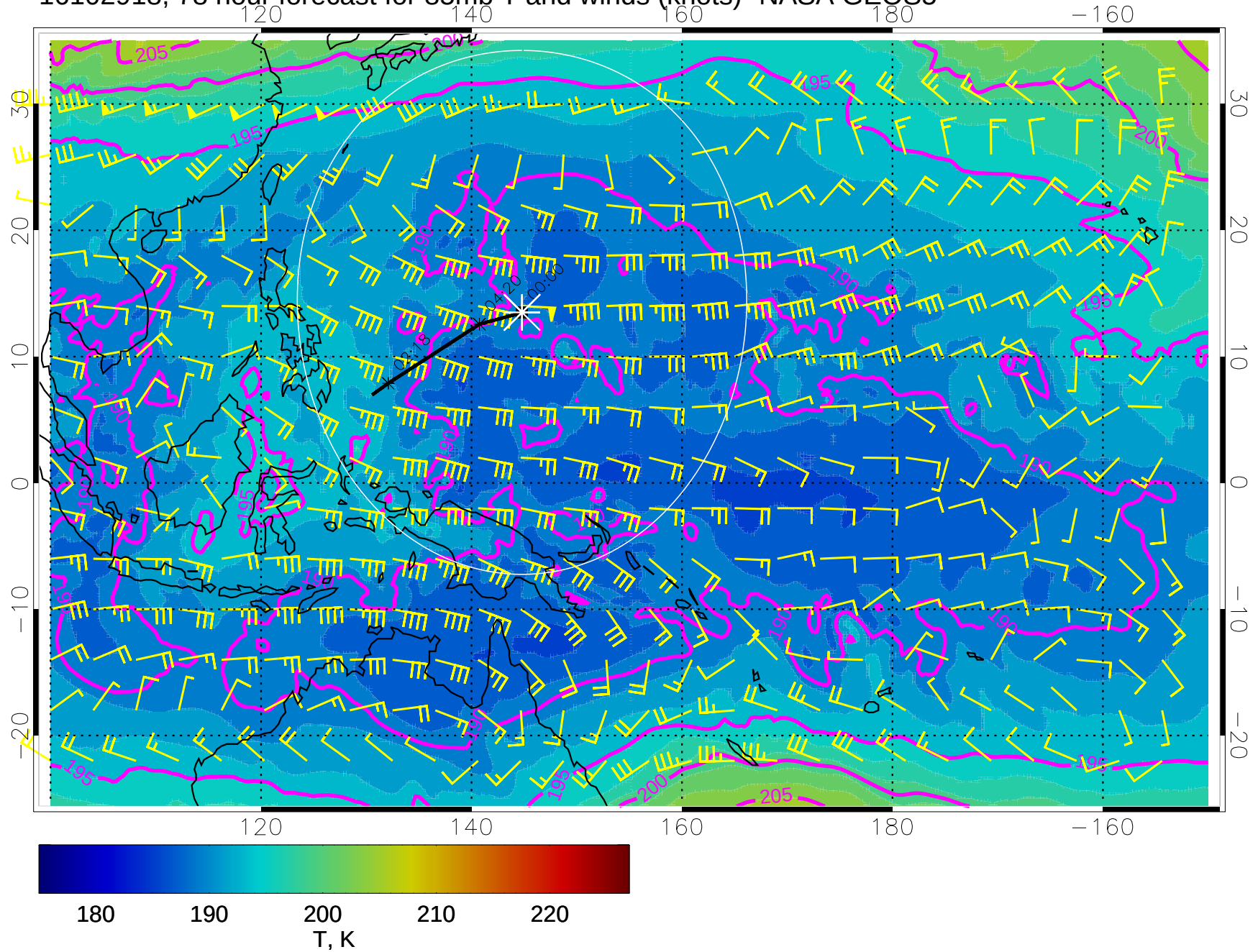
16102918, 78 hour forecast for 85mb T and winds (knots)- NASA GEOS5
