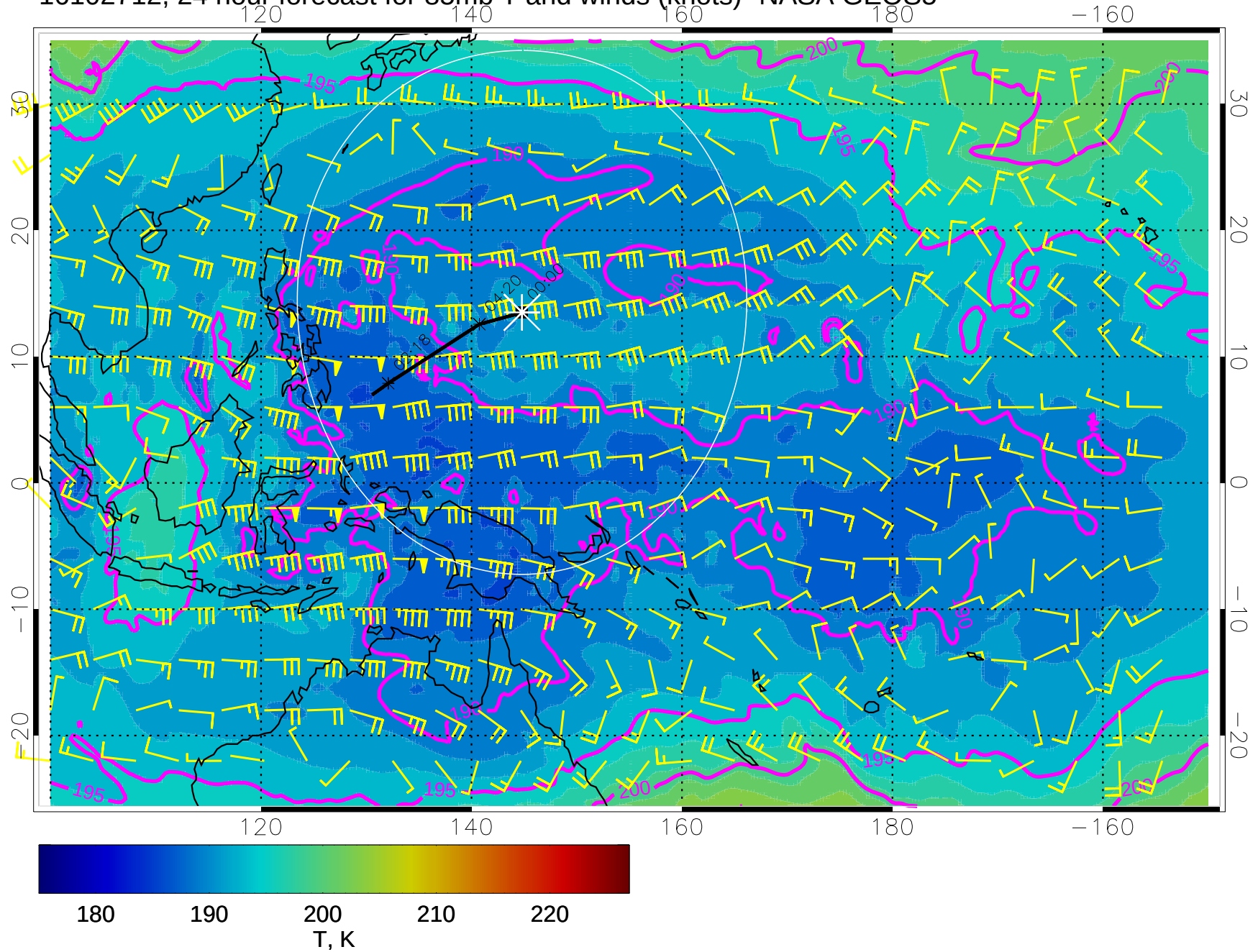
16102712, 24 hour forecast for 85mb T and winds (knots)- NASA GEOS5
