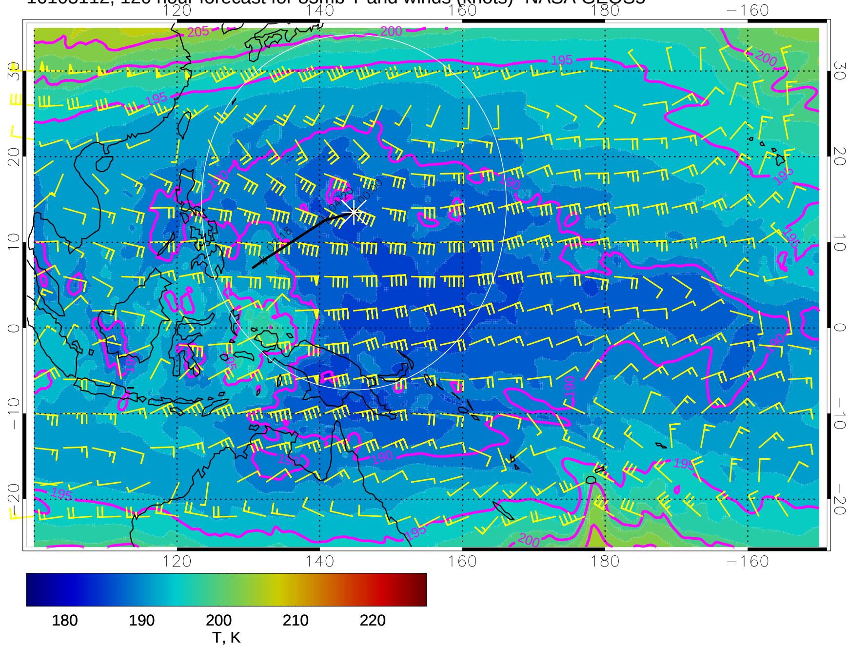
16103112, 120 hour forecast for 85mb T and winds (knots)- NASA GEOS5
