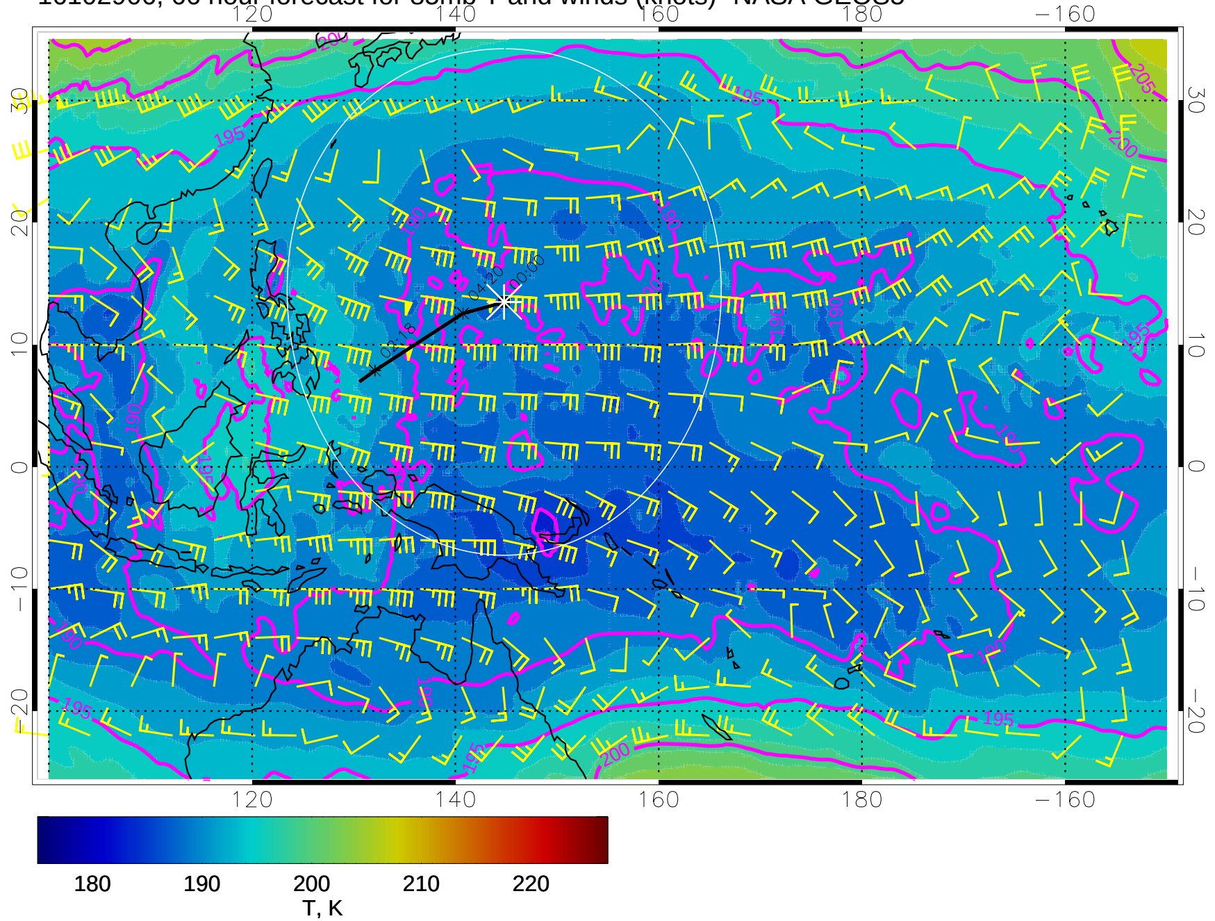
16102906, 66 hour forecast for 85mb T and winds (knots)- NASA GEOS5
