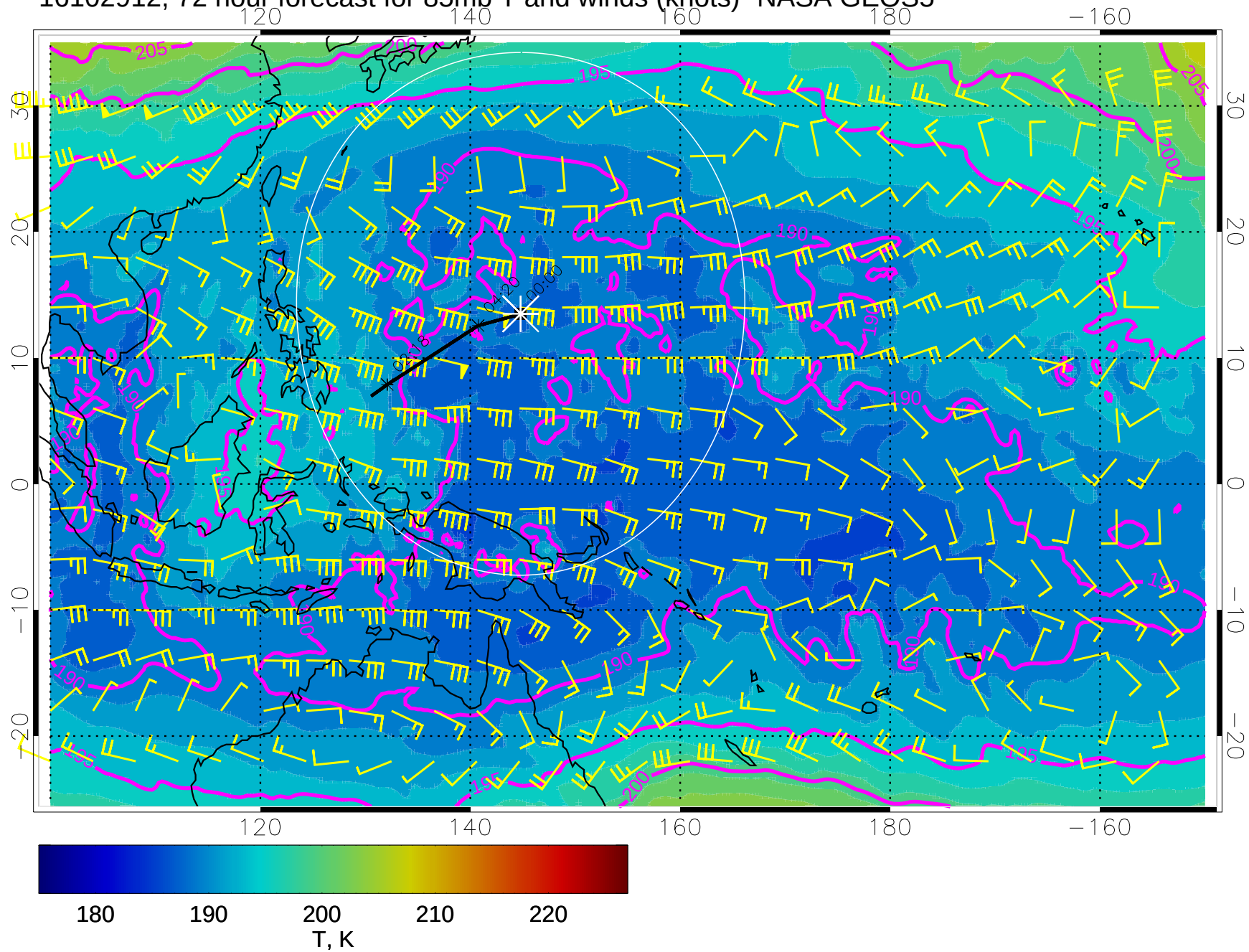
16102912, 72 hour forecast for 85mb T and winds (knots)- NASA GEOS5
