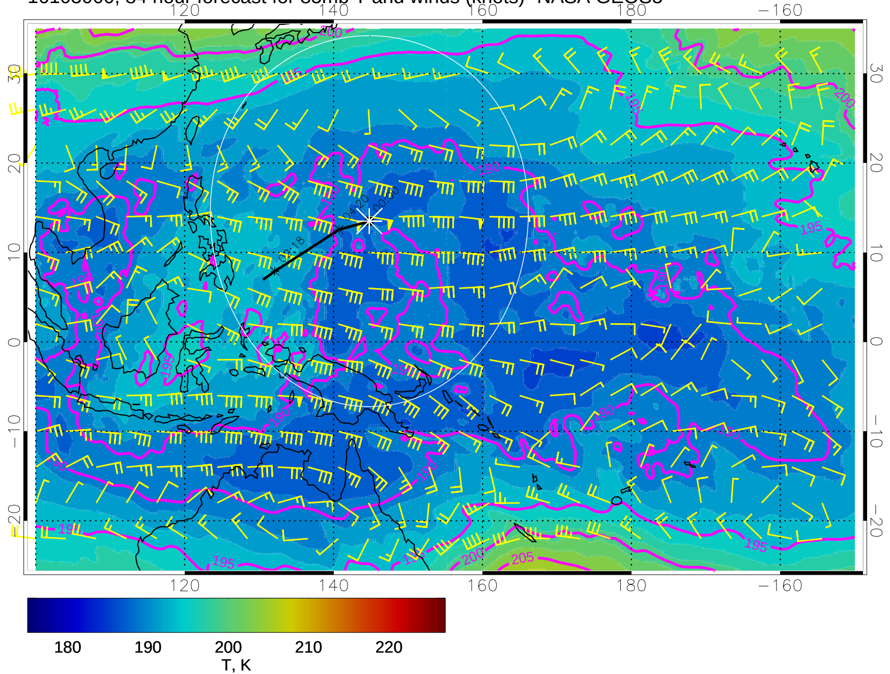
16103000, 84 hour forecast for 85mb T and winds (knots)- NASA GEOS5
