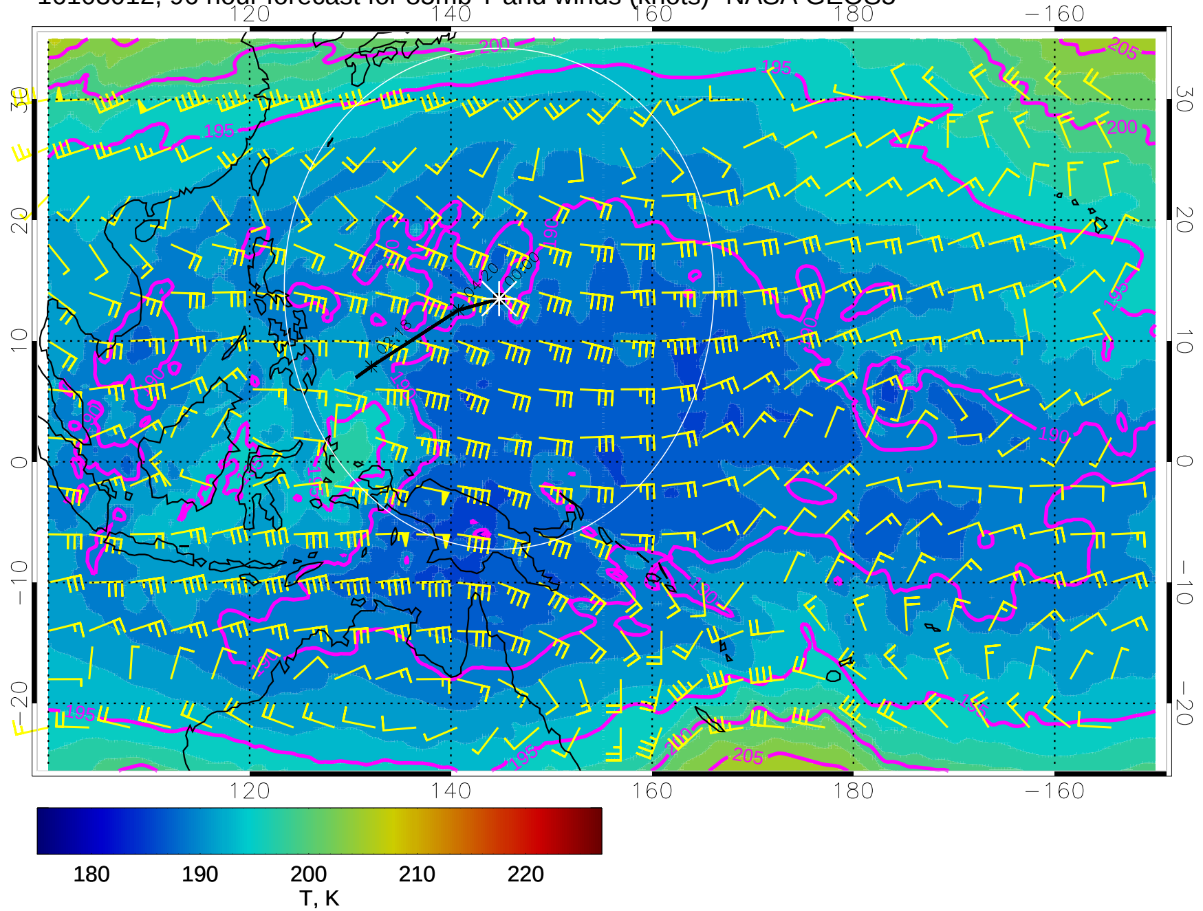
16103012, 96 hour forecast for 85mb T and winds (knots)- NASA GEOS5
