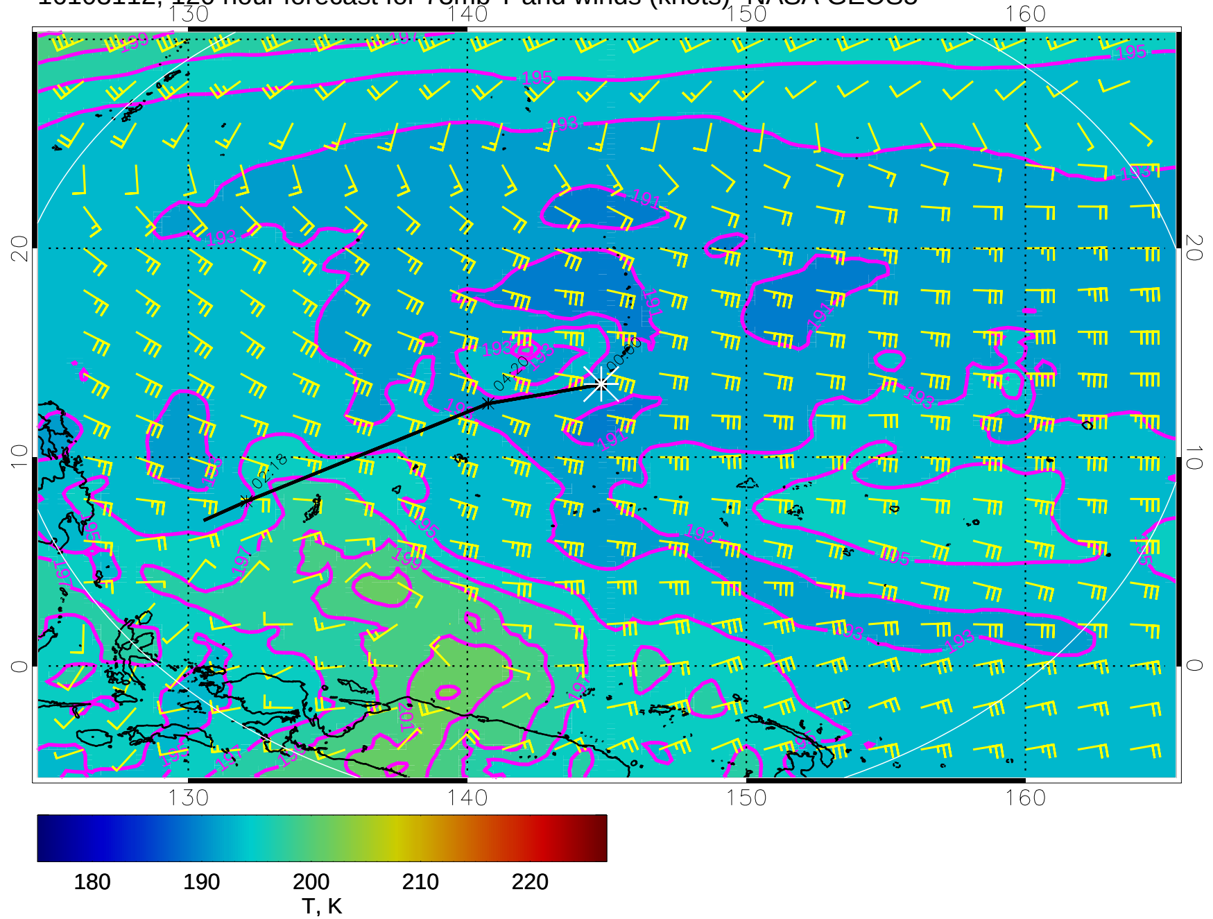
16103112, 120 hour forecast for 73mb T and winds (knots)- NASA GEOS5
