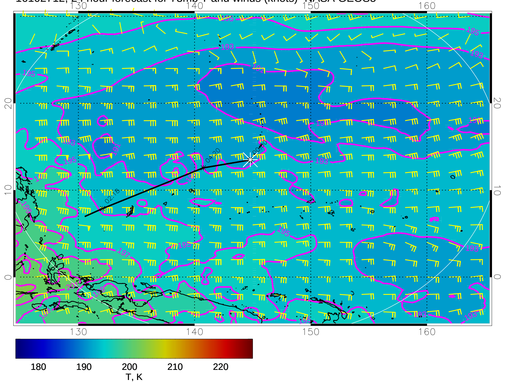
16102712, 24 hour forecast for 73mb T and winds (knots)- NASA GEOS5
