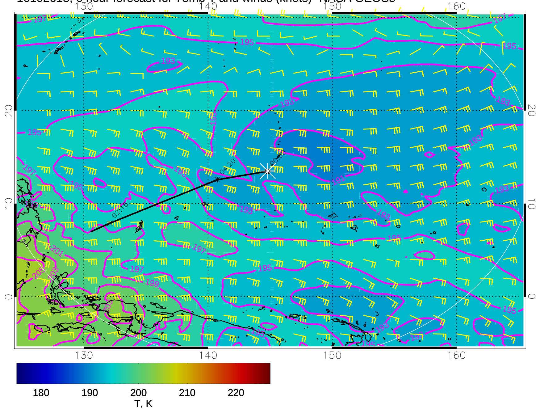
16102618, 6 hour forecast for 73mb T and winds (knots)- NASA GEOS5
