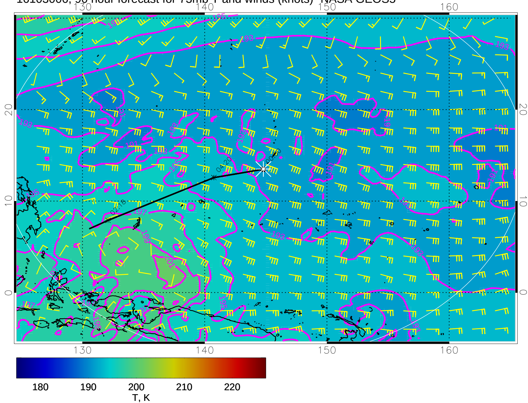
16103006, 90 hour forecast for 73mb T and winds (knots)- NASA GEOS5
