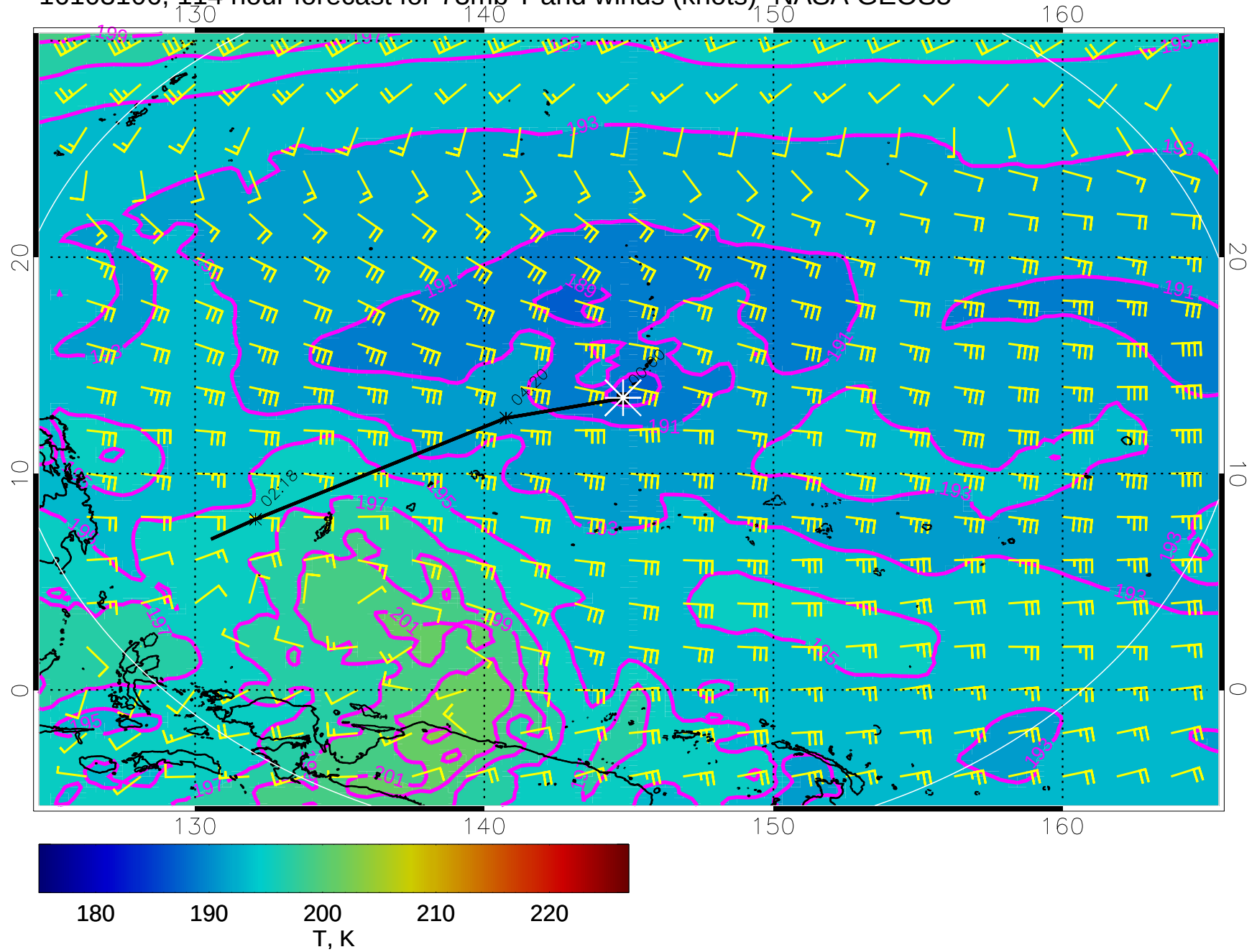
16103106, 114 hour forecast for 73mb T and winds (knots)- NASA GEOS5
