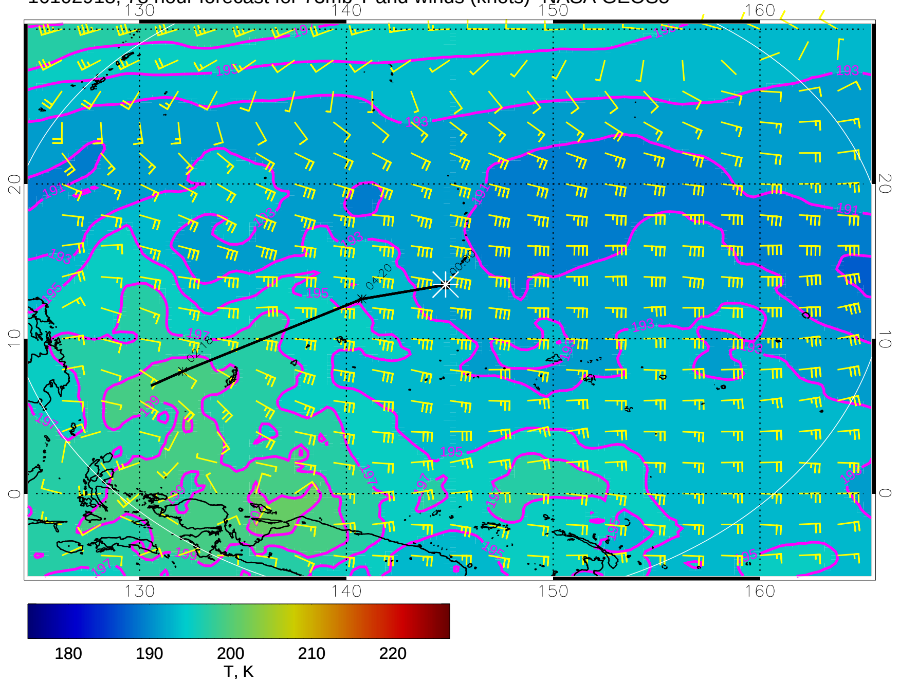
16102918, 78 hour forecast for 73mb T and winds (knots)- NASA GEOS5
