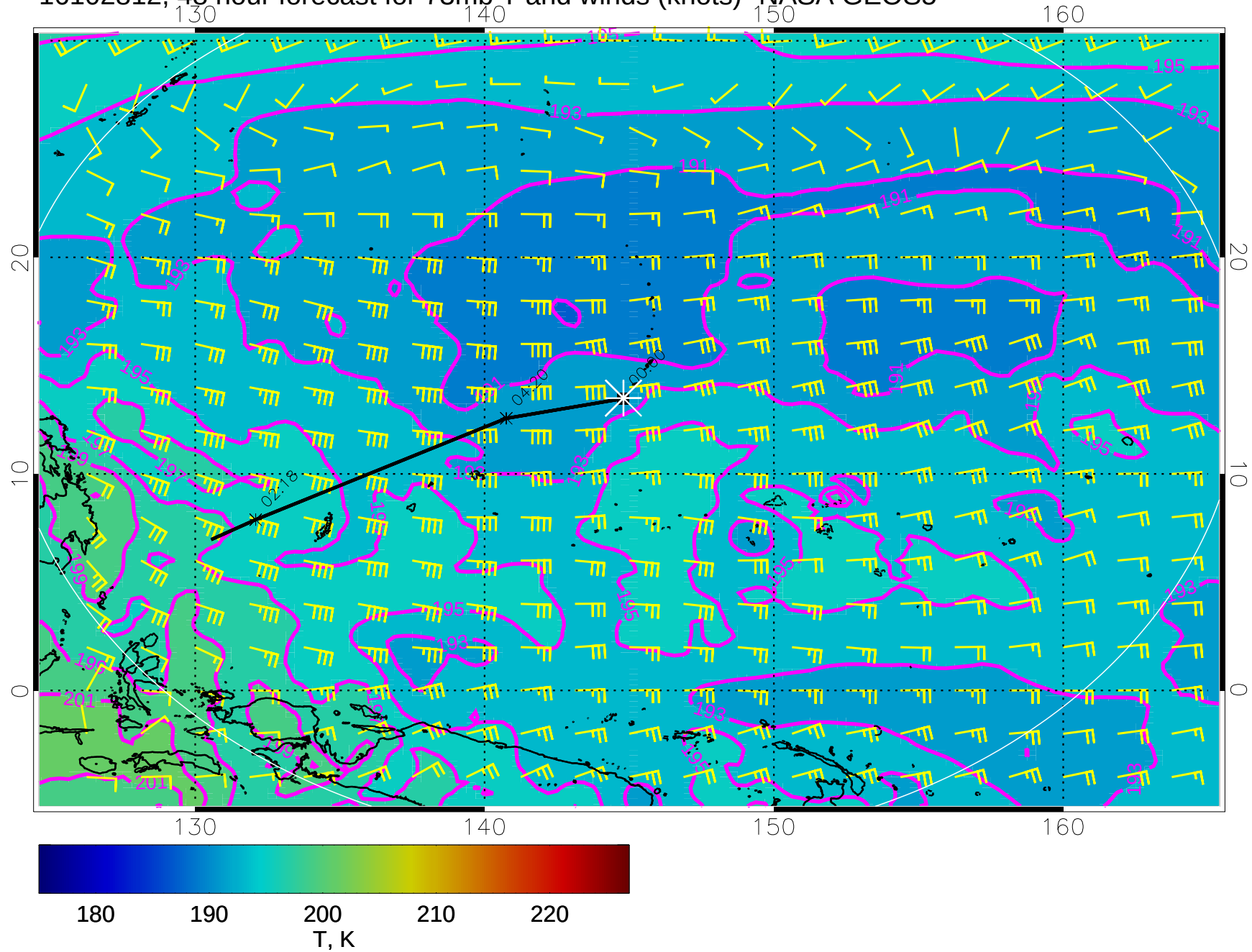
16102812, 48 hour forecast for 73mb T and winds (knots)- NASA GEOS5
