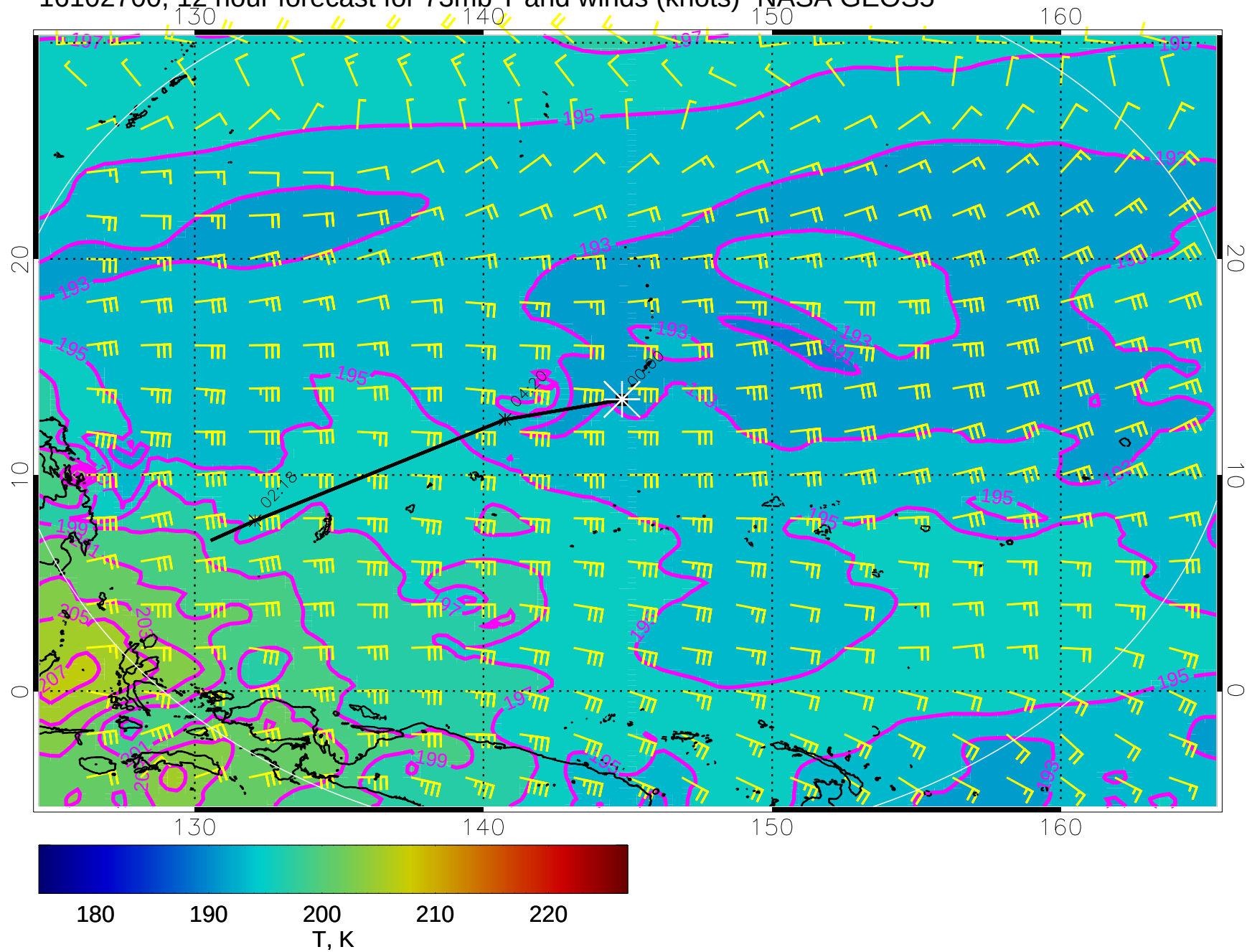
16102700, 12 hour forecast for 73mb T and winds (knots)- NASA GEOS5
