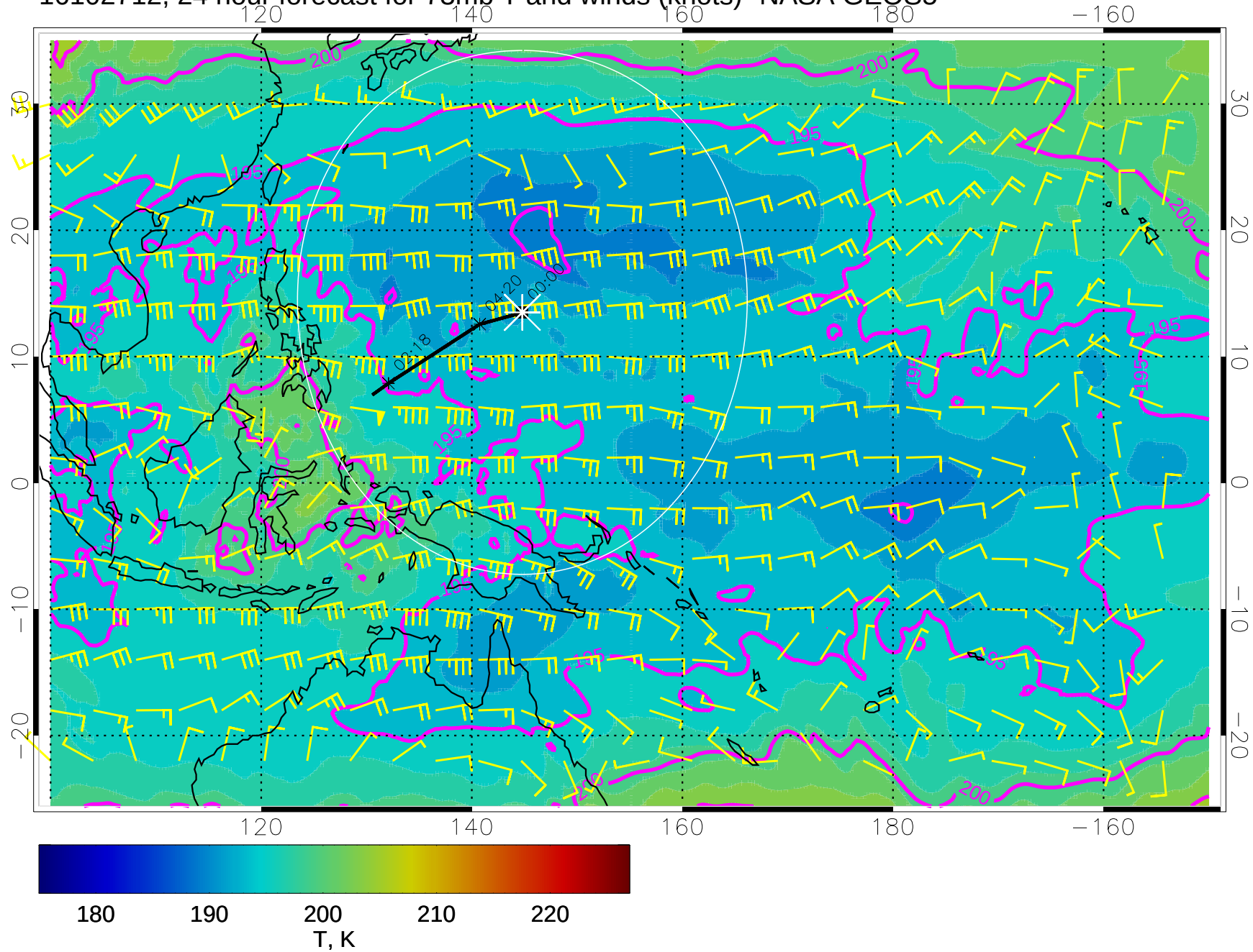
16102712, 24 hour forecast for 73mb T and winds (knots)- NASA GEOS5
