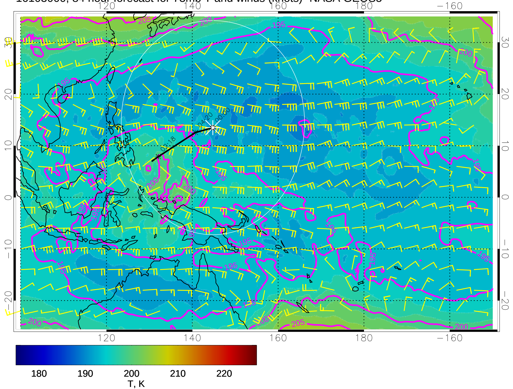
16103000, 84 hour forecast for 73mb T and winds (knots)- NASA GEOS5
