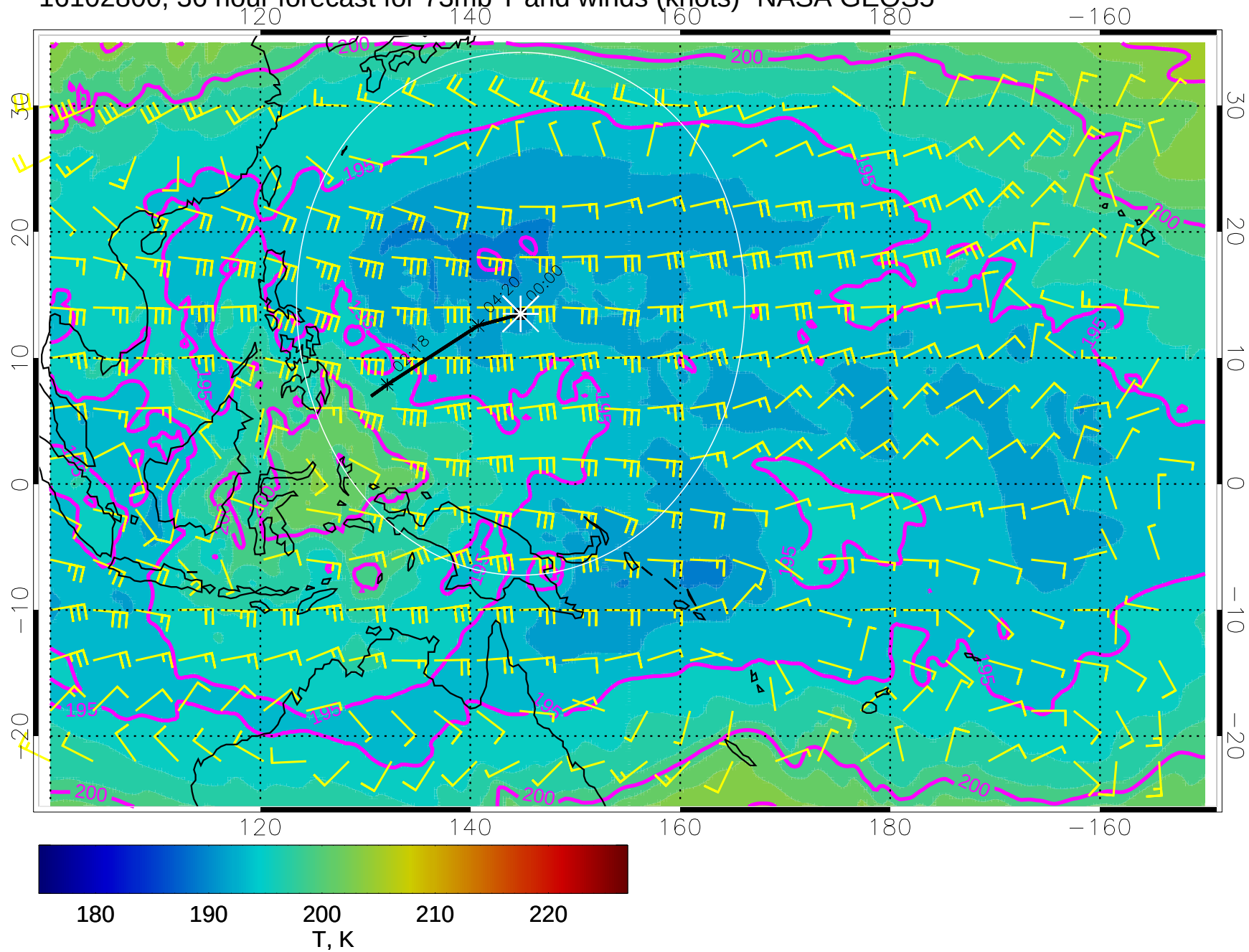
16102800, 36 hour forecast for 73mb T and winds (knots)- NASA GEOS5
