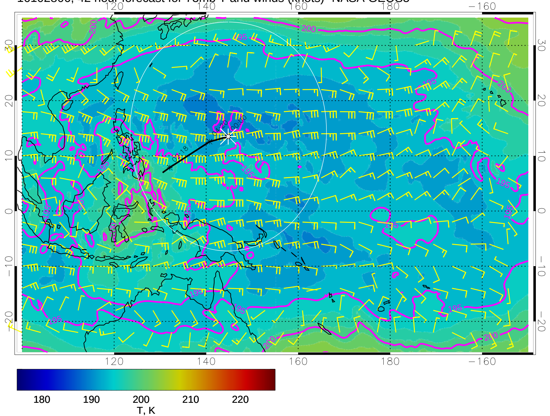
16102806, 42 hour forecast for 73mb T and winds (knots)- NASA GEOS5
