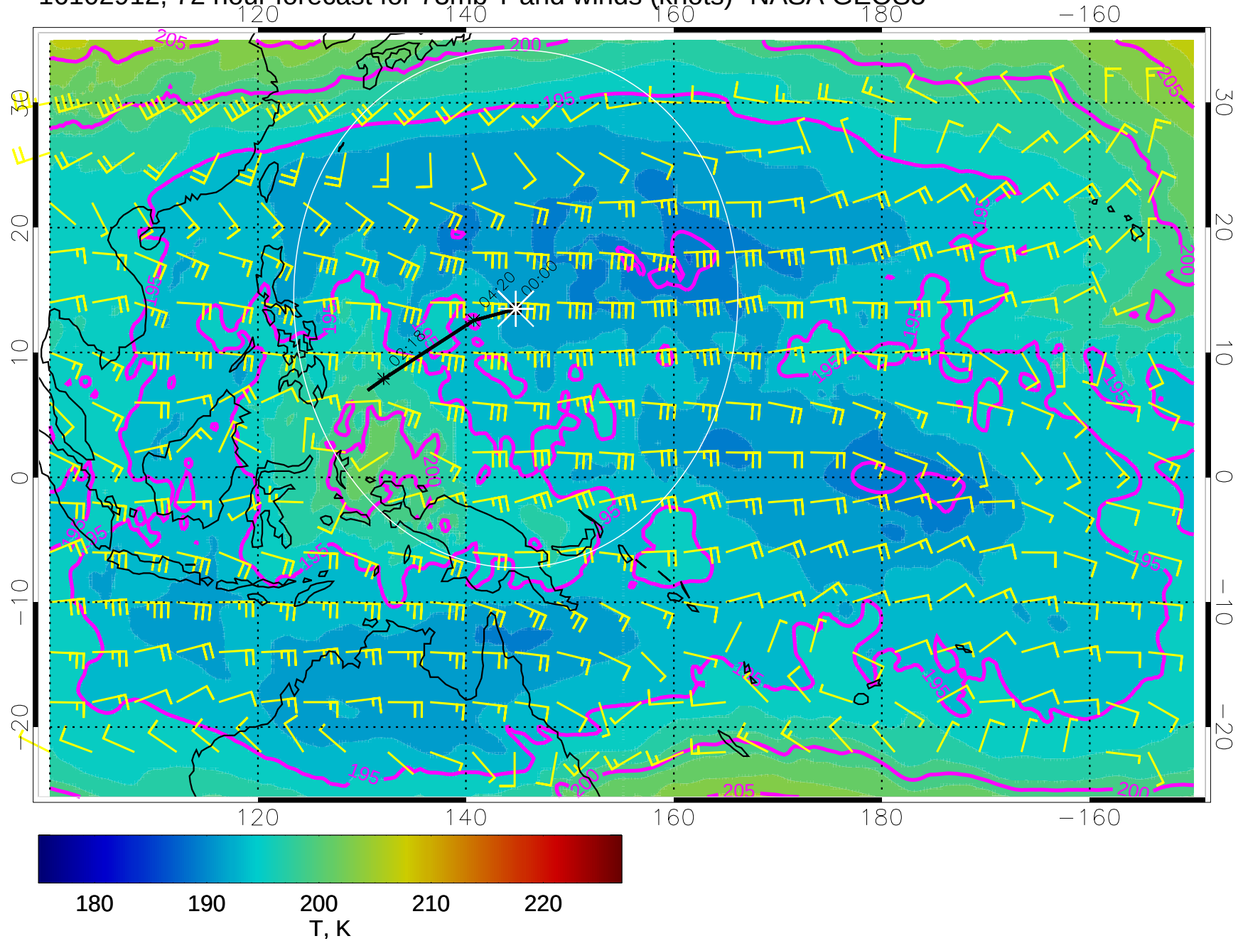
16102912, 72 hour forecast for 73mb T and winds (knots)- NASA GEOS5
