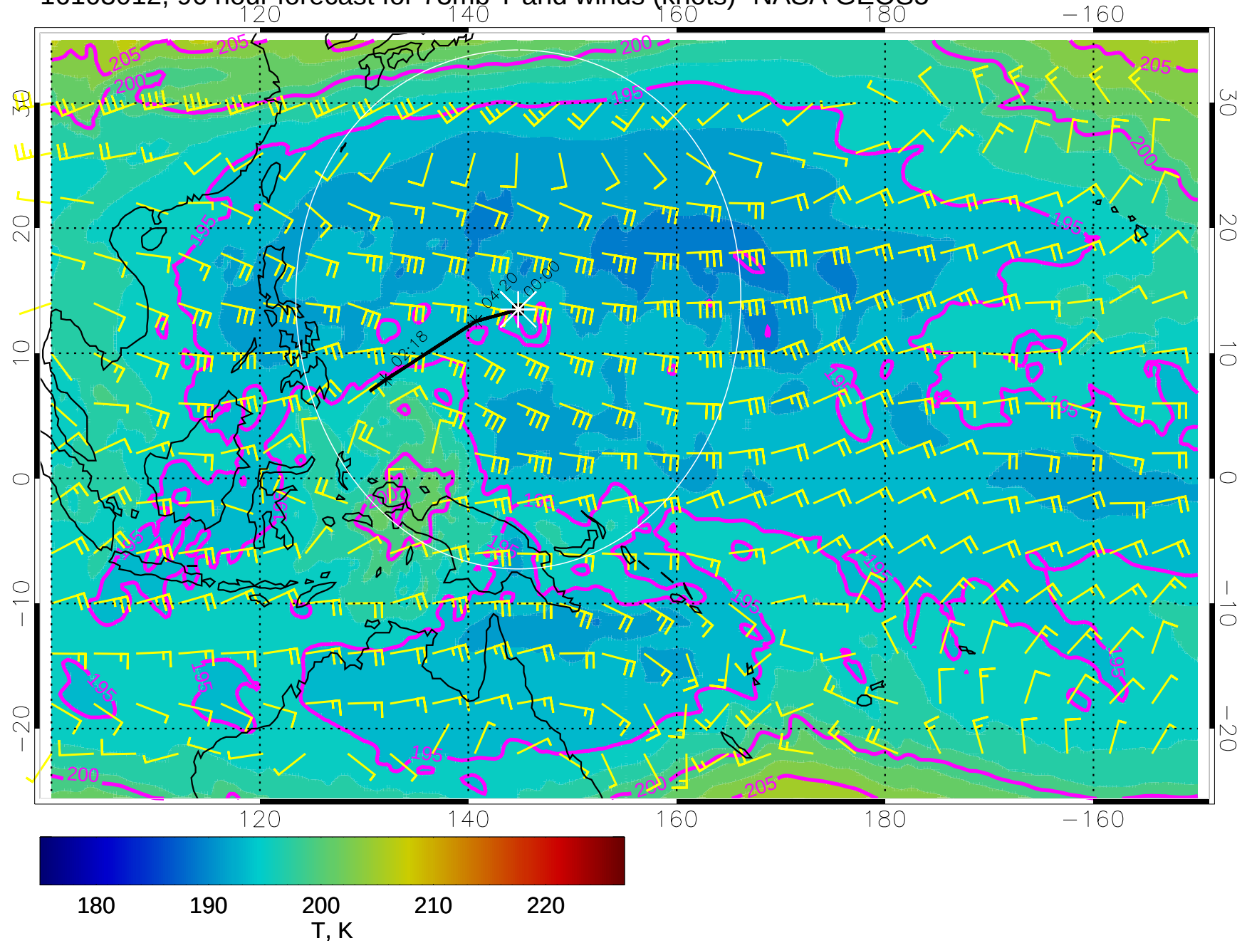
16103012, 96 hour forecast for 73mb T and winds (knots)- NASA GEOS5
