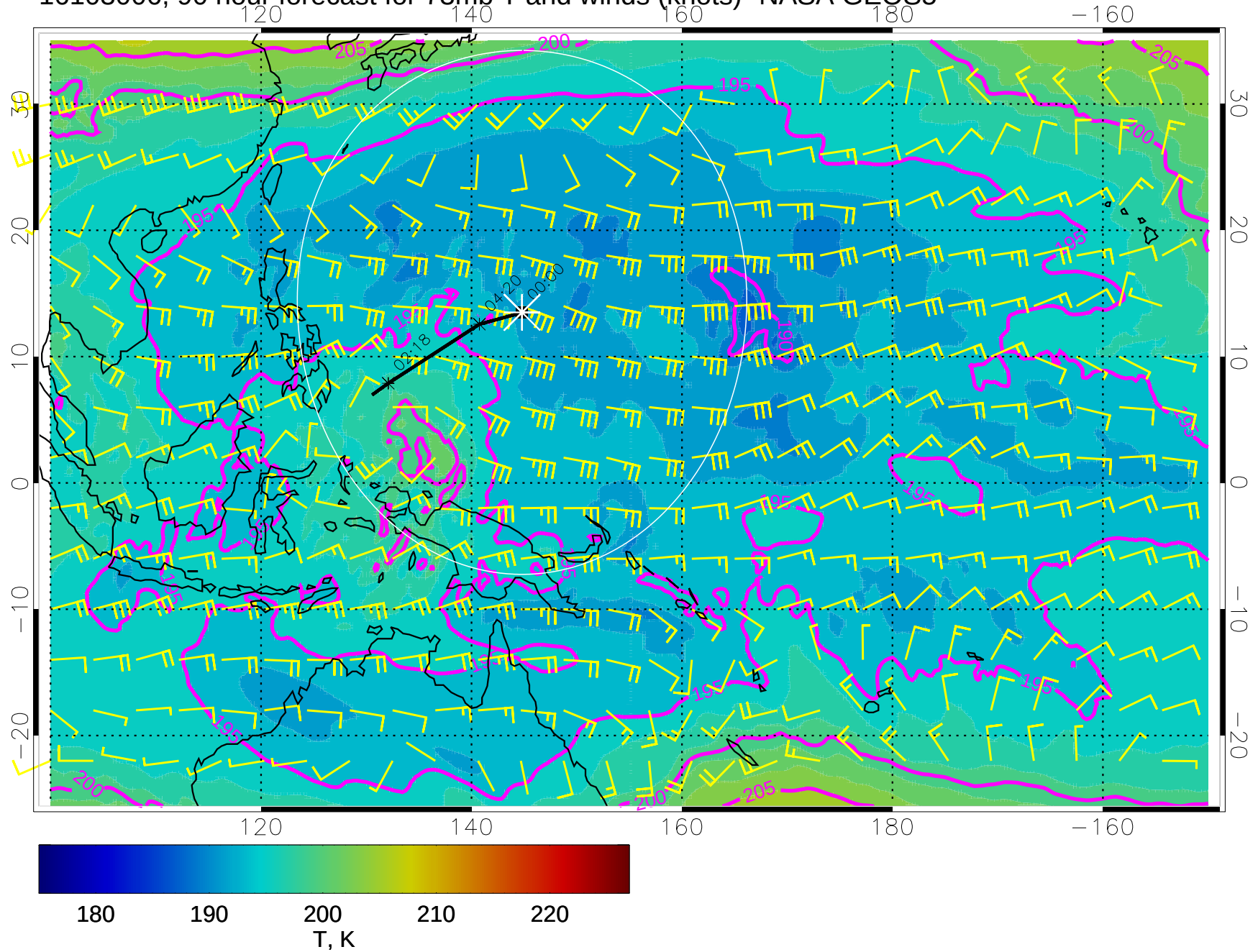
16103006, 90 hour forecast for 73mb T and winds (knots)- NASA GEOS5
