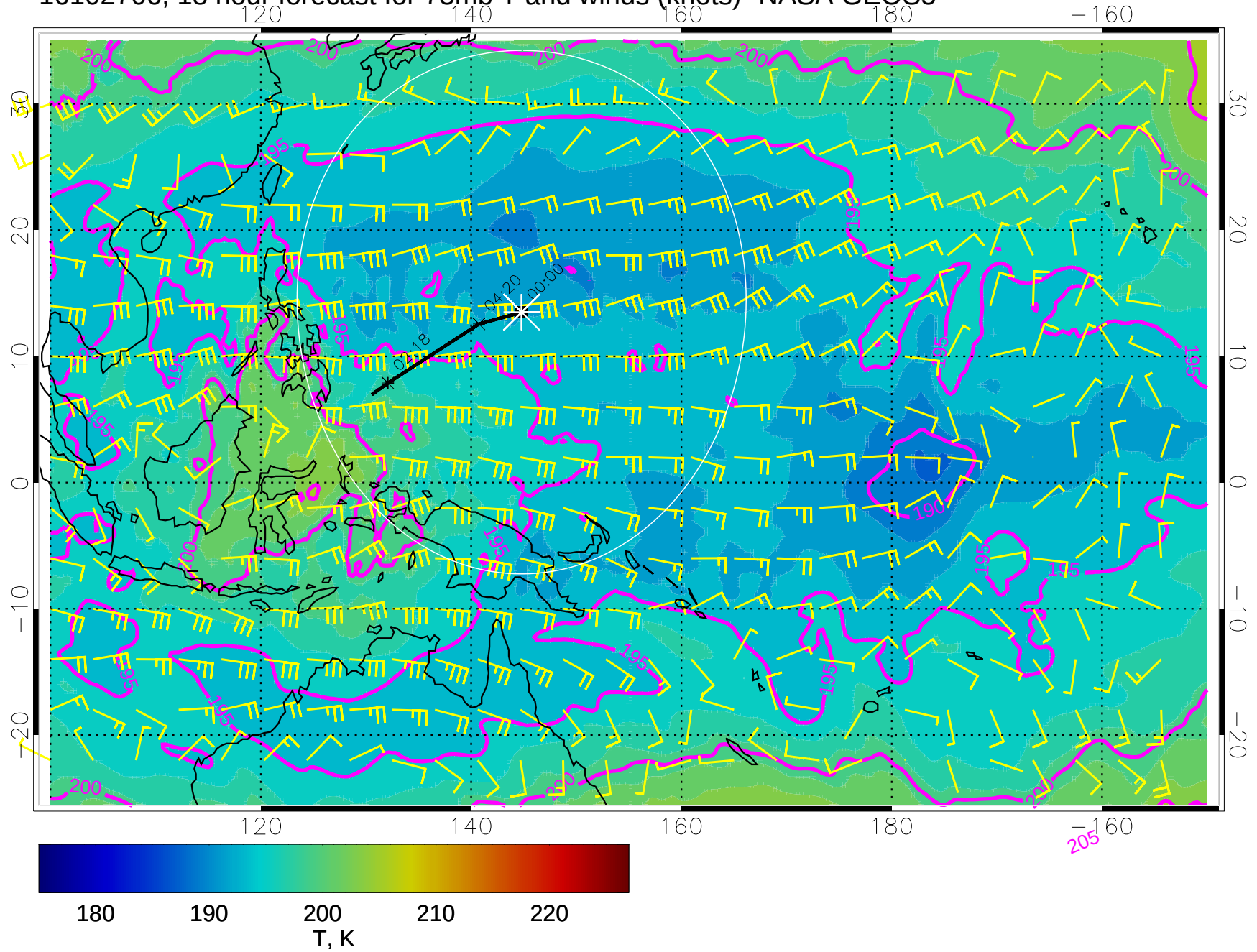
16102706, 18 hour forecast for 73mb T and winds (knots)- NASA GEOS5
