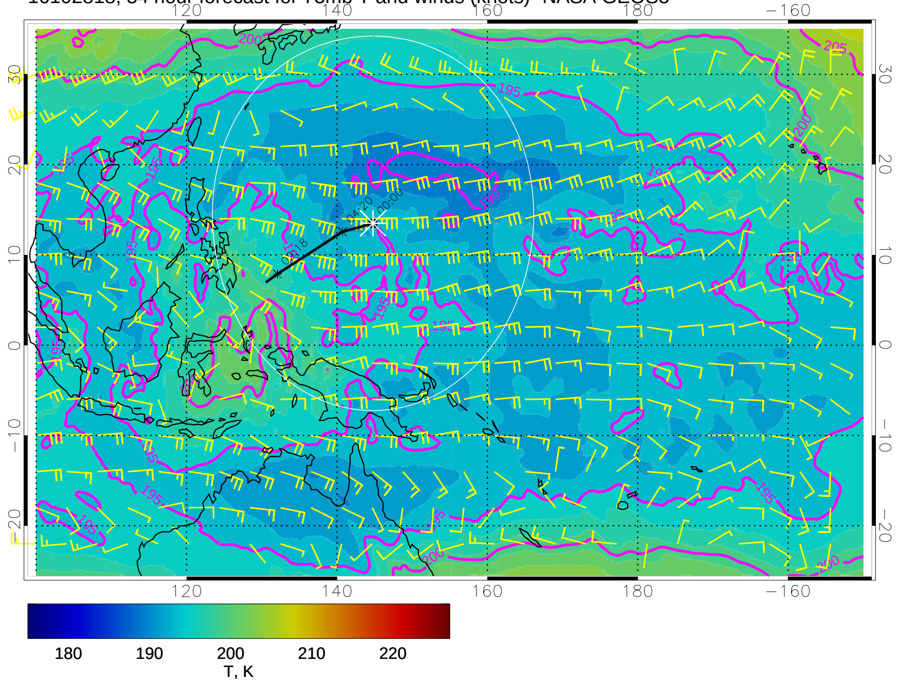
16102818, 54 hour forecast for 73mb T and winds (knots)- NASA GEOS5
