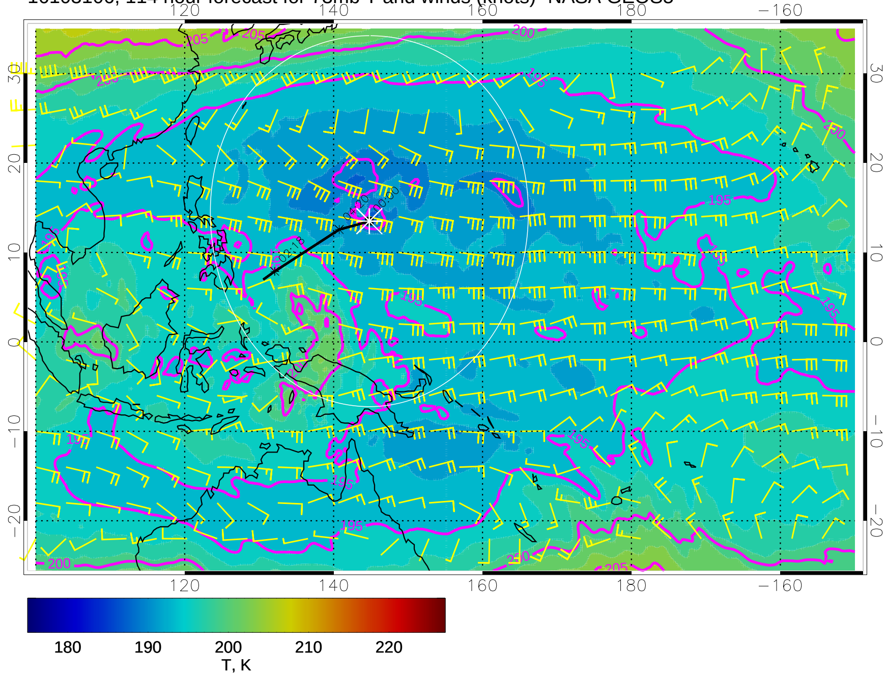
16103106, 114 hour forecast for 73mb T and winds (knots)- NASA GEOS5
