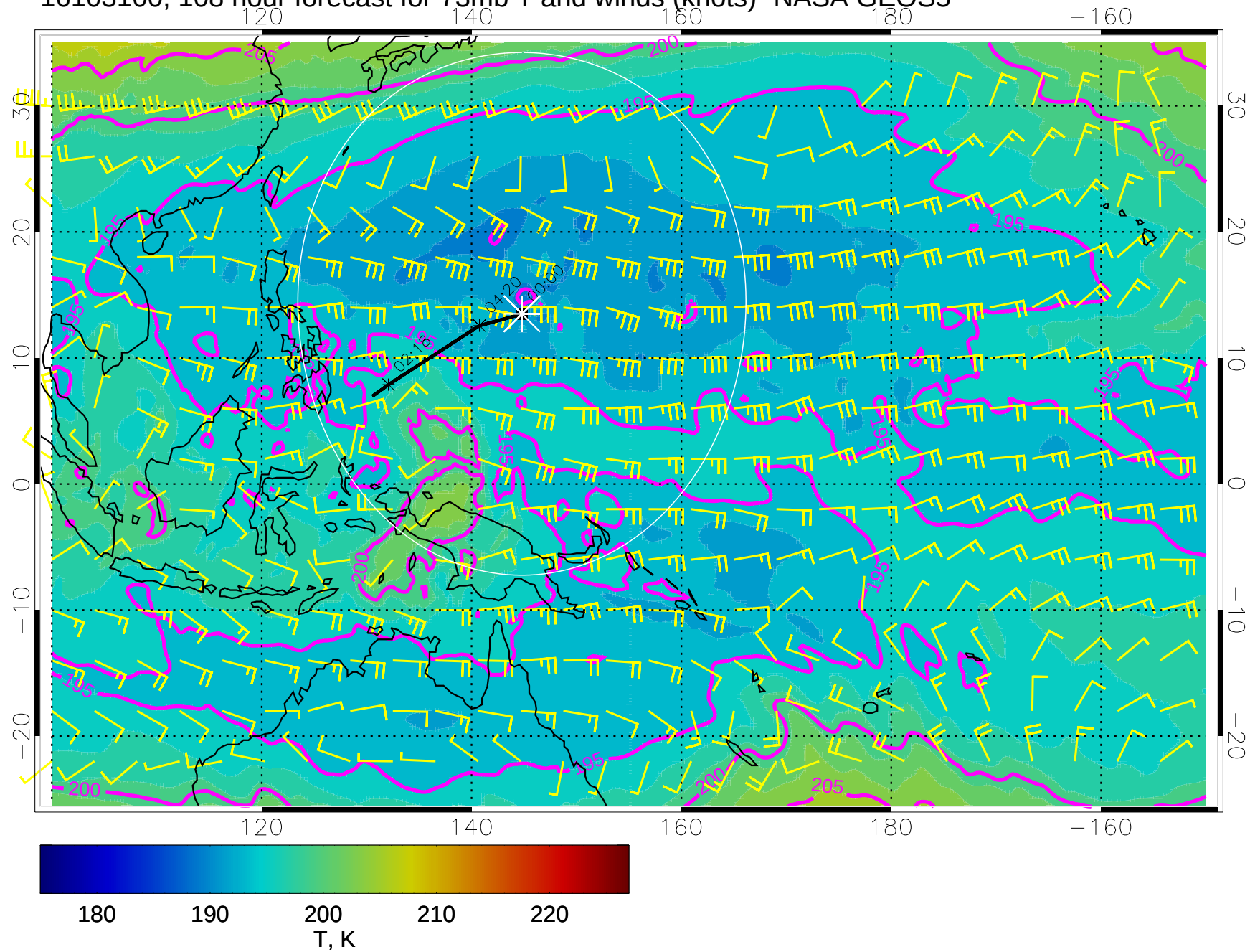
16103100, 108 hour forecast for 73mb T and winds (knots)- NASA GEOS5
