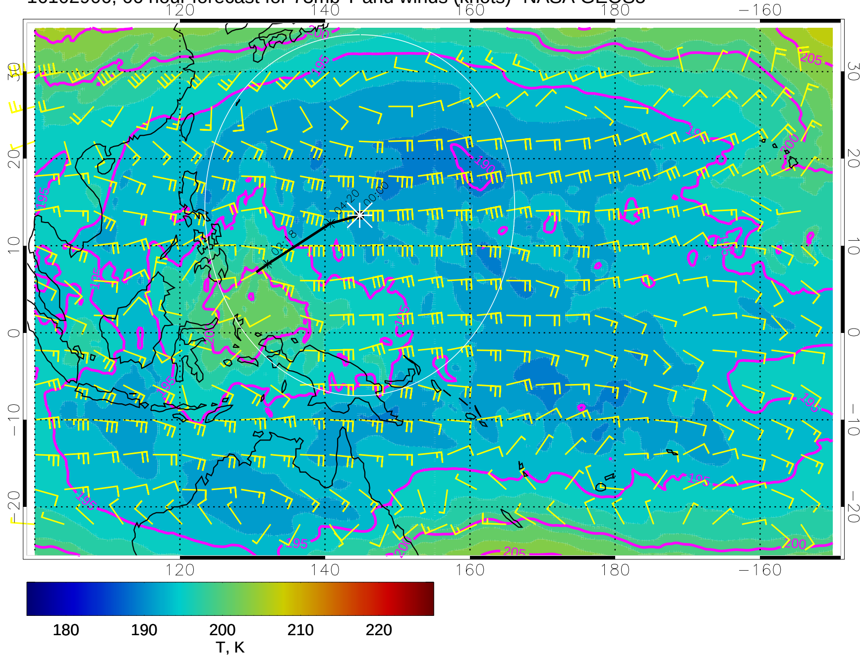
16102906, 66 hour forecast for 73mb T and winds (knots)- NASA GEOS5
