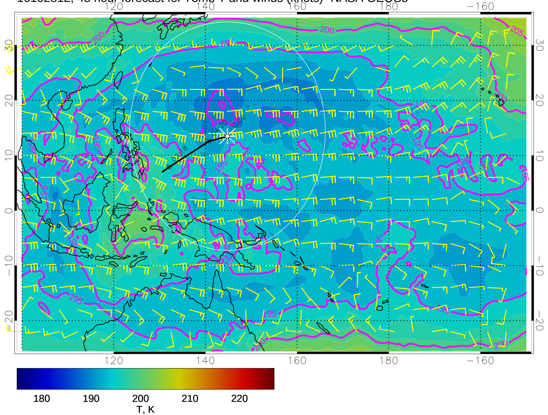
16102812, 48 hour forecast for 73mb T and winds (knots)- NASA GEOS5
