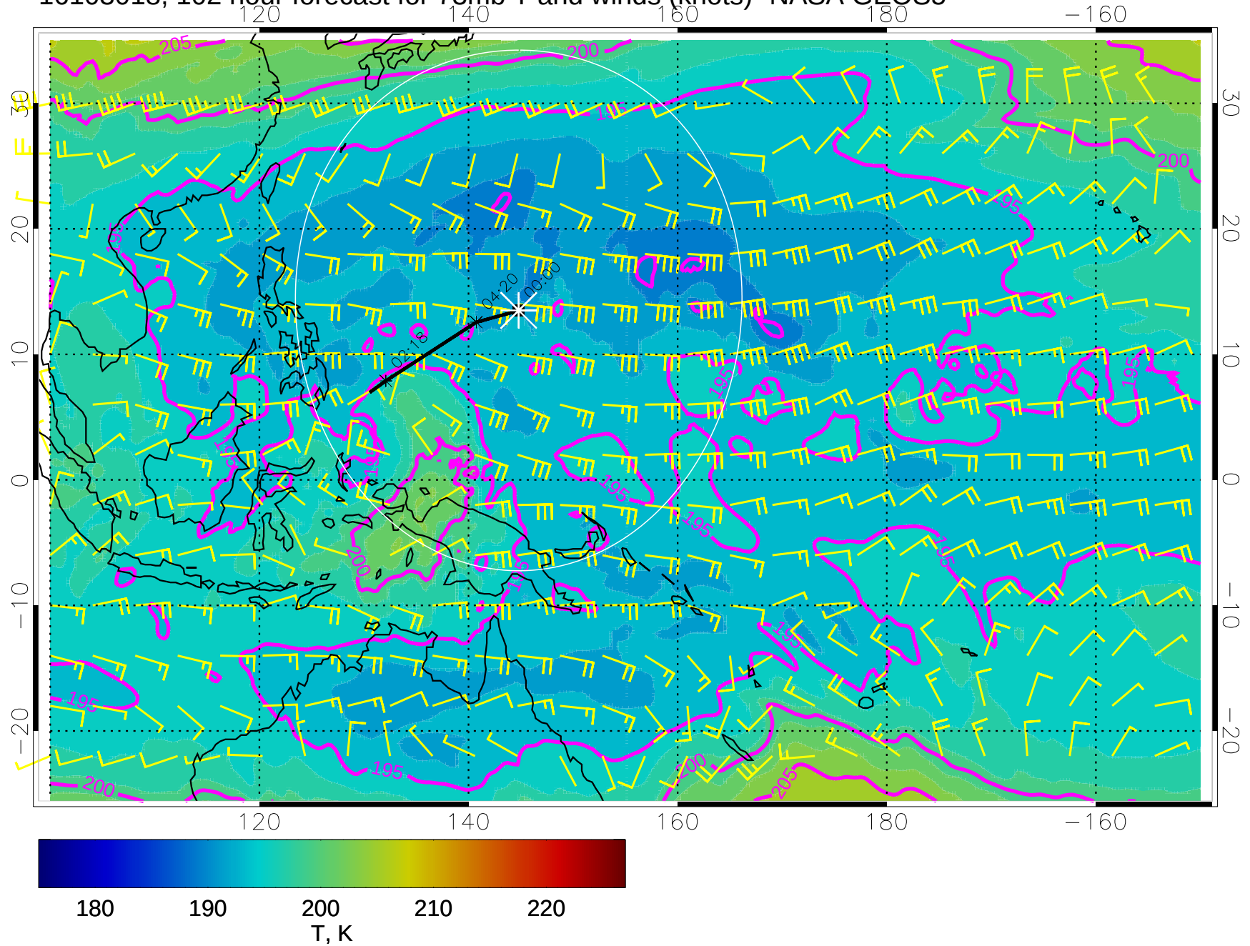
16103018, 102 hour forecast for 73mb T and winds (knots)- NASA GEOS5
