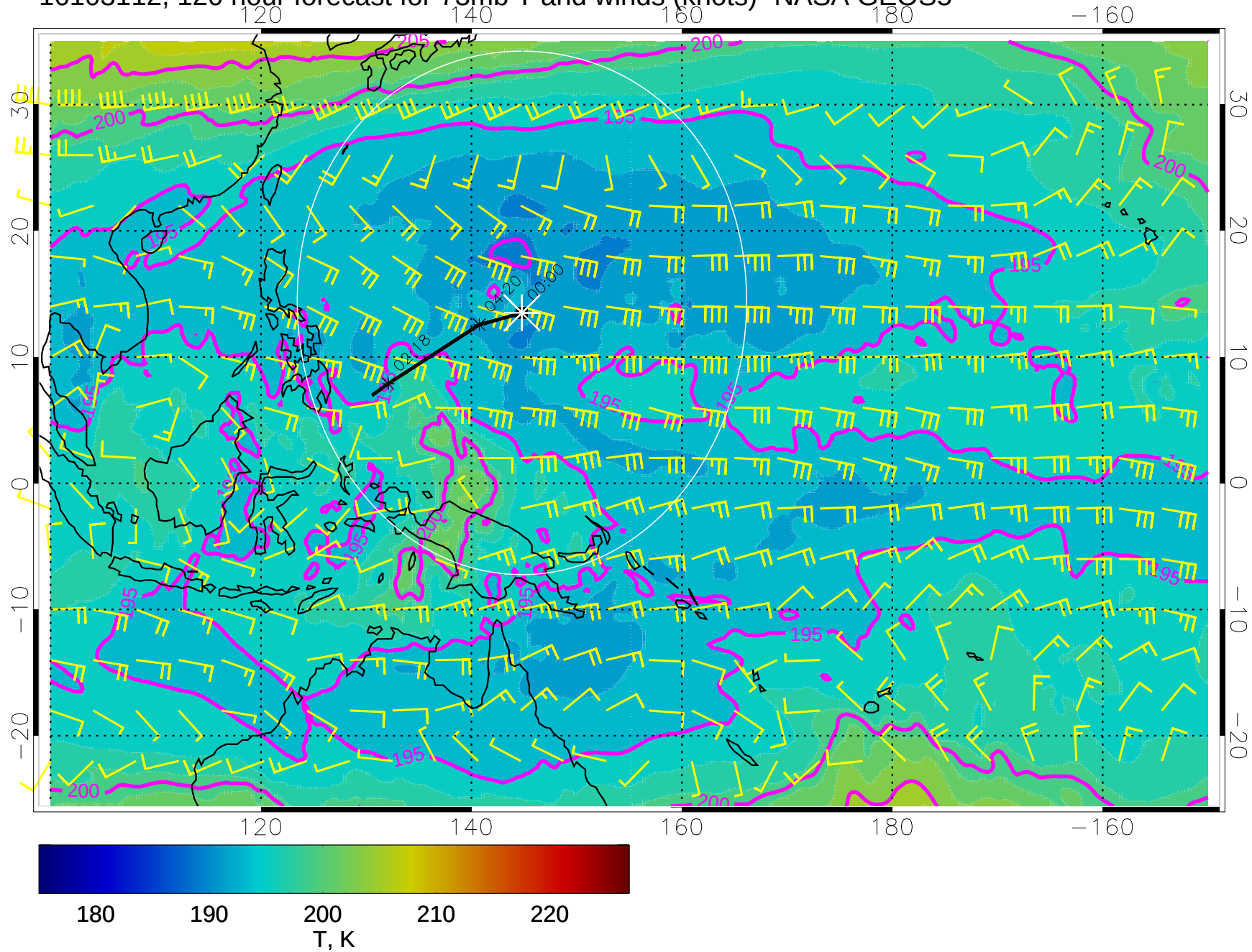
16103112, 120 hour forecast for 73mb T and winds (knots)- NASA GEOS5
