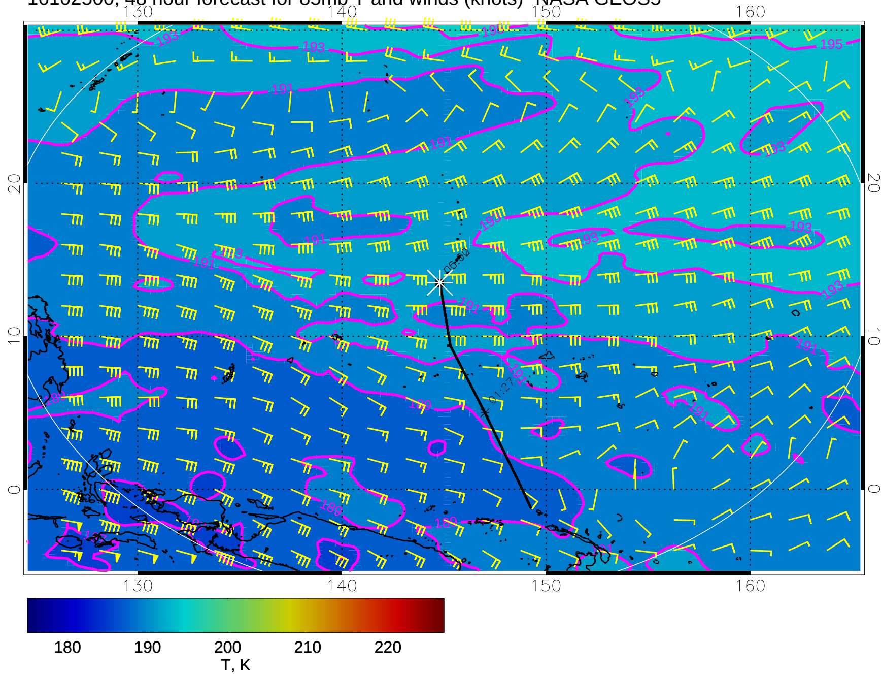
16102500, 48 hour forecast for 85mb T and winds (knots)- NASA GEOS5
