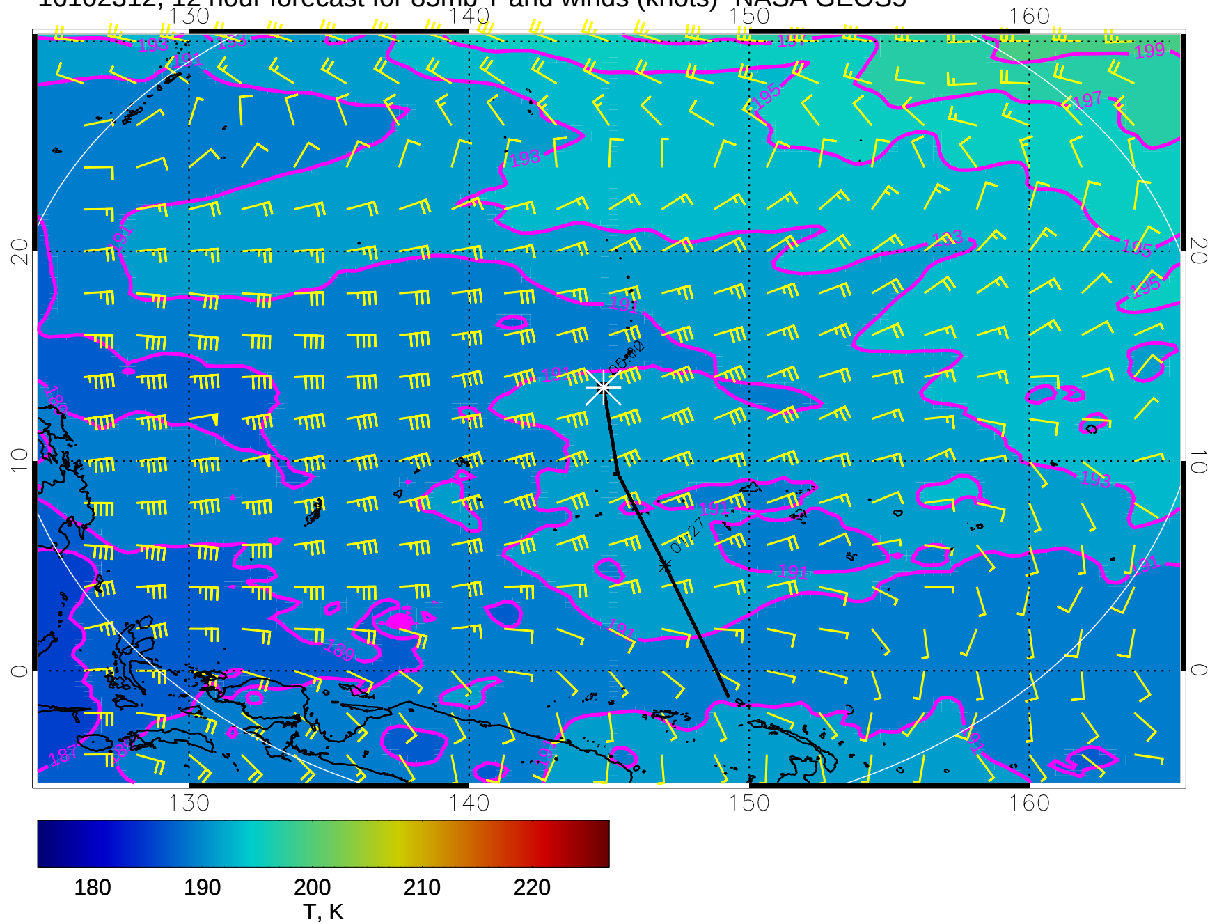
16102312, 12 hour forecast for 85mb T and winds (knots)- NASA GEOS5
