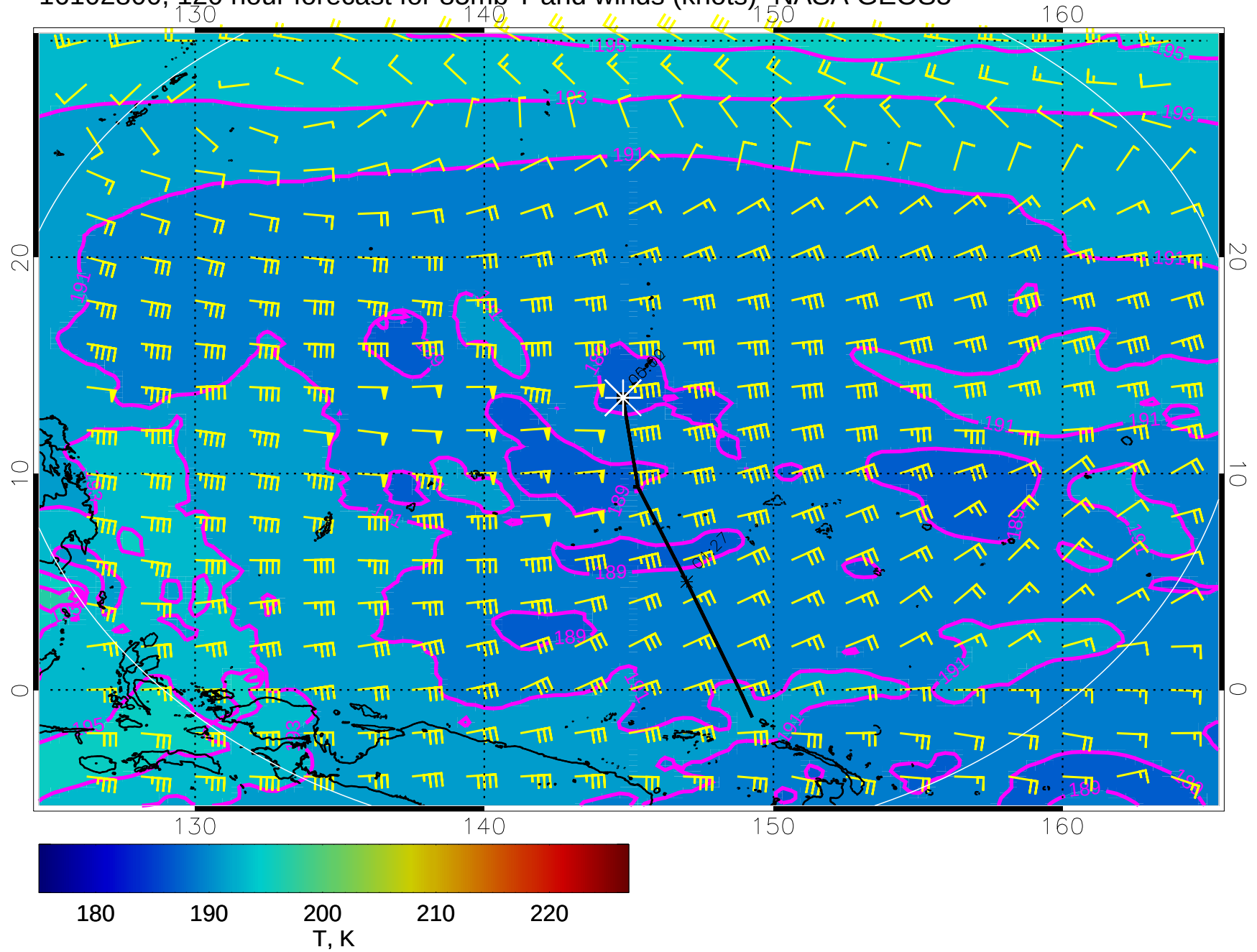
16102800, 120 hour forecast for 85mb T and winds (knots)- NASA GEOS5
