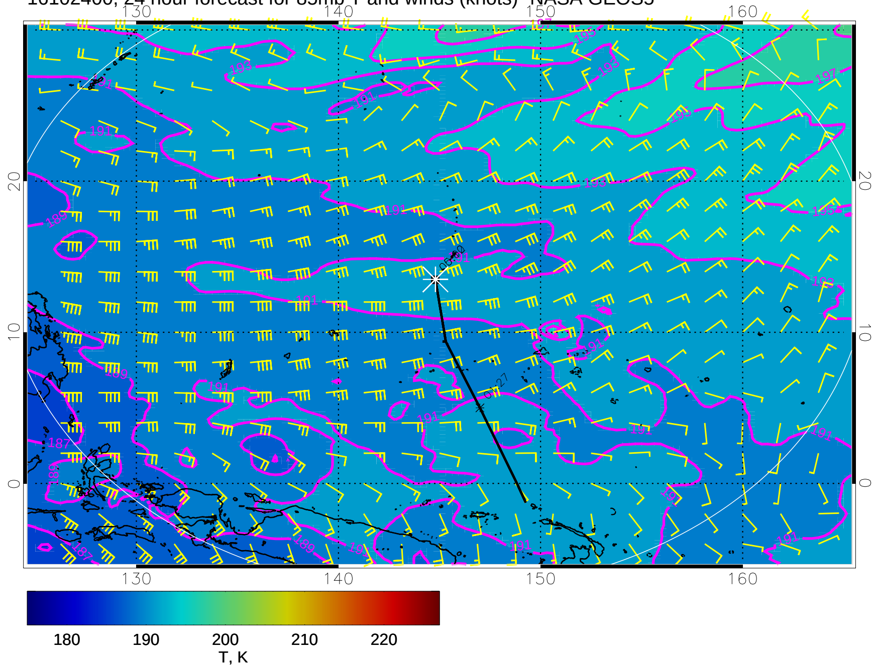
16102400, 24 hour forecast for 85mb T and winds (knots)- NASA GEOS5
