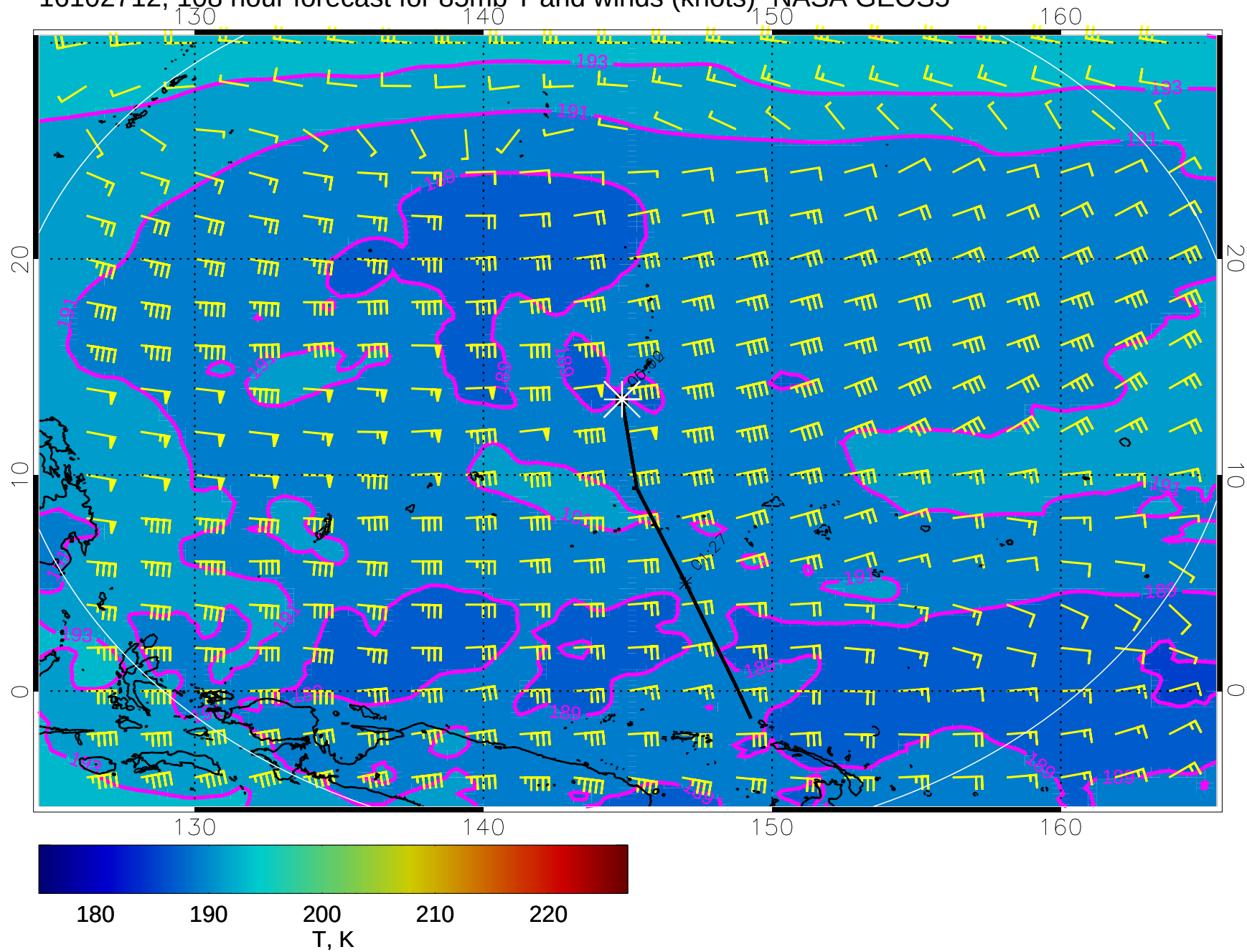
16102712, 108 hour forecast for 85mb T and winds (knots)- NASA GEOS5
