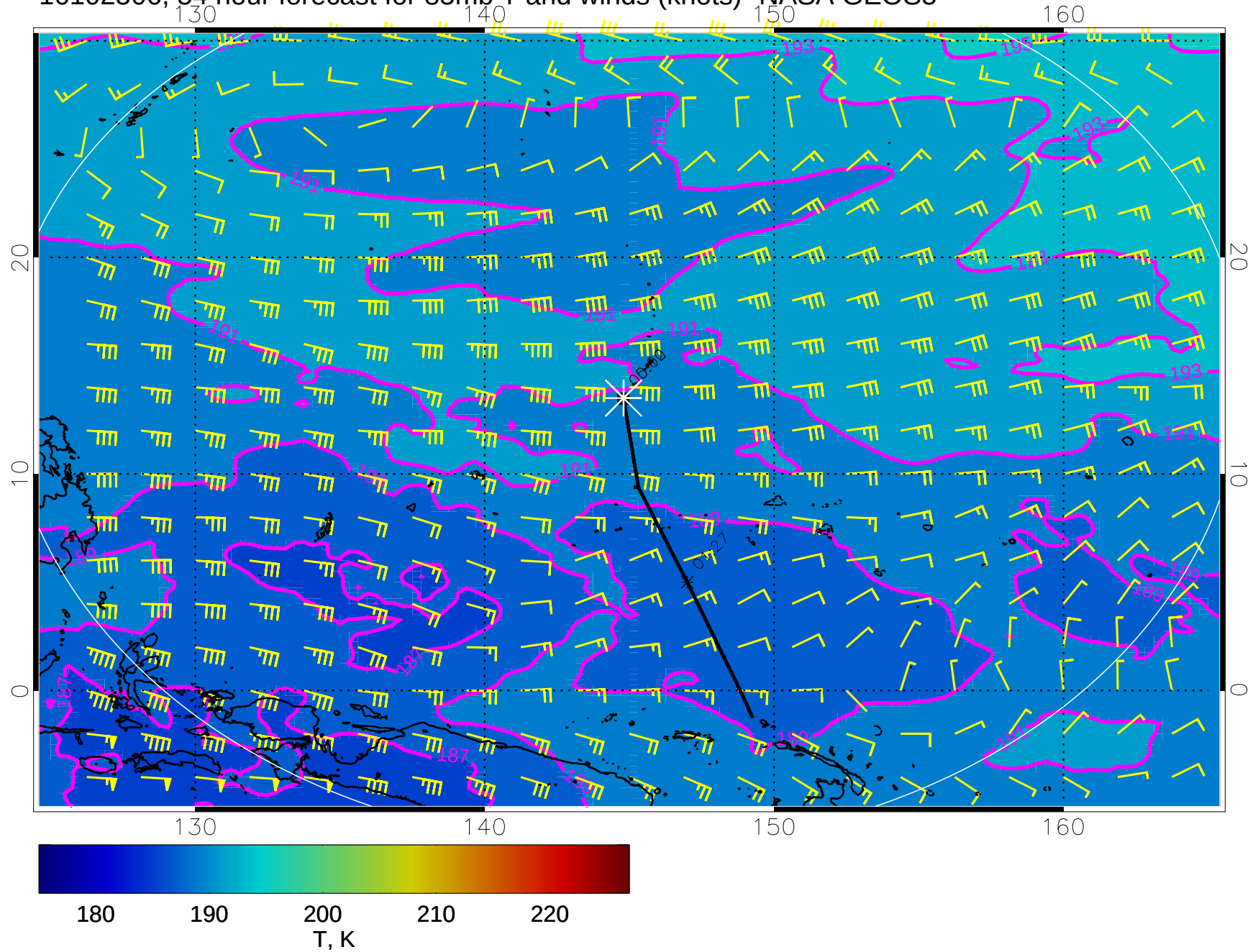
16102506, 54 hour forecast for 85mb T and winds (knots)- NASA GEOS5
