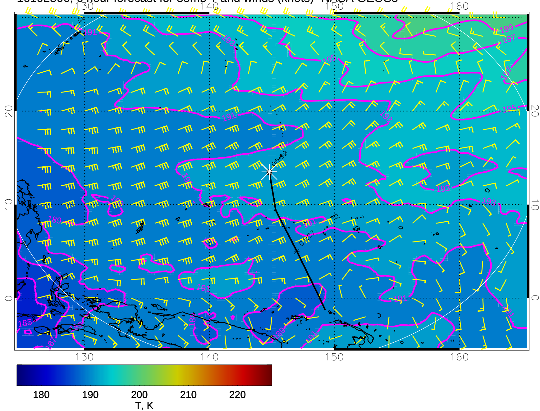
16102306, 6 hour forecast for 85mb T and winds (knots)- NASA GEOS5
