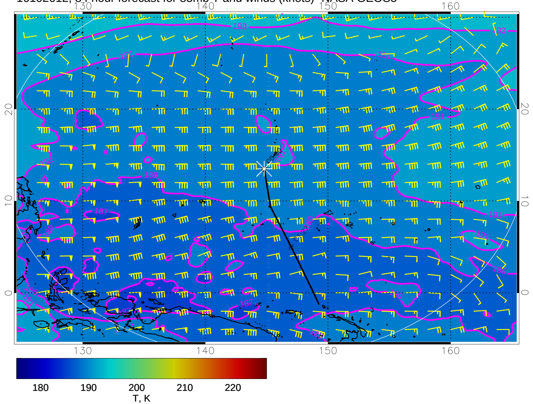
16102612, 84 hour forecast for 85mb T and winds (knots)- NASA GEOS5
