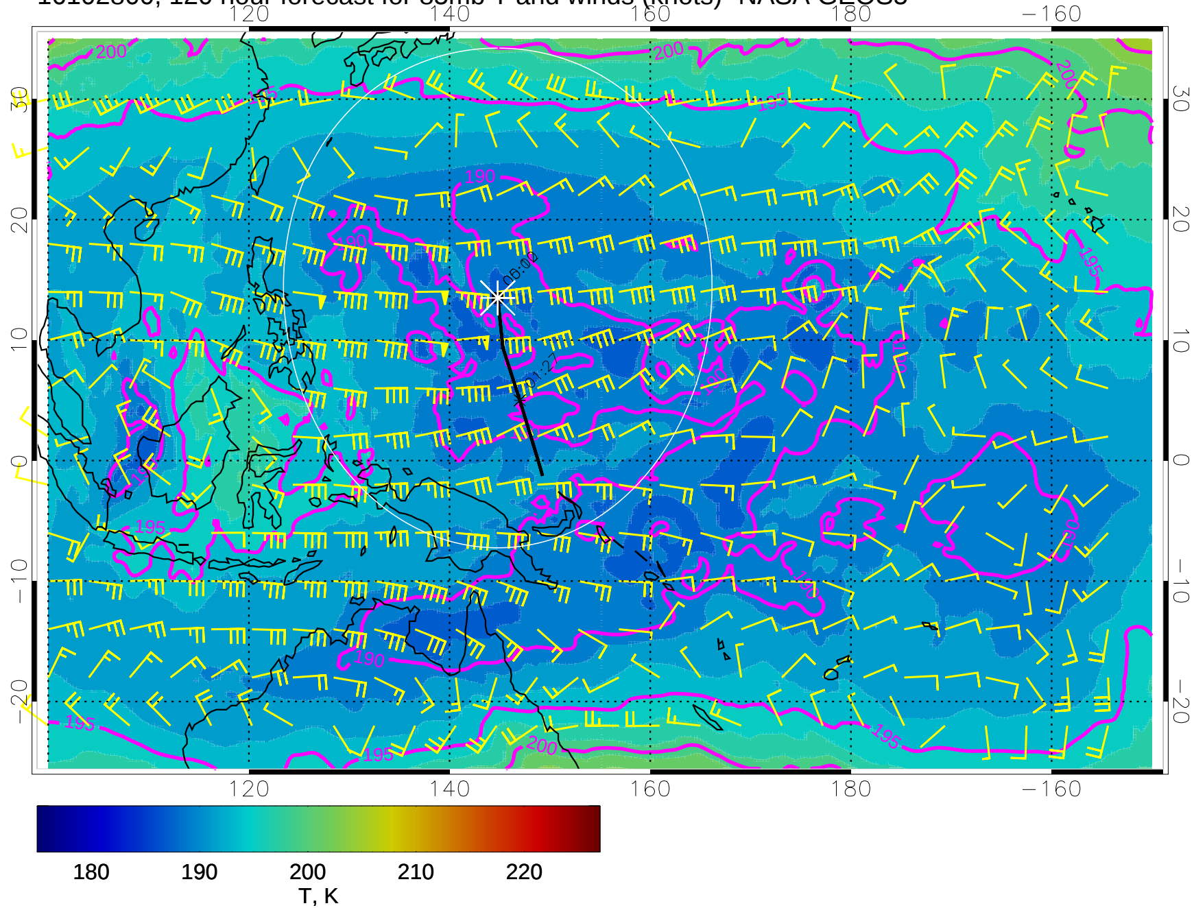
16102800, 120 hour forecast for 85mb T and winds (knots)- NASA GEOS5
