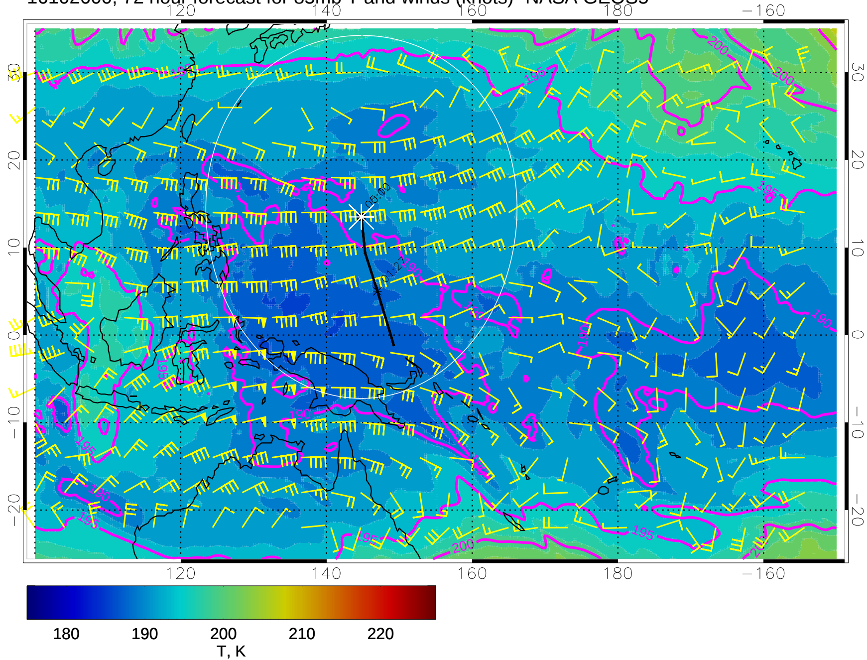
16102600, 72 hour forecast for 85mb T and winds (knots)- NASA GEOS5
