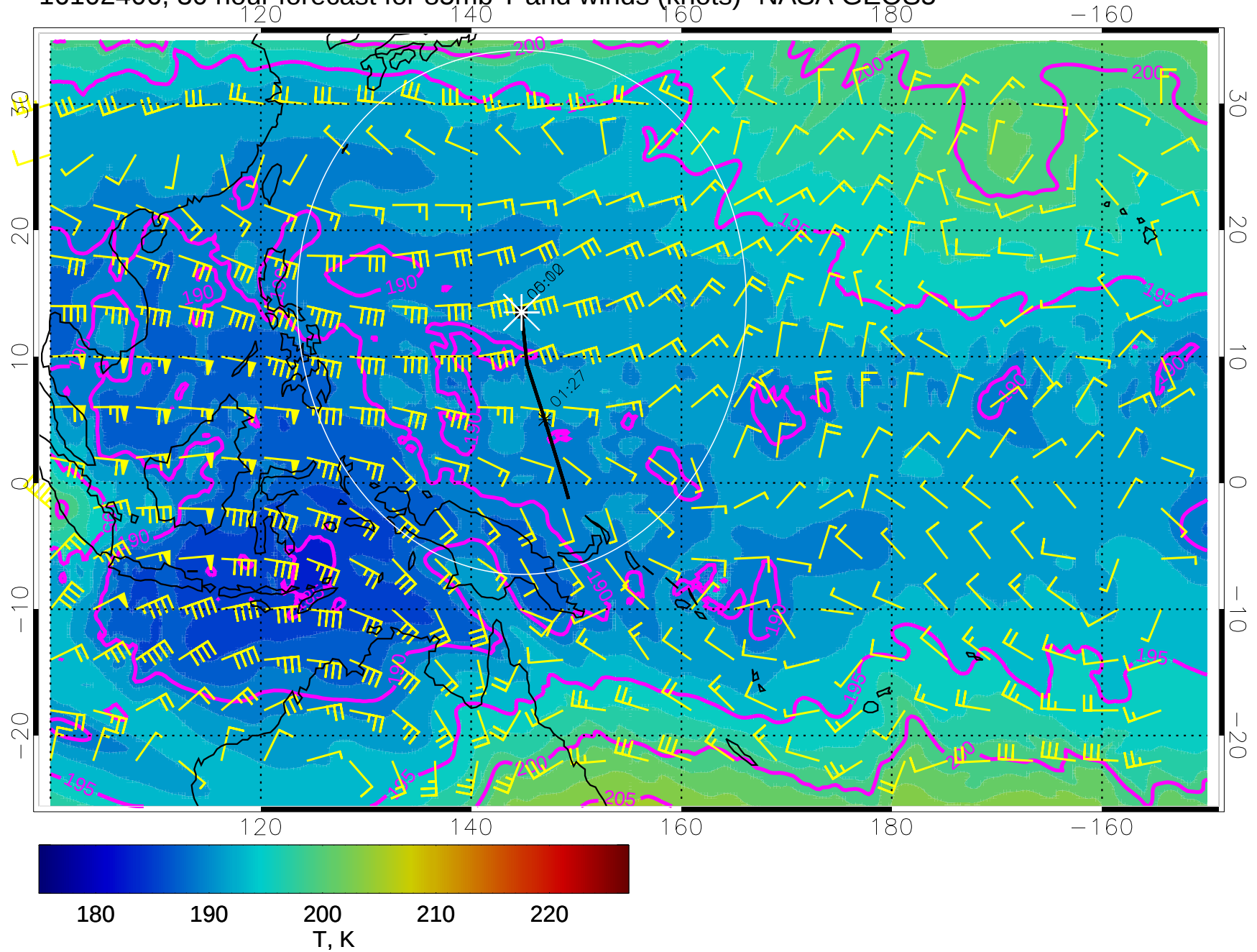
16102406, 30 hour forecast for 85mb T and winds (knots)- NASA GEOS5
