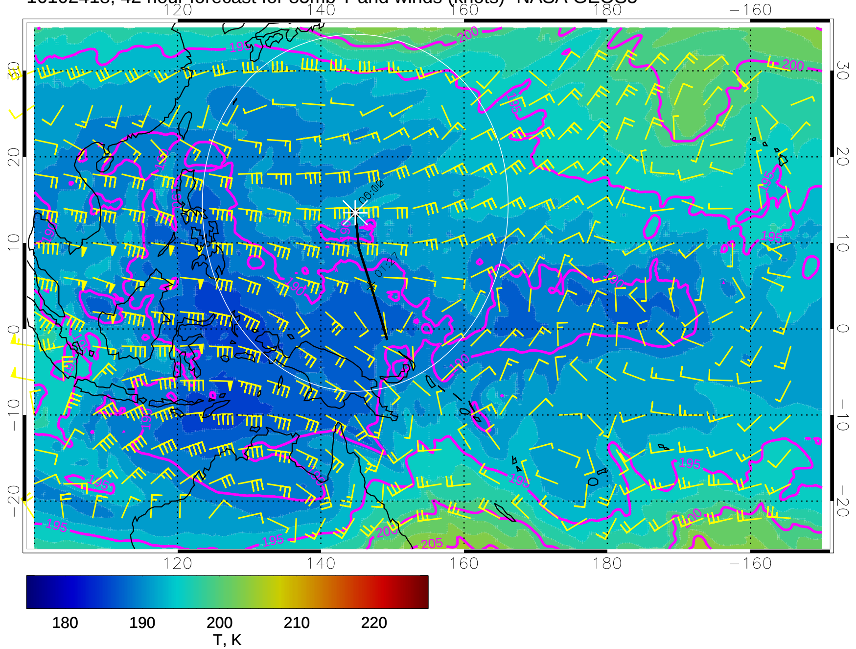
16102418, 42 hour forecast for 85mb T and winds (knots)- NASA GEOS5
