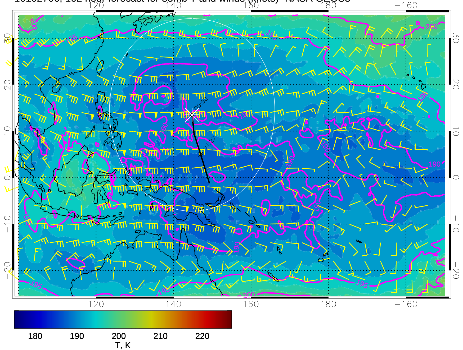
16102706, 102 hour forecast for 85mb T and winds (knots)- NASA GEOS5
