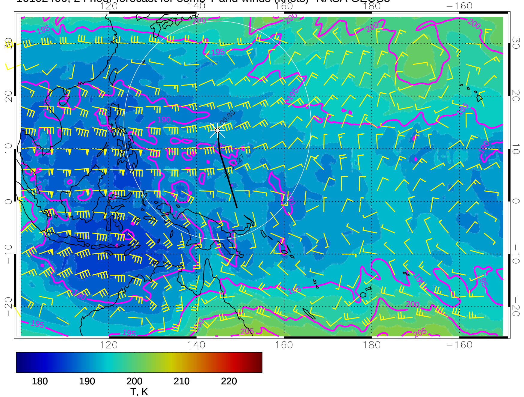
16102400, 24 hour forecast for 85mb T and winds (knots)- NASA GEOS5
