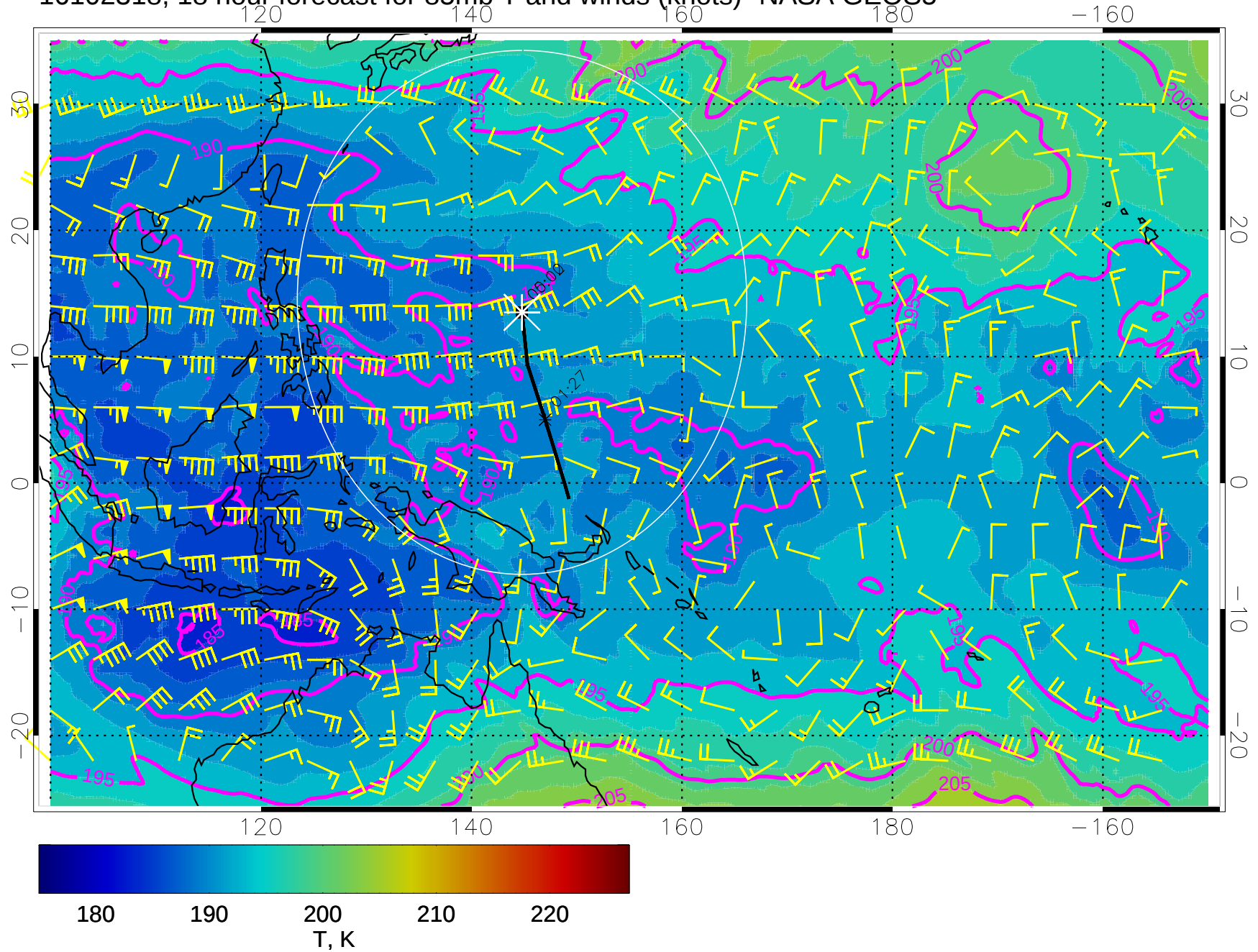
16102318, 18 hour forecast for 85mb T and winds (knots)- NASA GEOS5
