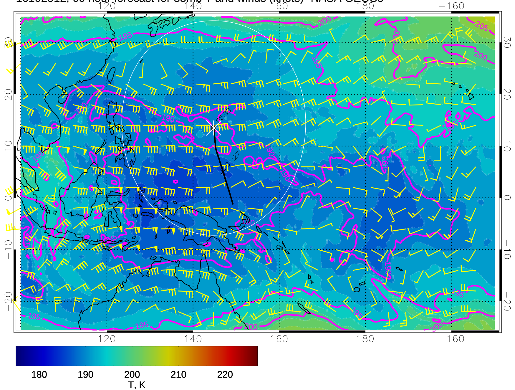
16102512, 60 hour forecast for 85mb T and winds (knots)- NASA GEOS5
