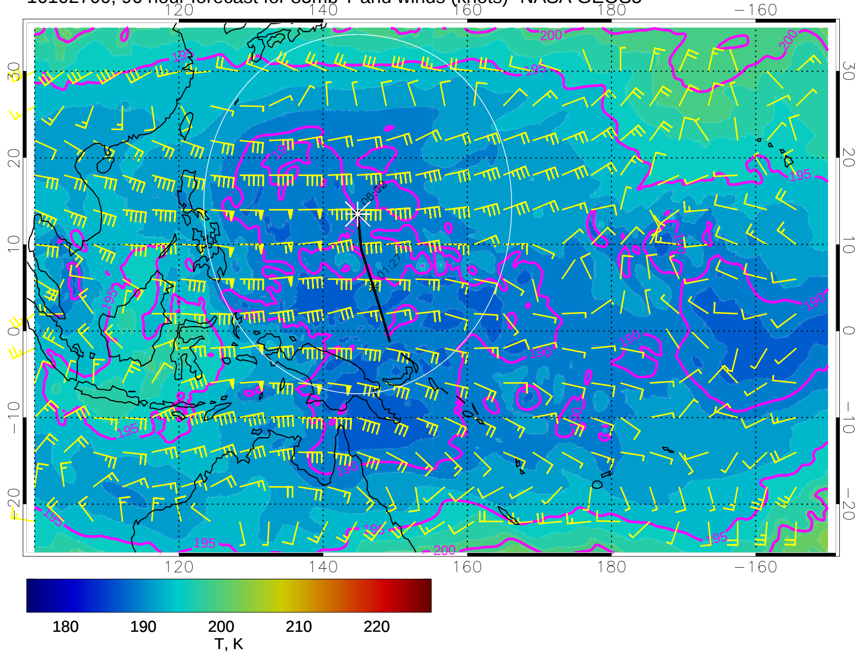
16102700, 96 hour forecast for 85mb T and winds (knots)- NASA GEOS5
