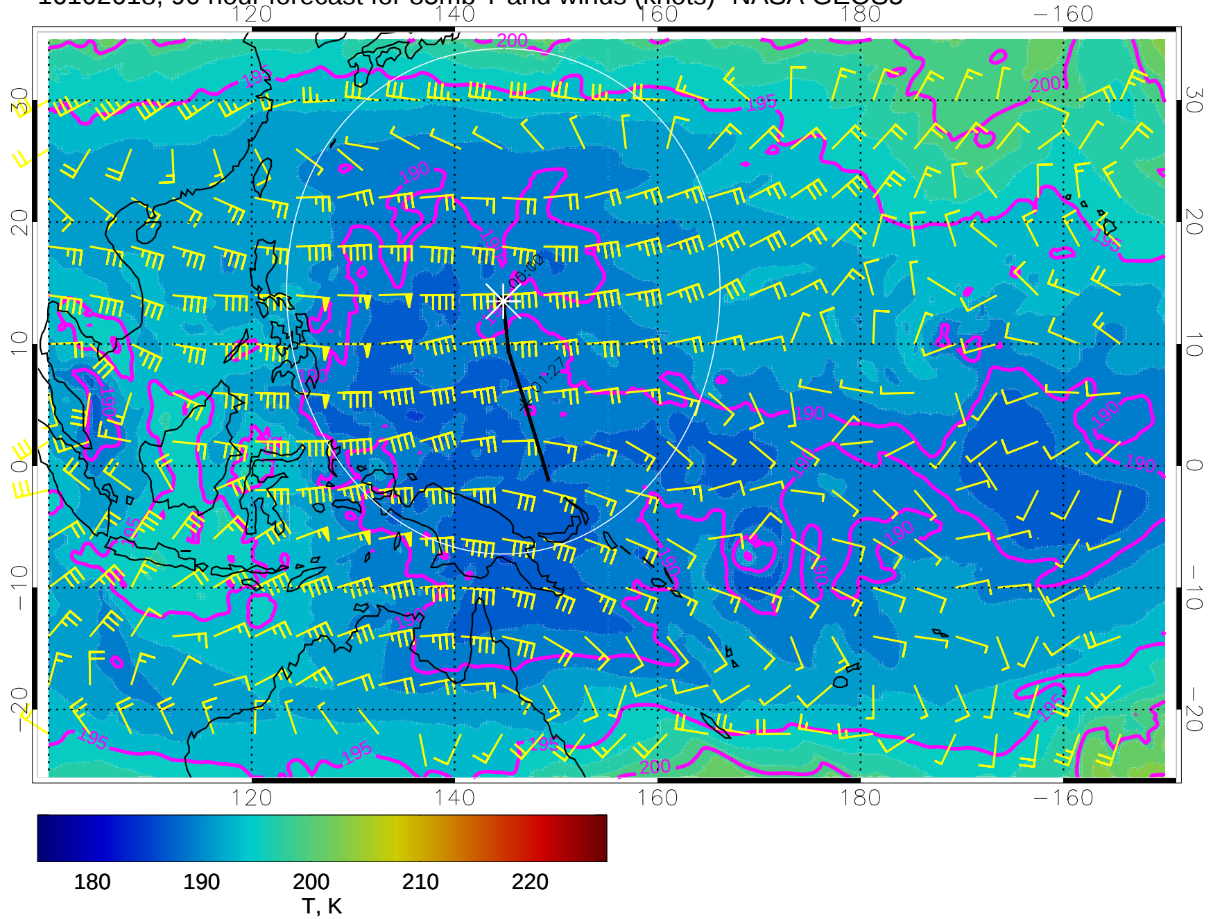
16102618, 90 hour forecast for 85mb T and winds (knots)- NASA GEOS5
