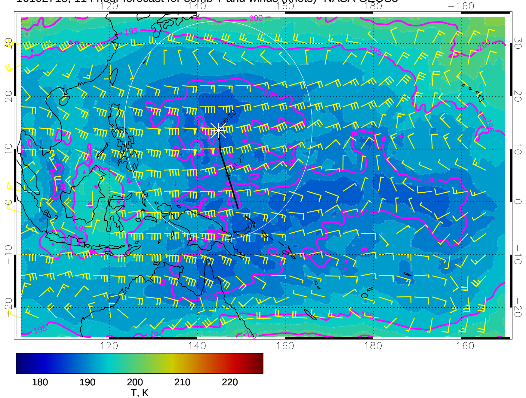
16102718, 114 hour forecast for 85mb T and winds (knots)- NASA GEOS5
