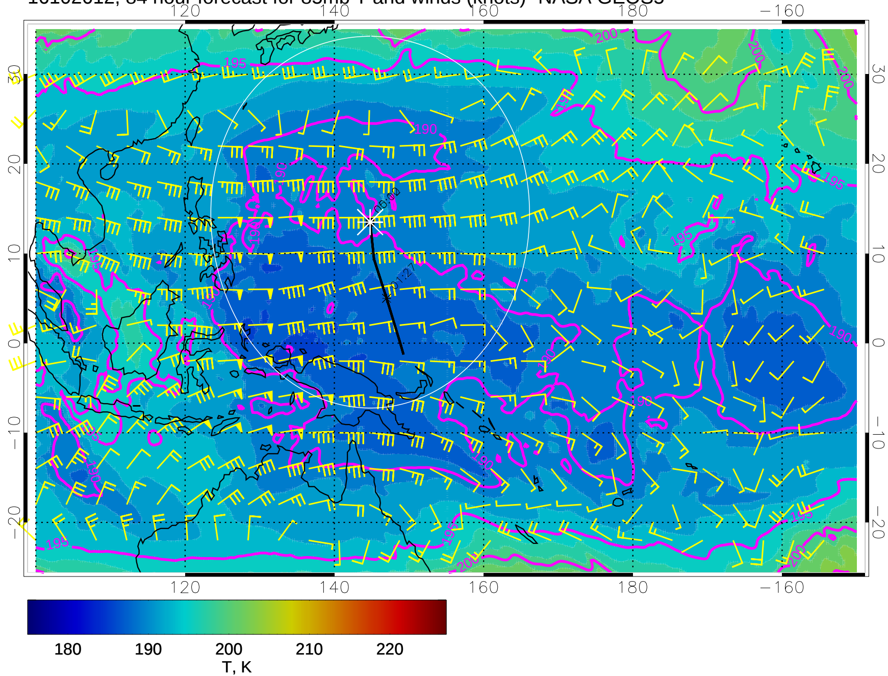
16102612, 84 hour forecast for 85mb T and winds (knots)- NASA GEOS5
