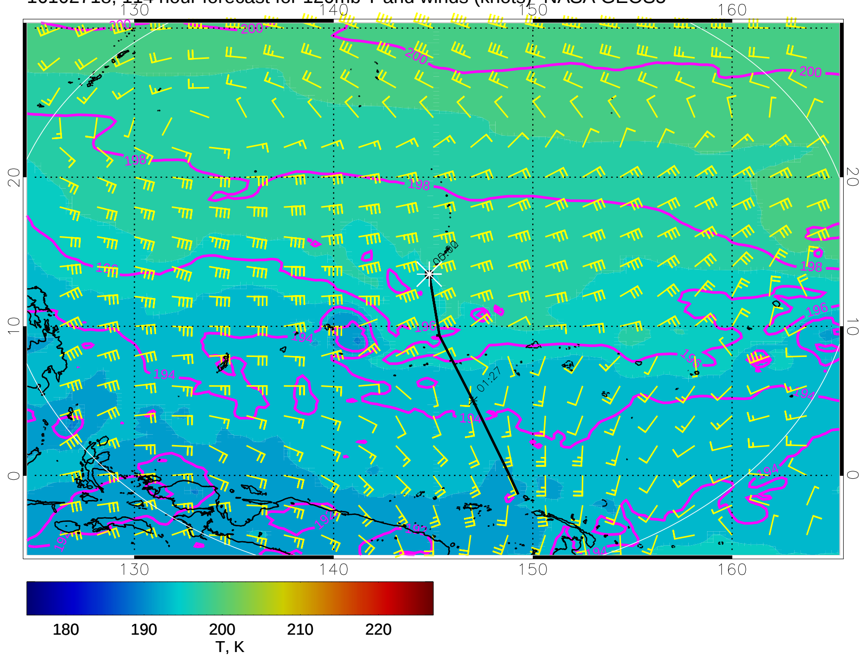
16102718, 114 hour forecast for 120mb T and winds (knots)- NASA GEOS5
