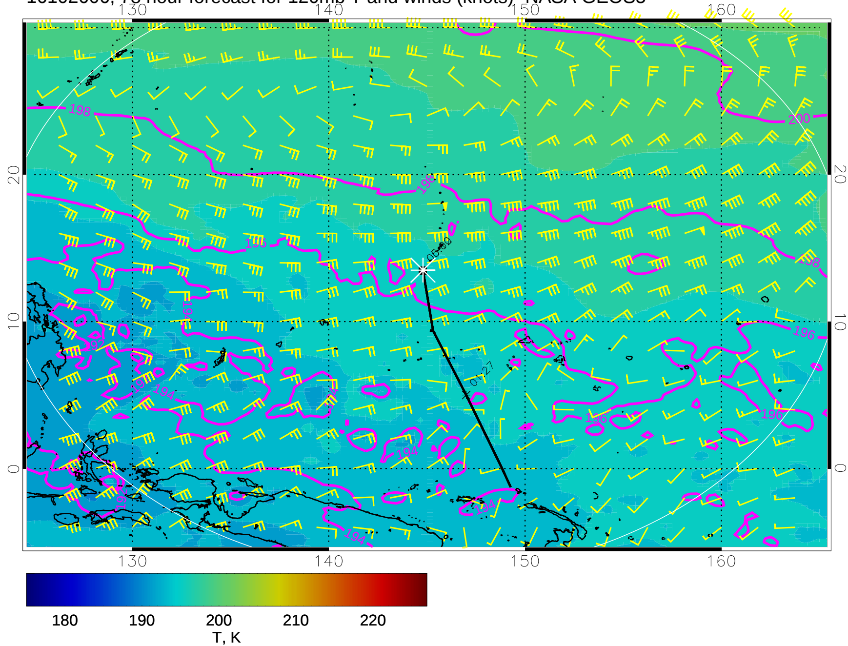
16102606, 78 hour forecast for 120mb T and winds (knots)- NASA GEOS5
