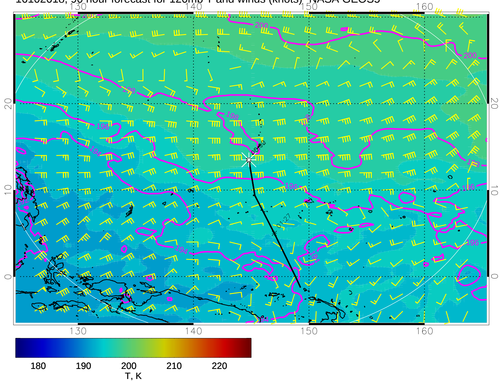
16102618, 90 hour forecast for 120mb T and winds (knots)- NASA GEOS5
