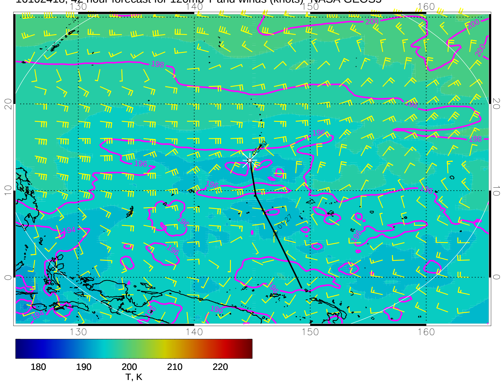
16102418, 42 hour forecast for 120mb T and winds (knots)- NASA GEOS5
