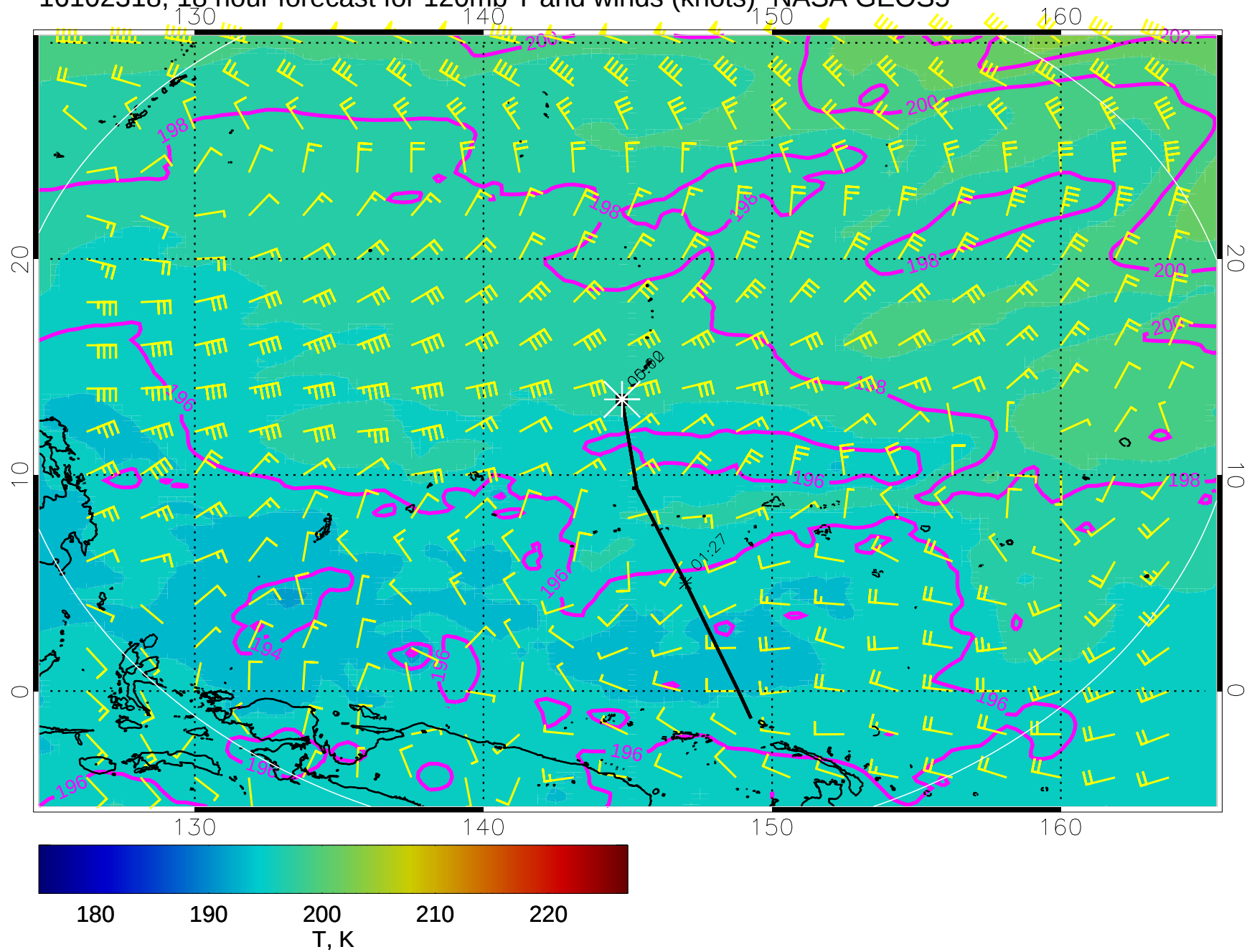
16102318, 18 hour forecast for 120mb T and winds (knots)- NASA GEOS5
