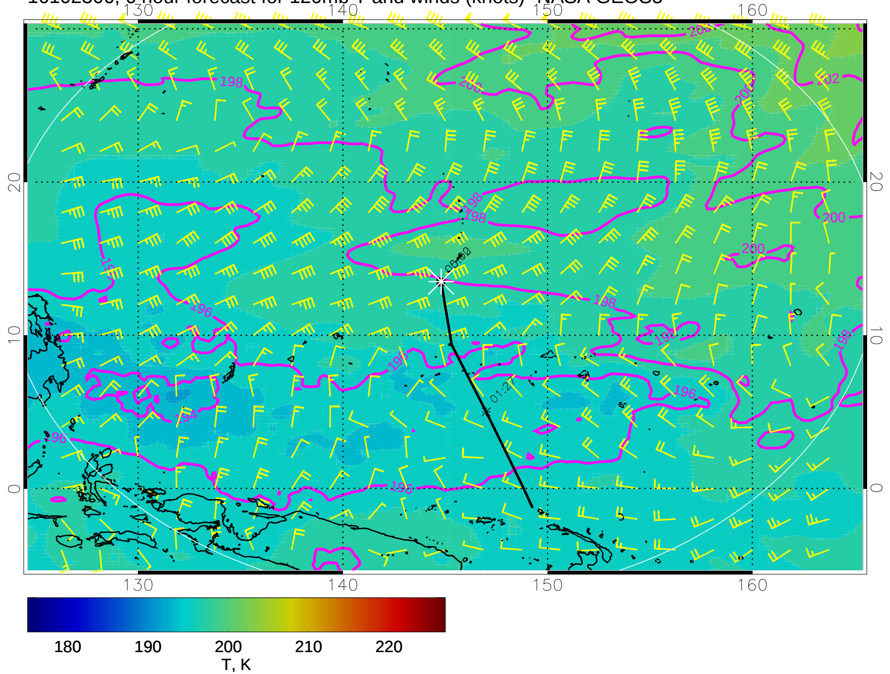
16102306, 6 hour forecast for 120mb T and winds (knots)- NASA GEOS5
