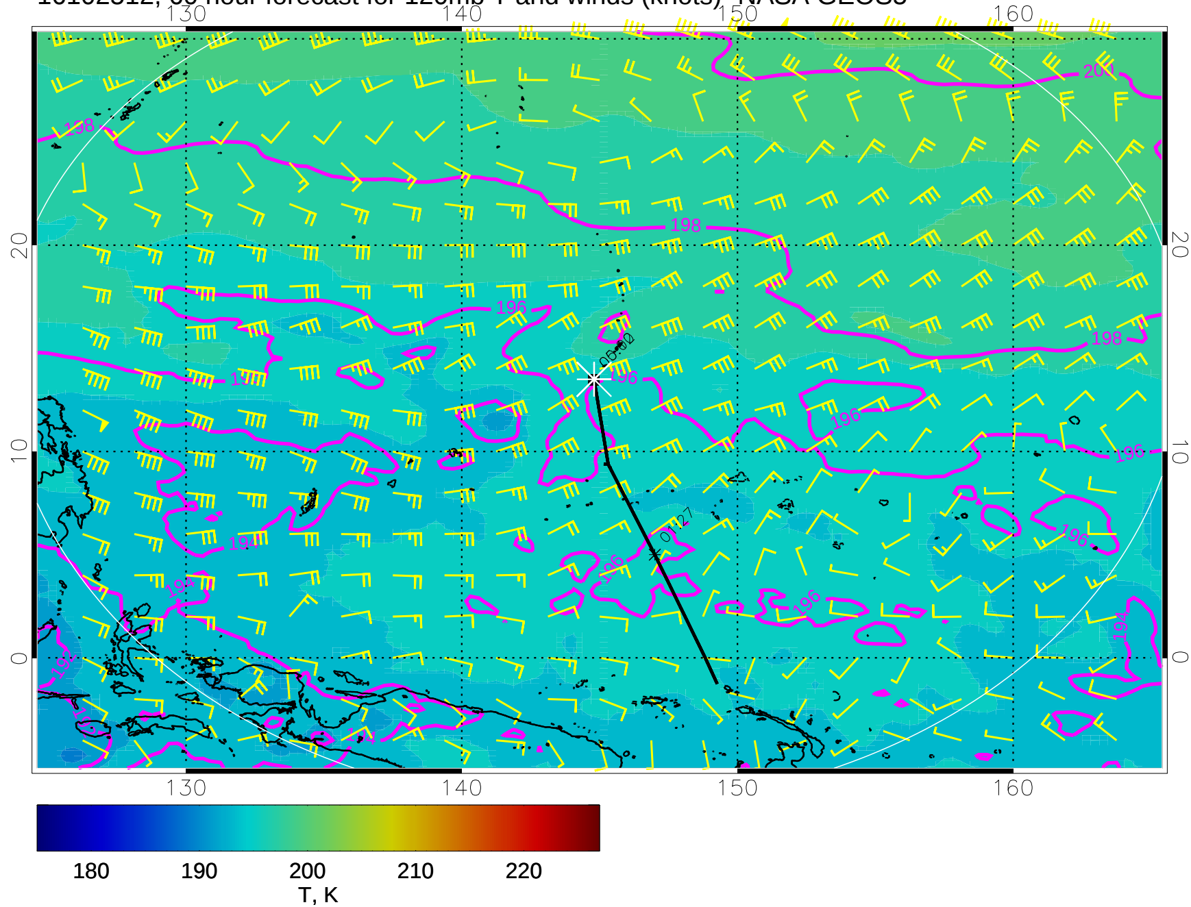
16102512, 60 hour forecast for 120mb T and winds (knots)- NASA GEOS5
