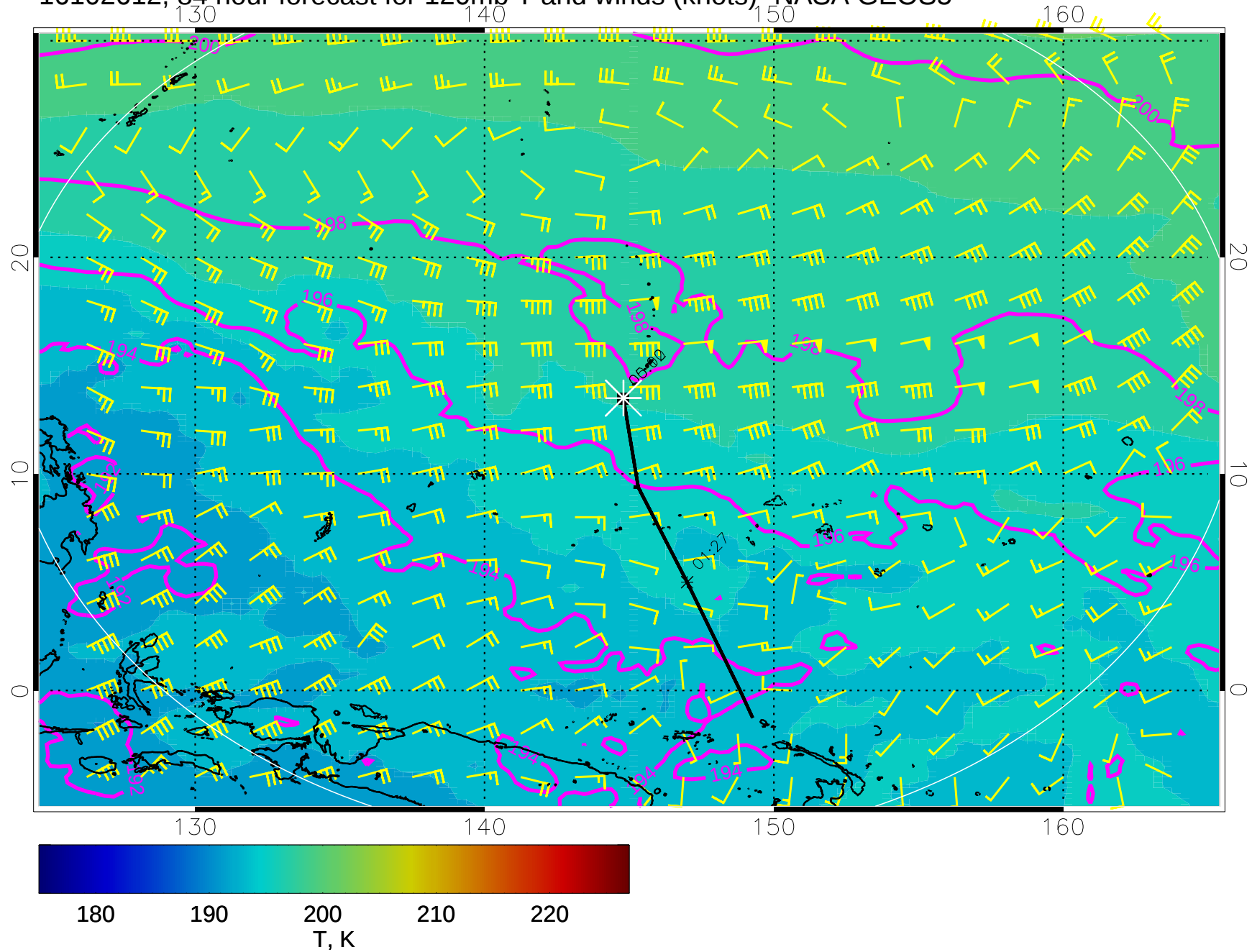
16102612, 84 hour forecast for 120mb T and winds (knots)- NASA GEOS5
