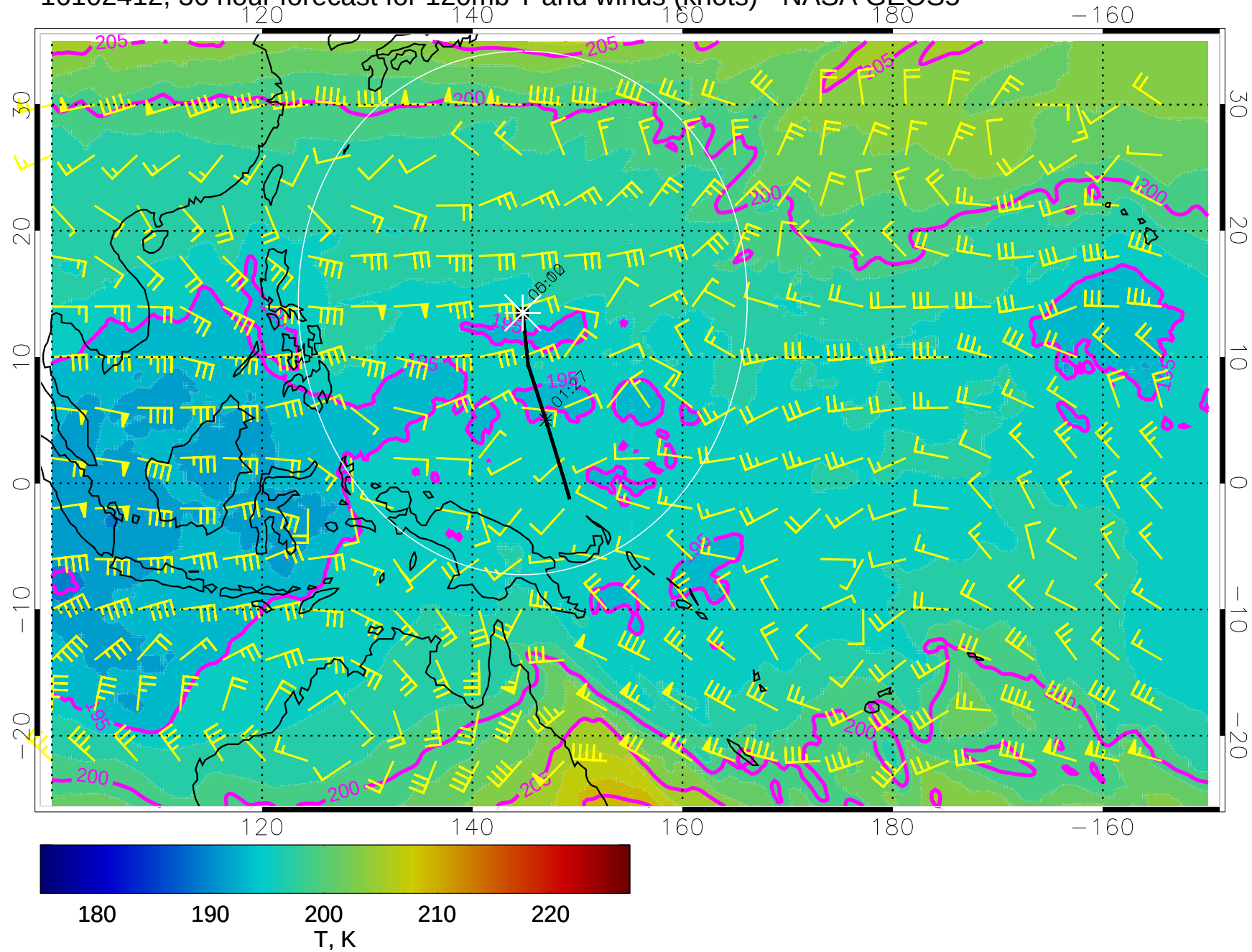
16102412, 36 hour forecast for 120mb T and winds (knots) - NASA GEOS5
