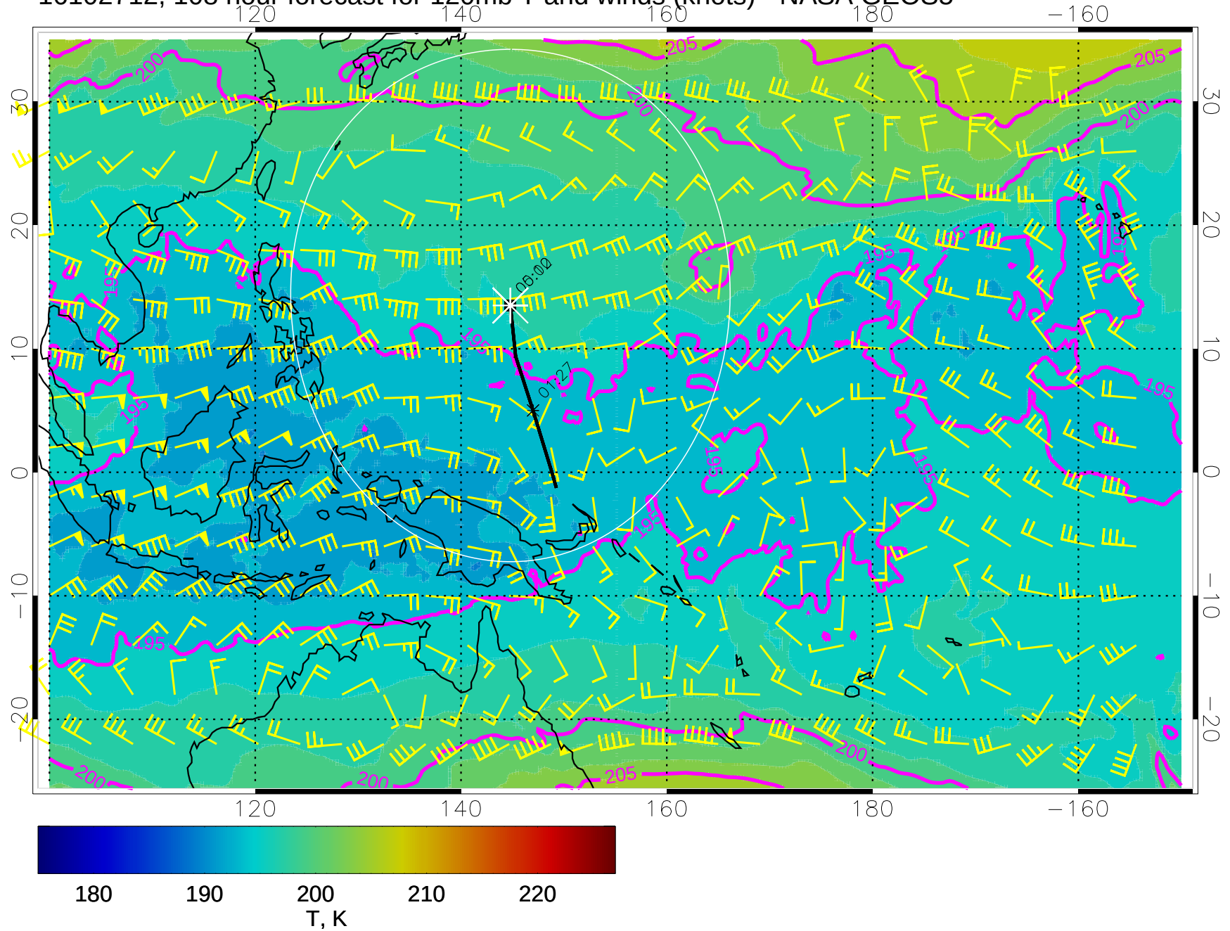
16102712, 108 hour forecast for 120mb T and winds (knots) - NASA GEOS5
