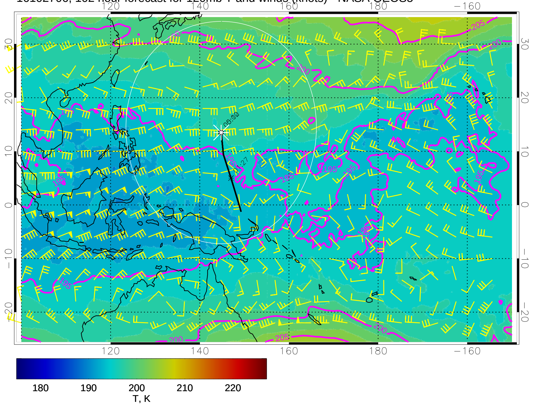
16102706, 102 hour forecast for 120mb T and winds (knots) - NASA GEOS5
