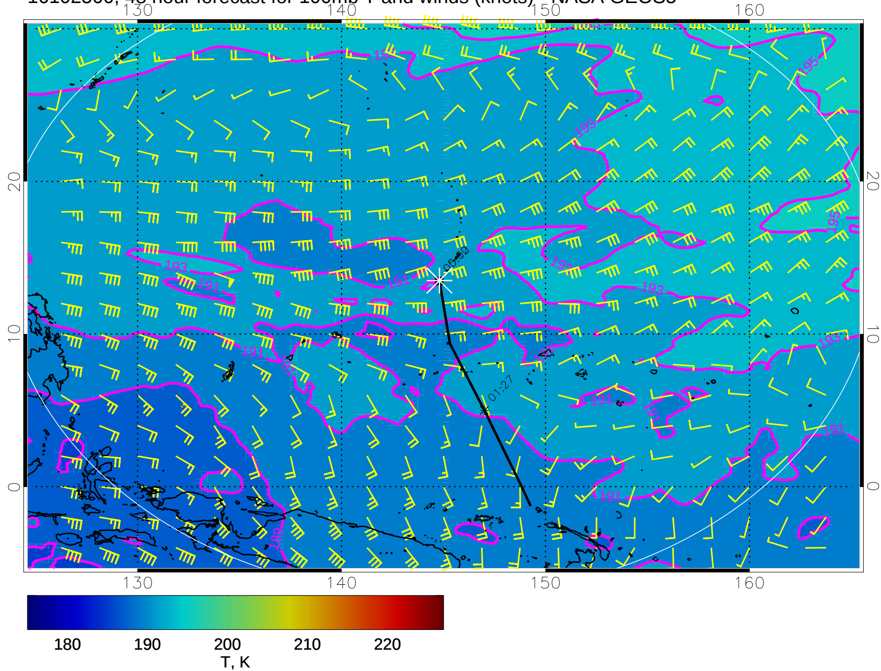
16102500, 48 hour forecast for 100mb T and winds (knots) - NASA GEOS5
