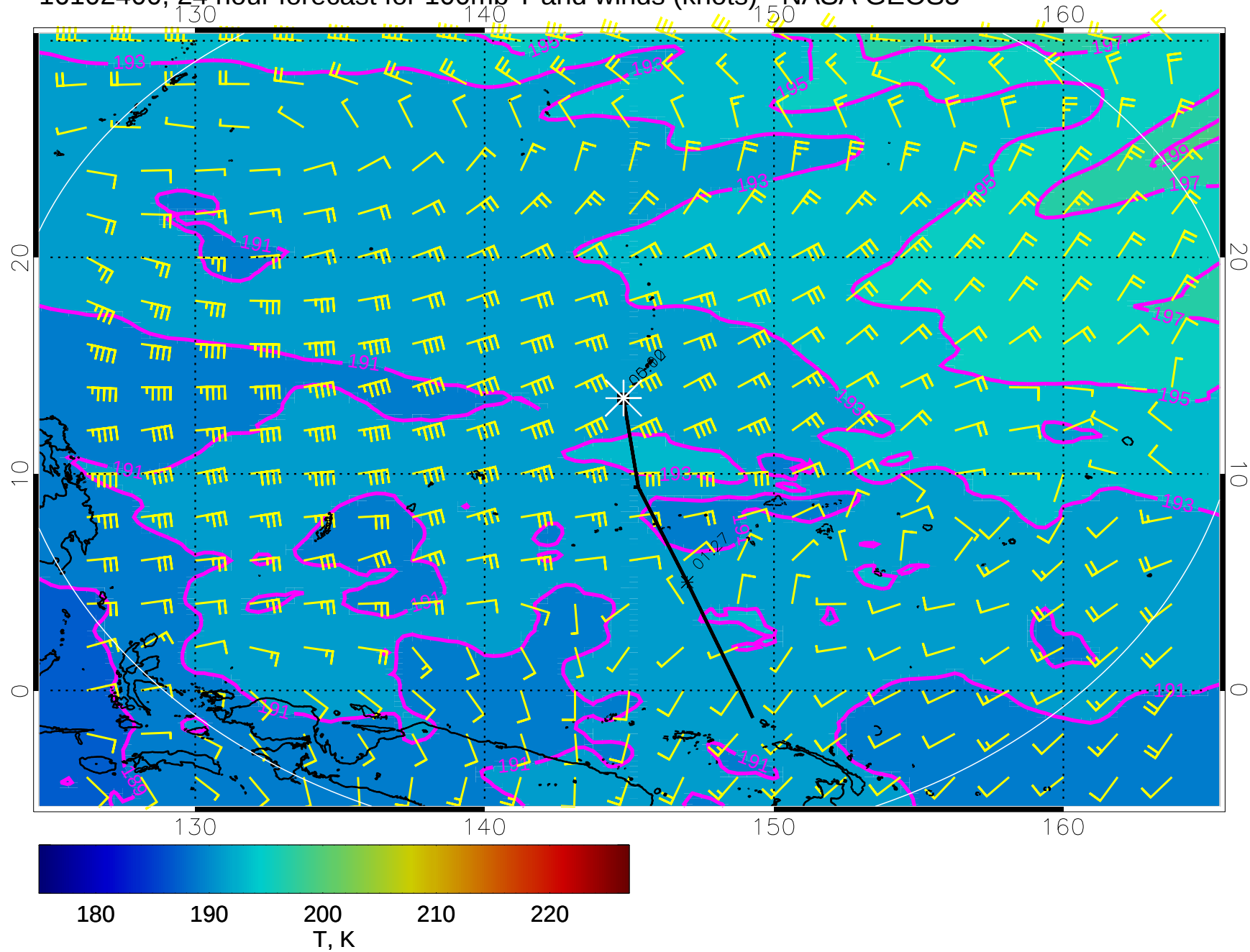
16102400, 24 hour forecast for 100mb T and winds (knots) - NASA GEOS5
