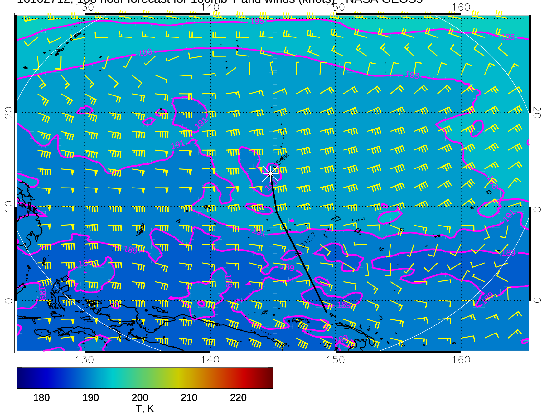
16102712, 108 hour forecast for 100mb T and winds (knots) - NASA GEOS5
