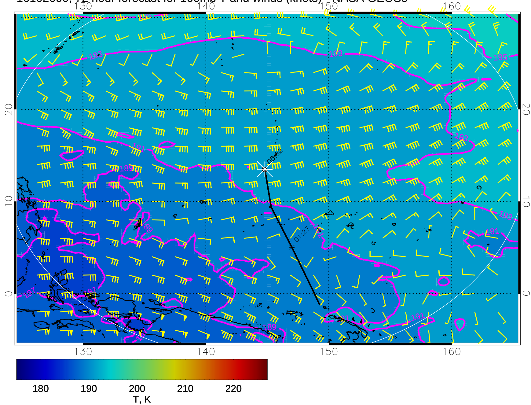
16102600, 72 hour forecast for 100mb T and winds (knots) - NASA GEOS5
