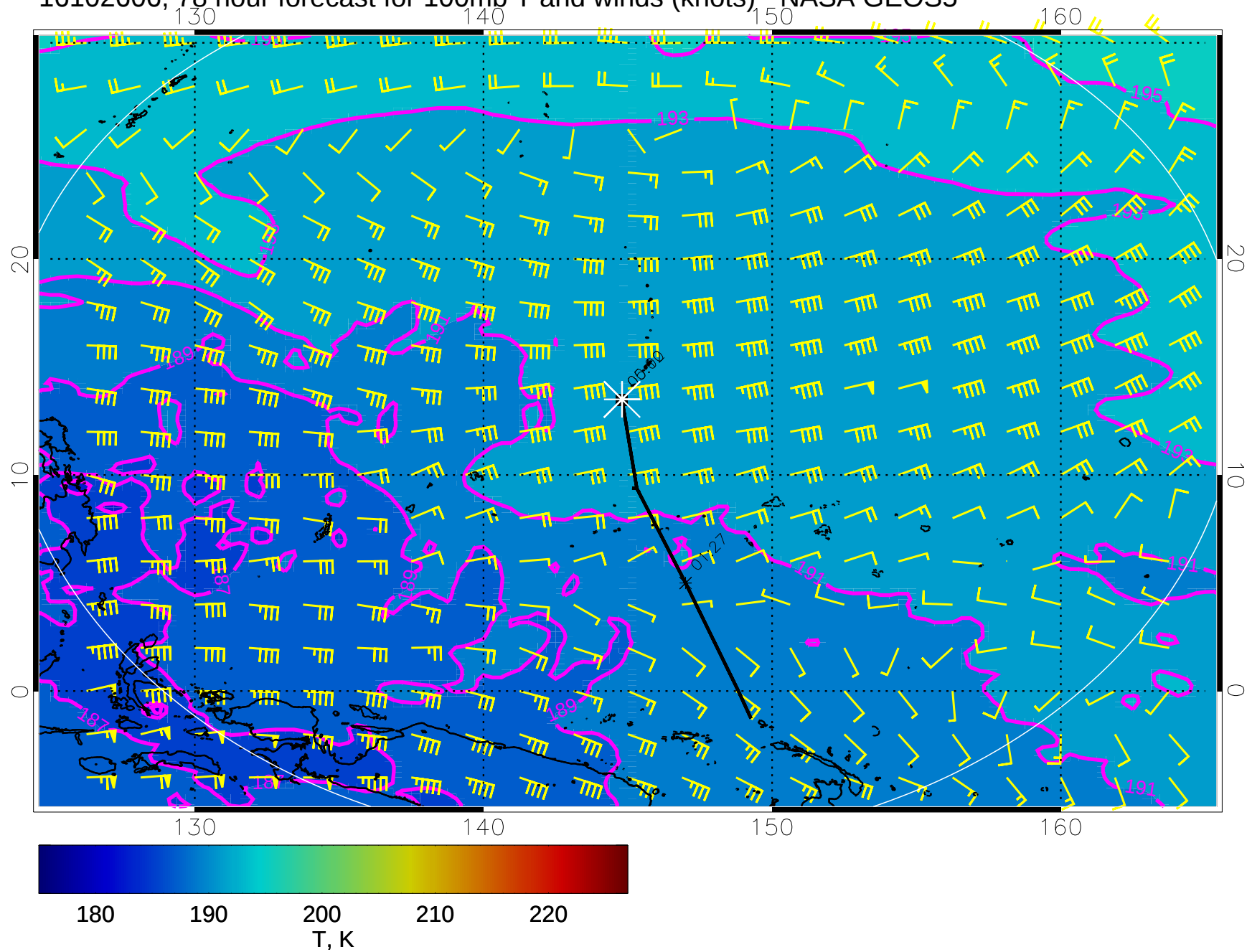
16102606, 78 hour forecast for 100mb T and winds (knots) - NASA GEOS5
