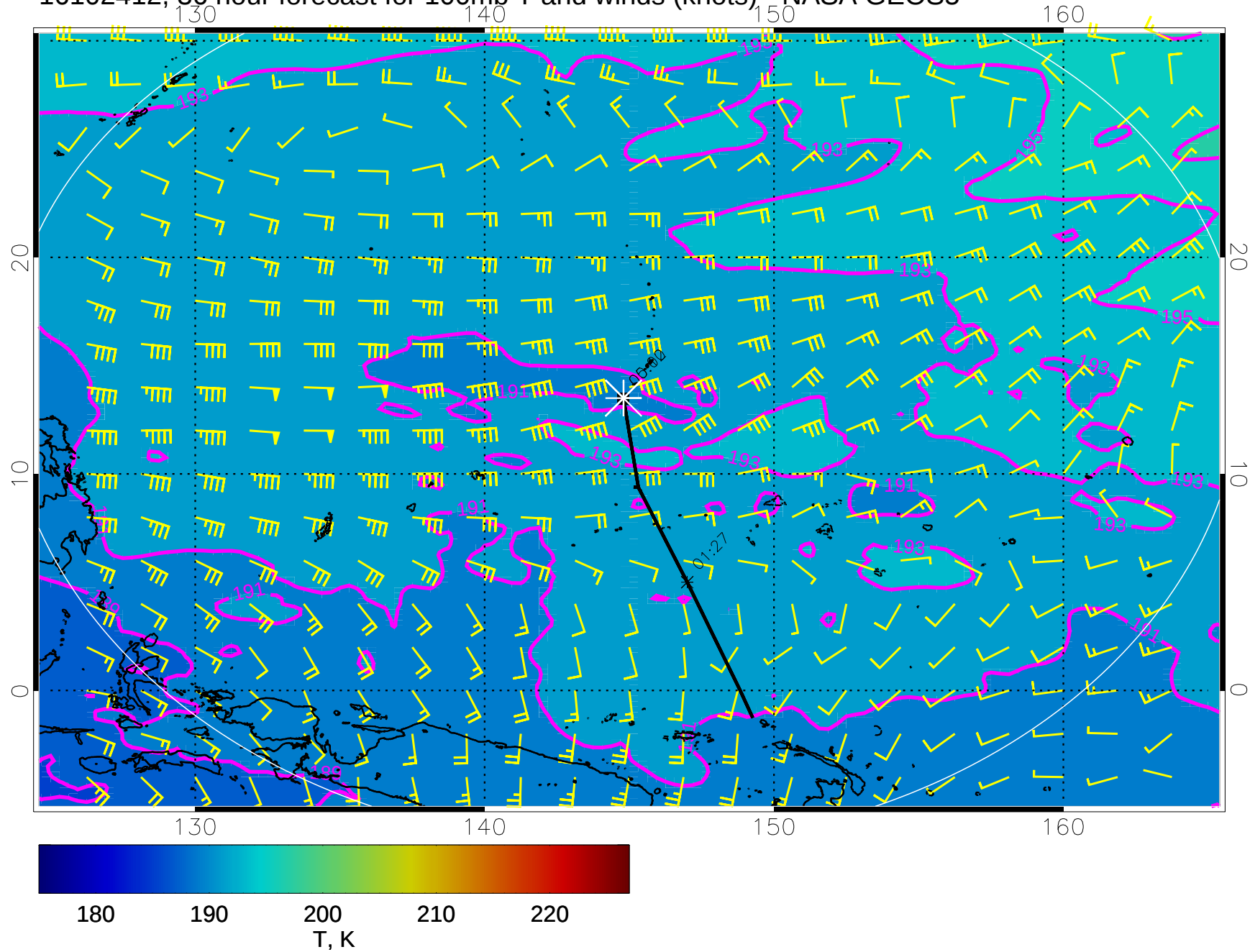
16102412, 36 hour forecast for 100mb T and winds (knots) - NASA GEOS5
