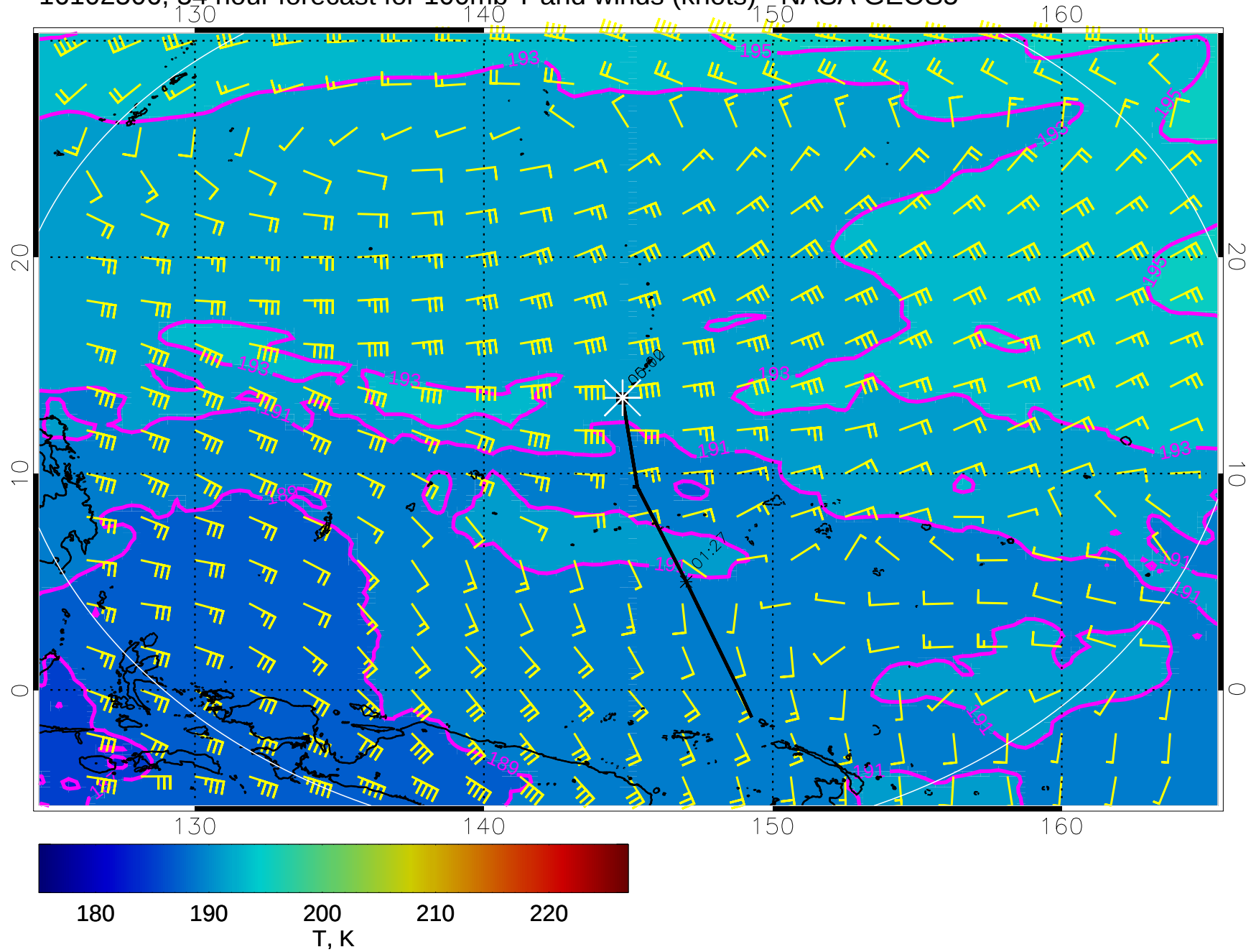
16102506, 54 hour forecast for 100mb T and winds (knots) - NASA GEOS5
