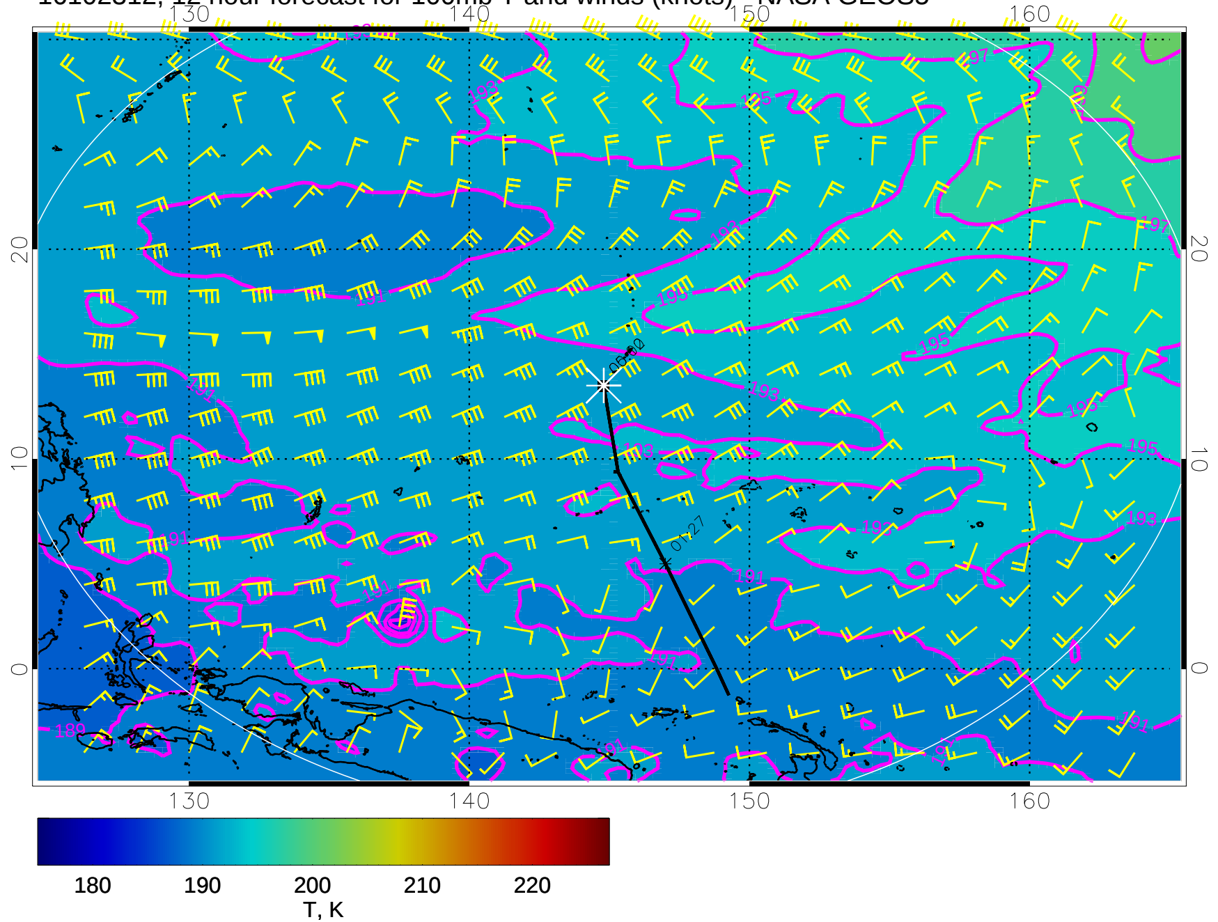
16102312, 12 hour forecast for 100mb T and winds (knots) - NASA GEOS5
