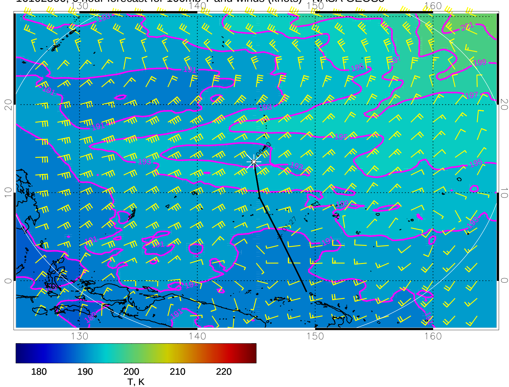
16102306, 6 hour forecast for 100mb T and winds (knots) - NASA GEOS5
