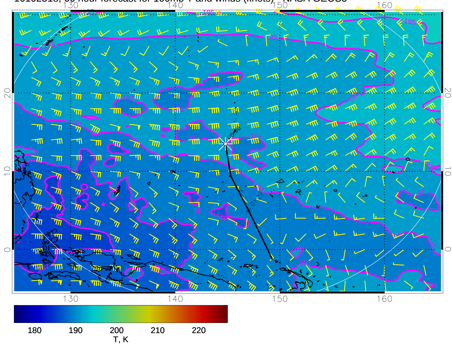
16102518, 66 hour forecast for 100mb T and winds (knots) - NASA GEOS5
