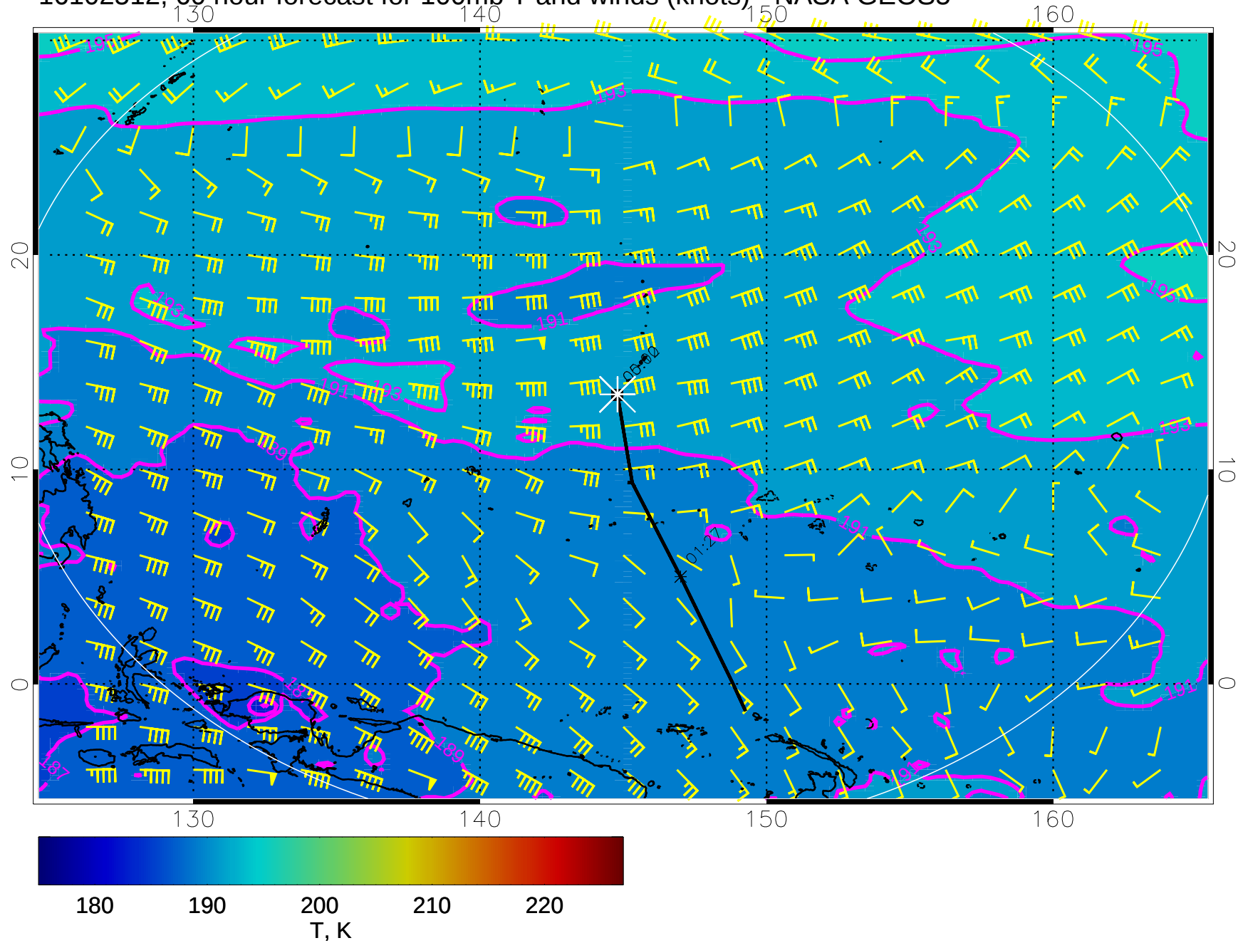
16102512, 60 hour forecast for 100mb T and winds (knots) - NASA GEOS5
