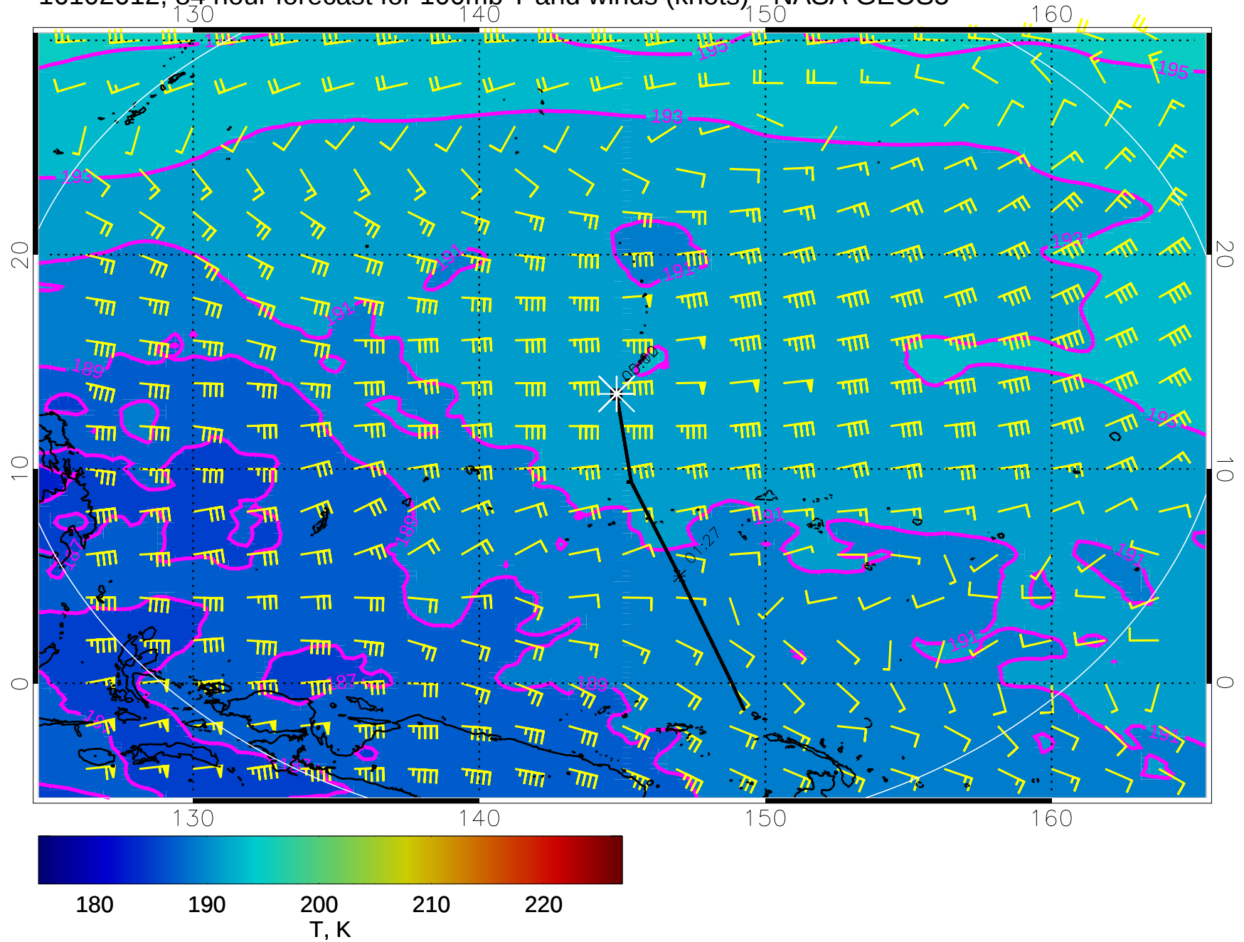
16102612, 84 hour forecast for 100mb T and winds (knots) - NASA GEOS5
