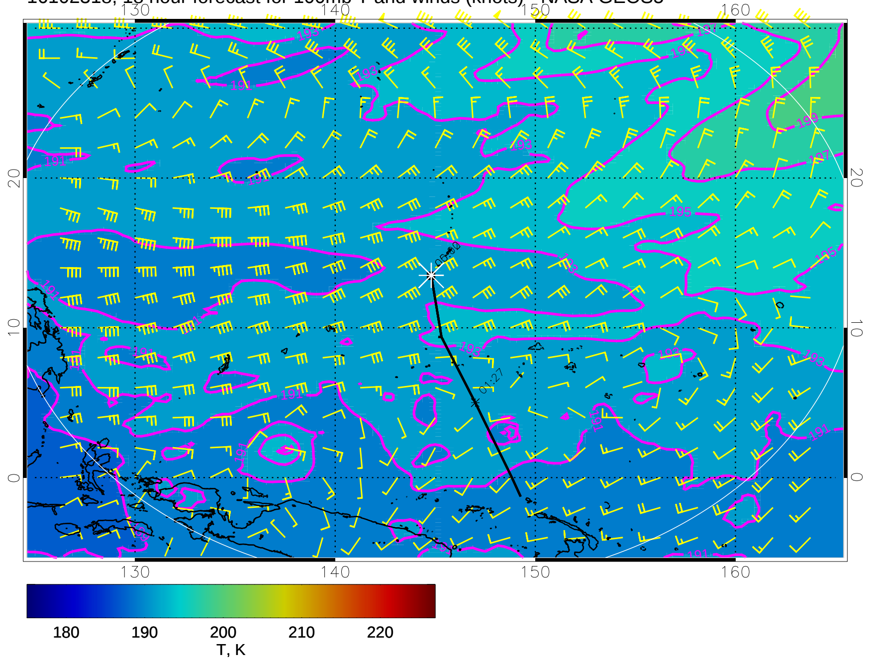
16102318, 18 hour forecast for 100mb T and winds (knots) - NASA GEOS5
