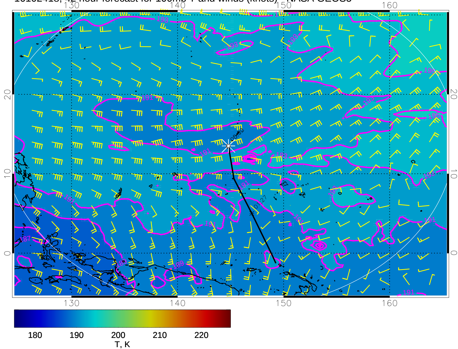
16102418, 42 hour forecast for 100mb T and winds (knots) - NASA GEOS5
