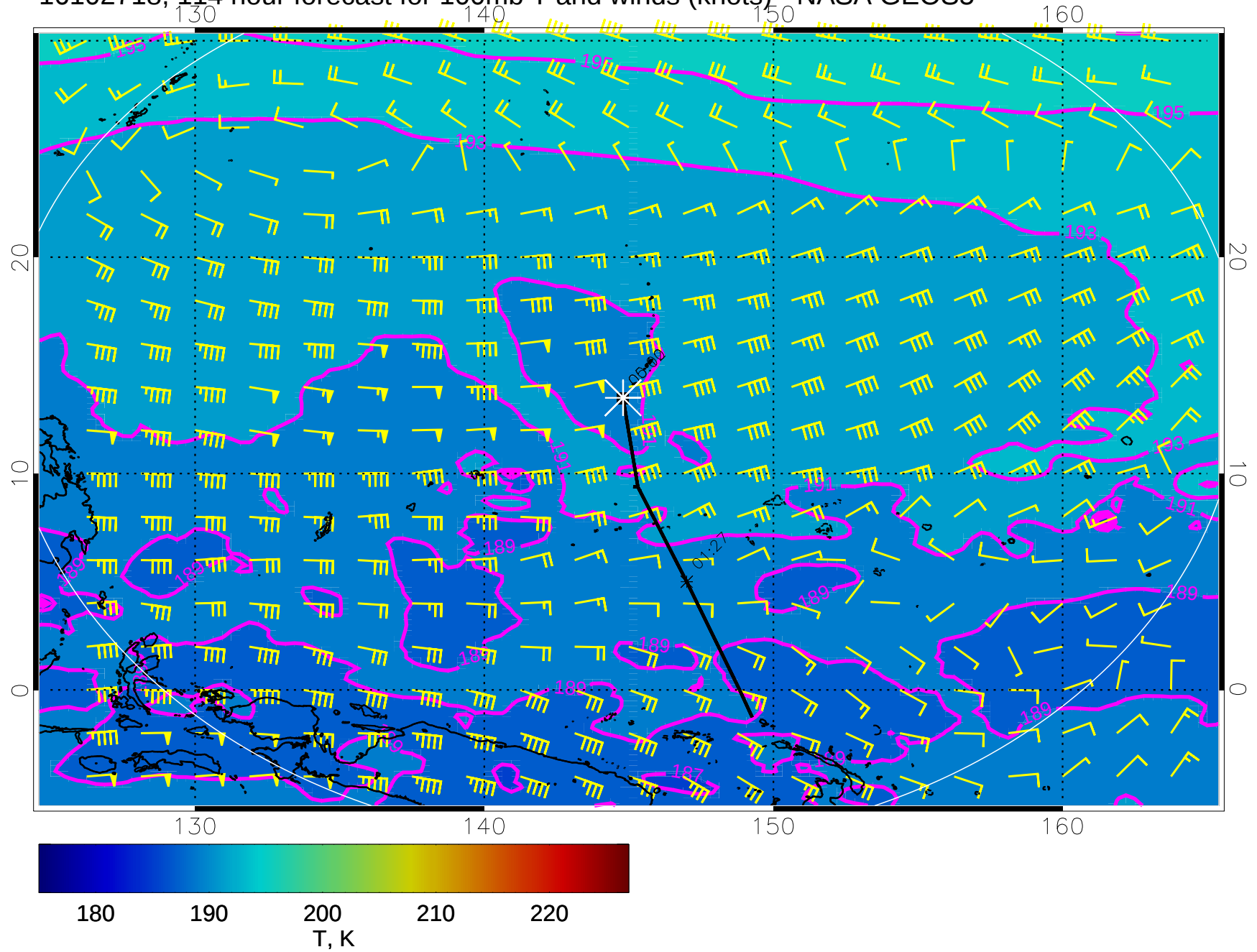
16102718, 114 hour forecast for 100mb T and winds (knots) - NASA GEOS5
