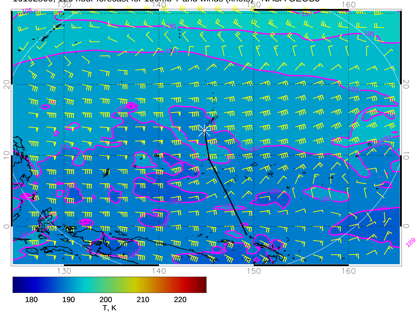
16102800, 120 hour forecast for 100mb T and winds (knots) - NASA GEOS5
