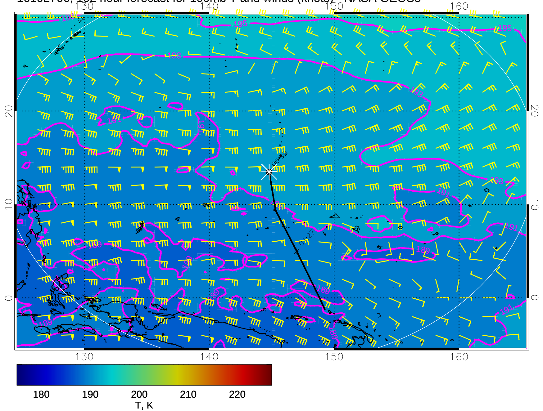
16102706, 102 hour forecast for 100mb T and winds (knots) - NASA GEOS5
