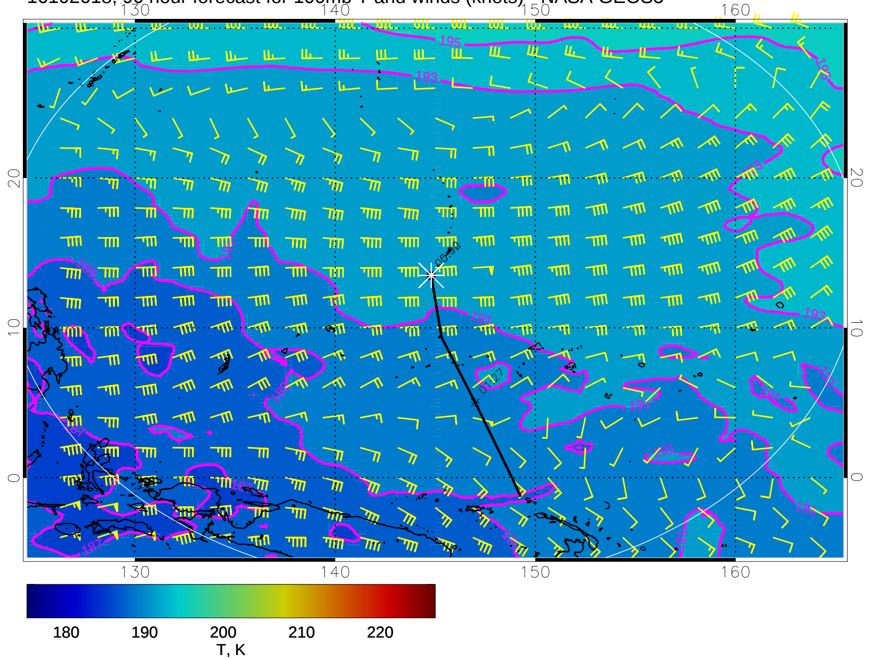
16102618, 90 hour forecast for 100mb T and winds (knots) - NASA GEOS5
