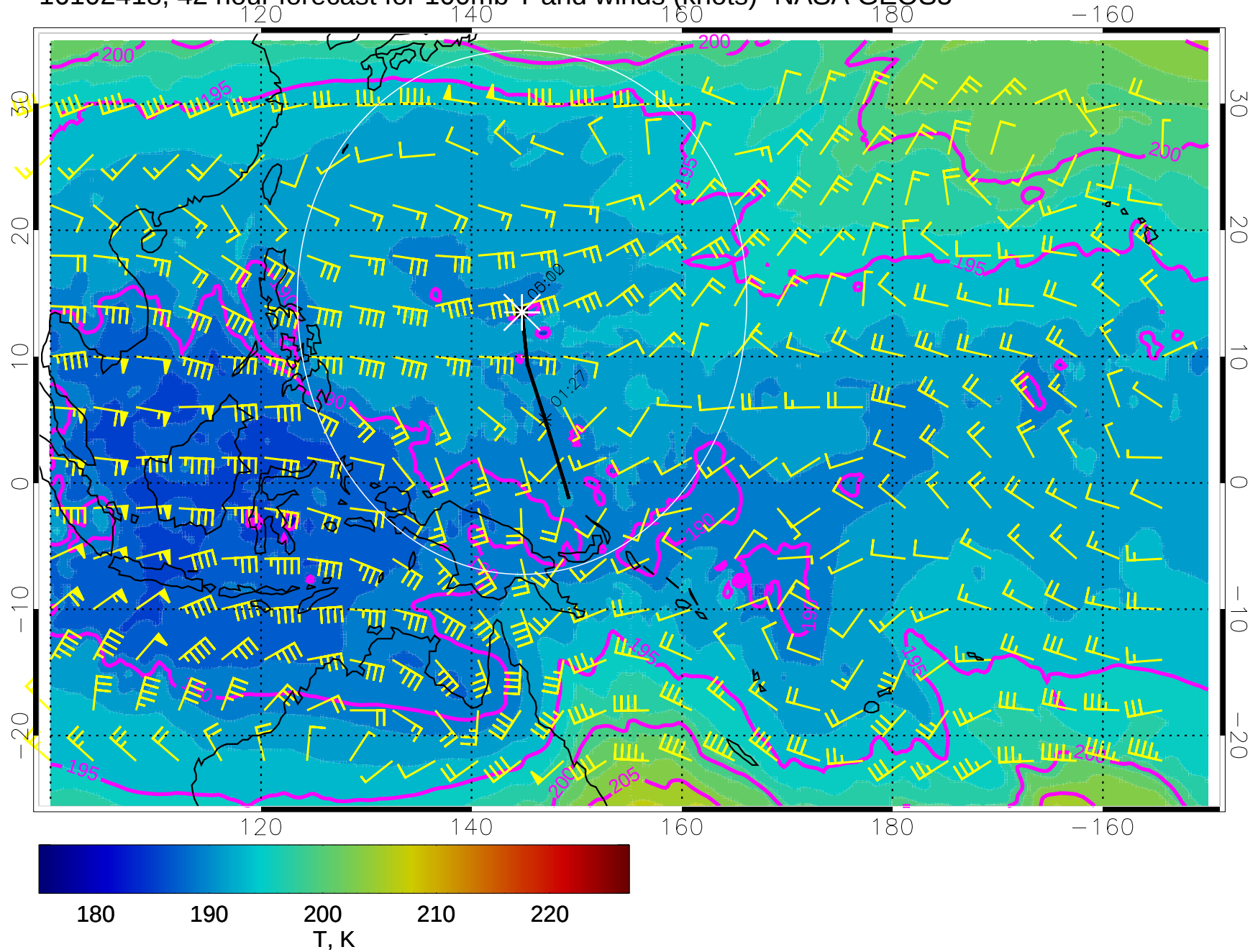
16102418, 42 hour forecast for 100mb T and winds (knots)- NASA GEOS5
