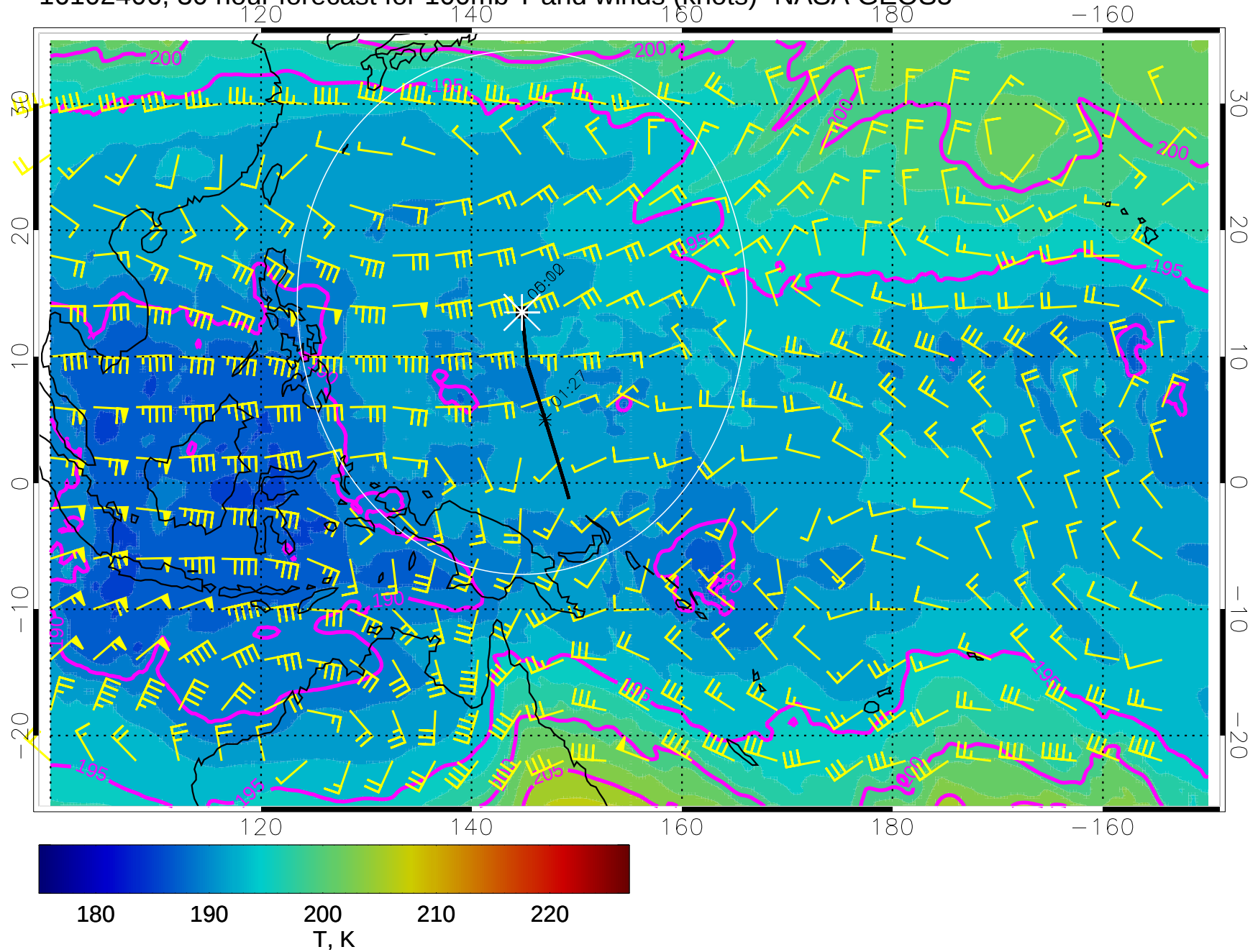
16102406, 30 hour forecast for 100mb T and winds (knots)- NASA GEOS5
