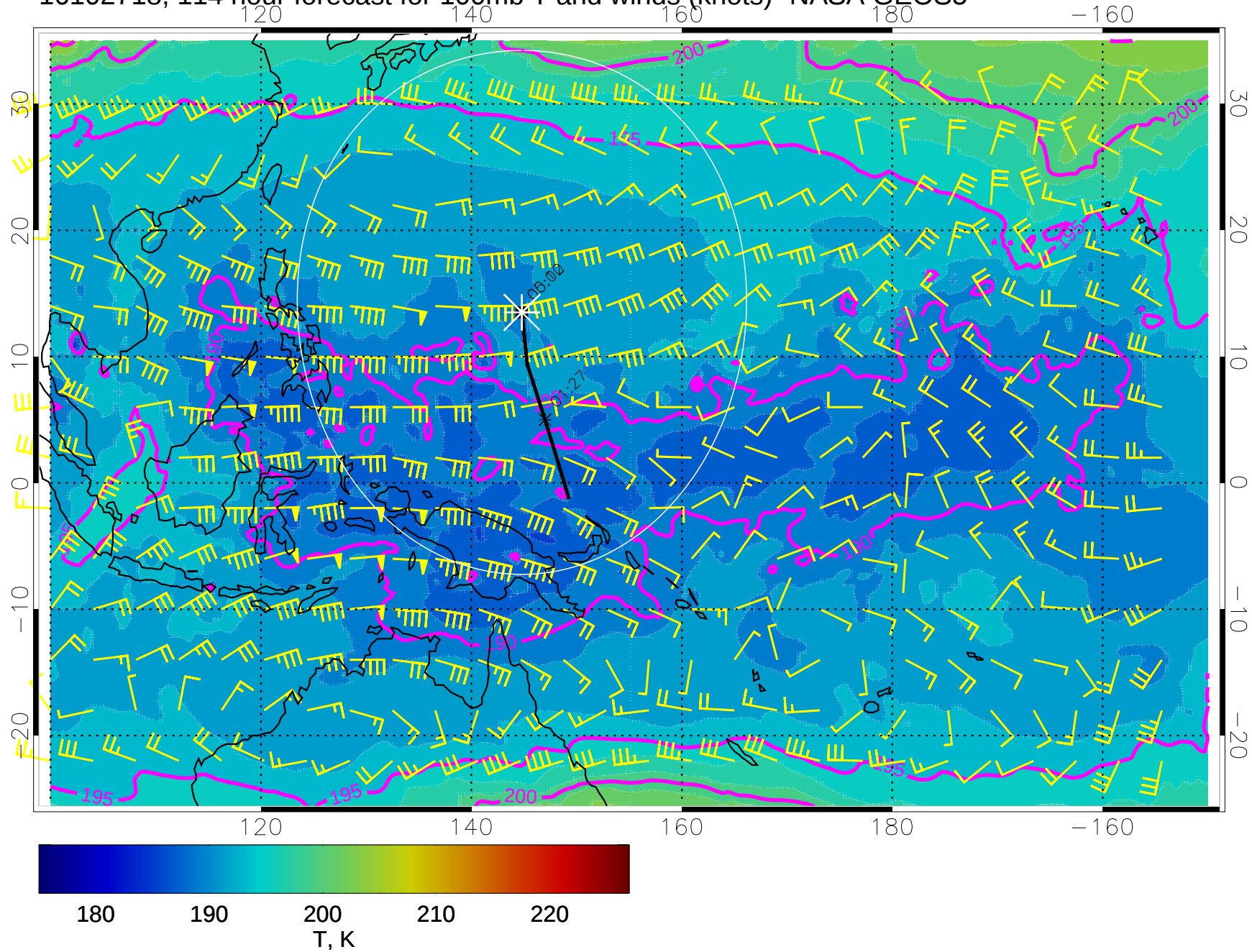
16102718, 114 hour forecast for 100mb T and winds (knots)- NASA GEOS5
