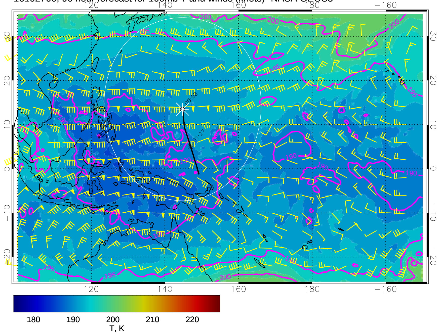
16102700, 96 hour forecast for 100mb T and winds (knots)- NASA GEOS5
