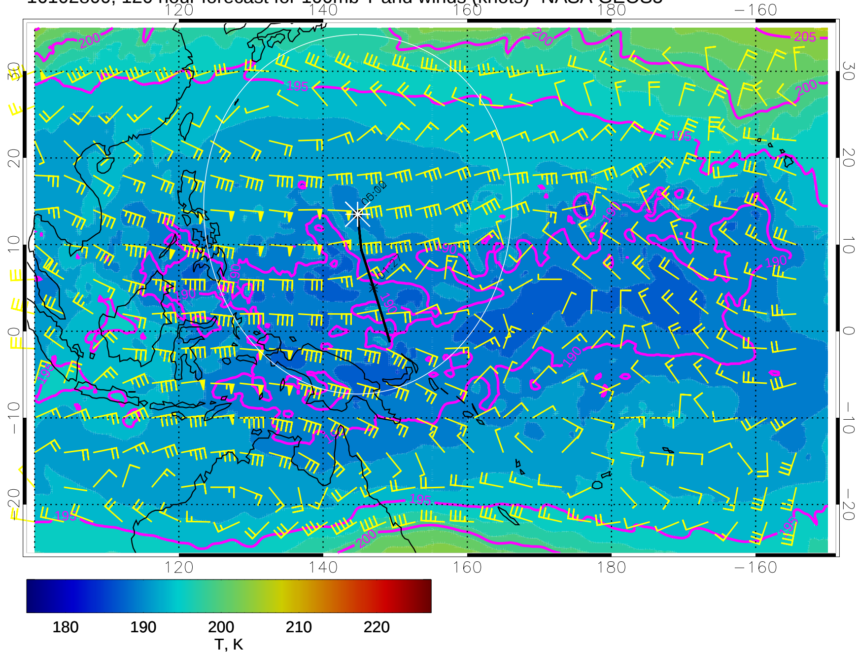
16102800, 120 hour forecast for 100mb T and winds (knots)- NASA GEOS5
