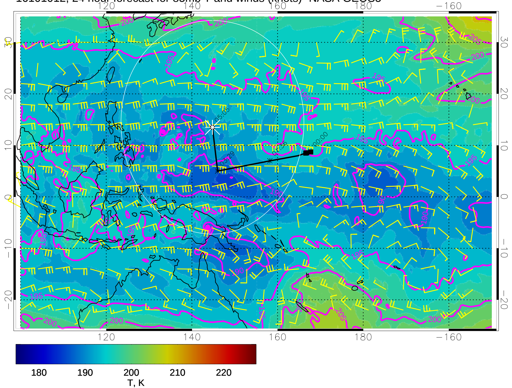
16101012, 24 hour forecast for 85mb T and winds (knots)- NASA GEOS5
