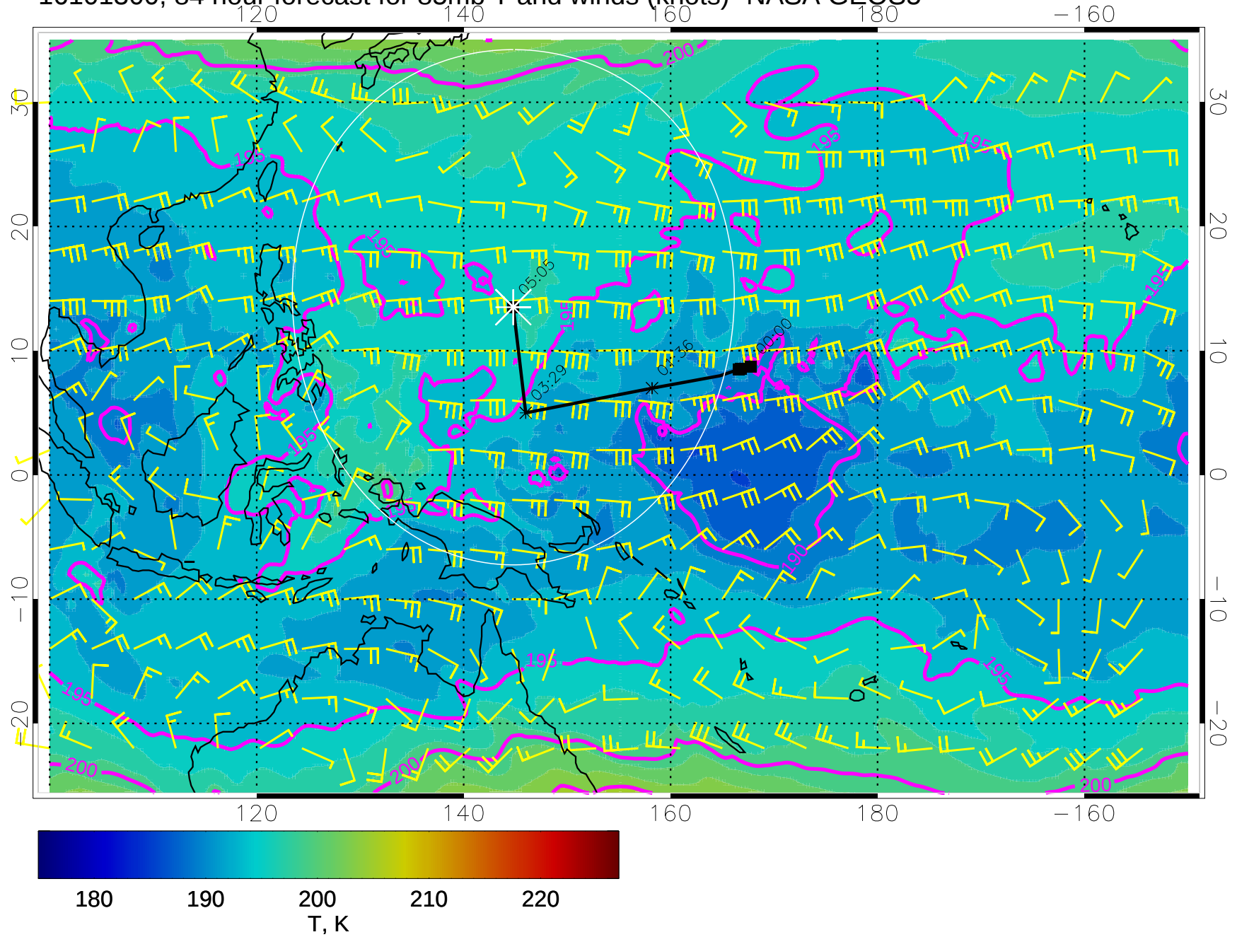
16101300, 84 hour forecast for 85mb T and winds (knots)- NASA GEOS5
