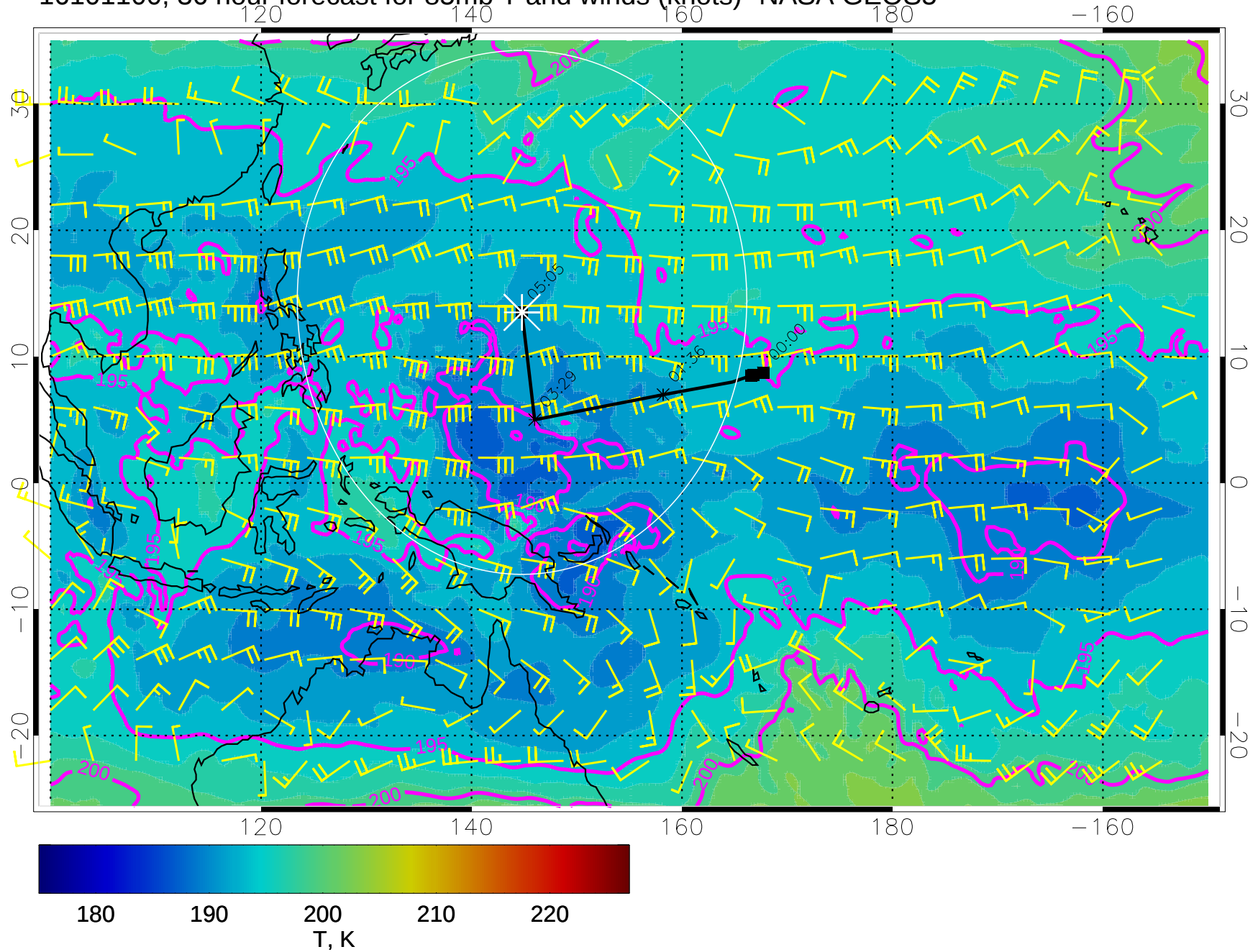
16101100, 36 hour forecast for 85mb T and winds (knots)- NASA GEOS5
