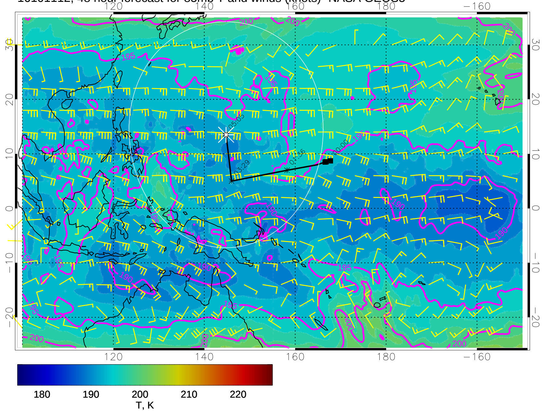
16101112, 48 hour forecast for 85mb T and winds (knots)- NASA GEOS5
