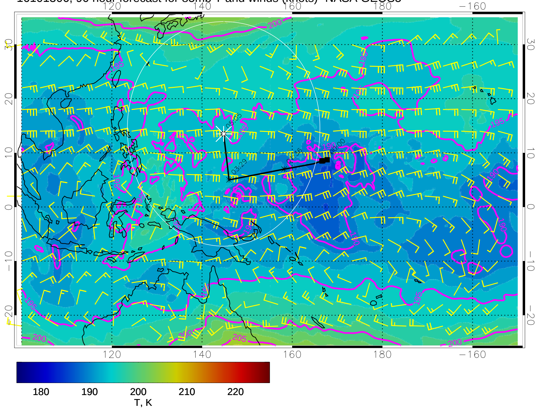
16101306, 90 hour forecast for 85mb T and winds (knots)- NASA GEOS5
