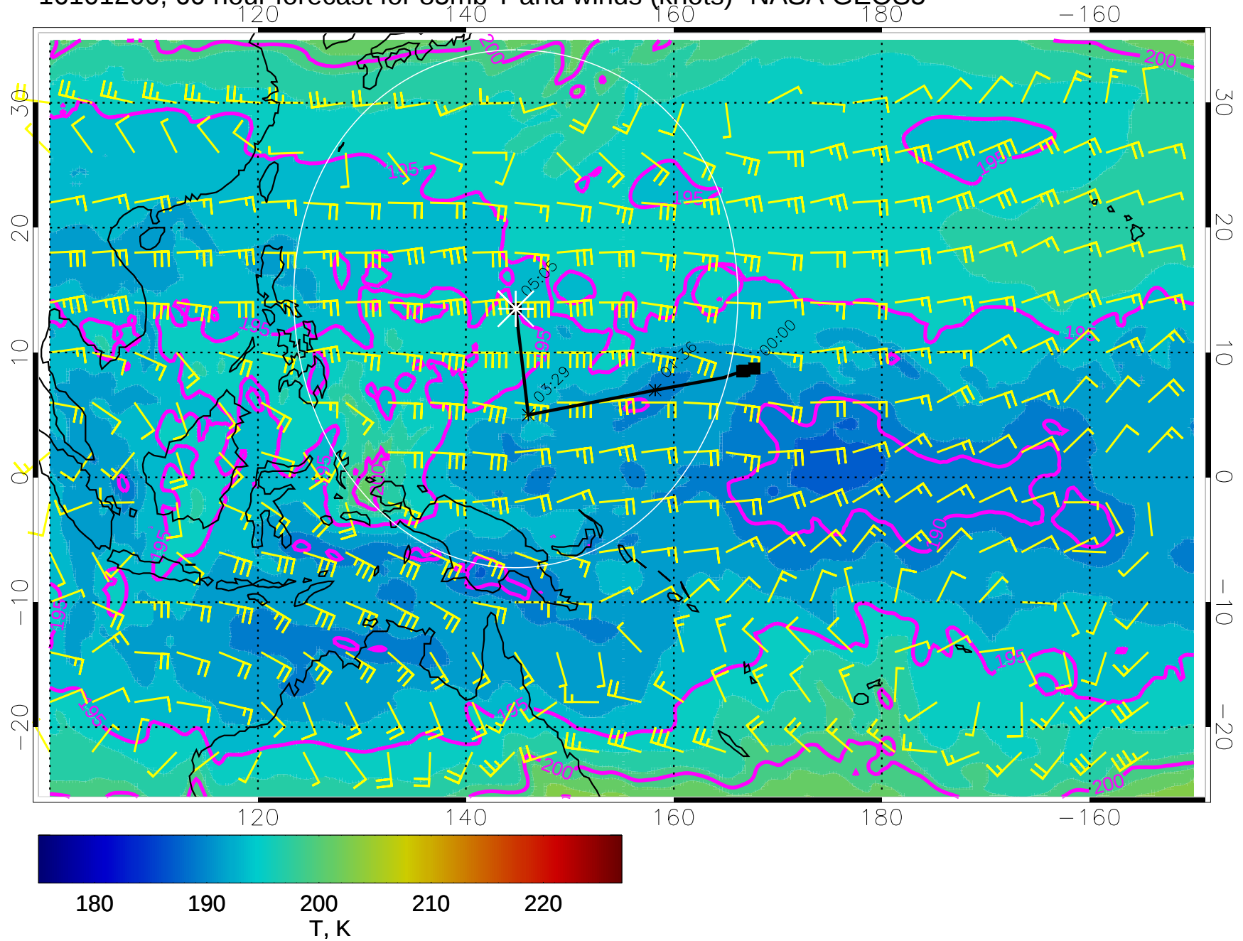
16101200, 60 hour forecast for 85mb T and winds (knots)- NASA GEOS5
