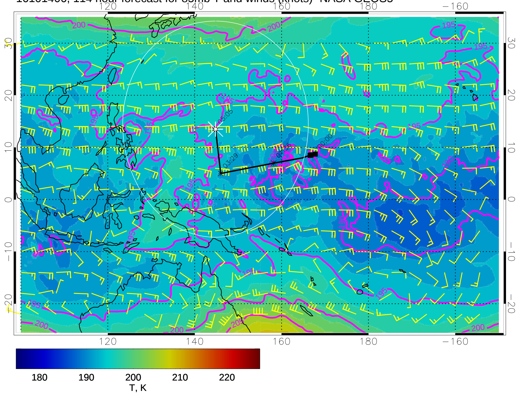
16101406, 114 hour forecast for 85mb T and winds (knots)- NASA GEOS5
