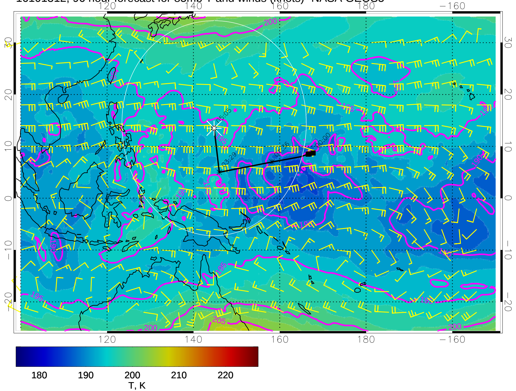
16101312, 96 hour forecast for 85mb T and winds (knots)- NASA GEOS5
