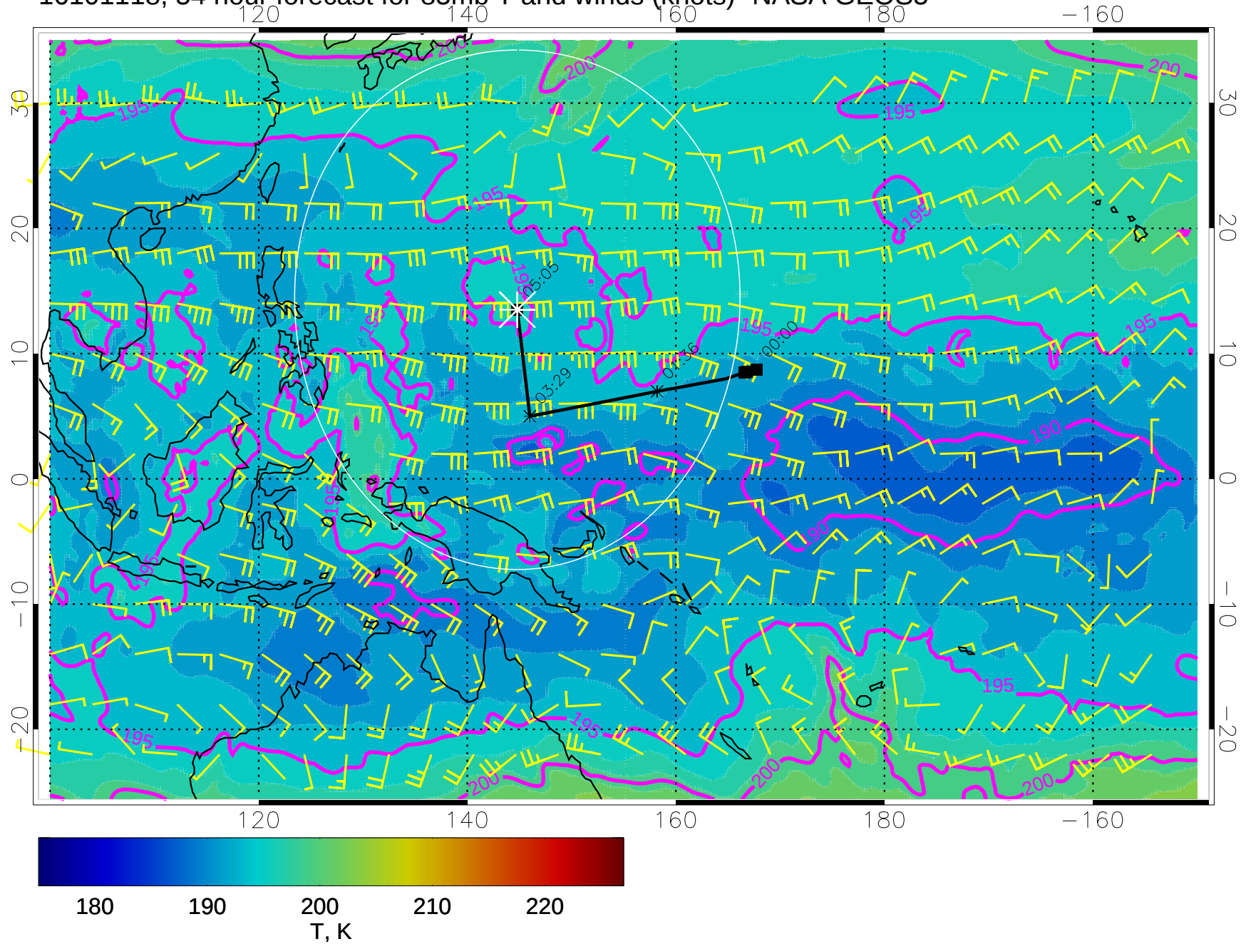
16101118, 54 hour forecast for 85mb T and winds (knots)- NASA GEOS5
