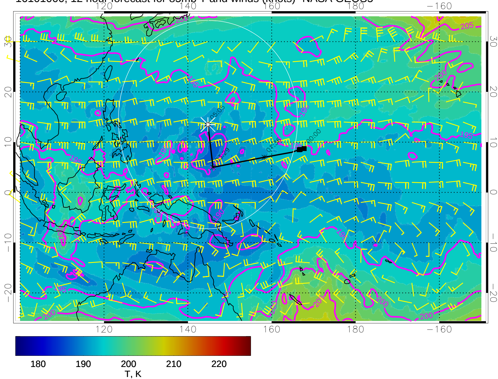
16101000, 12 hour forecast for 85mb T and winds (knots)- NASA GEOS5
