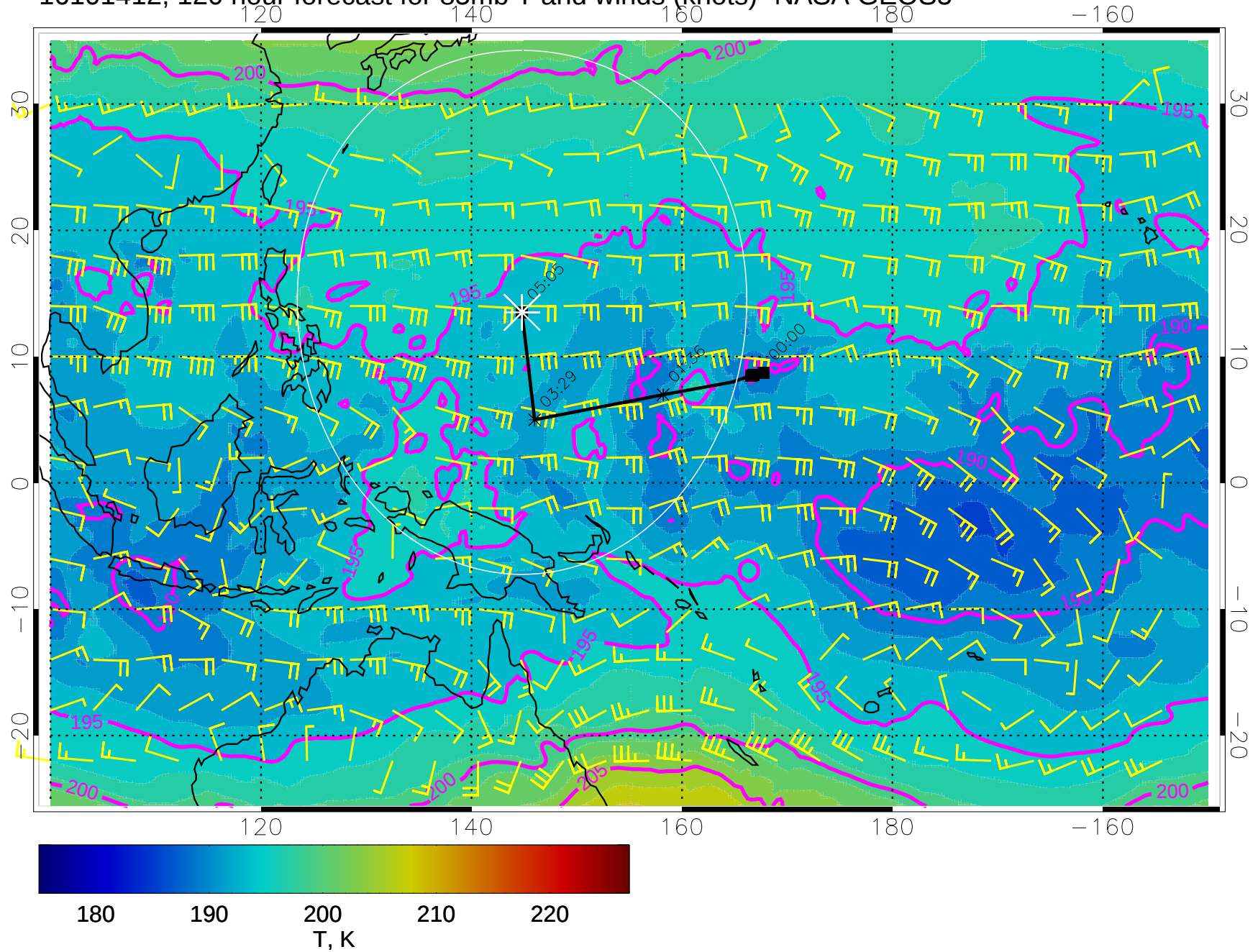
16101412, 120 hour forecast for 85mb T and winds (knots)- NASA GEOS5
