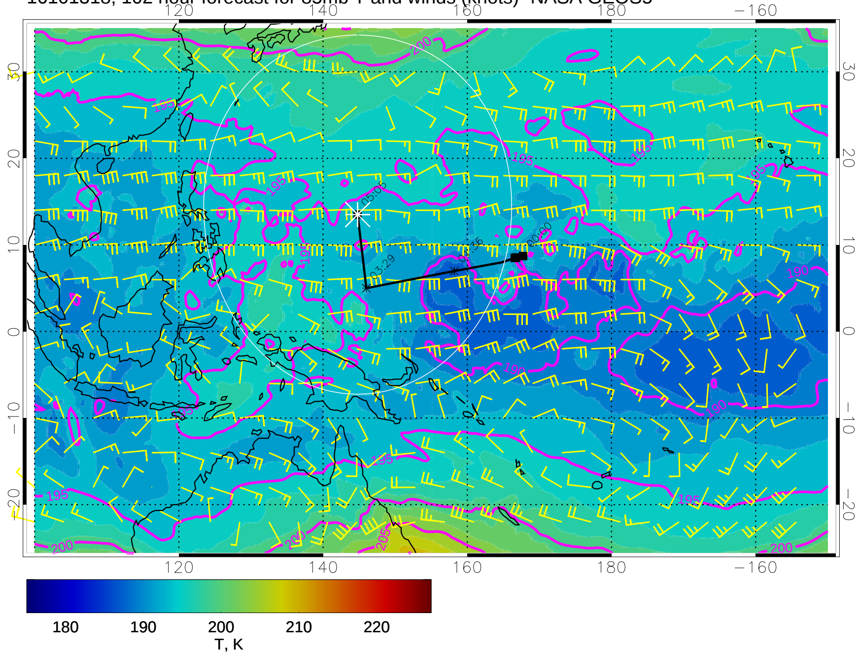
16101318, 102 hour forecast for 85mb T and winds (knots)- NASA GEOS5
