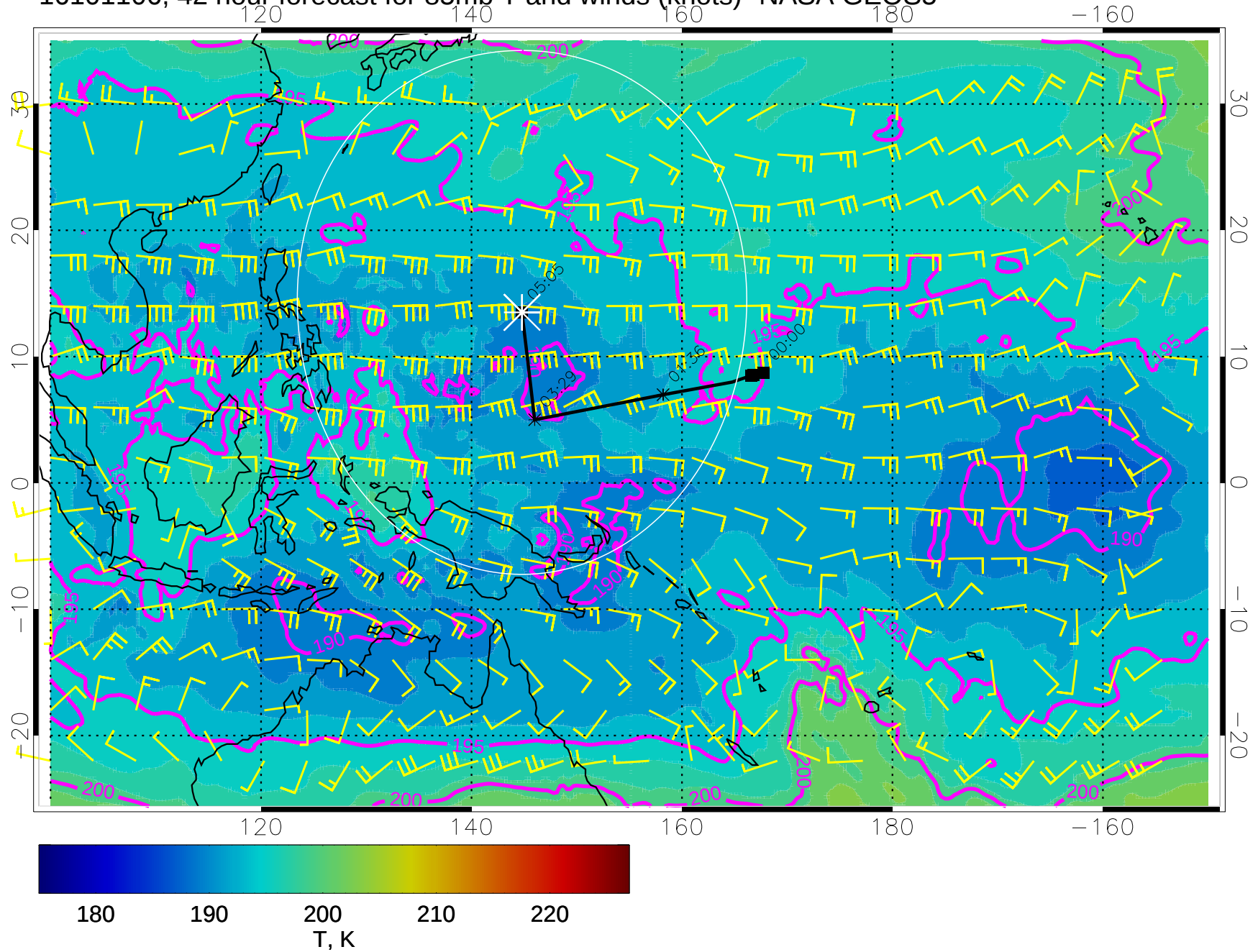
16101106, 42 hour forecast for 85mb T and winds (knots)- NASA GEOS5
