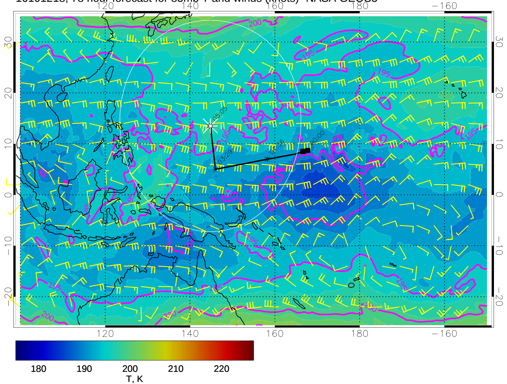
16101218, 78 hour forecast for 85mb T and winds (knots)- NASA GEOS5
