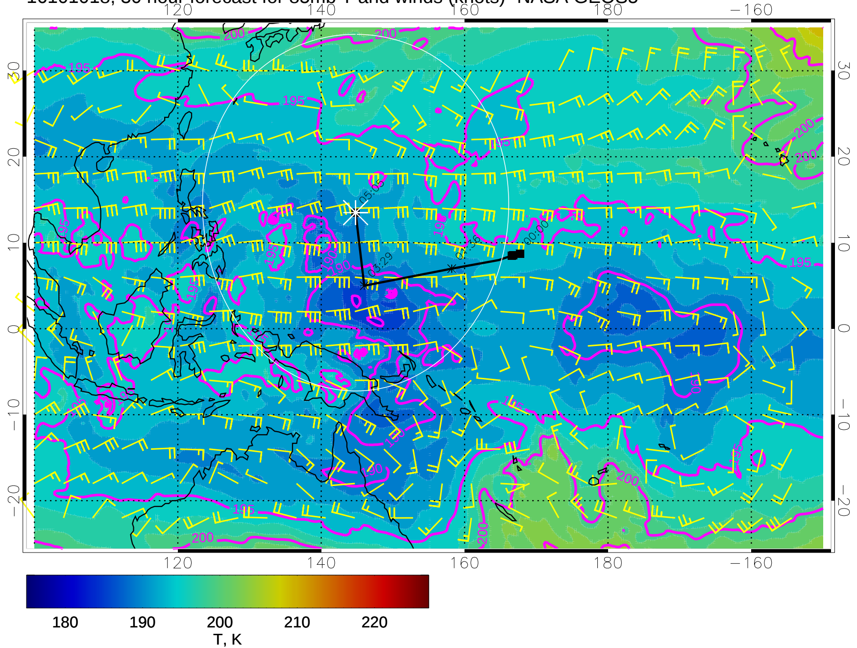
16101018, 30 hour forecast for 85mb T and winds (knots)- NASA GEOS5
