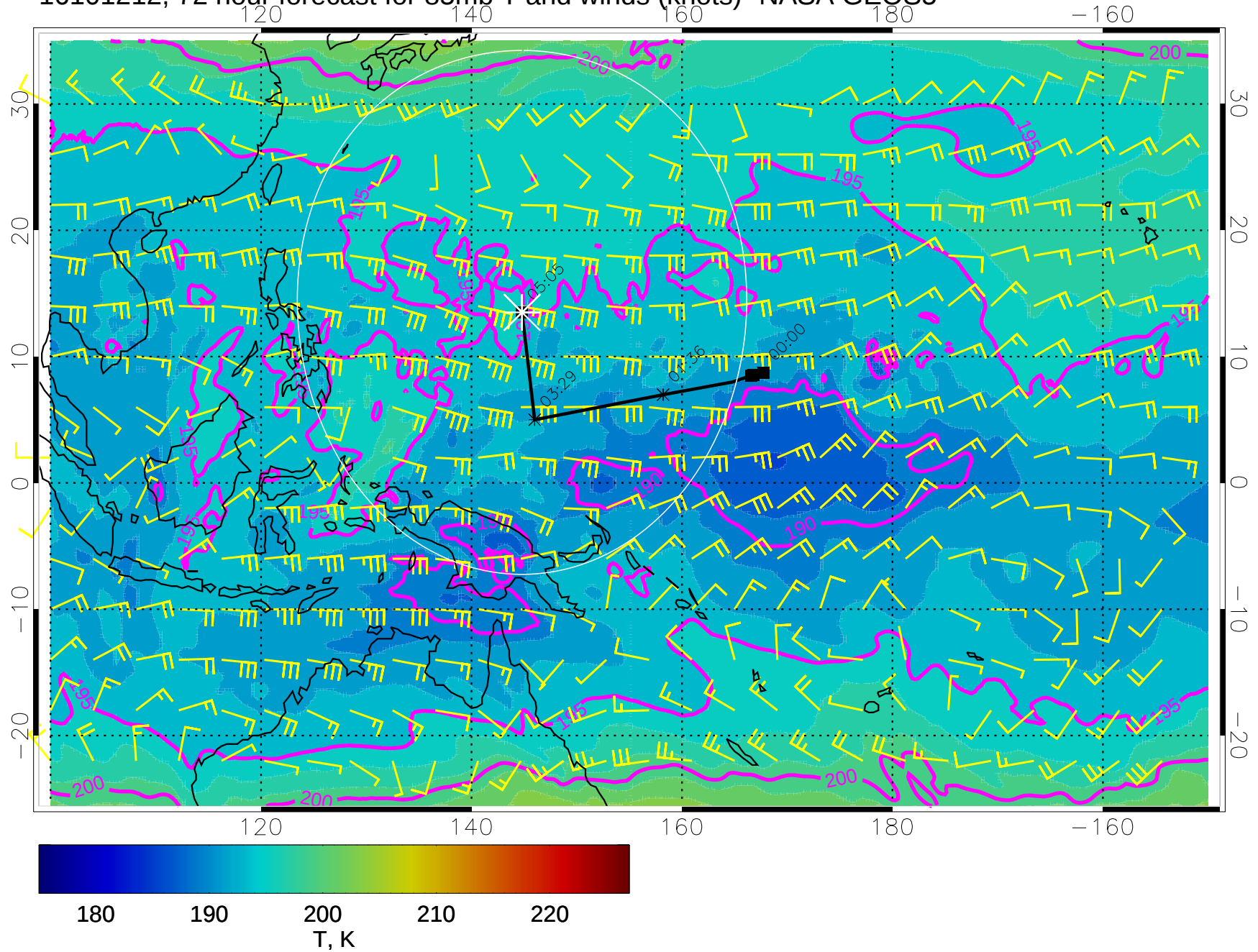
16101212, 72 hour forecast for 85mb T and winds (knots)- NASA GEOS5
