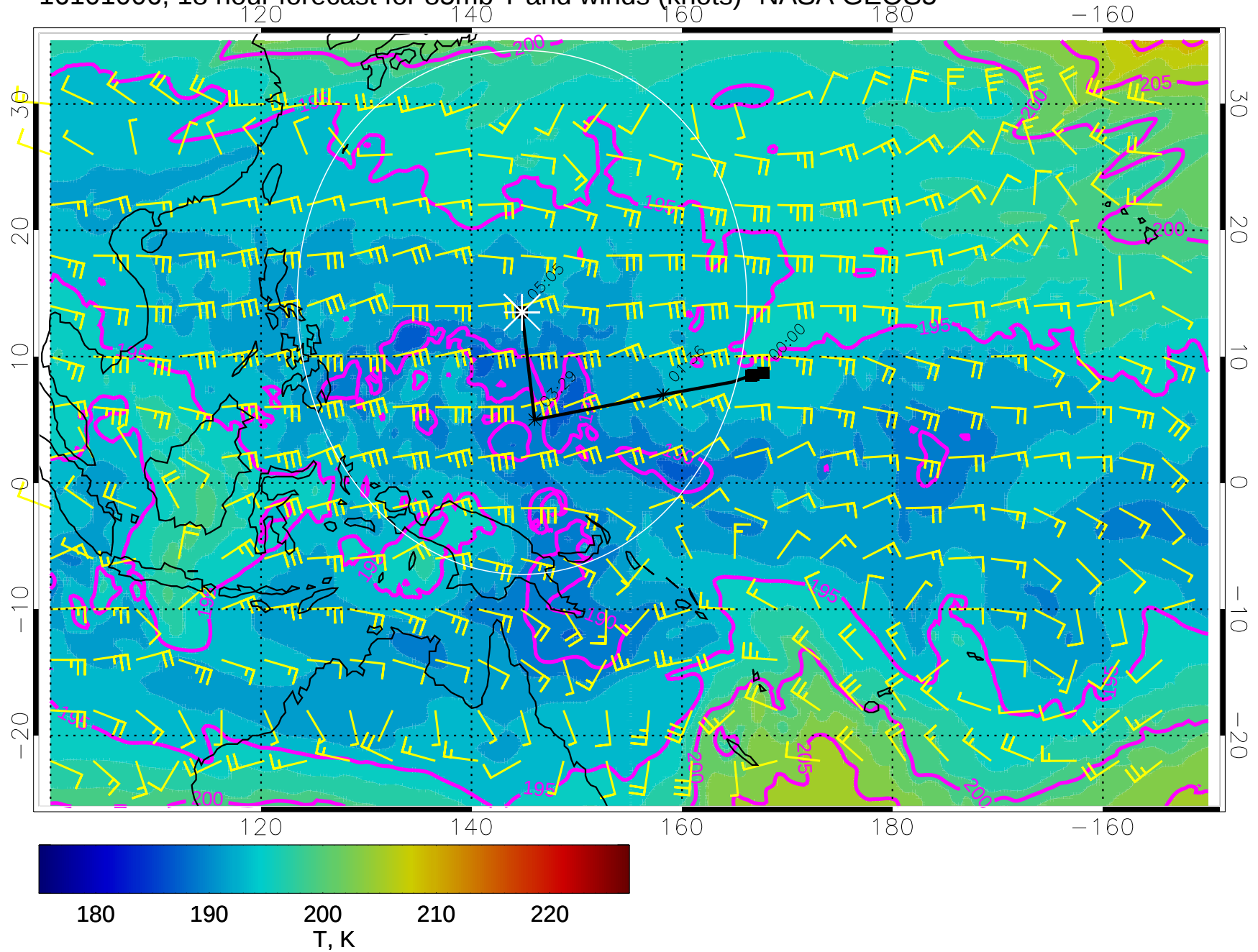
16101006, 18 hour forecast for 85mb T and winds (knots)- NASA GEOS5
