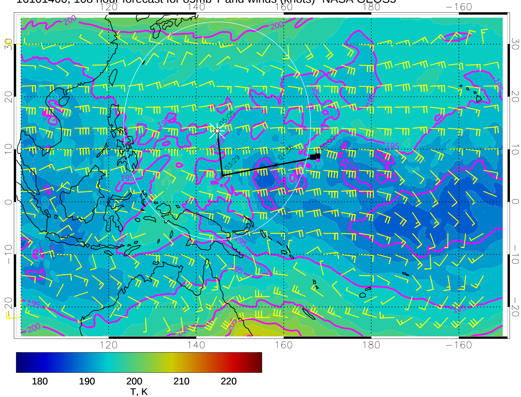
16101400, 108 hour forecast for 85mb T and winds (knots)- NASA GEOS5
