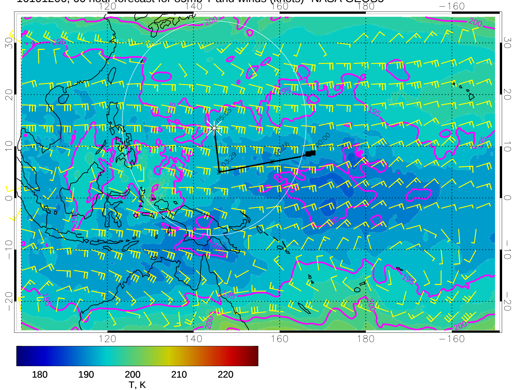
16101206, 66 hour forecast for 85mb T and winds (knots)- NASA GEOS5
