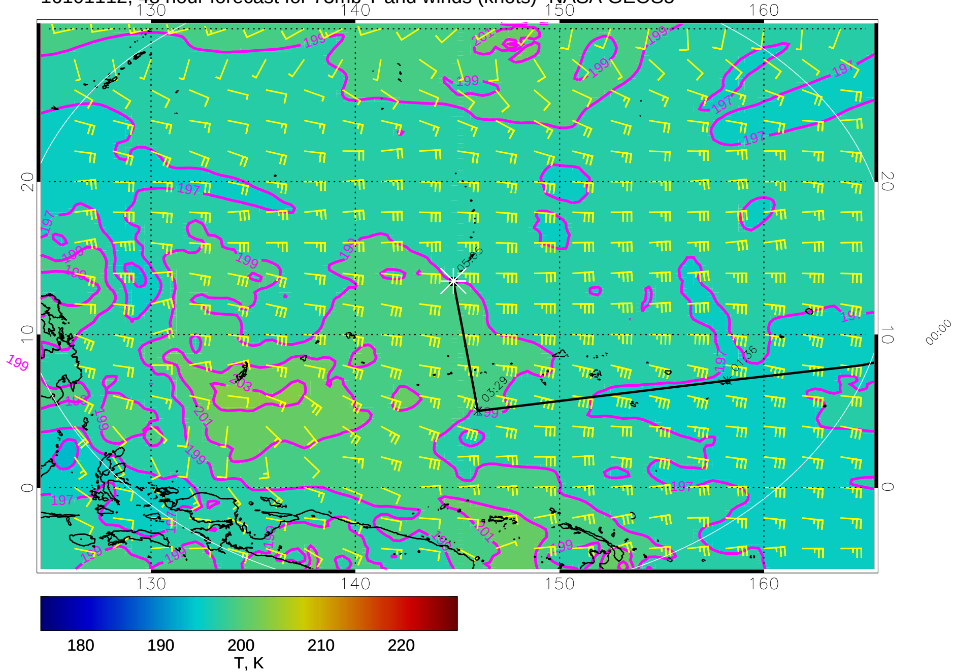
16101112, 48 hour forecast for 73mb T and winds (knots)- NASA GEOS5
