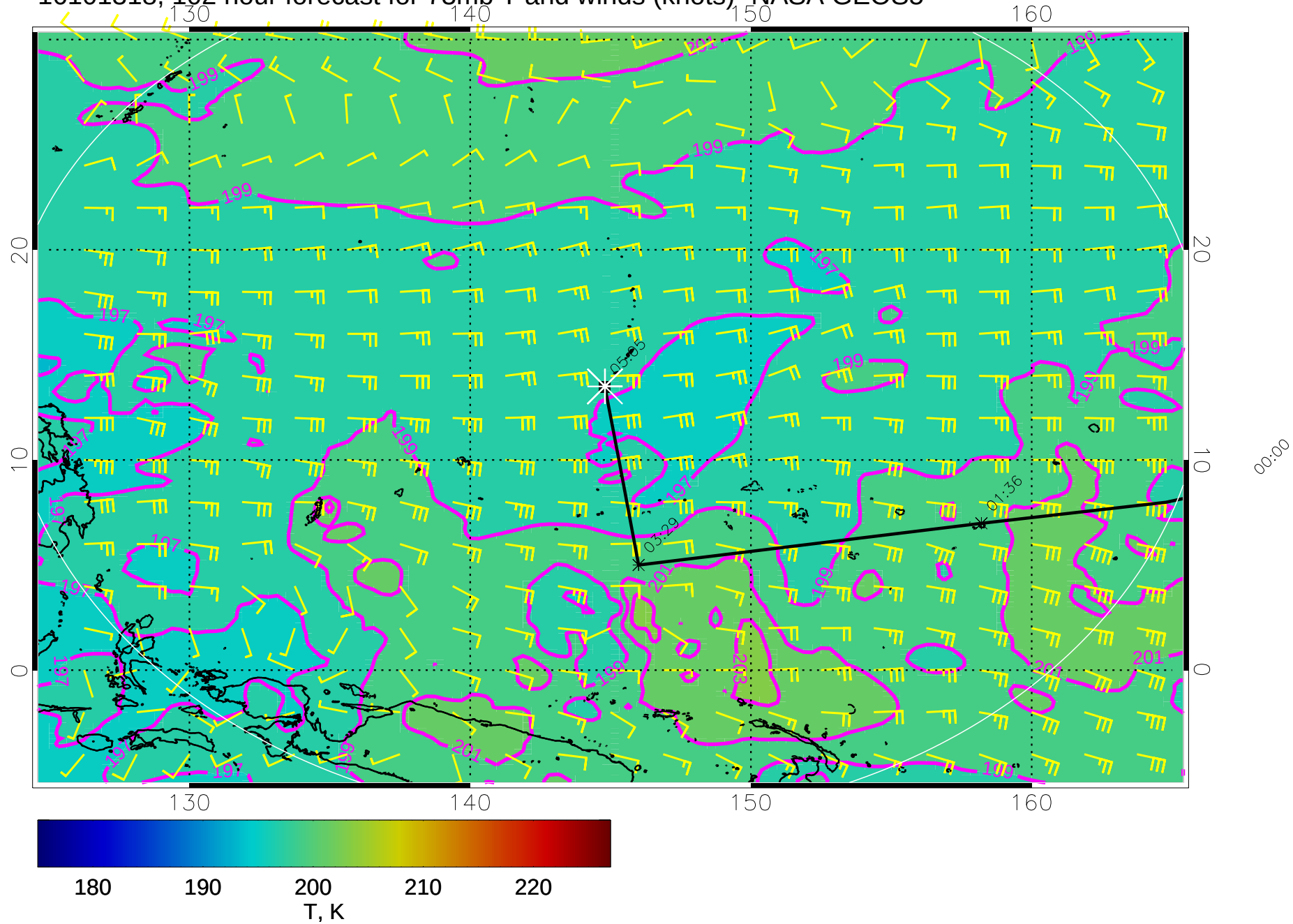
16101318, 102 hour forecast for 73mb T and winds (knots)- NASA GEOS5
