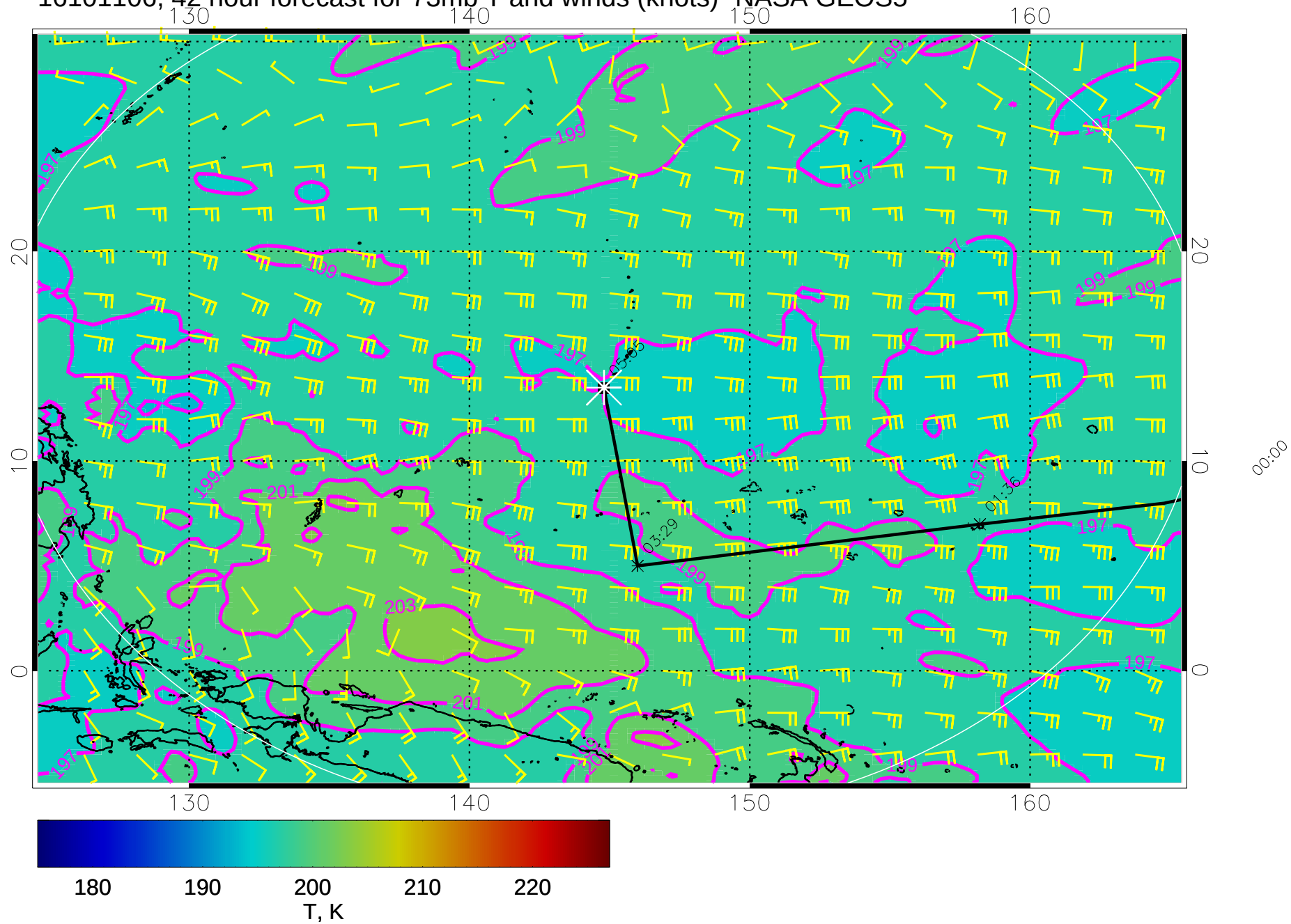
16101106, 42 hour forecast for 73mb T and winds (knots)- NASA GEOS5
