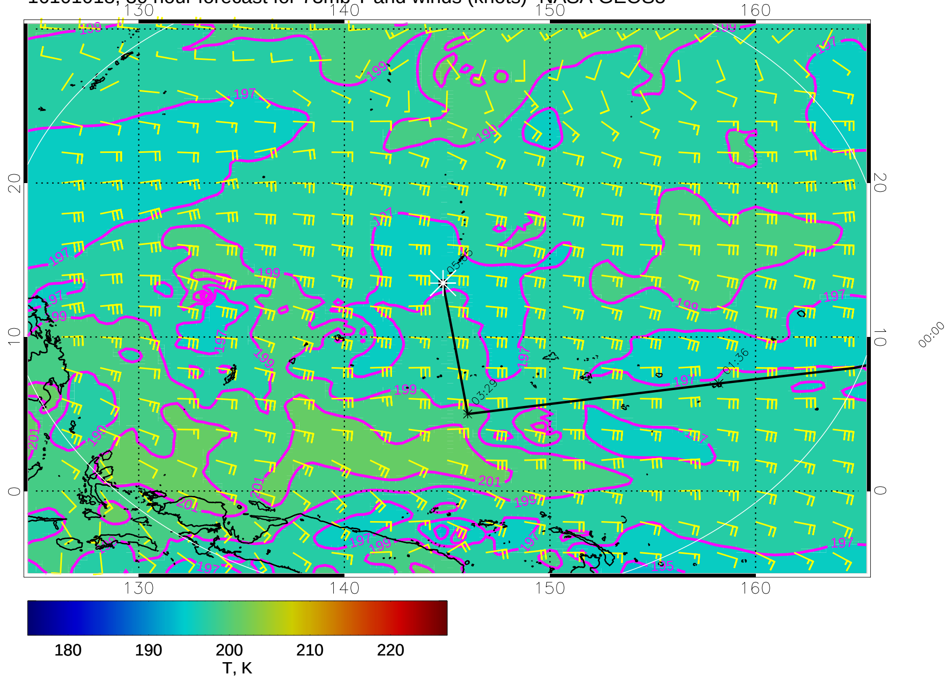
16101018, 30 hour forecast for 73mb T and winds (knots)- NASA GEOS5
