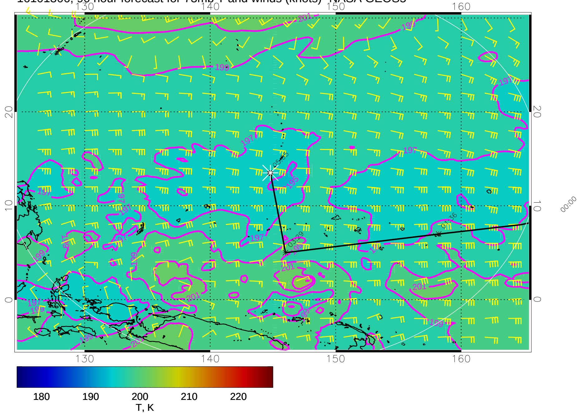
16101306, 90 hour forecast for 73mb T and winds (knots)- NASA GEOS5
