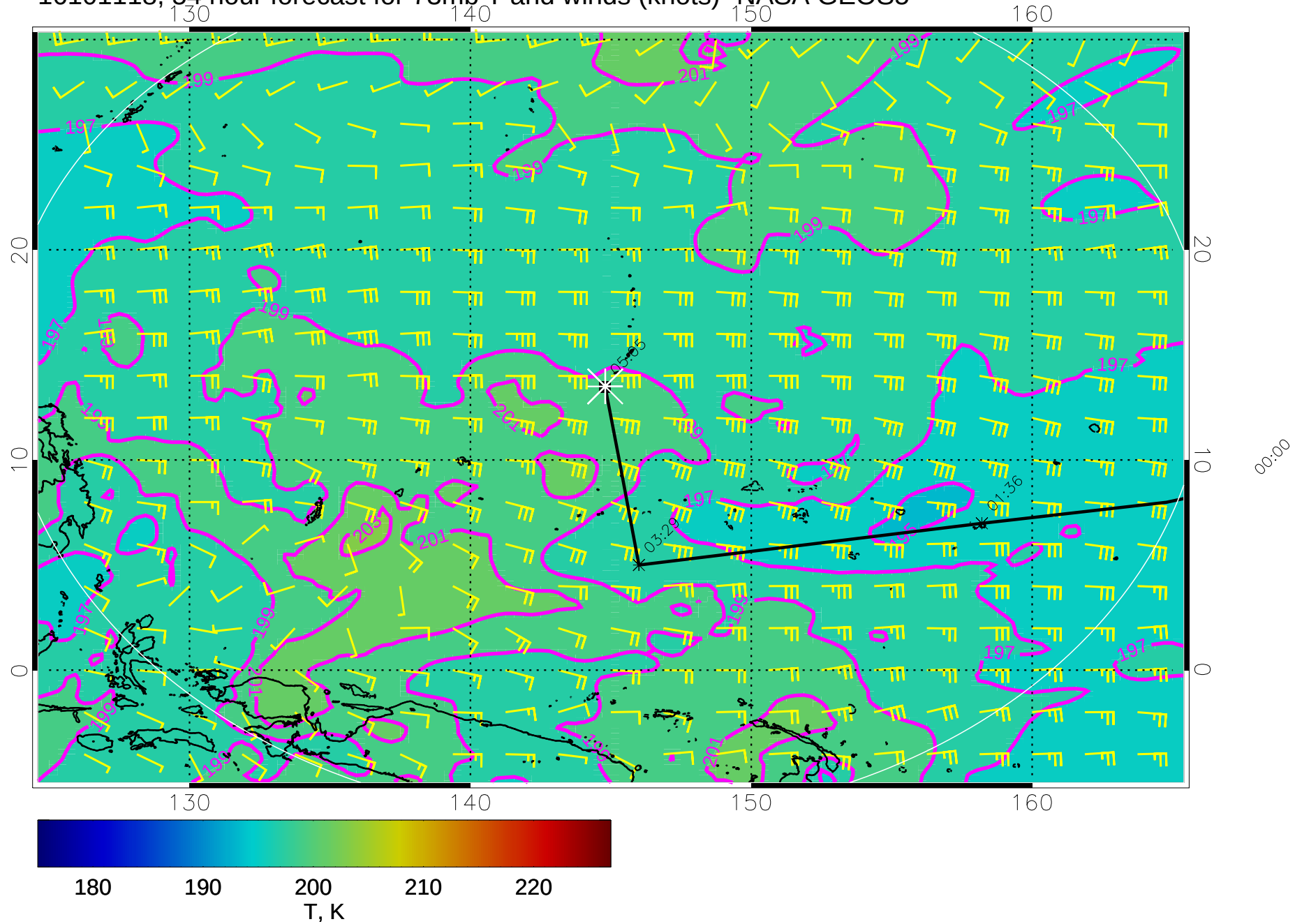
16101118, 54 hour forecast for 73mb T and winds (knots)- NASA GEOS5
