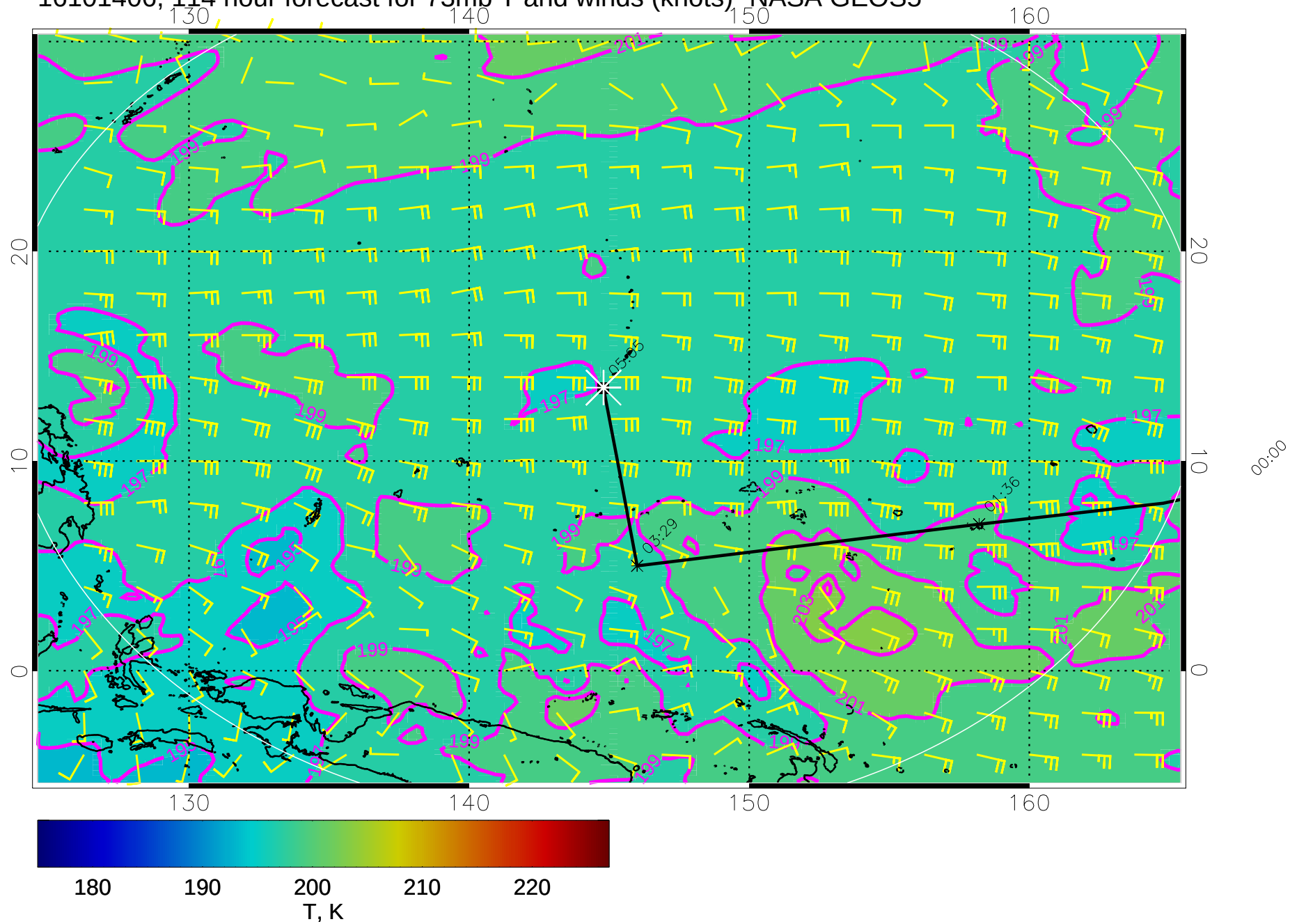
16101406, 114 hour forecast for 73mb T and winds (knots)- NASA GEOS5
