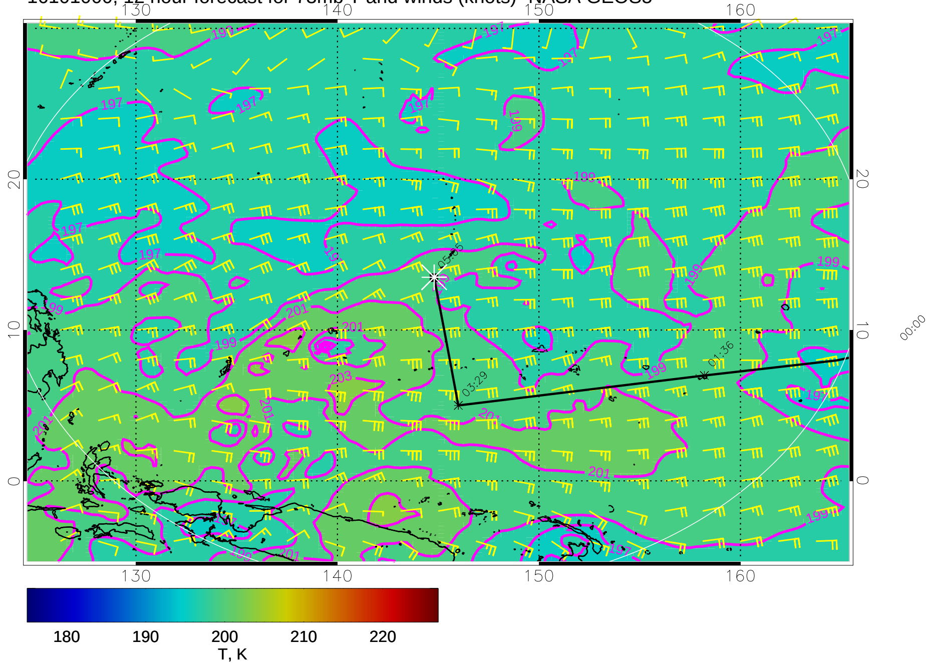
16101000, 12 hour forecast for 73mb T and winds (knots)- NASA GEOS5
