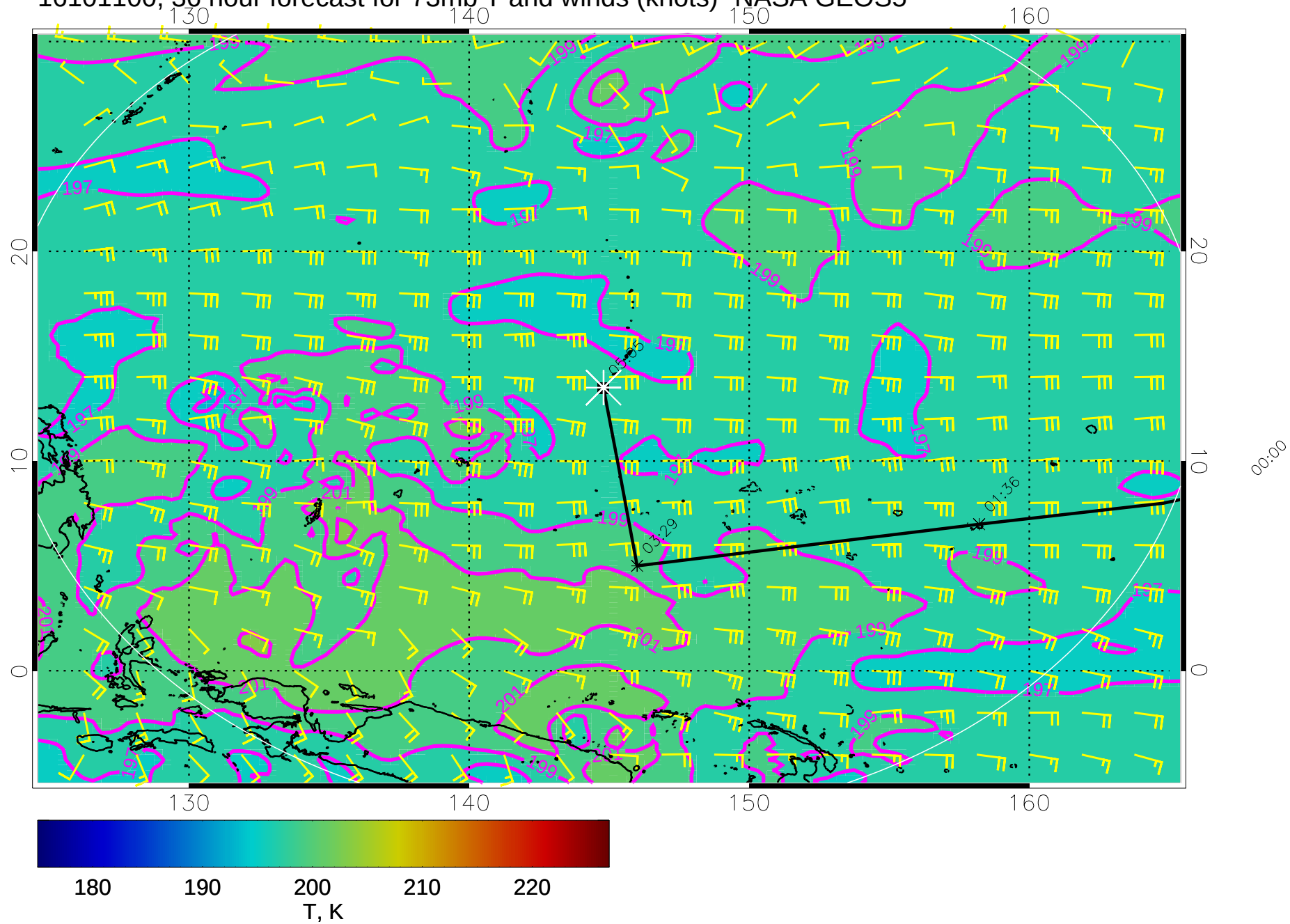
16101100, 36 hour forecast for 73mb T and winds (knots)- NASA GEOS5
