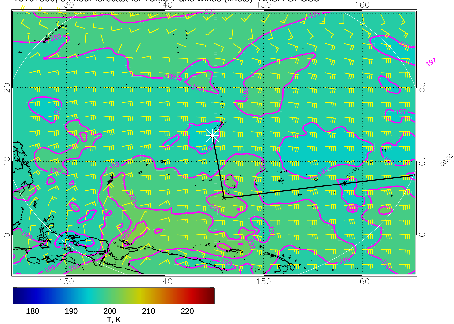
16101300, 84 hour forecast for 73mb T and winds (knots)- NASA GEOS5
