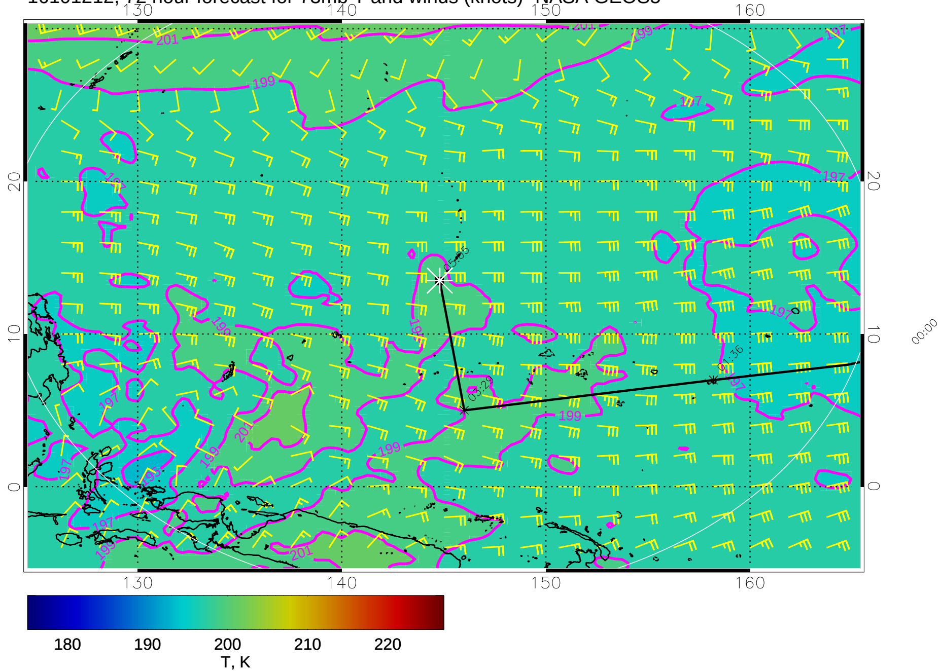
16101212, 72 hour forecast for 73mb T and winds (knots)- NASA GEOS5
