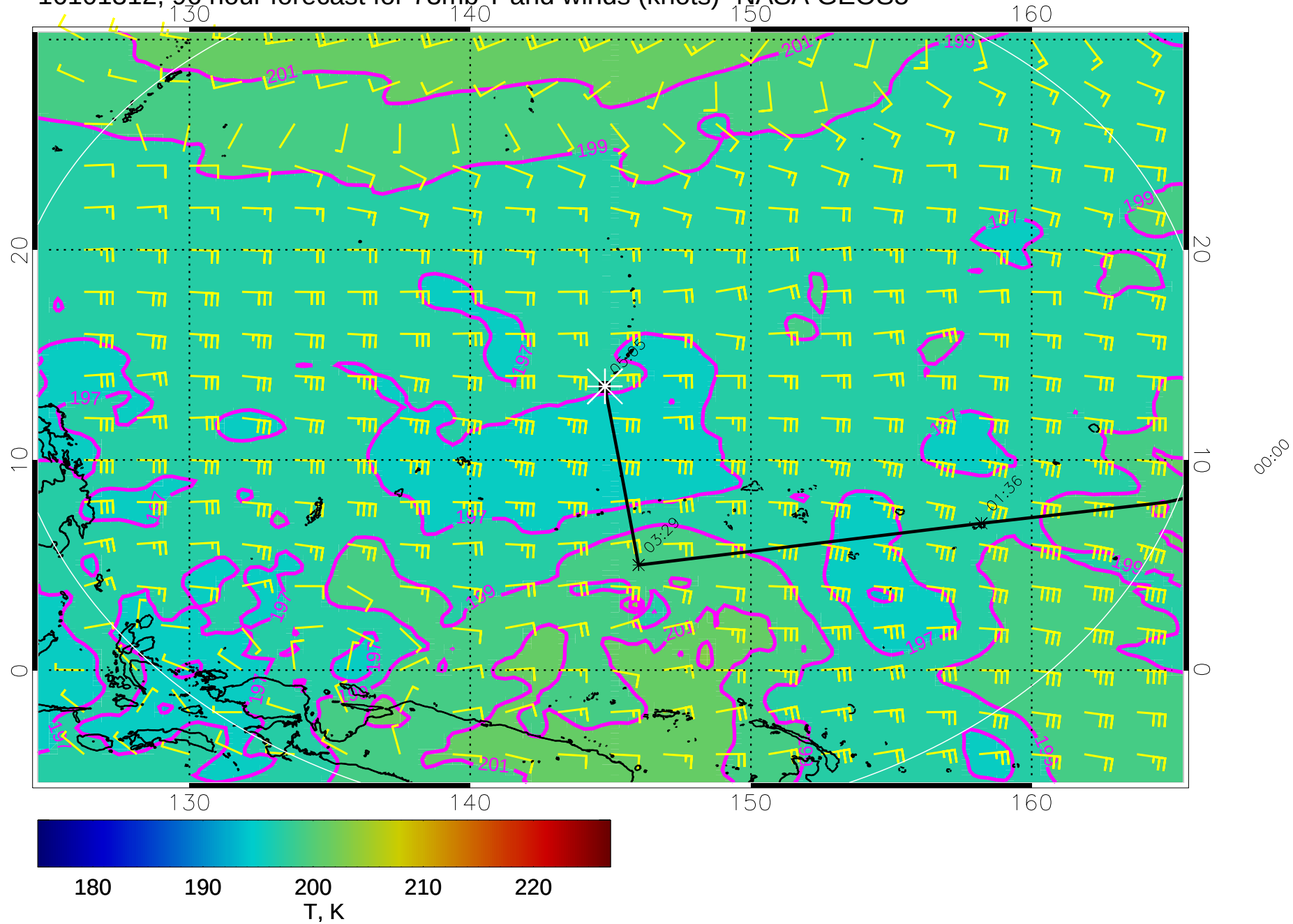
16101312, 96 hour forecast for 73mb T and winds (knots)- NASA GEOS5
