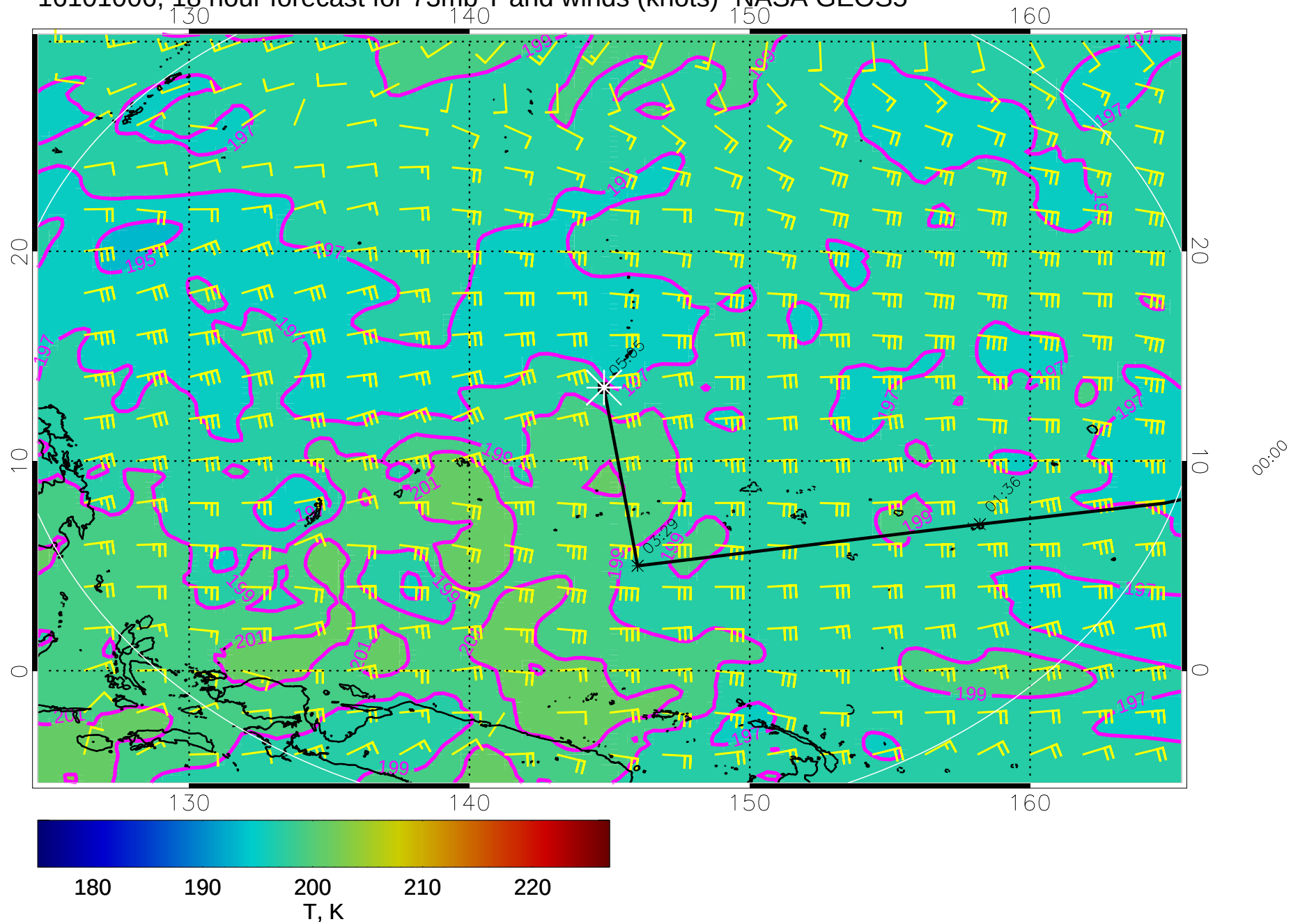
16101006, 18 hour forecast for 73mb T and winds (knots)- NASA GEOS5
