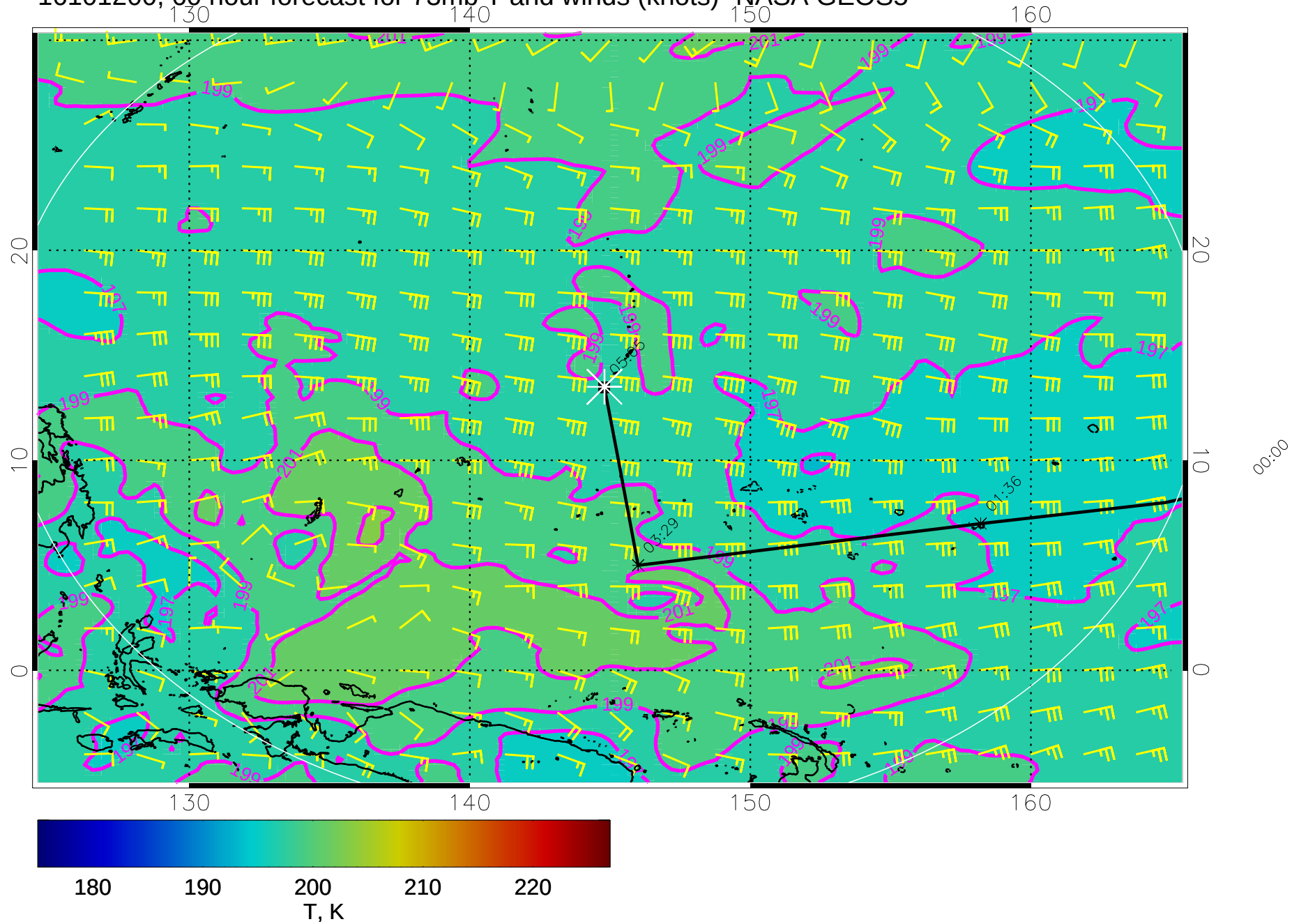
16101200, 60 hour forecast for 73mb T and winds (knots)- NASA GEOS5
