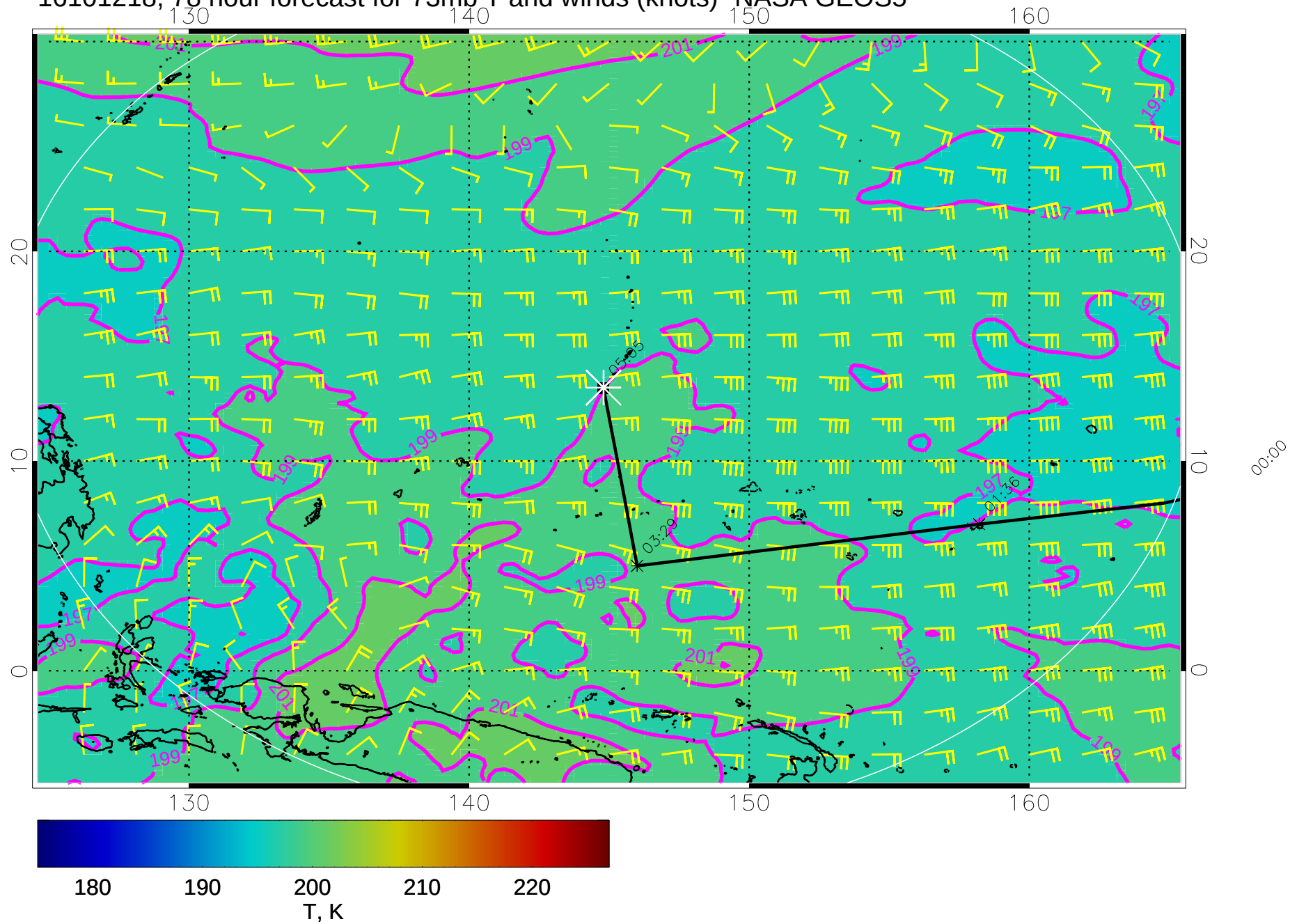
16101218, 78 hour forecast for 73mb T and winds (knots)- NASA GEOS5
