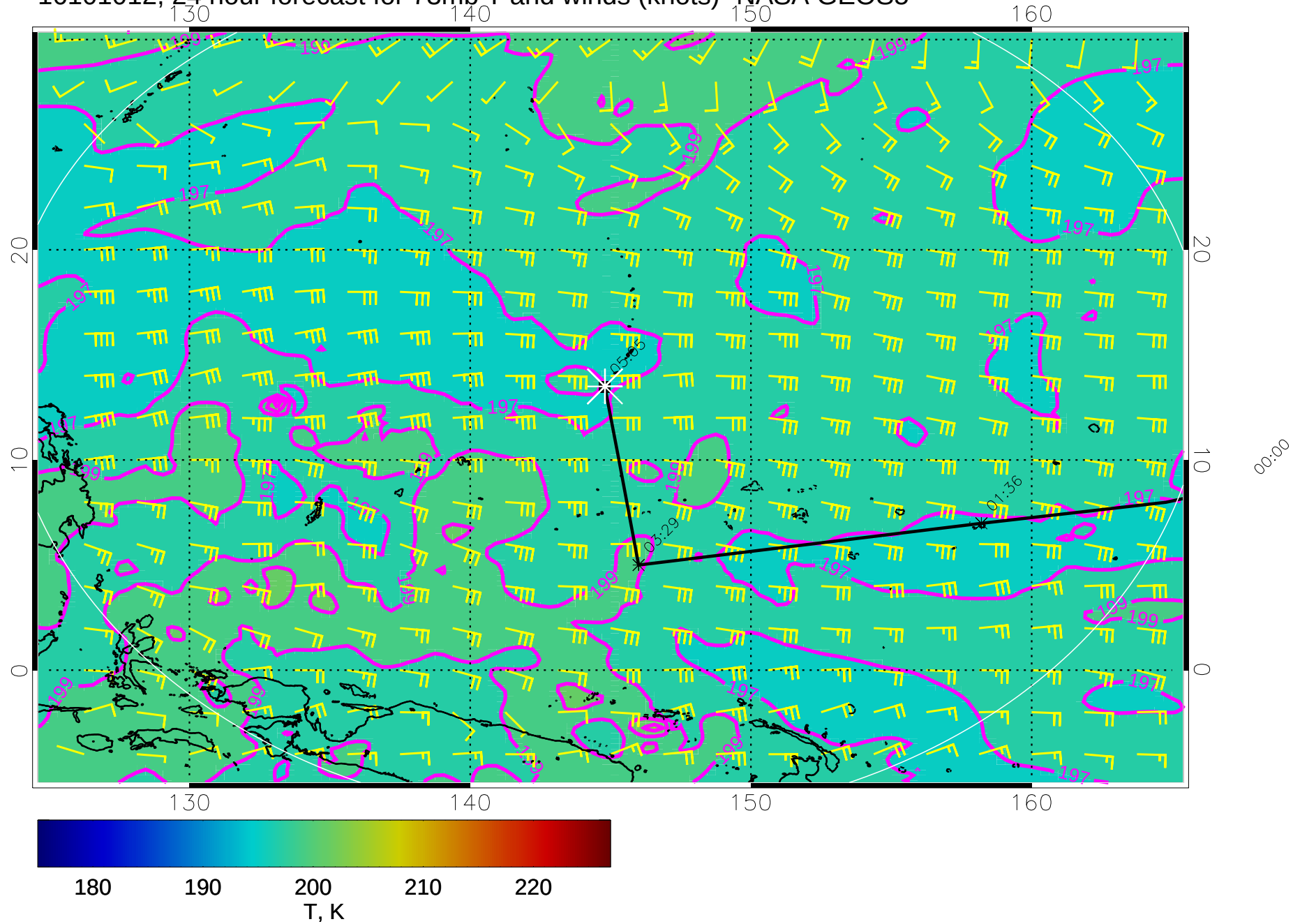
16101012, 24 hour forecast for 73mb T and winds (knots)- NASA GEOS5
