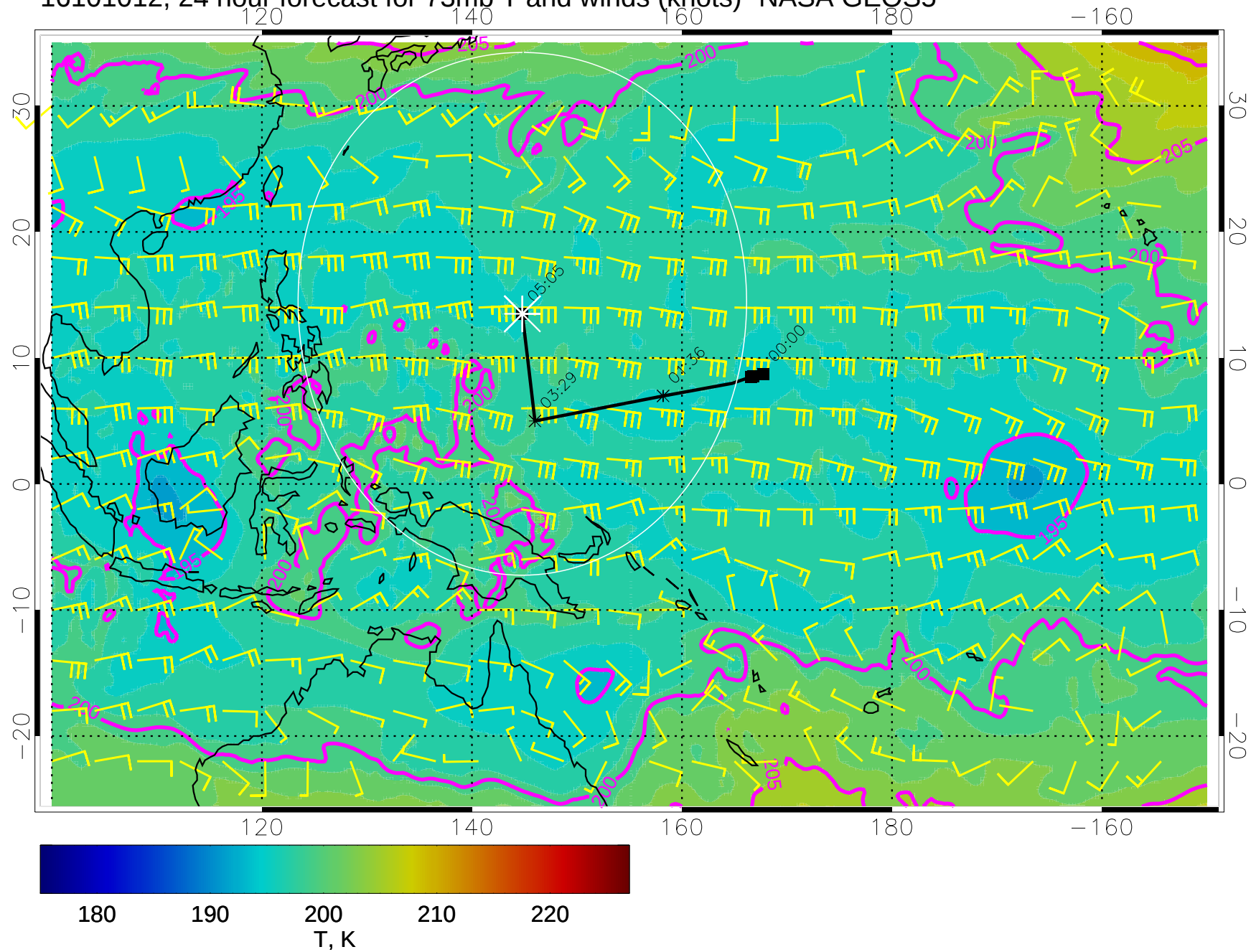
16101012, 24 hour forecast for 73mb T and winds (knots)- NASA GEOS5
