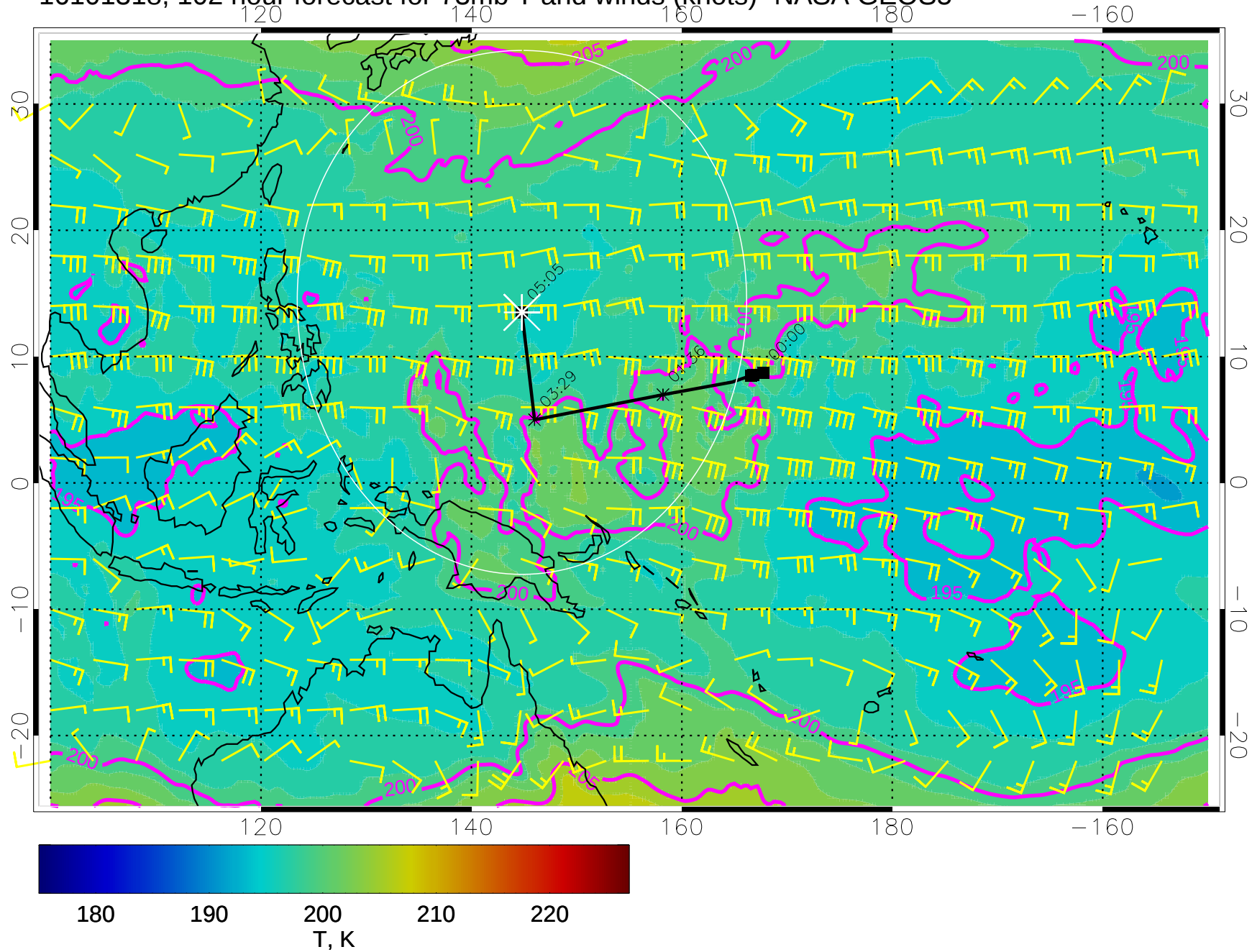
16101318, 102 hour forecast for 73mb T and winds (knots)- NASA GEOS5
