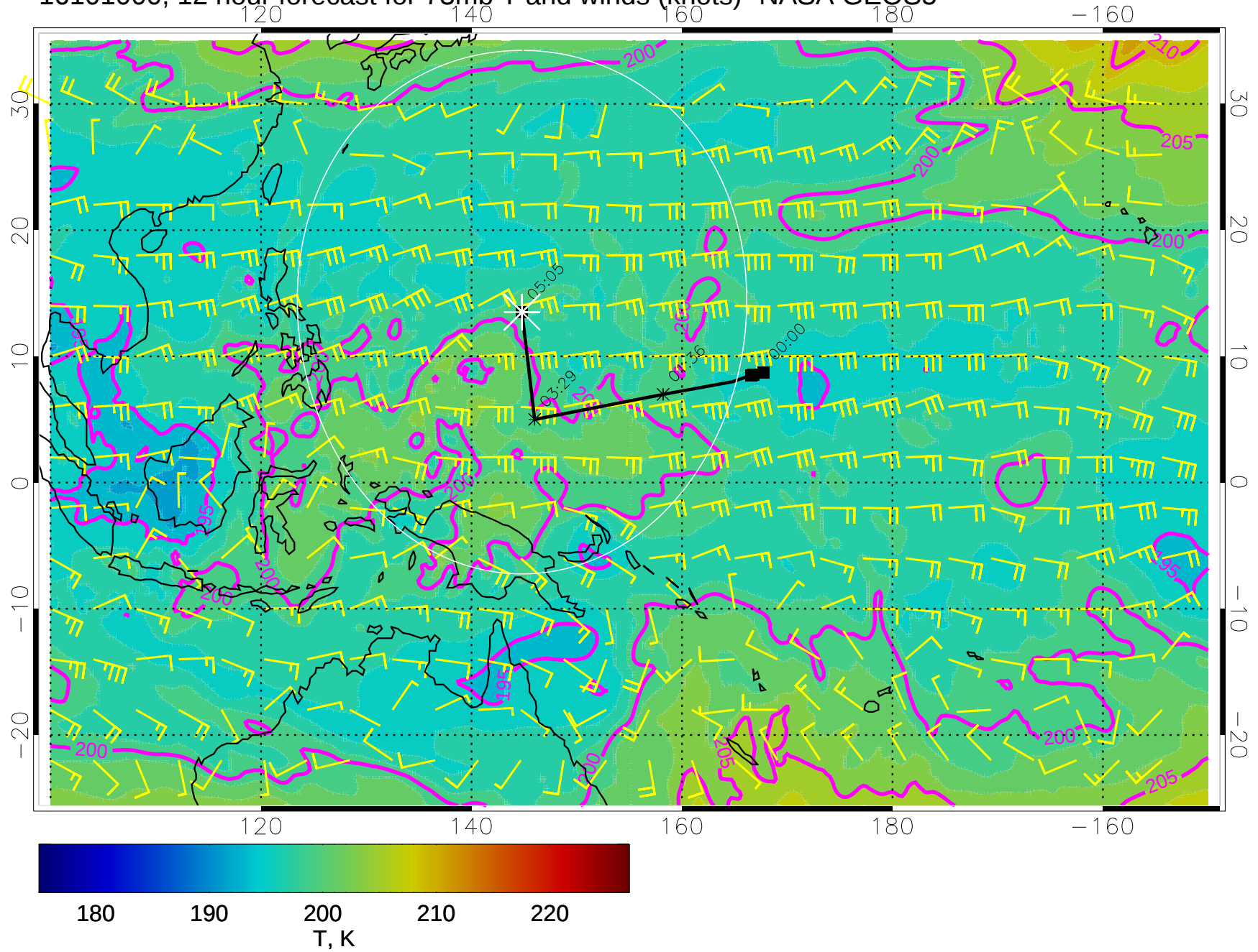
16101000, 12 hour forecast for 73mb T and winds (knots)- NASA GEOS5
