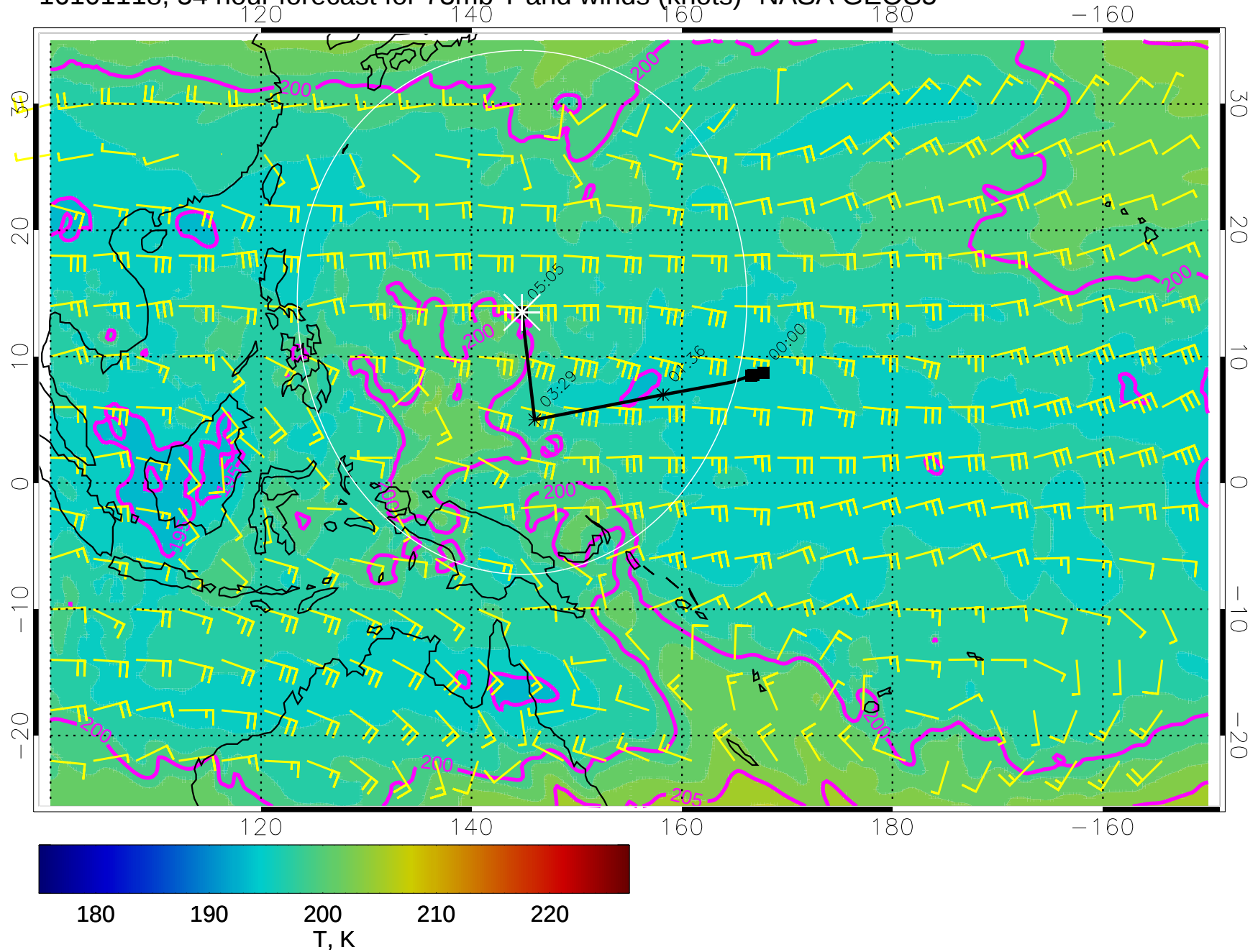
16101118, 54 hour forecast for 73mb T and winds (knots)- NASA GEOS5
