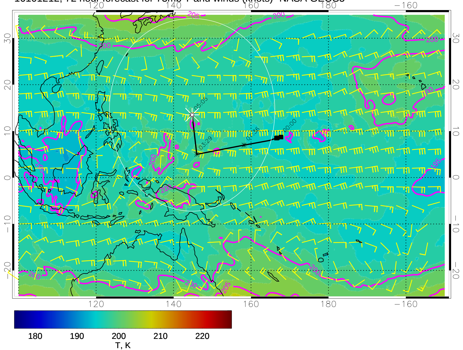
16101212, 72 hour forecast for 73mb T and winds (knots)- NASA GEOS5
