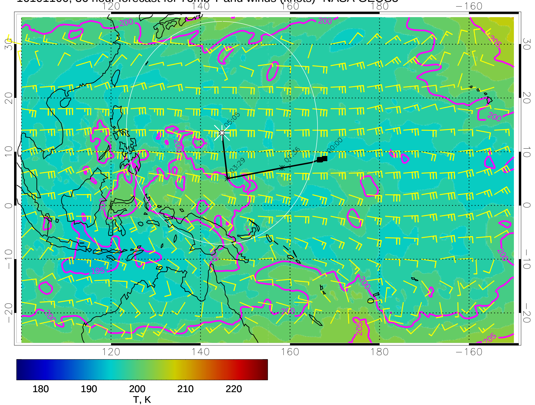
16101100, 36 hour forecast for 73mb T and winds (knots)- NASA GEOS5
