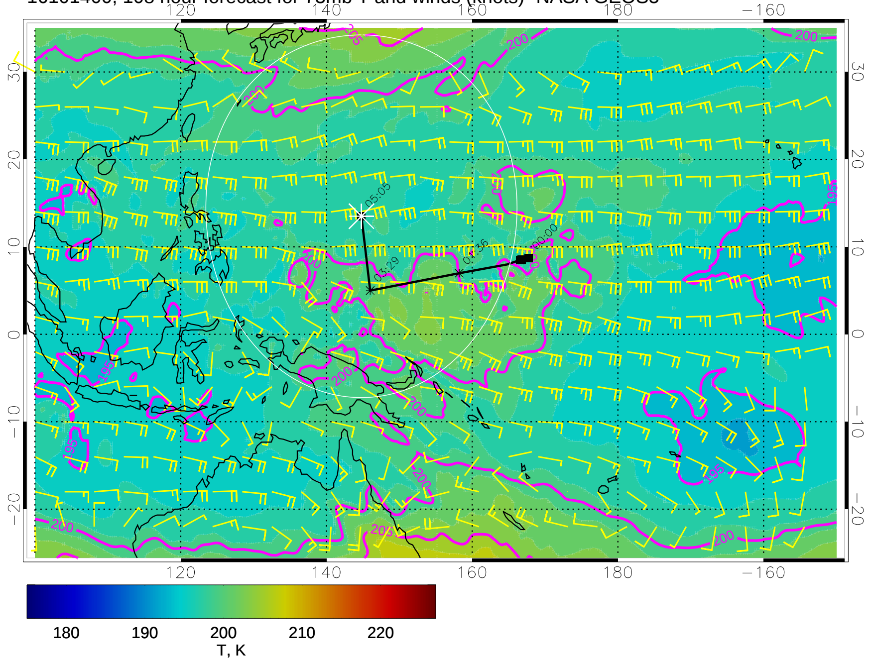
16101400, 108 hour forecast for 73mb T and winds (knots)- NASA GEOS5
