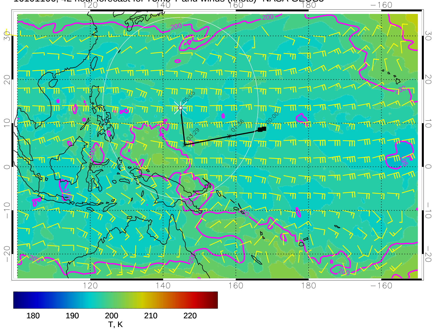
16101106, 42 hour forecast for 73mb T and winds (knots)- NASA GEOS5
