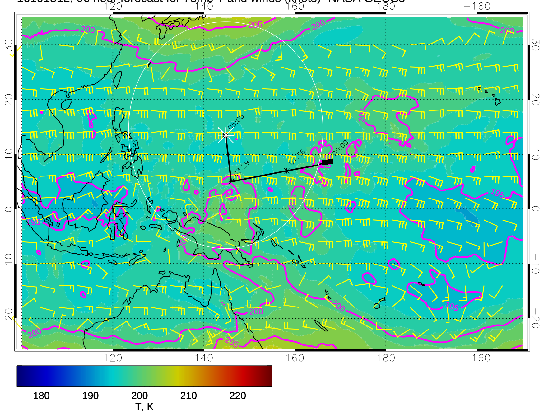
16101312, 96 hour forecast for 73mb T and winds (knots)- NASA GEOS5
