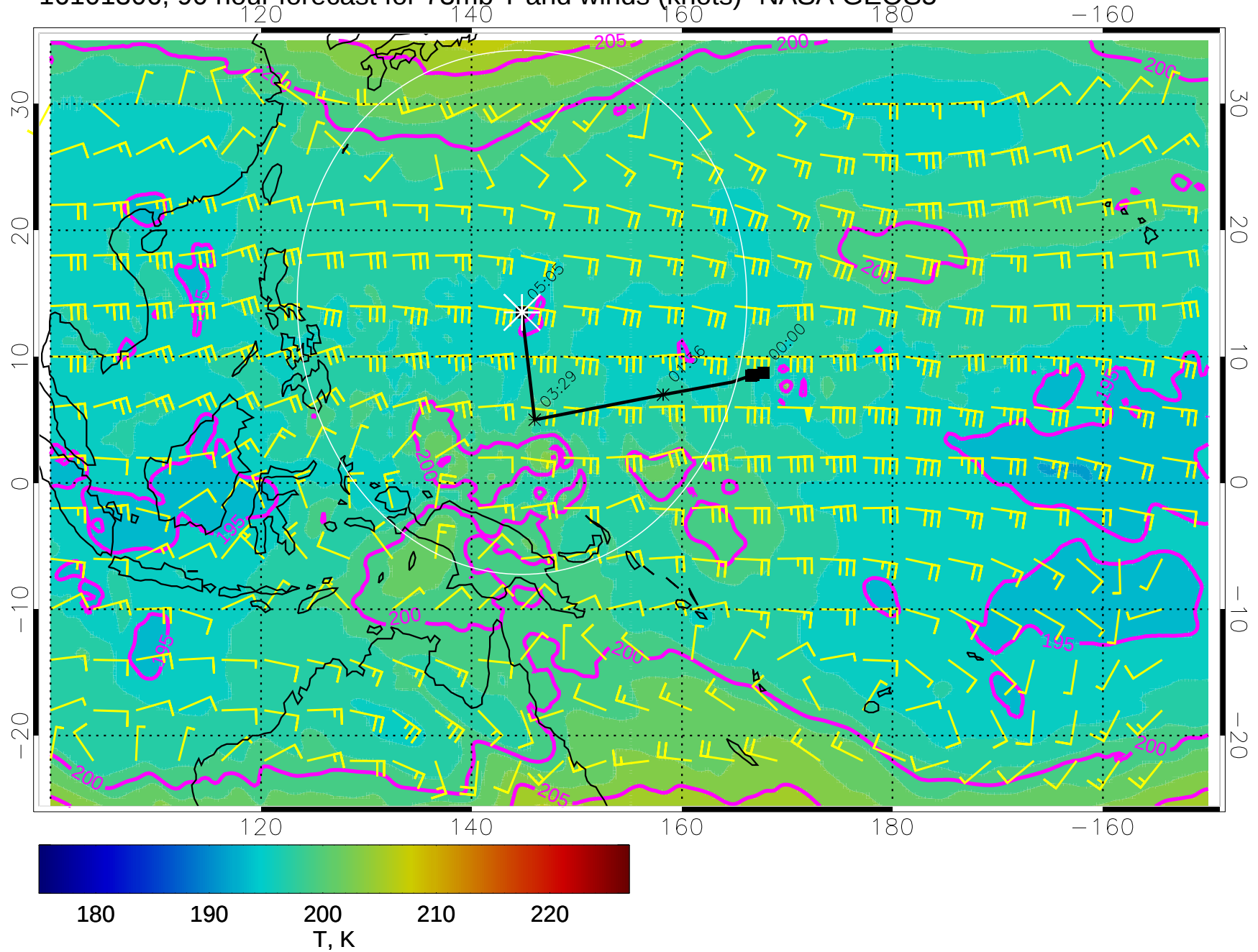
16101306, 90 hour forecast for 73mb T and winds (knots)- NASA GEOS5
