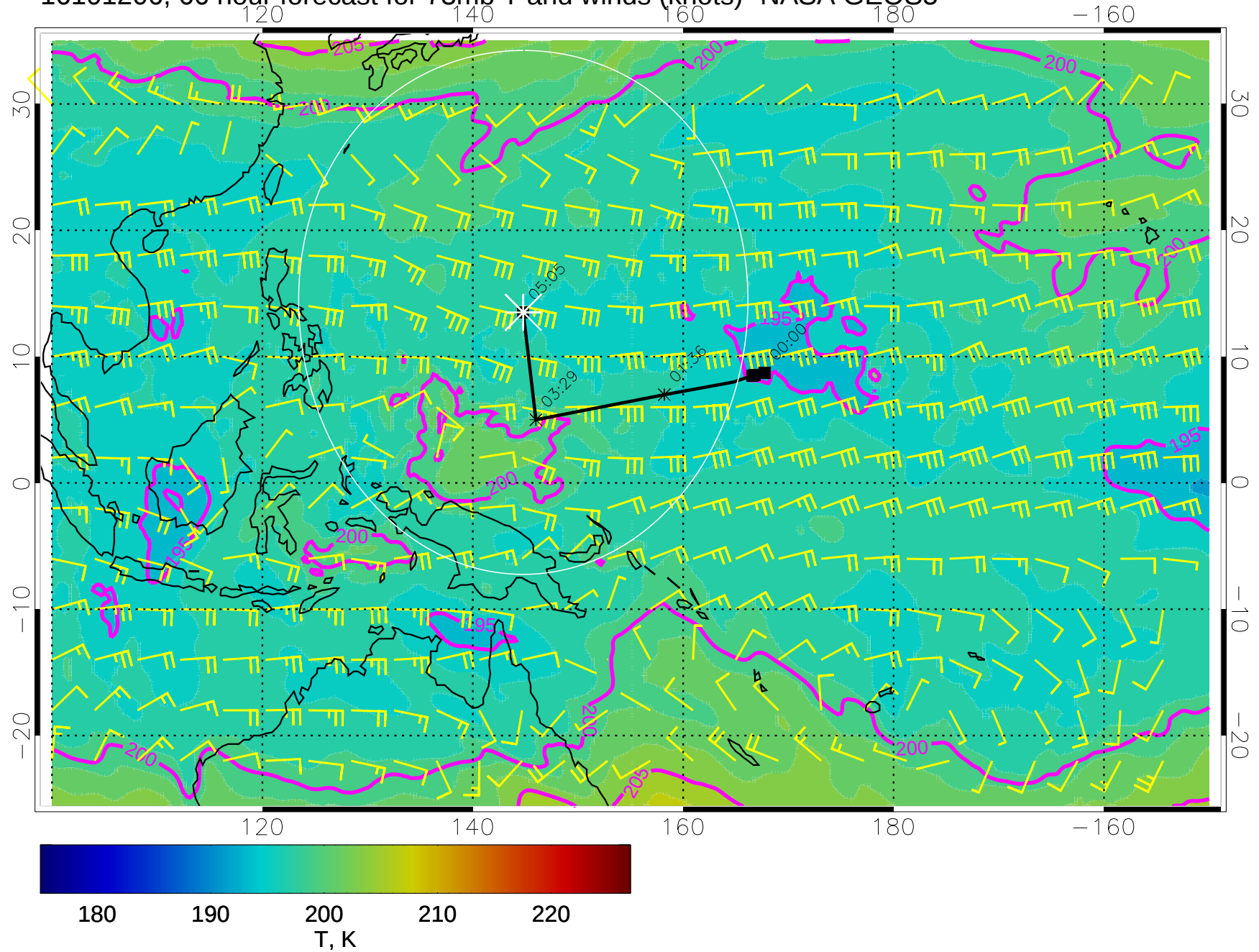
16101206, 66 hour forecast for 73mb T and winds (knots)- NASA GEOS5
