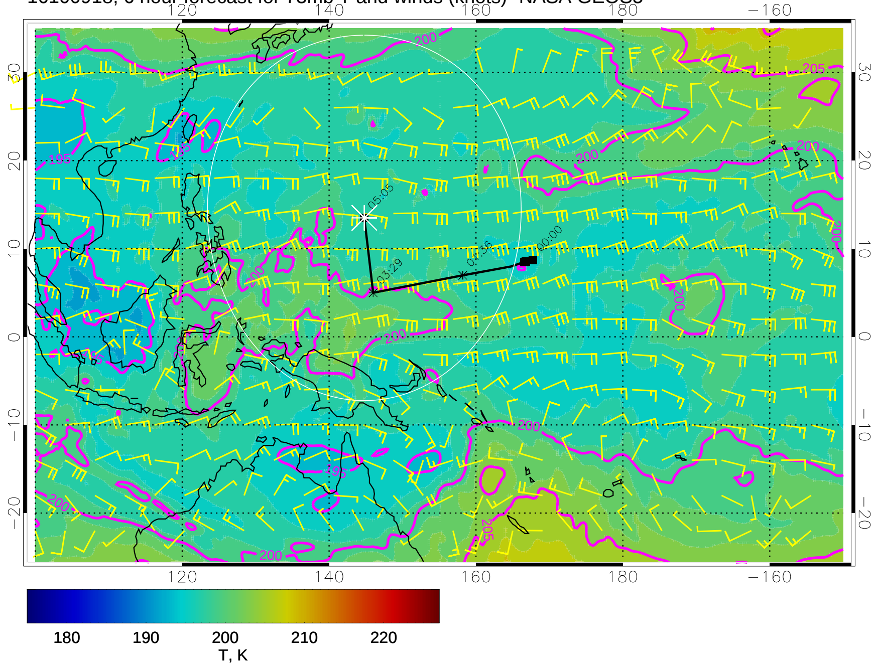
16100918, 6 hour forecast for 73mb T and winds (knots)- NASA GEOS5
