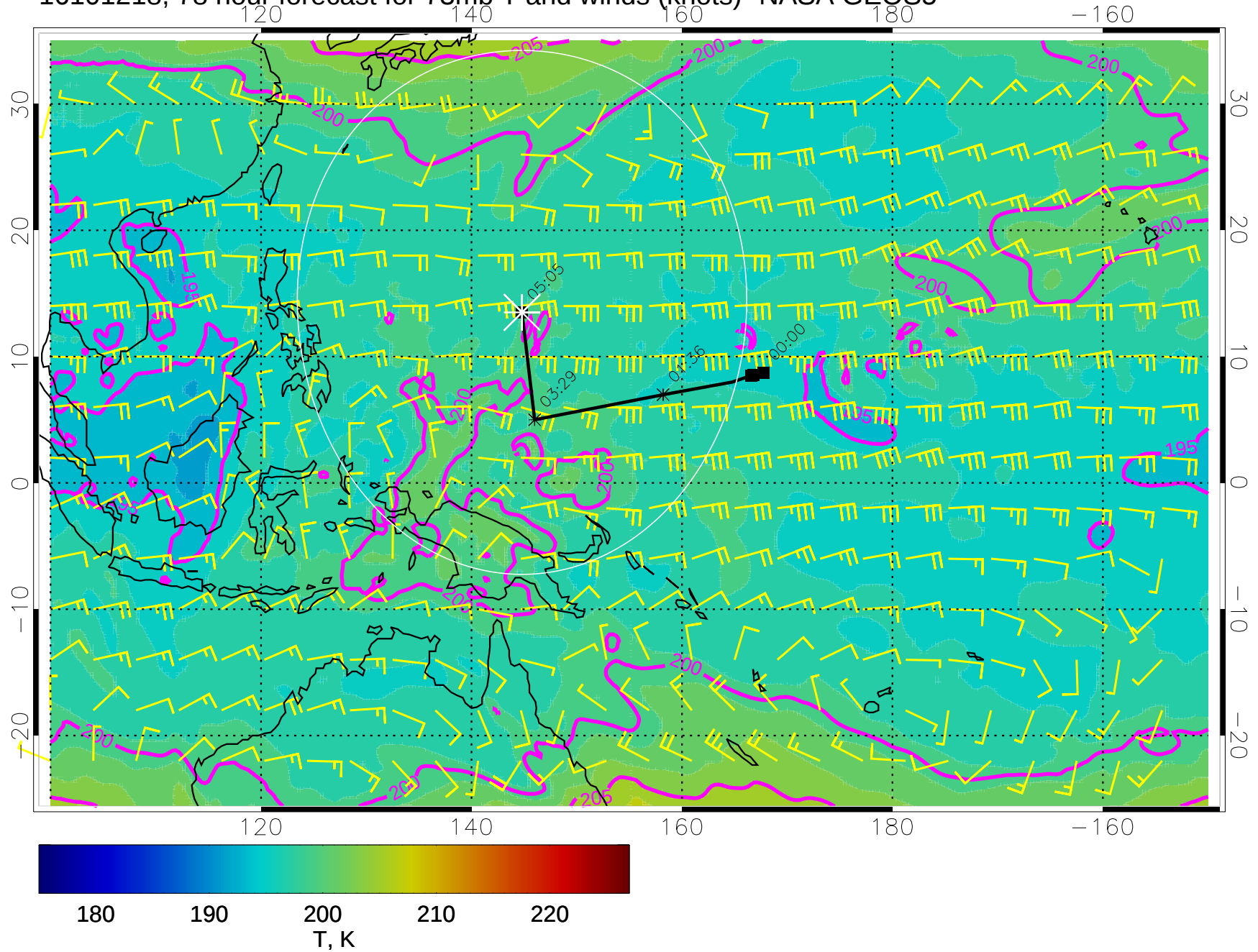
16101218, 78 hour forecast for 73mb T and winds (knots)- NASA GEOS5
