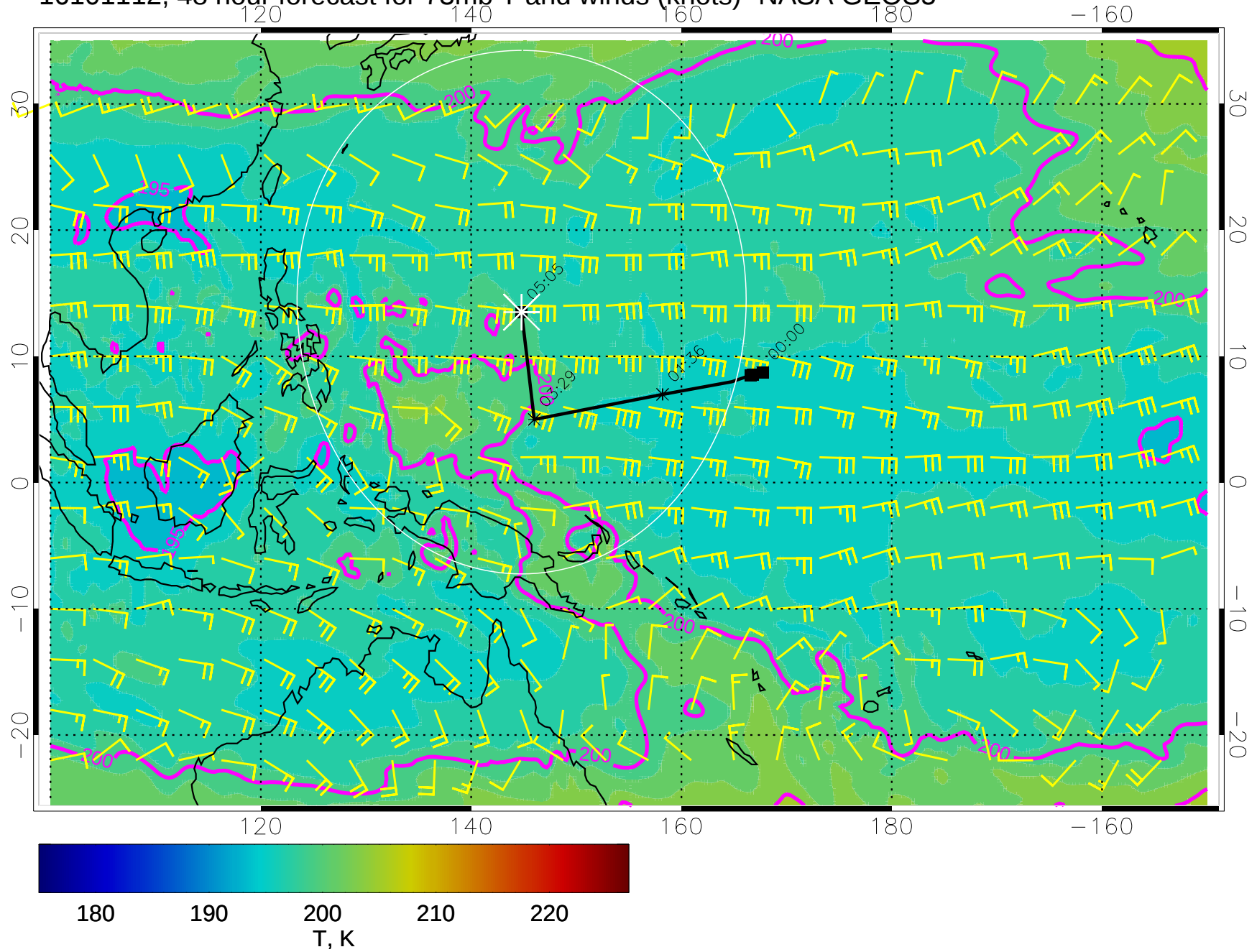
16101112, 48 hour forecast for 73mb T and winds (knots)- NASA GEOS5
