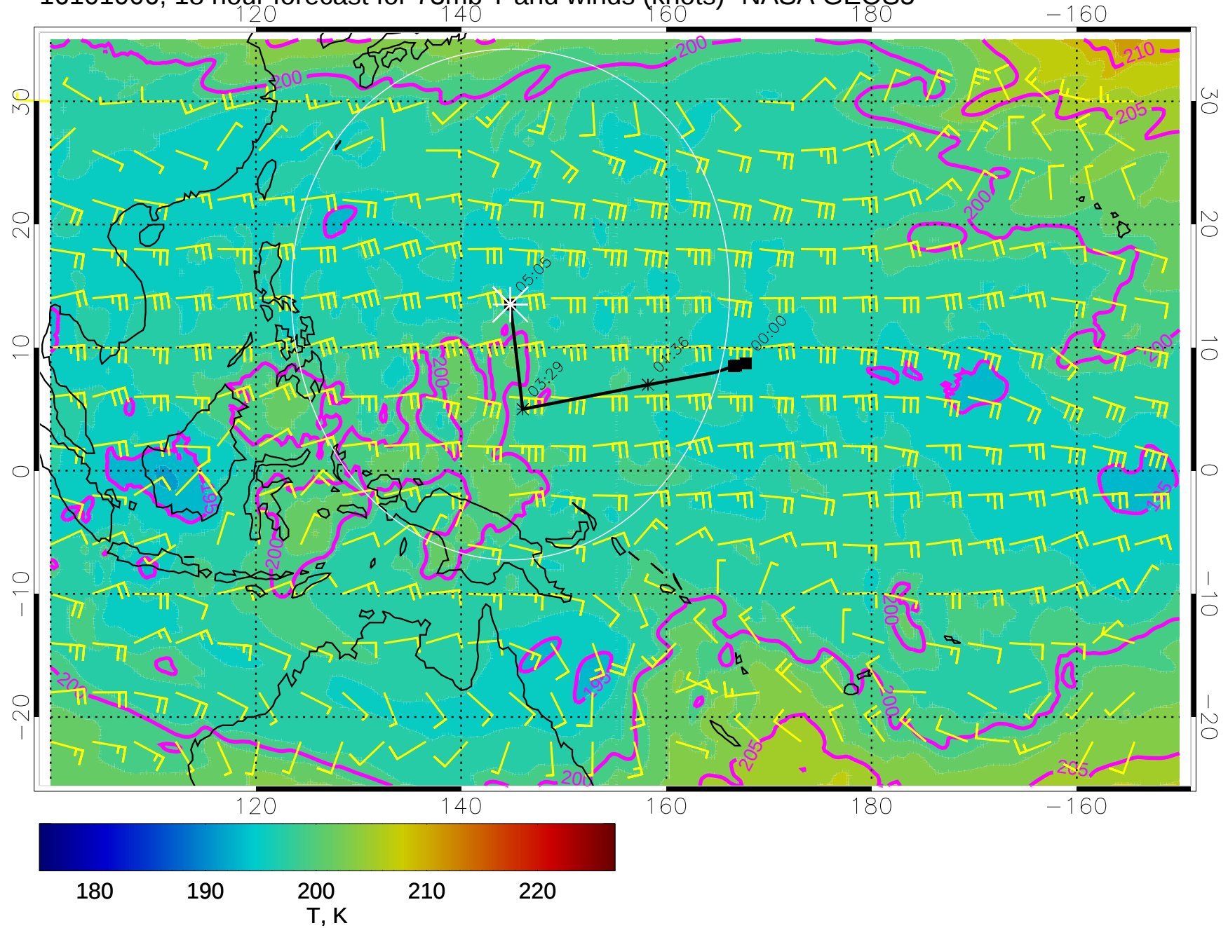
16101006, 18 hour forecast for 73mb T and winds (knots)- NASA GEOS5
