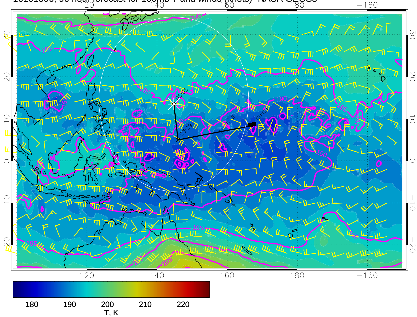
16101306, 90 hour forecast for 100mb T and winds (knots)- NASA GEOS5
