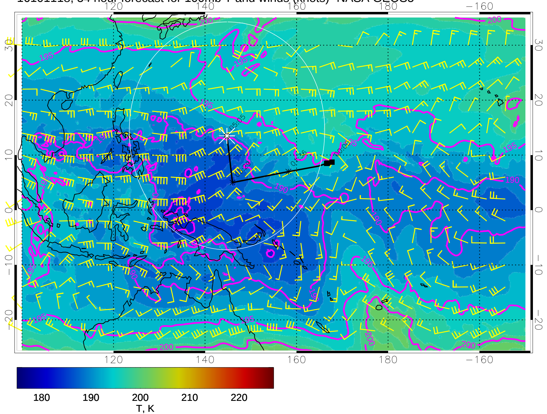
16101118, 54 hour forecast for 100mb T and winds (knots)- NASA GEOS5
