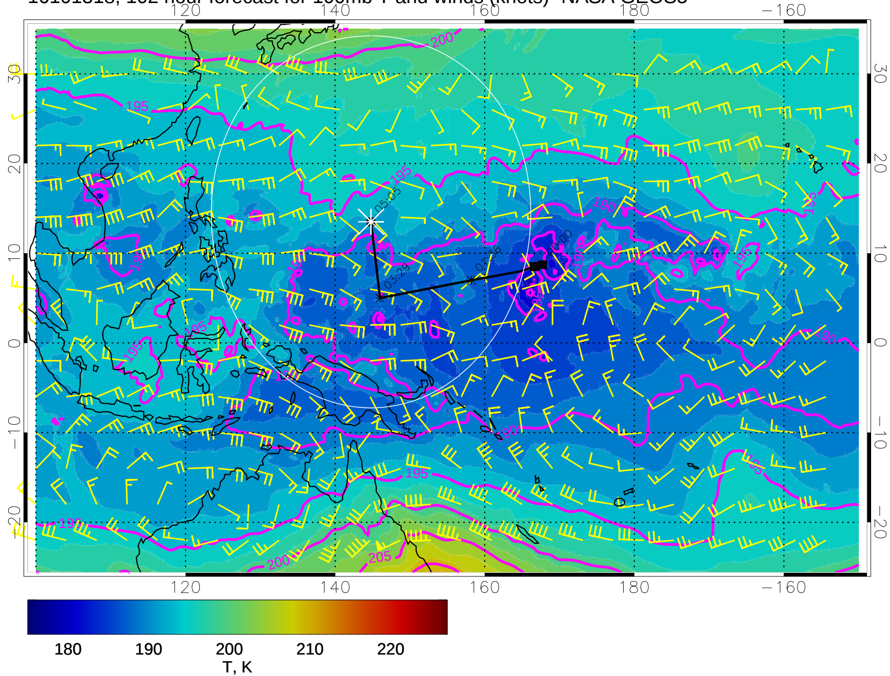
16101318, 102 hour forecast for 100mb T and winds (knots)- NASA GEOS5
