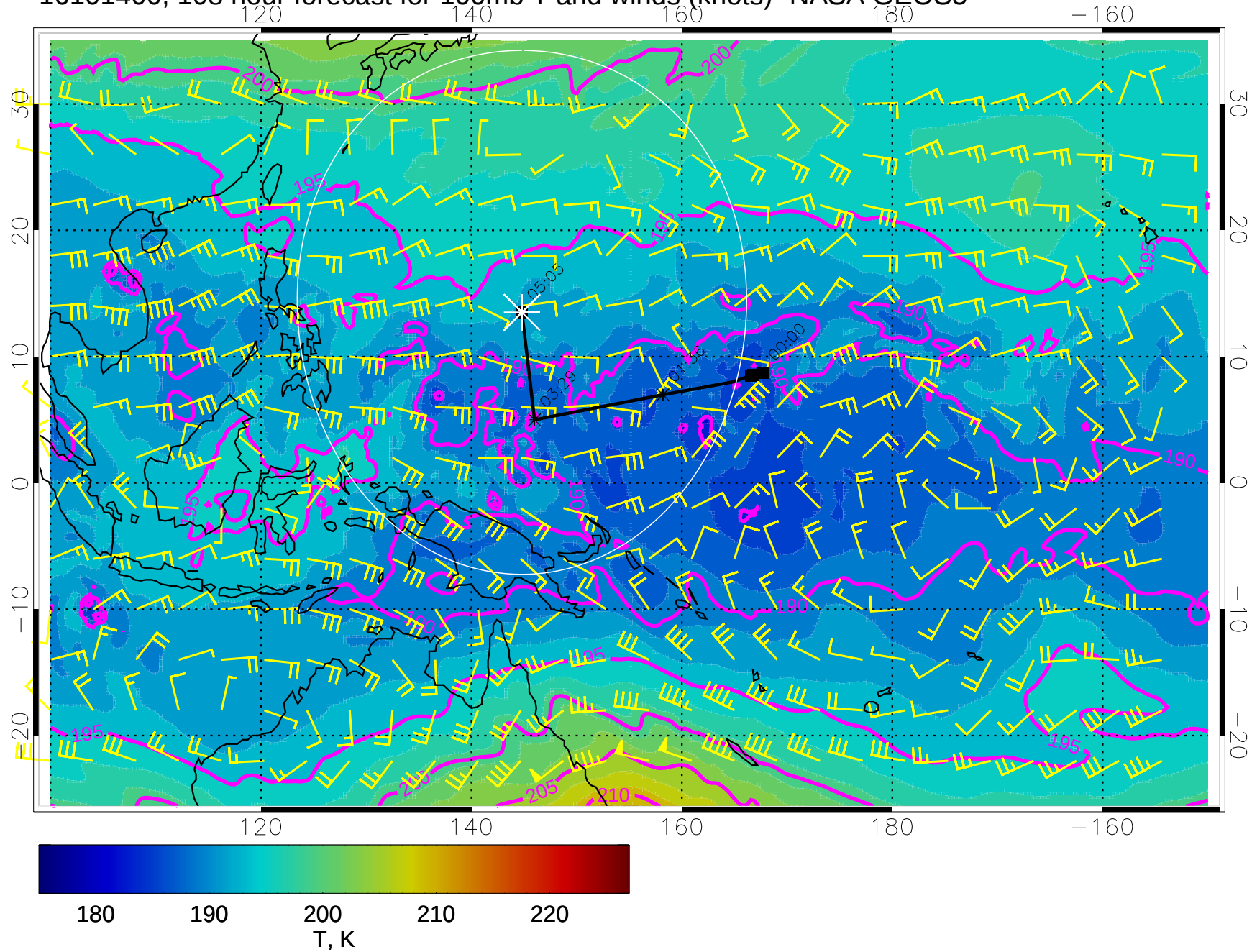
16101400, 108 hour forecast for 100mb T and winds (knots)- NASA GEOS5
