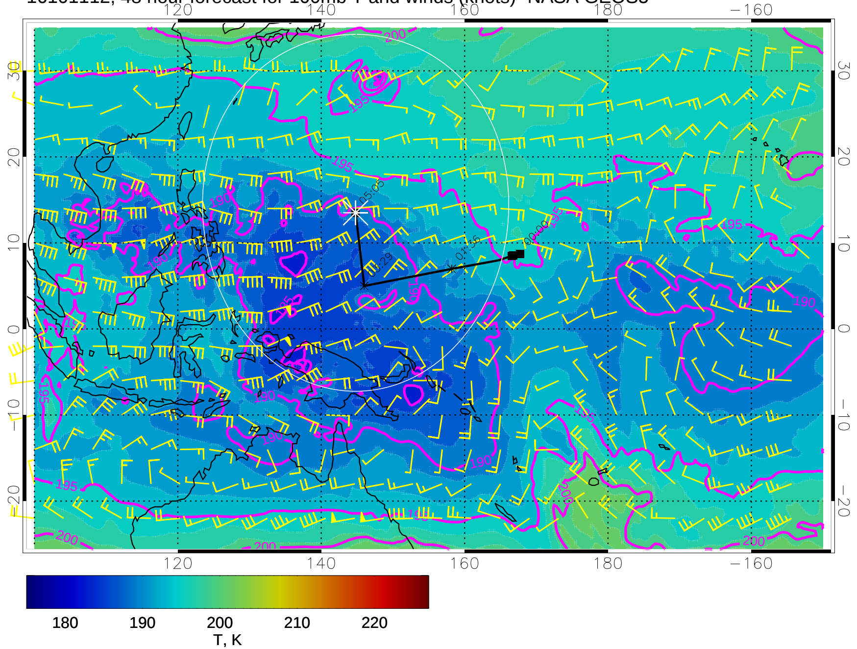
16101112, 48 hour forecast for 100mb T and winds (knots)- NASA GEOS5
