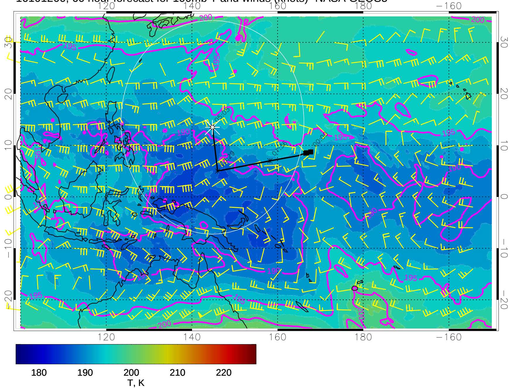
16101200, 60 hour forecast for 100mb T and winds (knots)- NASA GEOS5
