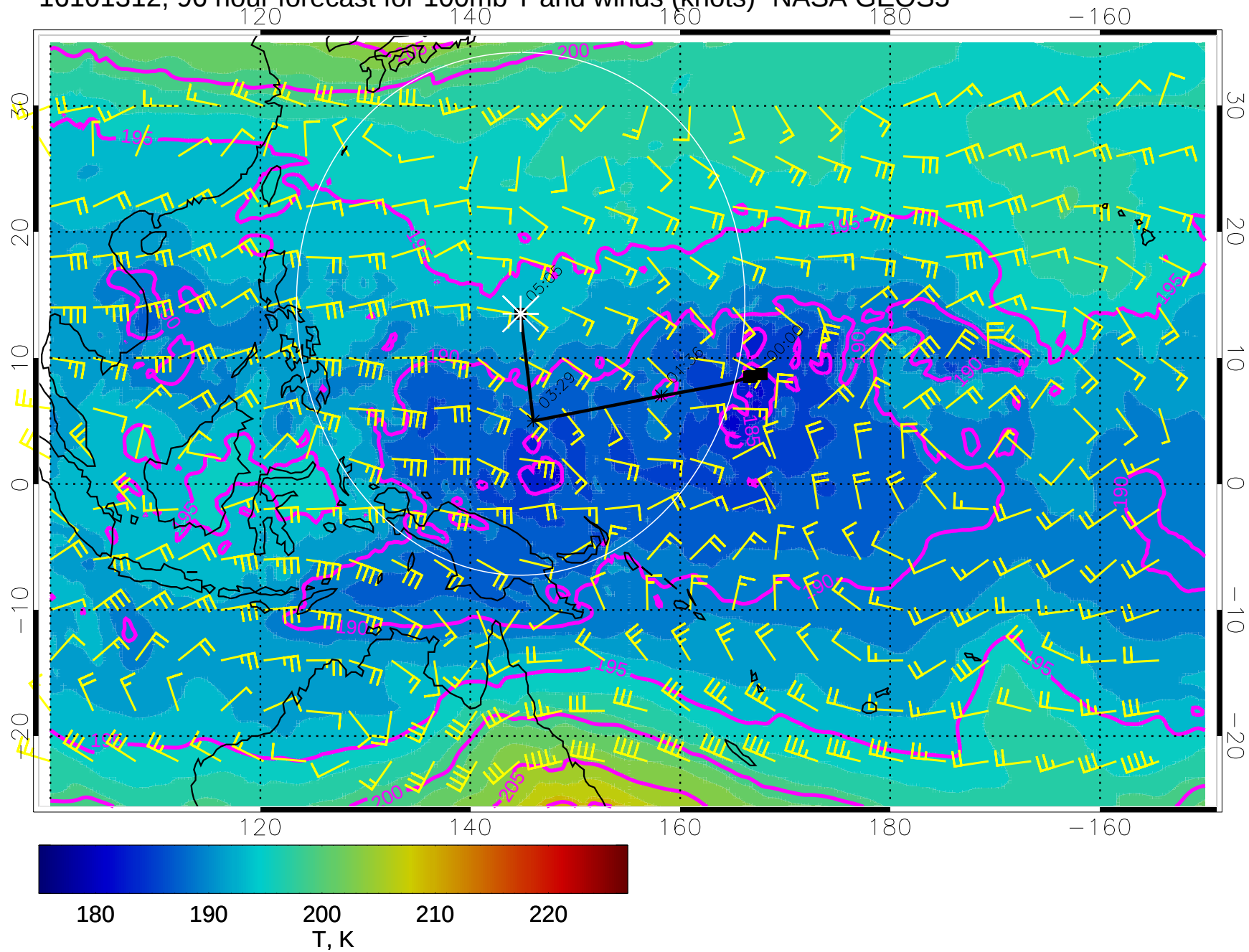
16101312, 96 hour forecast for 100mb T and winds (knots)- NASA GEOS5
