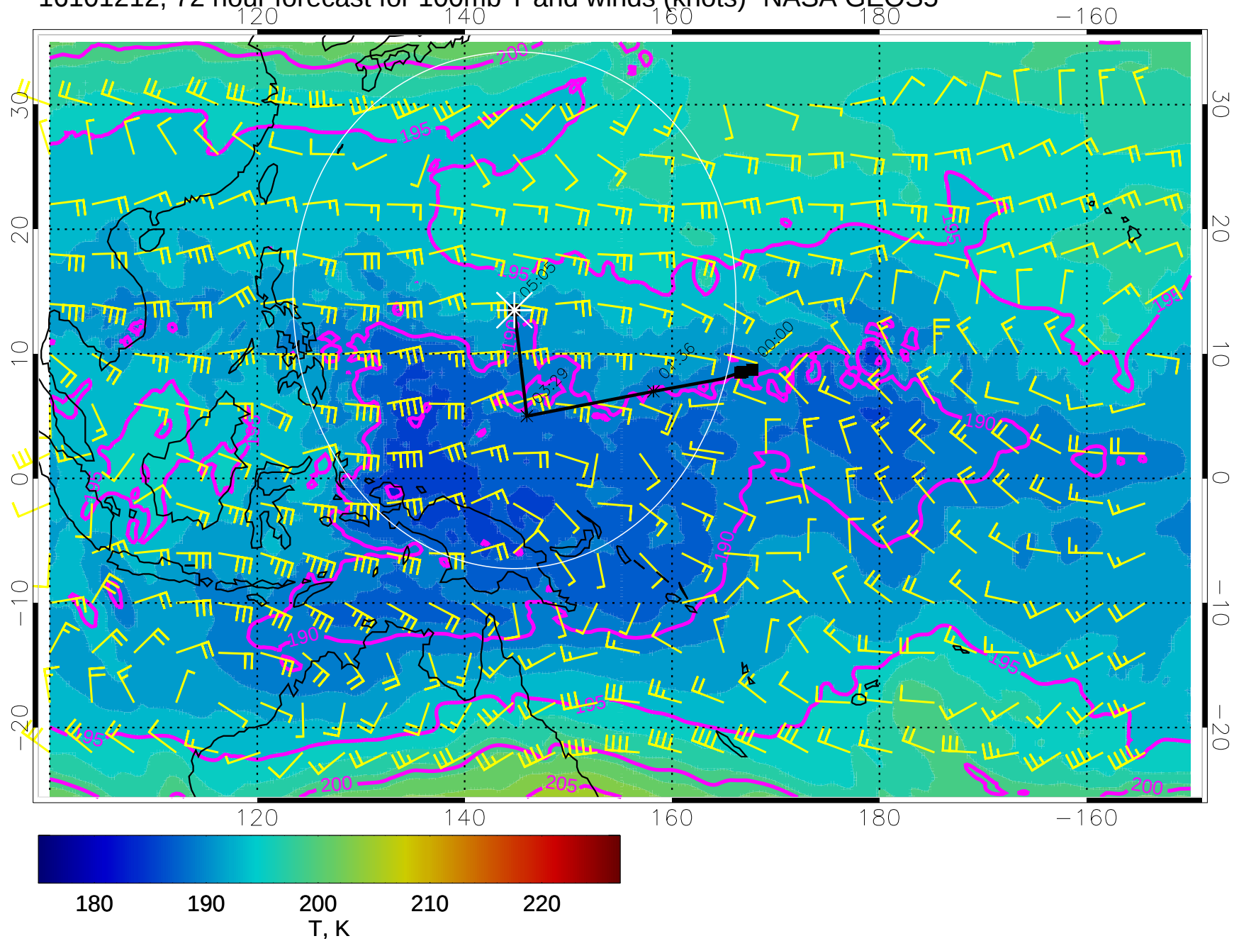
16101212, 72 hour forecast for 100mb T and winds (knots)- NASA GEOS5
