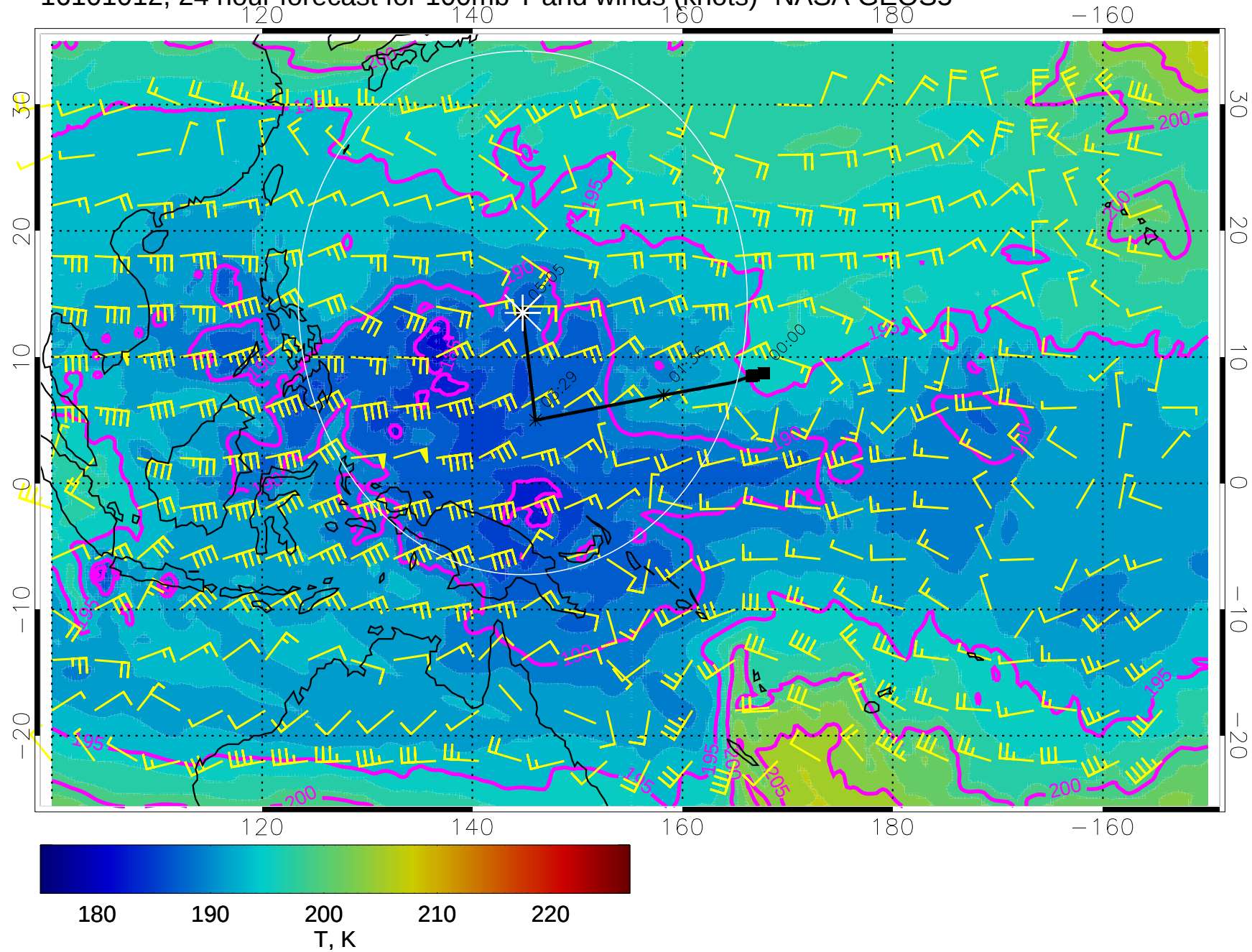
16101012, 24 hour forecast for 100mb T and winds (knots)- NASA GEOS5
