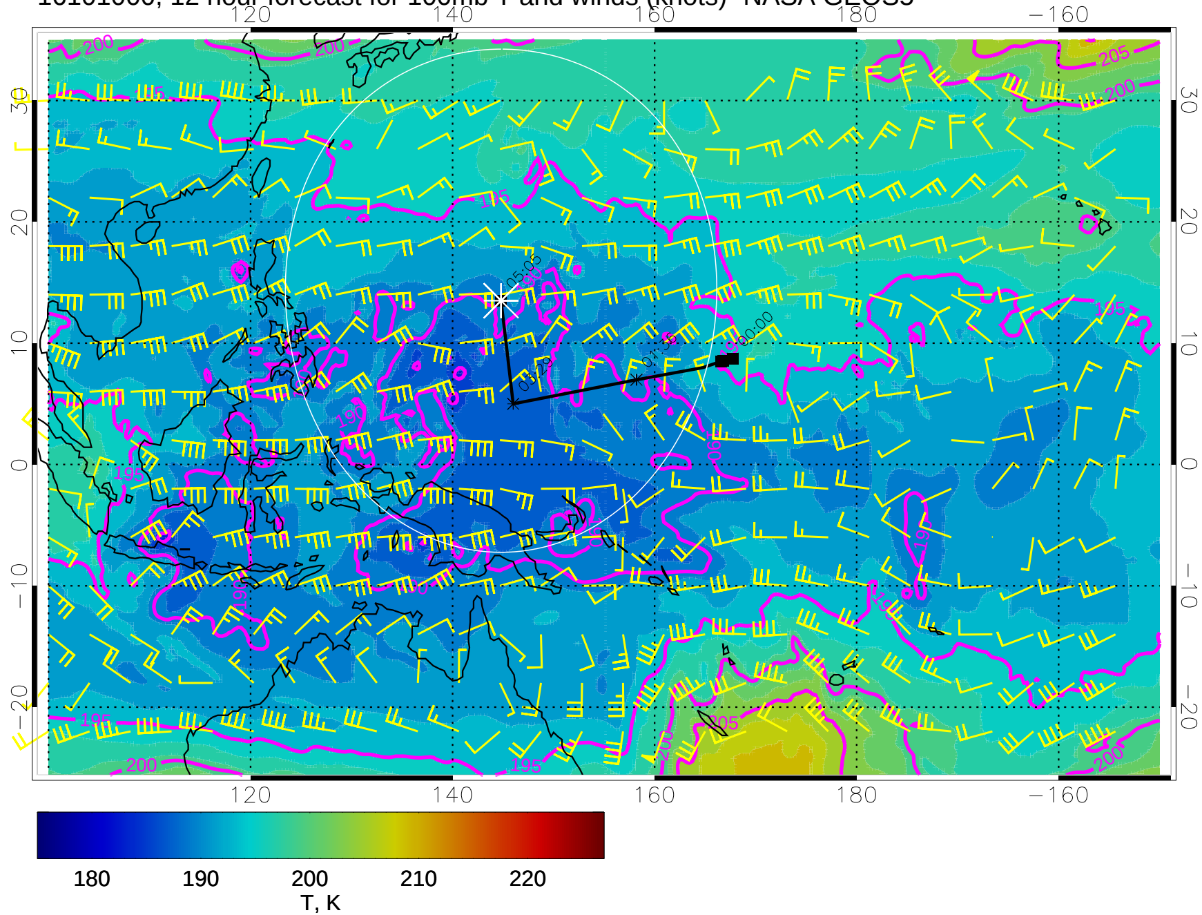
16101000, 12 hour forecast for 100mb T and winds (knots)- NASA GEOS5
