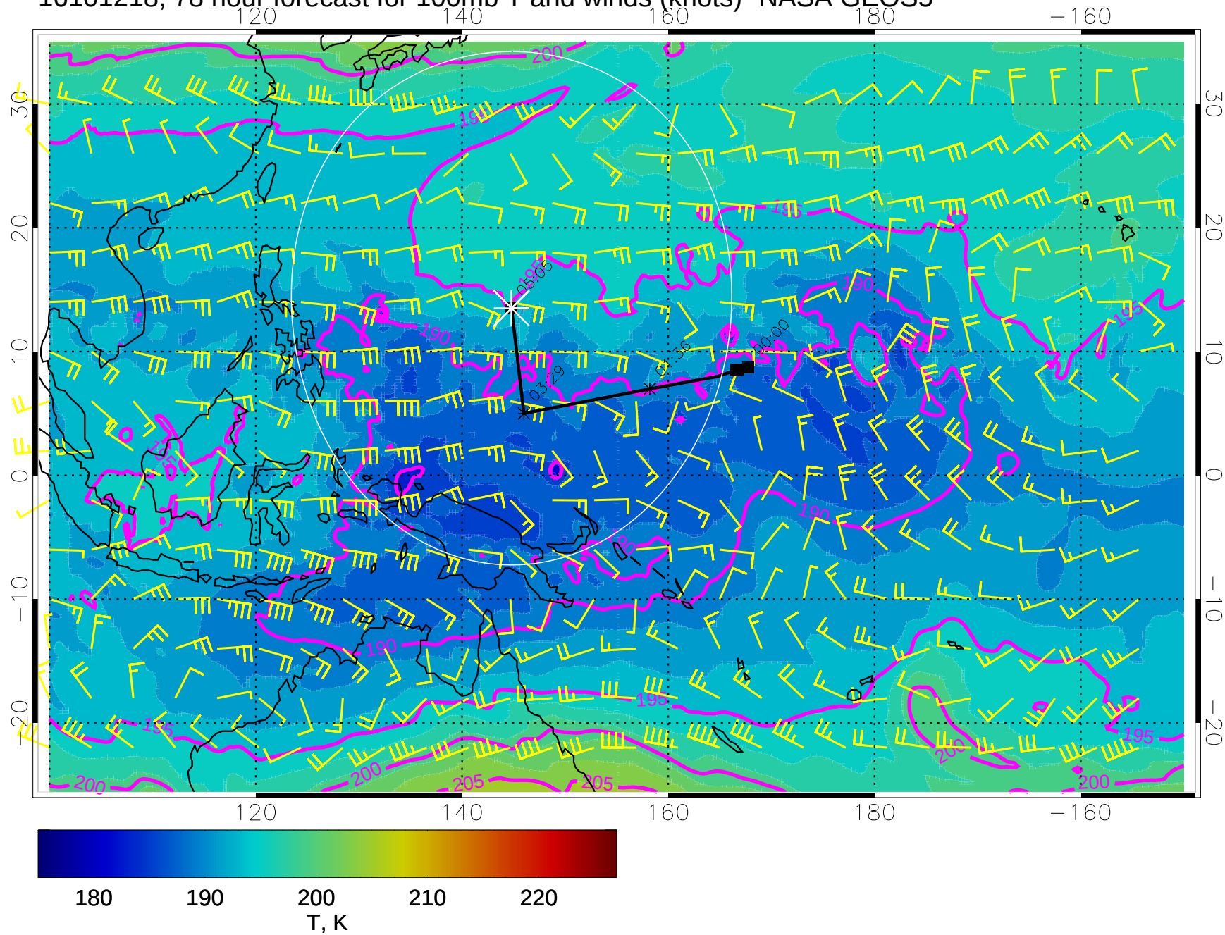
16101218, 78 hour forecast for 100mb T and winds (knots)- NASA GEOS5
