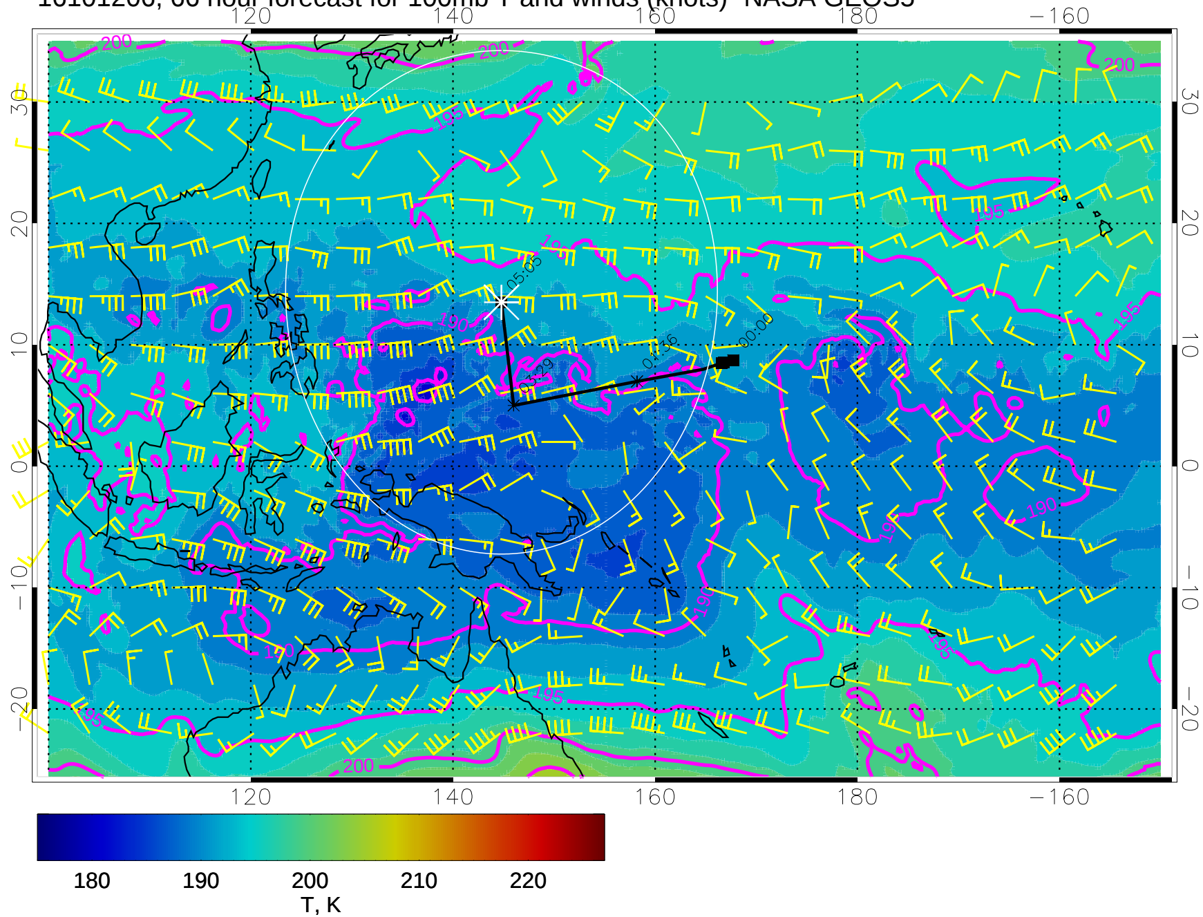
16101206, 66 hour forecast for 100mb T and winds (knots)- NASA GEOS5
