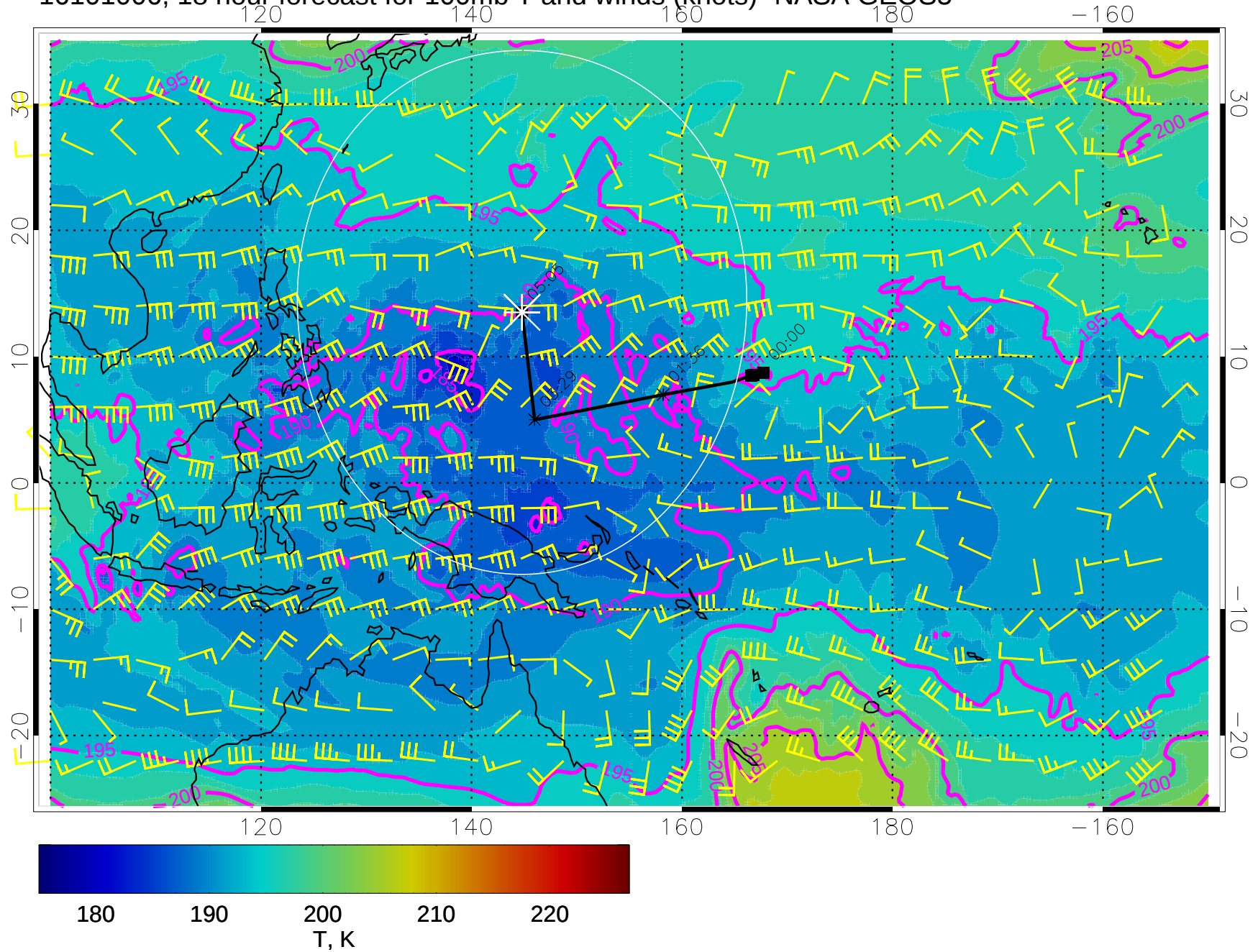
16101006, 18 hour forecast for 100mb T and winds (knots)- NASA GEOS5
