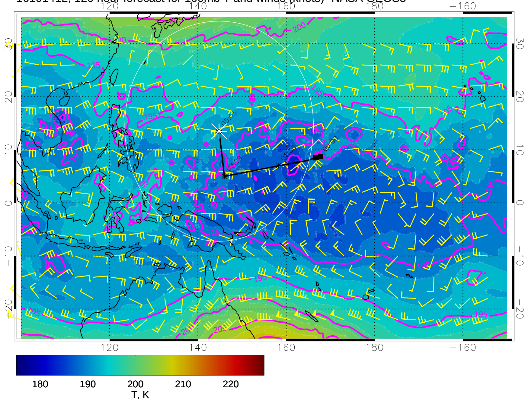
16101412, 120 hour forecast for 100mb T and winds (knots)- NASA GEOS5
