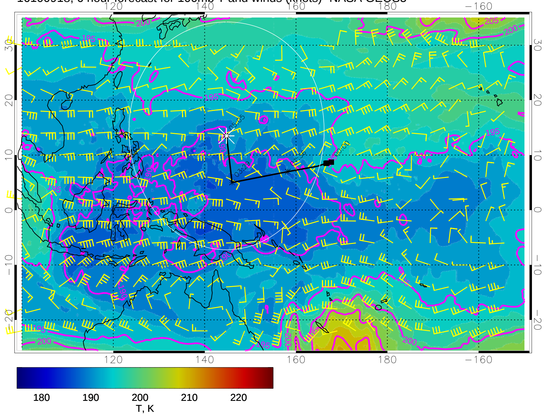
16100918, 6 hour forecast for 100mb T and winds (knots)- NASA GEOS5
