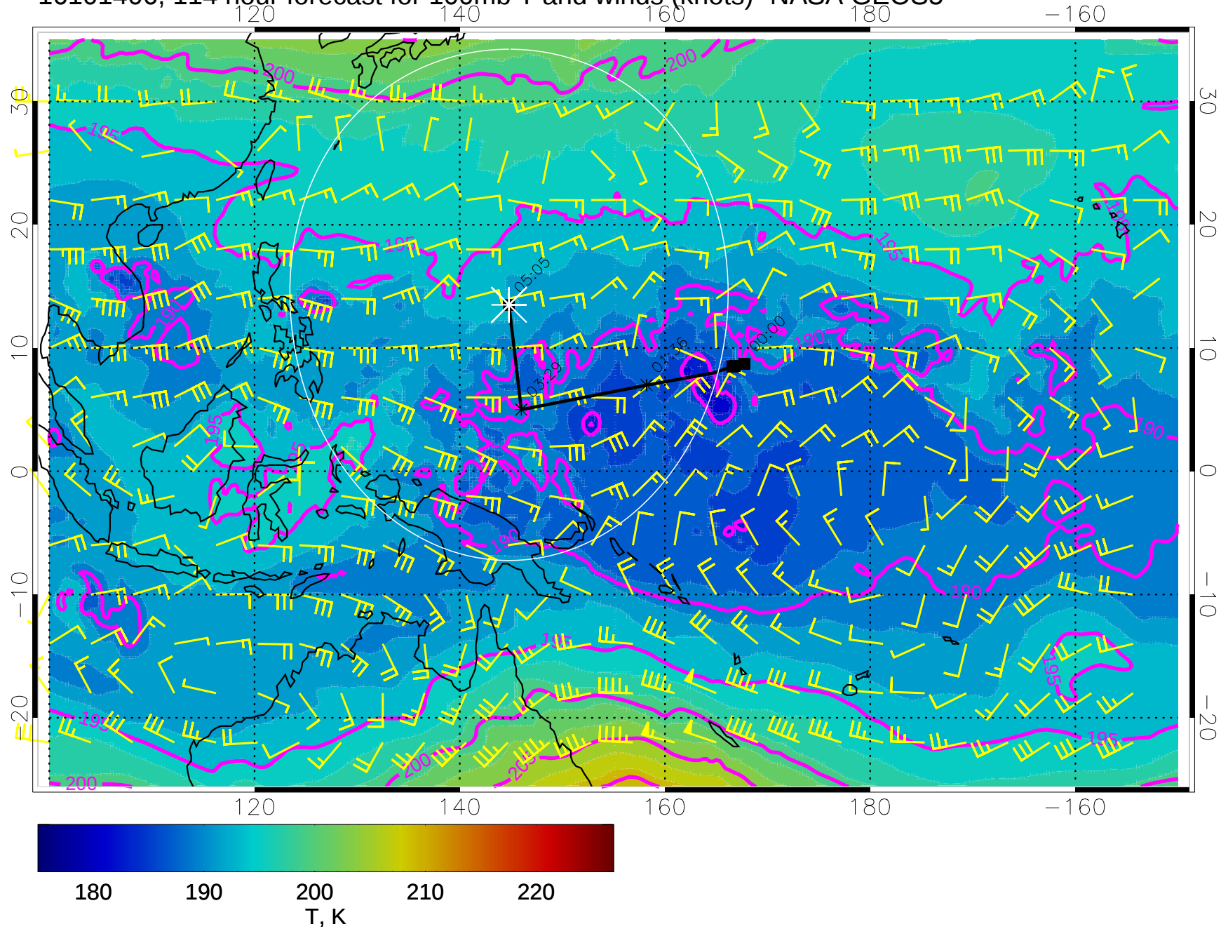
16101406, 114 hour forecast for 100mb T and winds (knots)- NASA GEOS5
