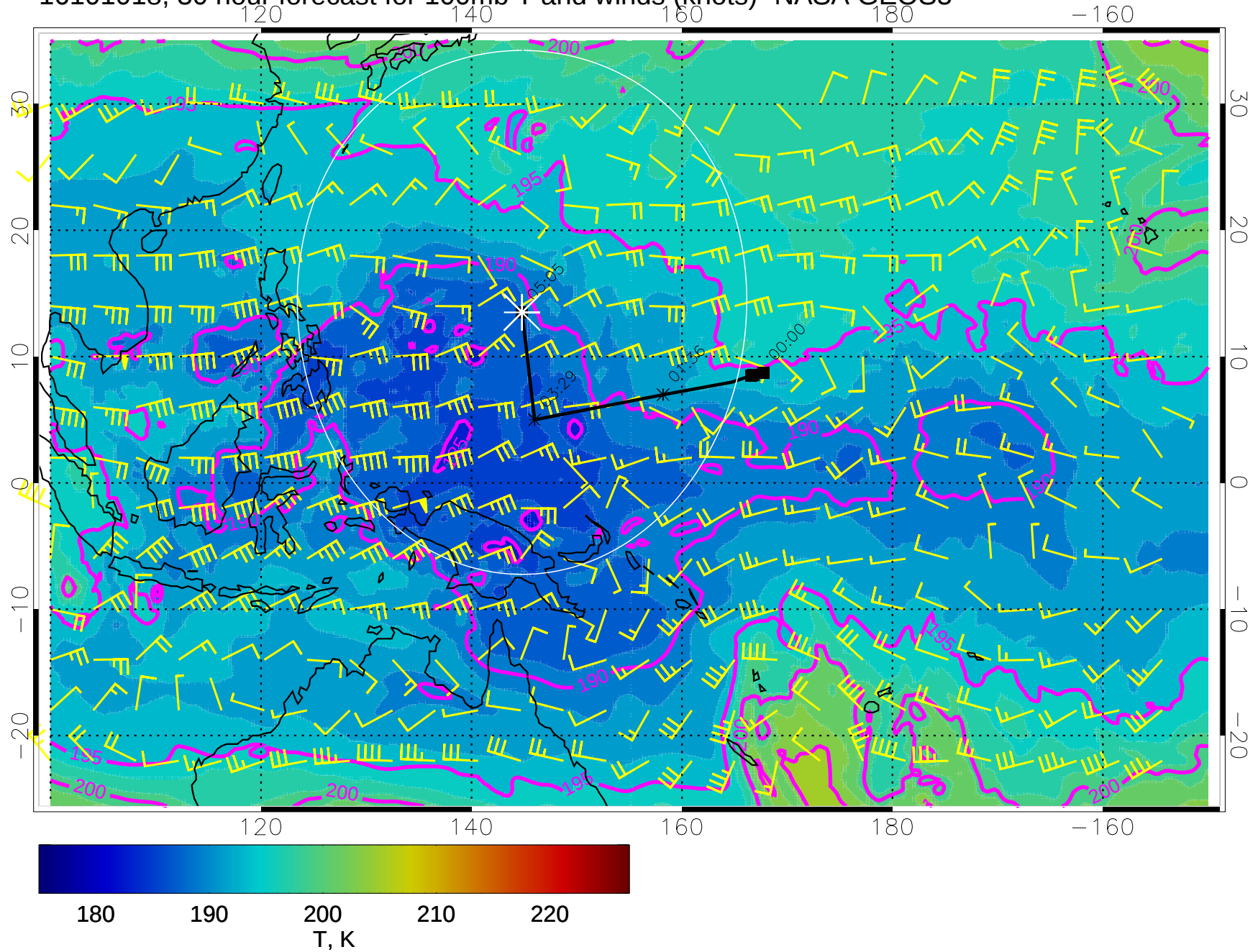
16101018, 30 hour forecast for 100mb T and winds (knots)- NASA GEOS5
