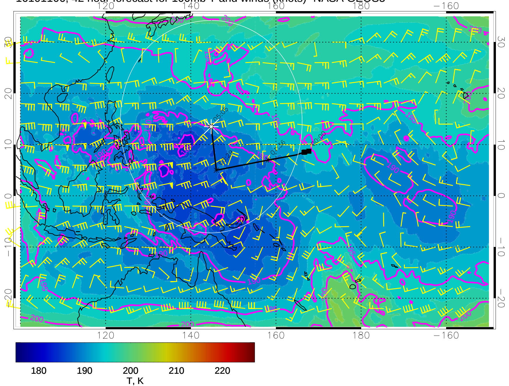
16101106, 42 hour forecast for 100mb T and winds (knots)- NASA GEOS5
