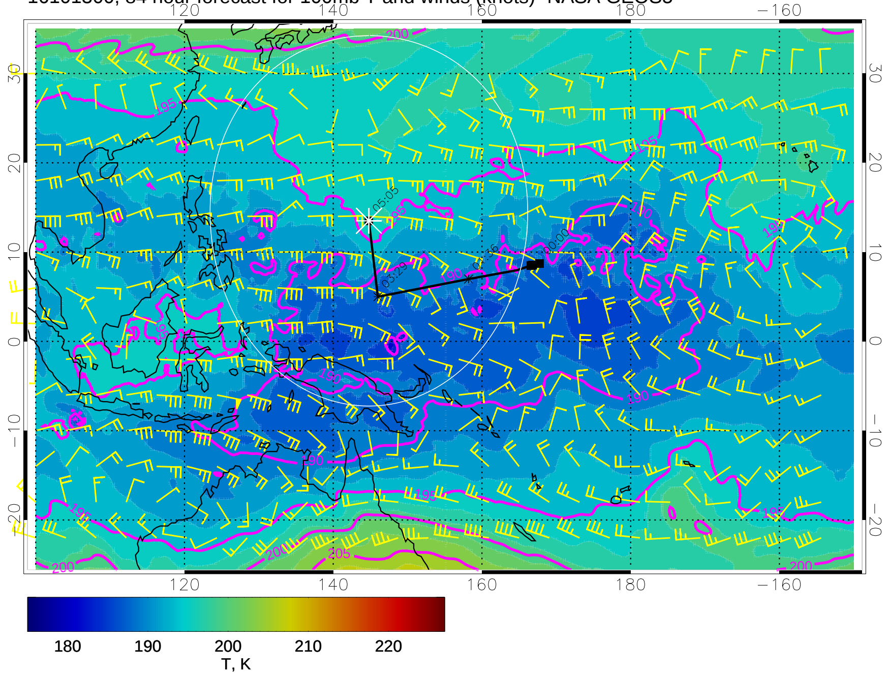
16101300, 84 hour forecast for 100mb T and winds (knots)- NASA GEOS5
