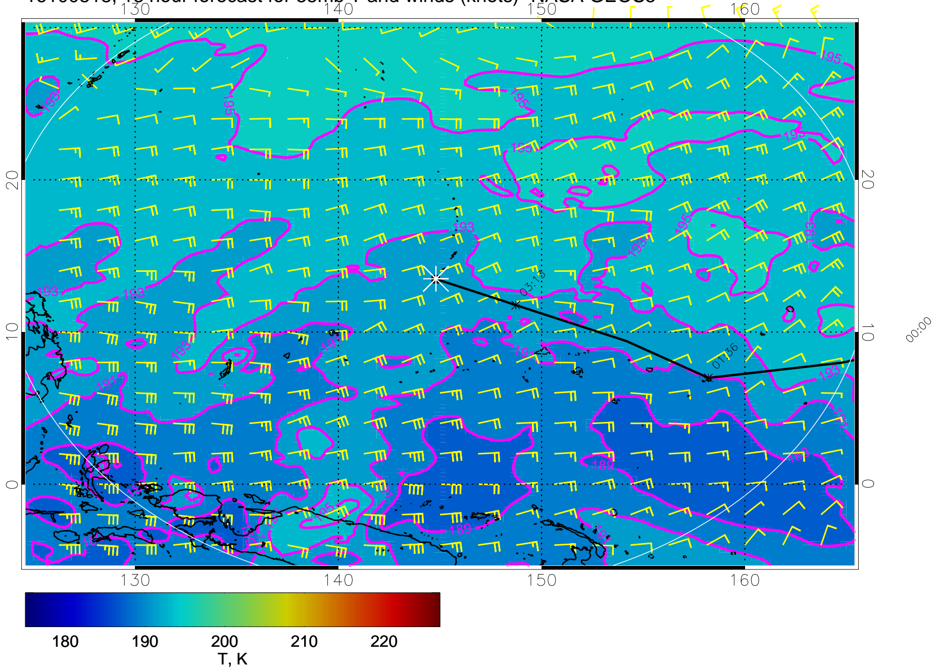
16100818, 18 hour forecast for 85mb T and winds (knots)- NASA GEOS5
