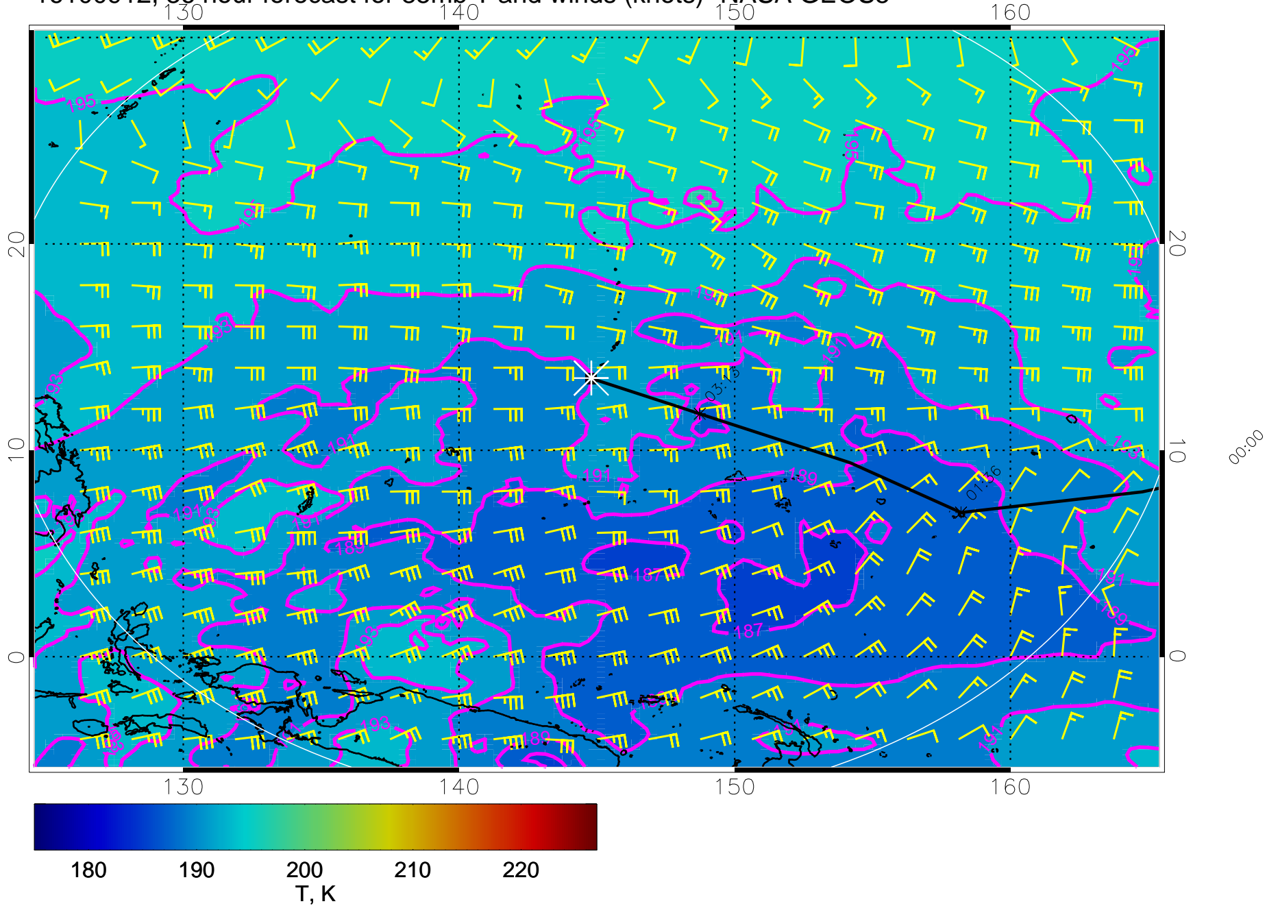
16100912, 36 hour forecast for 85mb T and winds (knots)- NASA GEOS5
