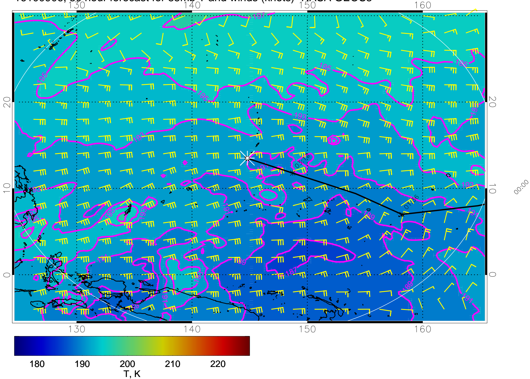
16100906, 30 hour forecast for 85mb T and winds (knots)- NASA GEOS5
