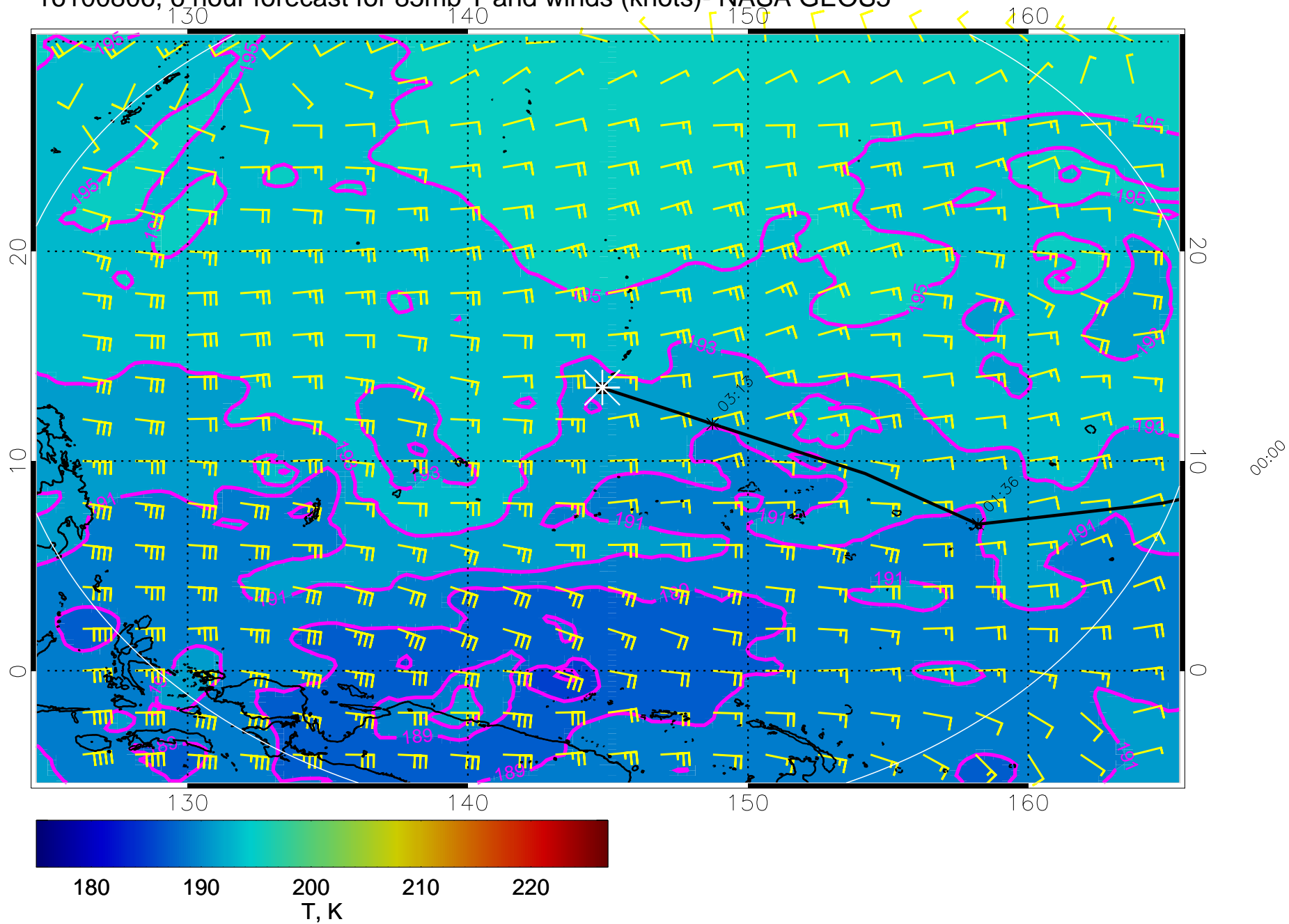
16100806, 6 hour forecast for 85mb T and winds (knots)- NASA GEOS5
