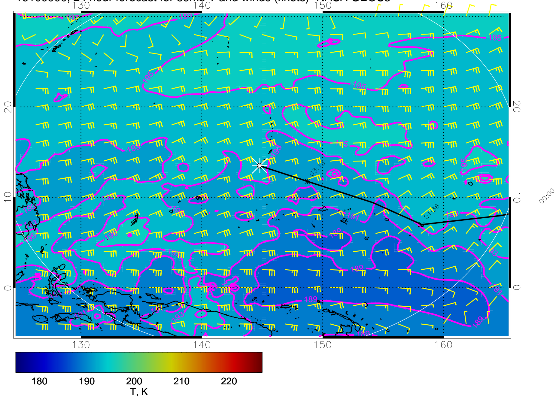
16100900, 24 hour forecast for 85mb T and winds (knots)- NASA GEOS5
