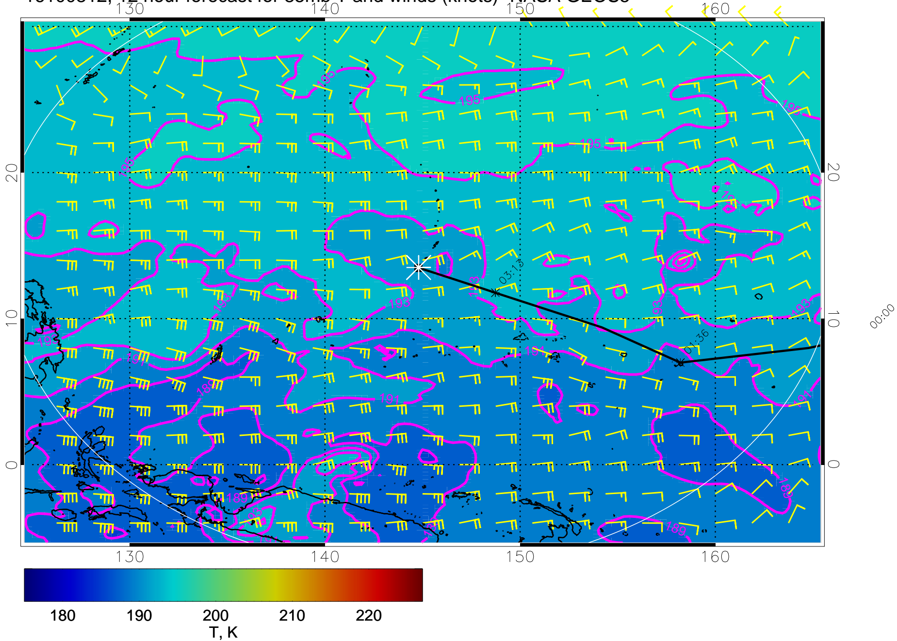
16100812, 12 hour forecast for 85mb T and winds (knots)- NASA GEOS5
