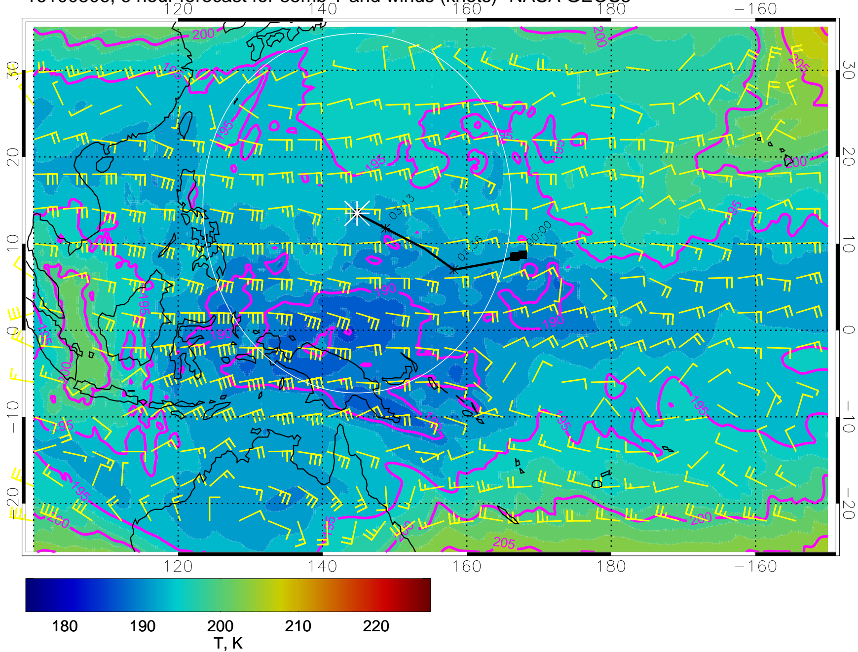
16100806, 6 hour forecast for 85mb T and winds (knots)- NASA GEOS5
