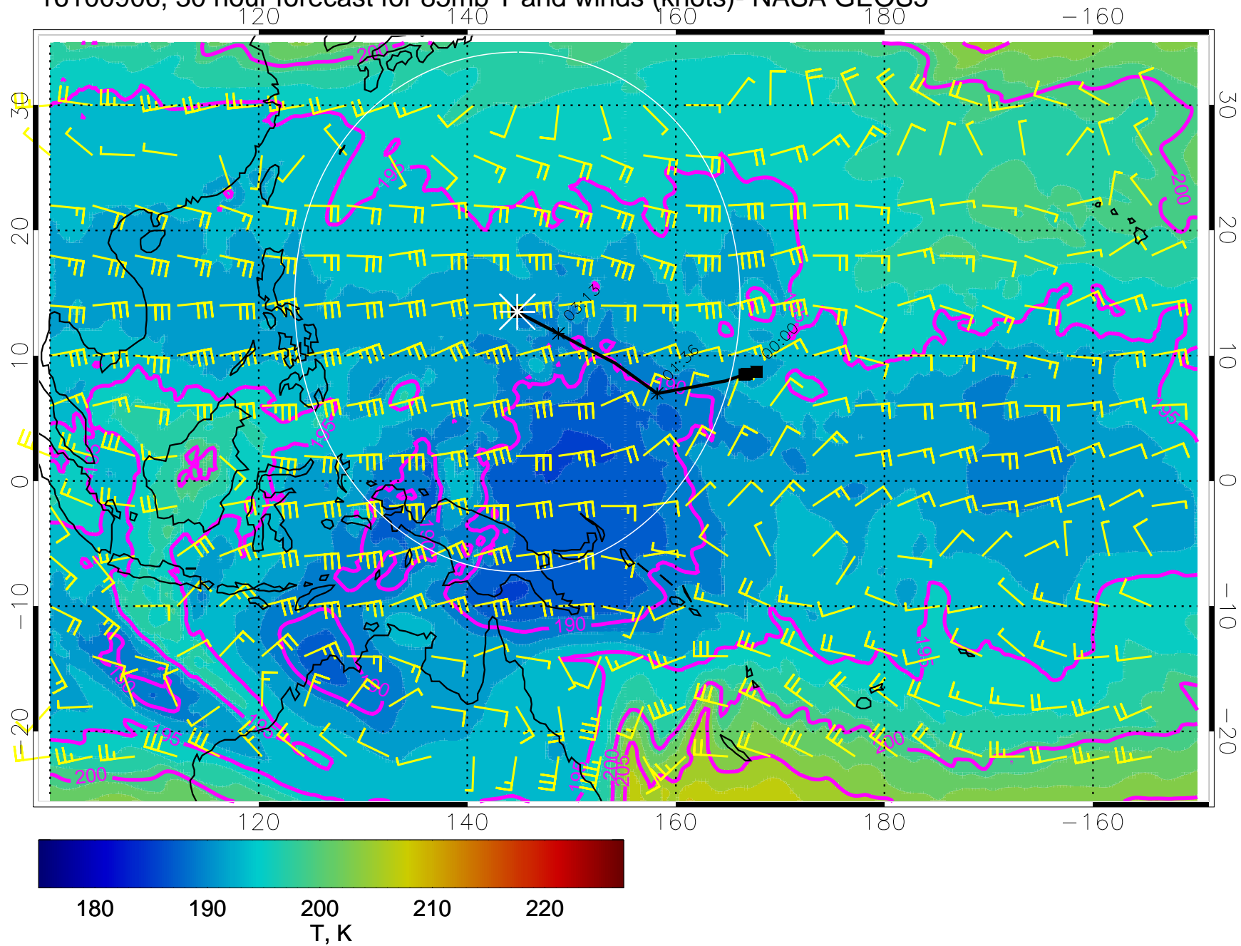
16100906, 30 hour forecast for 85mb T and winds (knots)- NASA GEOS5
