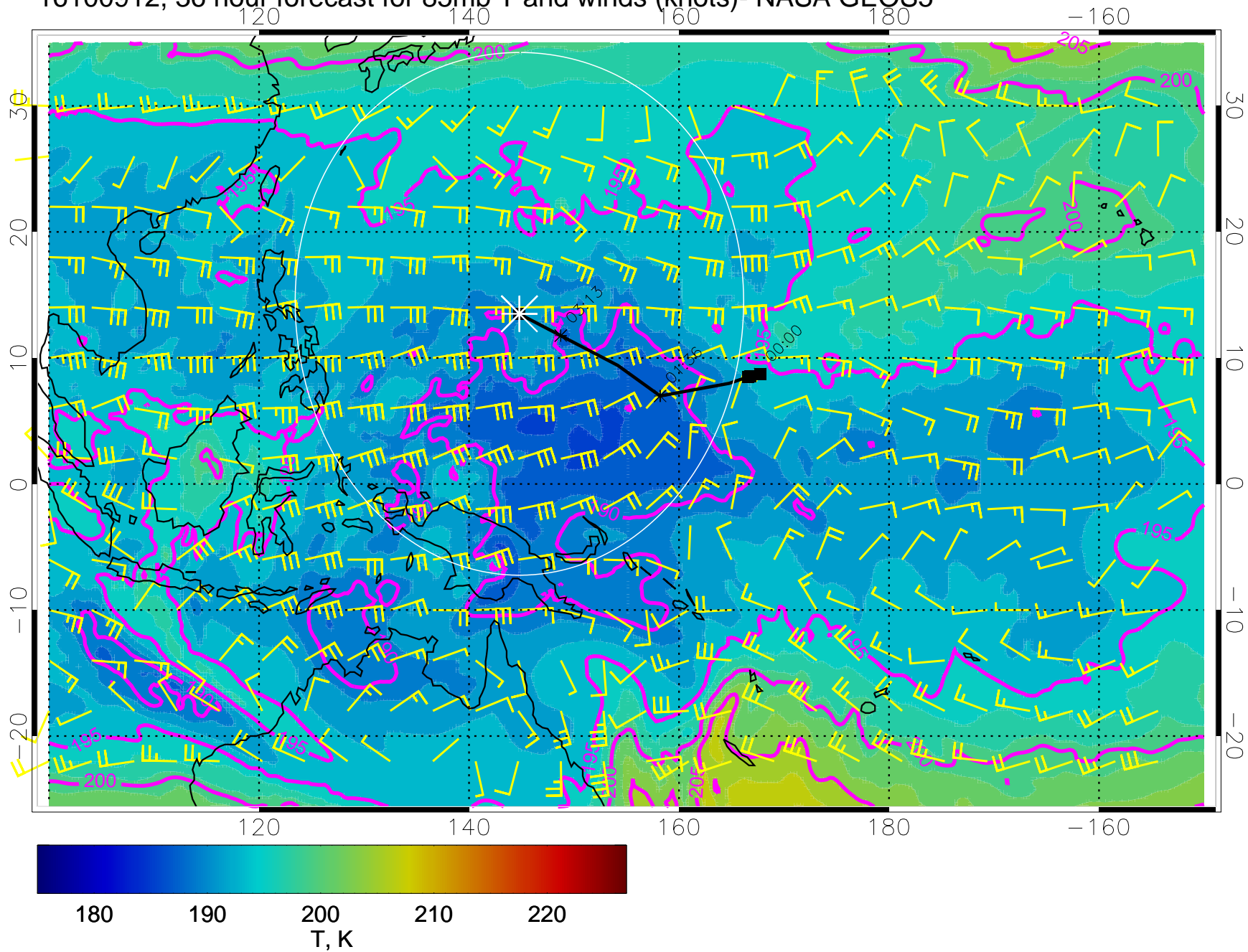
16100912, 36 hour forecast for 85mb T and winds (knots)- NASA GEOS5
