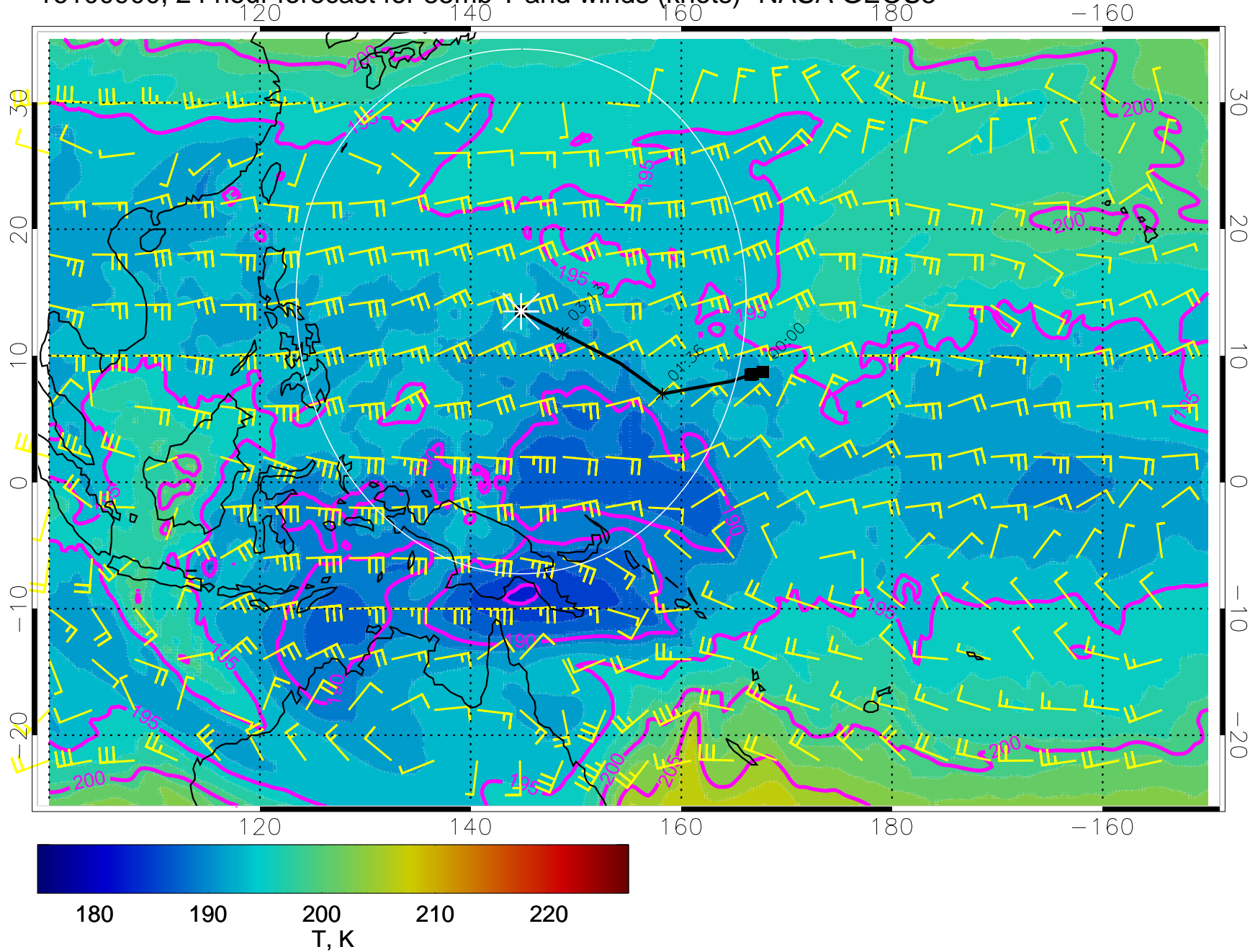
16100900, 24 hour forecast for 85mb T and winds (knots)- NASA GEOS5
