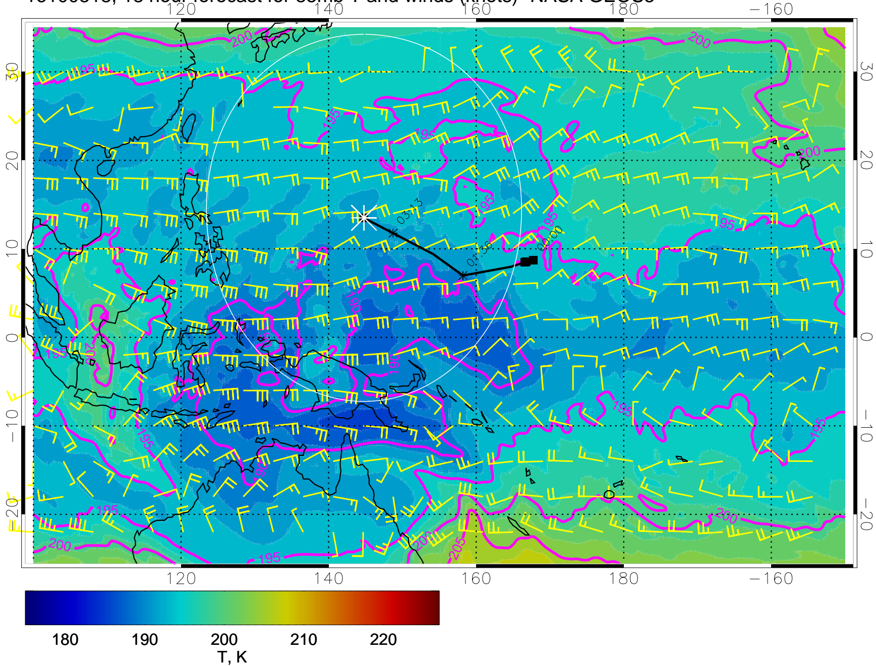
16100818, 18 hour forecast for 85mb T and winds (knots)- NASA GEOS5
