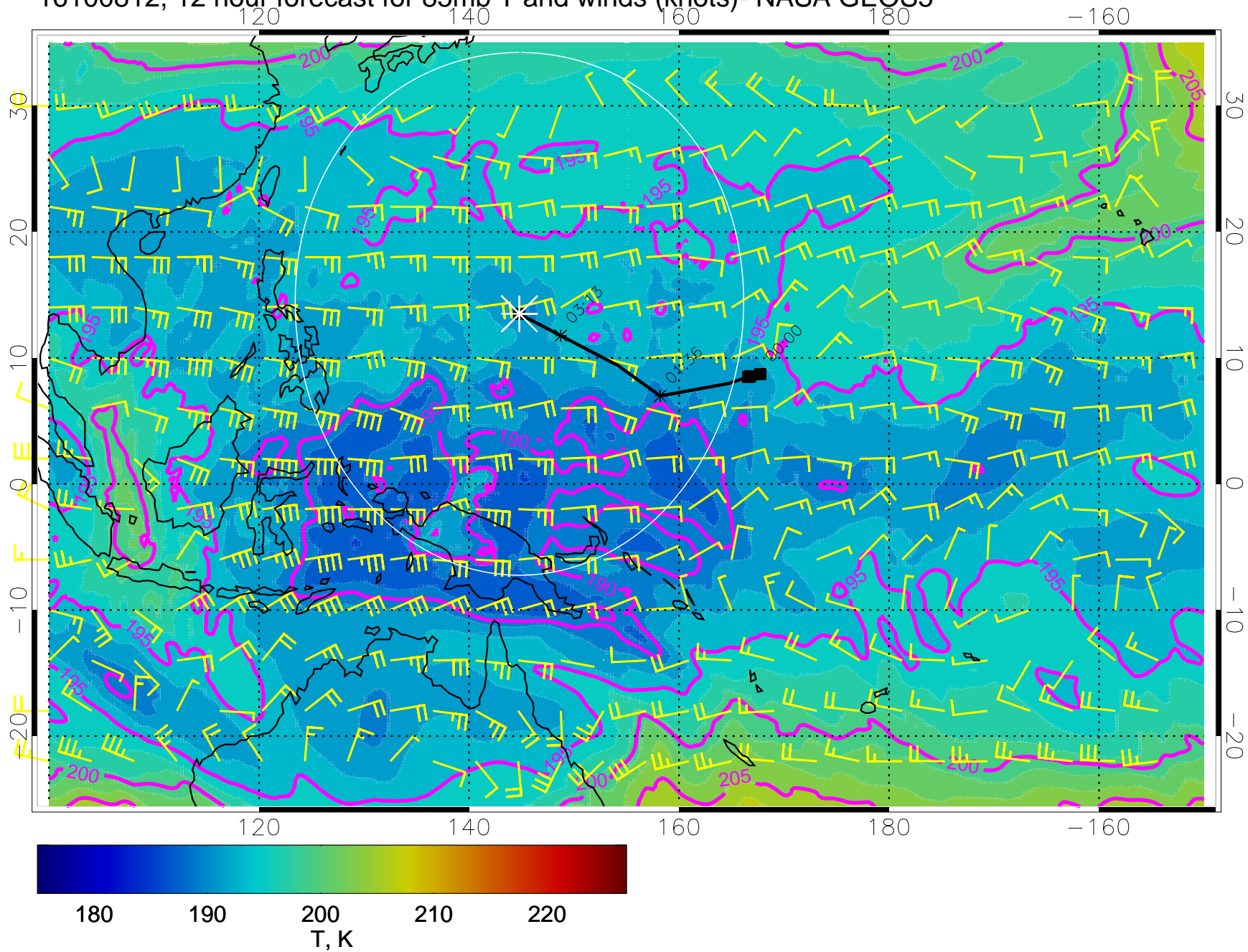
16100812, 12 hour forecast for 85mb T and winds (knots)- NASA GEOS5
