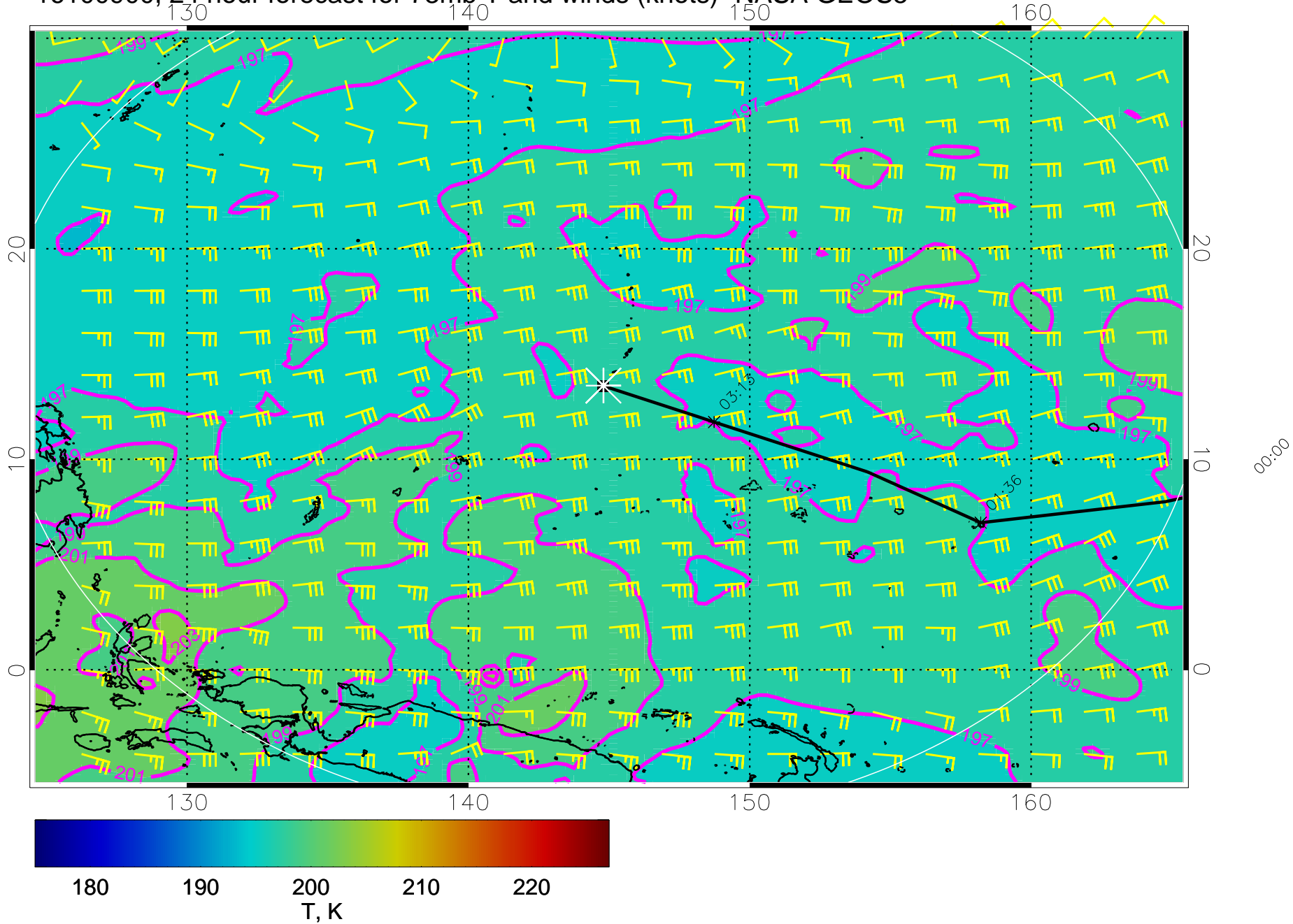
16100900, 24 hour forecast for 73mb T and winds (knots)- NASA GEOS5
