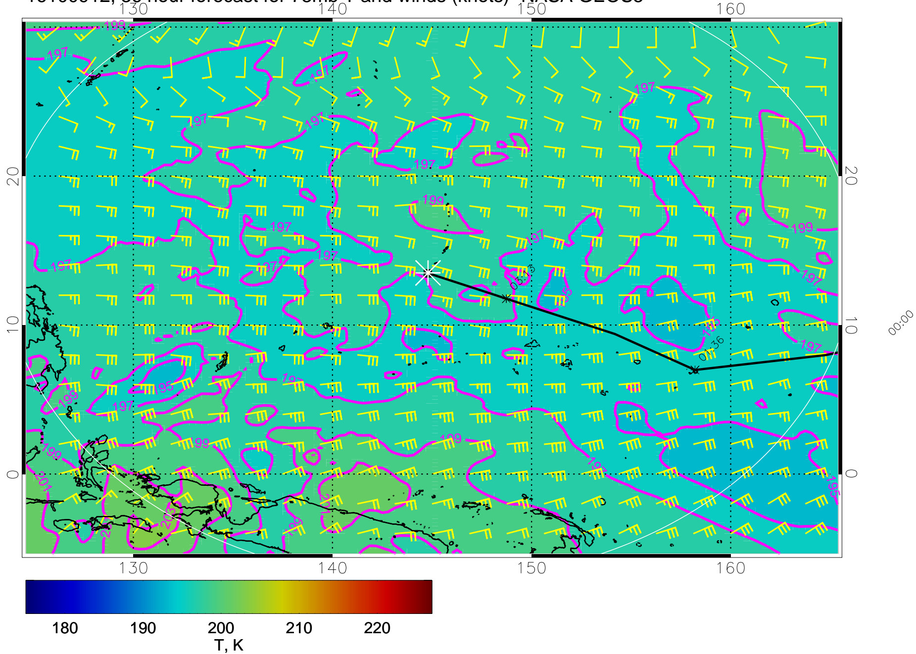
16100912, 36 hour forecast for 73mb T and winds (knots)- NASA GEOS5
