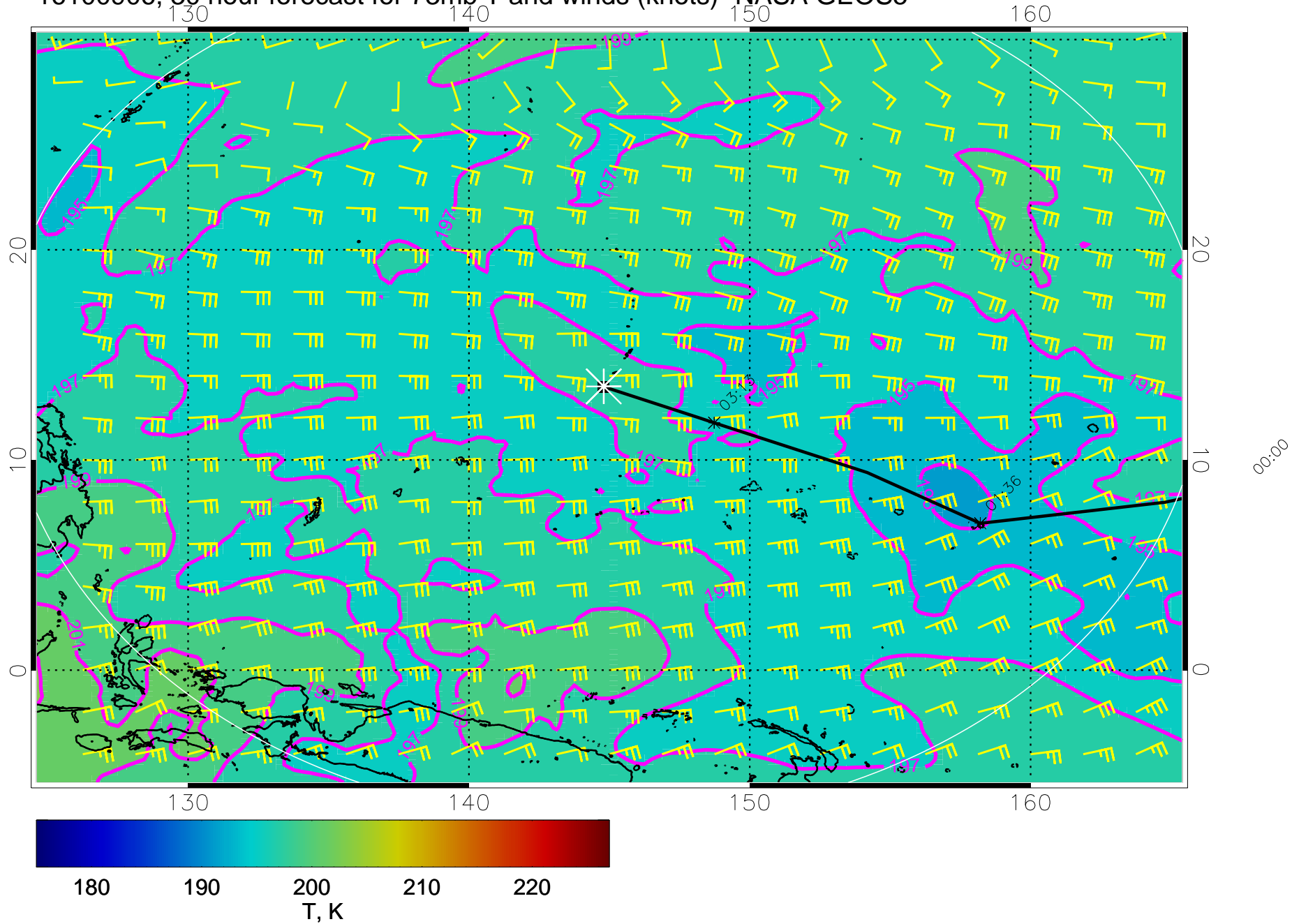
16100906, 30 hour forecast for 73mb T and winds (knots)- NASA GEOS5
