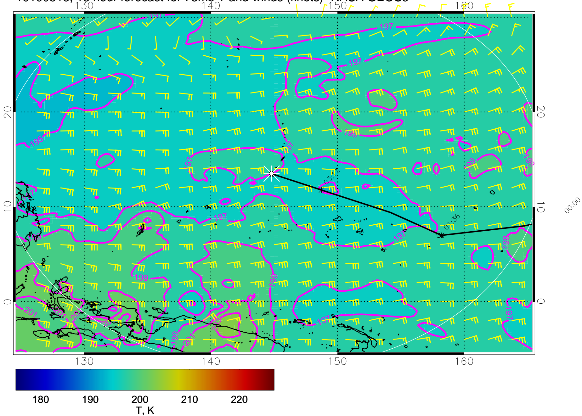
16100818, 18 hour forecast for 73mb T and winds (knots)- NASA GEOS5
