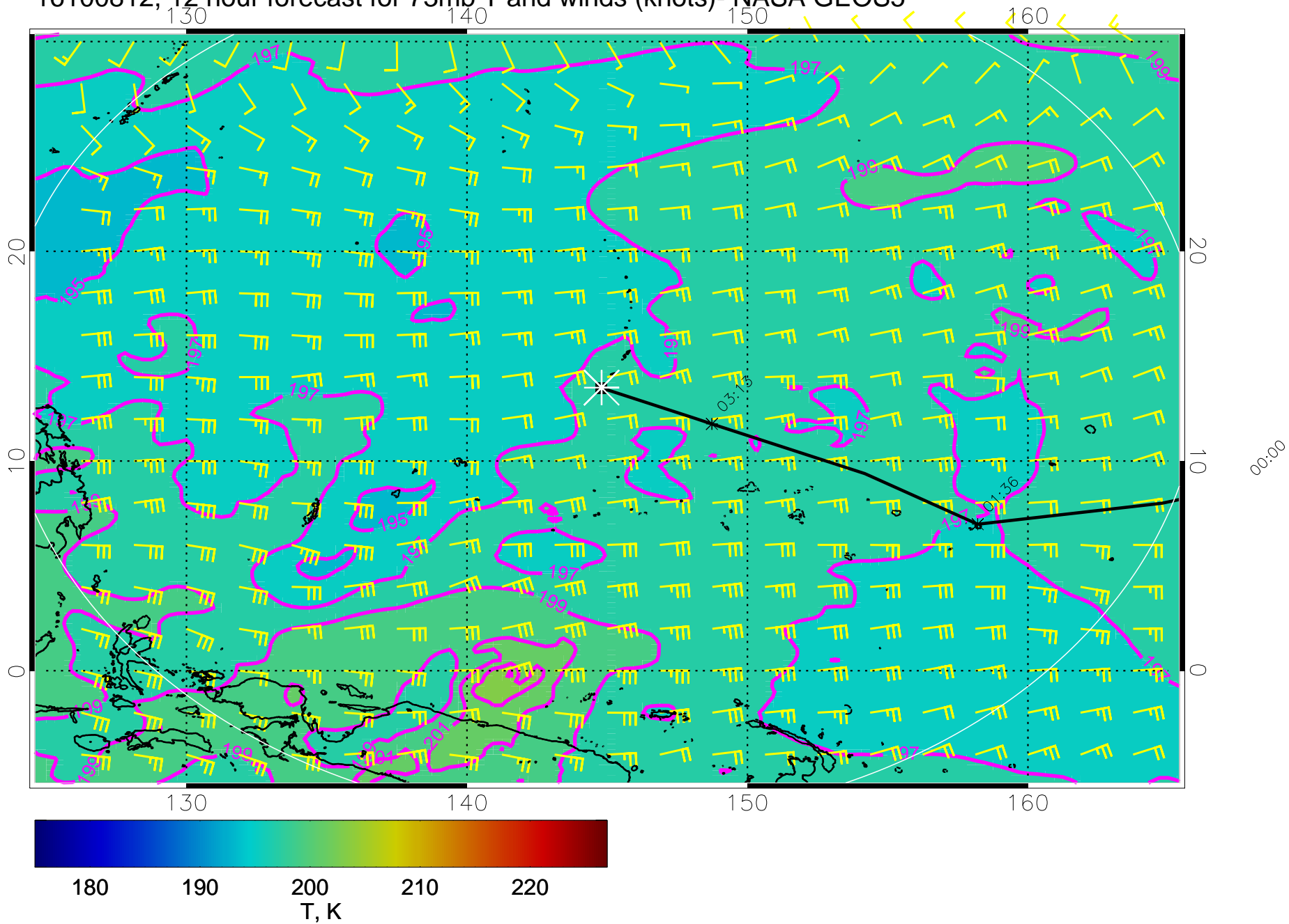
16100812, 12 hour forecast for 73mb T and winds (knots)- NASA GEOS5
