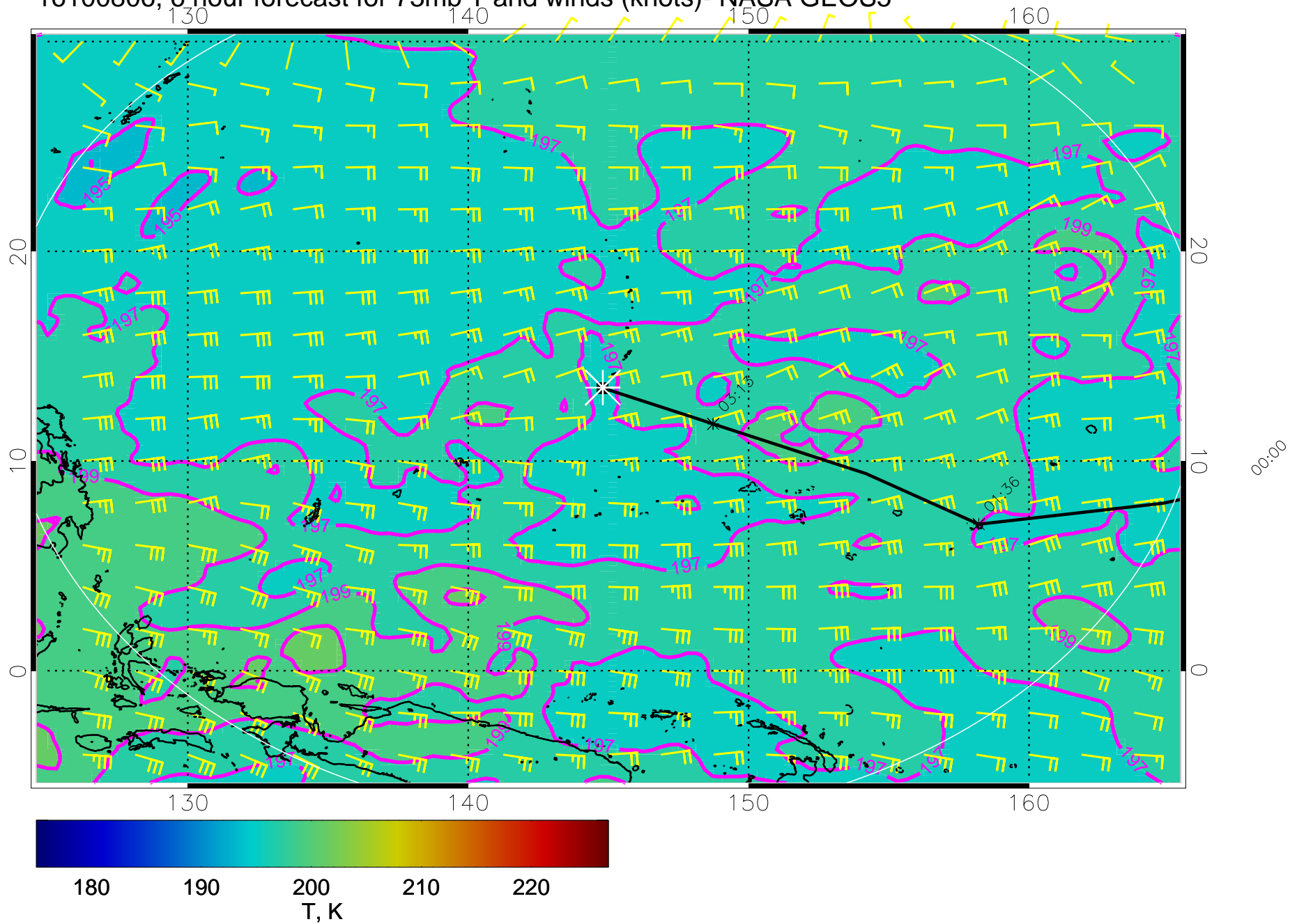
16100806, 6 hour forecast for 73mb T and winds (knots)- NASA GEOS5
