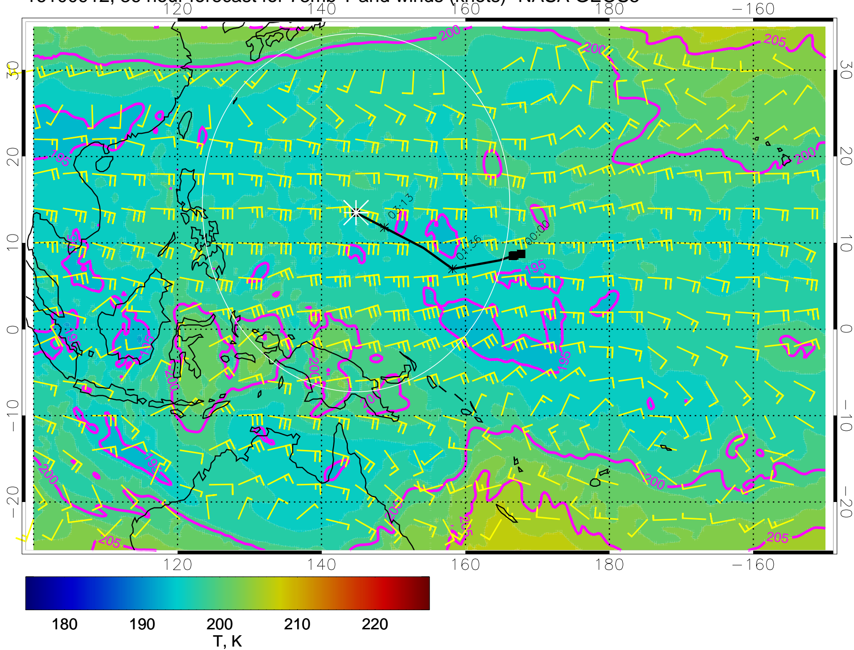
16100912, 36 hour forecast for 73mb T and winds (knots)- NASA GEOS5
