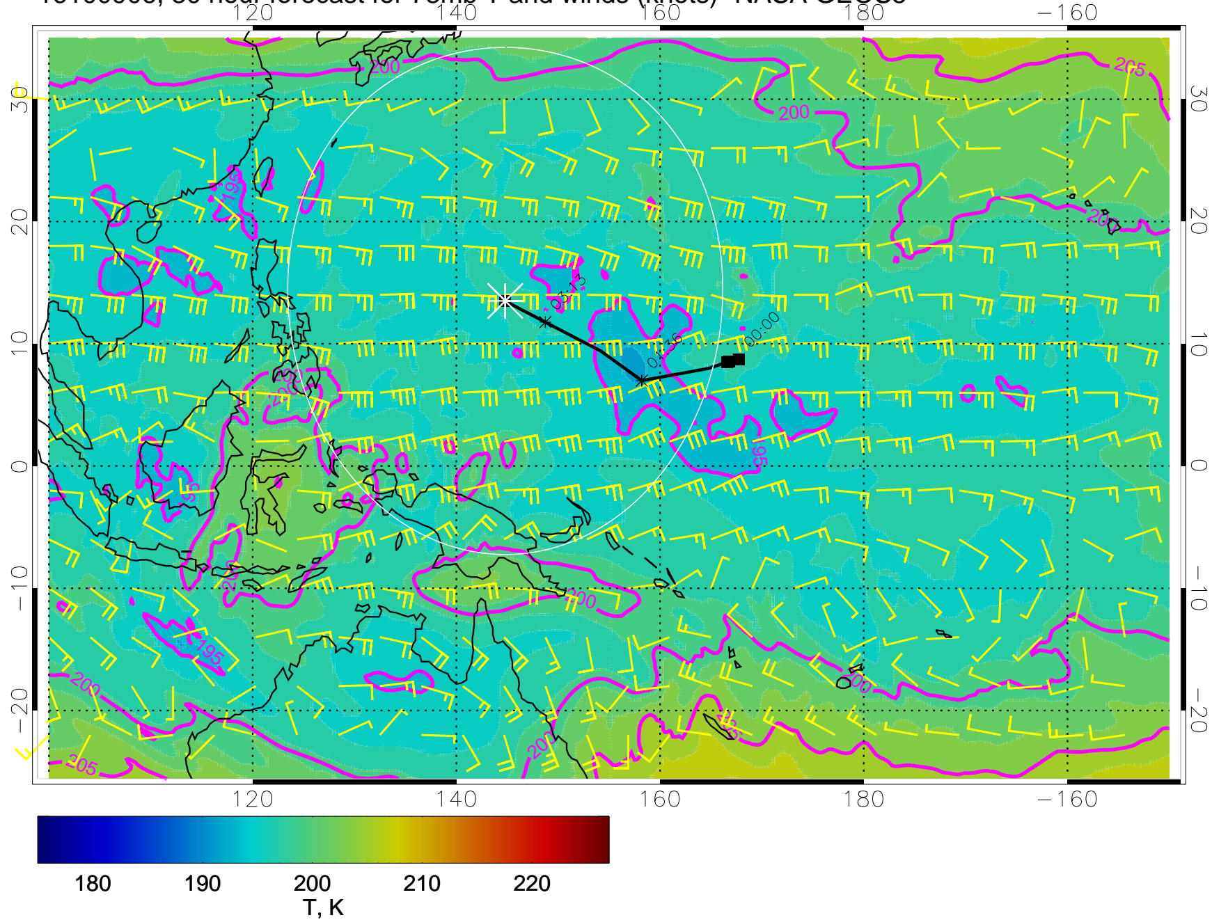
16100906, 30 hour forecast for 73mb T and winds (knots)- NASA GEOS5
