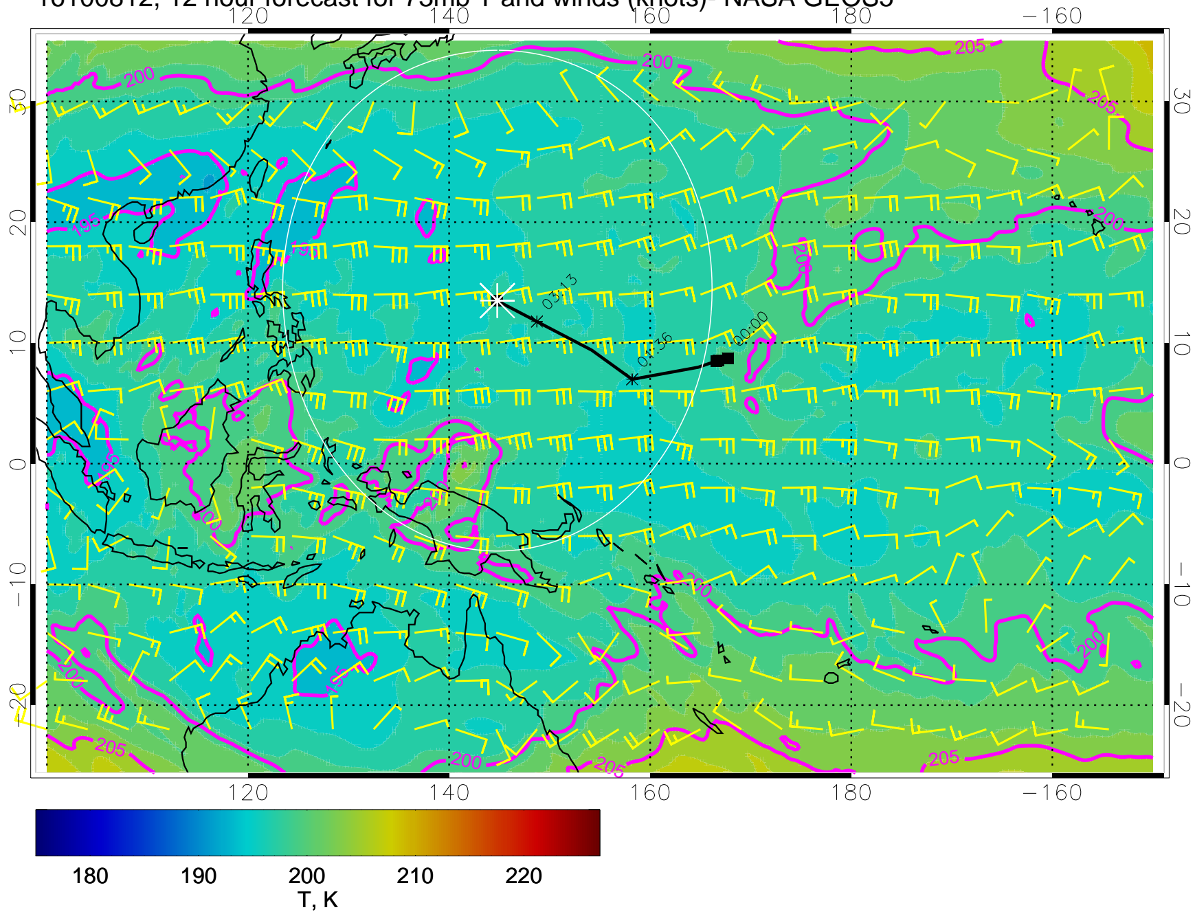
16100812, 12 hour forecast for 73mb T and winds (knots)- NASA GEOS5
