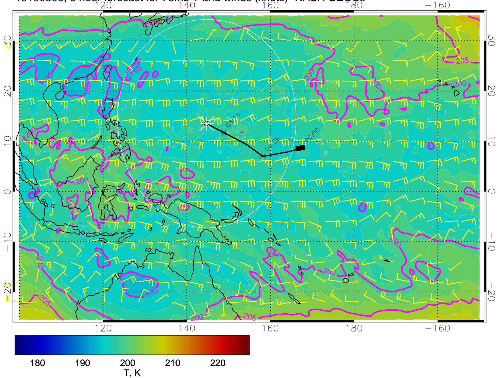
16100806, 6 hour forecast for 73mb T and winds (knots)- NASA GEOS5
