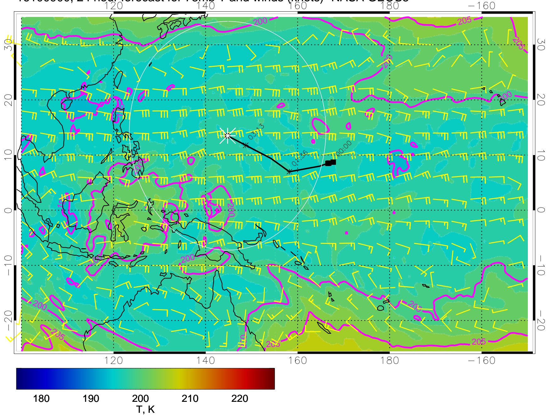
16100900, 24 hour forecast for 73mb T and winds (knots)- NASA GEOS5
