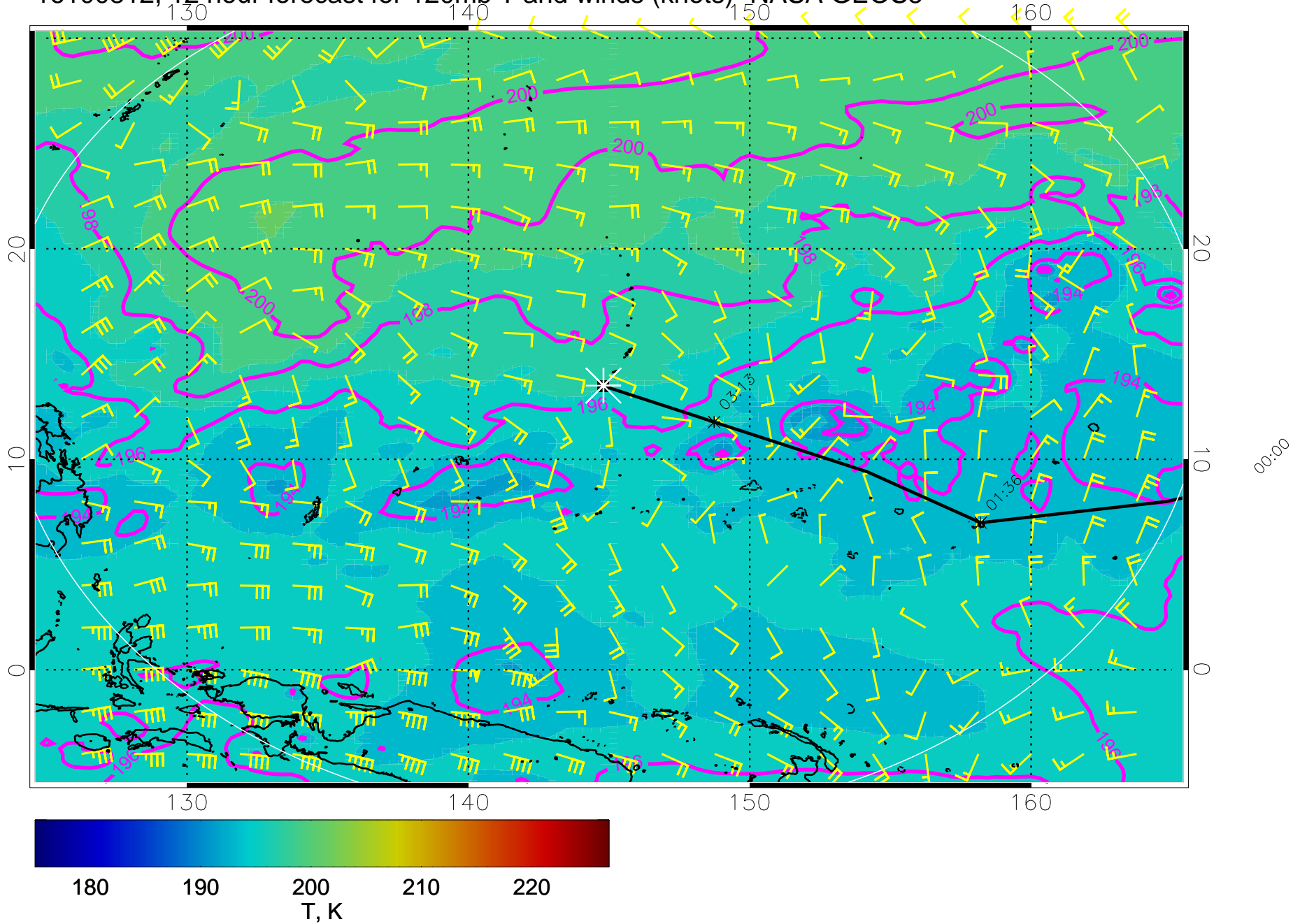
16100812, 12 hour forecast for 120mb T and winds (knots)- NASA GEOS5
