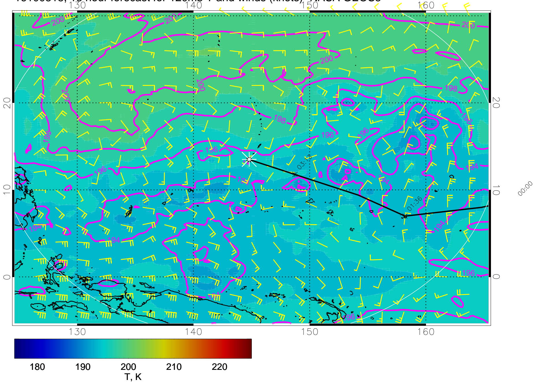
16100818, 18 hour forecast for 120mb T and winds (knots)- NASA GEOS5
