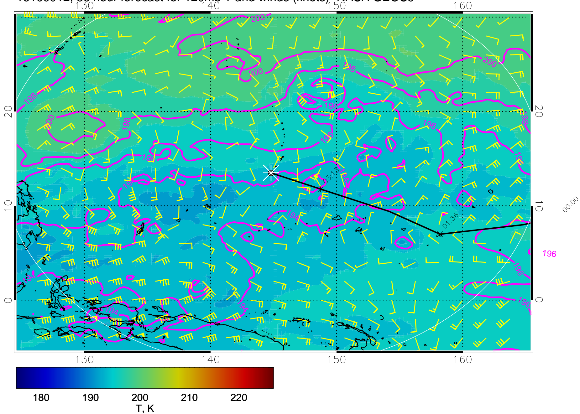
16100912, 36 hour forecast for 120mb T and winds (knots)- NASA GEOS5
