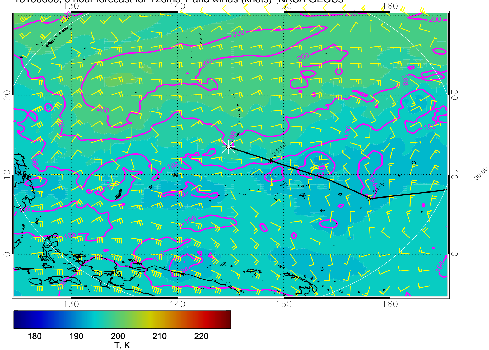
16100806, 6 hour forecast for 120mb T and winds (knots)- NASA GEOS5
