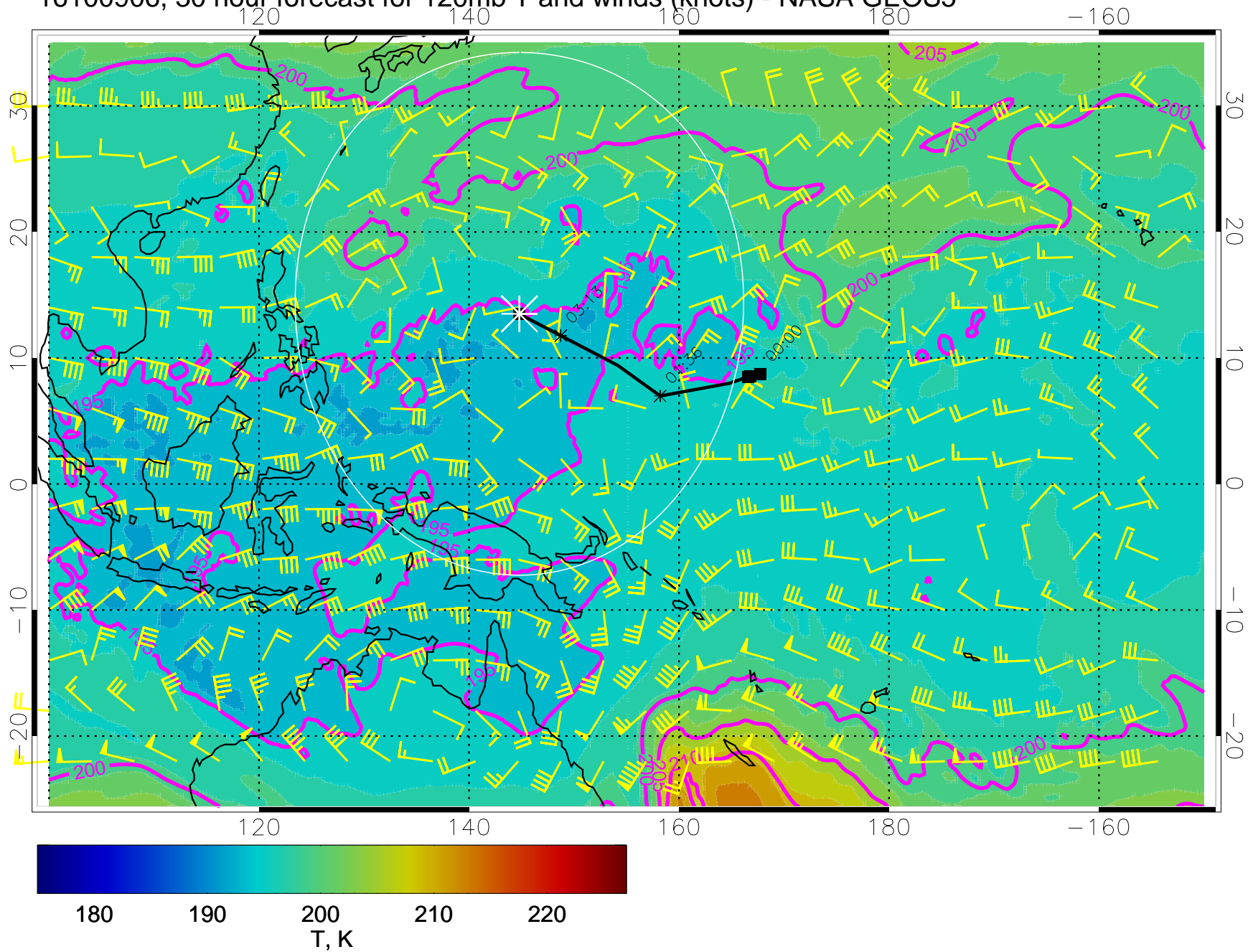
16100906, 30 hour forecast for 120mb T and winds (knots) - NASA GEOS5
