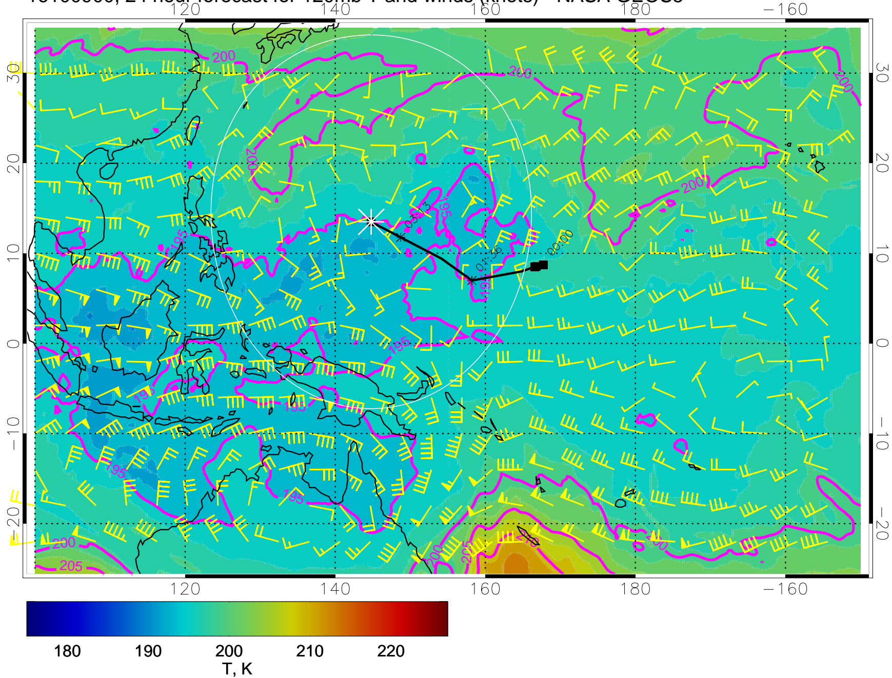
16100900, 24 hour forecast for 120mb T and winds (knots) - NASA GEOS5
