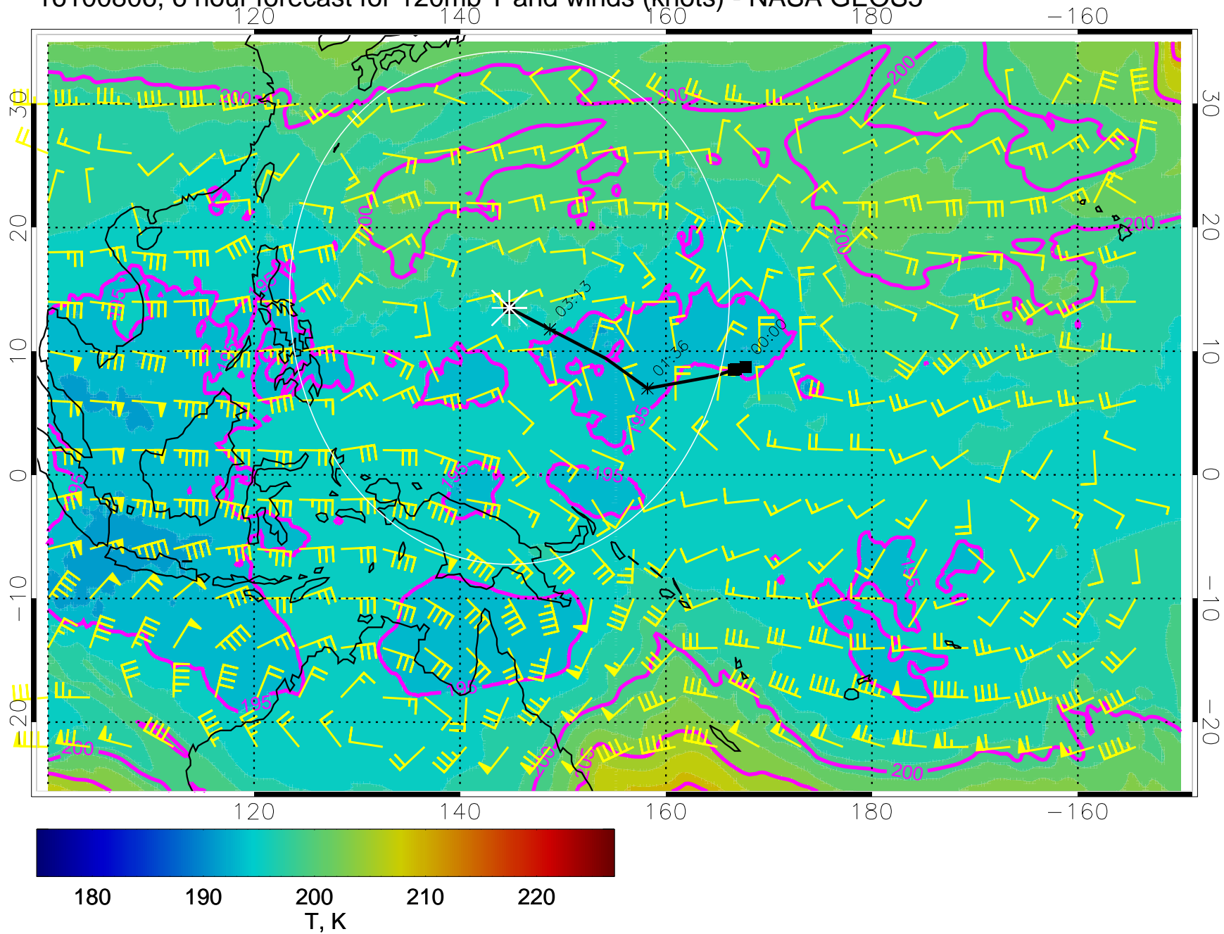
16100806, 6 hour forecast for 120mb T and winds (knots) - NASA GEOS5
