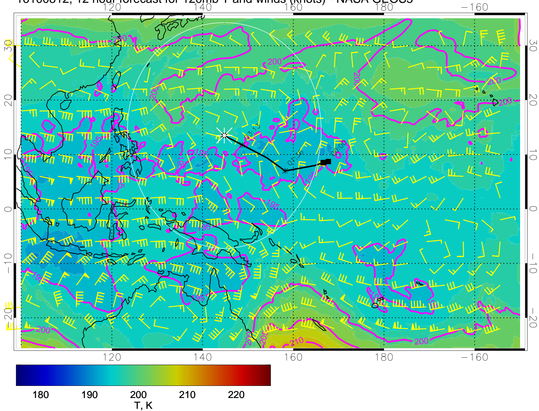
16100812, 12 hour forecast for 120mb T and winds (knots) - NASA GEOS5
