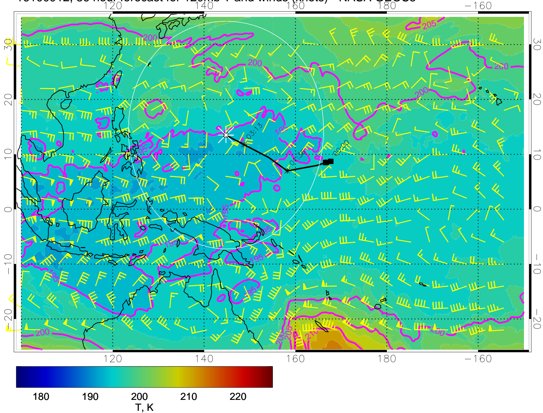
16100912, 36 hour forecast for 120mb T and winds (knots) - NASA GEOS5
