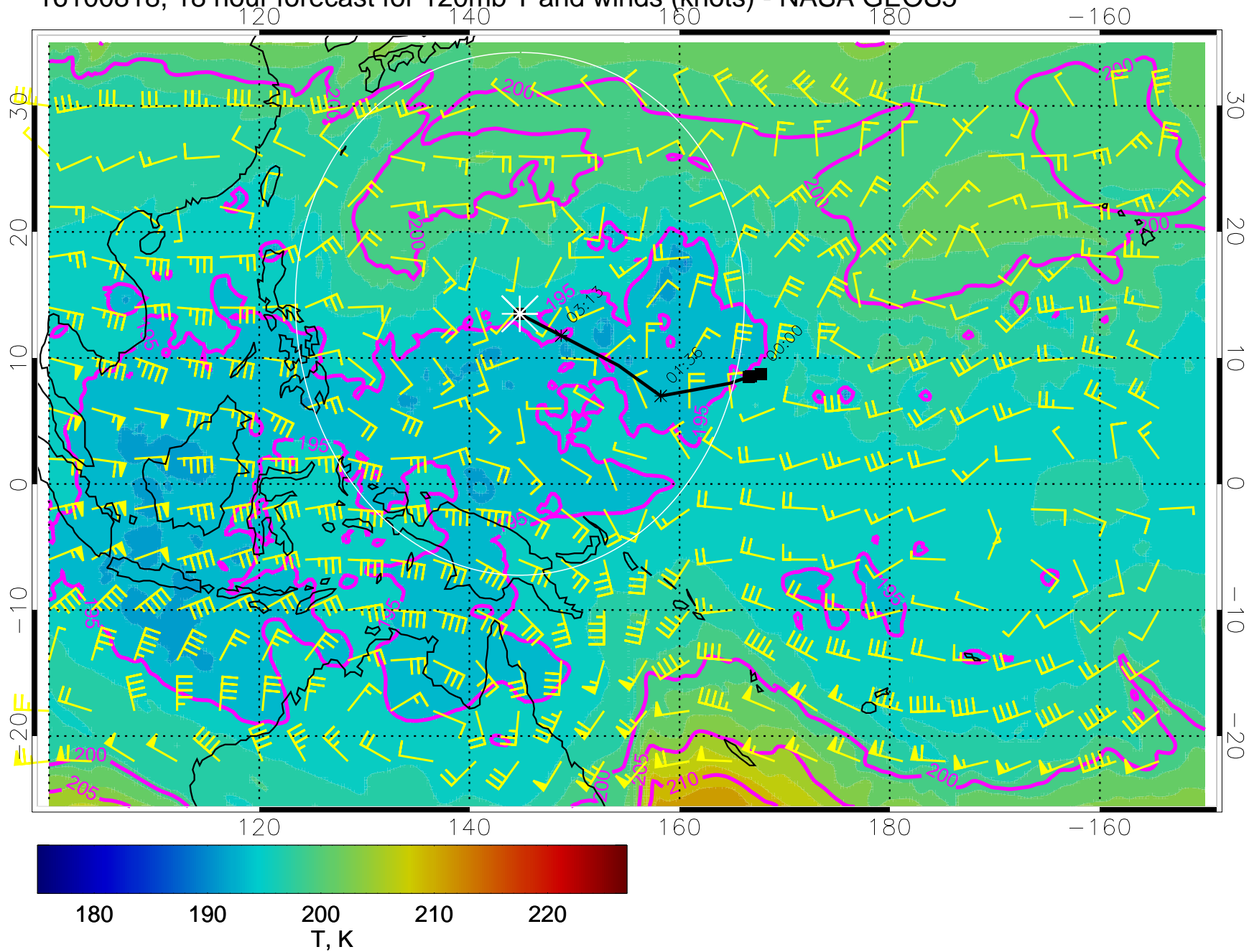
16100818, 18 hour forecast for 120mb T and winds (knots) - NASA GEOS5
