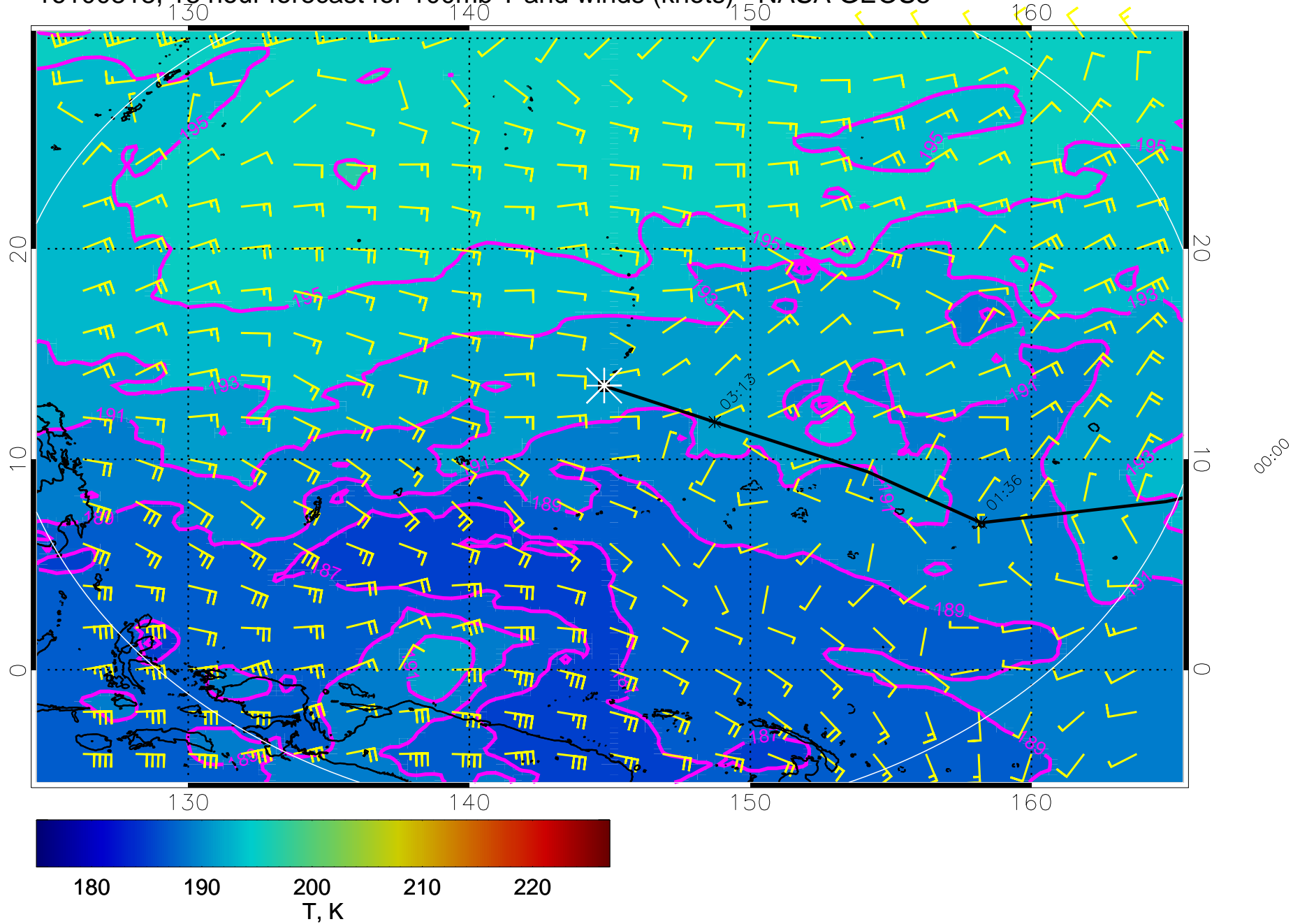
16100818, 18 hour forecast for 100mb T and winds (knots) - NASA GEOS5
