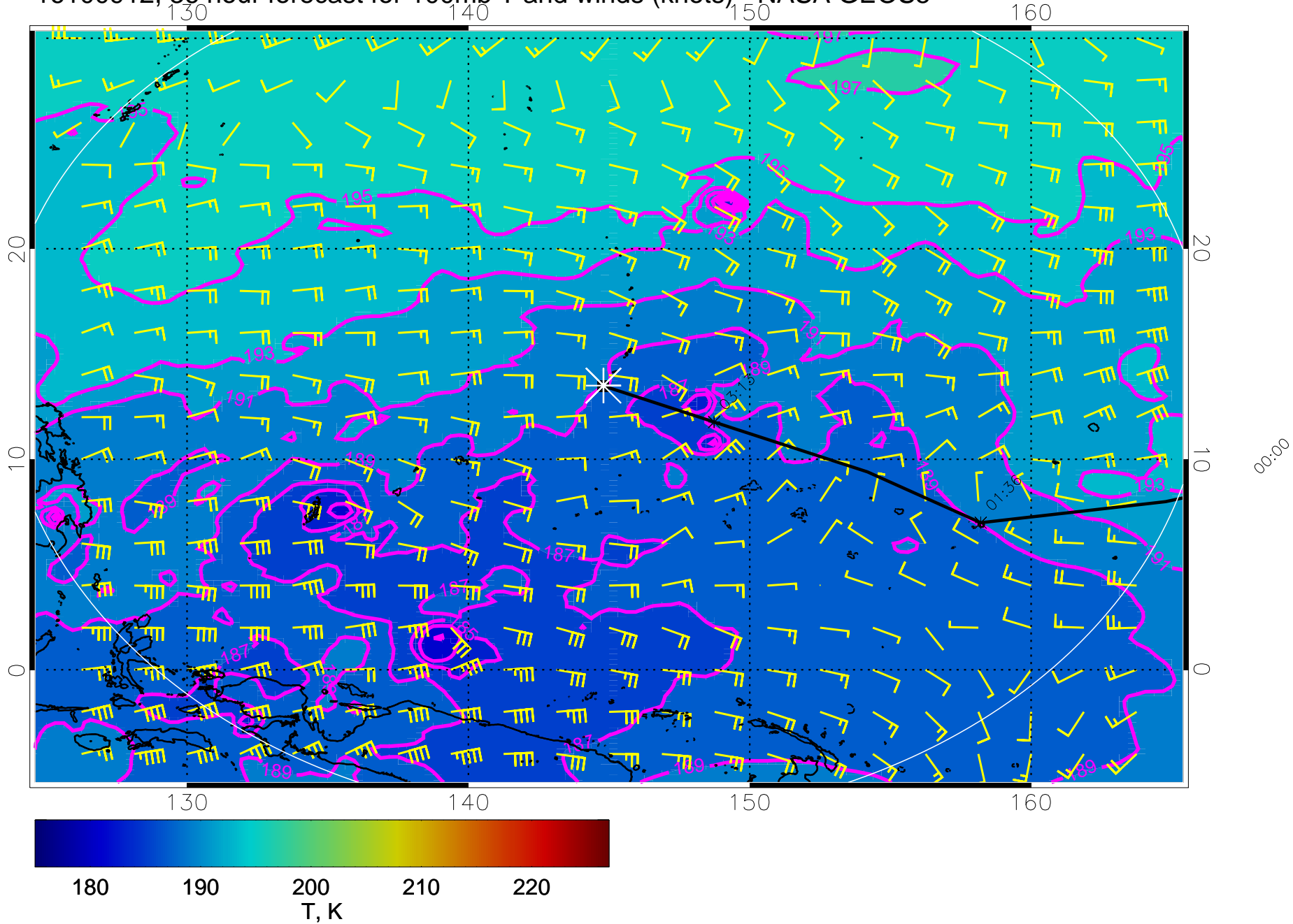
16100912, 36 hour forecast for 100mb T and winds (knots) - NASA GEOS5
