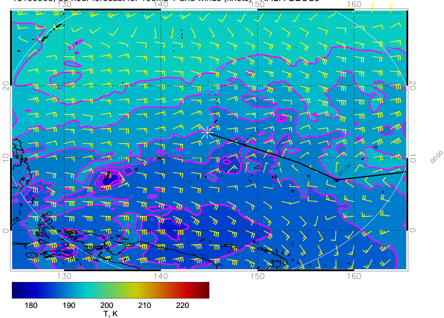
16100906, 30 hour forecast for 100mb T and winds (knots) - NASA GEOS5
