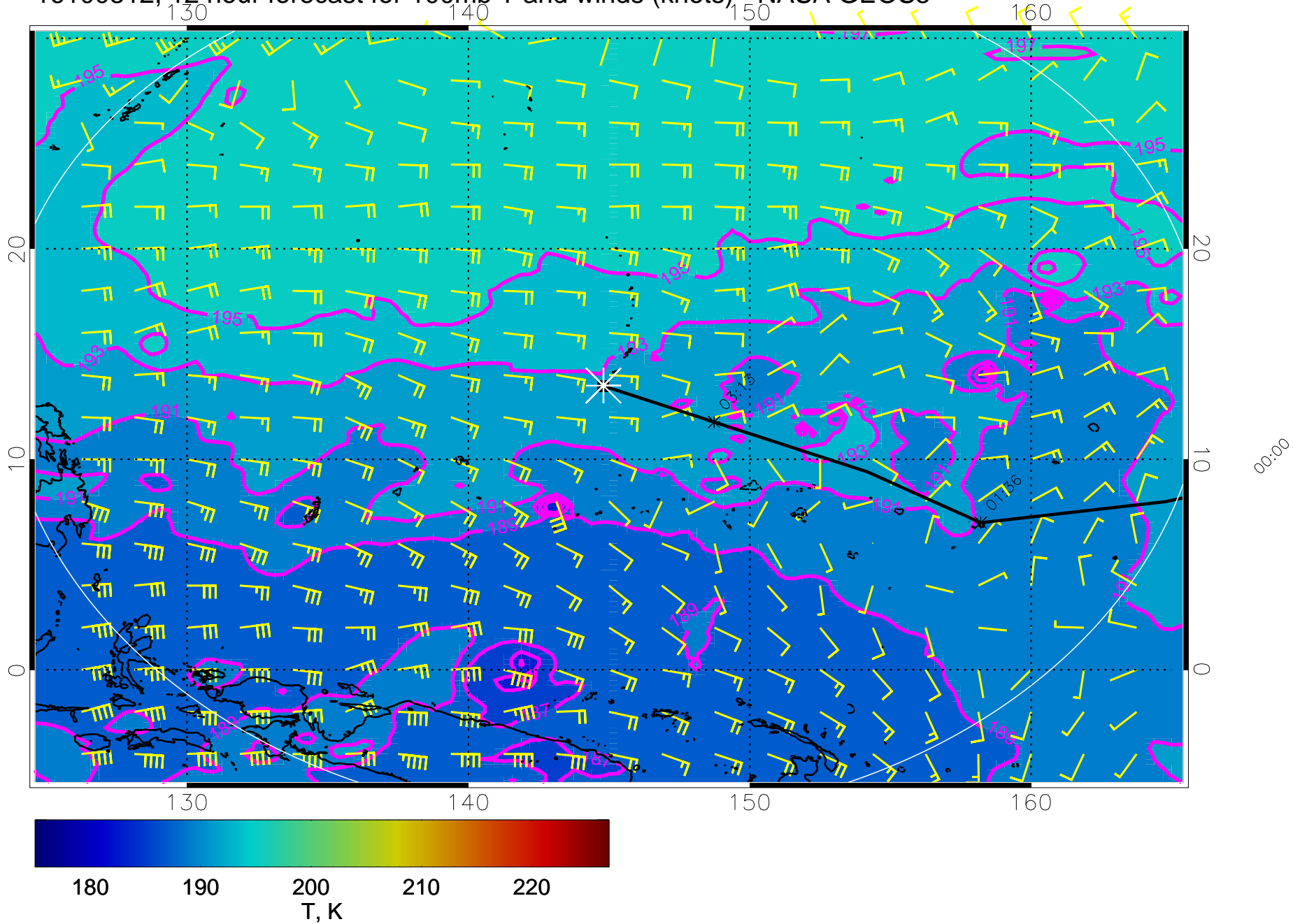
16100812, 12 hour forecast for 100mb T and winds (knots) - NASA GEOS5
