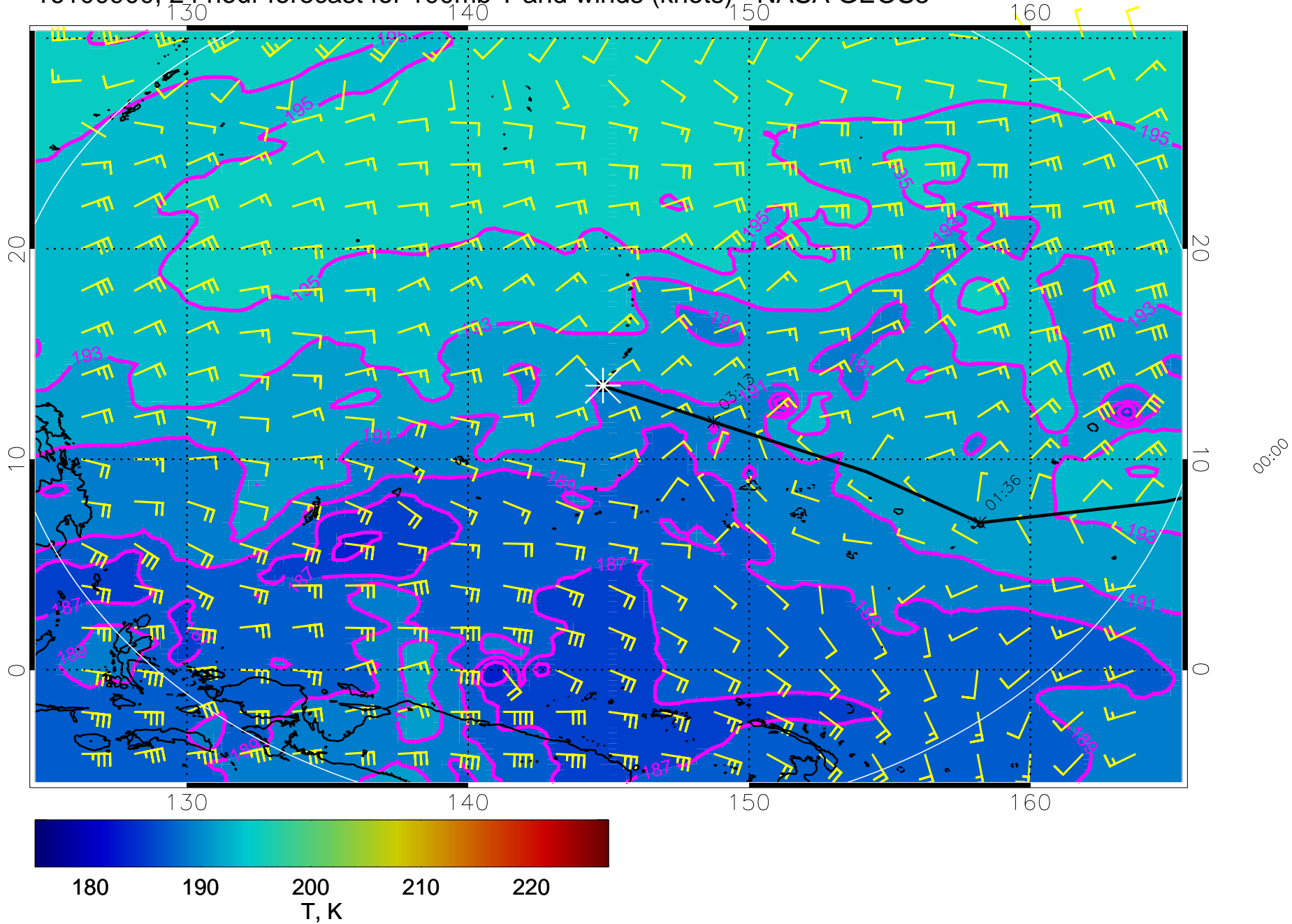
16100900, 24 hour forecast for 100mb T and winds (knots) - NASA GEOS5
