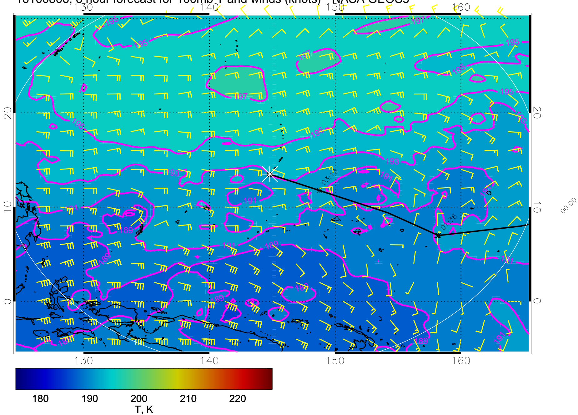
16100806, 6 hour forecast for 100mb T and winds (knots) - NASA GEOS5
