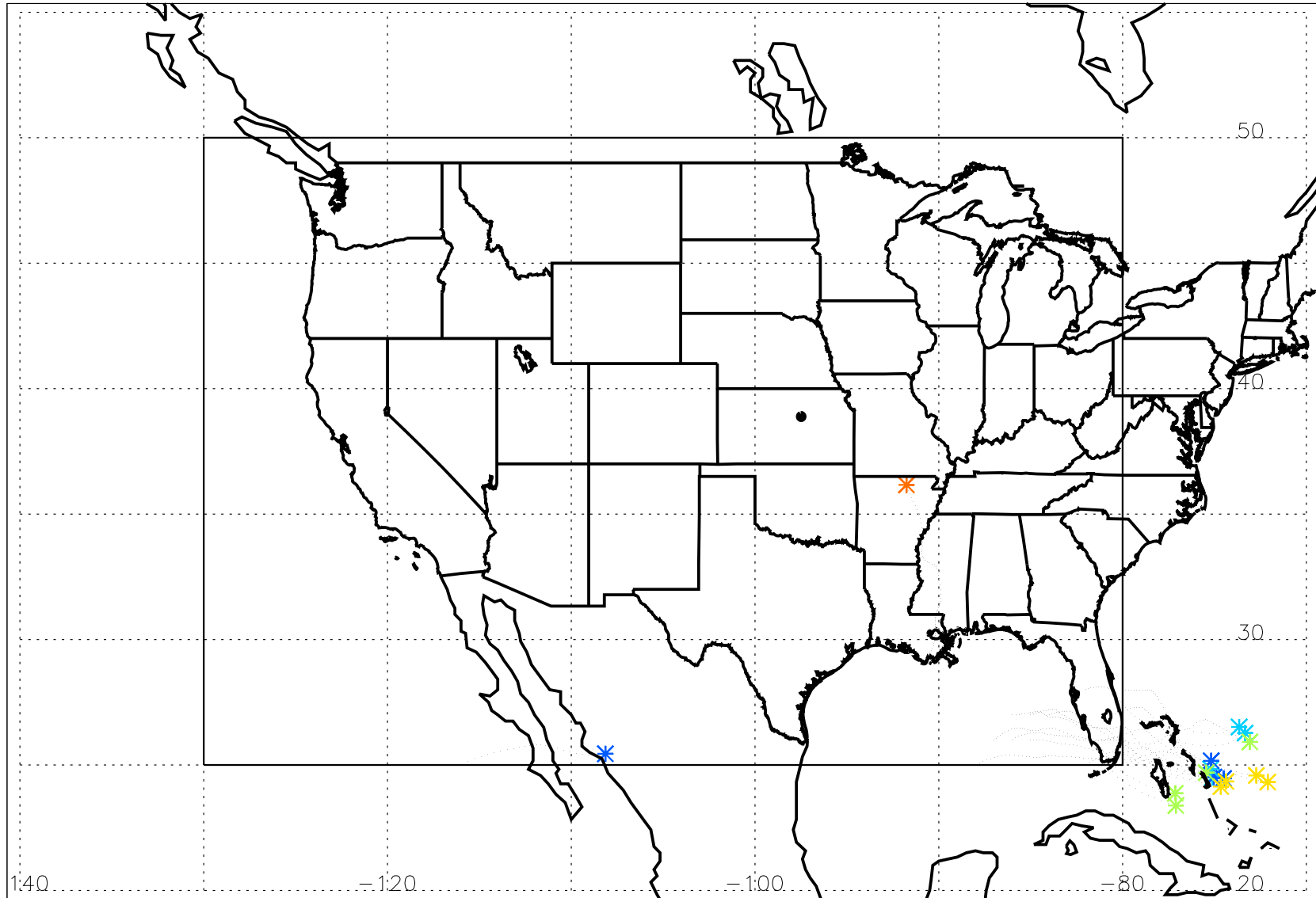
Convectively-influenced 7-day back trajectory at 58 kft level from boxed region on 08/03/2021, 18Z Fig. 3: Trajectories influenced by most recent convection (asterisks) between 0 and 3.5 days (As Fig. 2 but convection locations only)
