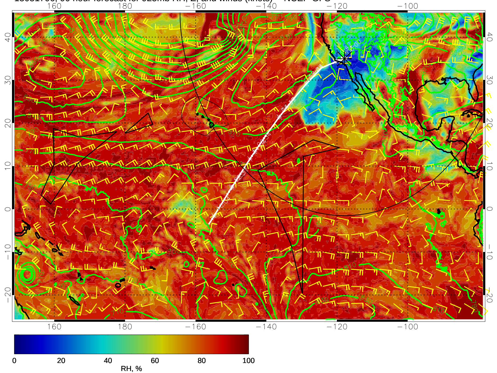
15031706, 90 hour forecast for 925mb RH, Z, and winds (knots) -- NCEP GFS
