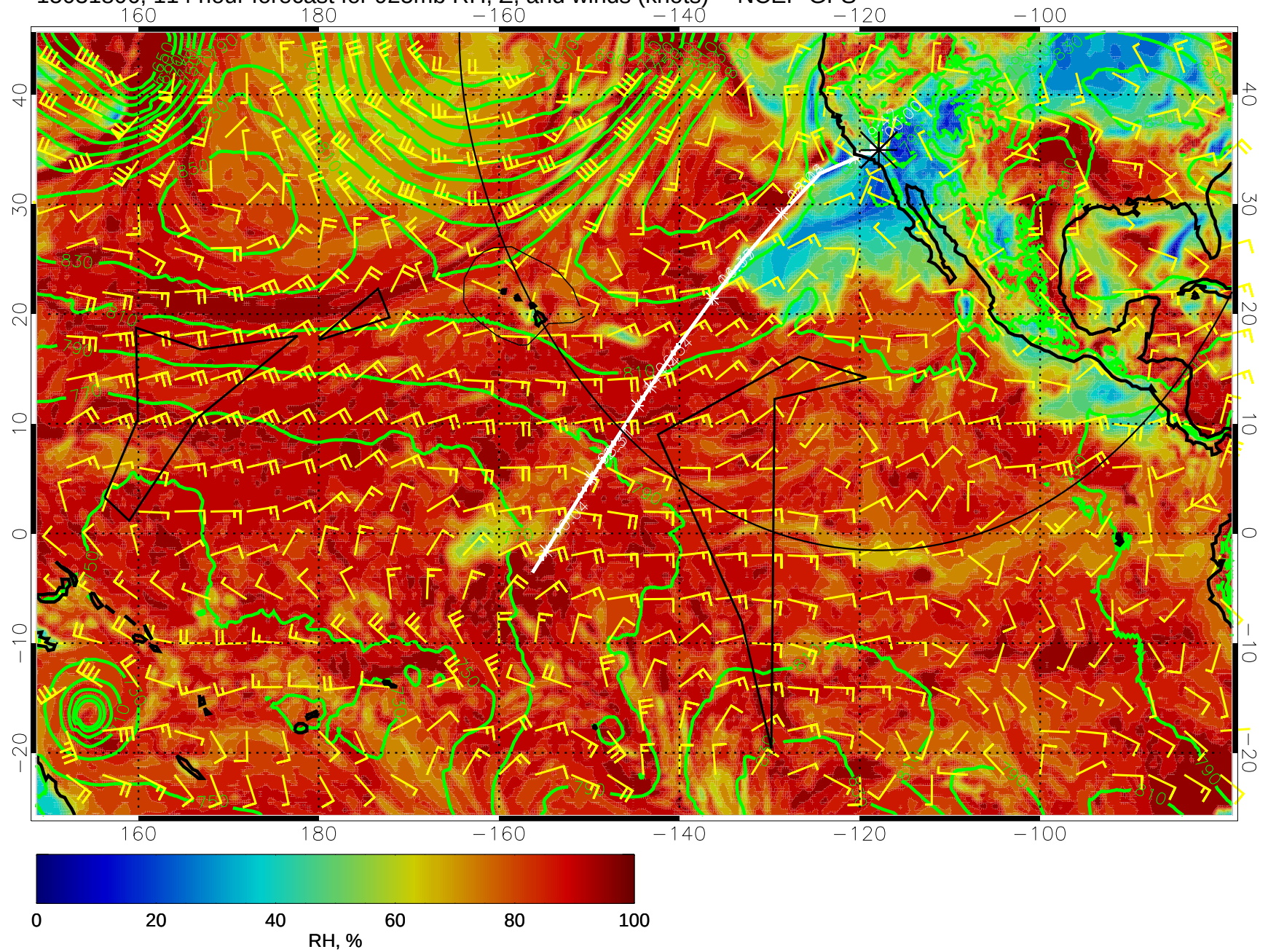
15031806, 114 hour forecast for 925mb RH, Z, and winds (knots) -- NCEP GFS
