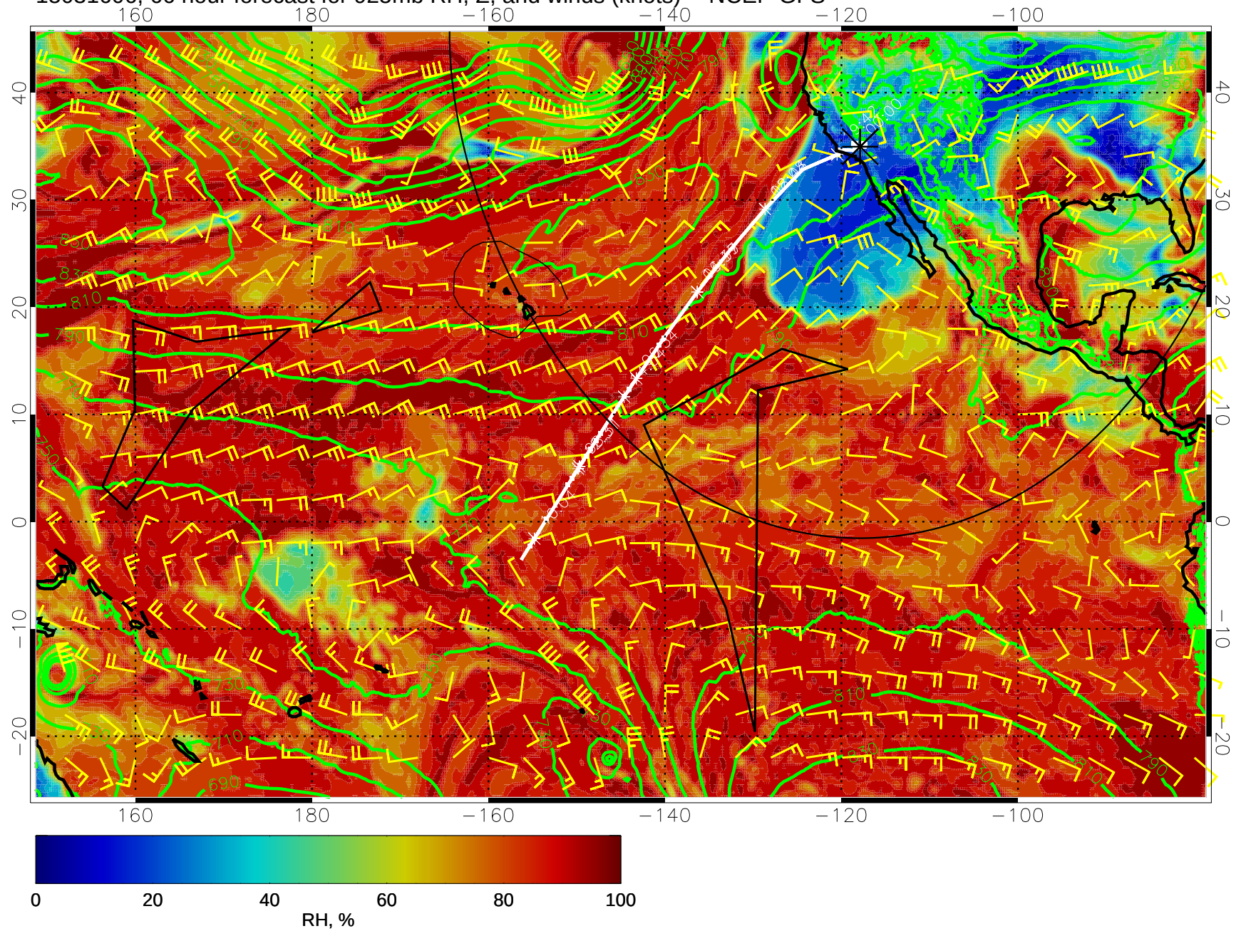
15031606, 66 hour forecast for 925mb RH, Z, and winds (knots) -- NCEP GFS
