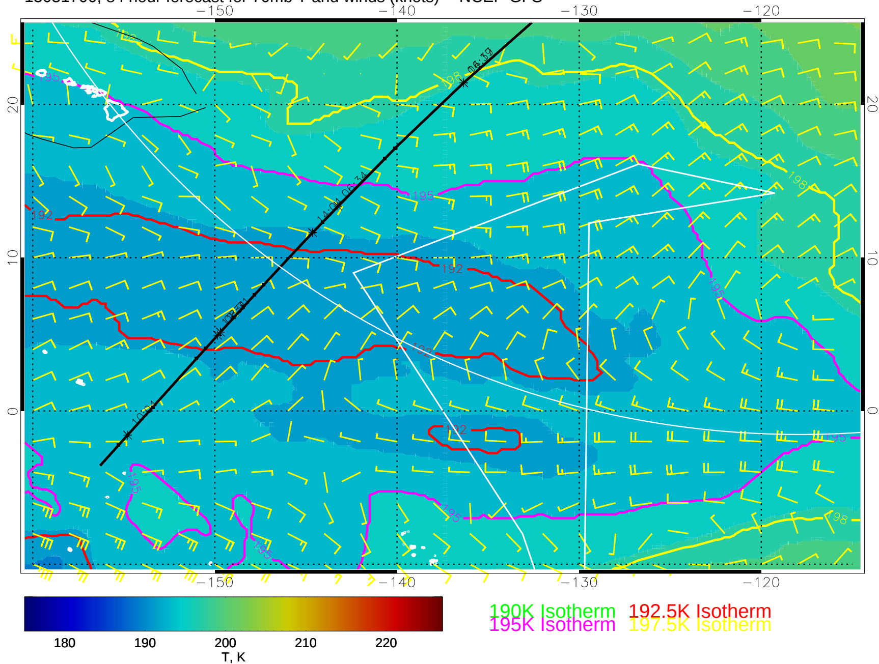
15031700, 84 hour forecast for 70mb T and winds (knots) -- NCEP GFS
