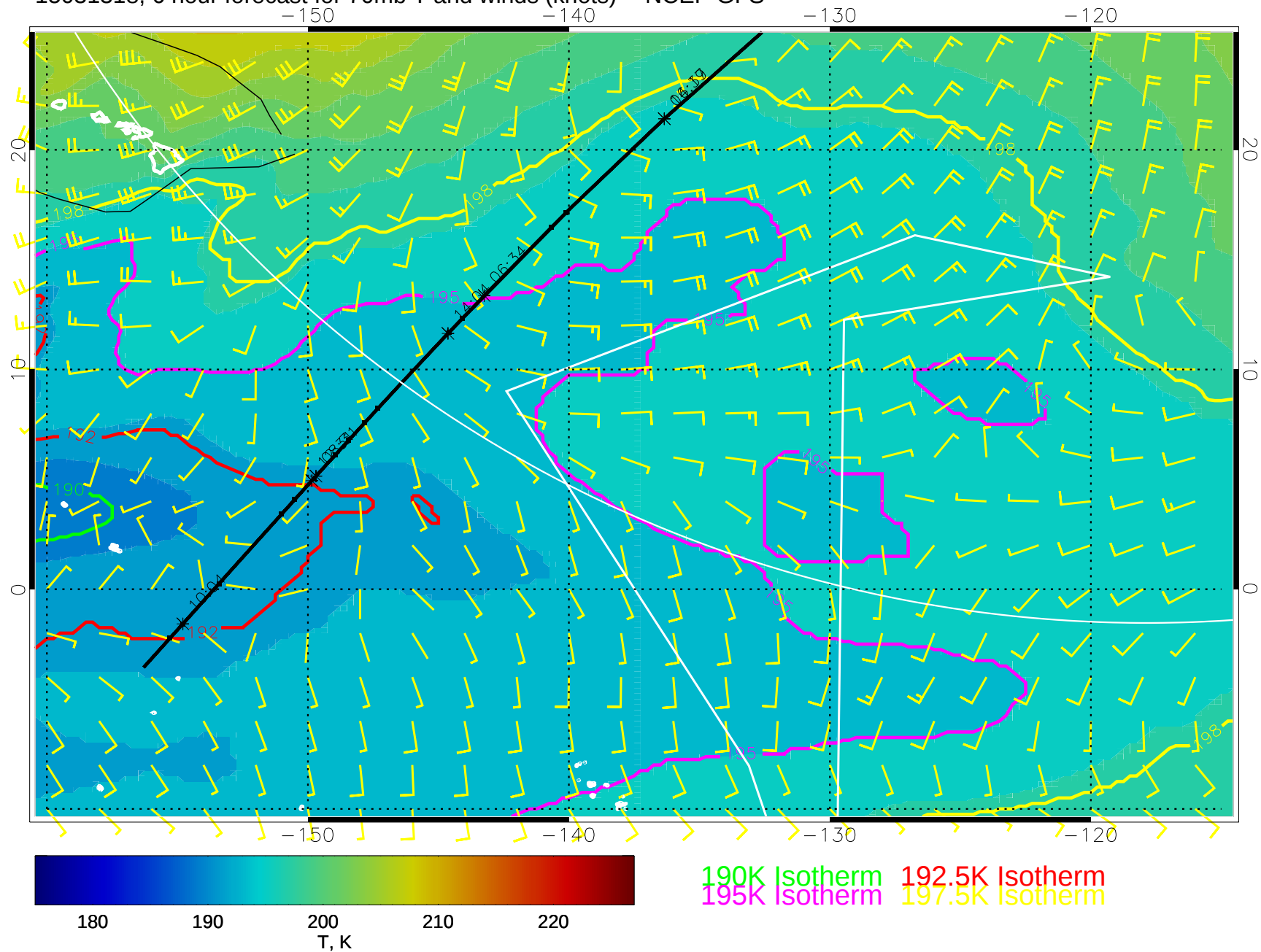
15031318, 6 hour forecast for 70mb T and winds (knots) -- NCEP GFS
