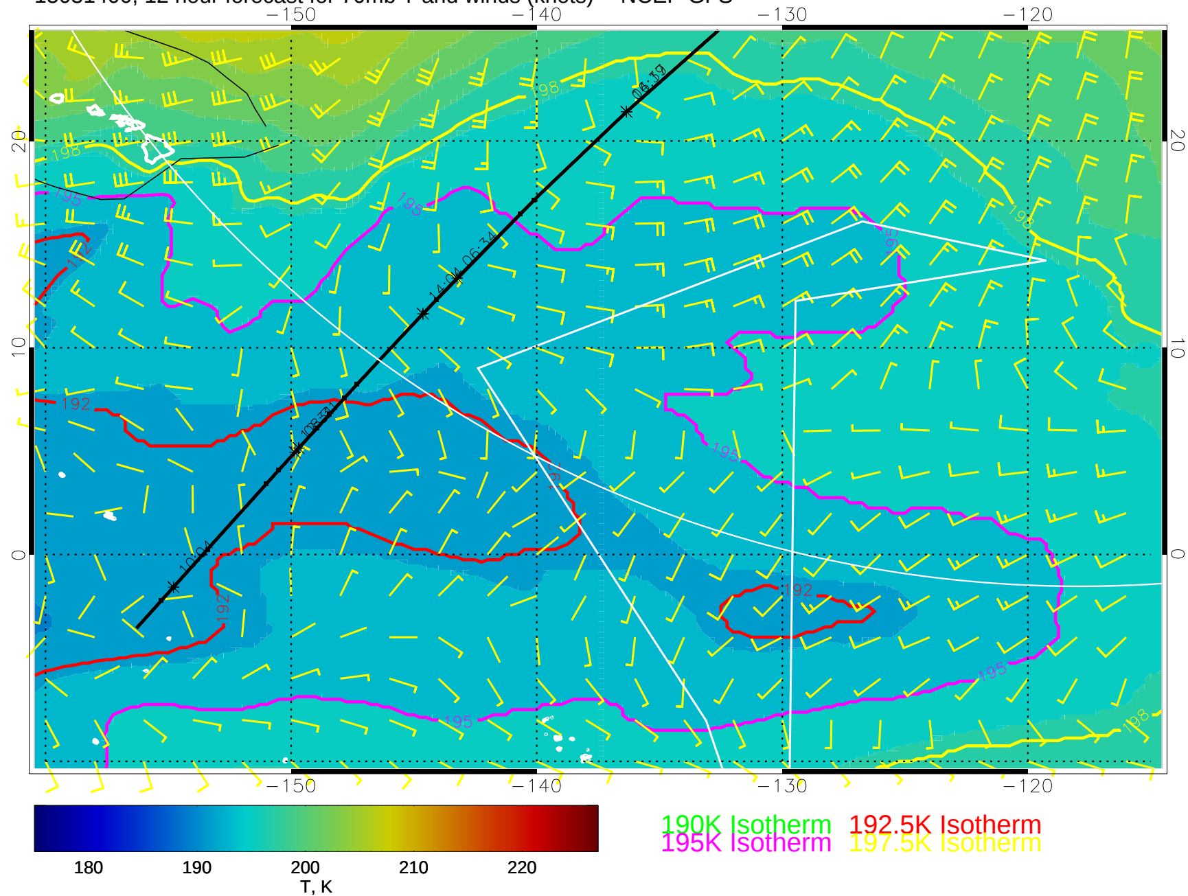
15031400, 12 hour forecast for 70mb T and winds (knots) -- NCEP GFS
