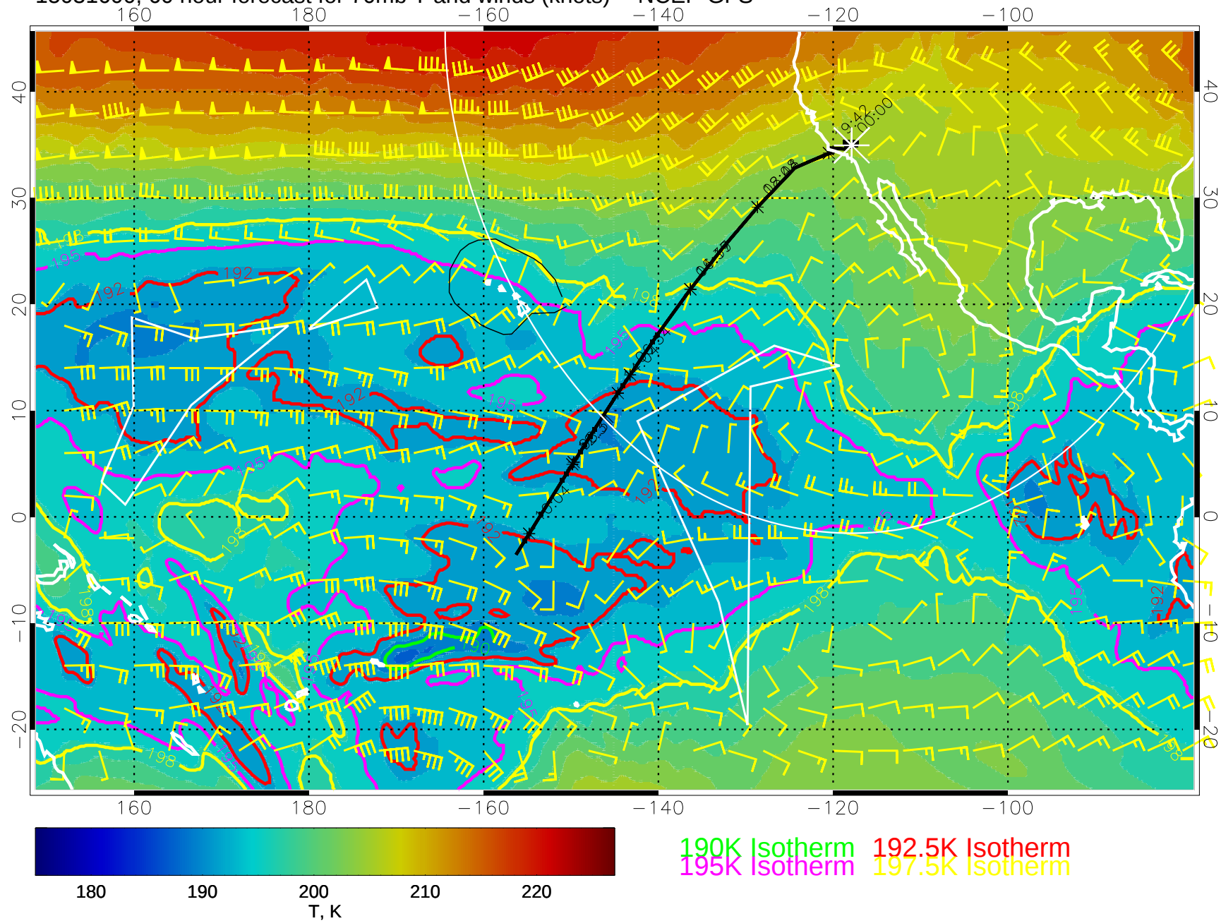
15031600, 60 hour forecast for 70mb T and winds (knots) -- NCEP GFS
