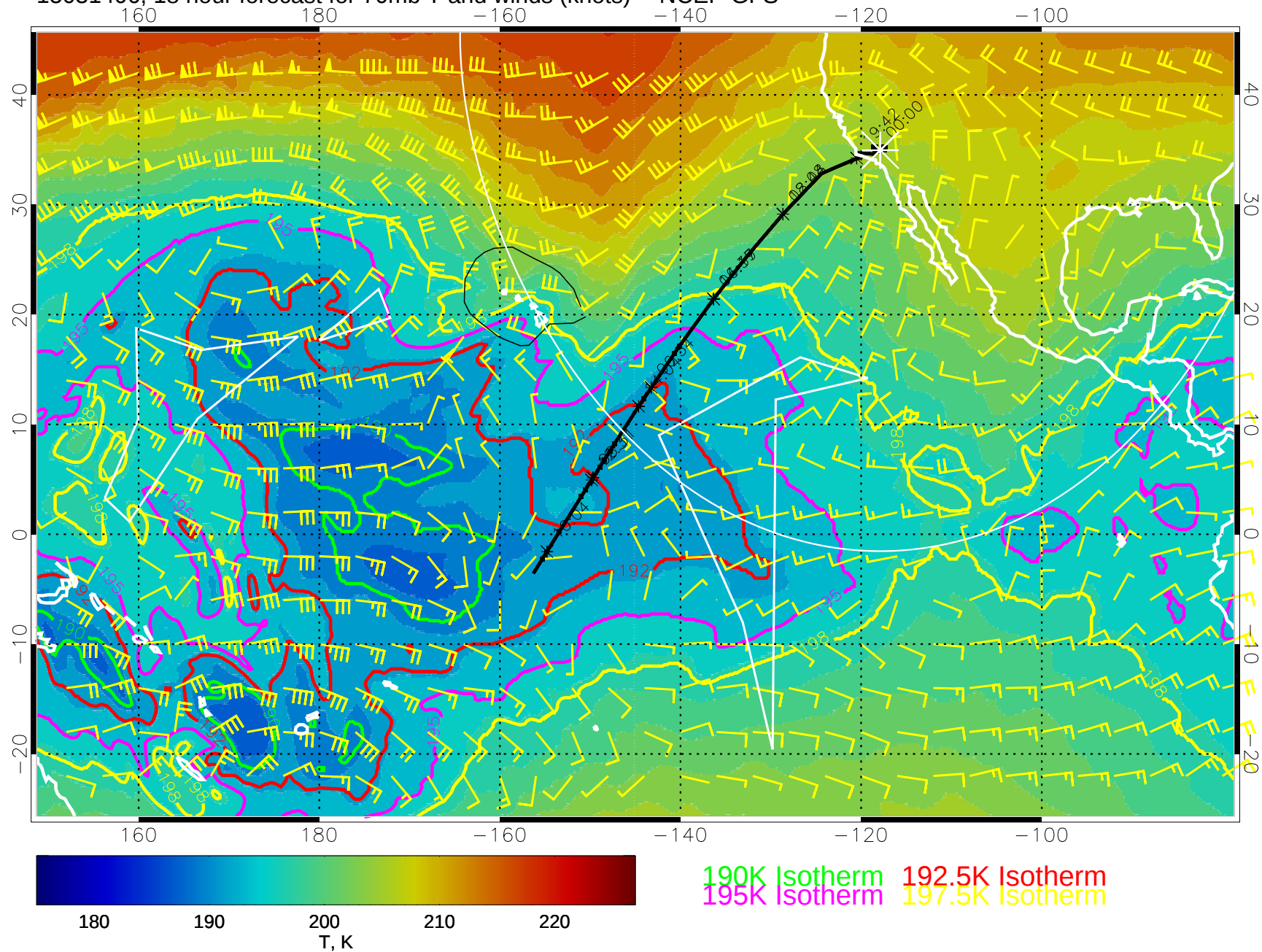
15031406, 18 hour forecast for 70mb T and winds (knots) -- NCEP GFS
