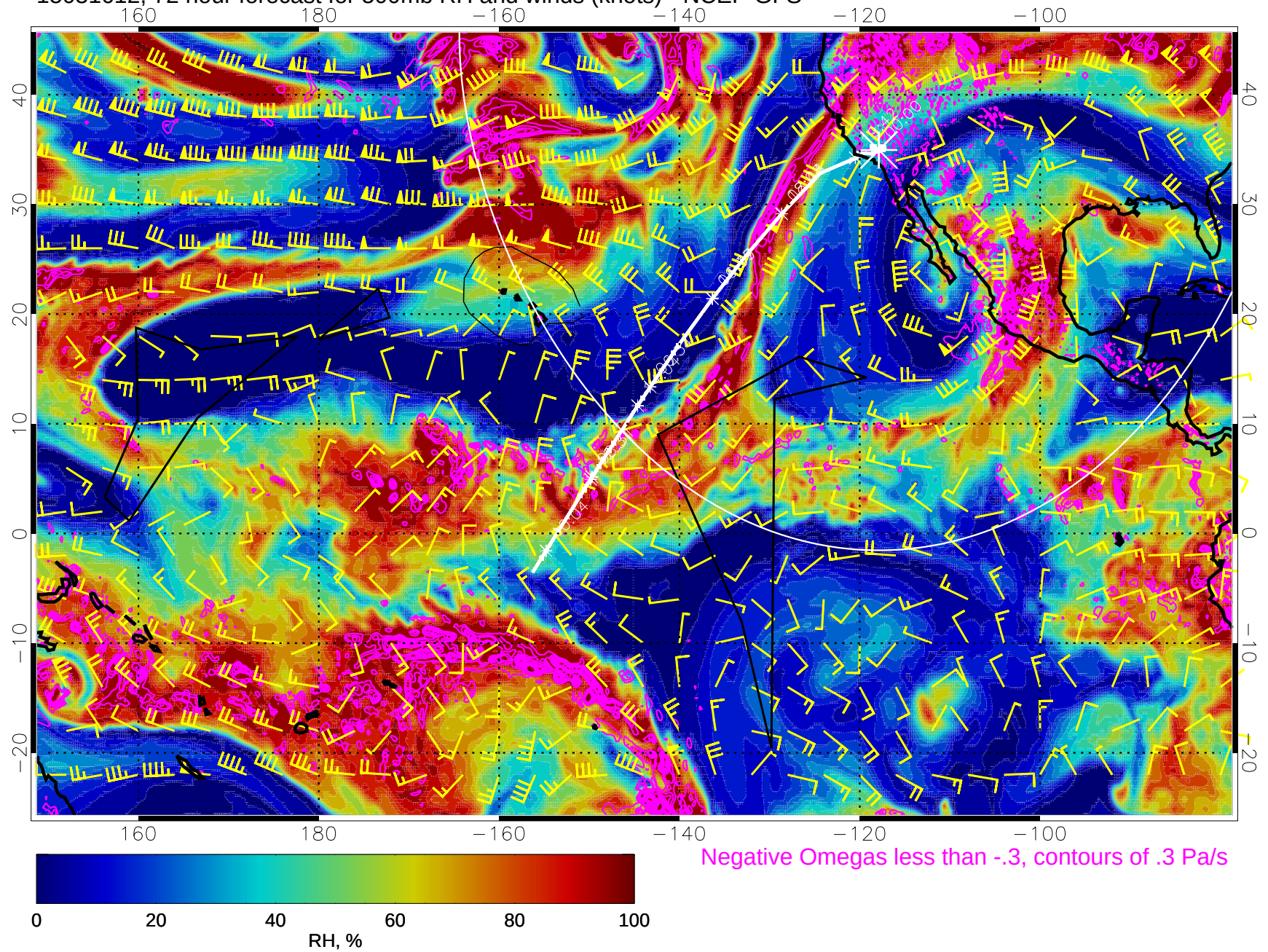
15031612, 72 hour forecast for 500mb RH and winds (knots) - NCEP GFS
