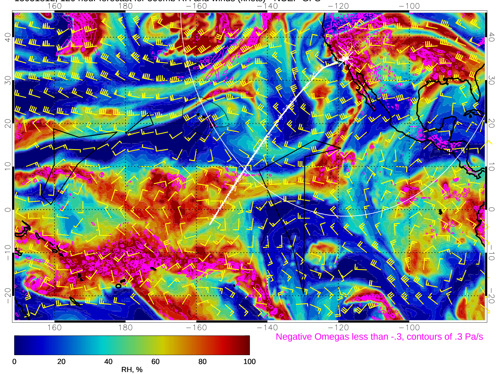
15031812, 120 hour forecast for 500mb RH and winds (knots) - NCEP GFS
