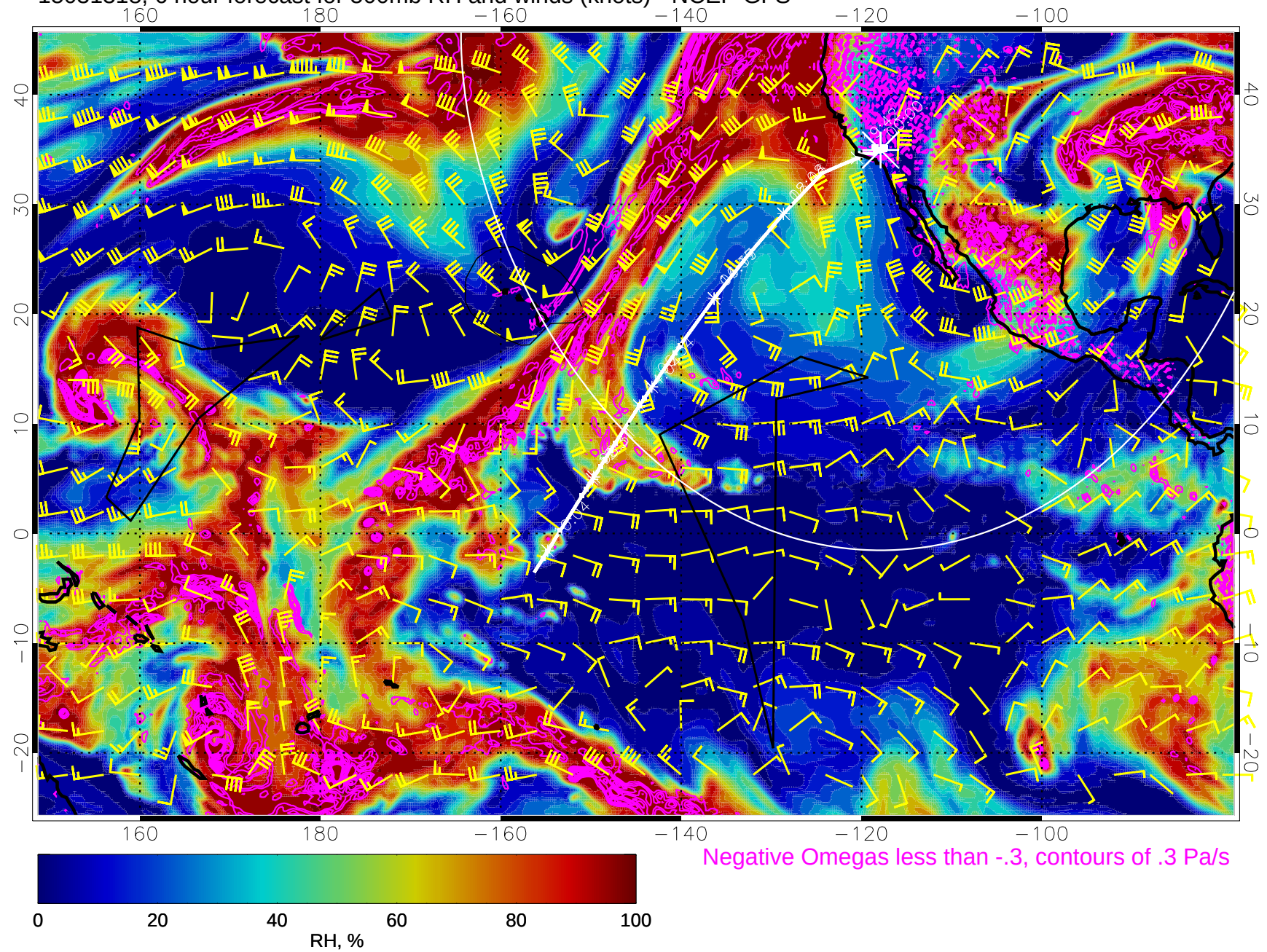
15031318, 6 hour forecast for 500mb RH and winds (knots) - NCEP GFS
