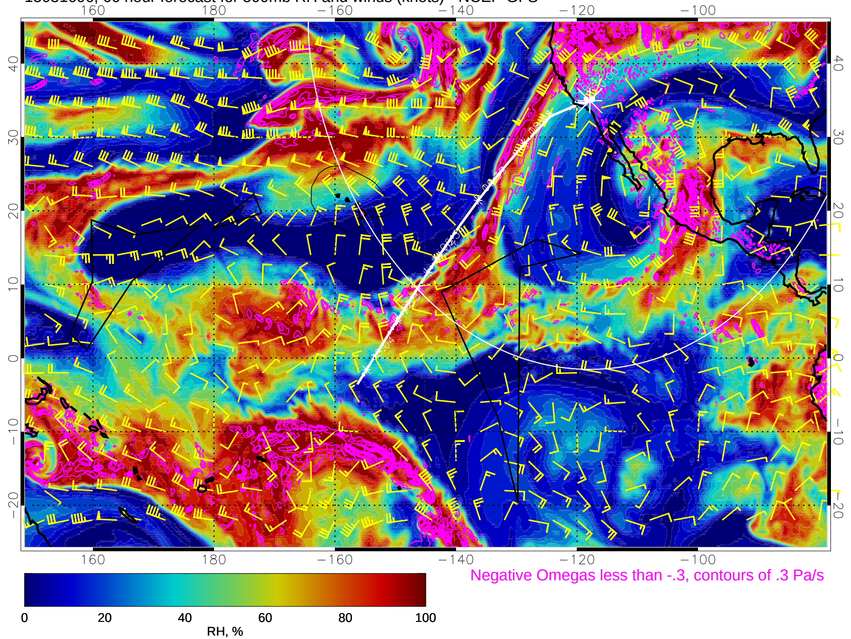
15031606, 66 hour forecast for 500mb RH and winds (knots) - NCEP GFS
