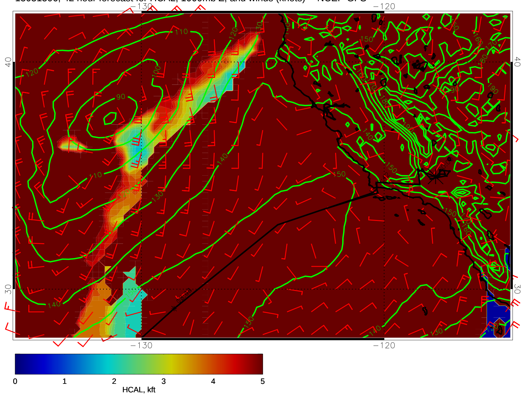
15031506, 42 hour forecast for HCAL, 1000mb Z, and winds (knots) -- NCEP GFS
