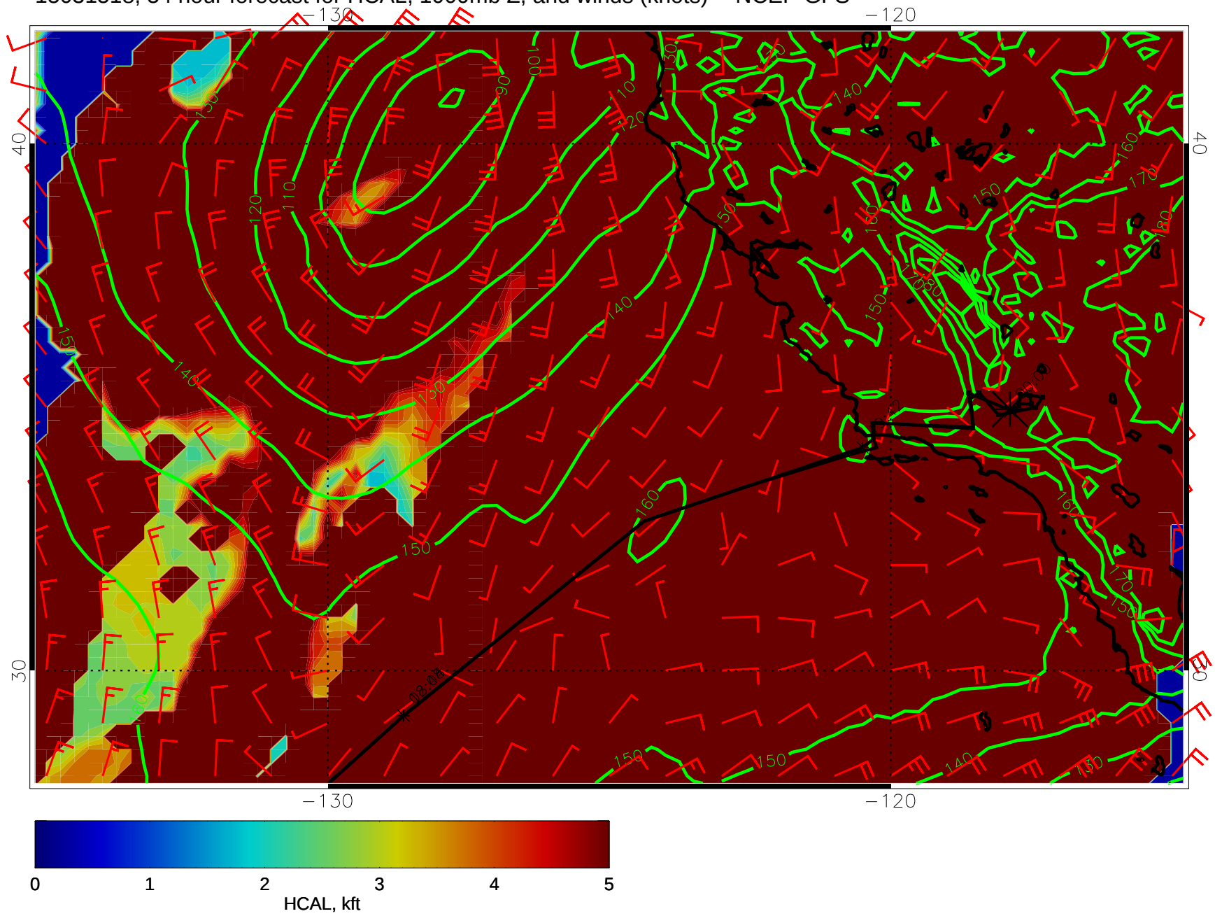
15031518, 54 hour forecast for HCAL, 1000mb Z, and winds (knots) -- NCEP GFS
