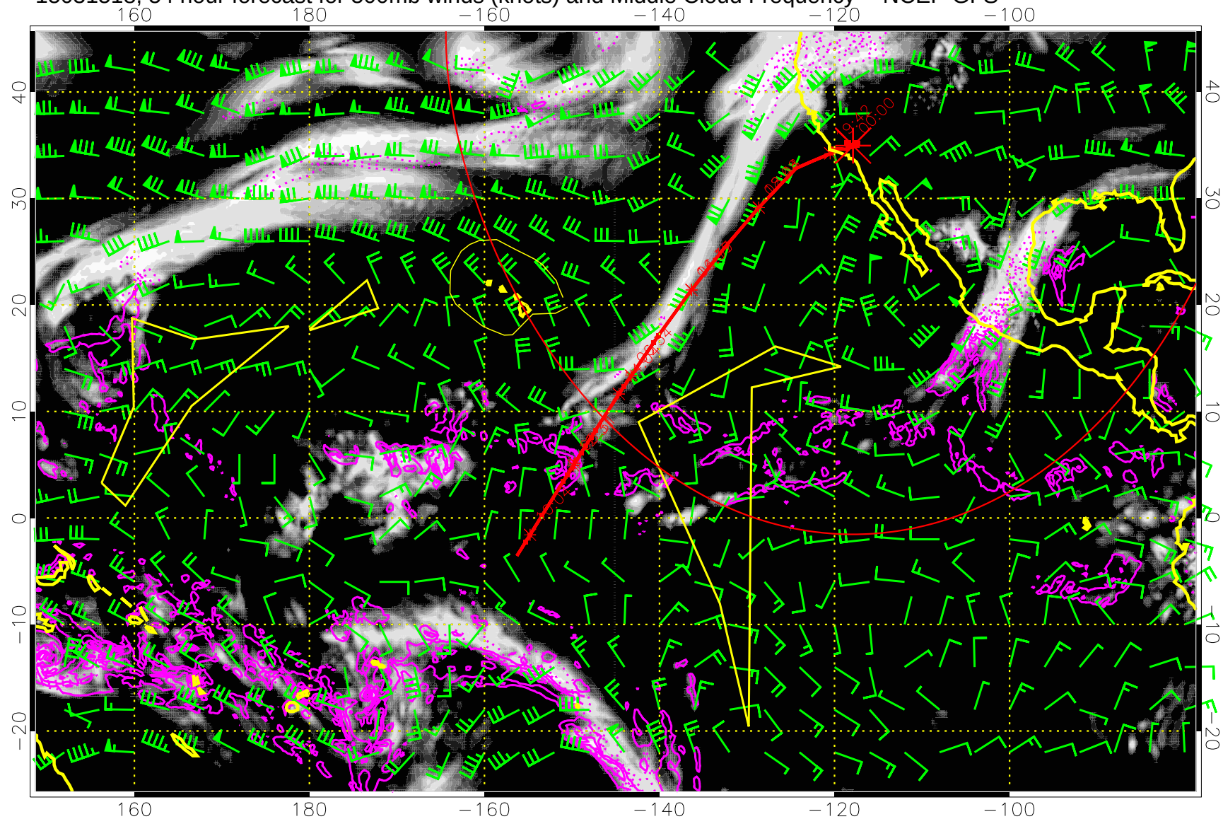
15031518, 54 hour forecast for 500mb winds (knots) and Middle Cloud Frequency -- NCEP GFS
