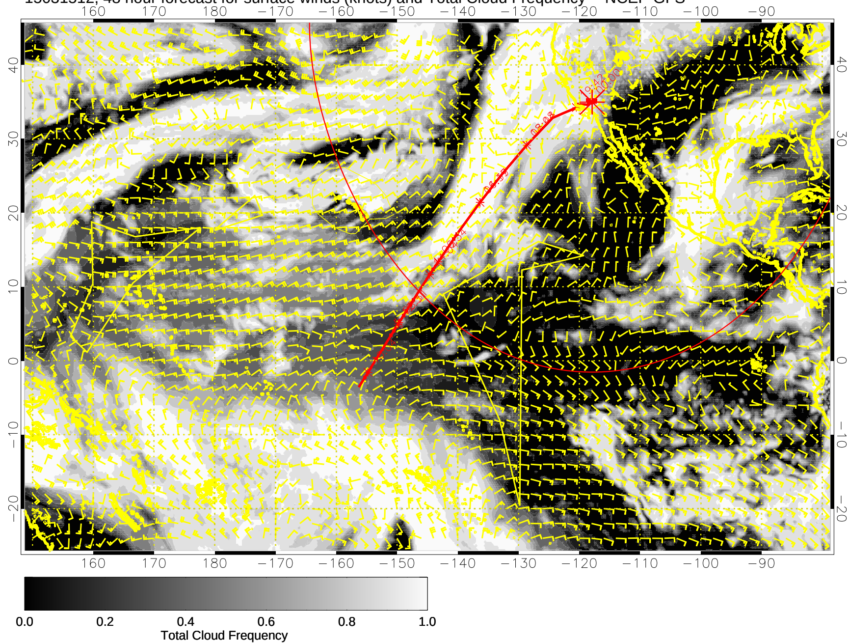
15031512, 48 hour forecast for surface winds (knots) and Total Cloud Frequency -- NCEP GFS
