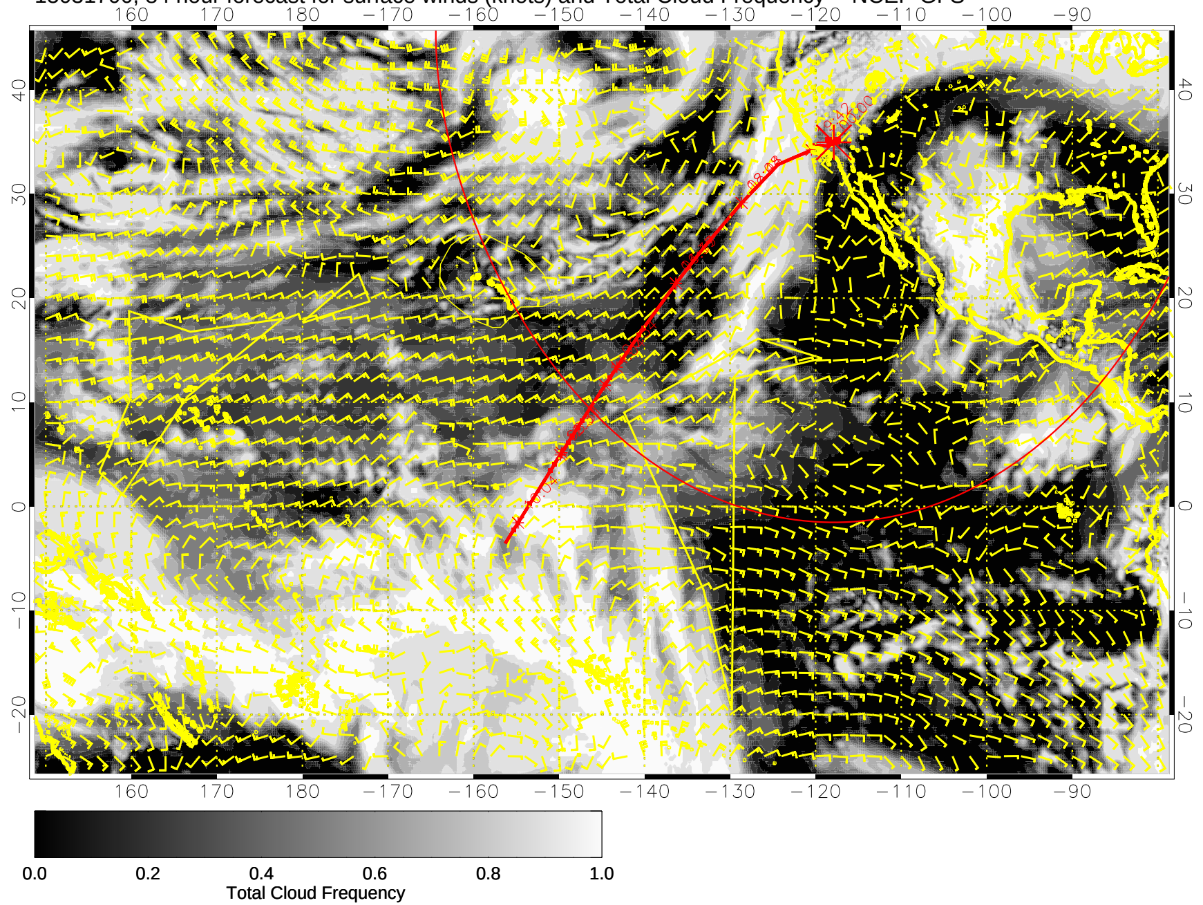
15031700, 84 hour forecast for surface winds (knots) and Total Cloud Frequency -- NCEP GFS
