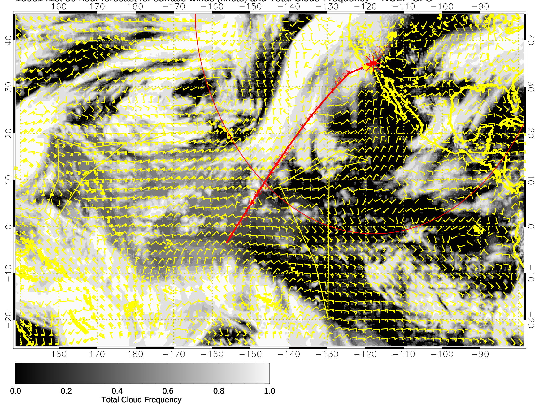
15031418, 30 hour forecast for surface winds (knots) and Total Cloud Frequency -- NCEP GFS
