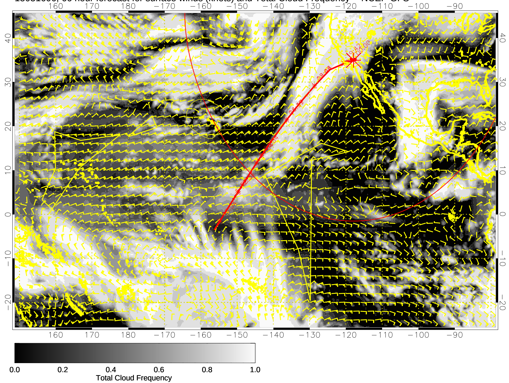
15031606, 66 hour forecast for surface winds (knots) and Total Cloud Frequency -- NCEP GFS
