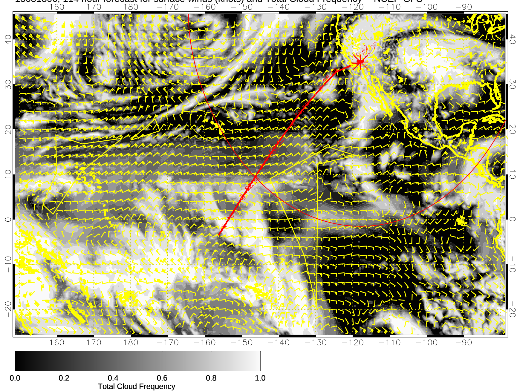
15031806, 114 hour forecast for surface winds (knots) and Total Cloud Frequency -- NCEP GFS
