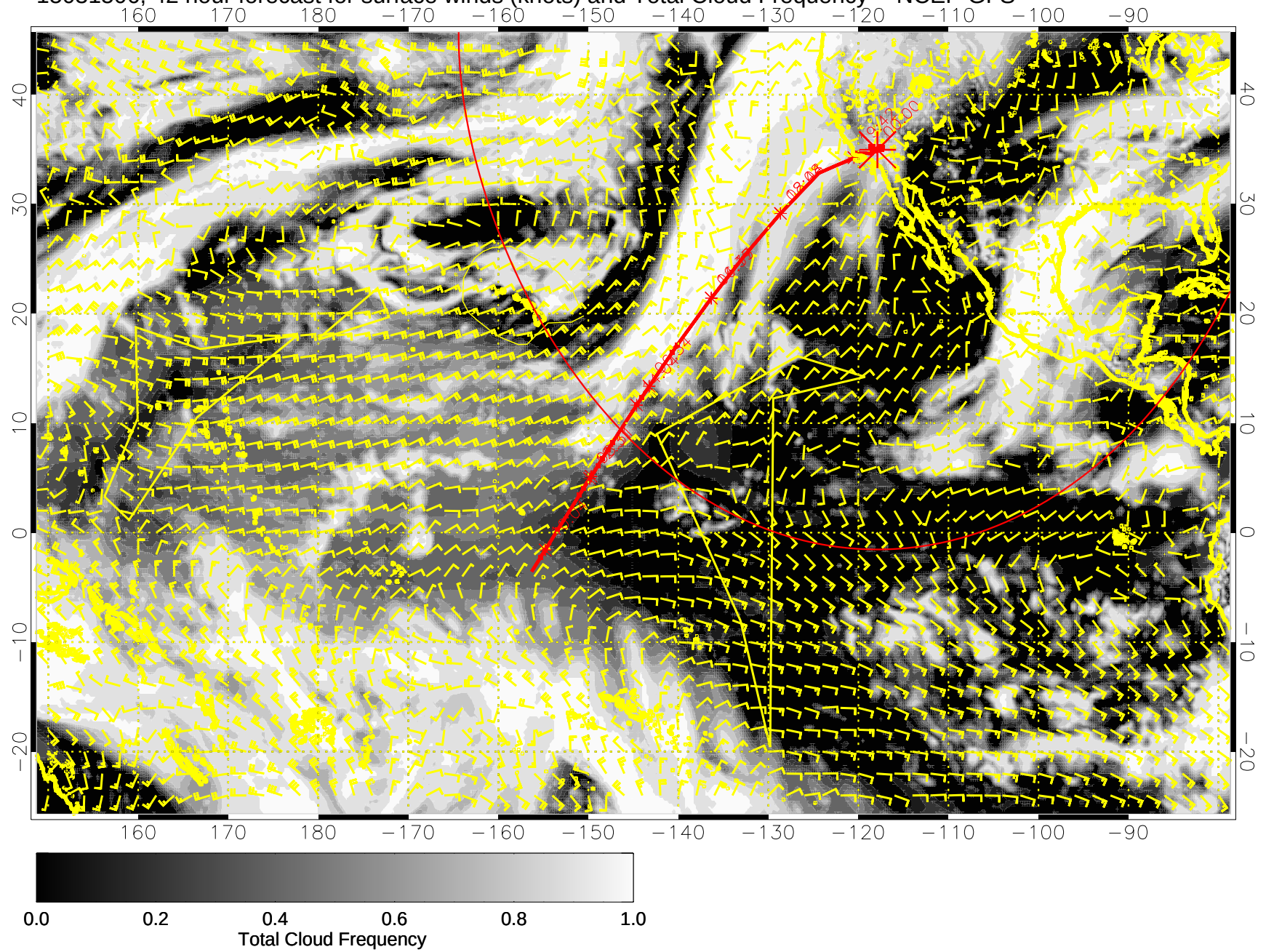
15031506, 42 hour forecast for surface winds (knots) and Total Cloud Frequency -- NCEP GFS
