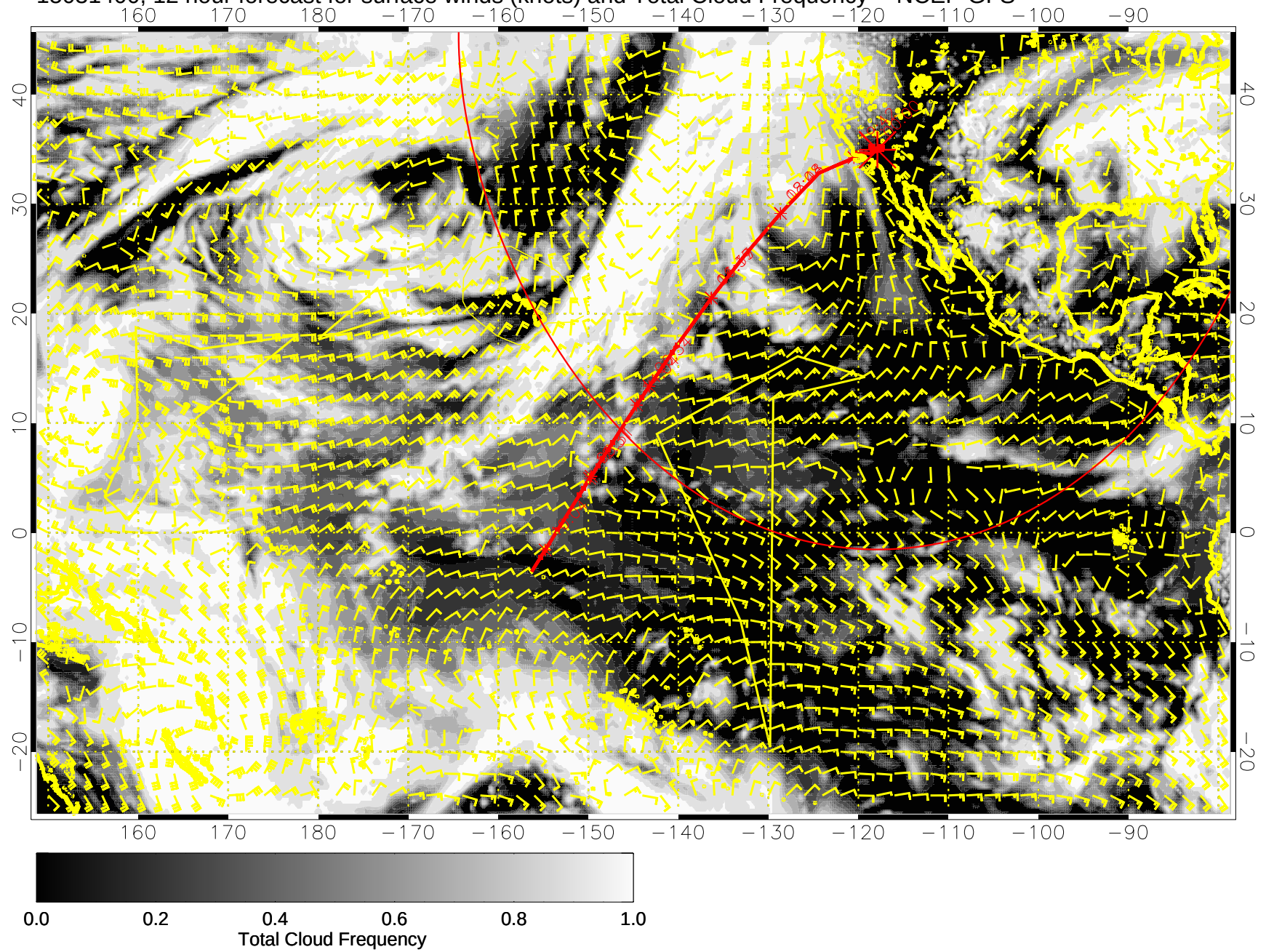
15031400, 12 hour forecast for surface winds (knots) and Total Cloud Frequency -- NCEP GFS
