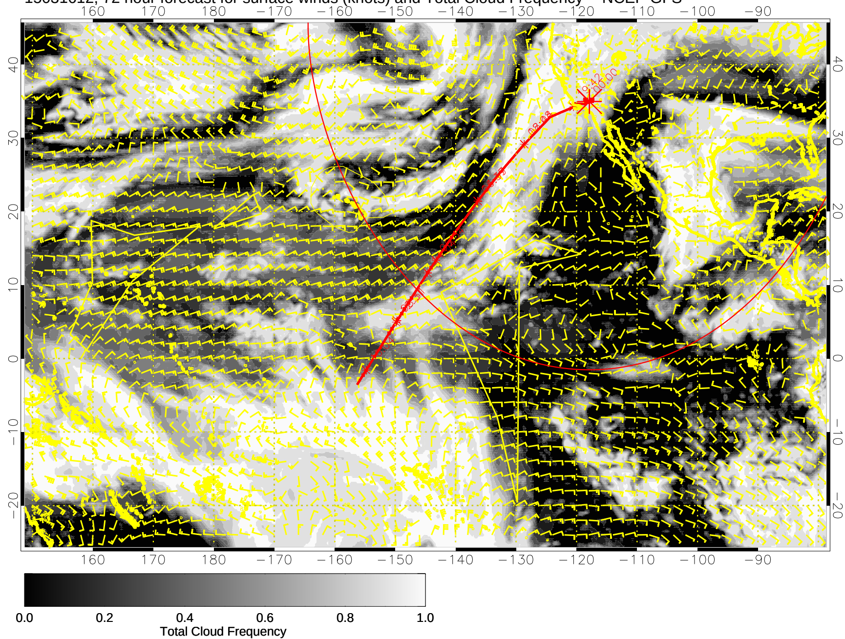
15031612, 72 hour forecast for surface winds (knots) and Total Cloud Frequency -- NCEP GFS
