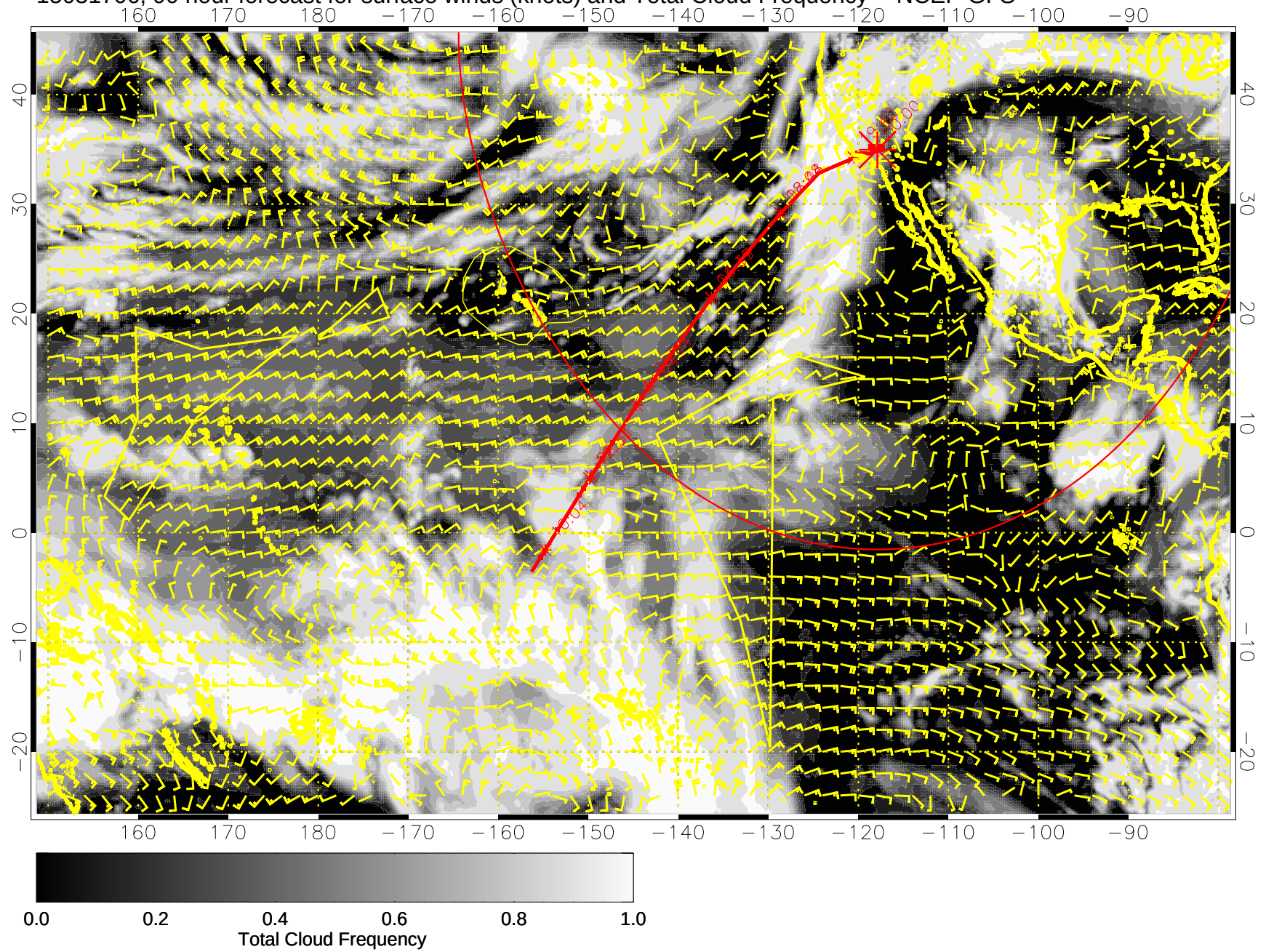
15031706, 90 hour forecast for surface winds (knots) and Total Cloud Frequency -- NCEP GFS
