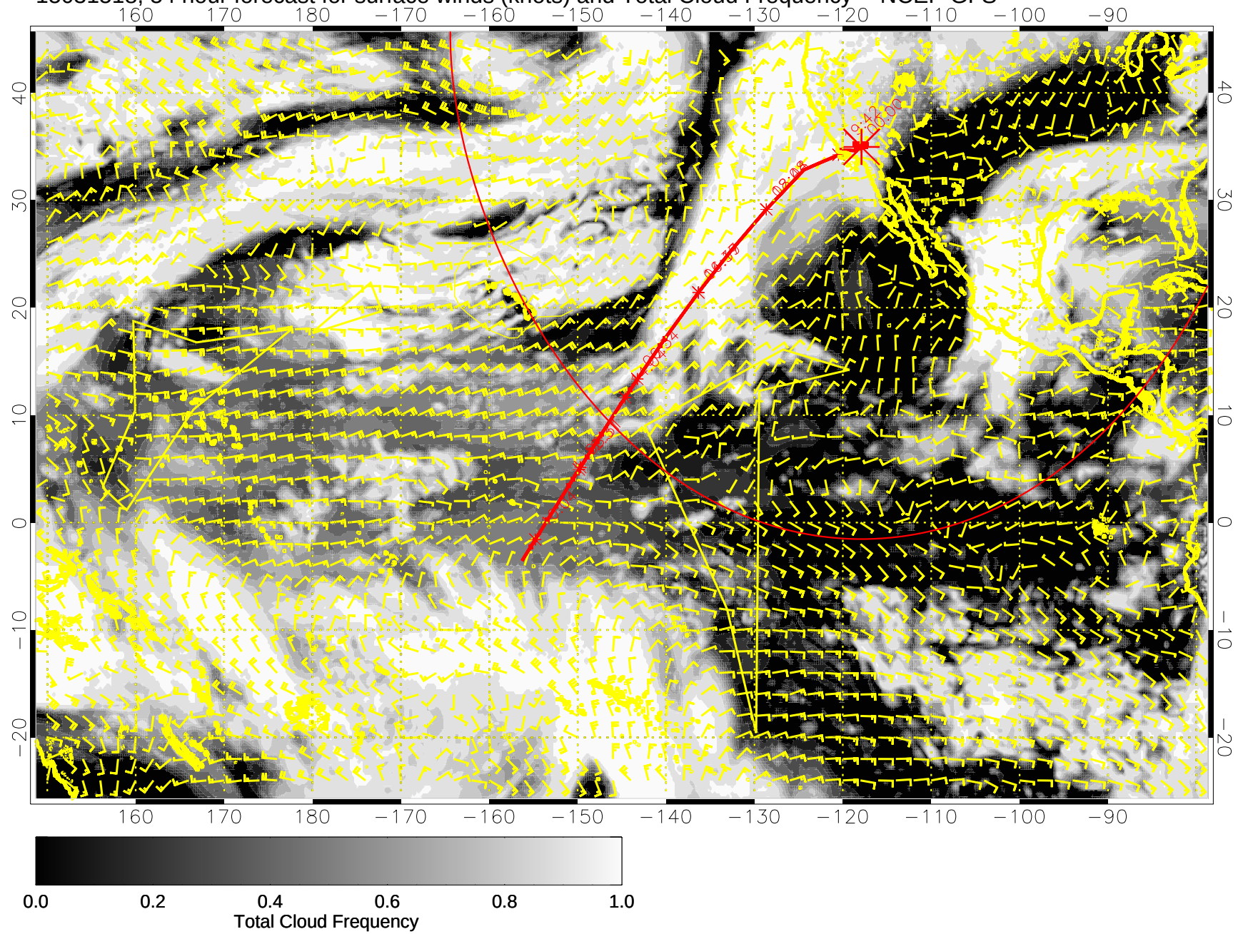
15031518, 54 hour forecast for surface winds (knots) and Total Cloud Frequency -- NCEP GFS
