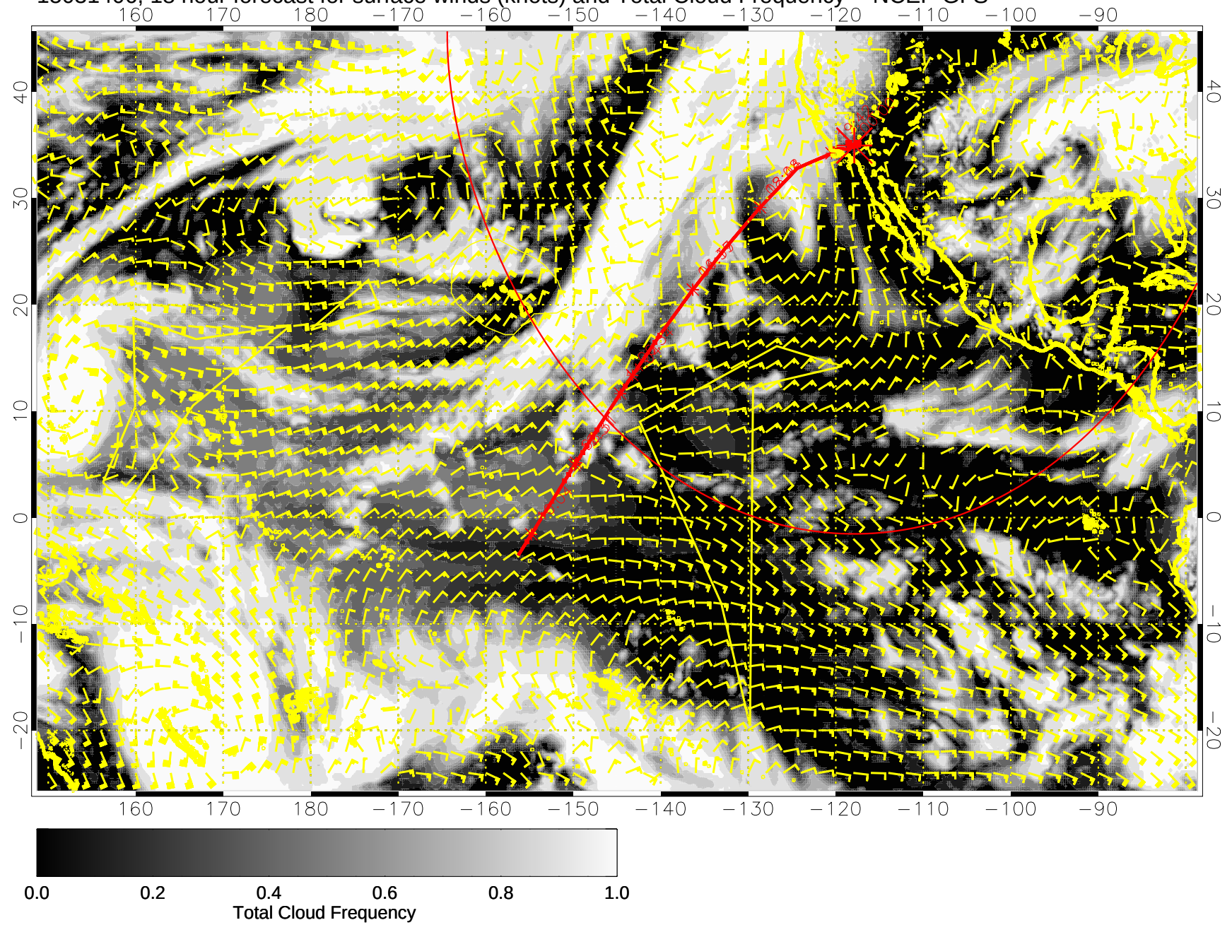
15031406, 18 hour forecast for surface winds (knots) and Total Cloud Frequency -- NCEP GFS
