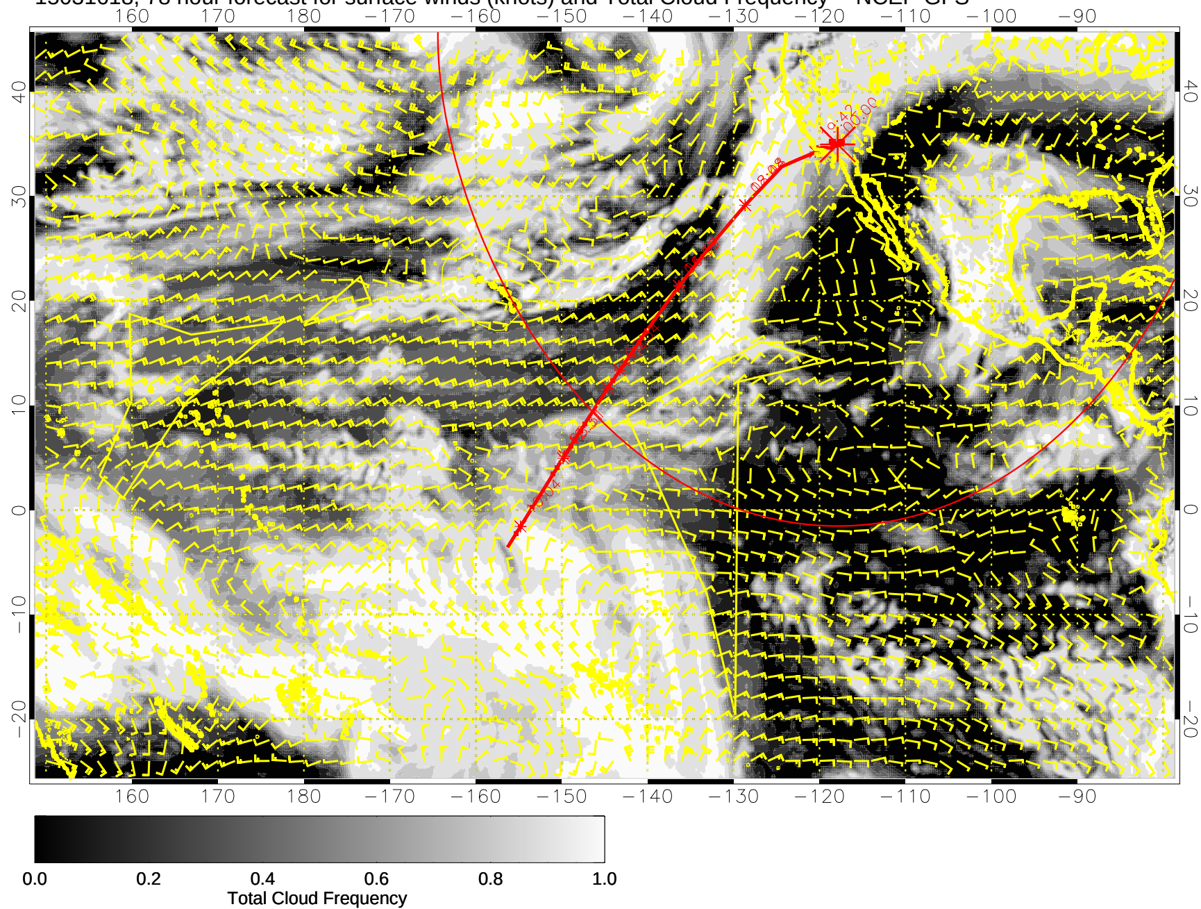
15031618, 78 hour forecast for surface winds (knots) and Total Cloud Frequency -- NCEP GFS
