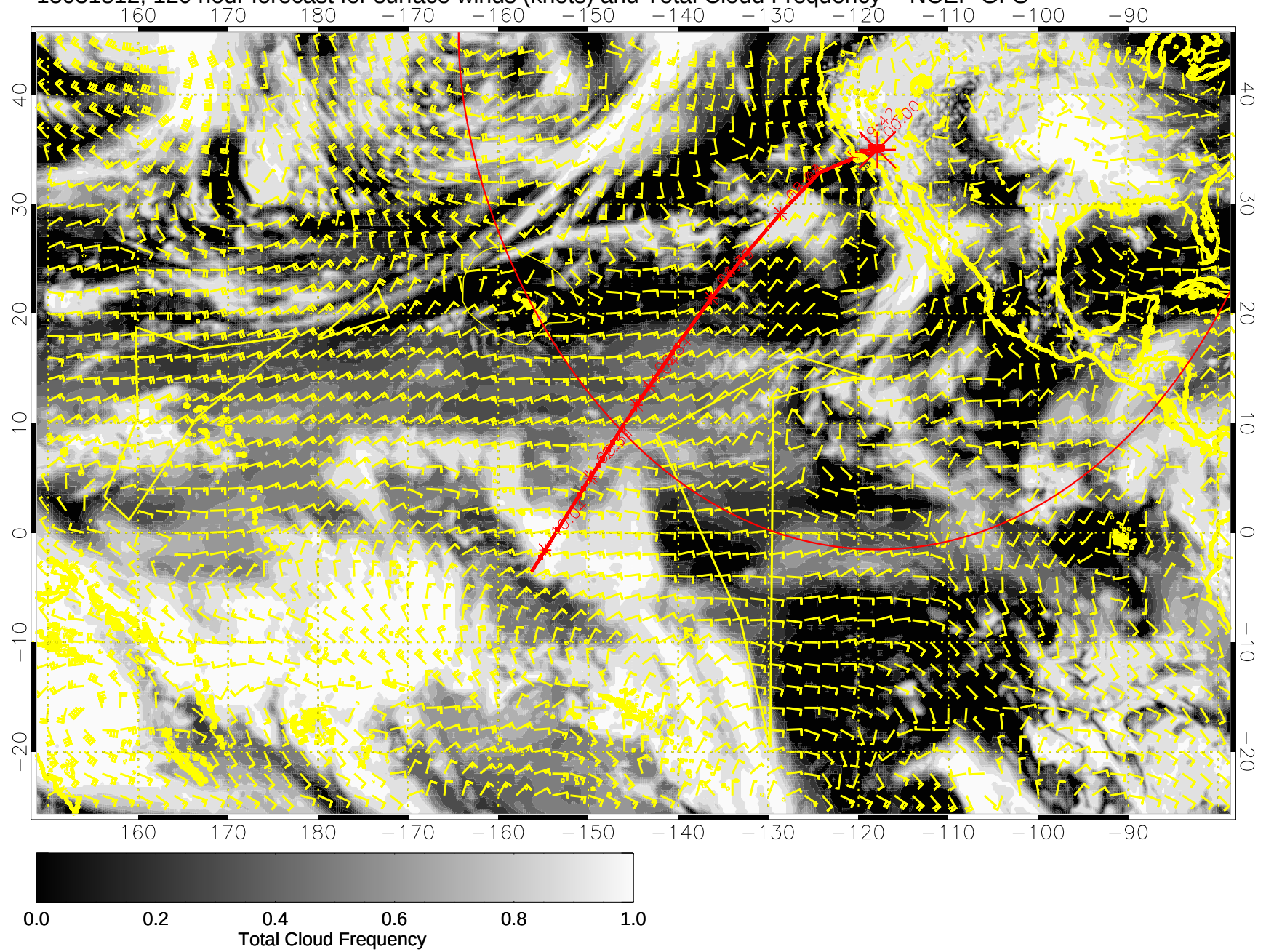
15031812, 120 hour forecast for surface winds (knots) and Total Cloud Frequency -- NCEP GFS
