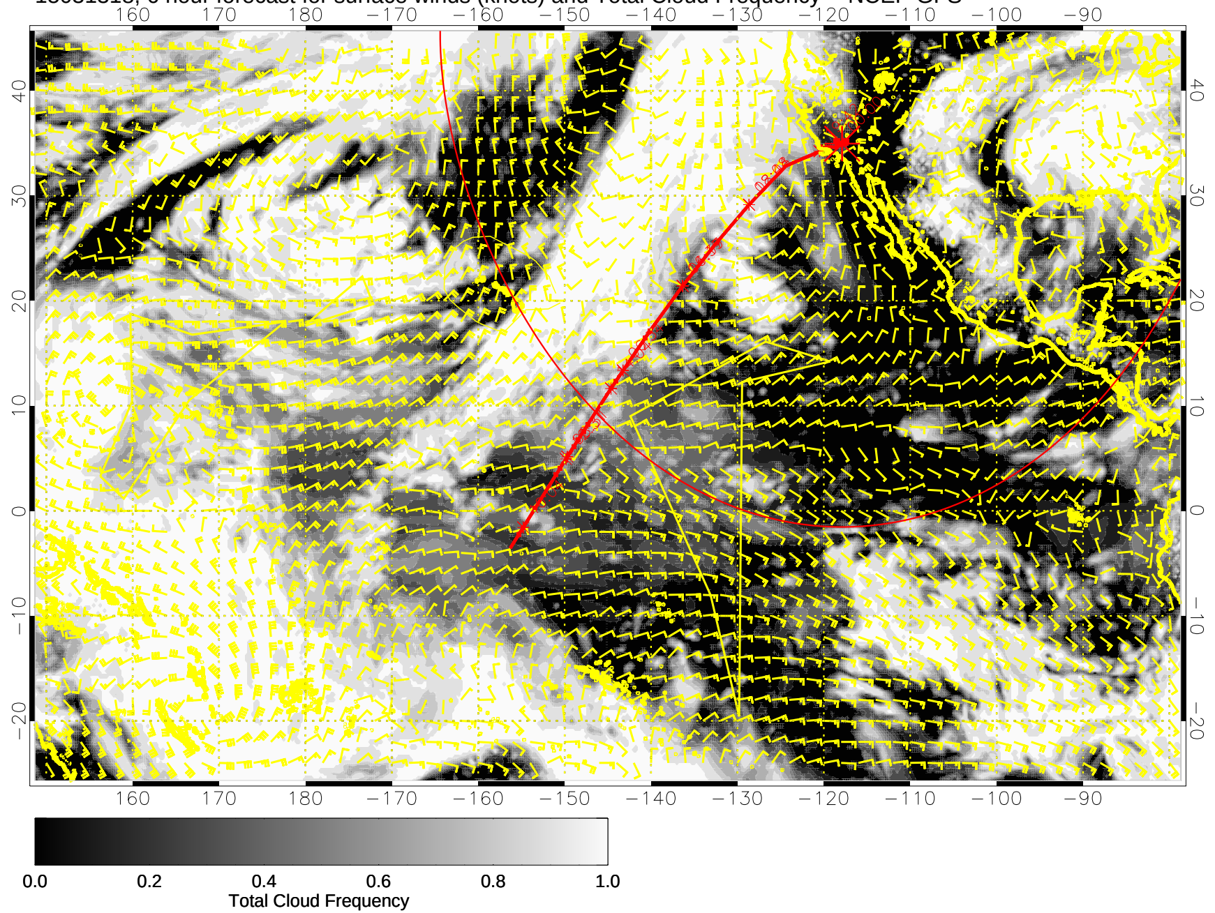
15031318, 6 hour forecast for surface winds (knots) and Total Cloud Frequency -- NCEP GFS
