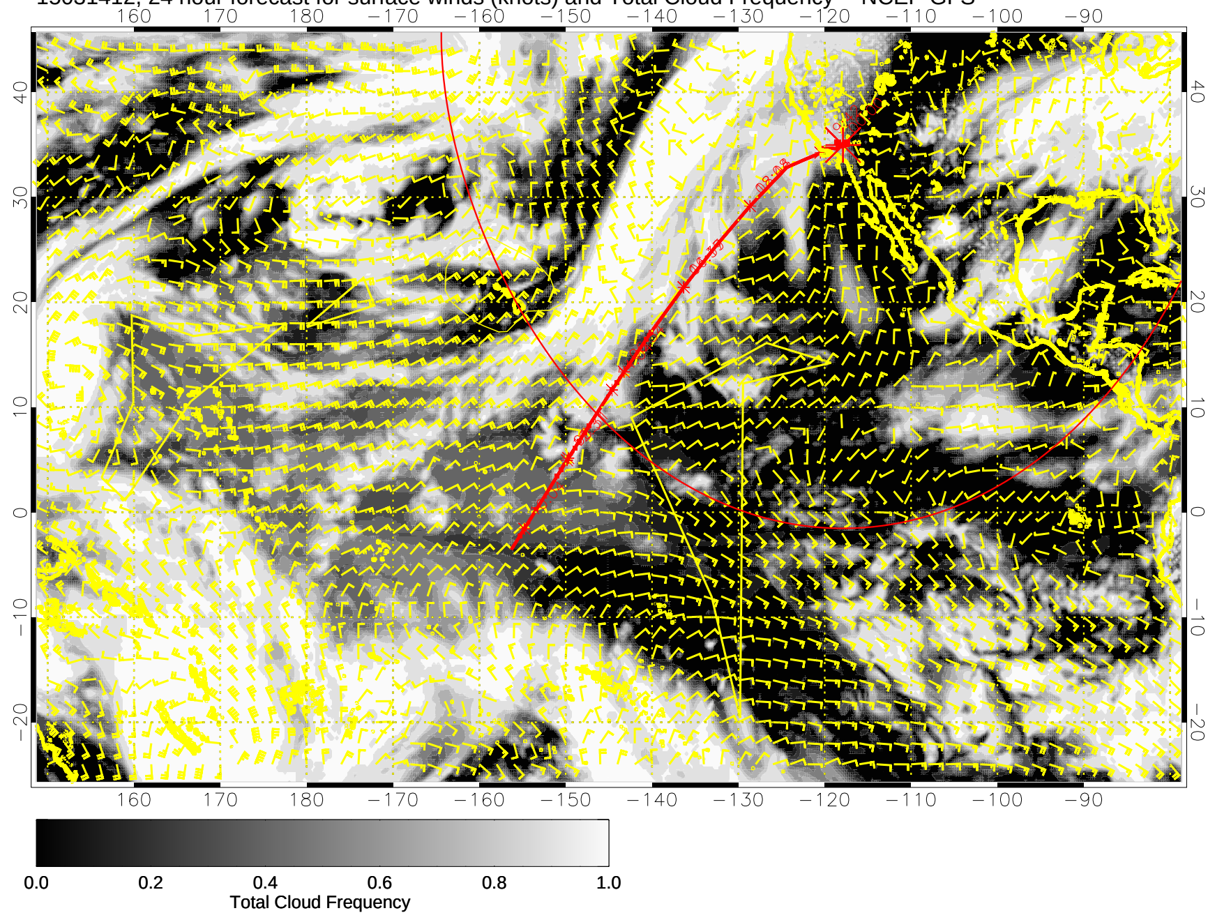
15031412, 24 hour forecast for surface winds (knots) and Total Cloud Frequency -- NCEP GFS
