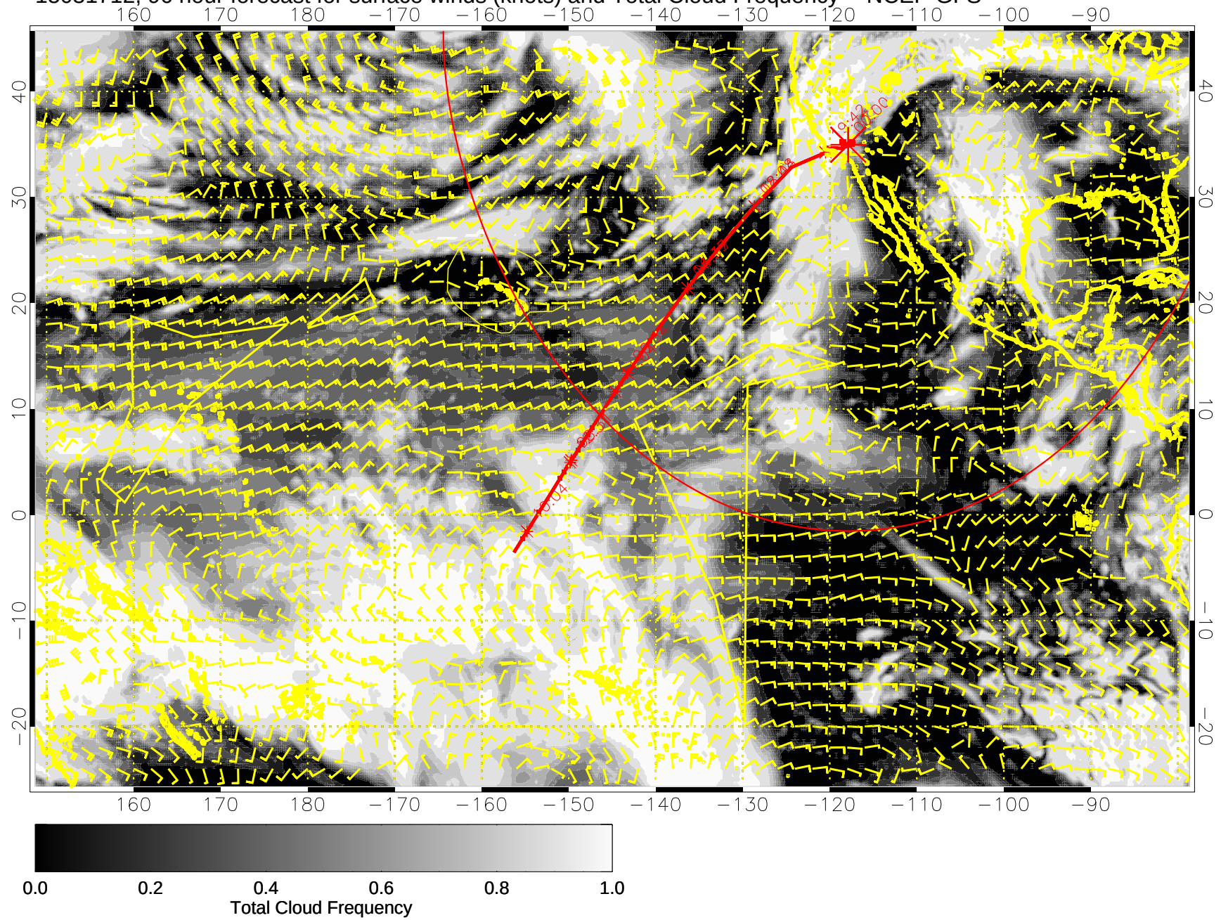
15031712, 96 hour forecast for surface winds (knots) and Total Cloud Frequency -- NCEP GFS
