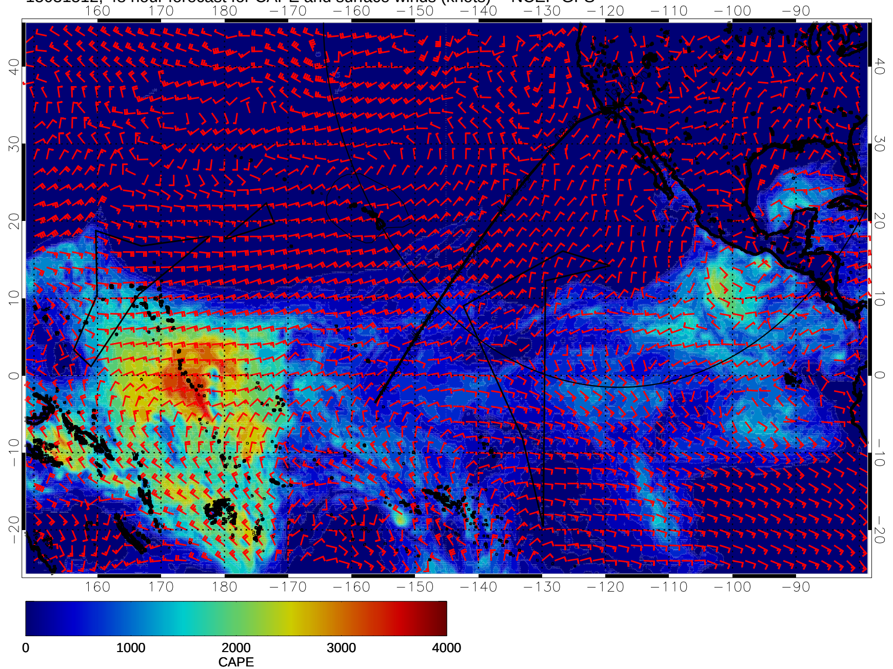
15031512, 48 hour forecast for CAPE and surface winds (knots) -- NCEP GFS
