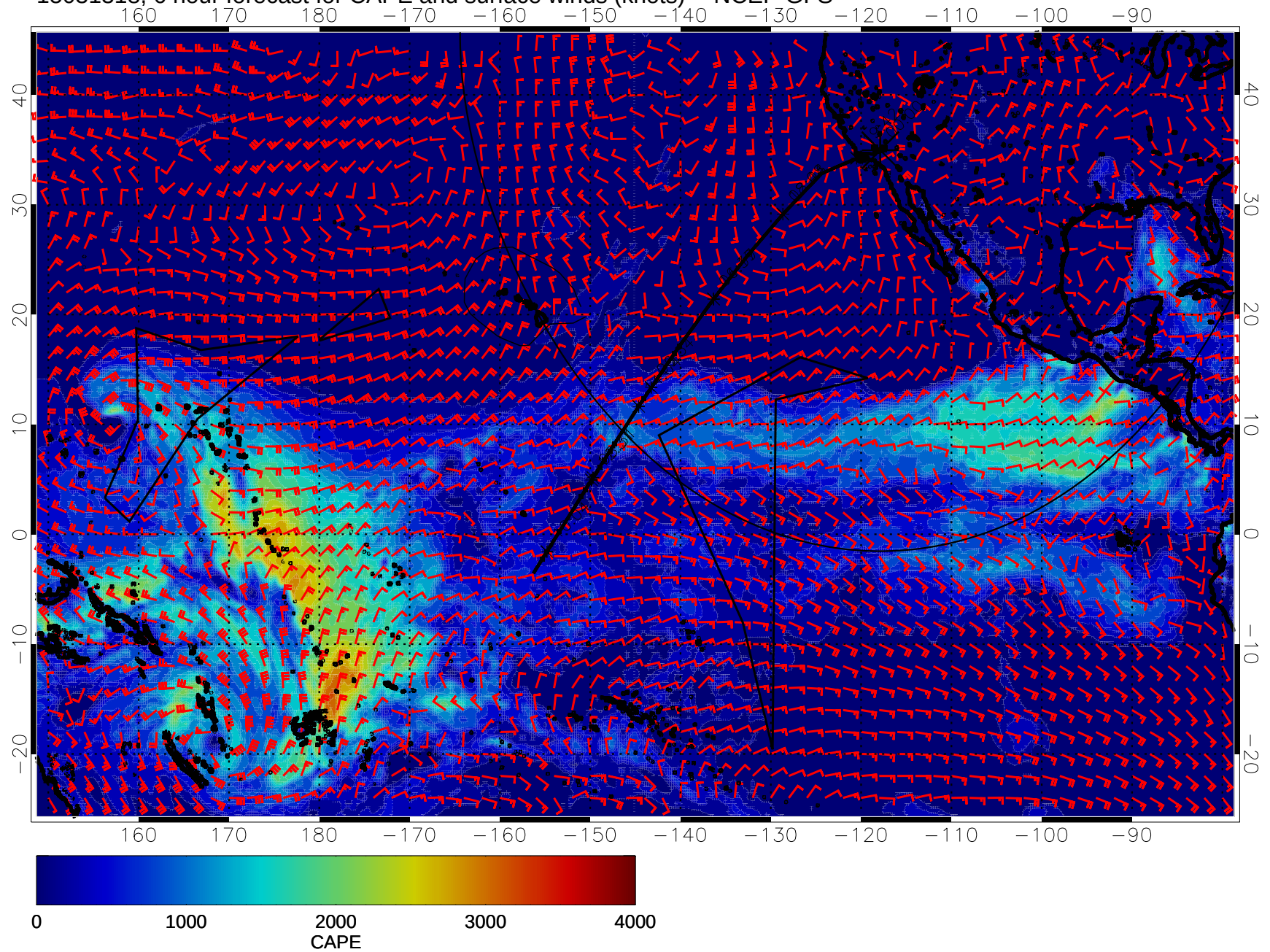
15031318, 6 hour forecast for CAPE and surface winds (knots) -- NCEP GFS
