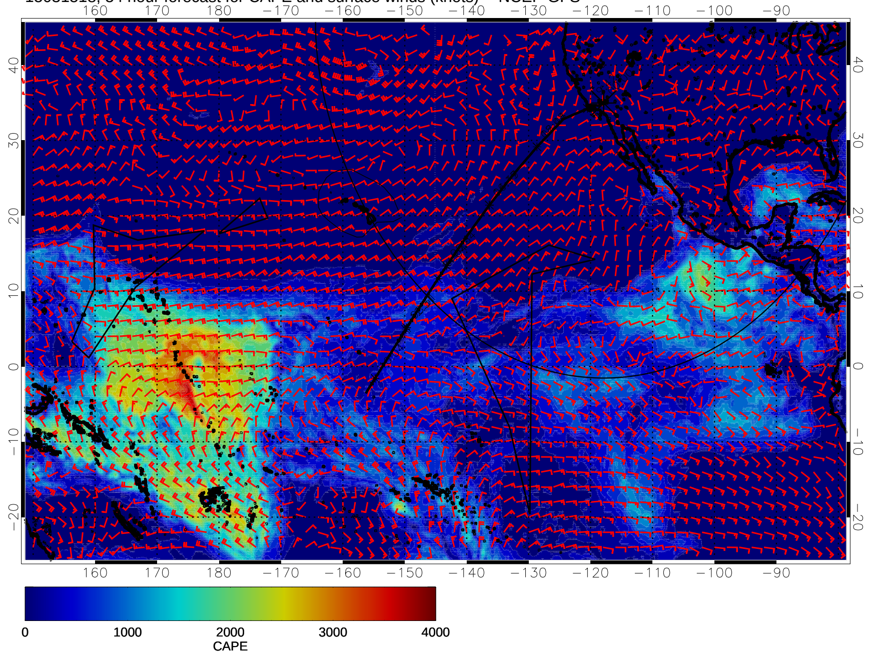
15031518, 54 hour forecast for CAPE and surface winds (knots) -- NCEP GFS
