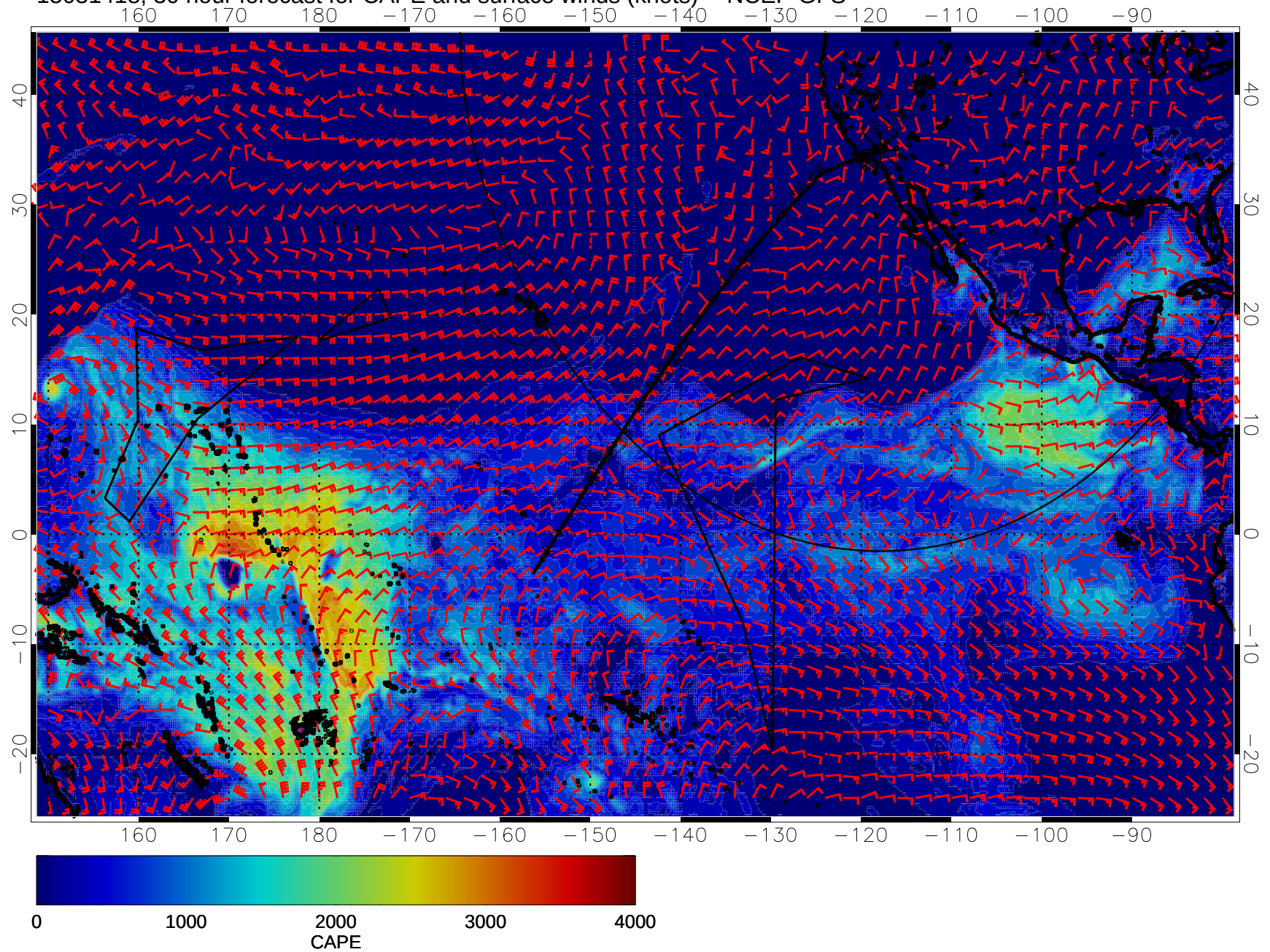
15031418, 30 hour forecast for CAPE and surface winds (knots) -- NCEP GFS
