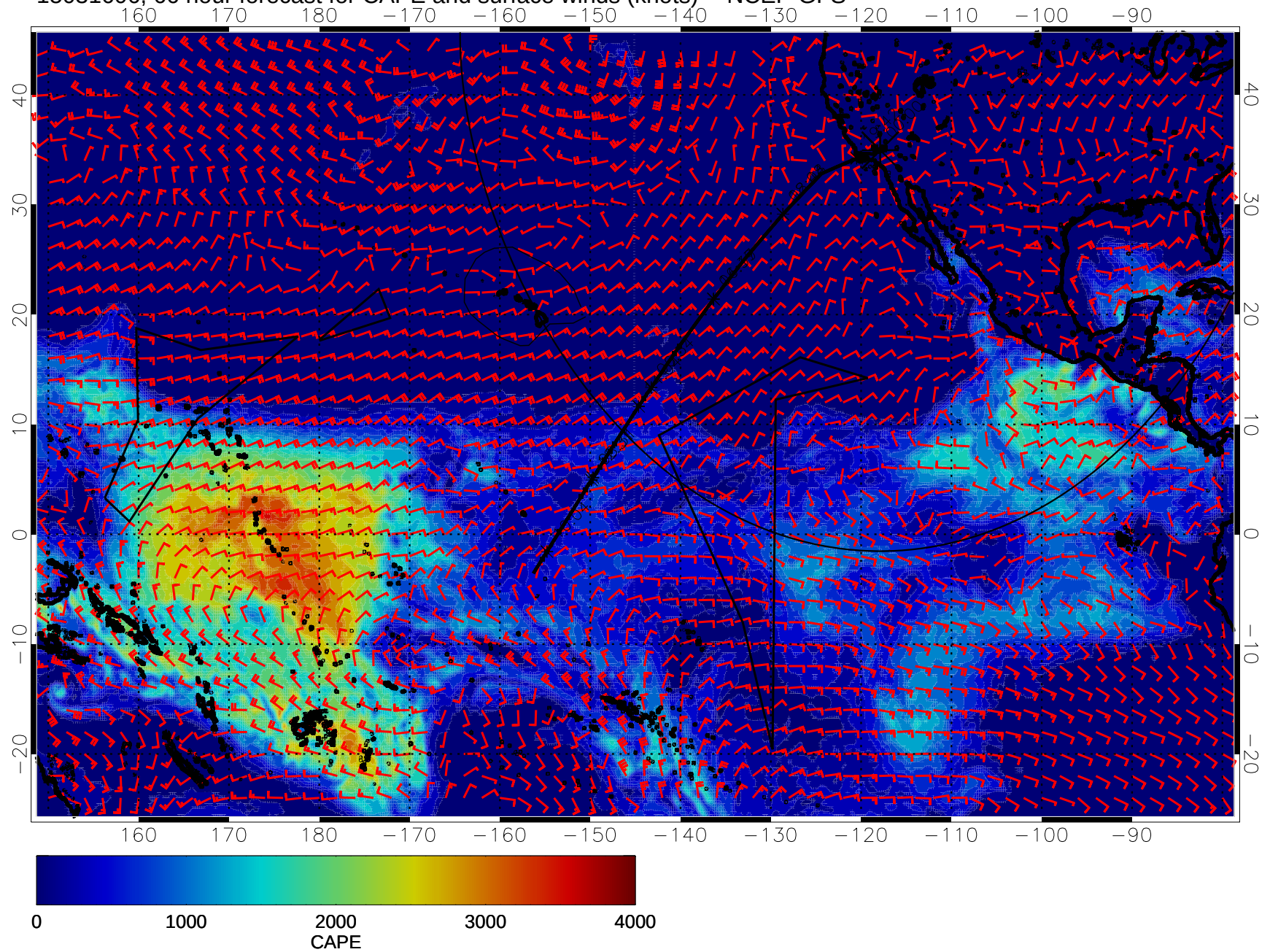
15031606, 66 hour forecast for CAPE and surface winds (knots) -- NCEP GFS
