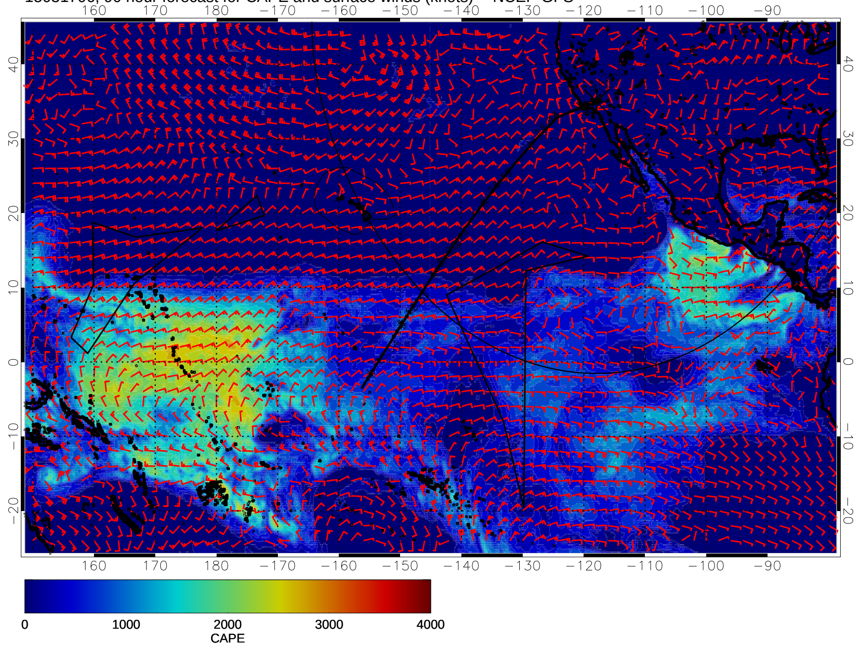
15031706, 90 hour forecast for CAPE and surface winds (knots) -- NCEP GFS
