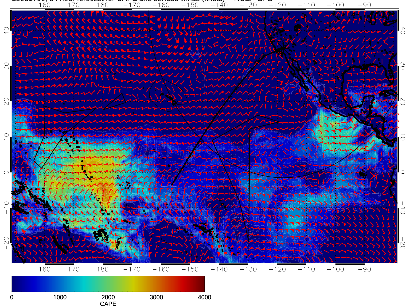
15031700, 84 hour forecast for CAPE and surface winds (knots) -- NCEP GFS
