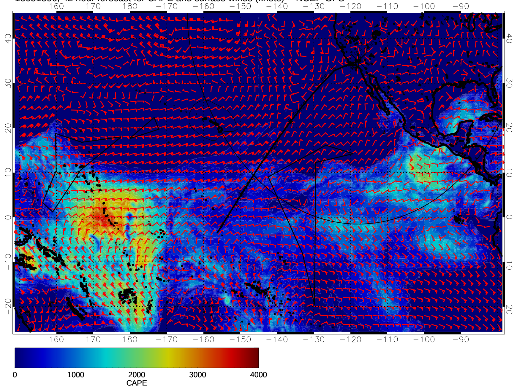
15031506, 42 hour forecast for CAPE and surface winds (knots) -- NCEP GFS
