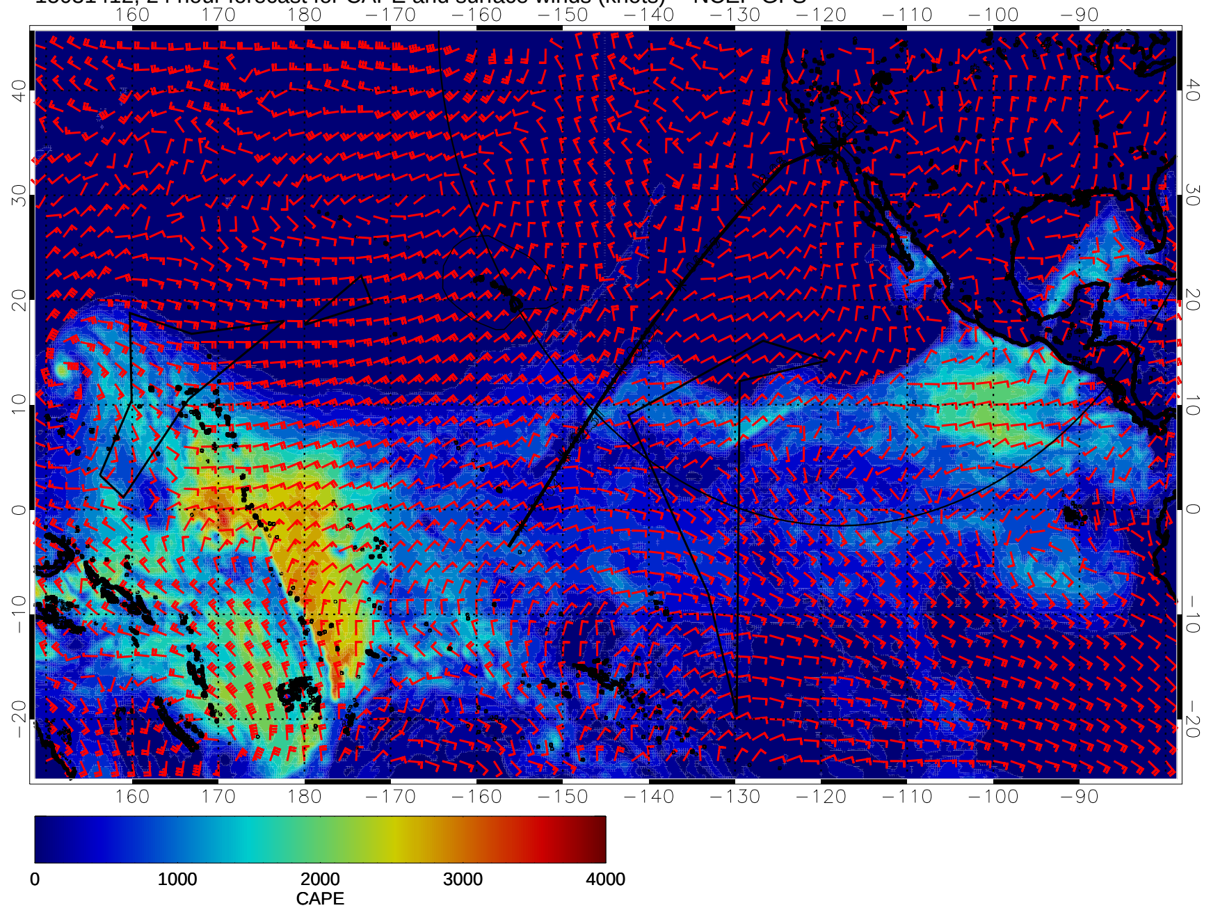
15031412, 24 hour forecast for CAPE and surface winds (knots) -- NCEP GFS
