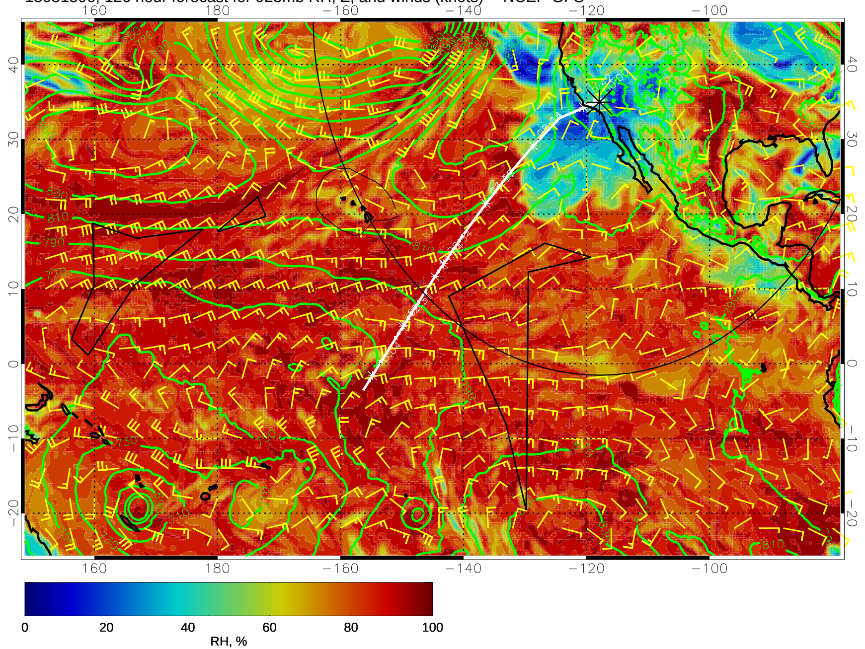
15031806, 126 hour forecast for 925mb RH, Z, and winds (knots) -- NCEP GFS
