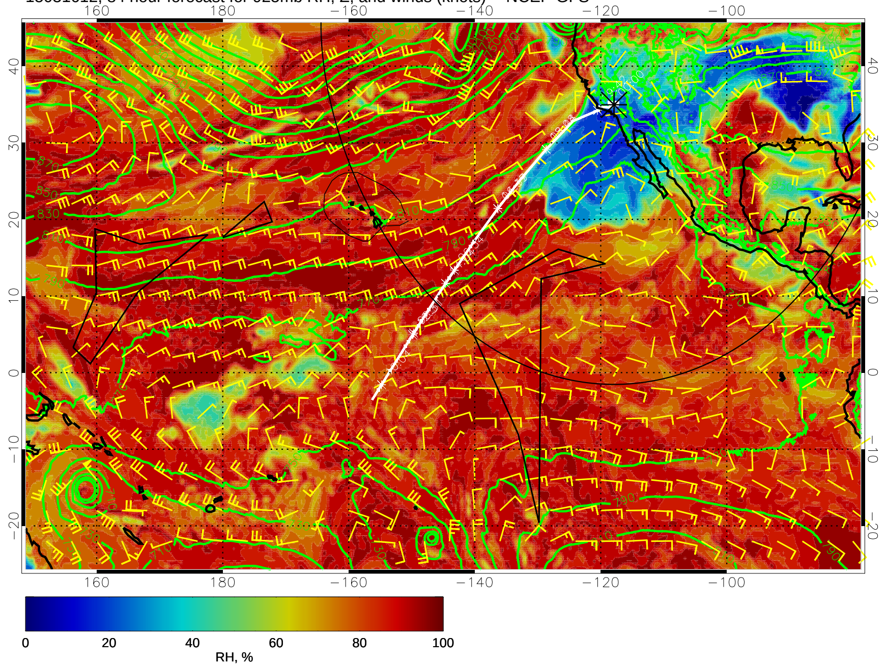
15031612, 84 hour forecast for 925mb RH, Z, and winds (knots) -- NCEP GFS
