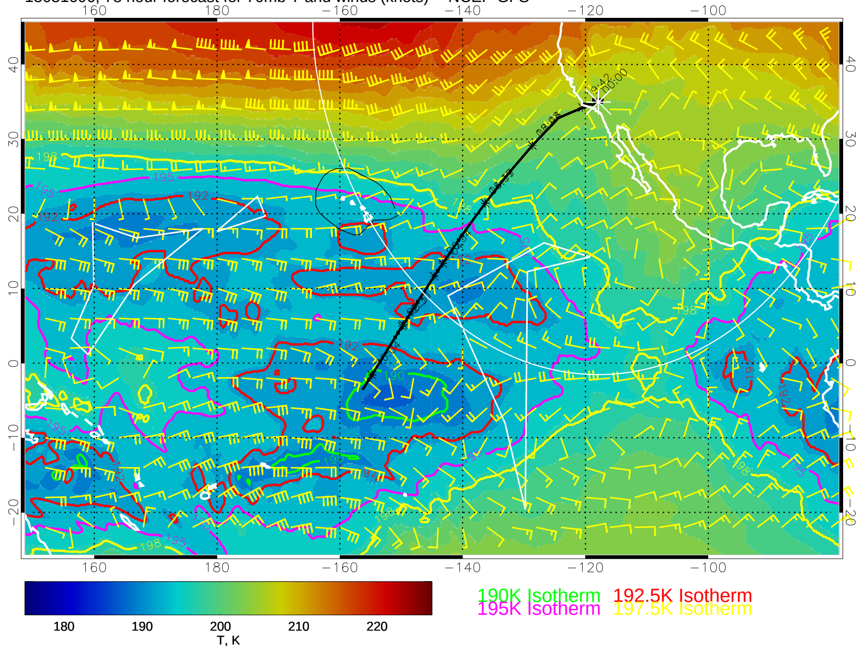
15031606, 78 hour forecast for 70mb T and winds (knots) -- NCEP GFS
