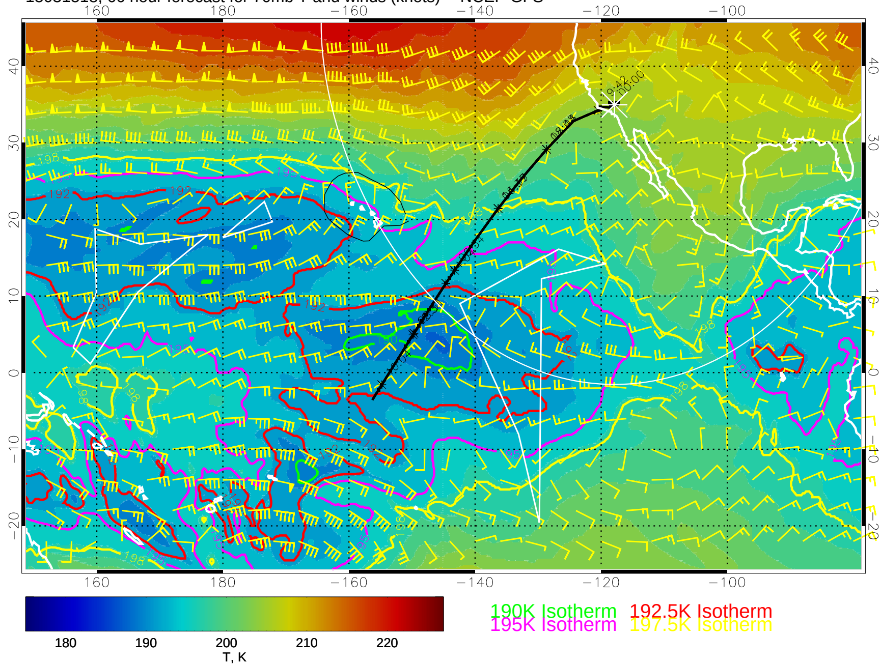
15031518, 66 hour forecast for 70mb T and winds (knots) -- NCEP GFS
