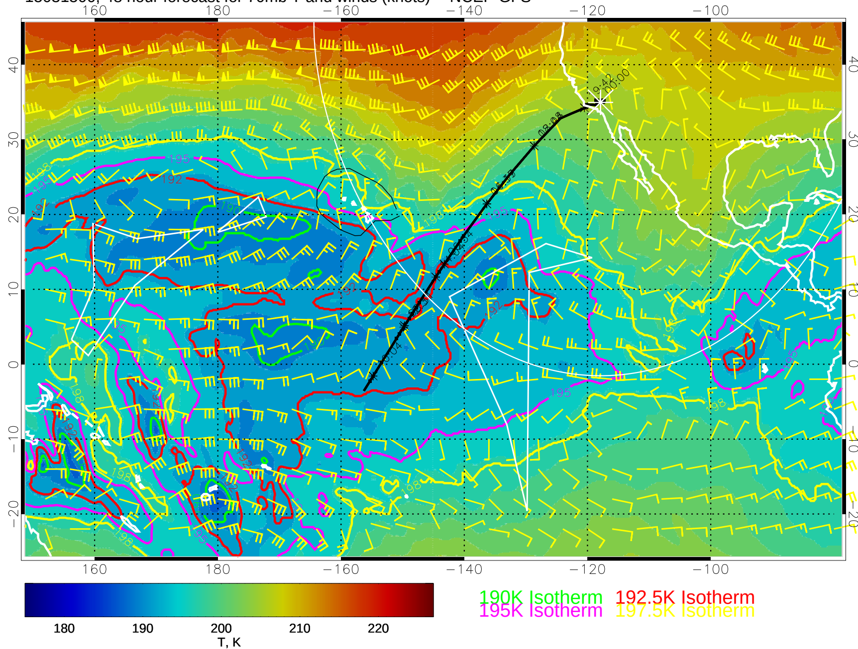
15031500, 48 hour forecast for 70mb T and winds (knots) -- NCEP GFS
