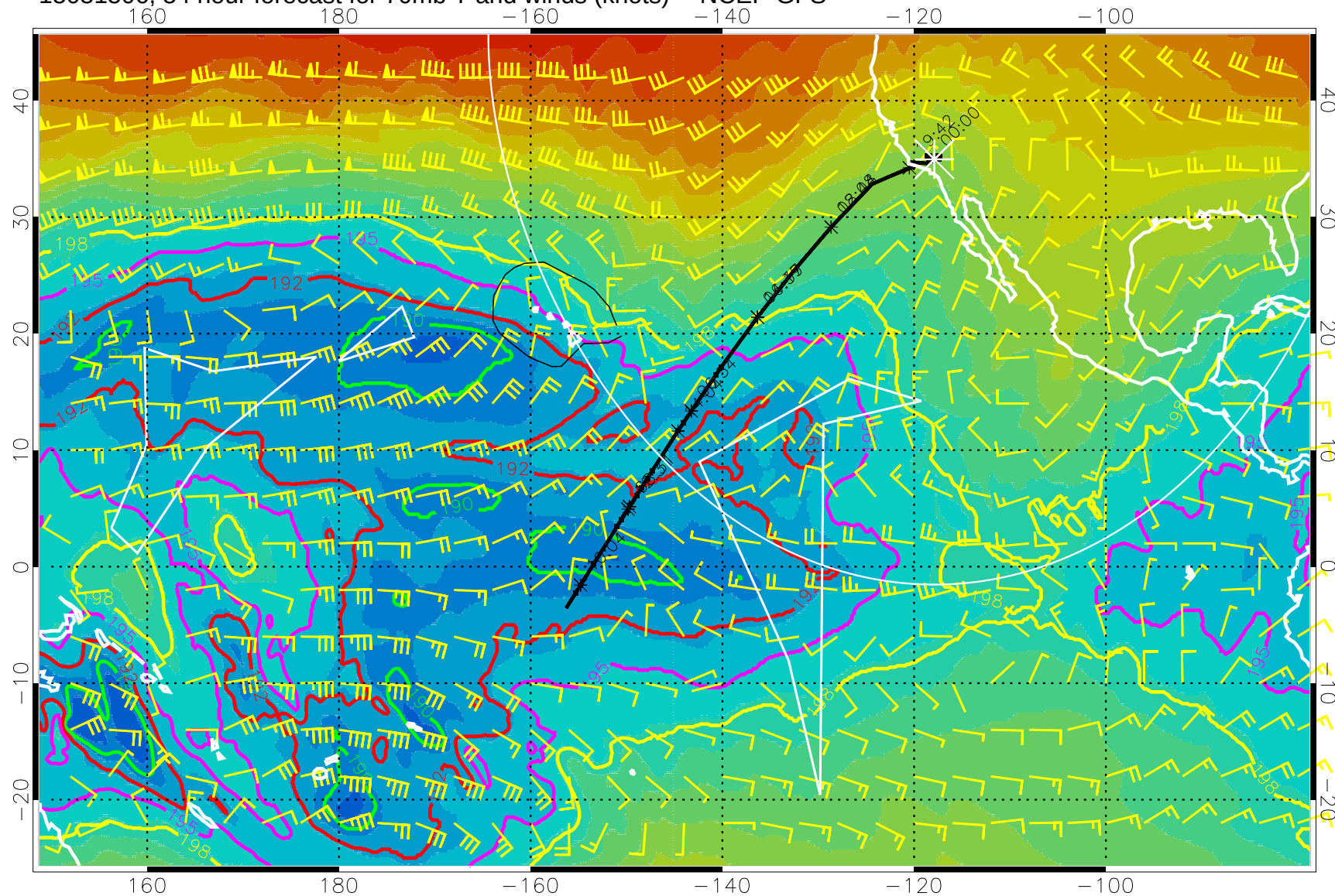
15031506, 54 hour forecast for 70mb T and winds (knots) -- NCEP GFS
