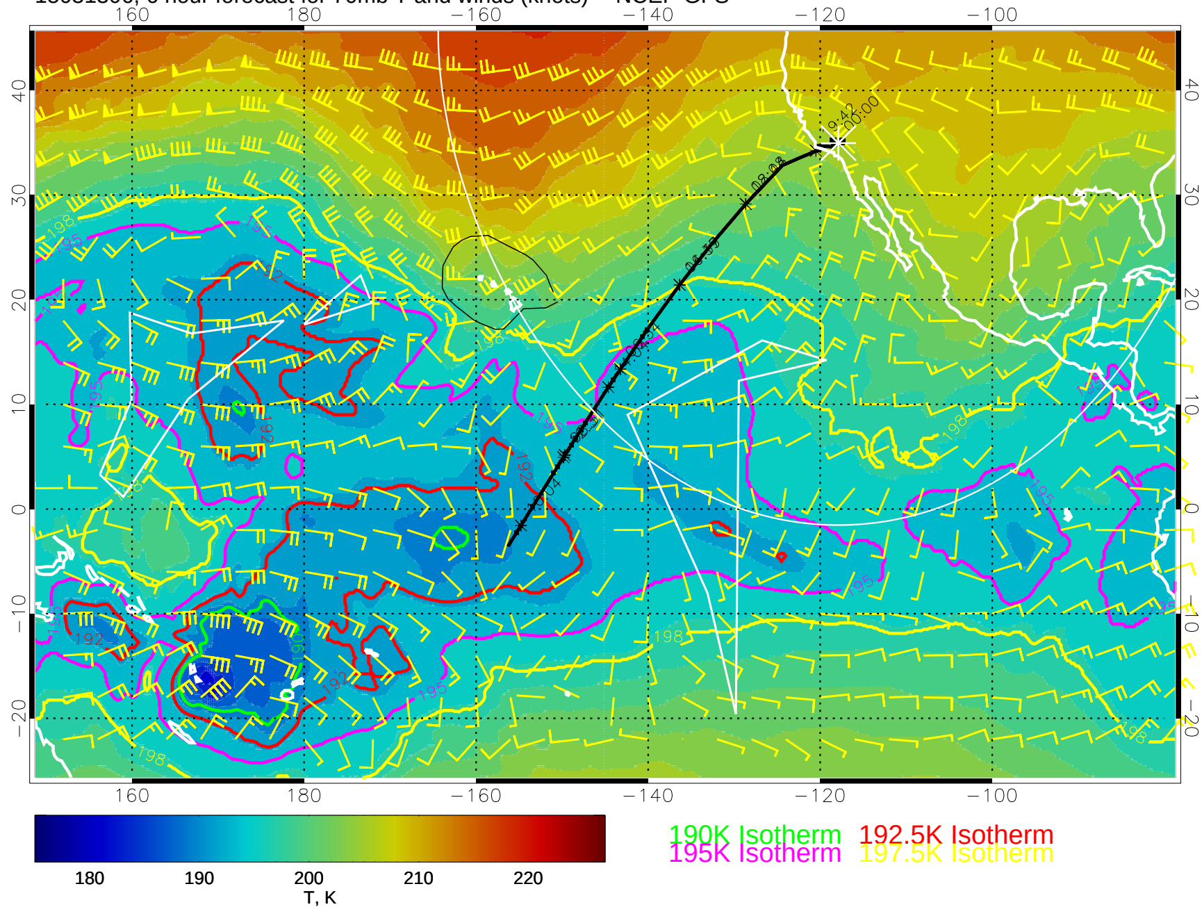
15031306, 6 hour forecast for 70mb T and winds (knots) -- NCEP GFS
