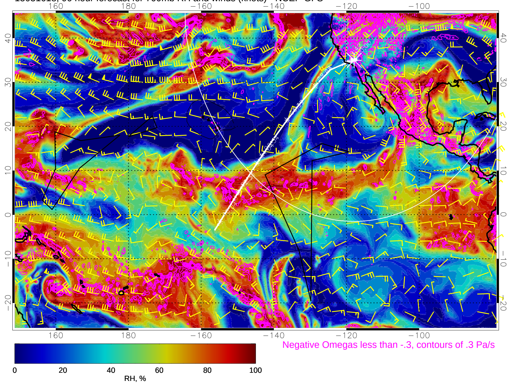
15031618, 90 hour forecast for 700mb RH and winds (knots) - NCEP GFS
