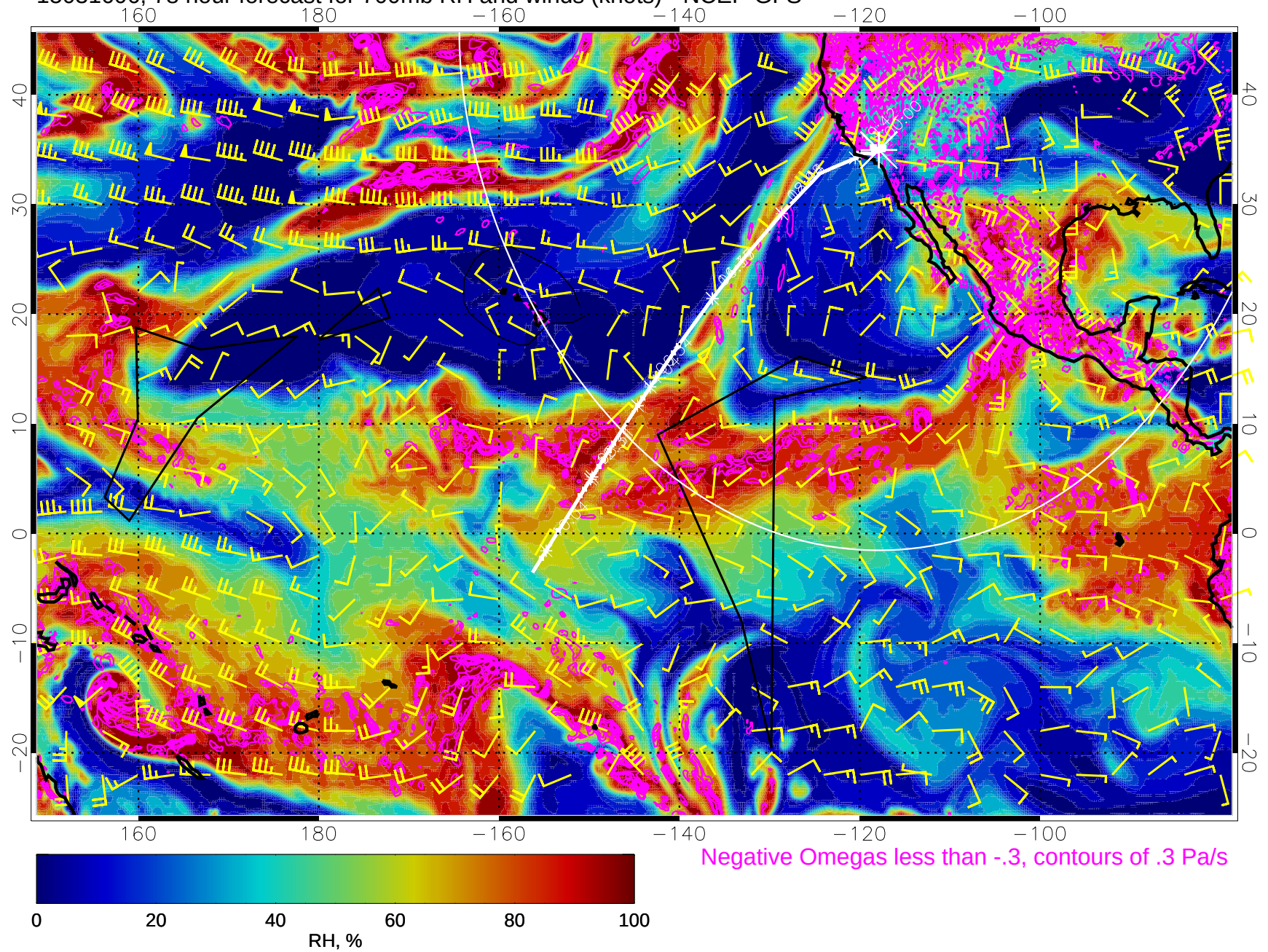
15031606, 78 hour forecast for 700mb RH and winds (knots) - NCEP GFS
