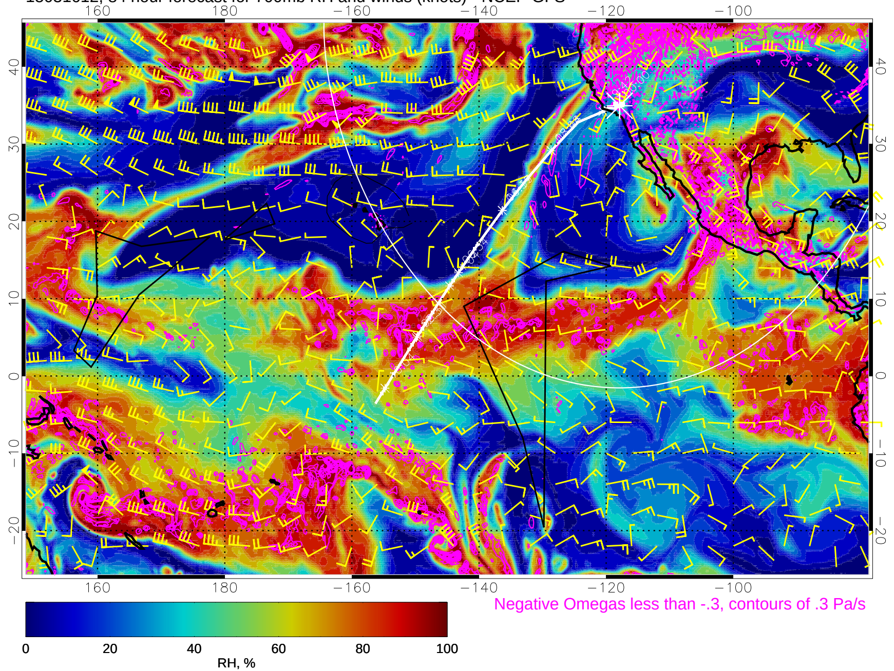
15031612, 84 hour forecast for 700mb RH and winds (knots) - NCEP GFS
