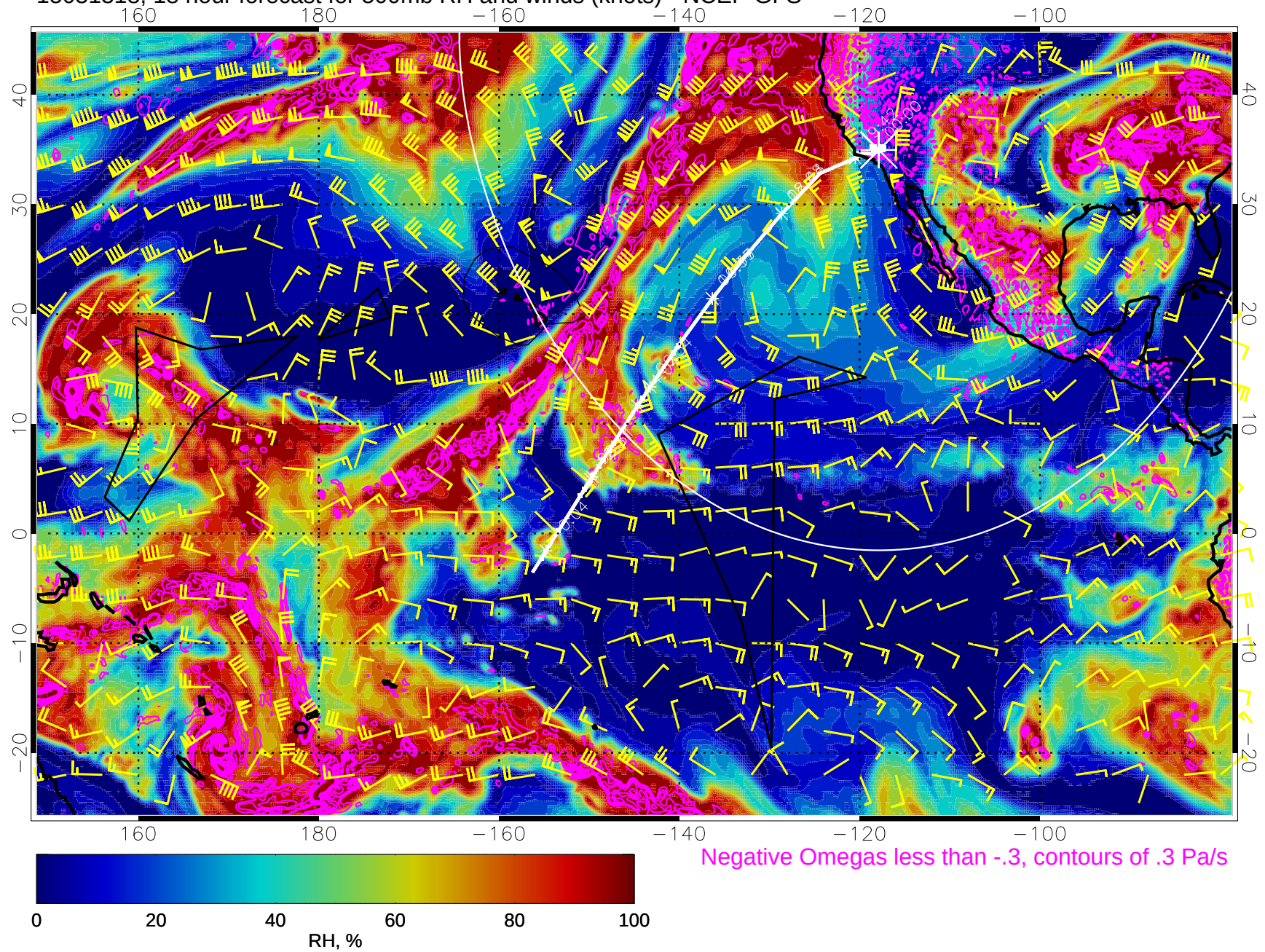
15031318, 18 hour forecast for 500mb RH and winds (knots) - NCEP GFS
