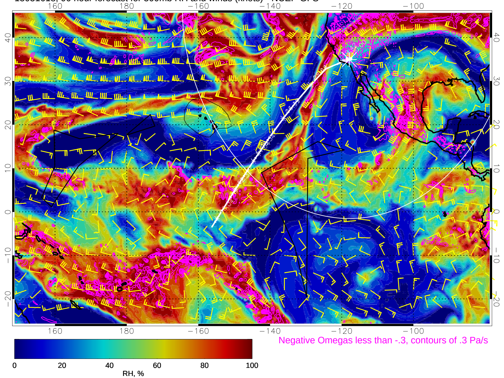
15031618, 90 hour forecast for 500mb RH and winds (knots) - NCEP GFS
