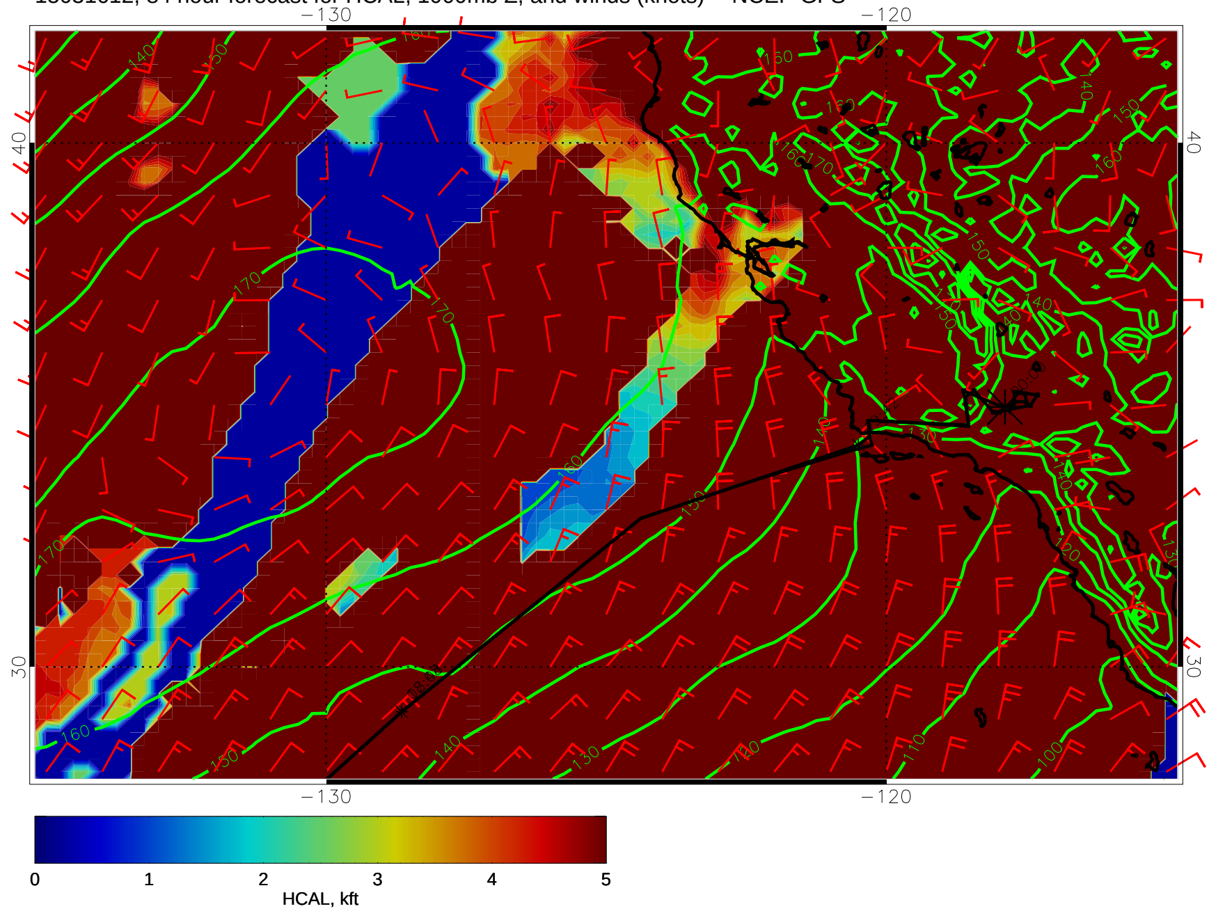
15031612, 84 hour forecast for HCAL, 1000mb Z, and winds (knots) -- NCEP GFS
