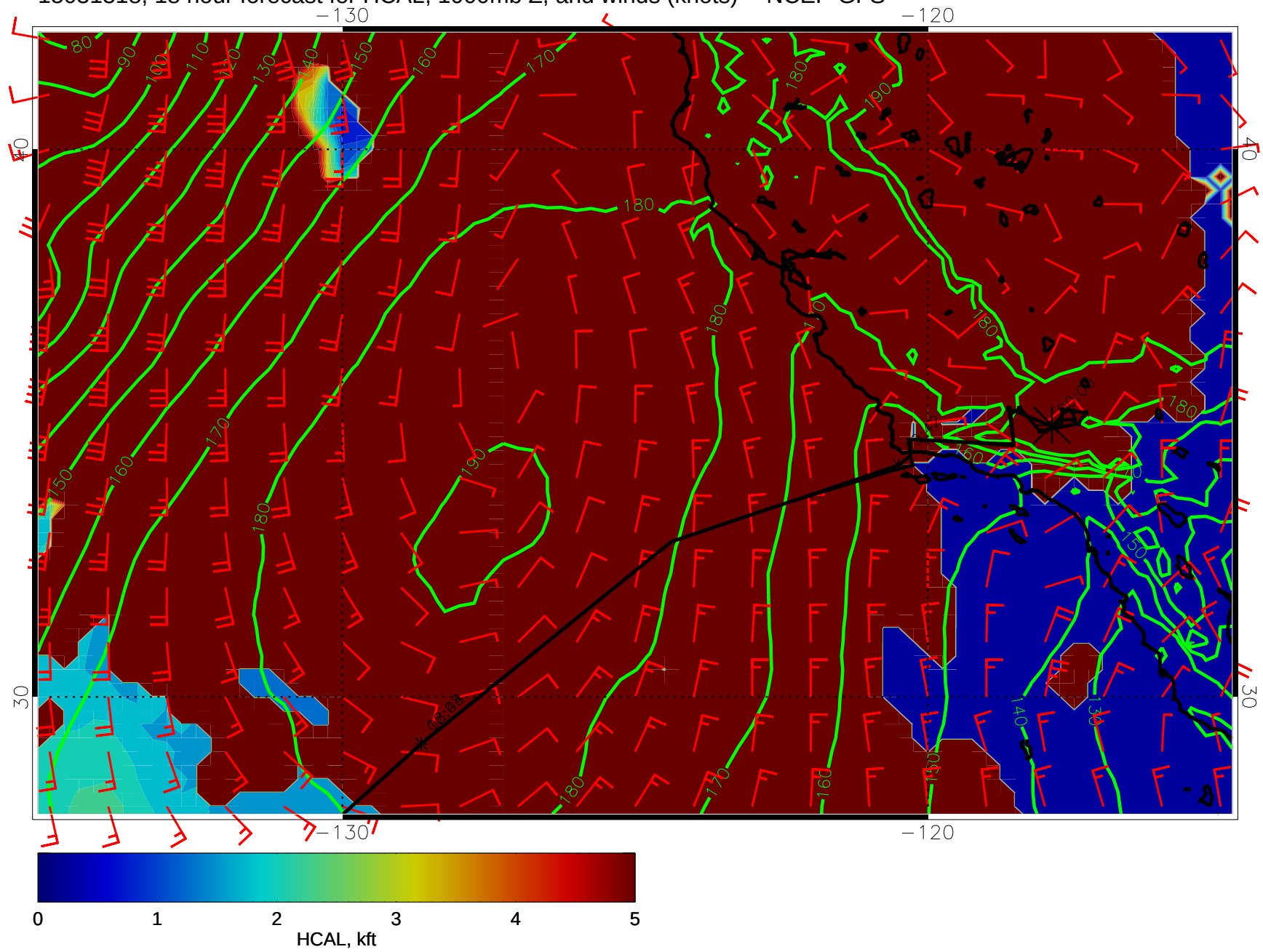
15031318, 18 hour forecast for HCAL, 1000mb Z, and winds (knots) -- NCEP GFS
