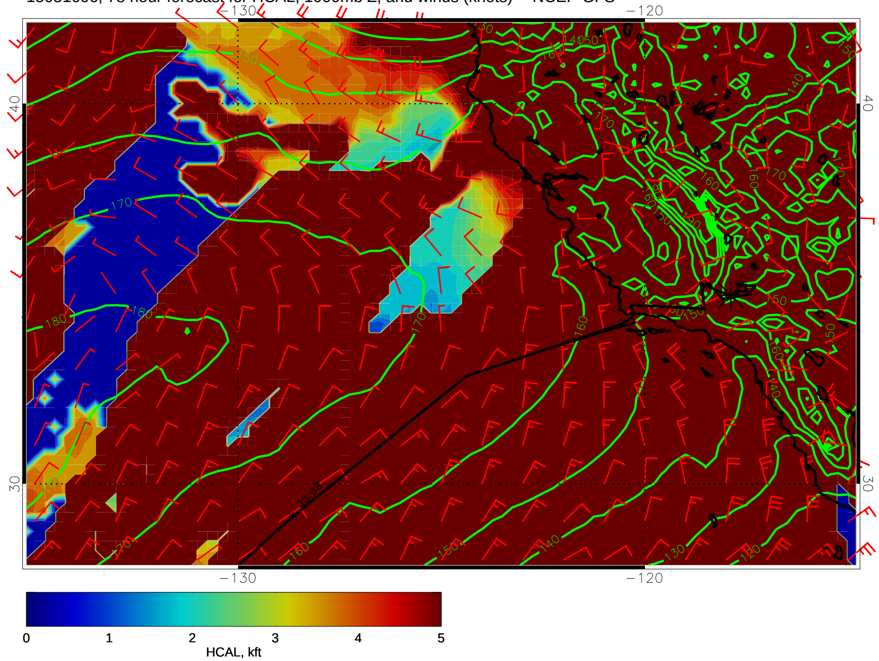
15031606, 78 hour forecast for HCAL, 1000mb Z, and winds (knots) -- NCEP GFS
