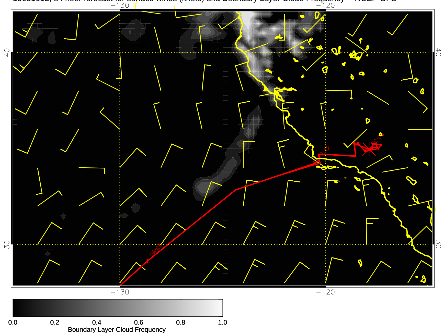
15031612, 84 hour forecast for surface winds (knots) and Boundary Layer Cloud Frequency -- NCEP GFS
