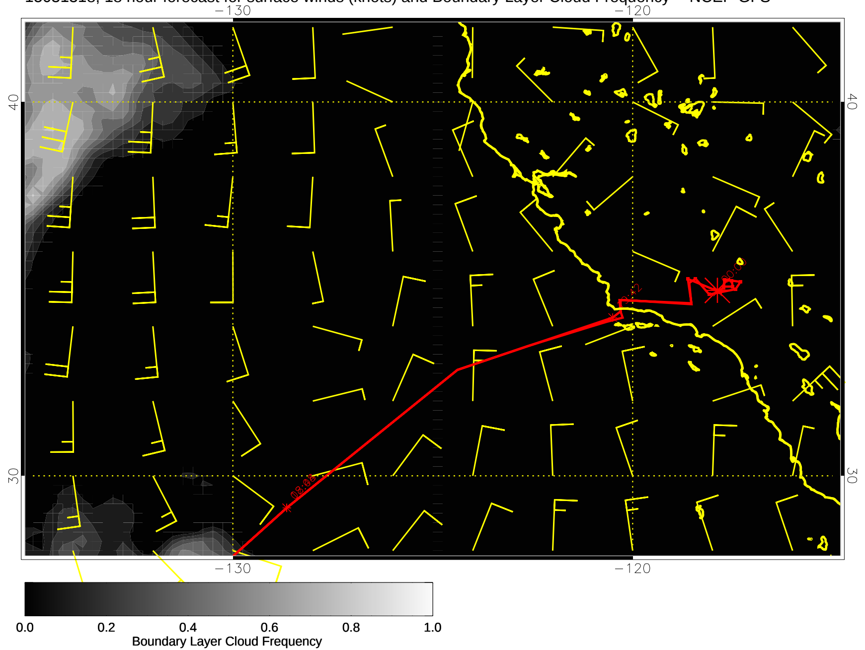
15031318, 18 hour forecast for surface winds (knots) and Boundary Layer Cloud Frequency -- NCEP GFS
