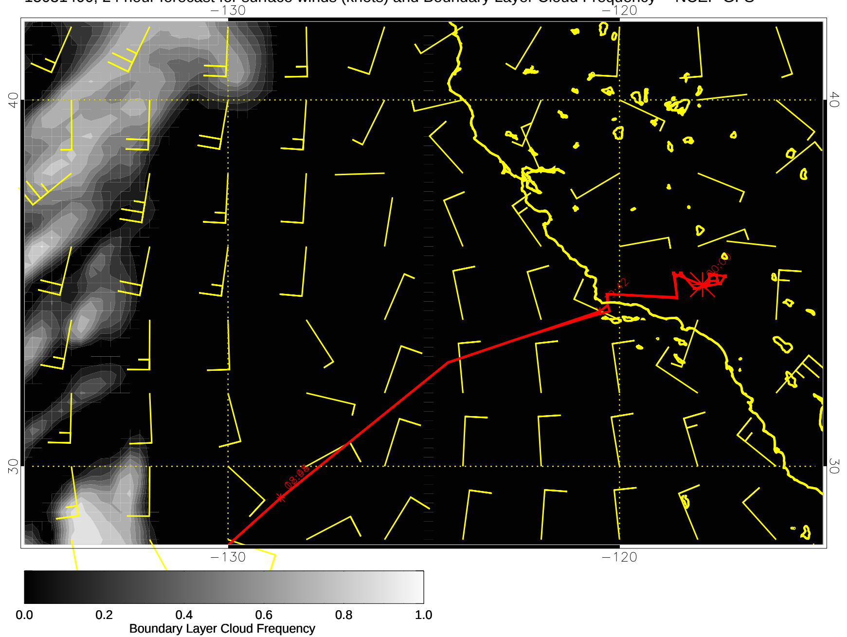
15031400, 24 hour forecast for surface winds (knots) and Boundary Layer Cloud Frequency -- NCEP GFS
