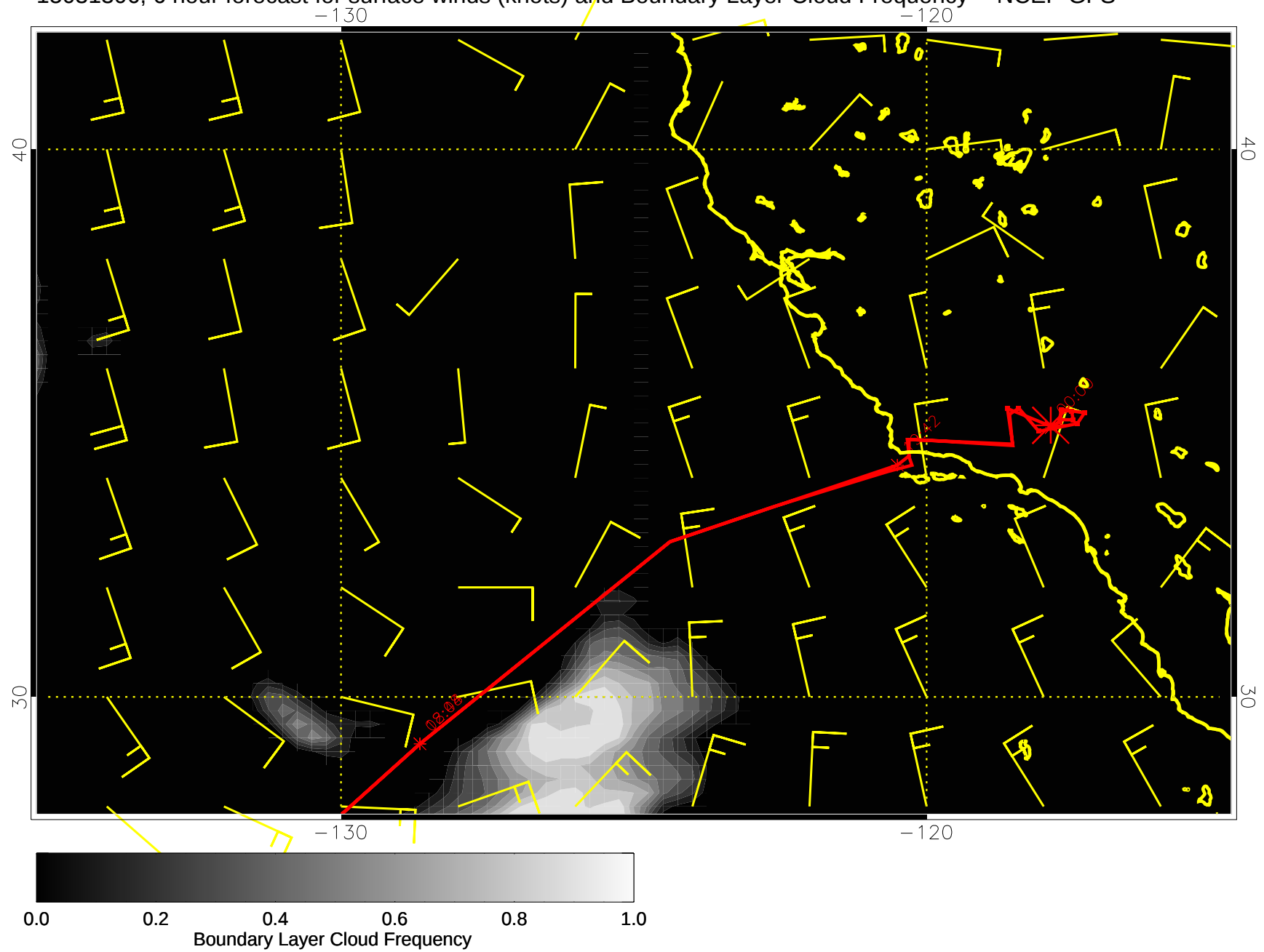
15031306, 6 hour forecast for surface winds (knots) and Boundary Layer Cloud Frequency -- NCEP GFS
