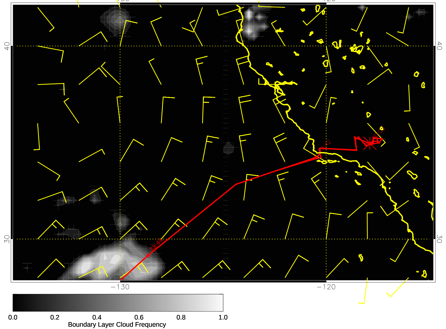
15031718, 114 hour forecast for surface winds (knots) and Boundary Layer Cloud Frequency -- NCEP GFS
