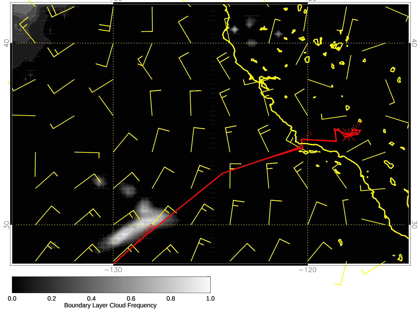
15031706, 102 hour forecast for surface winds (knots) and Boundary Layer Cloud Frequency -- NCEP GFS
