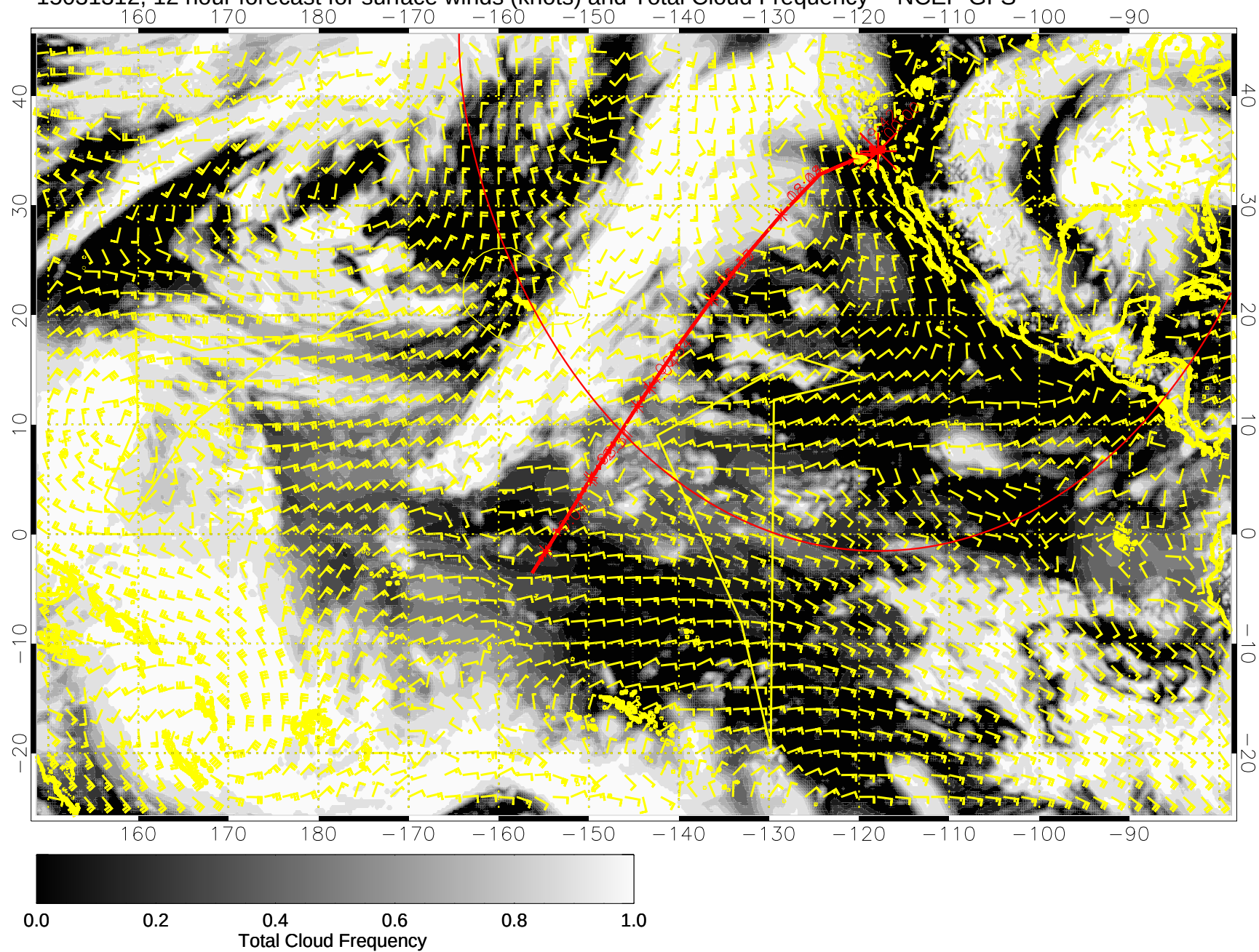
15031312, 12 hour forecast for surface winds (knots) and Total Cloud Frequency -- NCEP GFS
