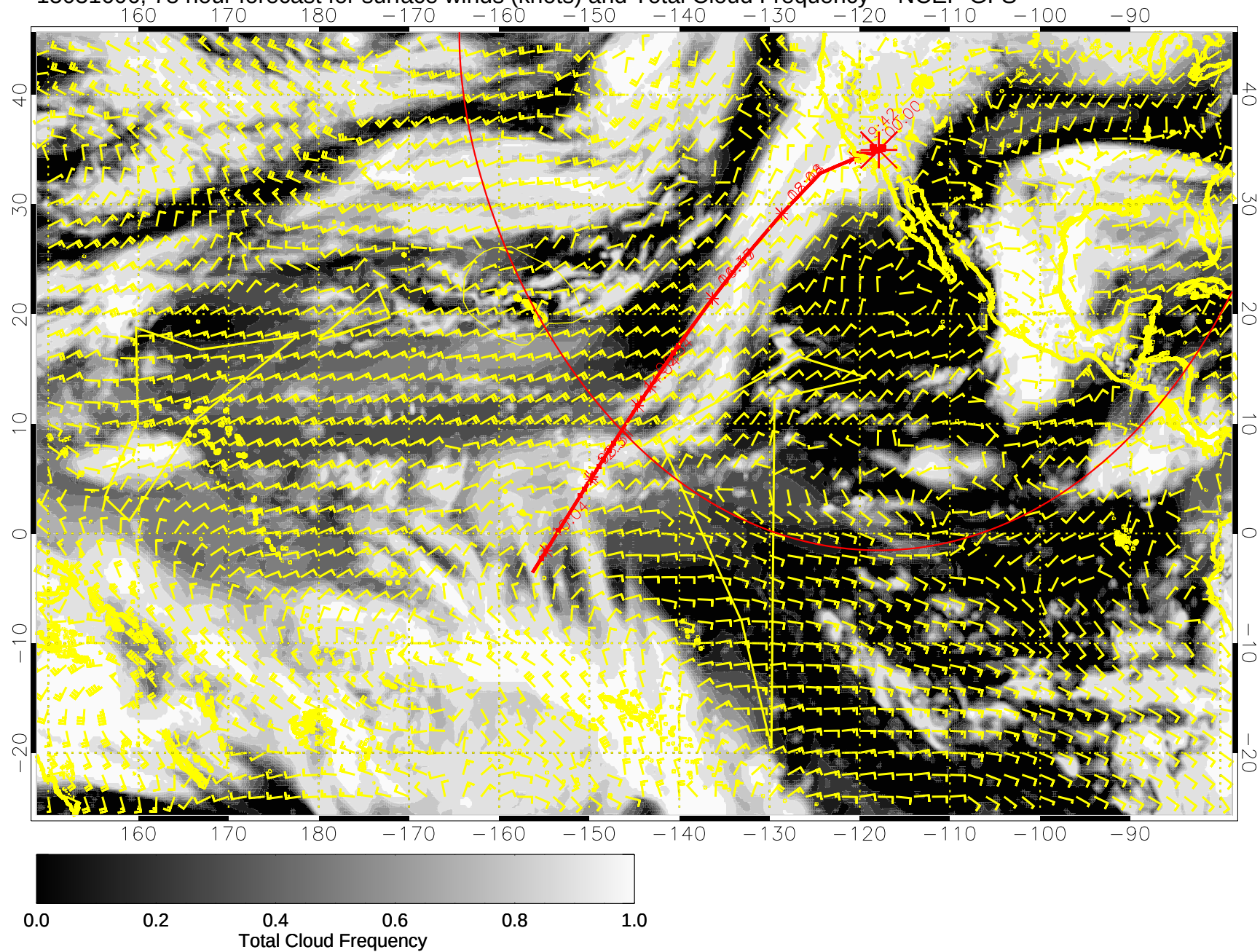
15031606, 78 hour forecast for surface winds (knots) and Total Cloud Frequency -- NCEP GFS
