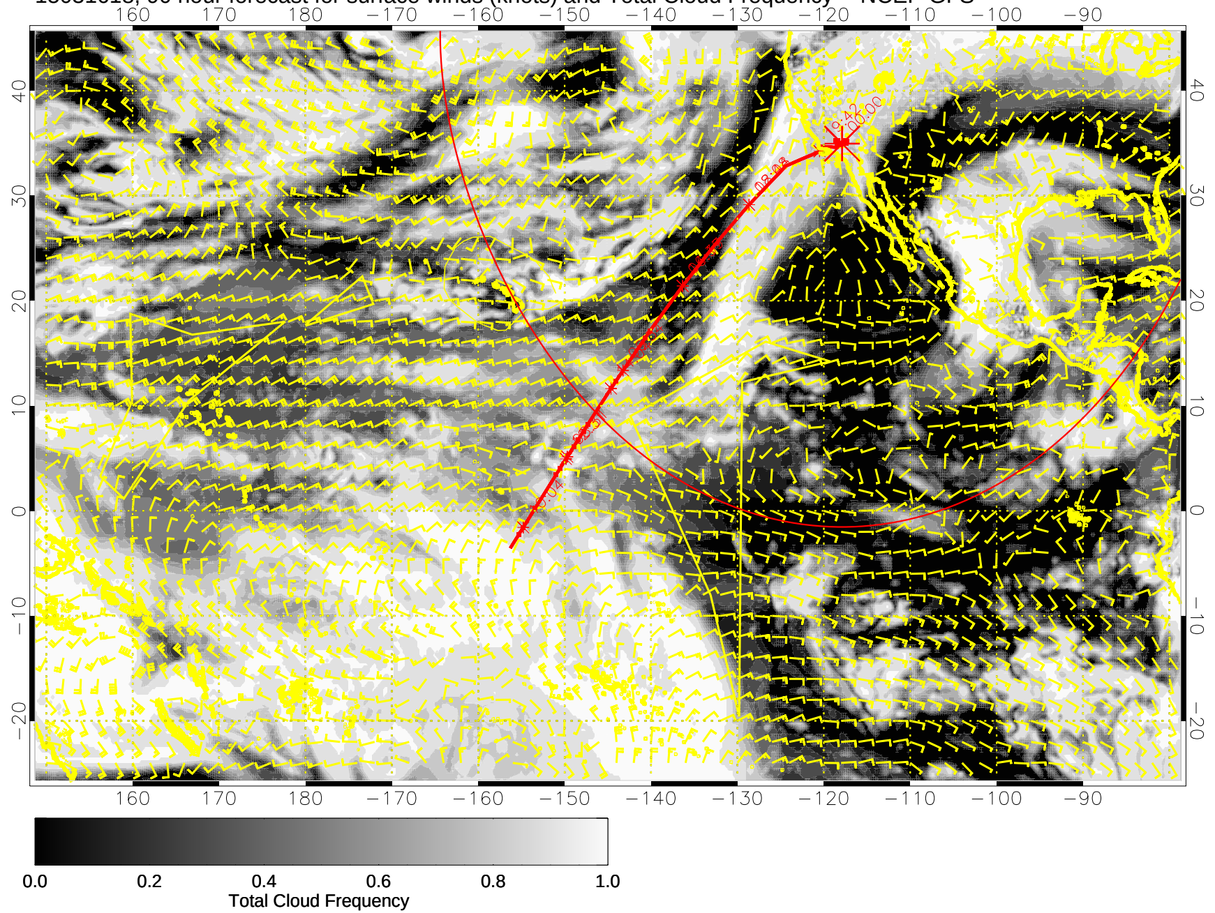
15031618, 90 hour forecast for surface winds (knots) and Total Cloud Frequency -- NCEP GFS
