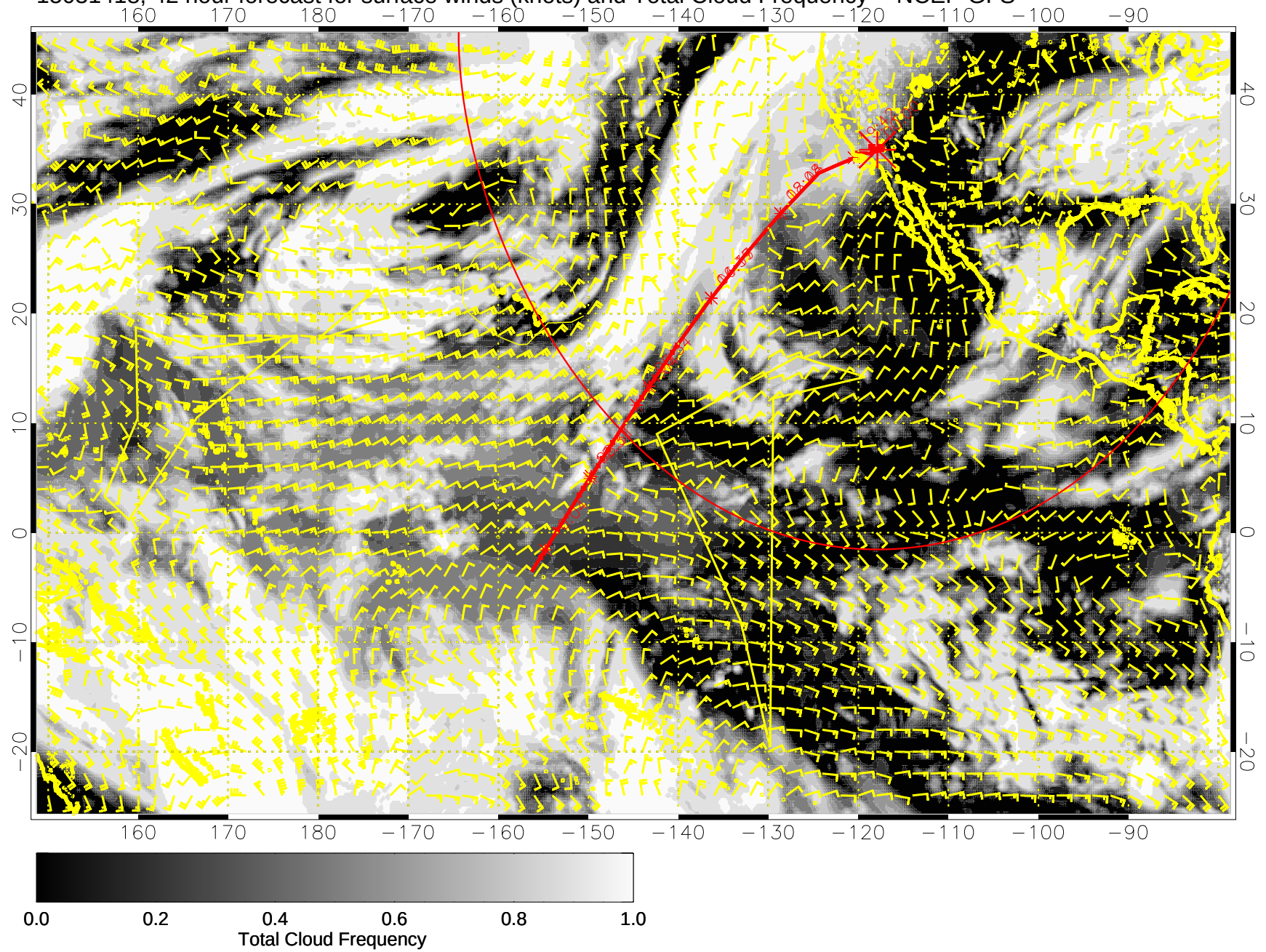
15031418, 42 hour forecast for surface winds (knots) and Total Cloud Frequency -- NCEP GFS
