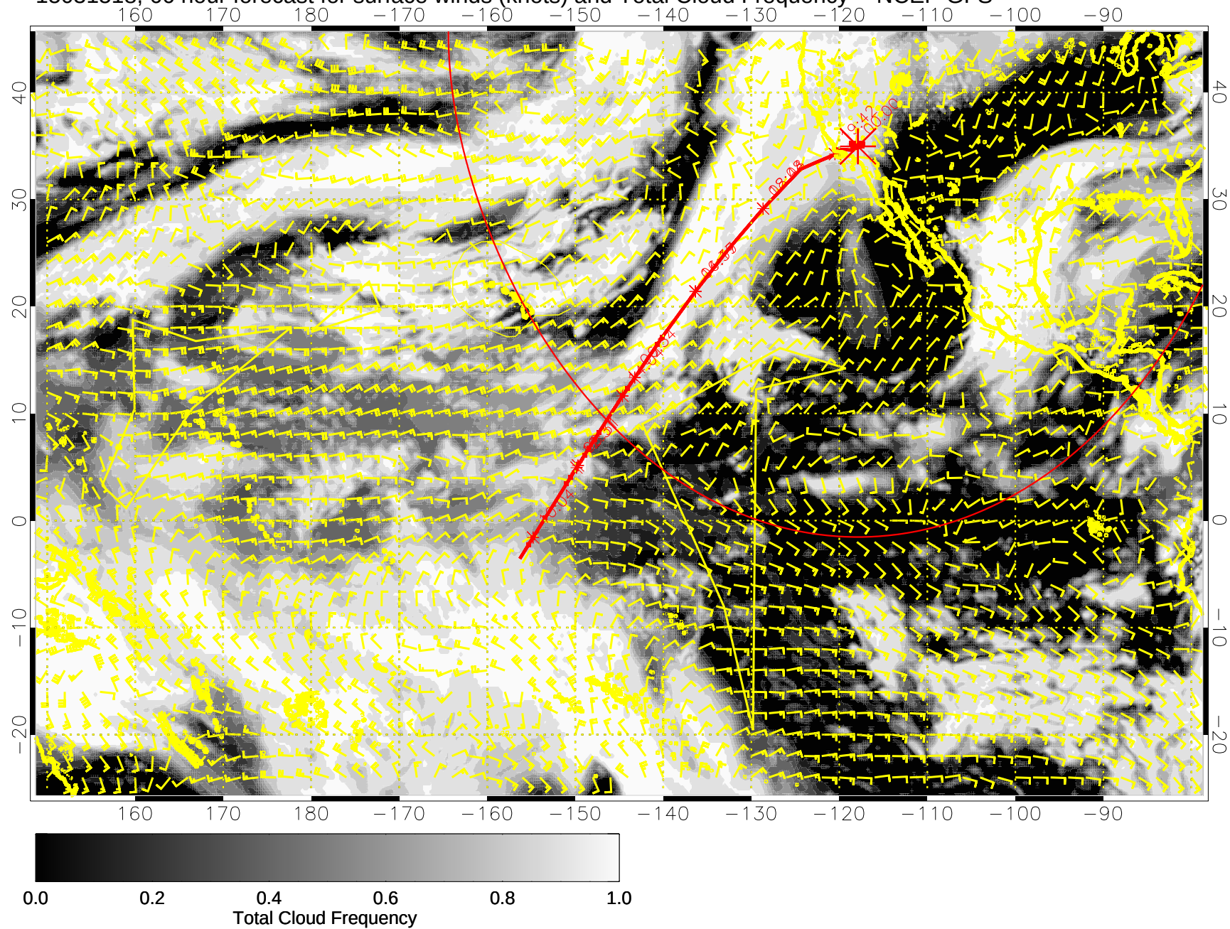
15031518, 66 hour forecast for surface winds (knots) and Total Cloud Frequency -- NCEP GFS
