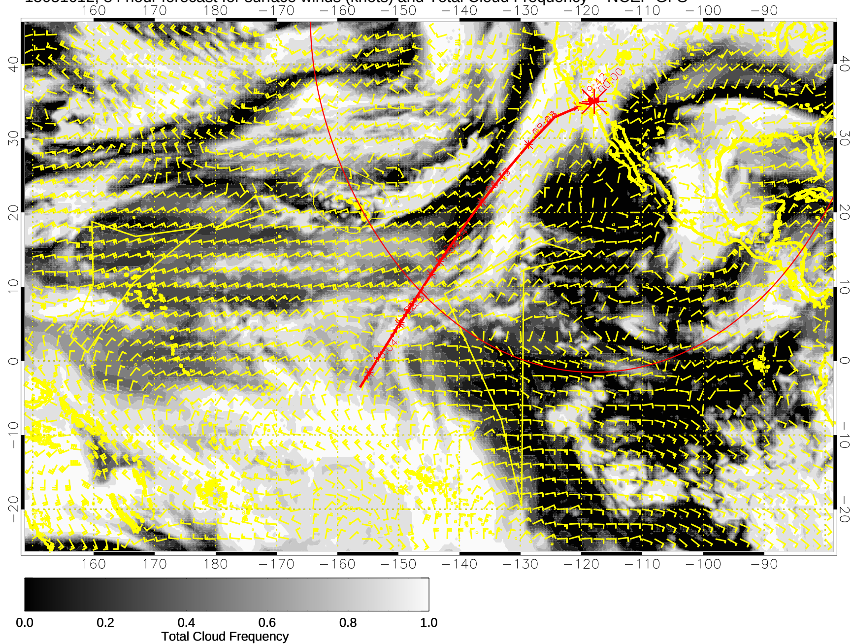
15031612, 84 hour forecast for surface winds (knots) and Total Cloud Frequency -- NCEP GFS
