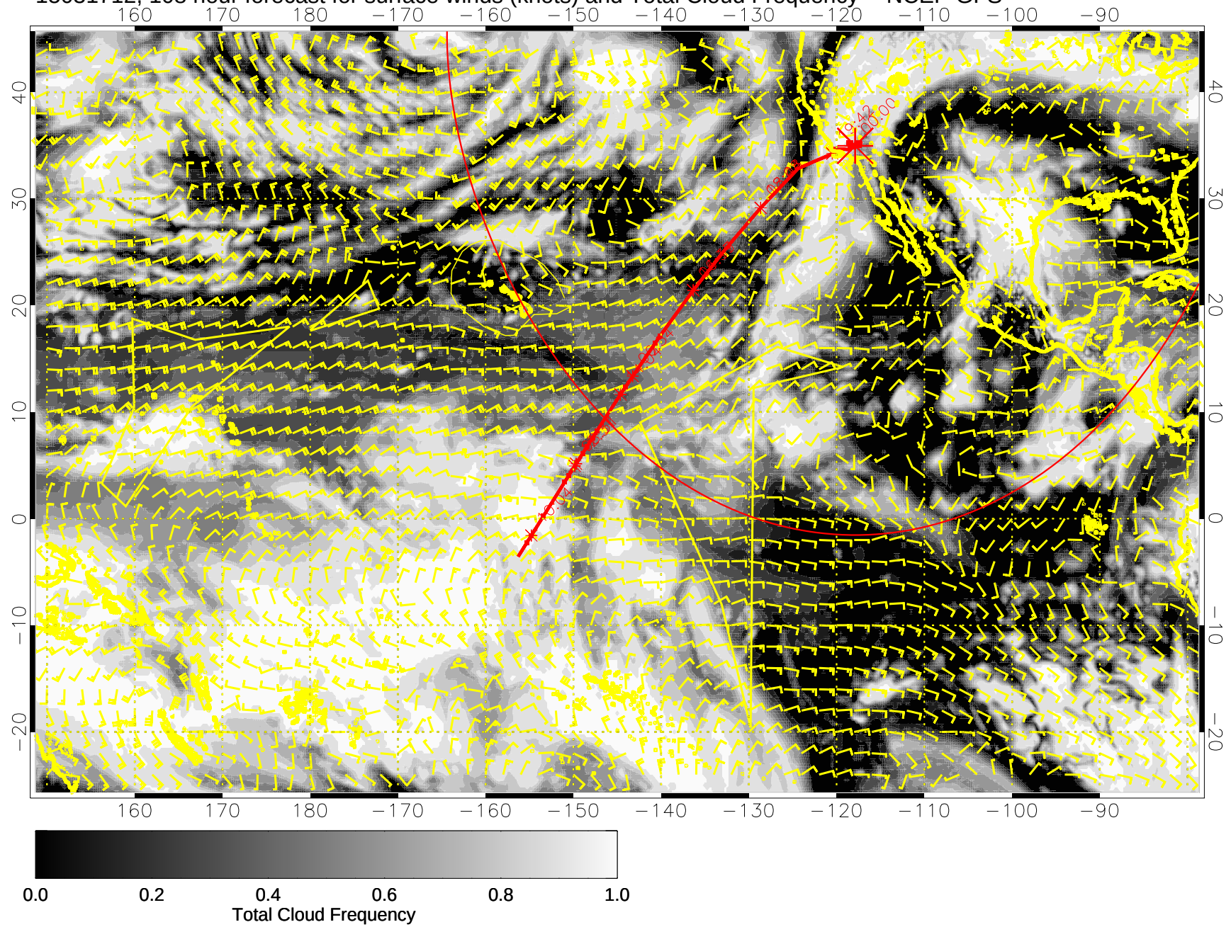
15031712, 108 hour forecast for surface winds (knots) and Total Cloud Frequency -- NCEP GFS
