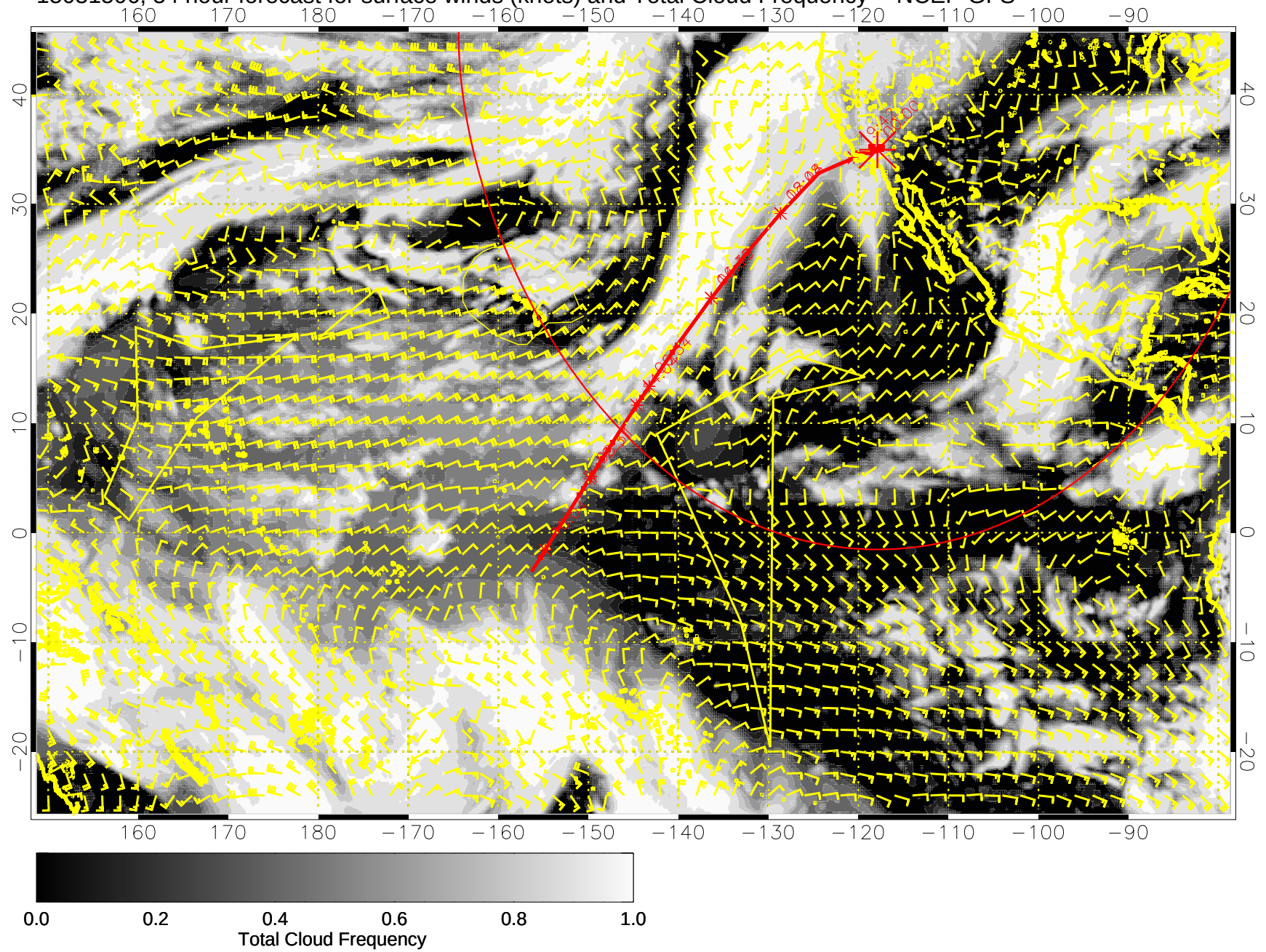
15031506, 54 hour forecast for surface winds (knots) and Total Cloud Frequency -- NCEP GFS
