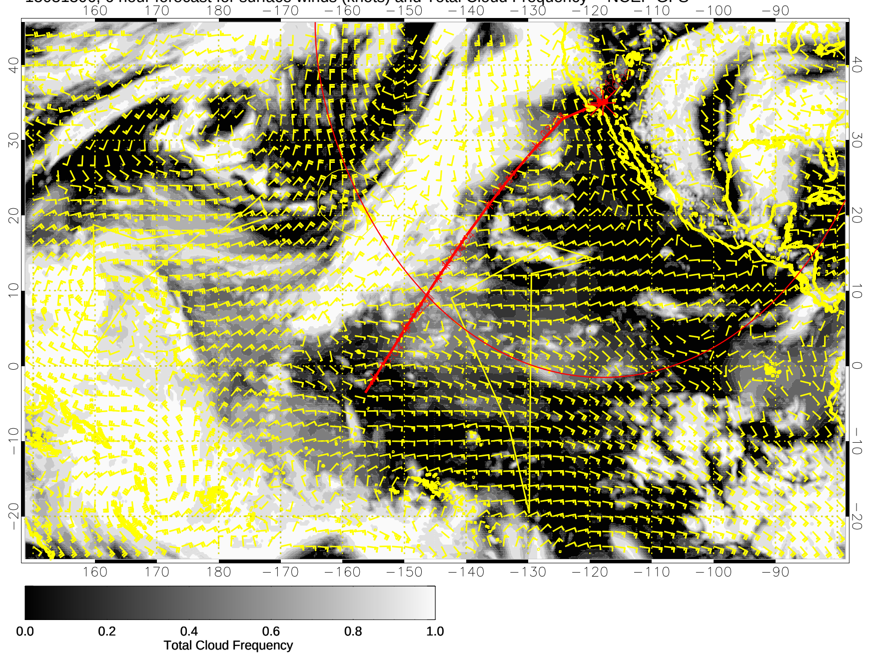
15031306, 6 hour forecast for surface winds (knots) and Total Cloud Frequency -- NCEP GFS
