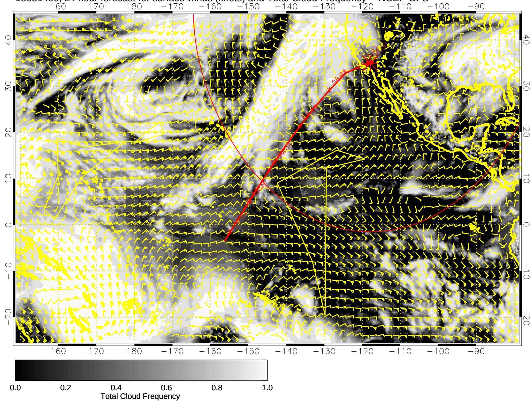
15031400, 24 hour forecast for surface winds (knots) and Total Cloud Frequency -- NCEP GFS
