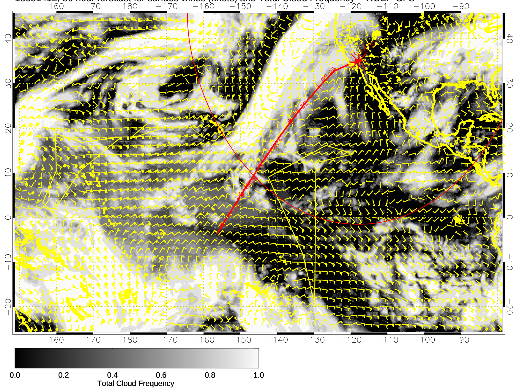
15031412, 36 hour forecast for surface winds (knots) and Total Cloud Frequency -- NCEP GFS
