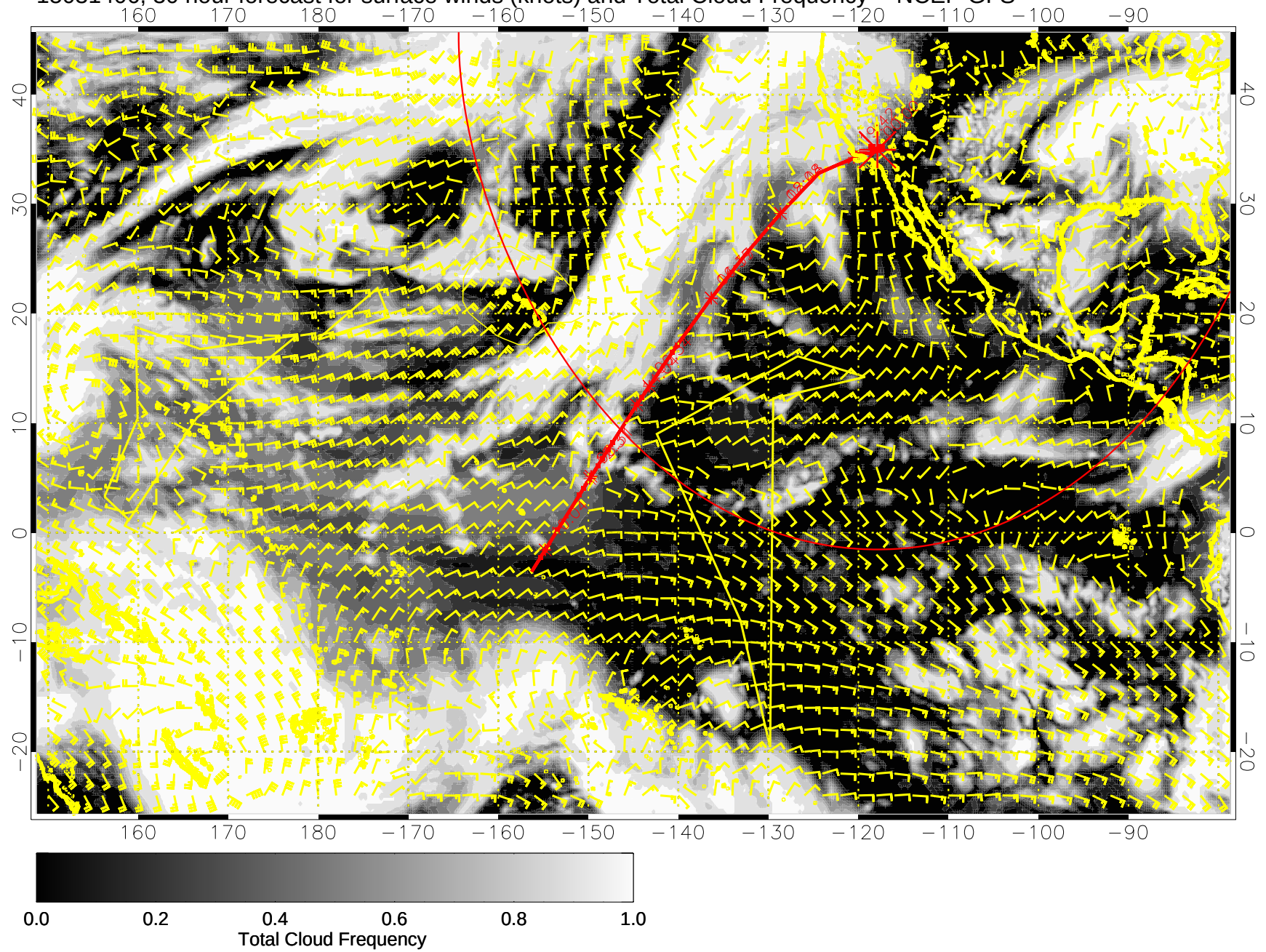
15031406, 30 hour forecast for surface winds (knots) and Total Cloud Frequency -- NCEP GFS
