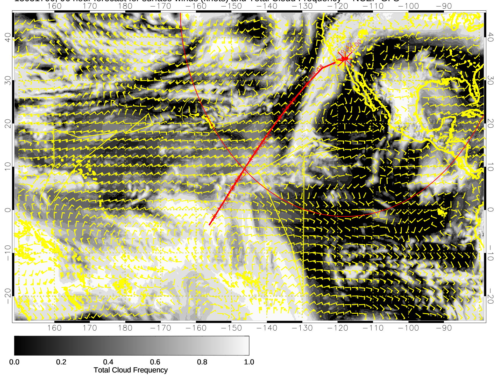
15031700, 96 hour forecast for surface winds (knots) and Total Cloud Frequency -- NCEP GFS
