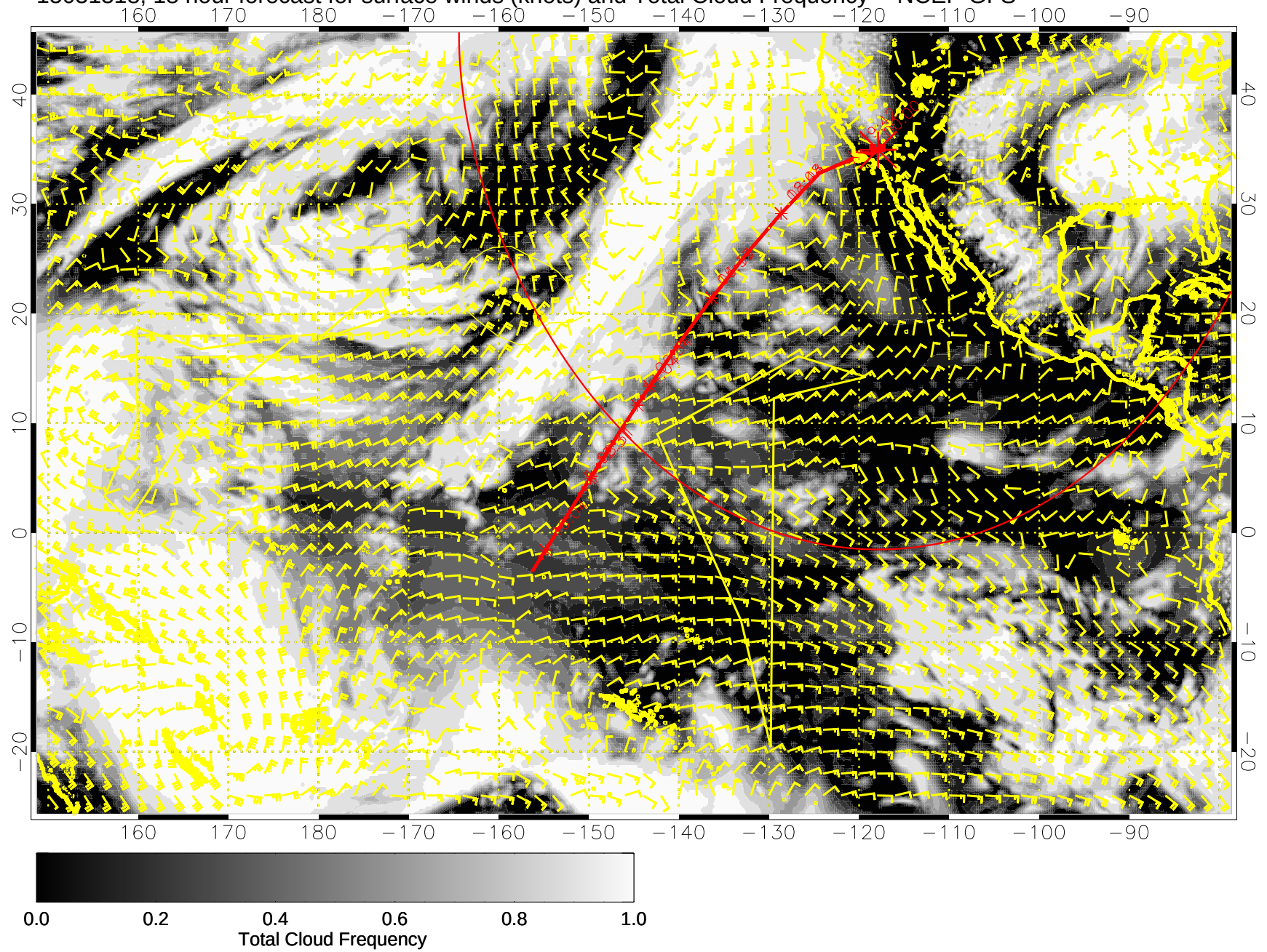
15031318, 18 hour forecast for surface winds (knots) and Total Cloud Frequency -- NCEP GFS
