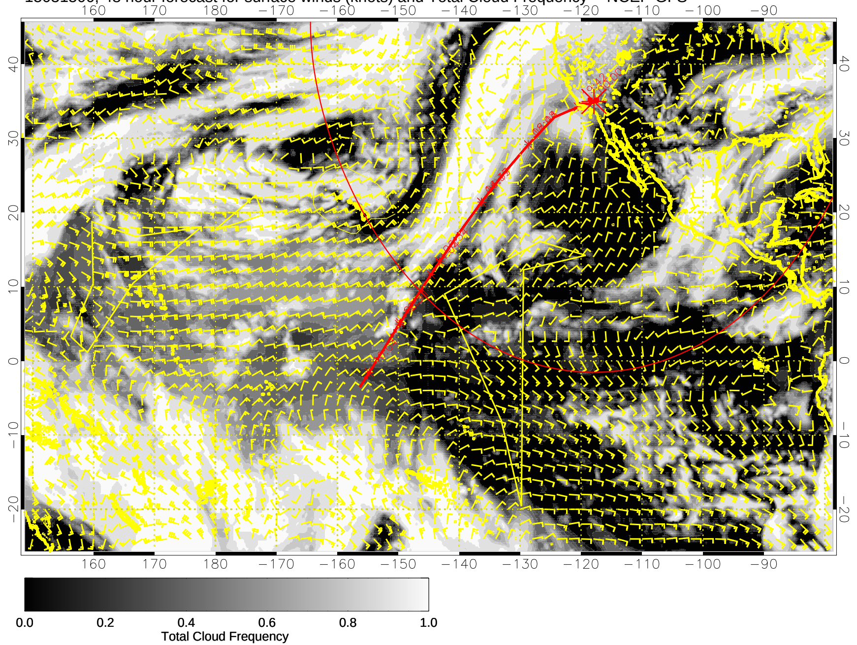
15031500, 48 hour forecast for surface winds (knots) and Total Cloud Frequency -- NCEP GFS
