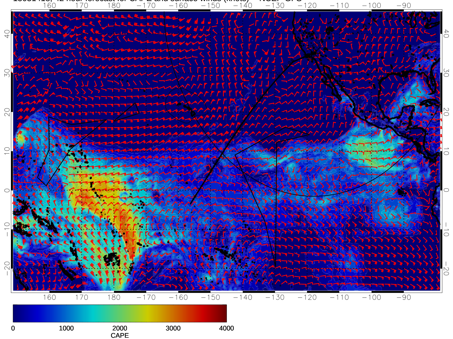
15031418, 42 hour forecast for CAPE and surface winds (knots) -- NCEP GFS
