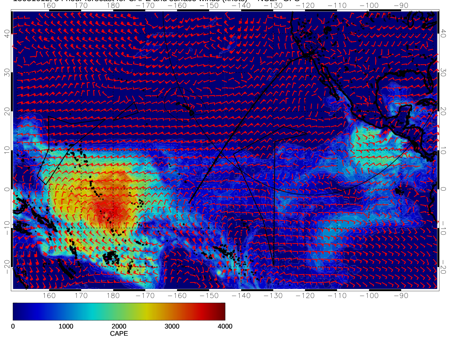
15031612, 84 hour forecast for CAPE and surface winds (knots) -- NCEP GFS
