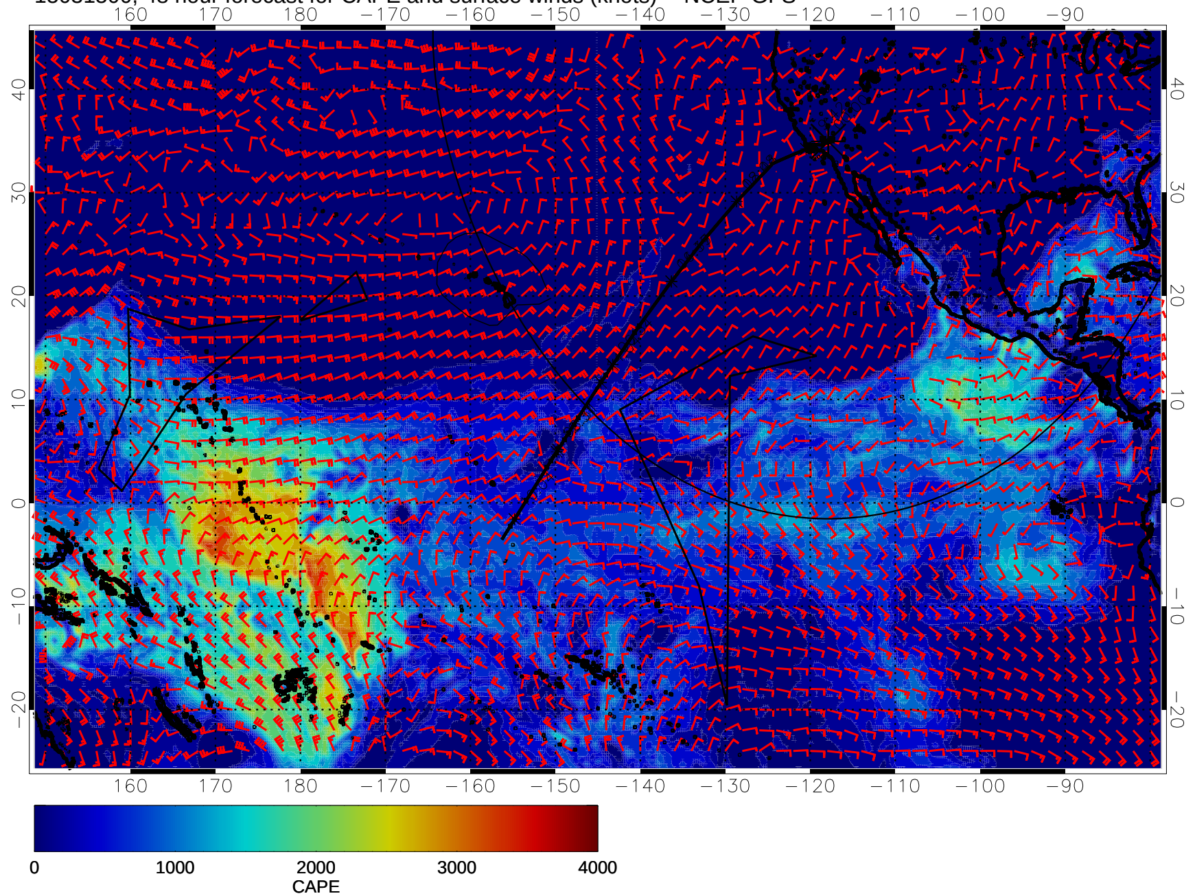
15031500, 48 hour forecast for CAPE and surface winds (knots) -- NCEP GFS
