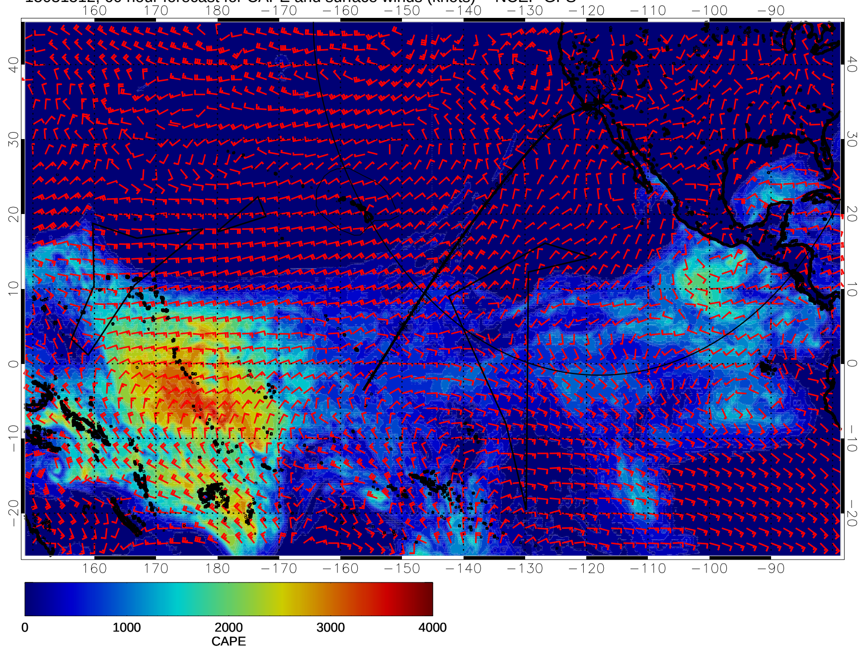
15031512, 60 hour forecast for CAPE and surface winds (knots) -- NCEP GFS
