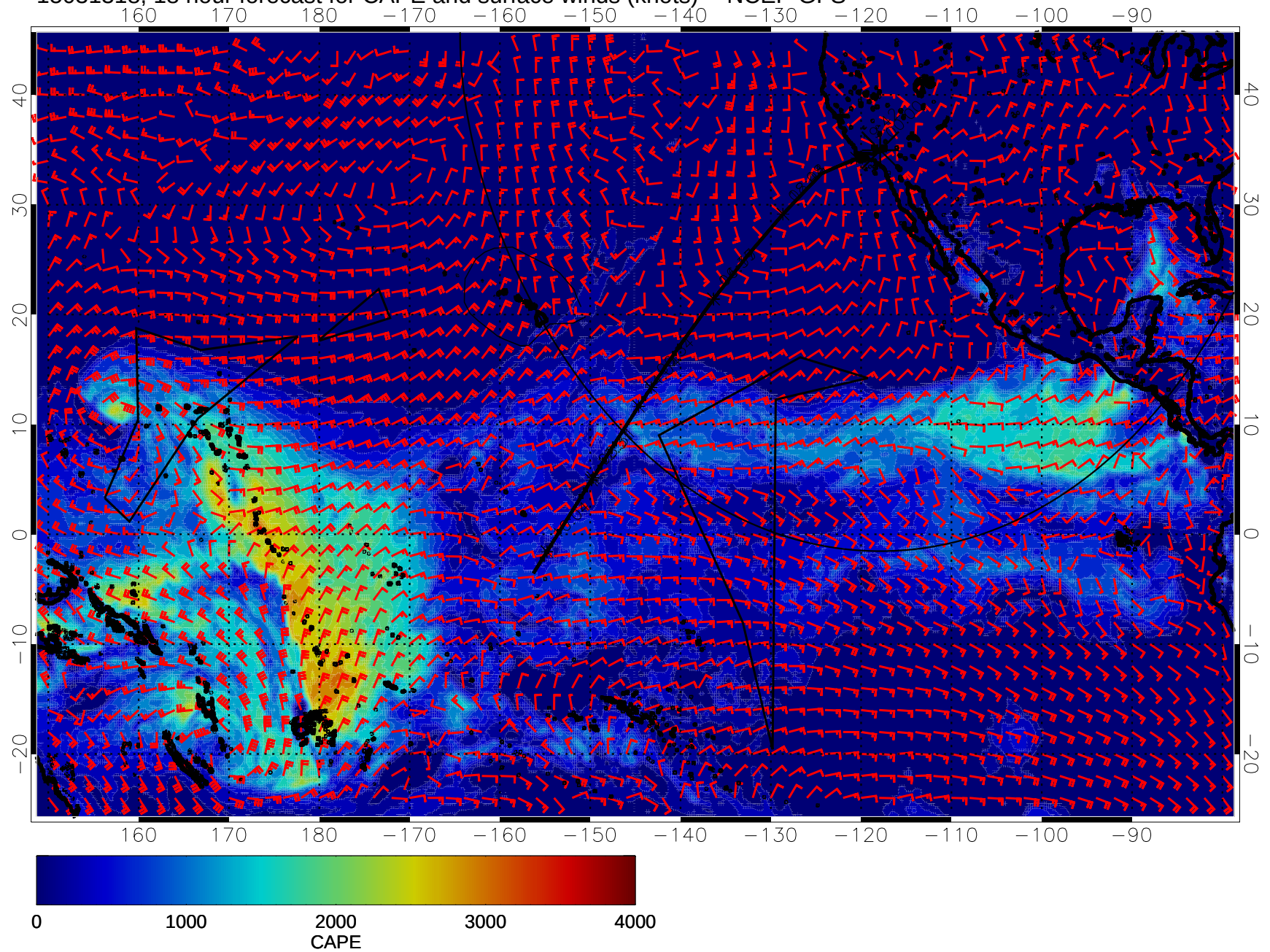
15031318, 18 hour forecast for CAPE and surface winds (knots) -- NCEP GFS
