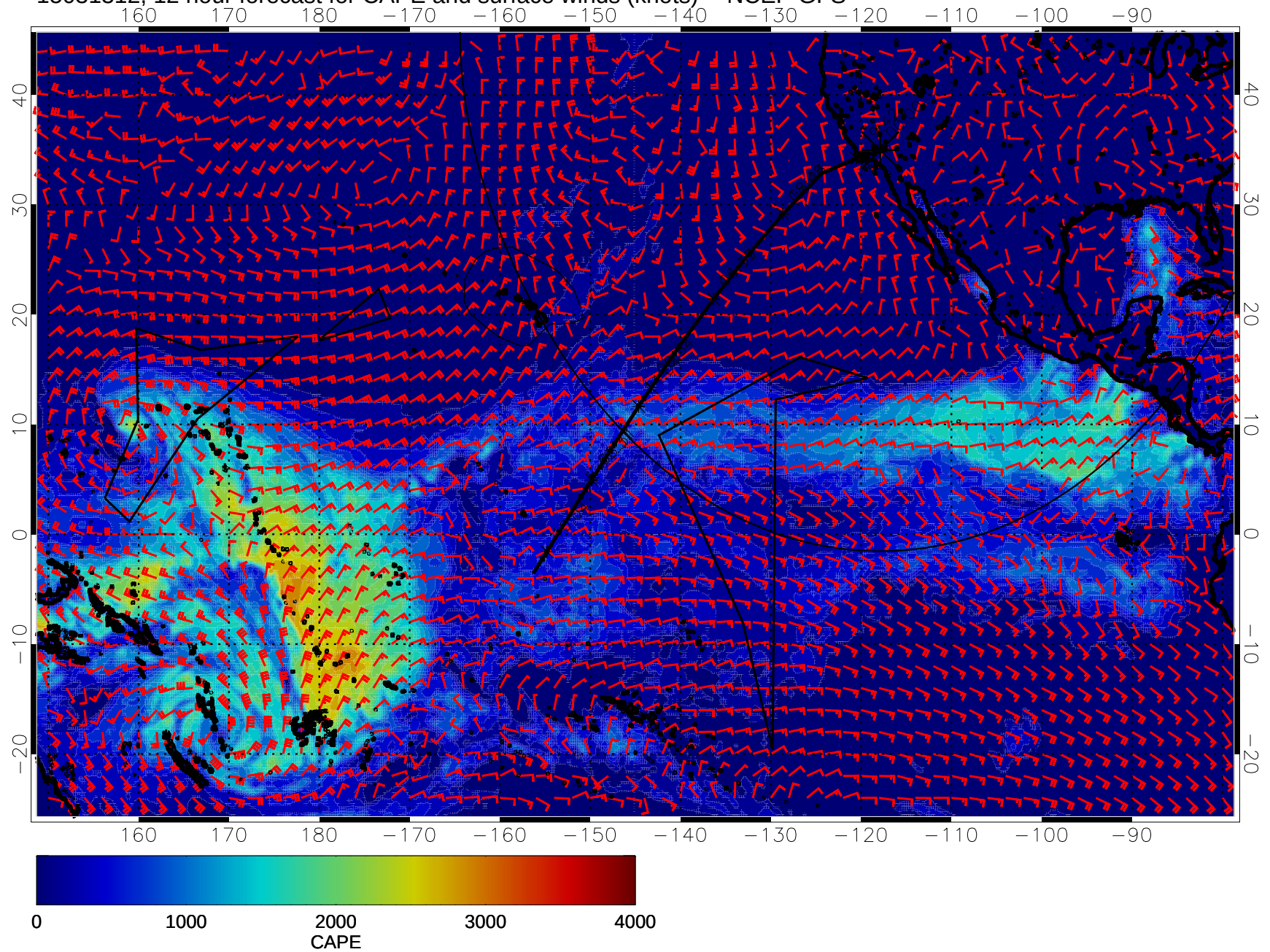
15031312, 12 hour forecast for CAPE and surface winds (knots) -- NCEP GFS
