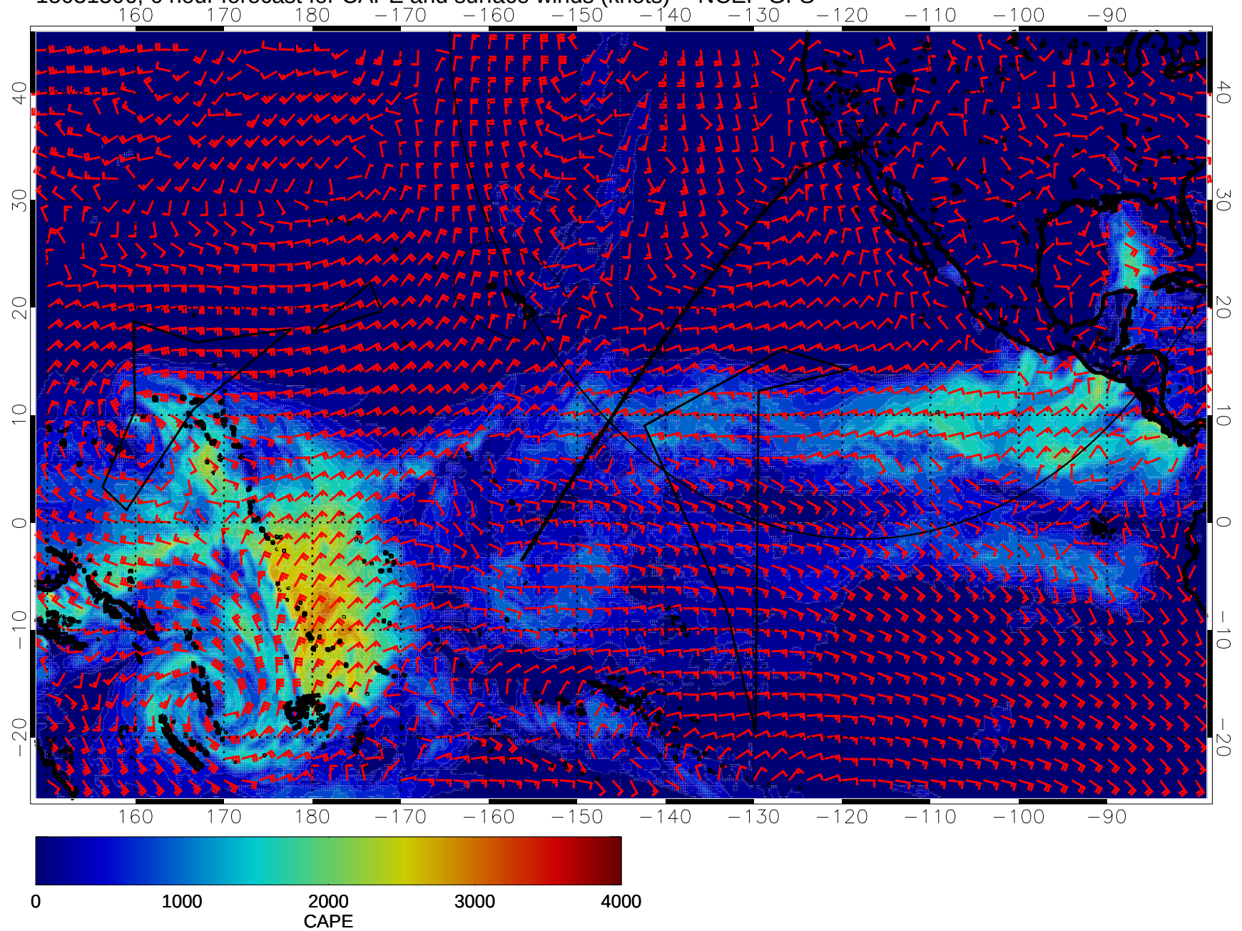
15031306, 6 hour forecast for CAPE and surface winds (knots) -- NCEP GFS
