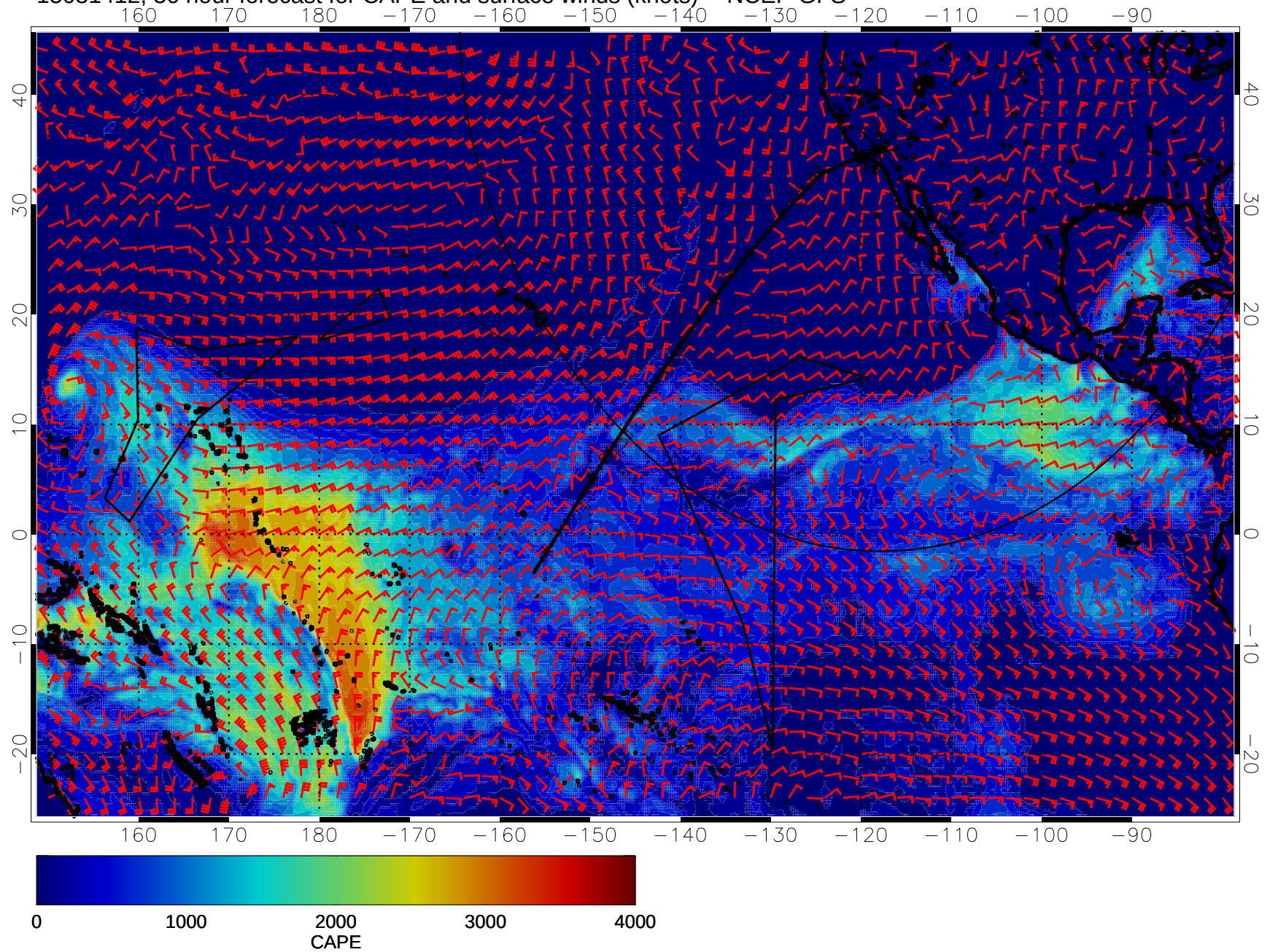
15031412, 36 hour forecast for CAPE and surface winds (knots) -- NCEP GFS
