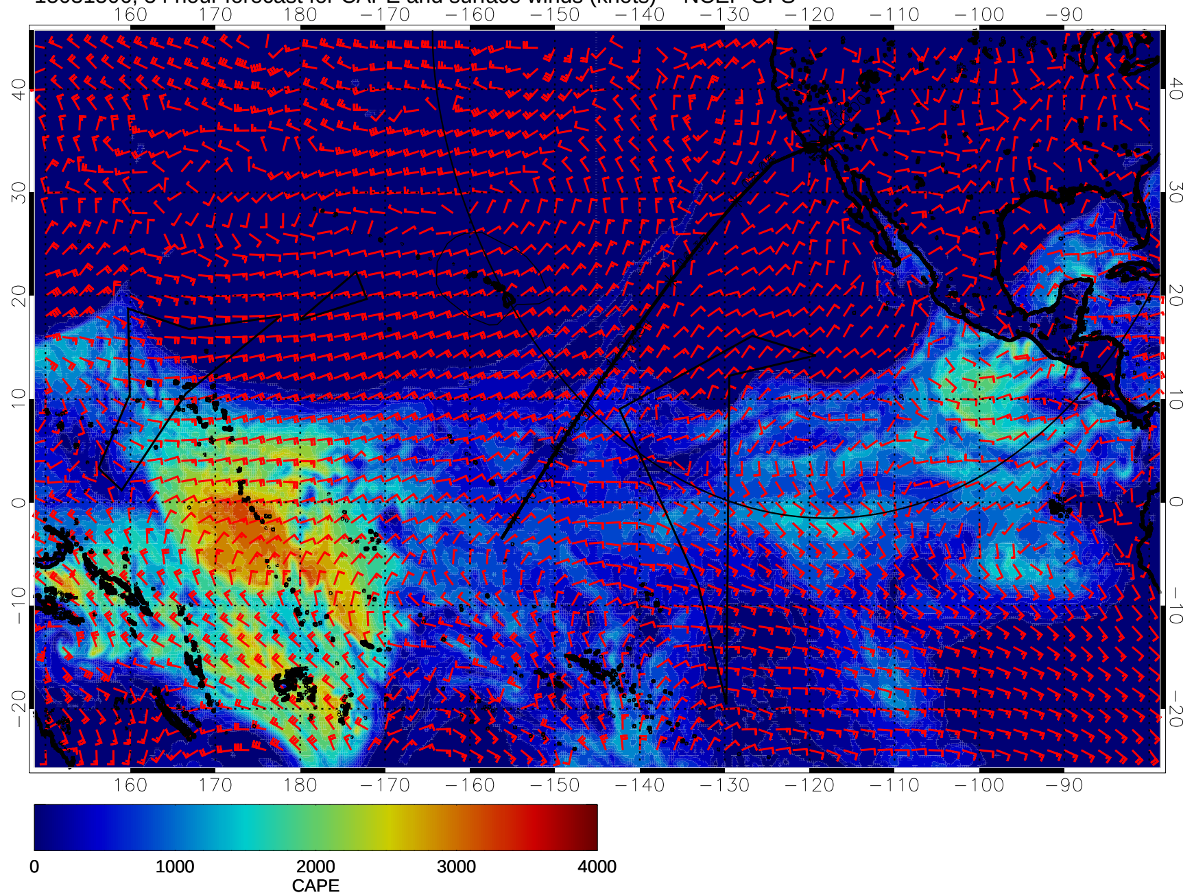
15031506, 54 hour forecast for CAPE and surface winds (knots) -- NCEP GFS
