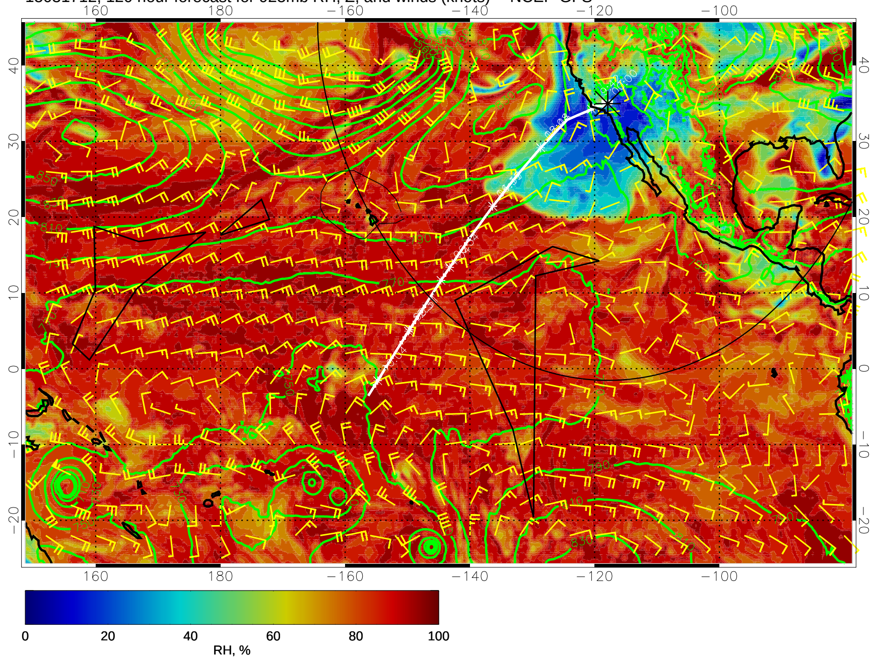
15031712, 120 hour forecast for 925mb RH, Z, and winds (knots) -- NCEP GFS
