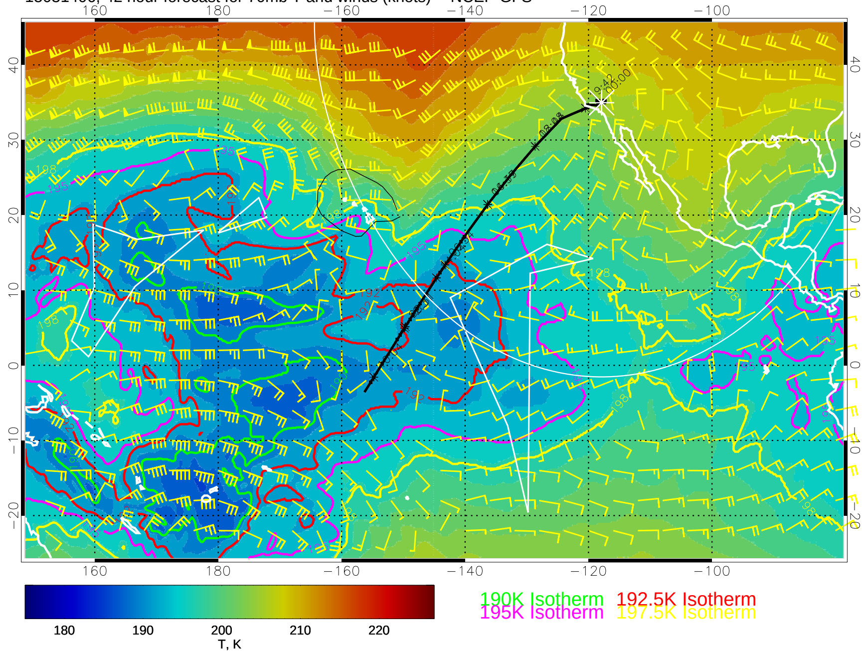
15031406, 42 hour forecast for 70mb T and winds (knots) -- NCEP GFS
