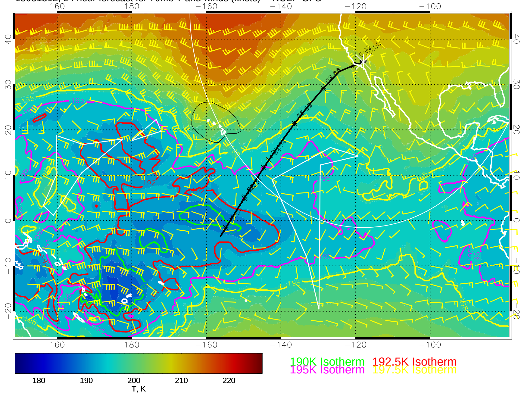
15031312, 24 hour forecast for 70mb T and winds (knots) -- NCEP GFS
