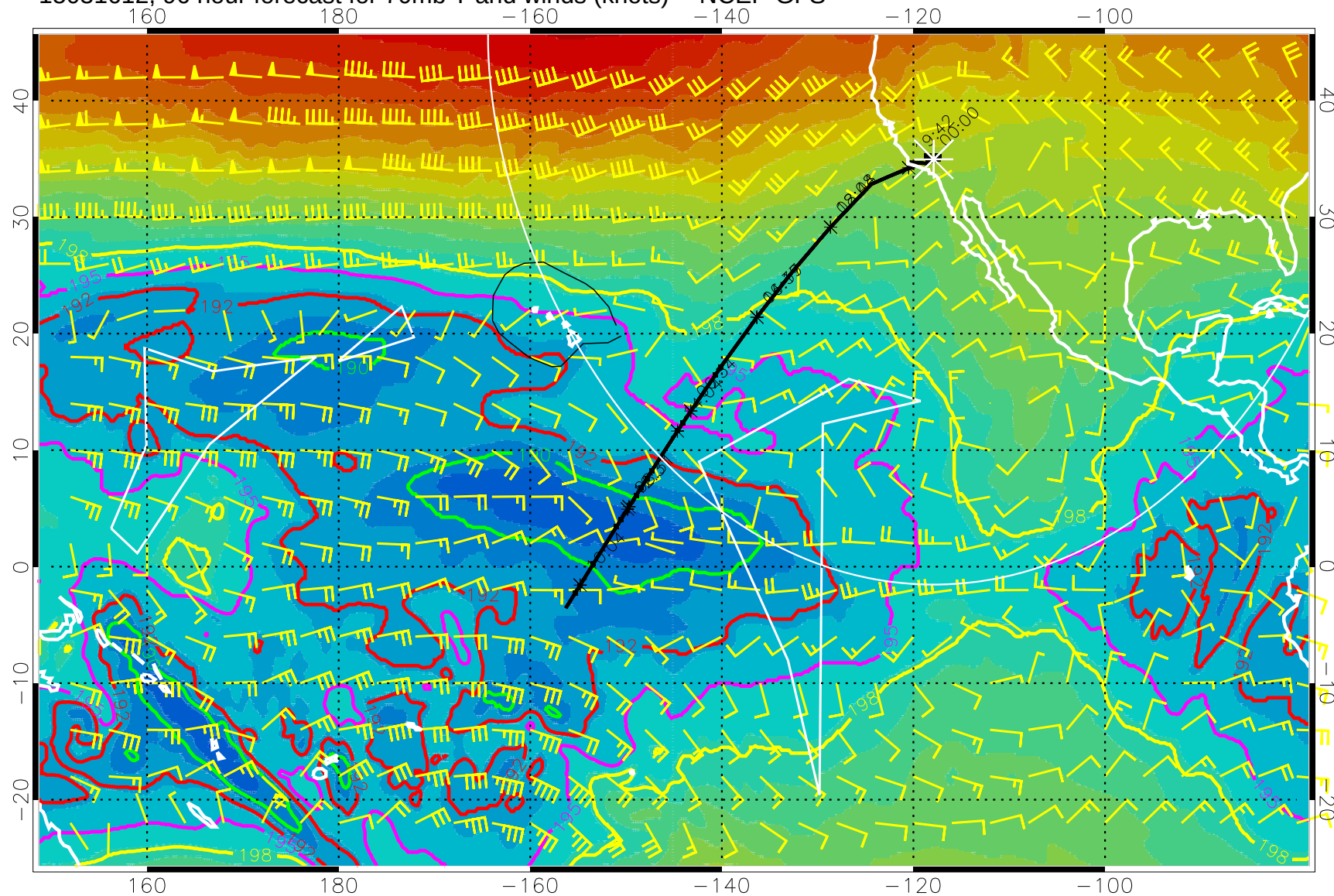
15031612, 96 hour forecast for 70mb T and winds (knots) -- NCEP GFS
