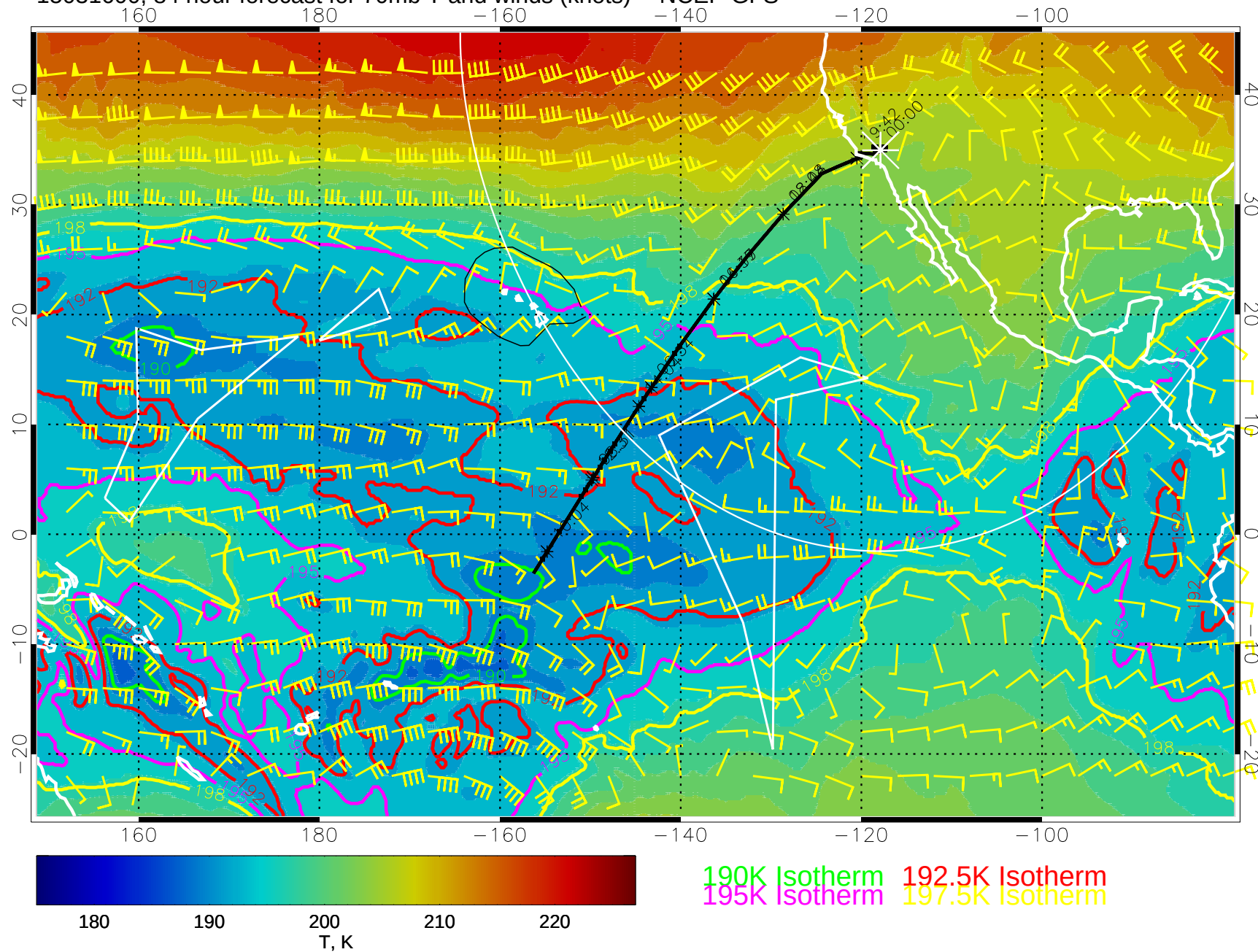
15031600, 84 hour forecast for 70mb T and winds (knots) -- NCEP GFS
