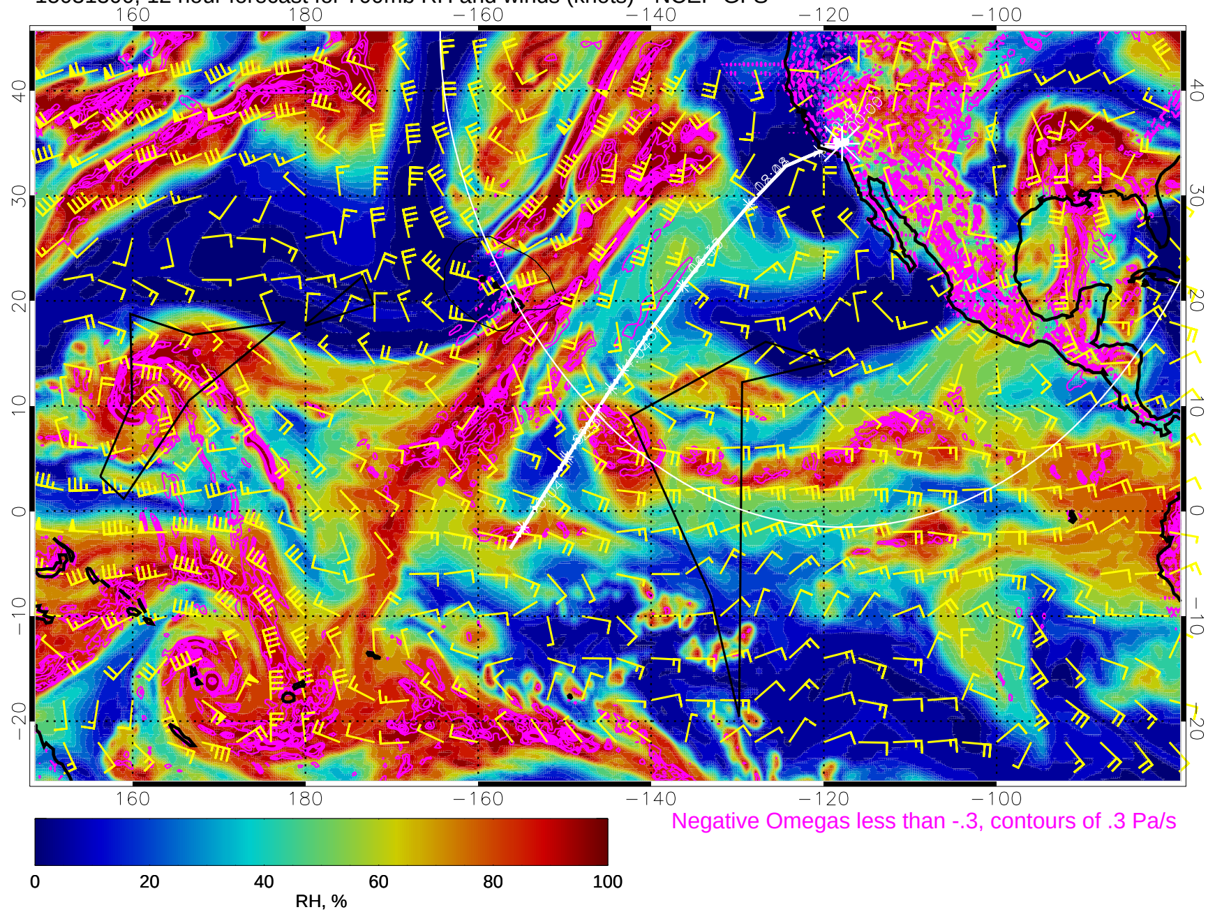
15031300, 12 hour forecast for 700mb RH and winds (knots) - NCEP GFS
