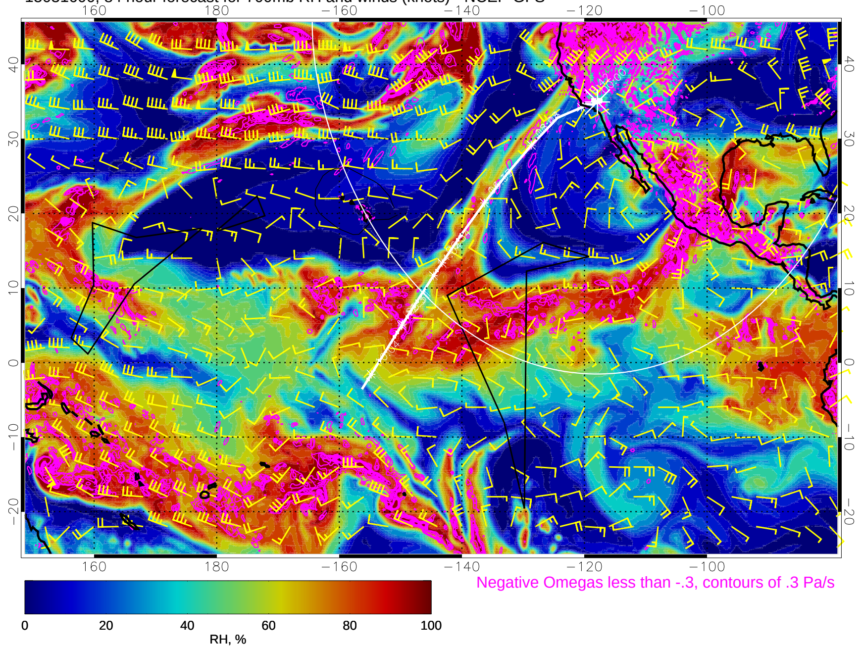
15031600, 84 hour forecast for 700mb RH and winds (knots) - NCEP GFS
