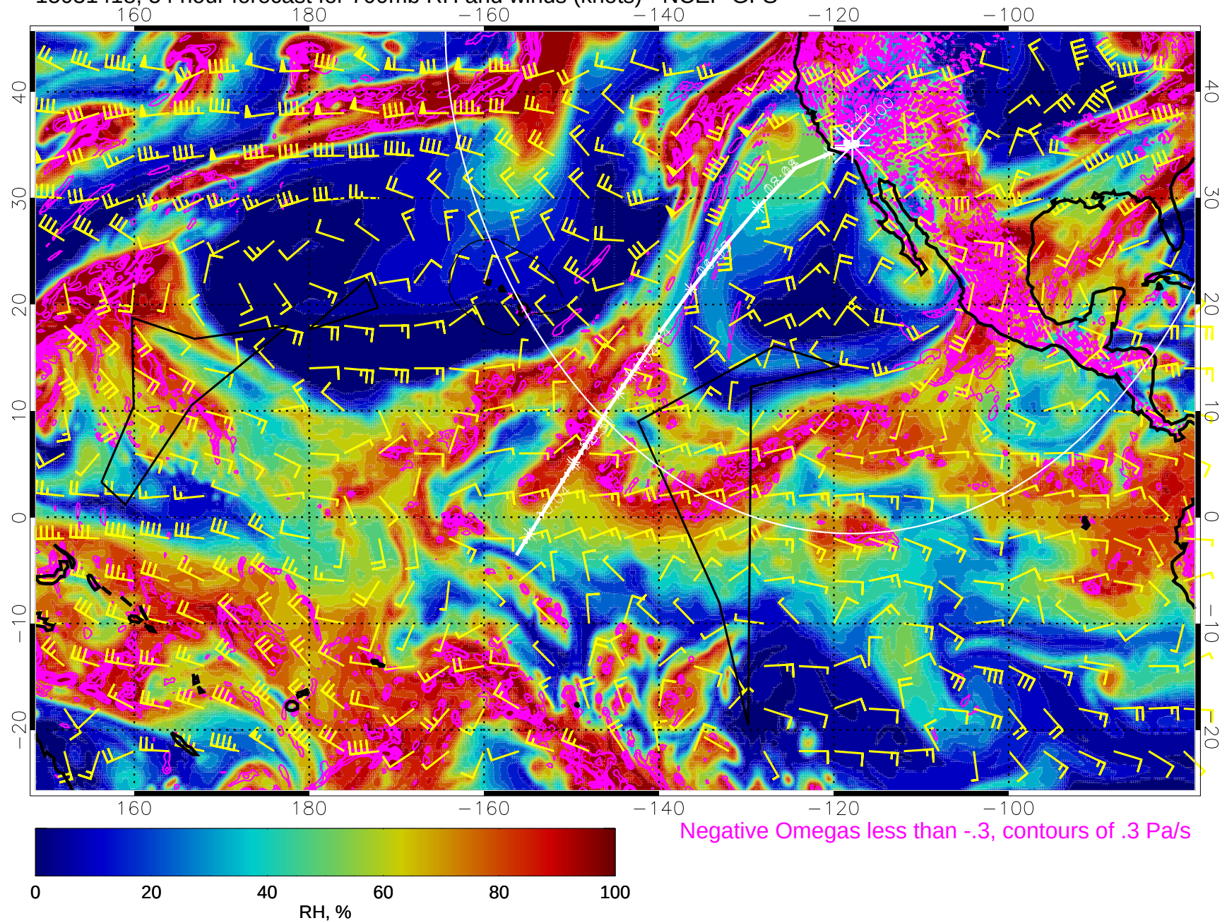
15031418, 54 hour forecast for 700mb RH and winds (knots) - NCEP GFS
