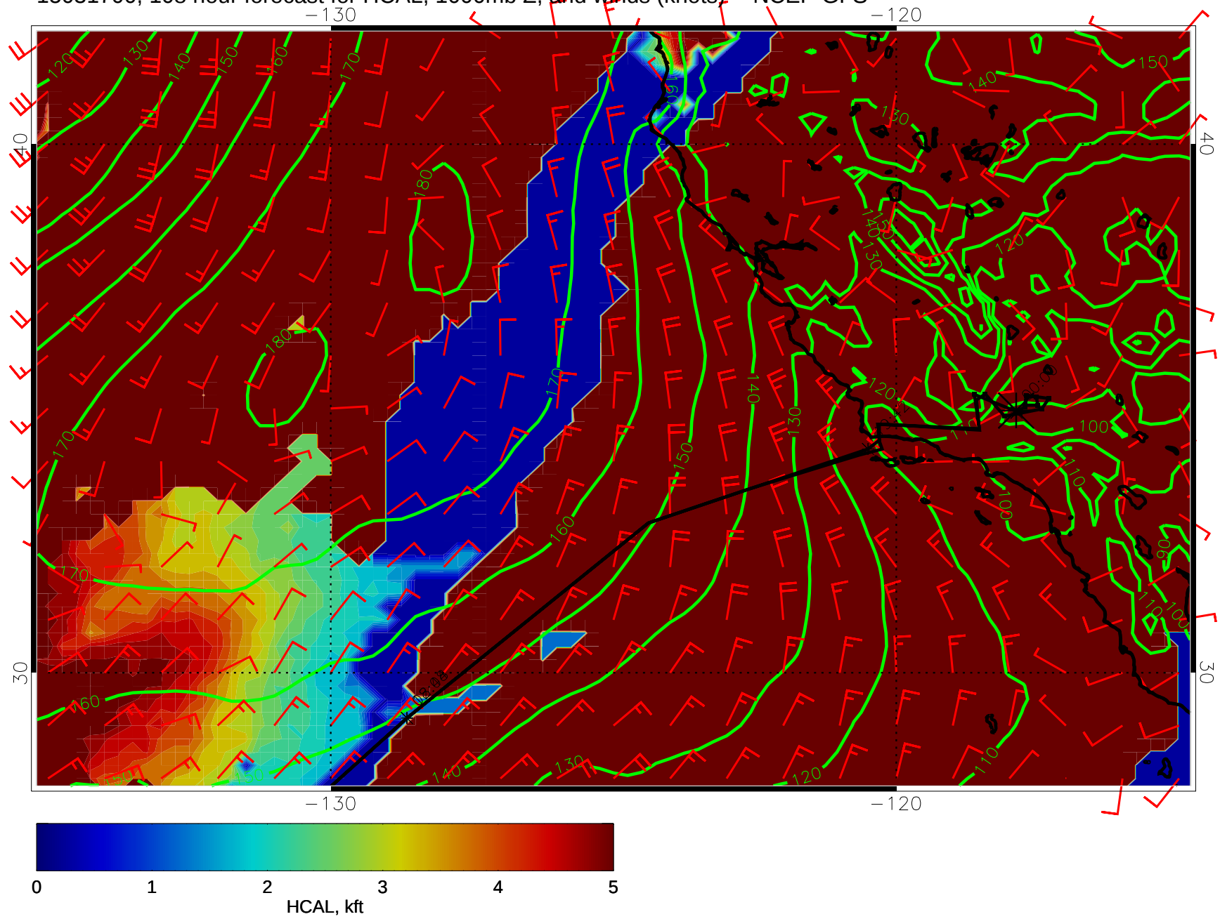
15031700, 108 hour forecast for HCAL, 1000mb Z, and winds (knots) -- NCEP GFS
