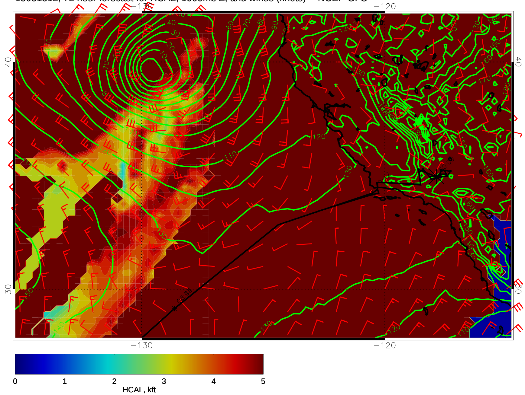
15031512, 72 hour forecast for HCAL, 1000mb Z, and winds (knots) -- NCEP GFS
