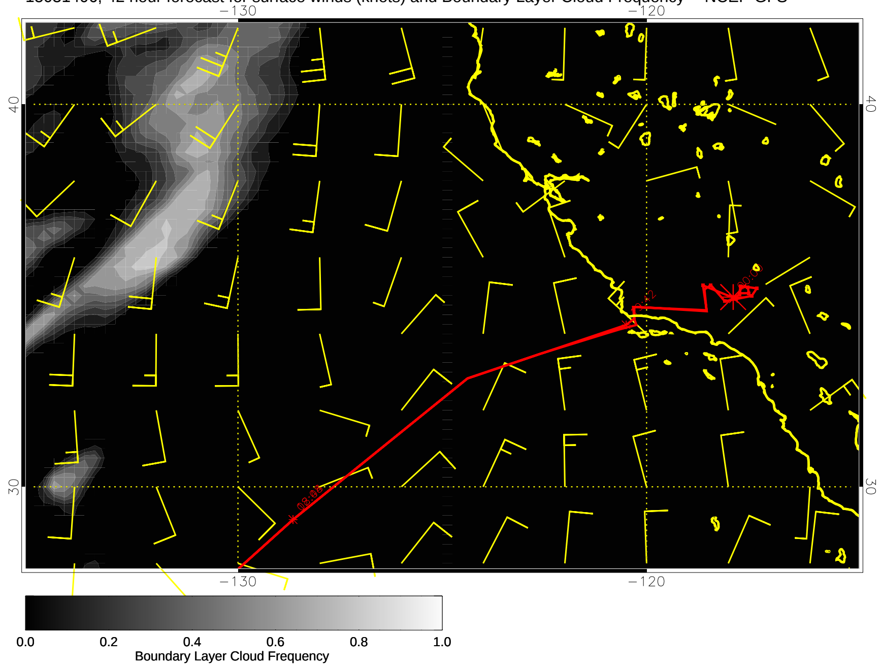
15031406, 42 hour forecast for surface winds (knots) and Boundary Layer Cloud Frequency -- NCEP GFS
