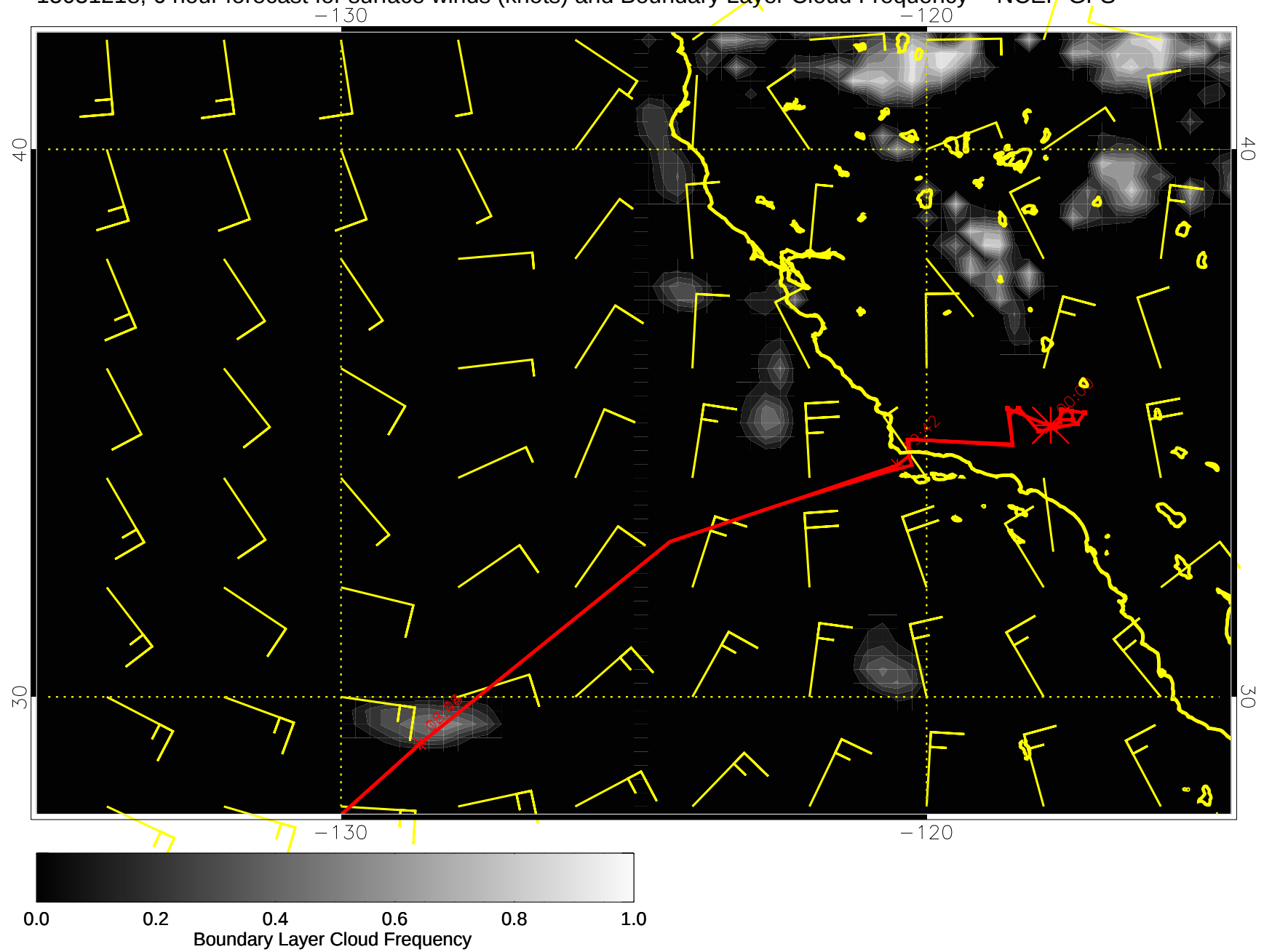
15031218, 6 hour forecast for surface winds (knots) and Boundary Layer Cloud Frequency -- NCEP GFS
