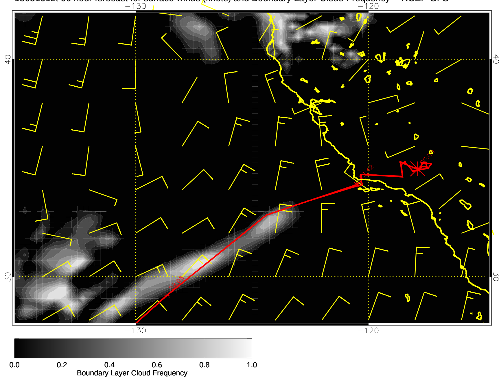
15031612, 96 hour forecast for surface winds (knots) and Boundary Layer Cloud Frequency -- NCEP GFS
