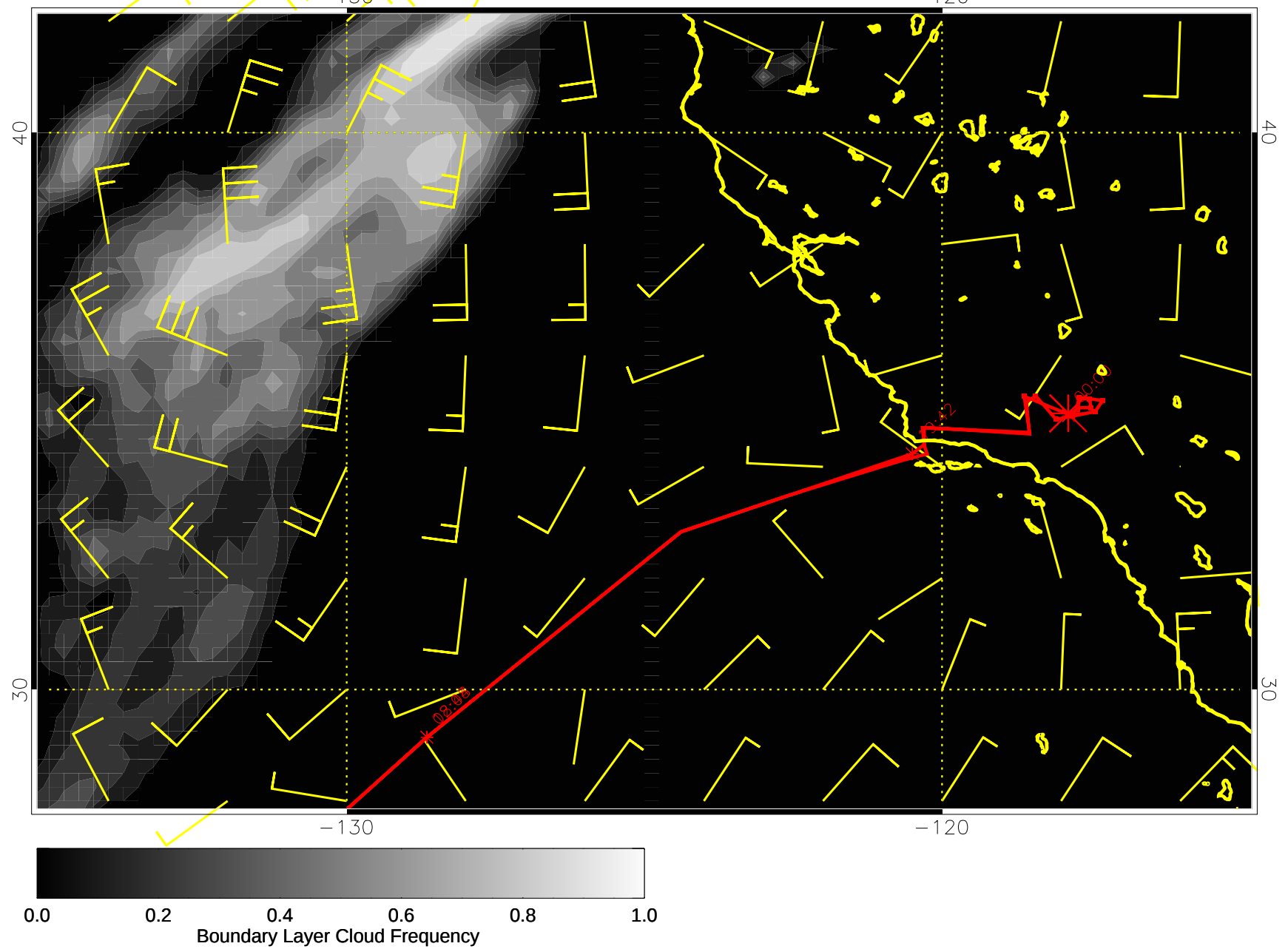
15031506, 66 hour forecast for surface winds (knots) and Boundary Layer Cloud Frequency -- NCEP GFS
