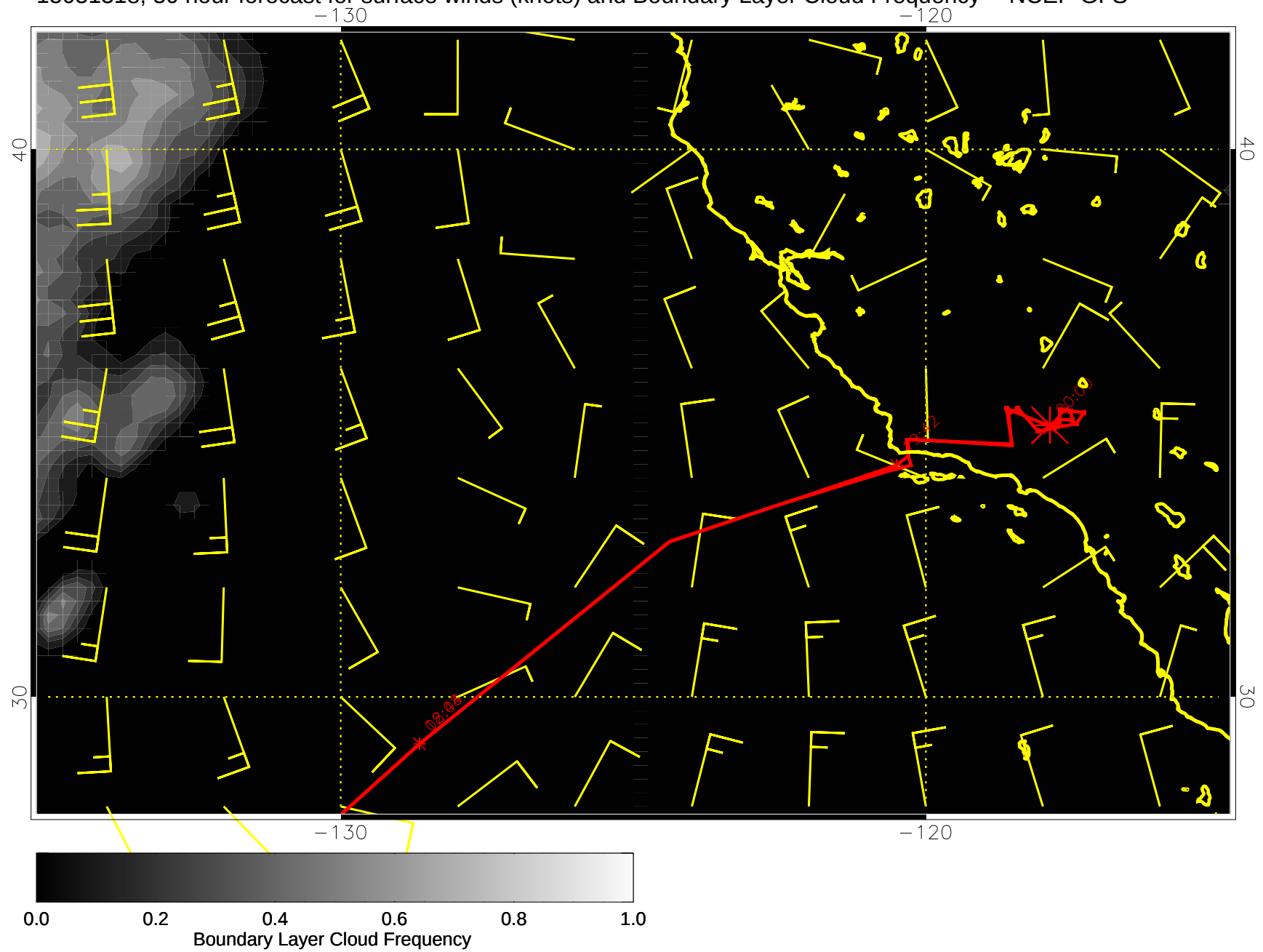
15031318, 30 hour forecast for surface winds (knots) and Boundary Layer Cloud Frequency -- NCEP GFS
